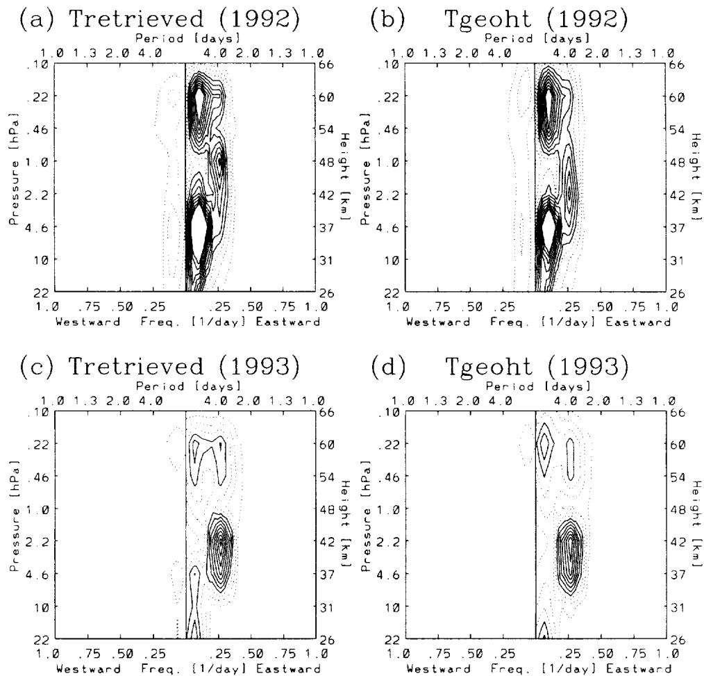
FIG. 1. (a) East-west power spectrum for wave 1 MLS temperature ( T_{\text{retrieved}} ) at 72°S for 18 August–6 September 1992. Dashed contours are at 10, 20, and 30 \text{K}^2 \text{ day} , and solid contours are from 40 to 100 \text{K}^2 \text{ day} by 10 \text{K}^2 \text{ day} . (b) Same as (a) but for temperature derived from MLS geopotential height ( T_{\text{geoht}} ). (c),(d) Same as (a),(b) but for 2–16 September 1993.
