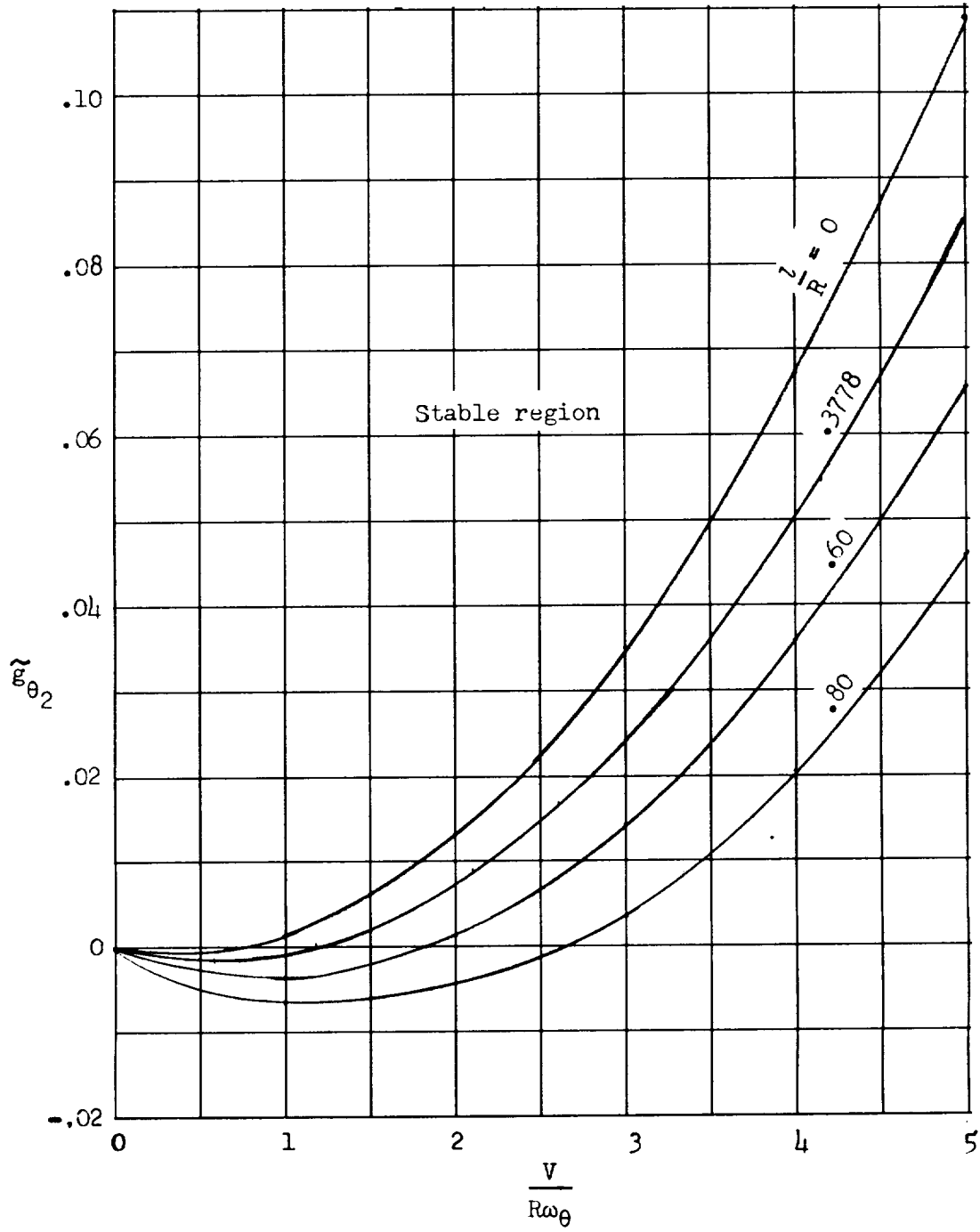
Figure 13.- Effect of pitch-axis location on stability boundary. J = 2.6 ; G = 1.0 ; \gamma = 1.0 .
