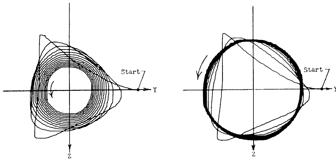
(a) Stable; g_{\theta} = 0.08 .
