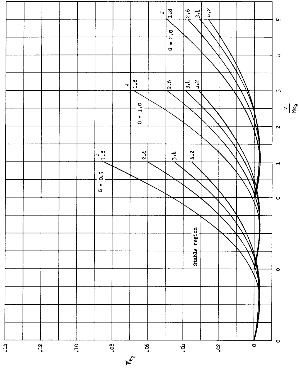
(c) S_{\Psi}/S_{\theta} = 1.96 .
