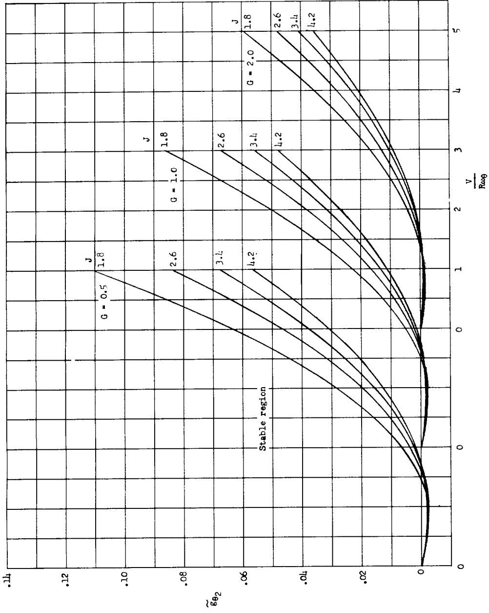
(b) S_{\psi}/S_{\theta} = 1.44 .
