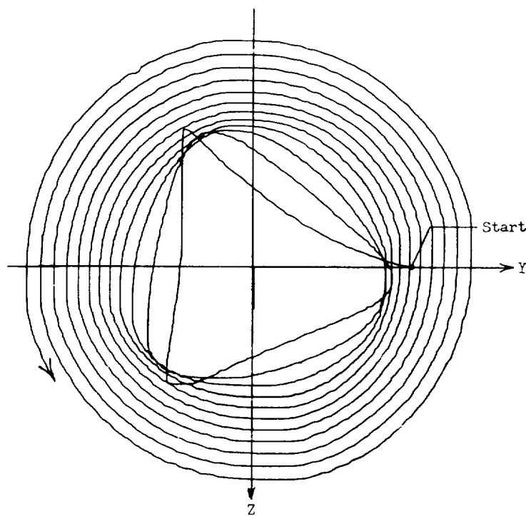
(a) Stable; g_{\theta} = 0.08 .
