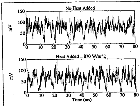
Figure 6.10- Unsteady hot-wire traces from the centreline of the wake-induced wedge with and without heat added.
