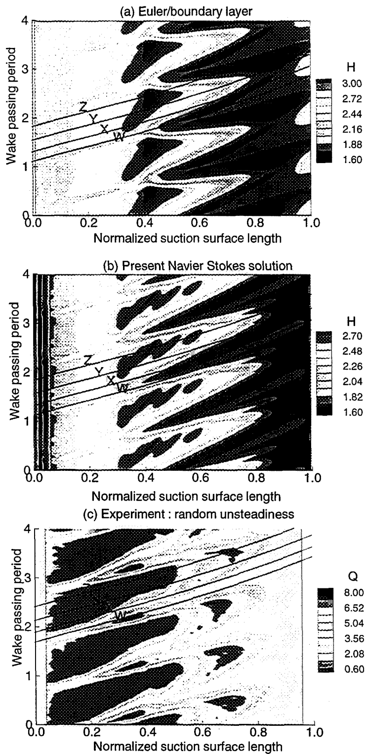
Fig. 7 Predicted distribution of instantaneous shape factor from unsteady NS and Boundary layer codes. The experimental data is random unsteadiness in skin friction coefficient in percent
