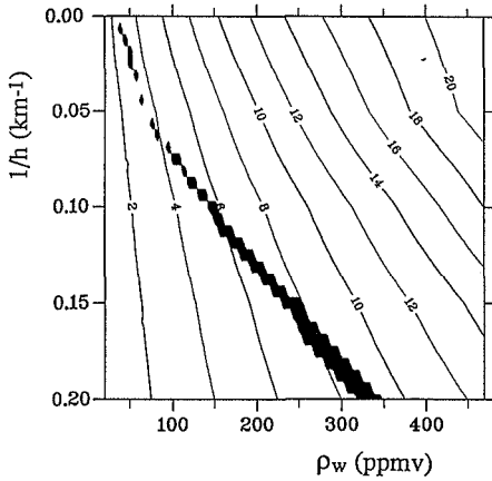
Figure 9. Intersection of domains obtained separately for O 2 and H 2 .
