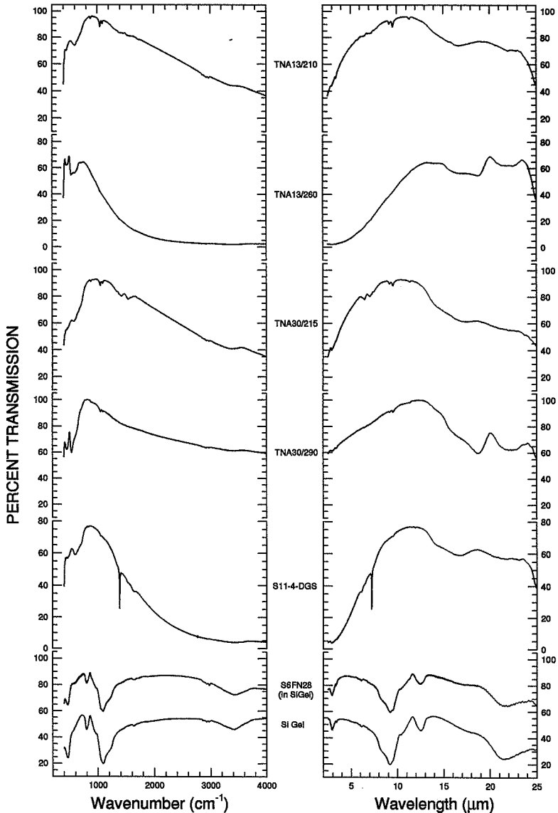
Figure 3. Transmission spectra of well-characterized nanophase ferric materials. The TNA series nanophase iron oxide samples were produced in the lab by oxidation in air of trinuclear acetato hydroxy iron(III) nitrate [Morris et al. , 1991], the S11-4-DGS synthetic ferrihydrite sample was prepared by D.G. Schulze, and the S6FN28 nanophase iron oxide sample was produced in the lab by calcining silica gel impregnated with ferric nitrate solutions in air at 550°C [Morris et al. , 1989]. The transmission spectrum of S6FN28 is shown along with a spectrum of the silica gel material alone that has been offset by 30% relative to S6FN28. Data are in frequency on the left and wavelength on the right.
