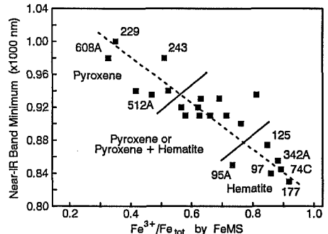
Figure 6. Position of near-IR band minimum as a function of Fe^{3+}/Fe_{tot} .
