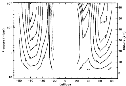
Figure 2b. Zonal-mean zonal winds, in m/s, calculated from the geostrophic thermal wind equation. Positive values represent eastward winds, negative contours are dashed, the zero contour is thicker, and the contour interval is nonuniform.
