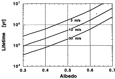
Figure 6. Lifetime of a lake initially 1 km deep in Chryse basin for wind speeds of 3, 10, and 30 m s -1 .
