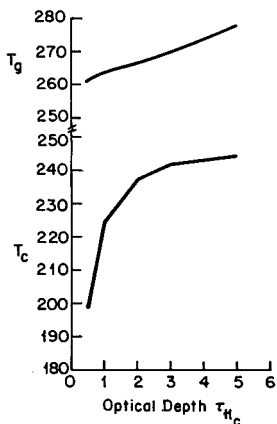
Figure 6: Dust storm interior model. Ground temperature (upper curve) and cloud temperature (lower curve) are plotted as functions of the 11- \mu\text{m} dust cloud optical depth. The dust storm top is fixed at 4 km, and the 11- \mu\text{m} optical depth above 4 km is set to 0.4. T_{4\text{ km}} is set to 220 K and T_{24\text{ km}} = 200 K.
