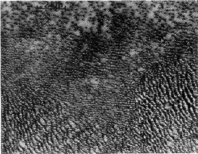
Figure 3b. Enlargement of the central area of Figure 3a, showing the elongation of barchan horns into seifs.
