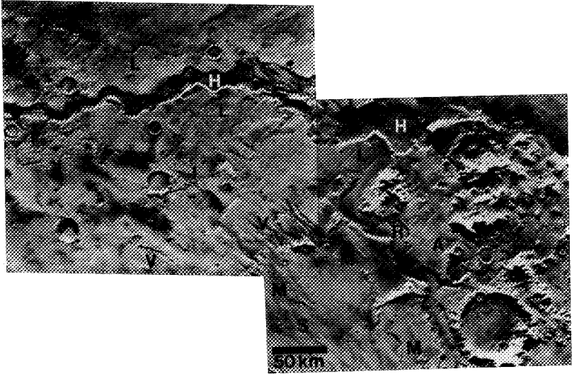
Figure 17. Harmakhis Vallis (H) and lower extremity of Reull Vallis (R) on eastern rim of Hellas. Rim material locally is dissected by degraded-appearing valleys (V) that emerge from smooth plateau deposits (S). These deposits in turn are capped in places by etched appearing mesas (M). Smooth, lobate, channeled material (L) may be deposit of Reull Vallis; note how deposit surrounds and channels cut inliers of rim material (I). Note debris aprons (A) along walls of valles and bases of massifs and layering in south wall of Reull Vallis (arrows). (Viking images 329S25 and 26; centered at \sim 40.00^{\circ}\text{S} , 265.00^{\circ} , 235 m/pixel).
