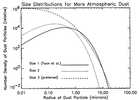
Figure 1b. Dust particle size distributions, based on the modified gamma distribution. All of the model calculations presented employ one of these size distributions, for which the parameters are provided in Table 2. Size distribution 1 corresponds to the Toon et al. model; size distribution 2 exhibits a size distribution width similar to the Toon et al. model, but with roughly one half the average particle sizes. Size distribution 3 exhibits a very broad size distribution width, and is found to obtain a dust opacity variation between visible and 30- \mu\text{m} wavelengths most appropriate to the observed variation.
