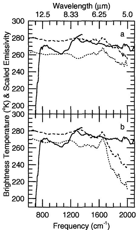
Figure 7. Comparison of Mariner 7 spectrum of Mars, 12° latitude, 3.6° longitude (solid line), to 91-1 (dotted line), scaled to 270°K, and PH-1 (dashed line) scaled to 280°K, for both (a) coarse and (b) fine grain size samples.
