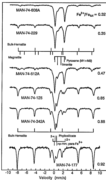
Figure 1. Mössbauer spectra for Manicouagan impact melt rocks having lowest and highest values of \text{Fe}^{3+}/\text{Fe}_{\text{tot}} .
