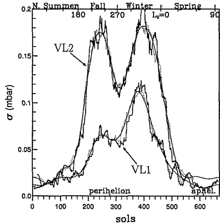
Figure 4. Seasonal evolution of the amplitude of the transient pressure oscillations at both Viking sites computed as the running quadratic mean over 25 (thick solid curve) and 50 (dotted curve) consecutive sols of the difference between the instantaneous (diurnally averaged) Viking pressure and the eight-harmonic fit. The thin solid curve is the eight-harmonic L_S fit to the dotted curve.
