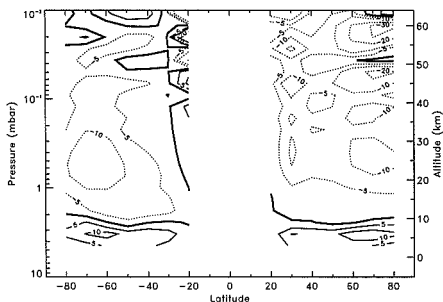
Figure 5. Eliassen-Palm flux divergence ( (\rho a \cos \phi)^{-1} \nabla \cdot \mathcal{F} ) in units of \text{ms}^{-1}/\text{d} . Negative contours are dashed, the zero contour is thicker, and the contour interval is nonuniform.
