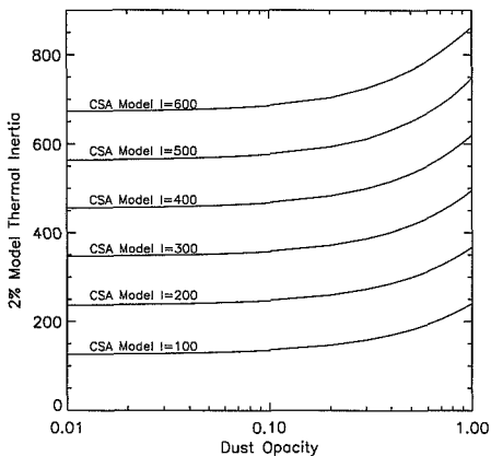
Figure 2. Contours of constant CSA model thermal inertias plotted on dust opacity versus 2% model thermal inertia.
