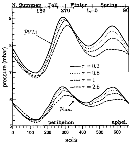
Figure 24. Simulated Viking 1 pressure and planetary averaged surface pressure p_{\text{atm}} for the dust sensitivity experiments ( \tau = 0.2, 0.5, 1 , and 2.5 ).
