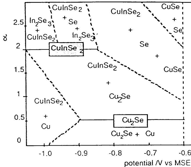
Figure 2. Qualitative phase diagram of electrochemically deposited compounds in the Cu-In-Se system.
