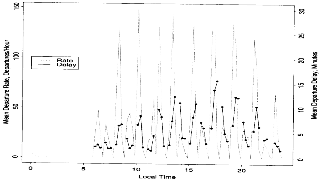
Figure 2-1. Mean Departure Rate and Mean Delay in June 1995 for The William B. Hartsfield Atlanta International Airport
