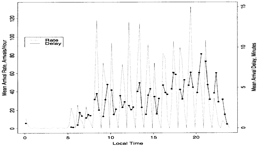
Figure 2-11. Mean Arrival Rate and Mean Delay in June 1993 for Newark International Airport
