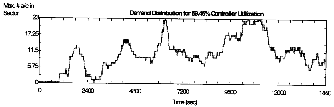
Figure 3-12. Demand Distribution for Utilization 59.46 percent
