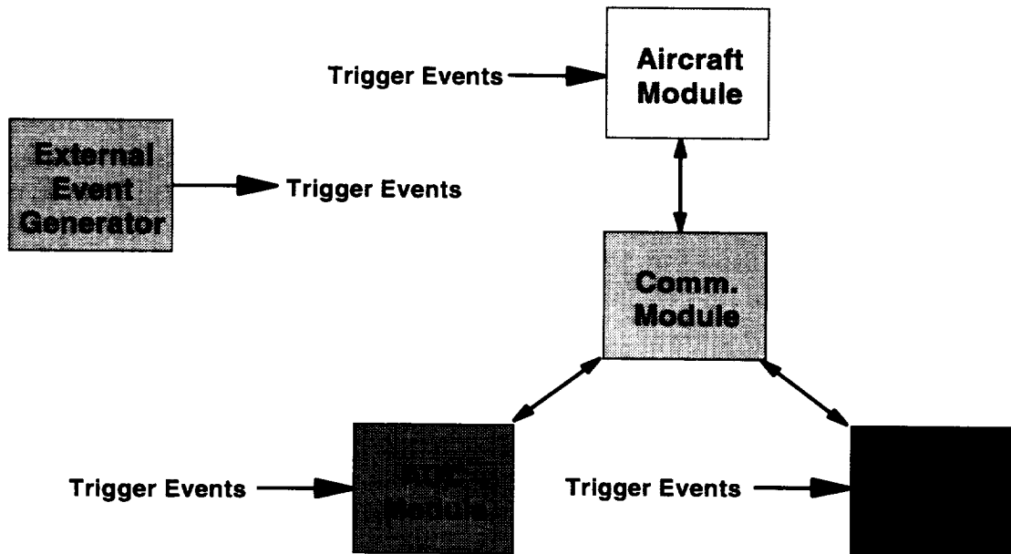
Figure 3-6. FAM Architecture
