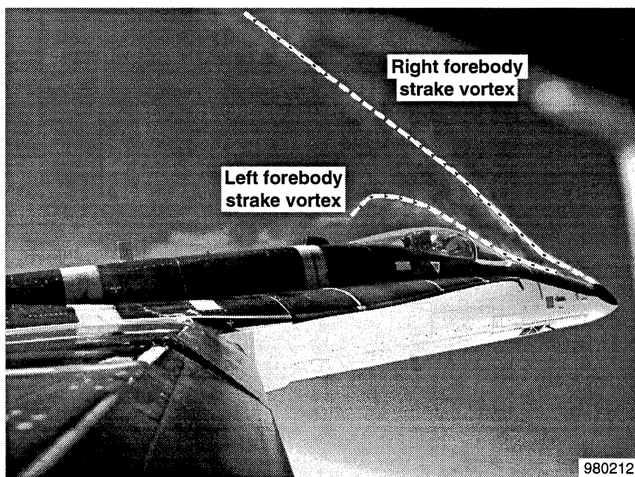
Figure 9. Forebody/strake vortex flow visualization for \alpha = 50^\circ , \delta_{s, d} \approx 30^\circ , and \delta_{s, L/R} = 5^\circ/35^\circ .
