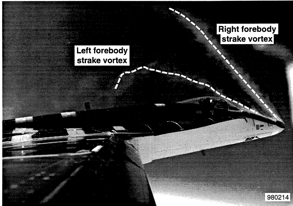
Figure 11. Forebody/strake vortex flow visualization for \alpha = 47.2^\circ , \beta = 3.9^\circ and \delta_s, L/R = 0^\circ/90^\circ .
