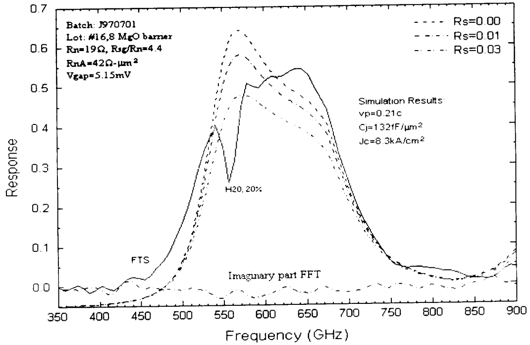
Fig. 4 FTS response of an All NbTiN junction with MgO barrier.
