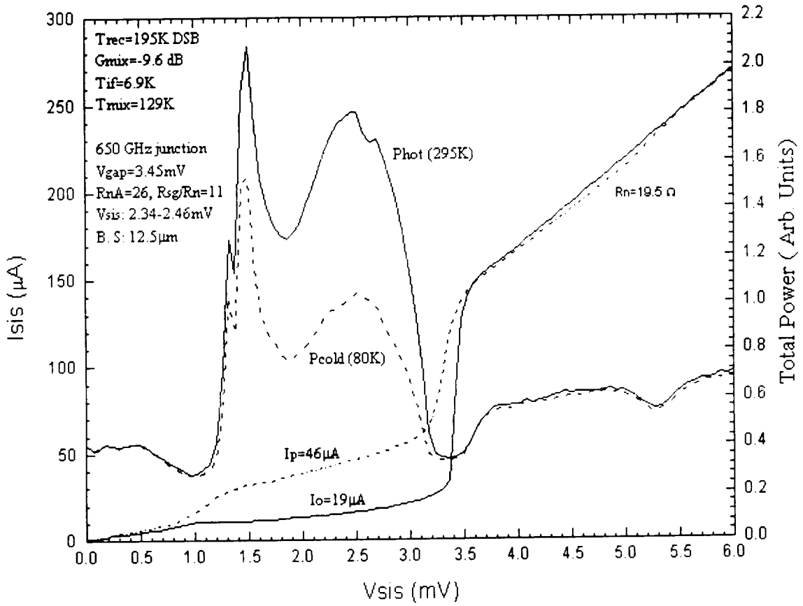
Fig 9 Heterodyne response of an Al-N x barrier junction at 588 GHz.
