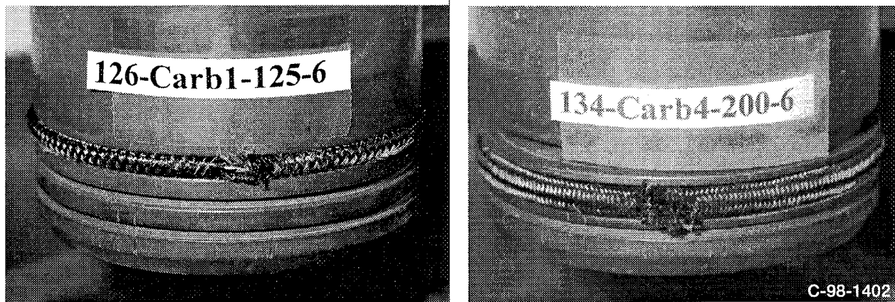
Figure 8.—Photos of carbon seals after 900 °F flow/scrubbing tests. (a) Carbon-1 (1/8 in. diameter). (b) Carbon-4 (0.20 in. diameter).
