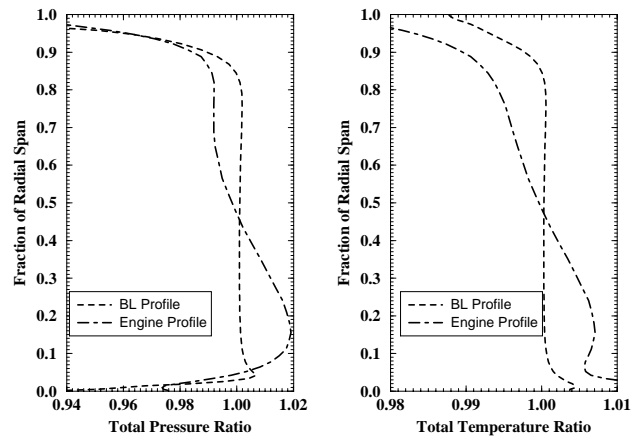
Fig. 11 Comparison of spanwise variation of inflow total pressure and total temperature ratio profiles for profiles for the EEE LP turbine analyses with variations in inlet profile.
