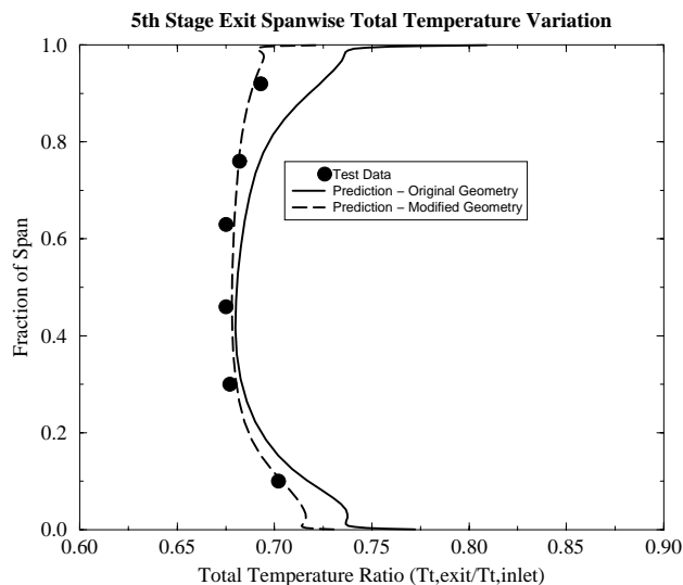
Fig. 10 Comparison of predicted and experimental spanwise variation in fifth stage exit total temperature distributions for EEE LP turbine analyses with variations in first vane reset and endwall modeling.
