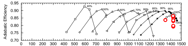
Fig. 7 Comparison of predicted and experimental total pressure ratio and adiabatic efficiency versus corrected flow rate for the core inlet of the EEE fan section.
