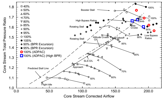
Fig. 7 Comparison of predicted and experimental total pressure ratio and adiabatic efficiency versus corrected flow rate for the core inlet of the EEE fan section.
