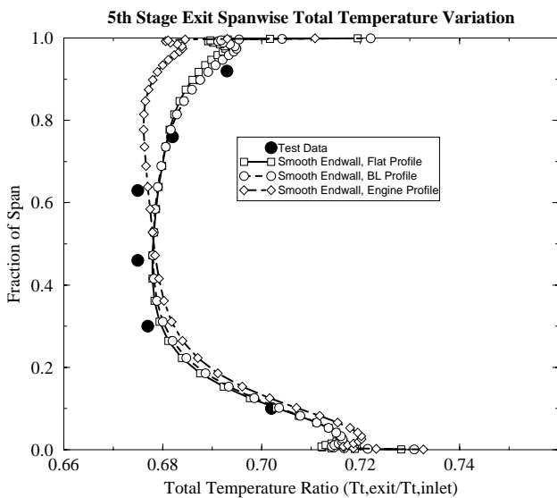
Fig. 12 Comparison of predicted and experimental spanwise variation in fifth stage exit total temperature distributions for EEE LP turbine analyses with variations in inlet profile.
