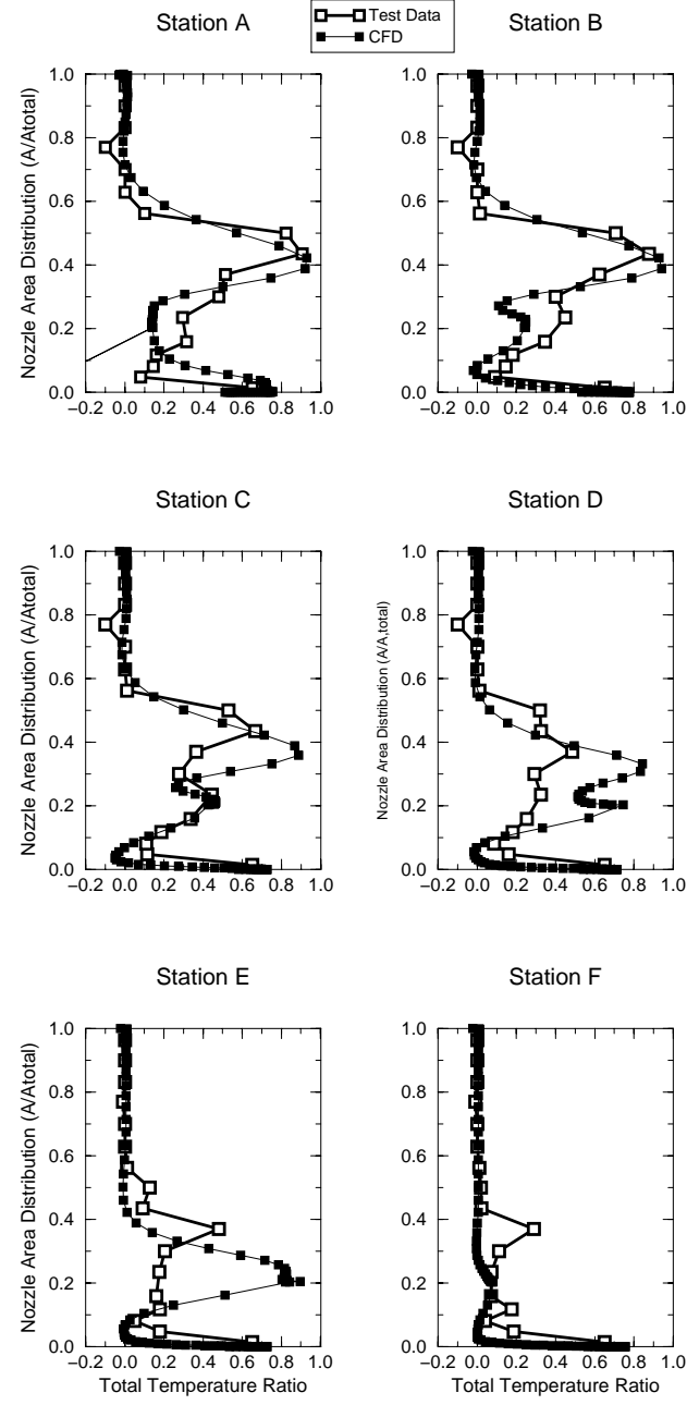
Fig. 19 Comparison of predicted and experimental radial total temperature surveys for the EEE lobed exhaust mixer.
