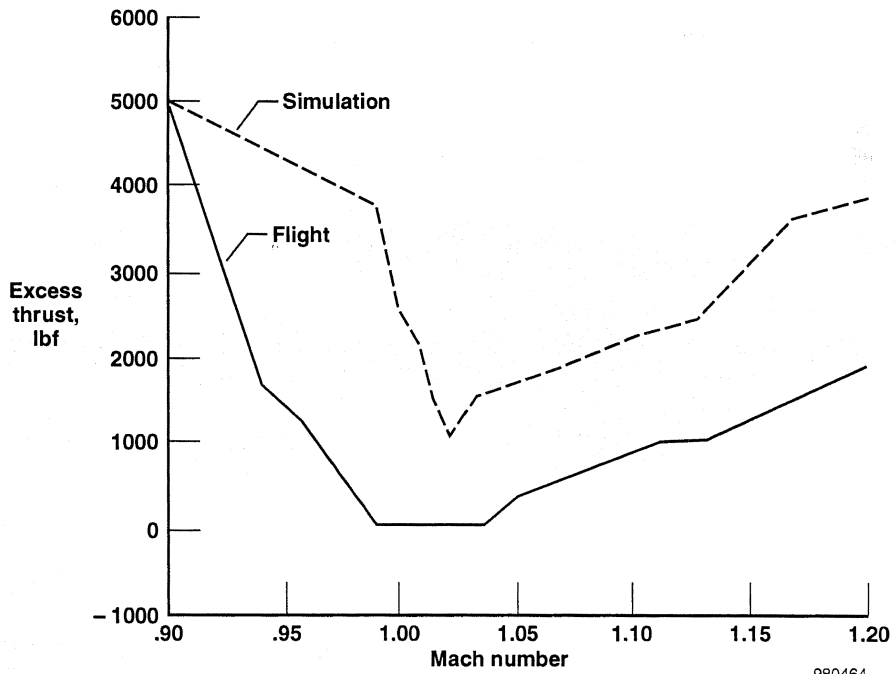
Figure 13. Flight data compared with flight-day temperature simulation data for the LASRE transonic acceleration at an altitude of 27,000 ft.
