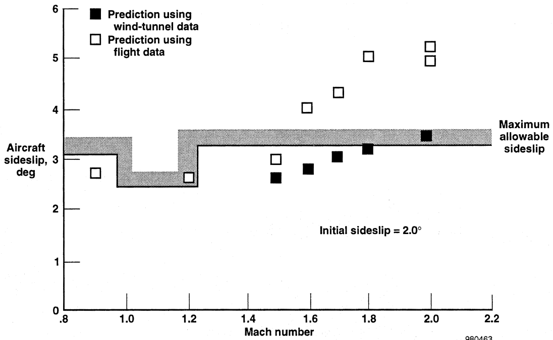
Figure 12. Comparison of wind-tunnel with flight-derived sideslip from an SR-71 engine out (2° initial sideslip).
