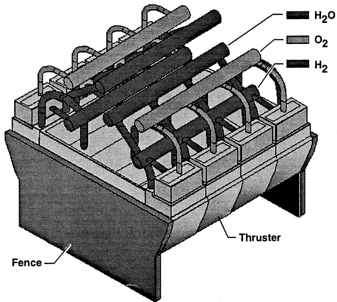
Figure 8. The LASRE aerospike rocket engine.
