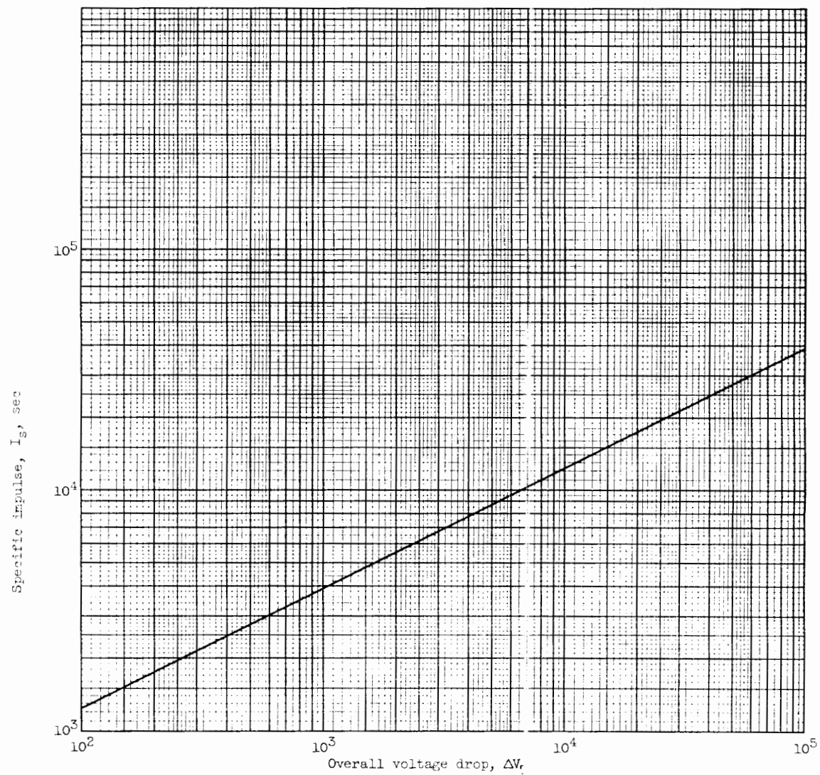
Figure 2. - Graphs for determining ion-rocket-engine performance.
