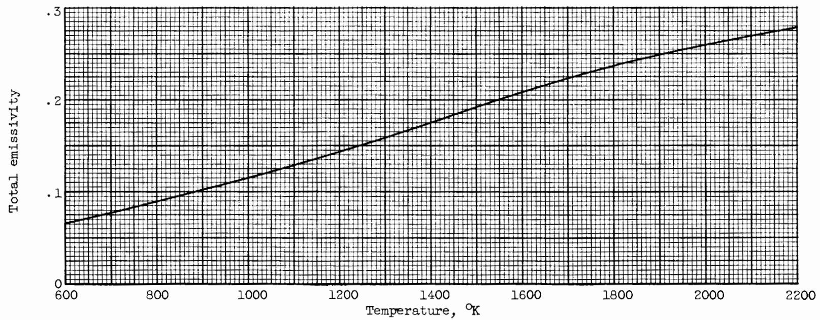
Figure 3. - Emissivity of tungsten (ref. 11).
