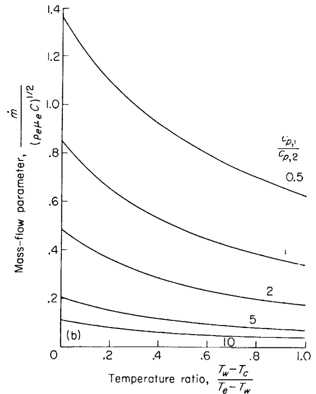
(b) Two-dimensional flow.
