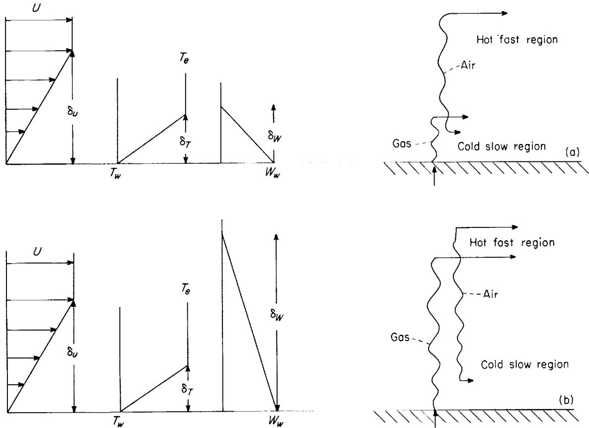
(a) c_{p,2} > c_{p,1} ; maximum shielding when N_{Pr,w} is large and N_{Sc,w} is large. (b) c_{p,1} > c_{p,2} ; maximum shielding when N_{Pr,w} is large and N_{Sc,w} is small.
