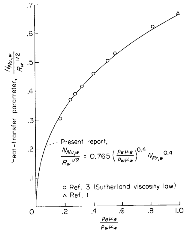
FIGURE 6.—Variation of \frac{Nu_w}{R_w^{1/2}} with \frac{\rho_e \mu_e}{\rho_w \mu_w} . Axisymmetric stagnation point; no injection.
