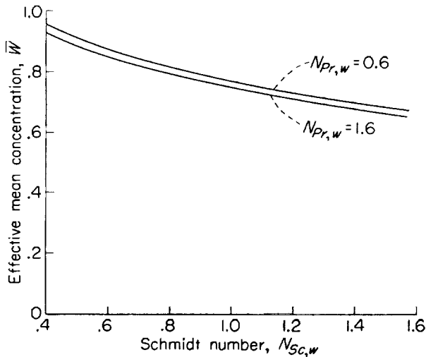
FIGURE 8.—Variation of \bar{W} with N_{Sc,w} . ( \bar{W} is virtually independent of N_{Pr,w} .)
