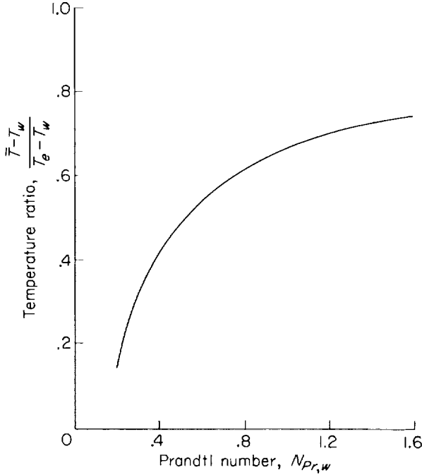
FIGURE 7.—Variation of \frac{\bar{T}-T_w}{T_e-T_w} with N_{Pr,w} .
