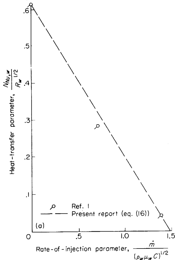
(a) Axisymmetric case. N_{Pr,w} = 0.7 ; \frac{T_w}{T_e} = 0.05 .
