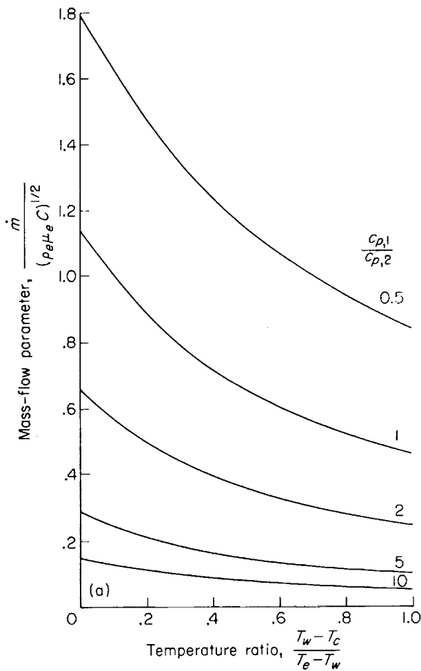
(a) Axisymmetric flow.
