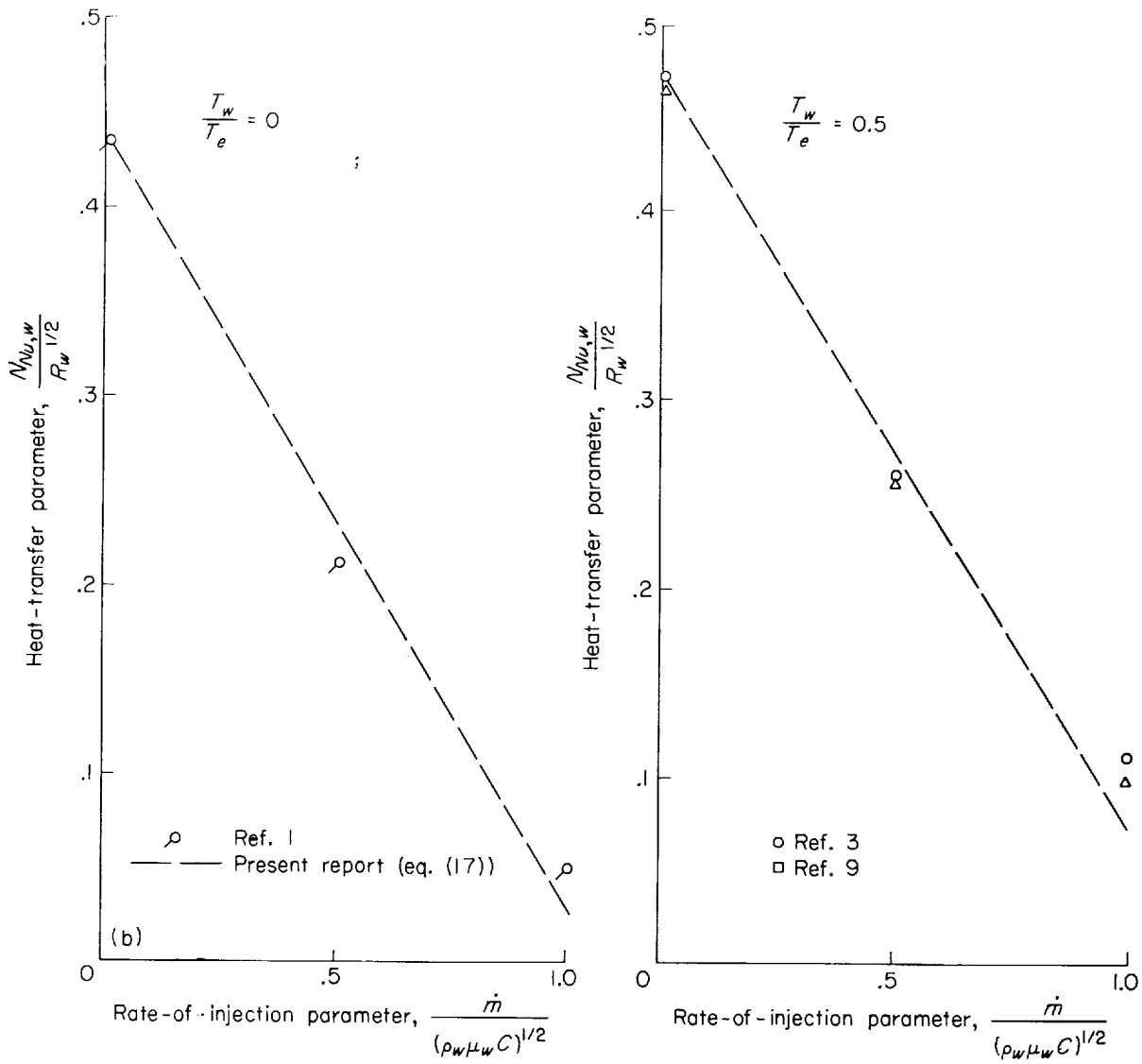
(b) Two-dimensional case. N_{Pr,w} = 0.7 .
