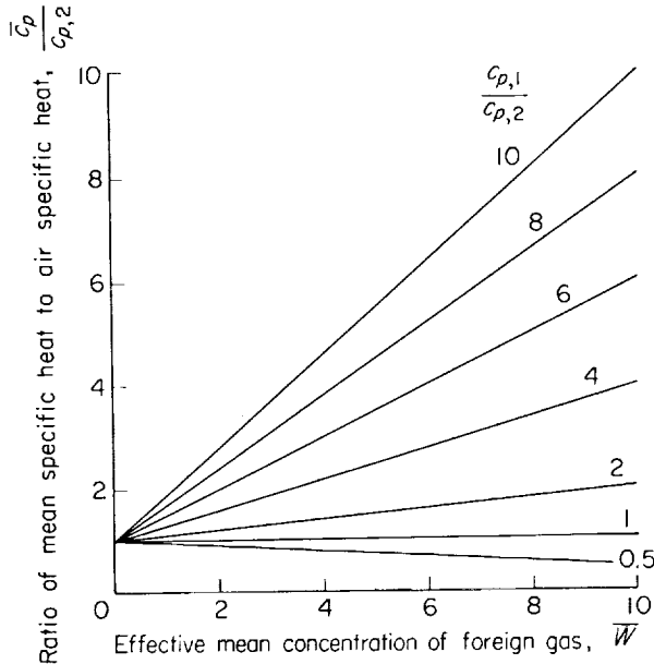
FIGURE 10.—Variation of \frac{\bar{c}_p}{c_{p,2}} with \bar{W} for various values of \frac{c_{p,1}}{c_{p,2}} .
