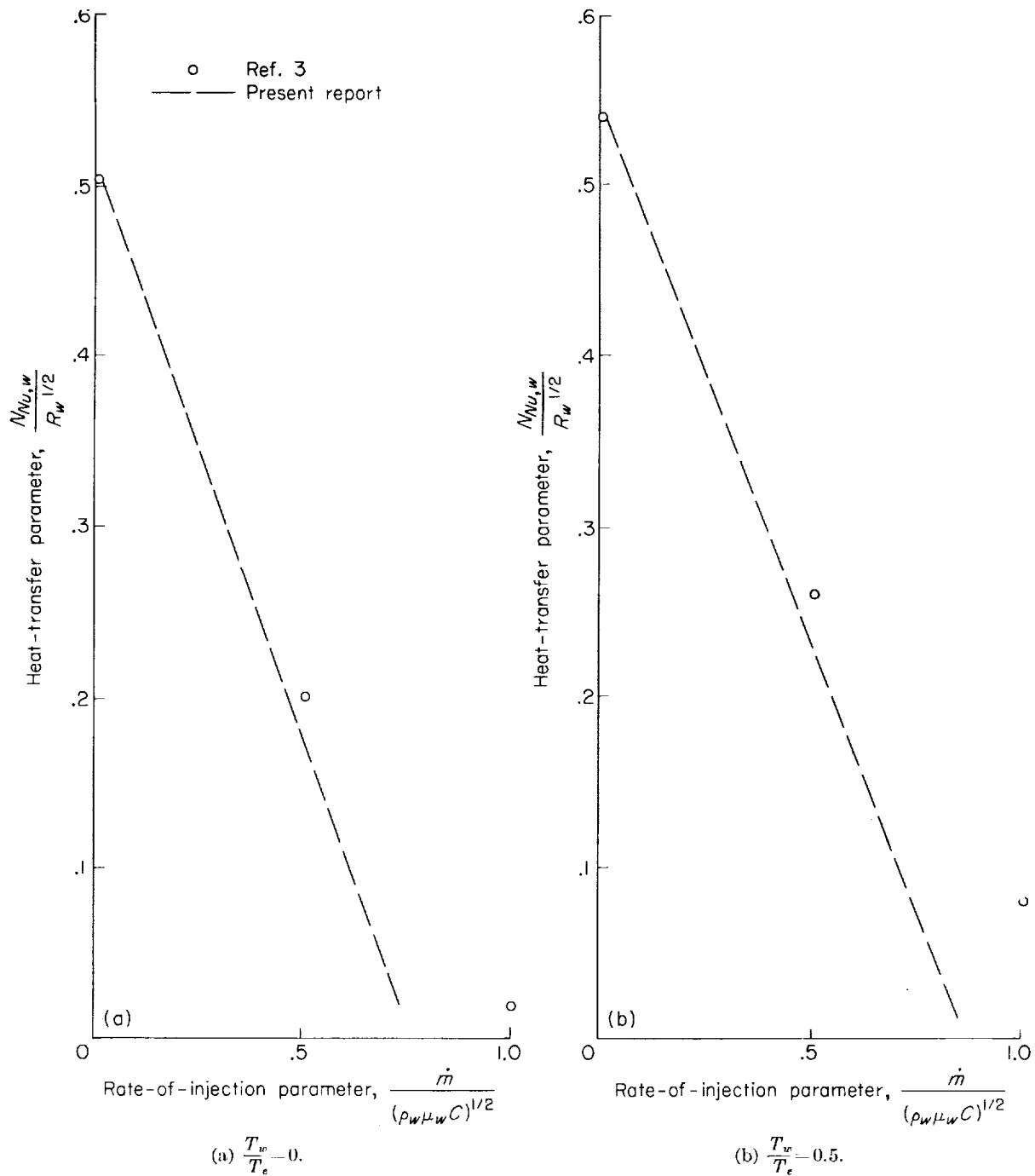
FIGURE 3.—Effect of air-to-air injection on heat-transfer parameter for two-dimensional case. N_{Pr,w} = 1 .
