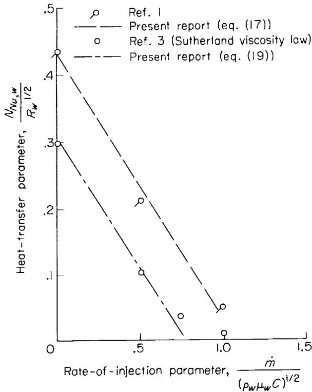
FIGURE 5.—Effect of air-to-air injection on heat-transfer parameter for two-dimensional case. N_{Pr,w} = 0.7 ; \frac{T_w}{T_c} = 0.05 .
