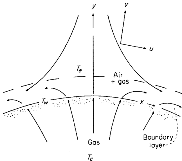
FIGURE 1.—Flow configuration.
