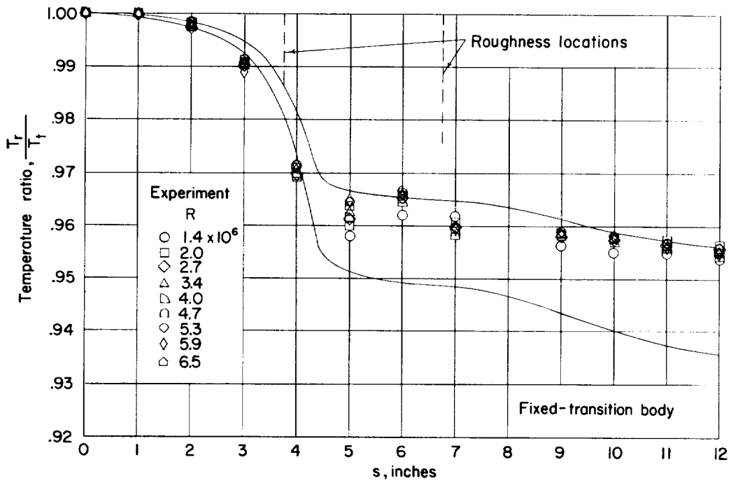
Figure 10.- Comparison of experimental recovery-temperature ratios with calculated recovery-temperature ratios for model C.
