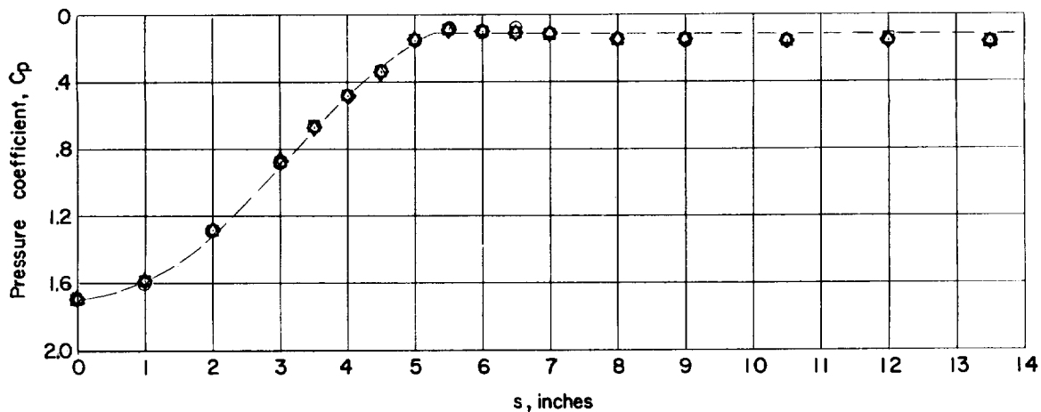
Figure 3.- Comparison of experimental pressure coefficients with calculated theoretical pressure coefficients for model B.
