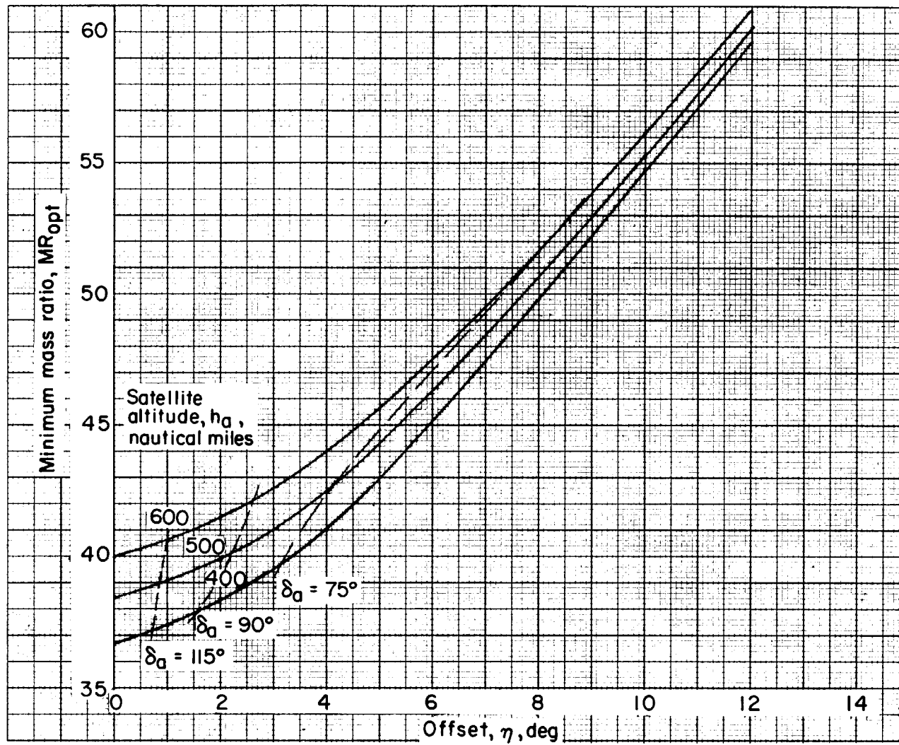
Figure 8.- Minimum mass ratio for launch to rendezvous as a function of the offset of the launch point from the orbital plane for three satellite altitudes. I_{sp} = 235 sec.
