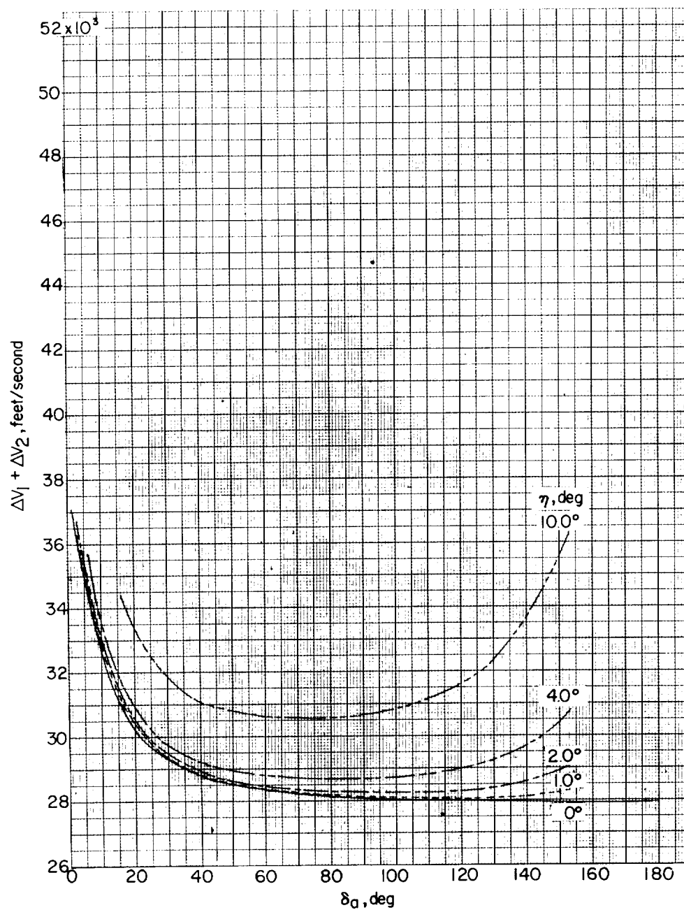
(c) 600-nautical-mile satellite.
