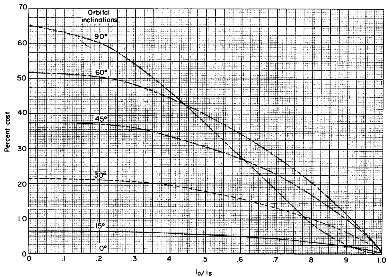
(a) 400-nautical-mile satellite.
