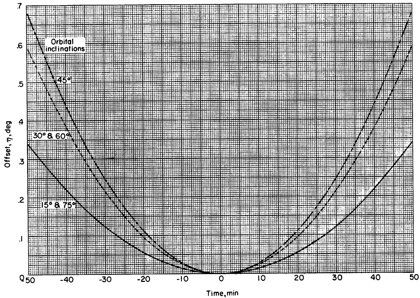
Figure 4.- Offset near the tangency condition as a function of time for orbital inclinations of 15°, 30°, 45°, 60°, and 75° for 400 nautical miles.
