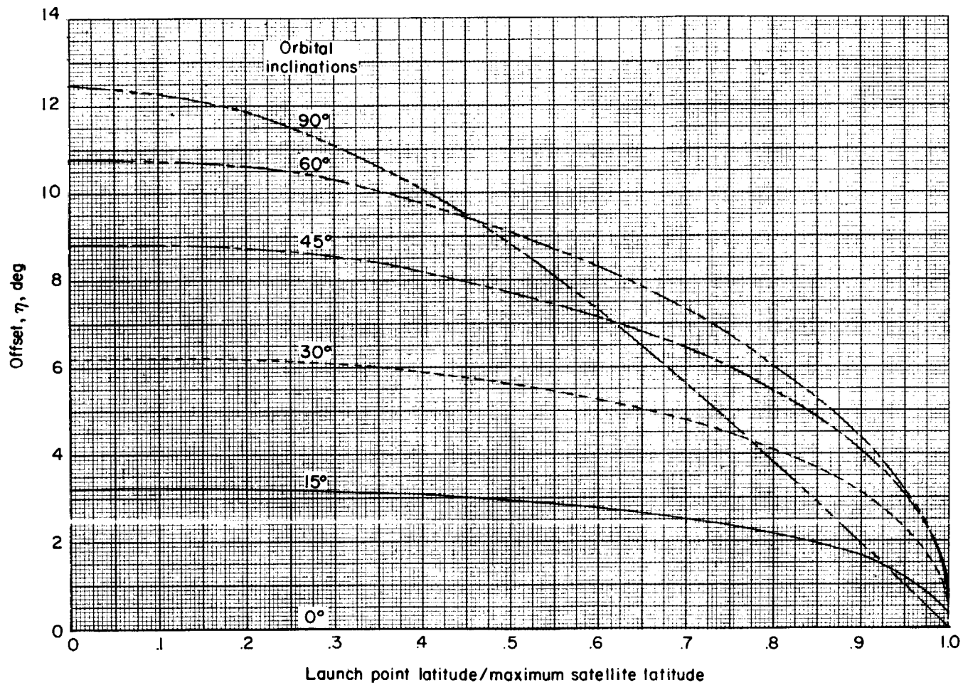
(a) 400-nautical-mile satellite.
