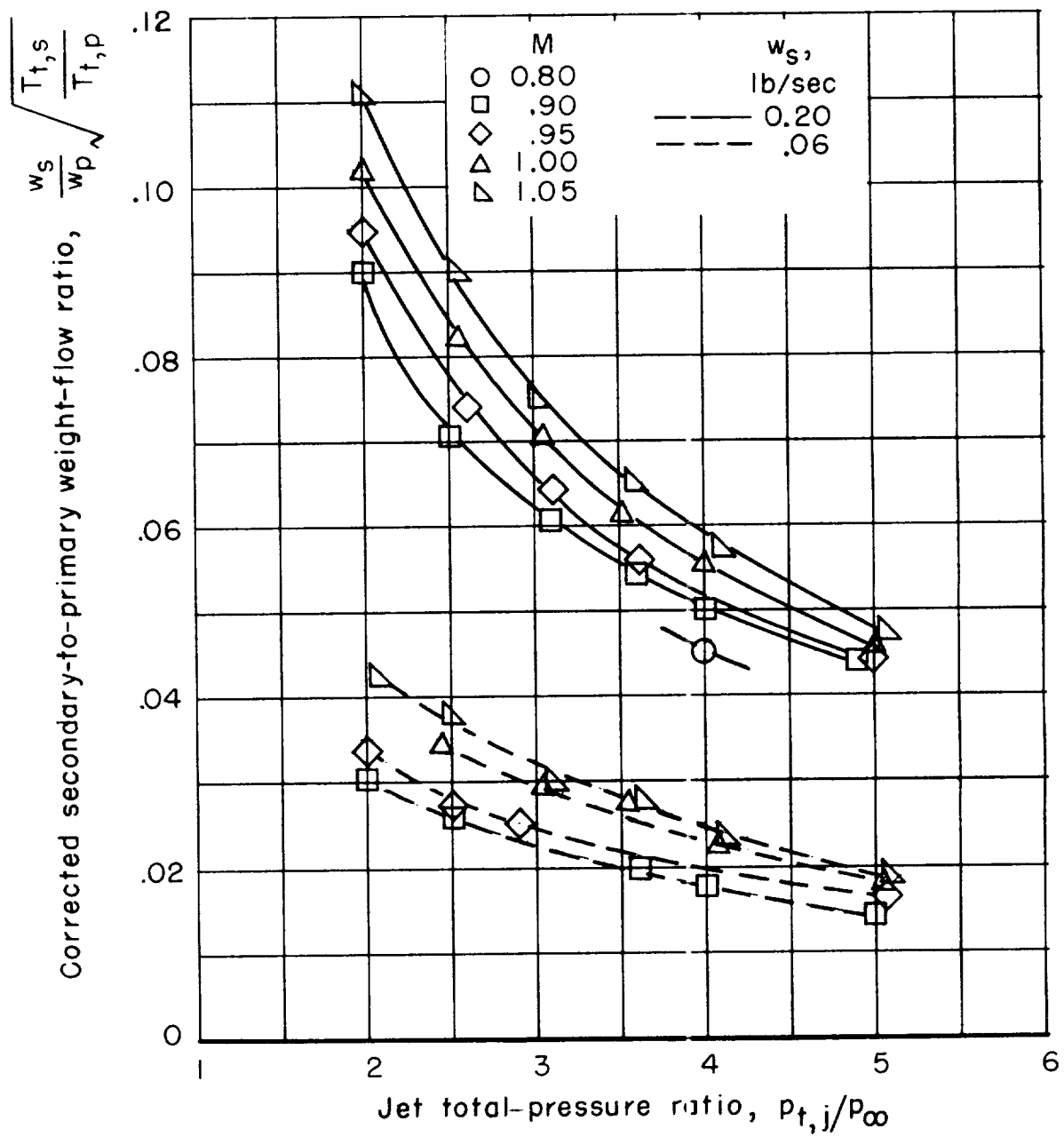
Figure 8.- Variation of corrected secondary-to-primary weight-flow ratio with jet total-pressure ratio for all test Mach numbers.
