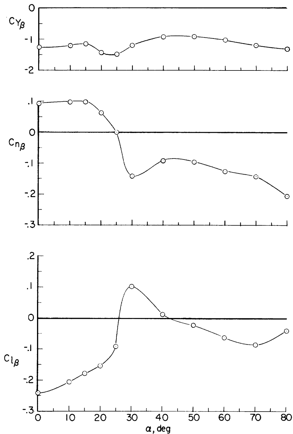
Figure 5.- Variation of static lateral stability derivatives with angle of attack. \beta = \pm 5^\circ .
