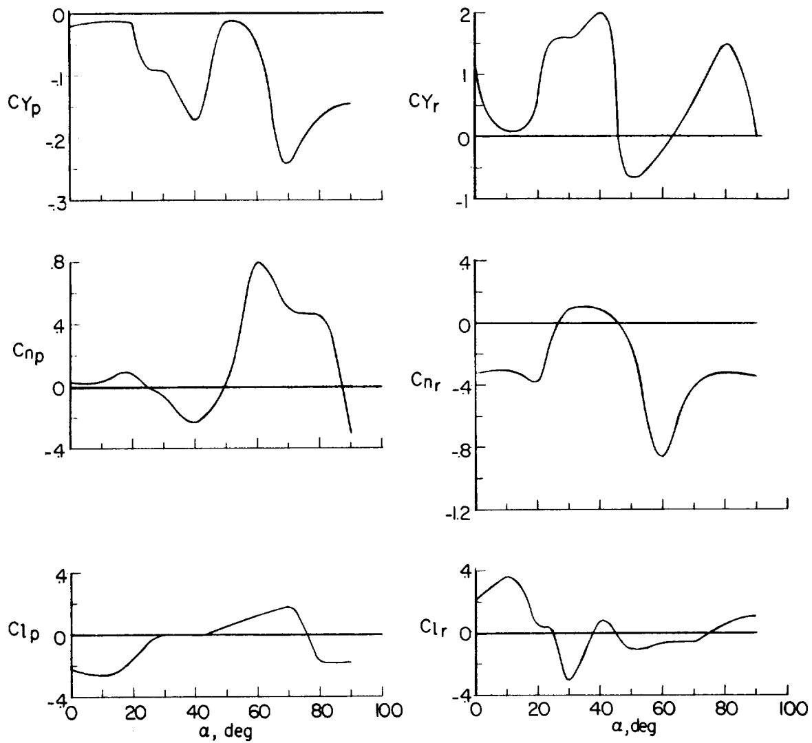
Figure 10.- Variation of rolling and yawing velocity derivatives with angle of attack. Determined from data for k = 0.15 in figure 8.
