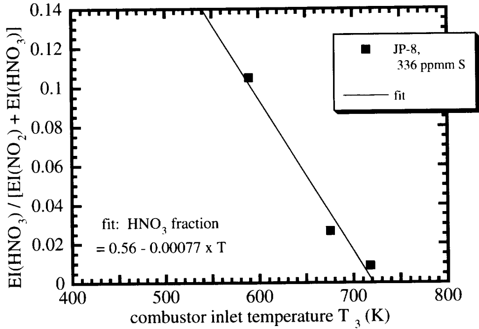
Figure E-11. Fraction of \text{NO}_2 converted into \text{HNO}_3 at 13.7 km altitude.
