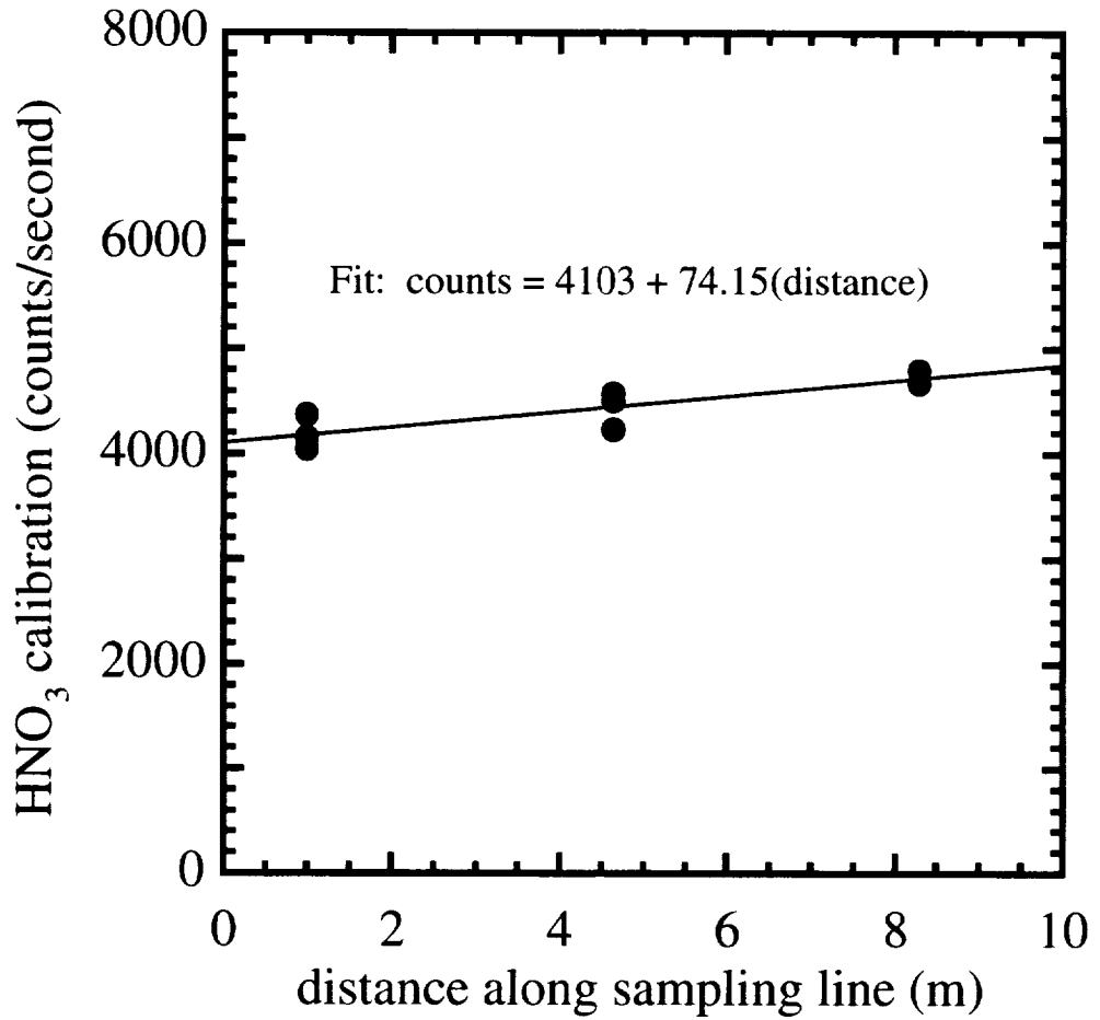
Figure E-2. Ion signal due to HNO 3 injected sequentially at three points along the sampling line. The data indicate that there is a 15% loss of HNO 3 over the full 8.3-m length of the sampling line.
