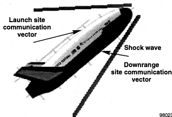
Figure 5. Communication vectors and plasma.
