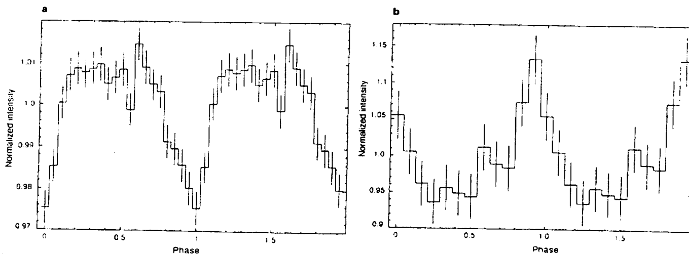
Figure 2 Epoch folded pulse profiles of SGR1806-20. a, RXTE/PCA data in 20 phase bins at the fundamental period of 7.476551 s, between 2 and 24 keV. b, ASCA data (from the 1993 observation of SGR1806 - 20) in 12 phase bins (to increase the signal to noise ratio) at the fundamental period of 7.468525 s
