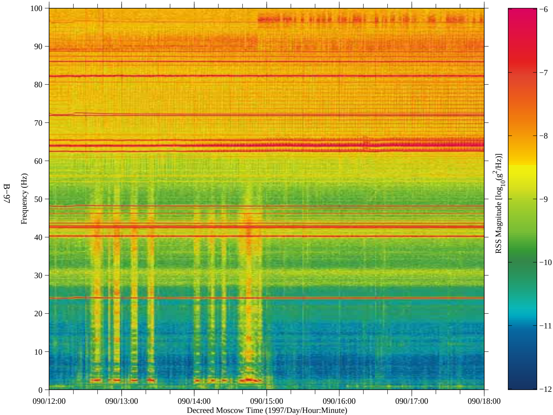
Figure 85: SAMS data from Mir, TSH A (fc=100 Hz)
