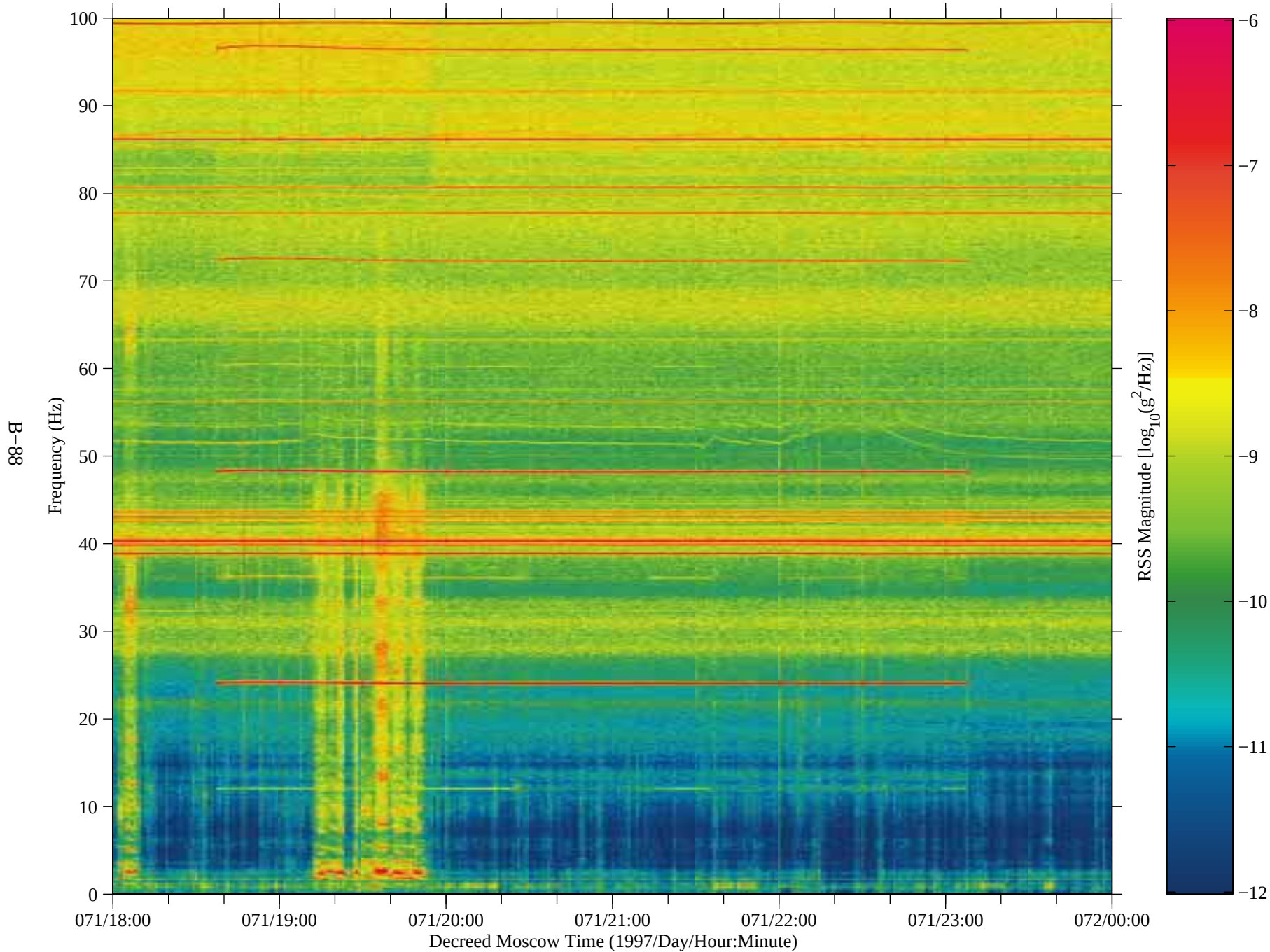
Figure 77: SAMS data from Mir, TSH A (fc=100 Hz)
