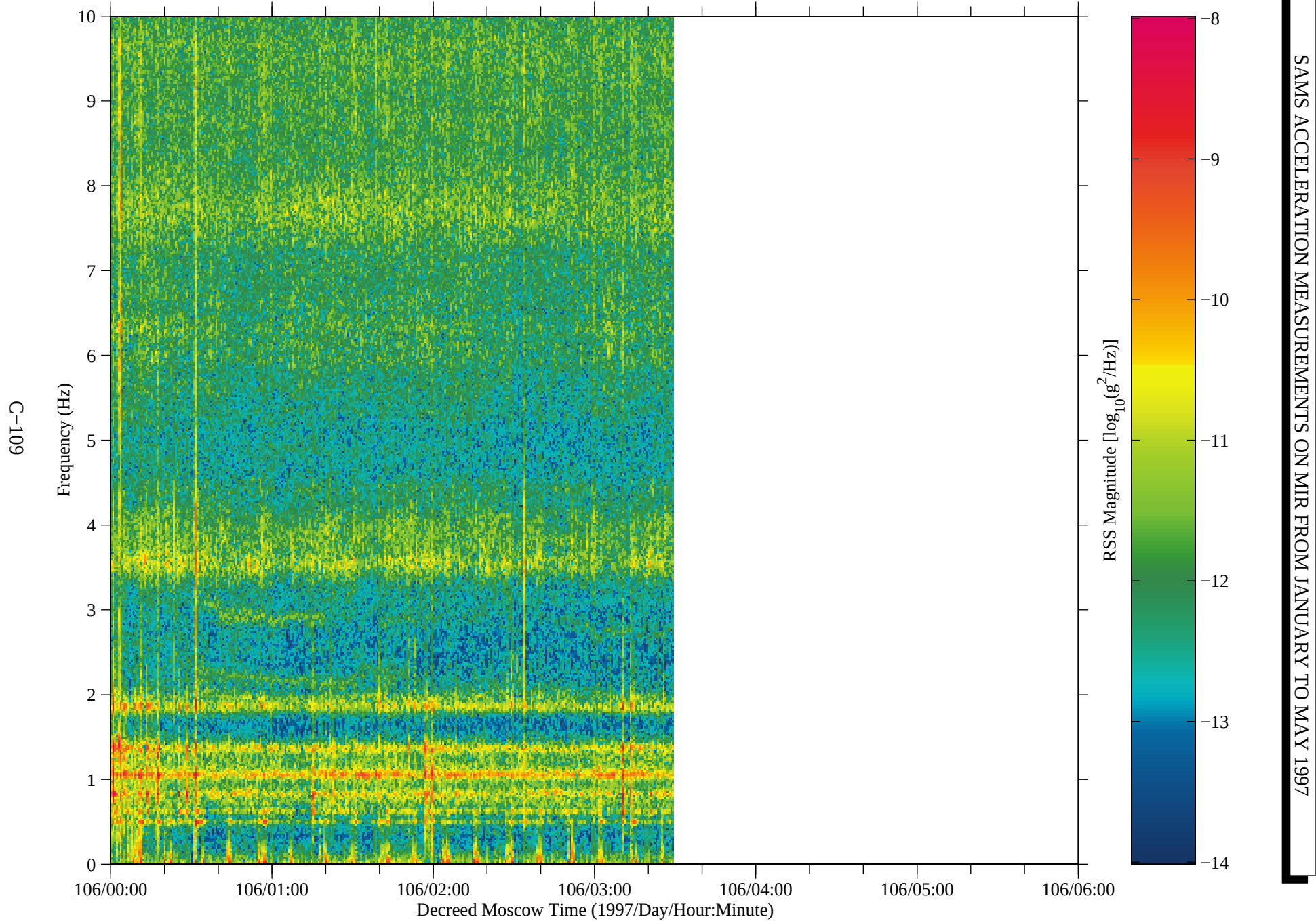
Figure 95: SAMS data from Mir, TSH B (fc=10 Hz)
