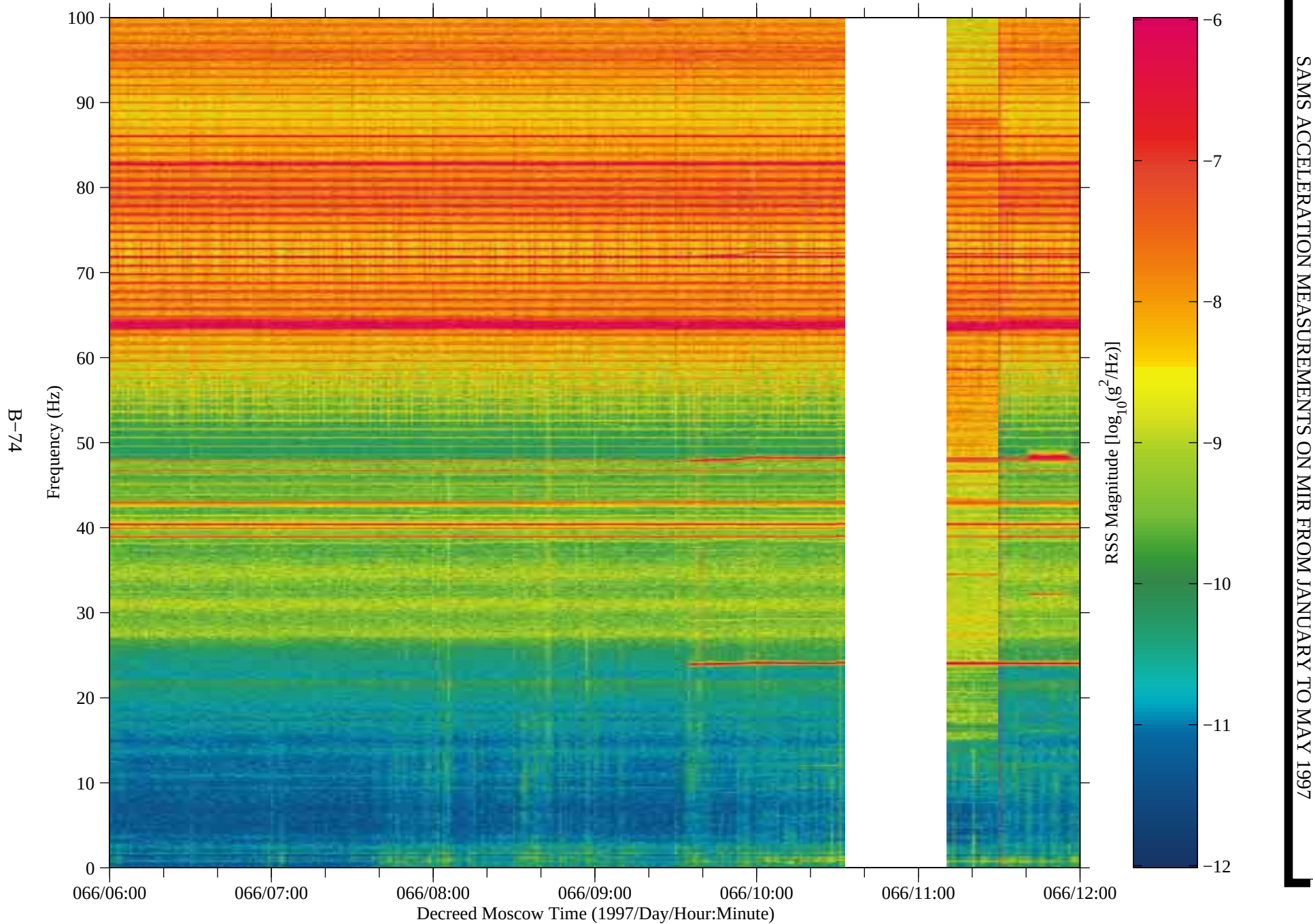
Figure 65: SAMS data from Mir, TSH A (fc=100 Hz)
