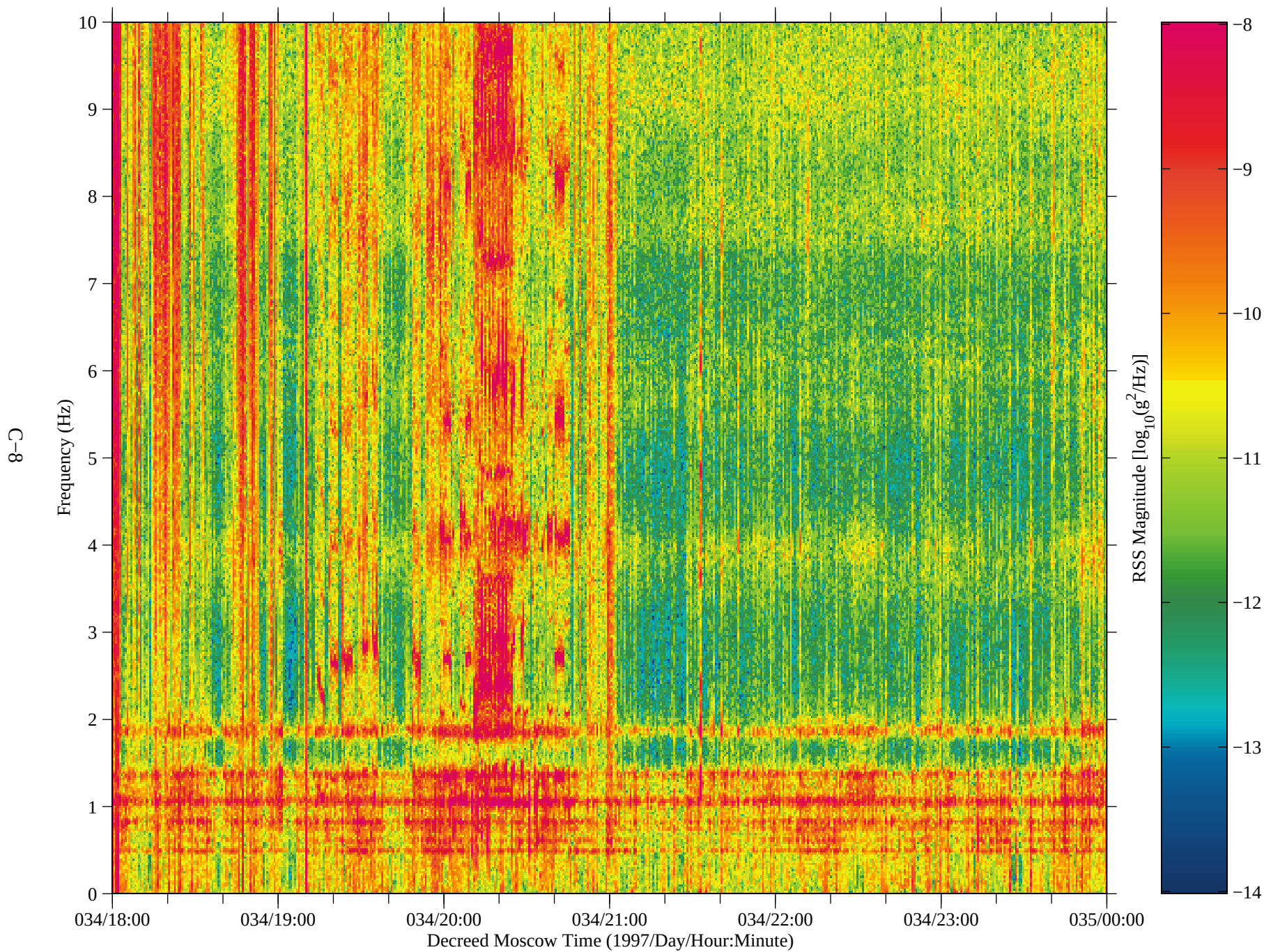
Figure 4: SAMS data from Mir, TSH B (fc=10 Hz)
