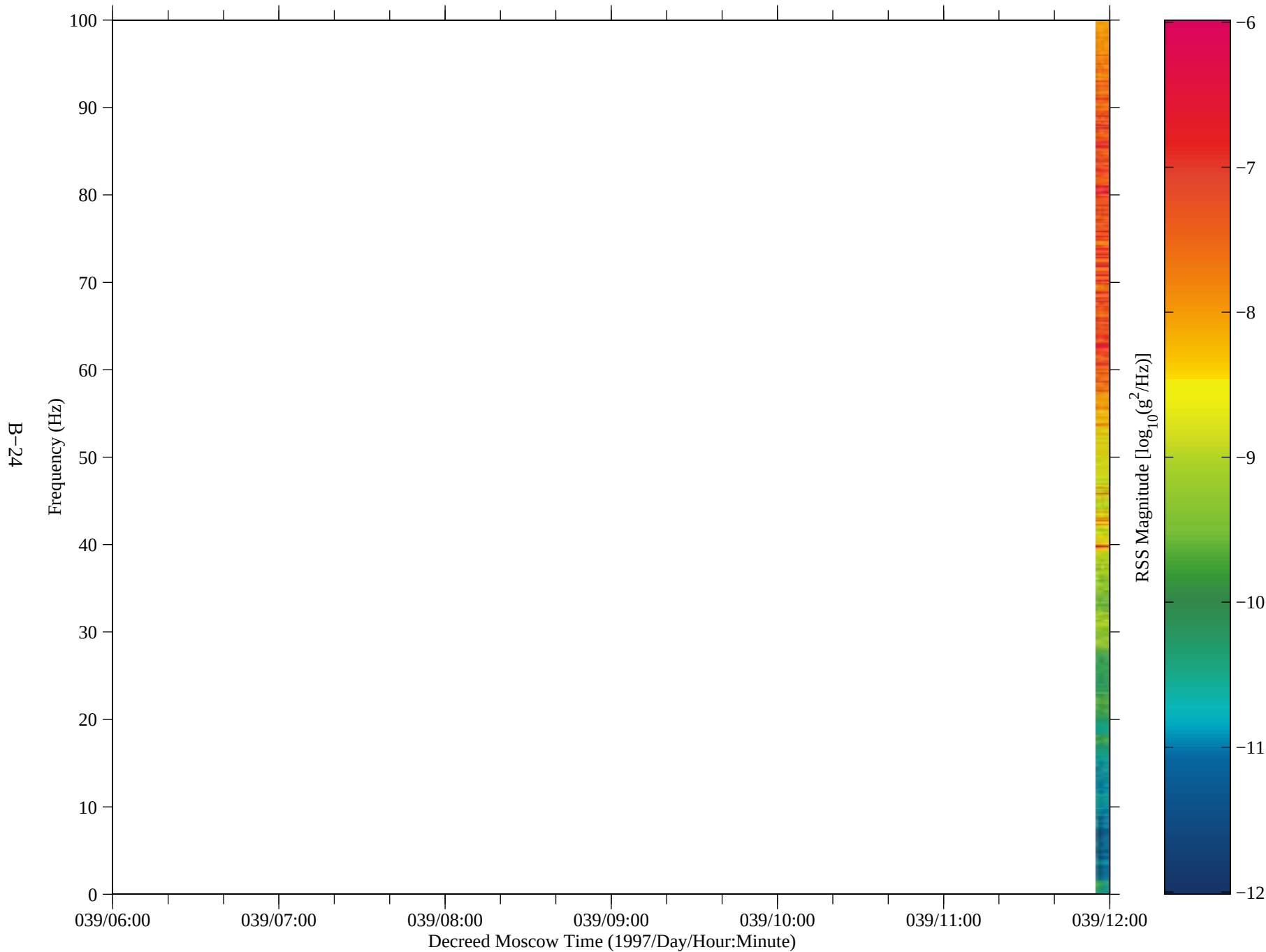
Figure 19: SAMS data from Mir, TSH A (fc=100 Hz)
