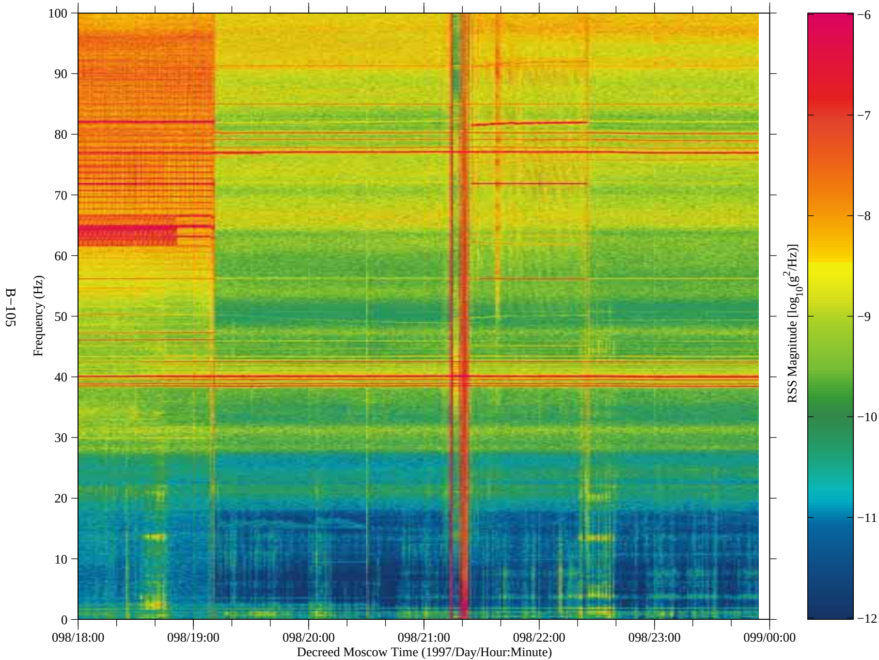
Figure 92: SAMS data from Mir, TSH A (fc=100 Hz)
