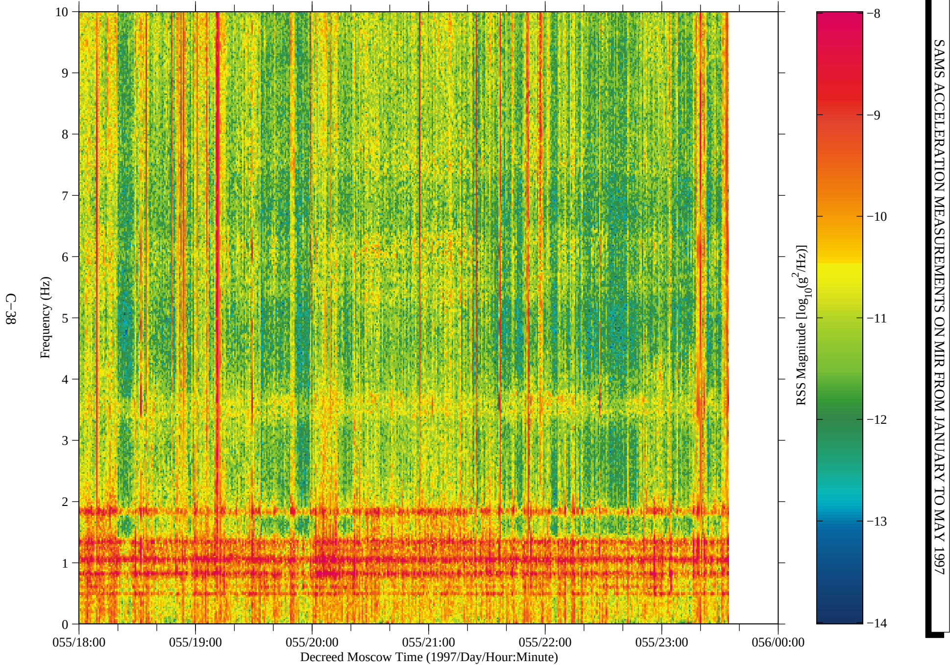
Figure 31: SAMS data from Mir, TSH B (fc=10 Hz)
