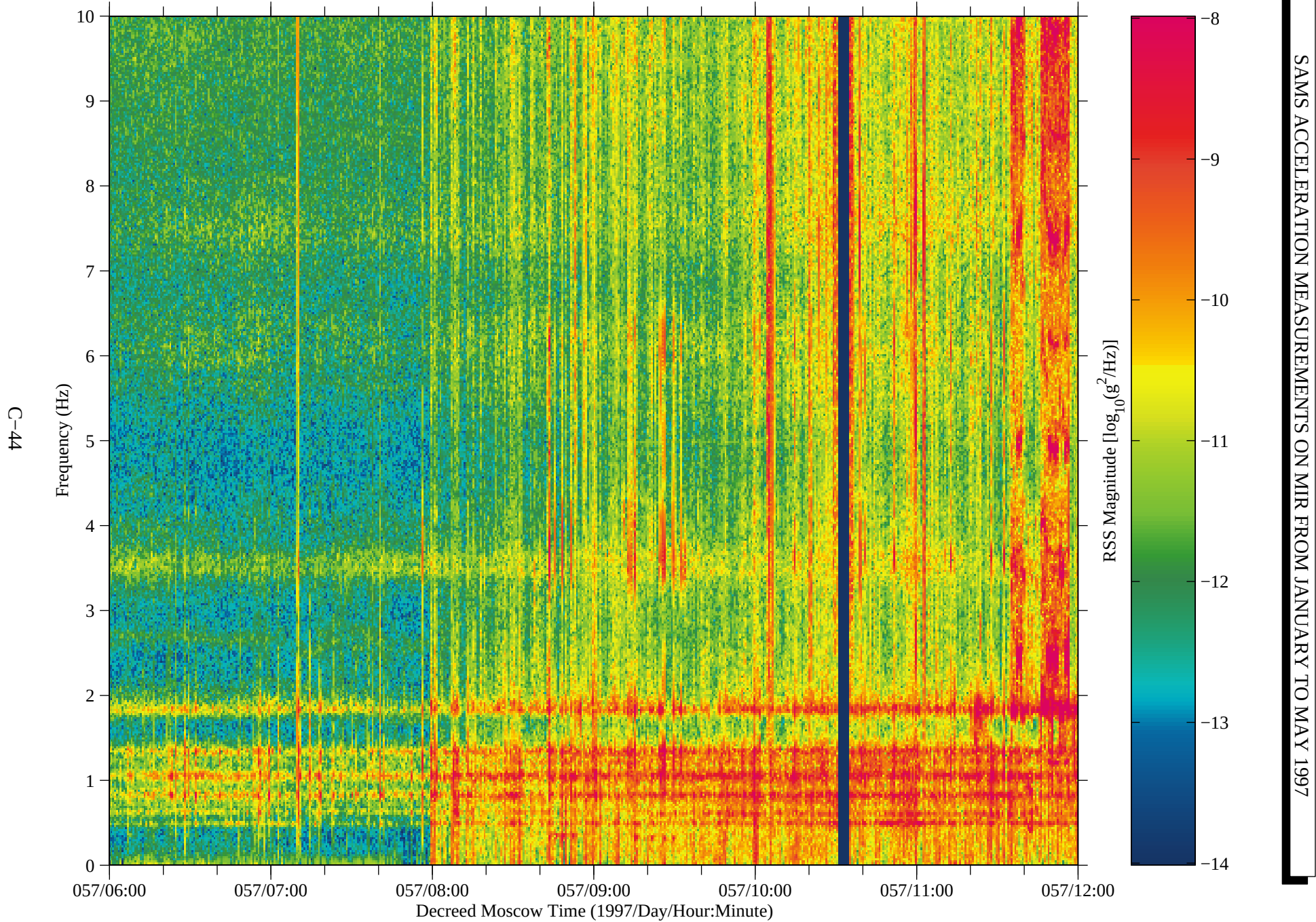
Figure 36: SAMS data from Mir, TSH B (fc=10 Hz)
