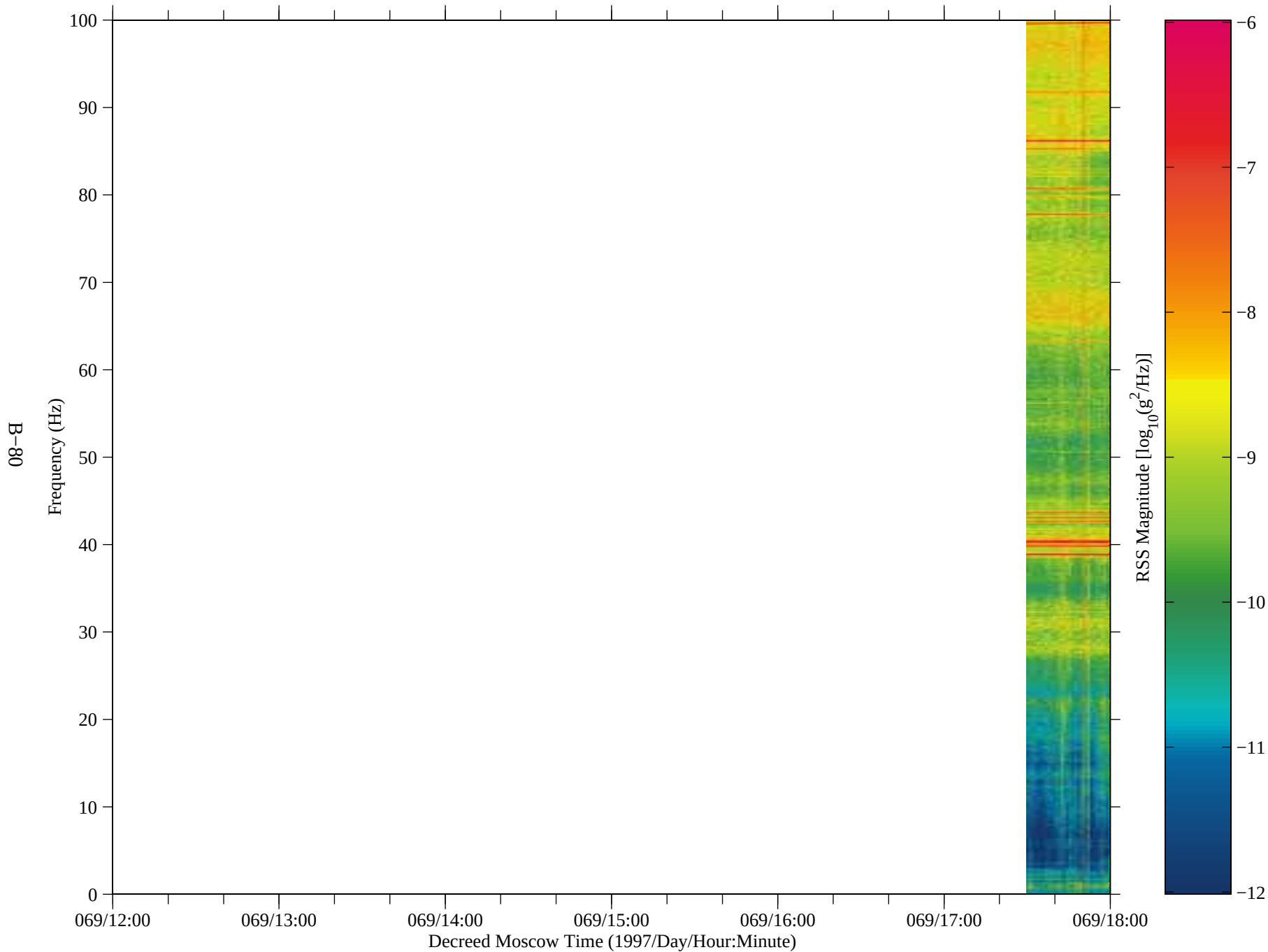
Figure 70: SAMS data from Mir, TSH A (fc=100 Hz)
