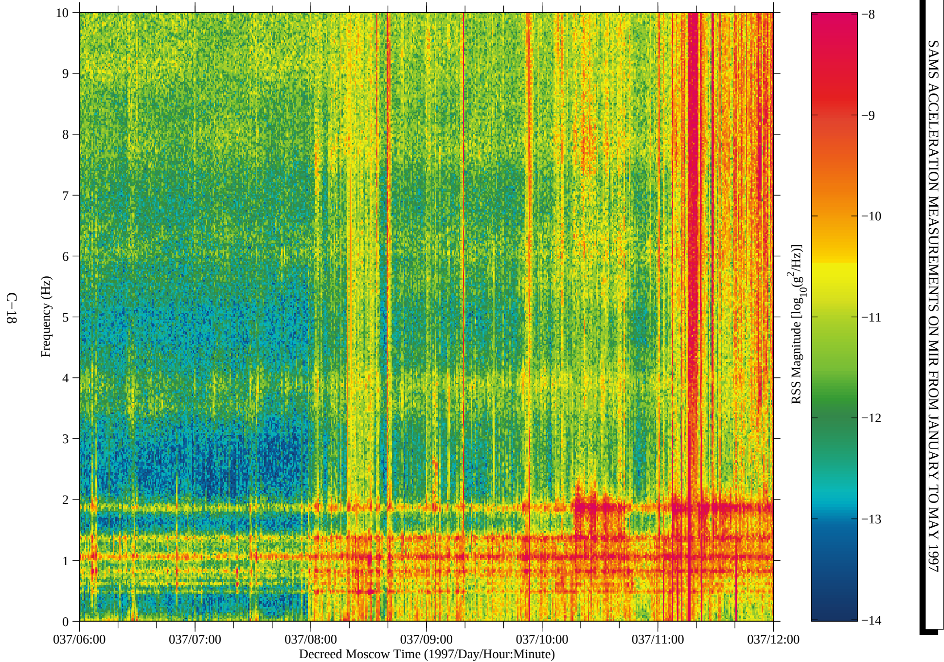
Figure 14: SAMS data from Mir, TSH B (fc=10 Hz)
