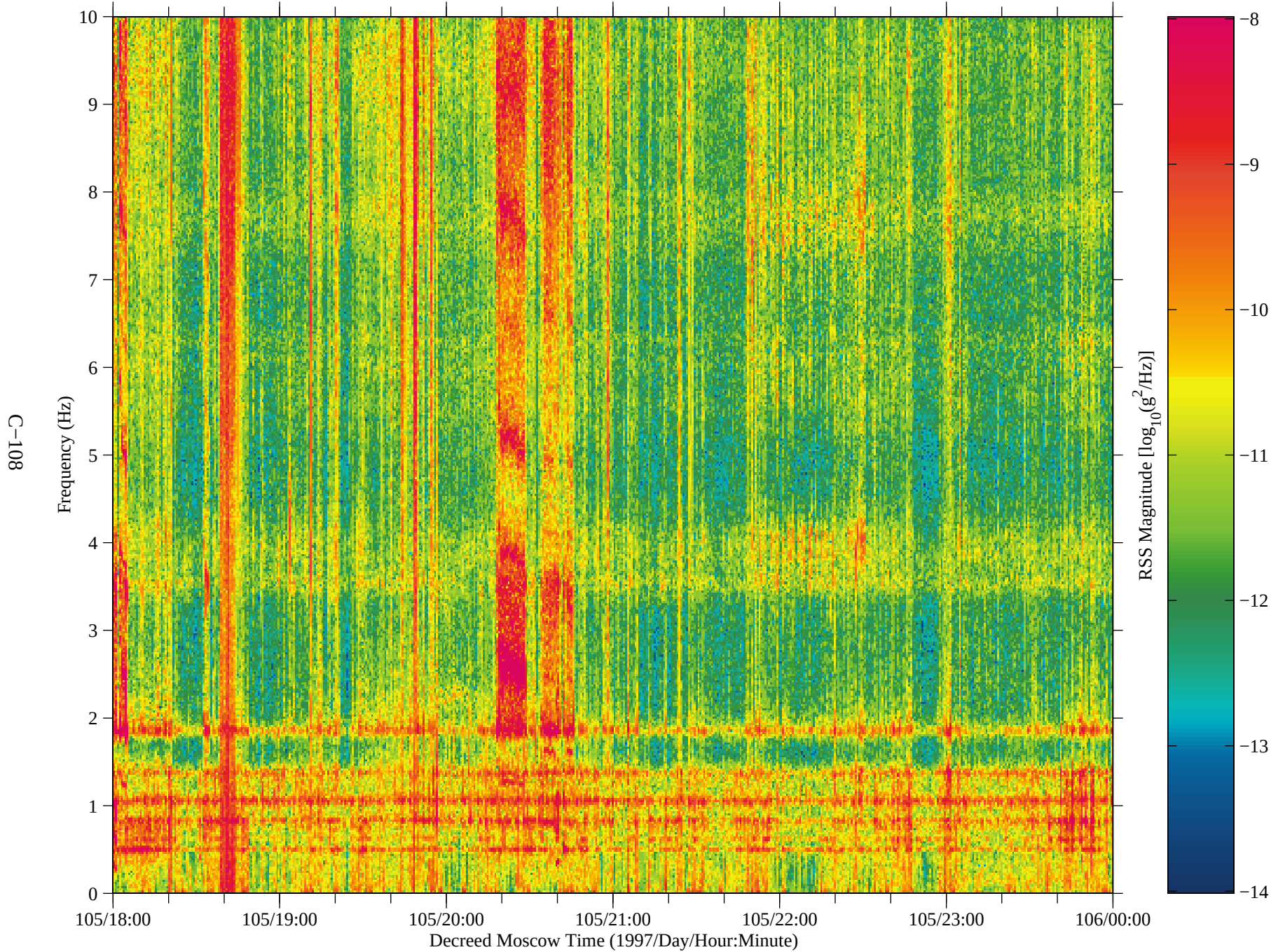
Figure 94: SAMS data from Mir, TSH B (fc=10 Hz)
