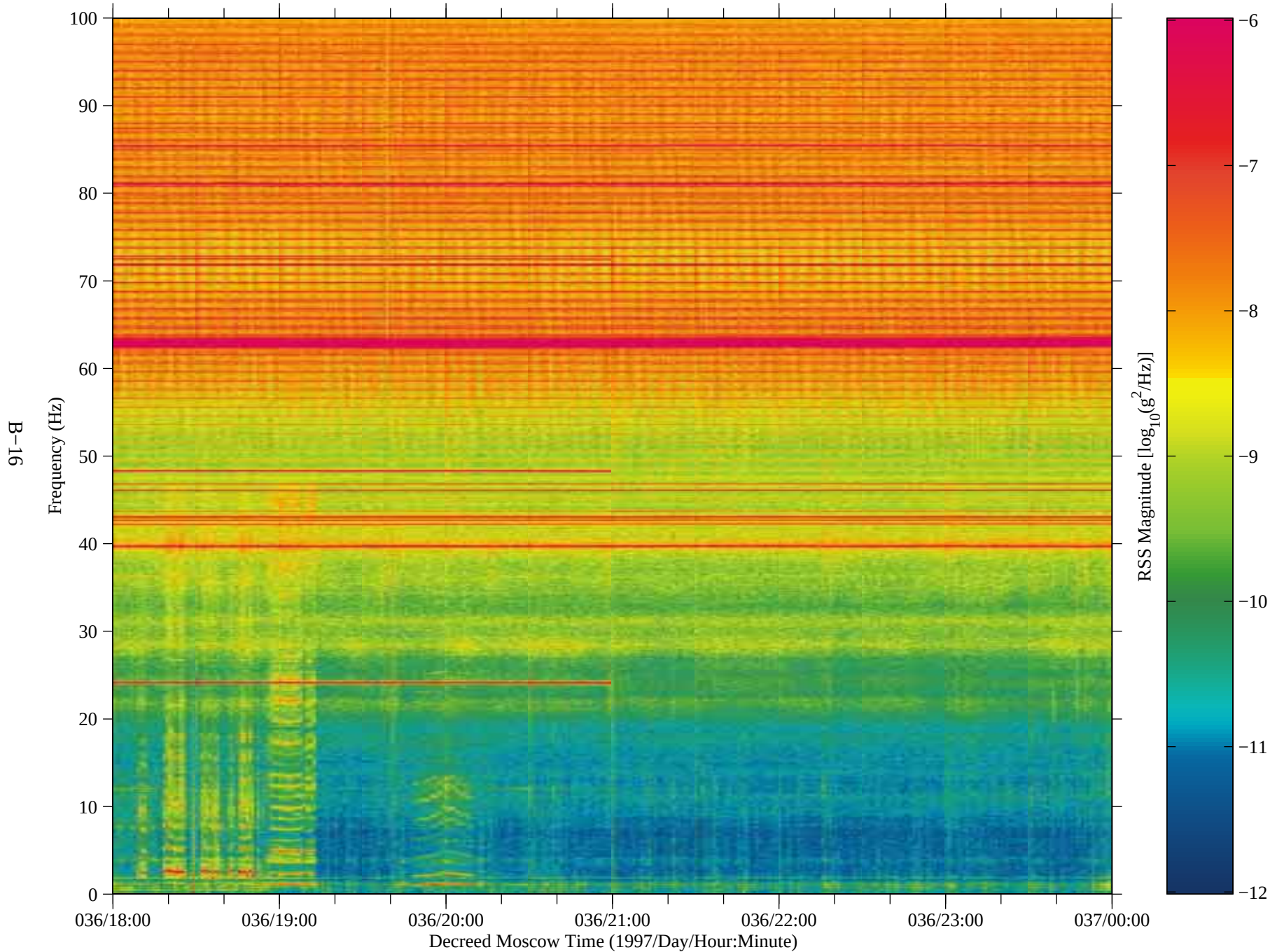
Figure 12: SAMS data from Mir, TSH A (fc=100 Hz)
