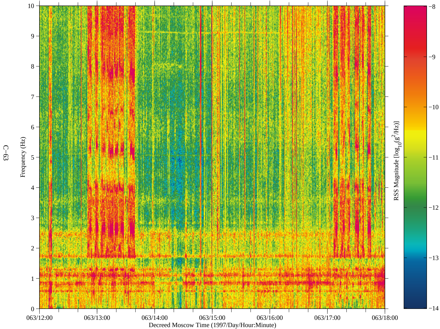
Figure 54: SAMS data from Mir, TSH B (fc=10 Hz)
