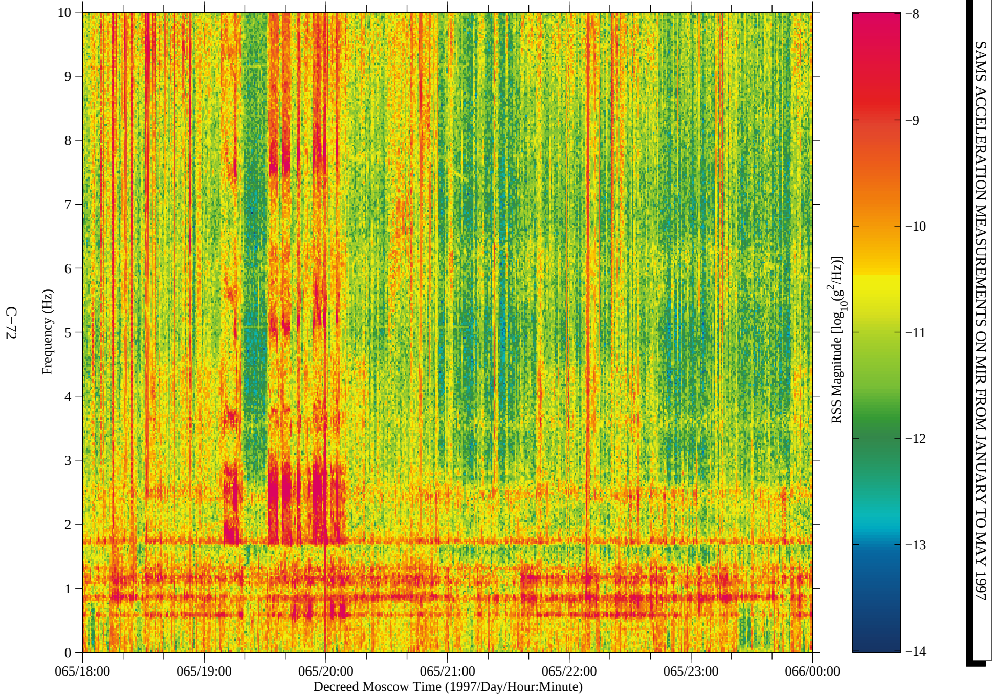
Figure 63: SAMS data from Mir, TSH B (fc=10 Hz)
