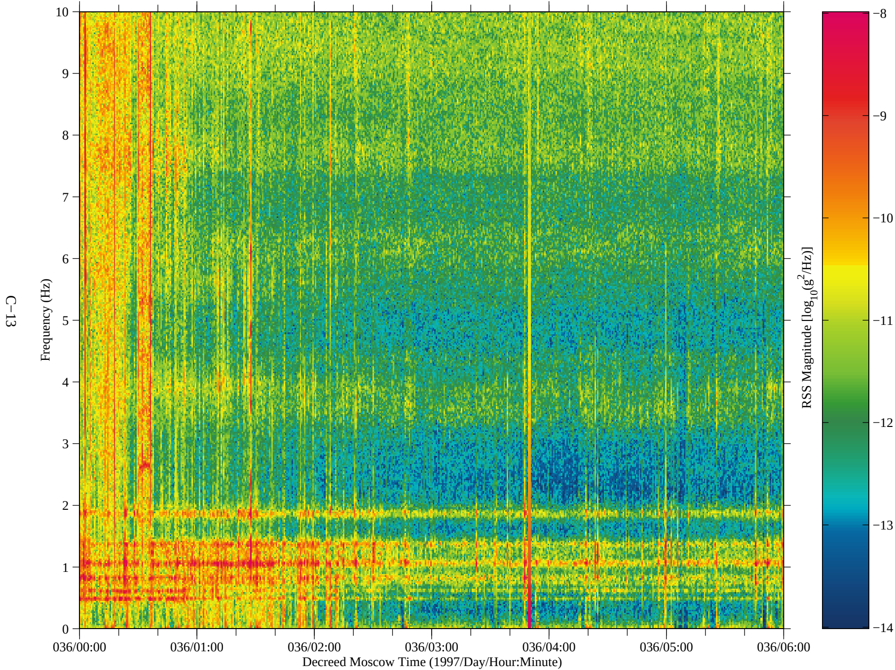
Figure 9: SAMS data from Mir, TSH B (fc=10 Hz)
