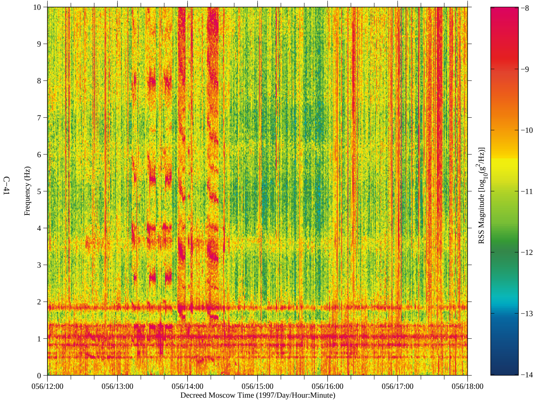
Figure 33: SAMS data from Mir, TSH B (fc=10 Hz)
