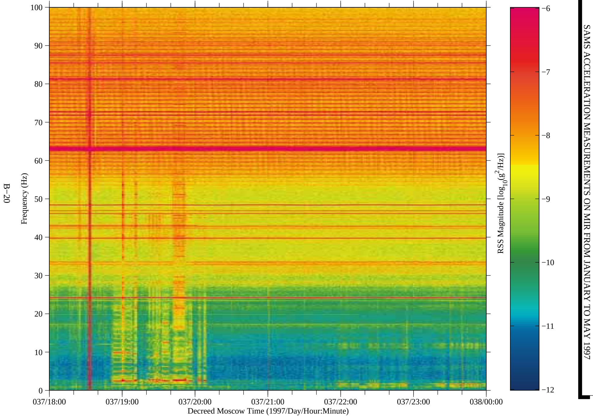
Figure 16: SAMS data from Mir, TSH A (fc=100 Hz)
