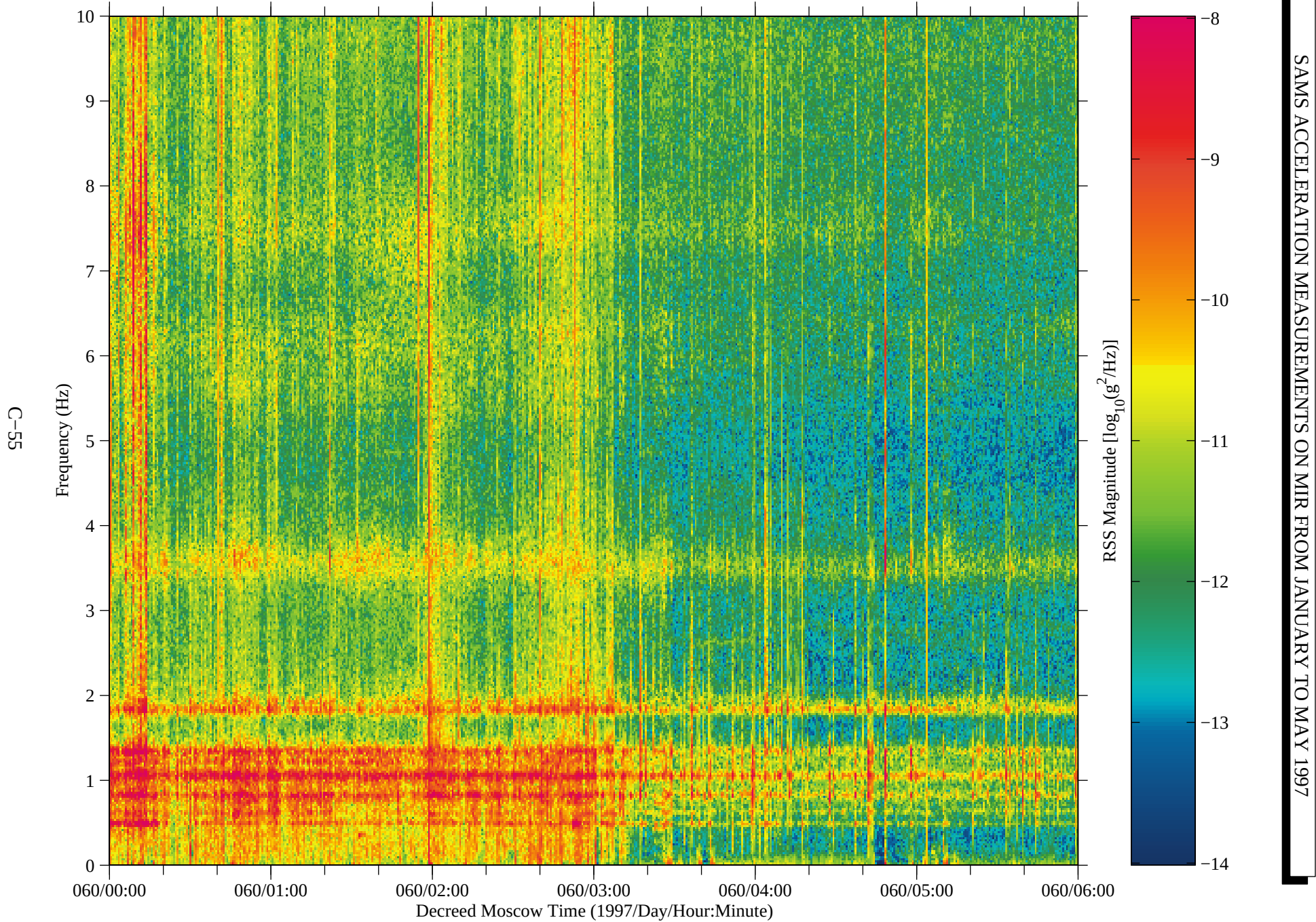
Figure 47: SAMS data from Mir, TSH B (fc=10 Hz)
