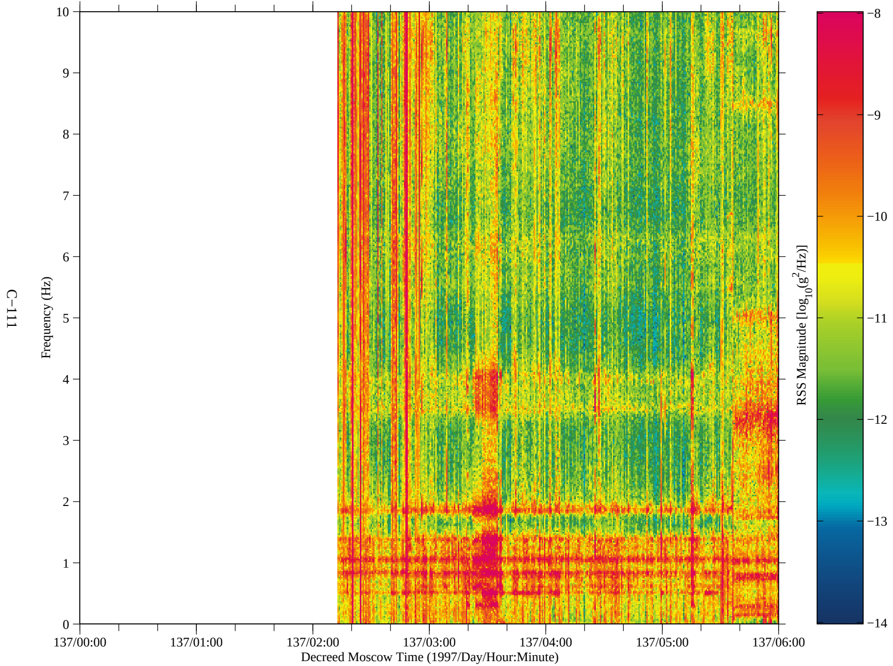
Figure 96: SAMS data from Mir, TSH B (fc=10 Hz)
