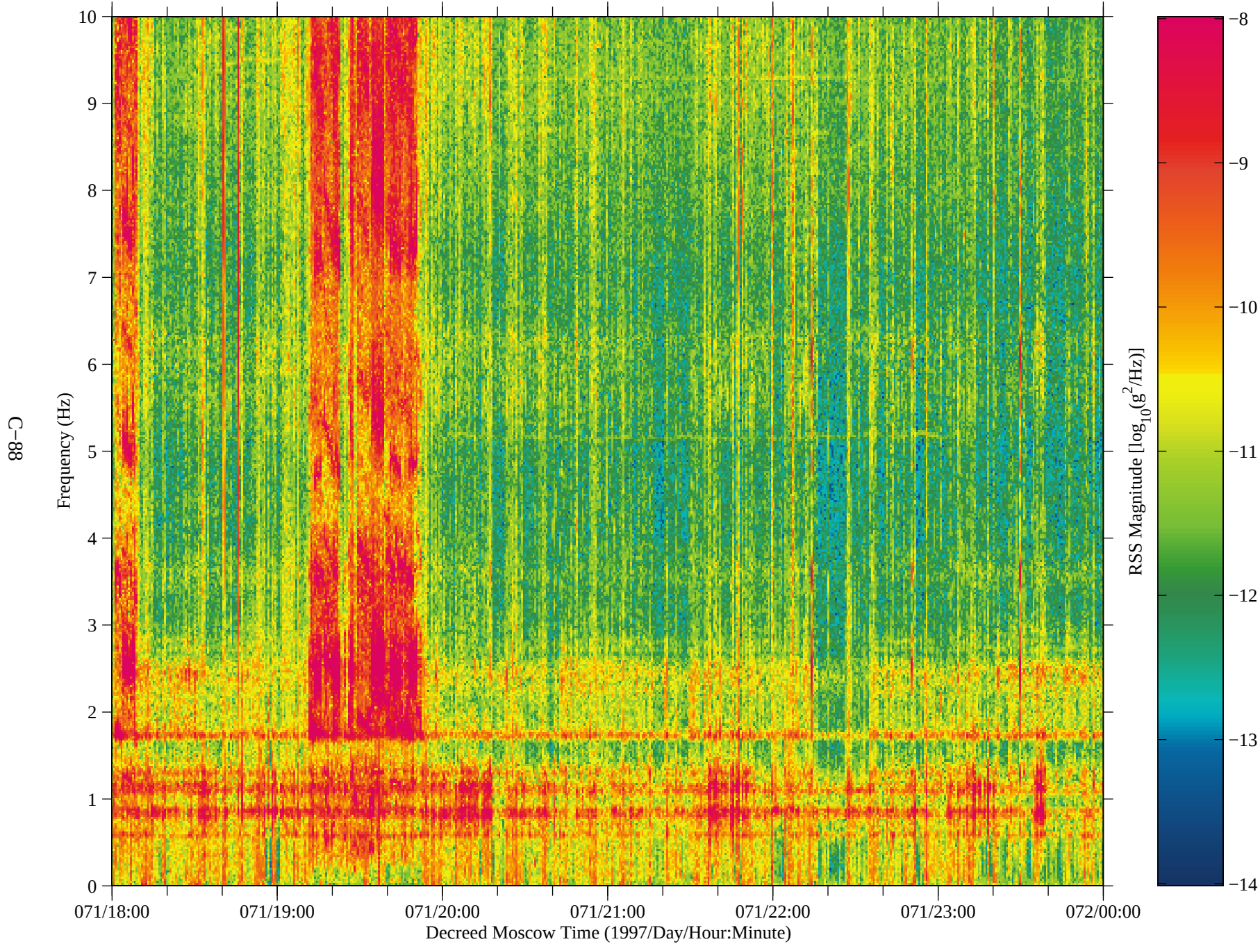
Figure 77: SAMS data from Mir, TSH B (fc=10 Hz)
