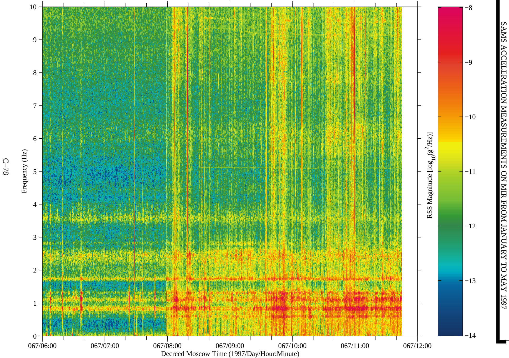
Figure 69: SAMS data from Mir, TSH B (fc=10 Hz)
