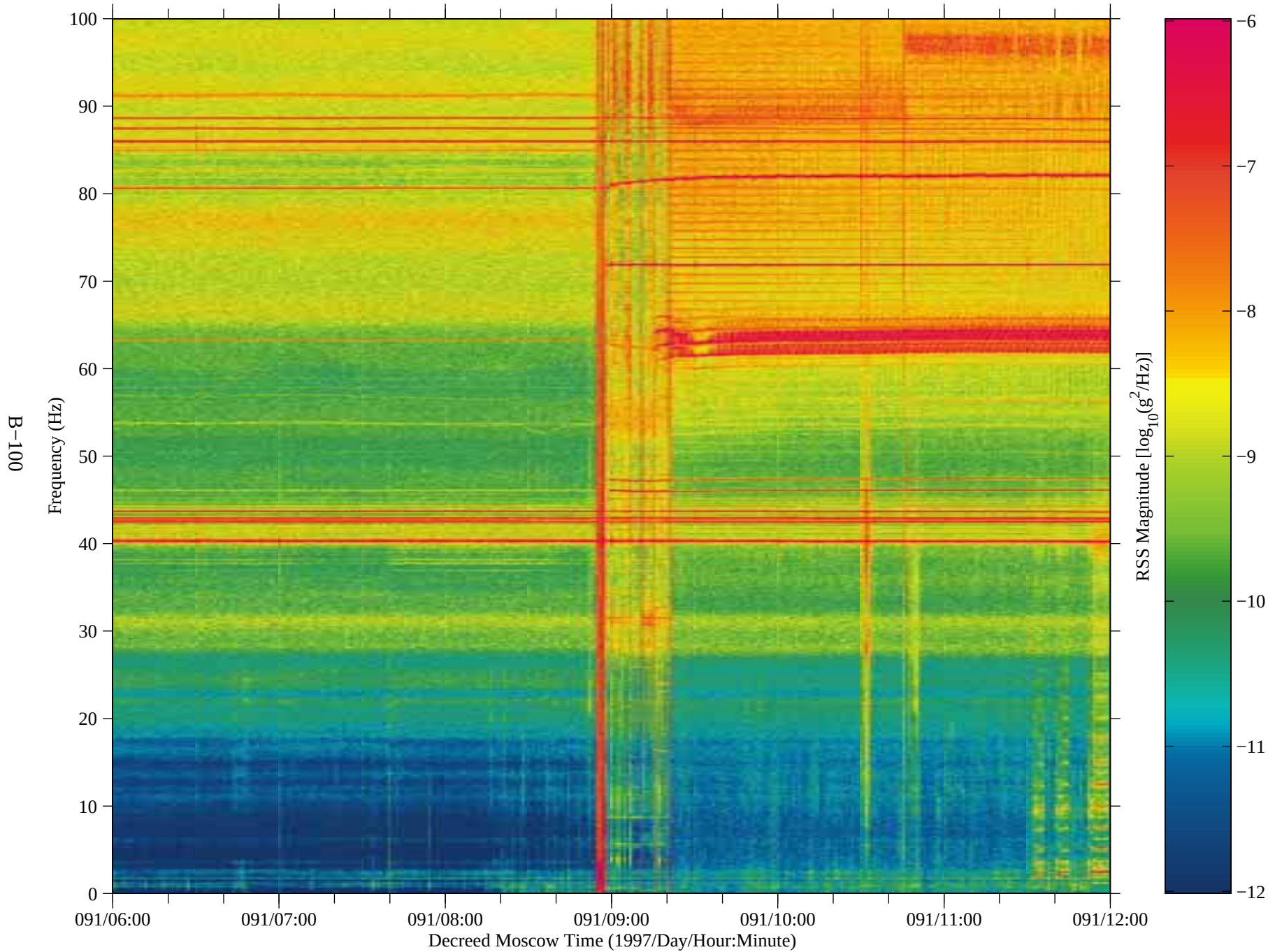
Figure 88: SAMS data from Mir, TSH A (fc=100 Hz)
