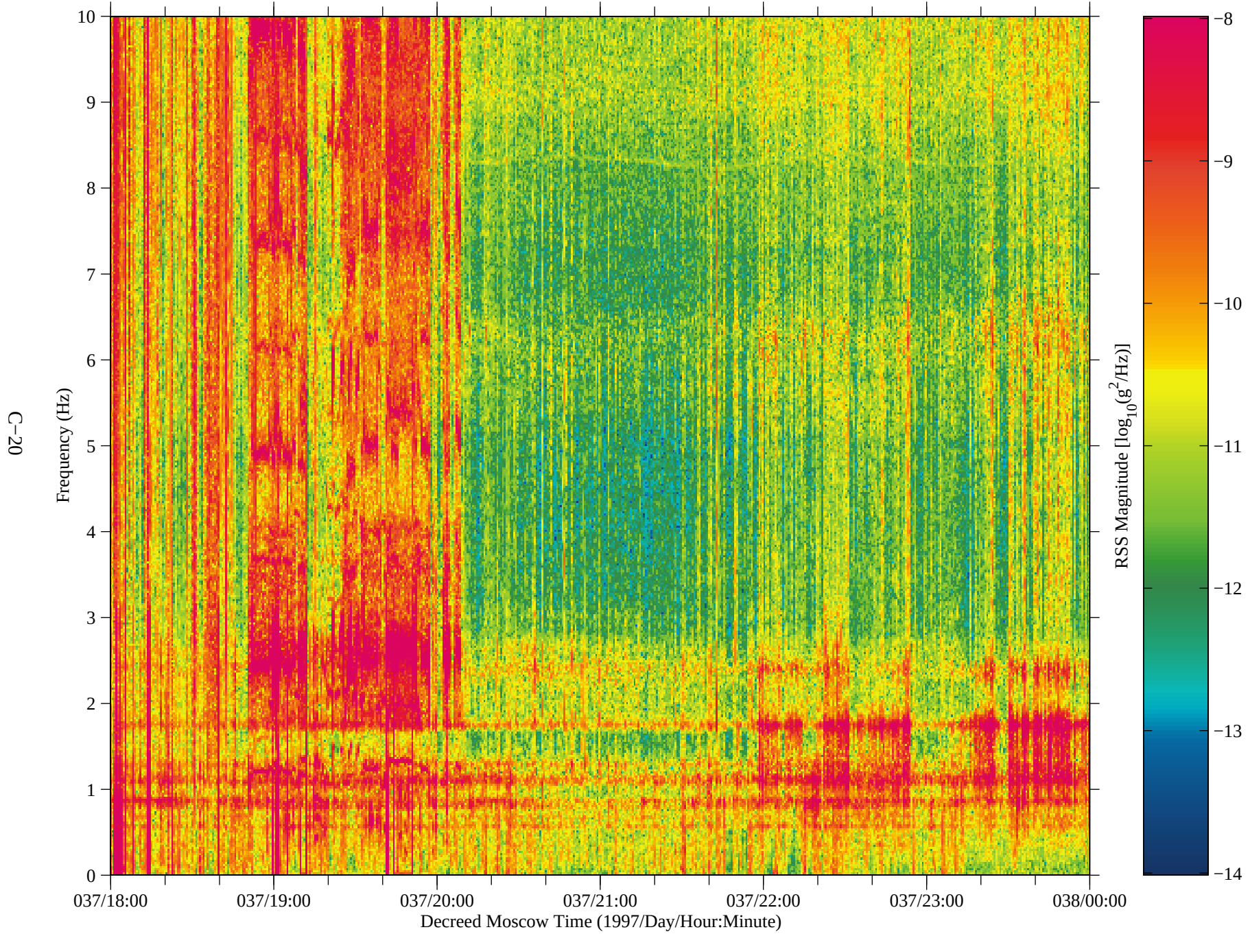
Figure 16: SAMS data from Mir, TSH B (fc=10 Hz)
