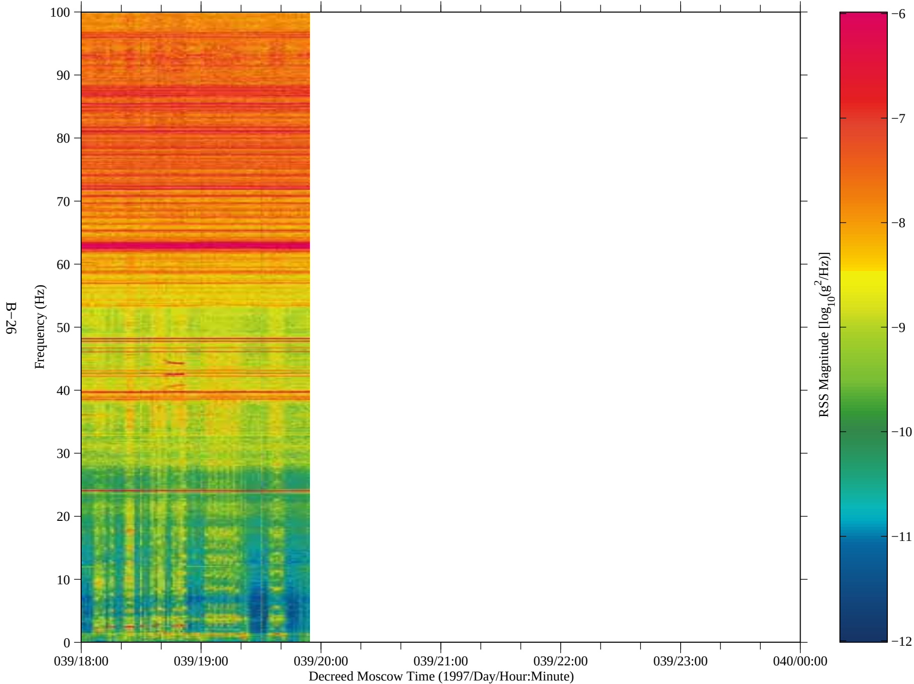
Figure 21: SAMS data from Mir, TSH A (fc=100 Hz)
