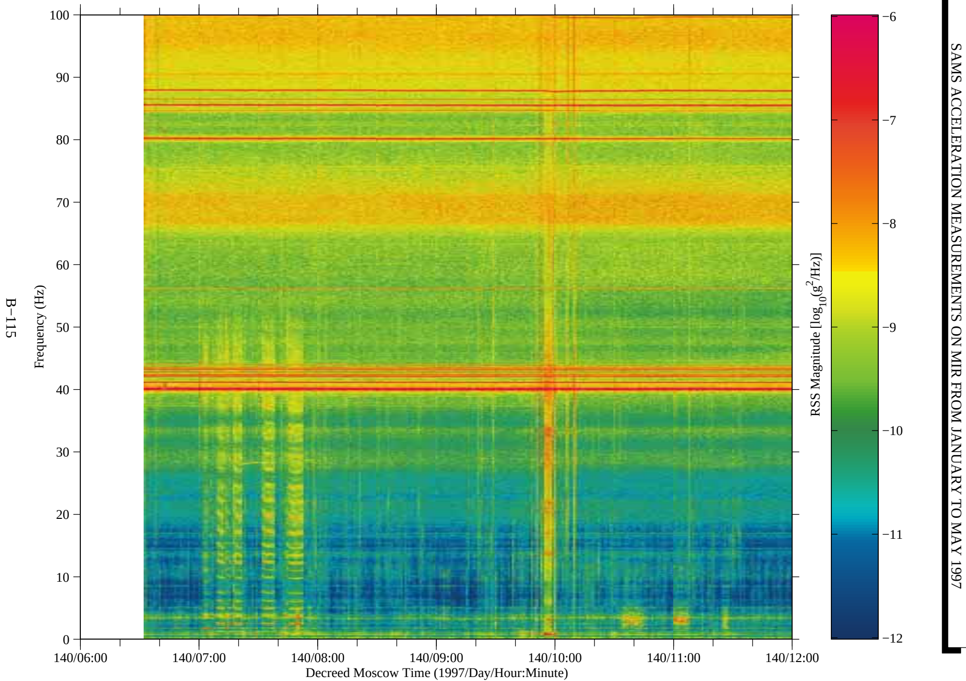
Figure 99: SAMS data from Mir, TSH A (fc=100 Hz)
