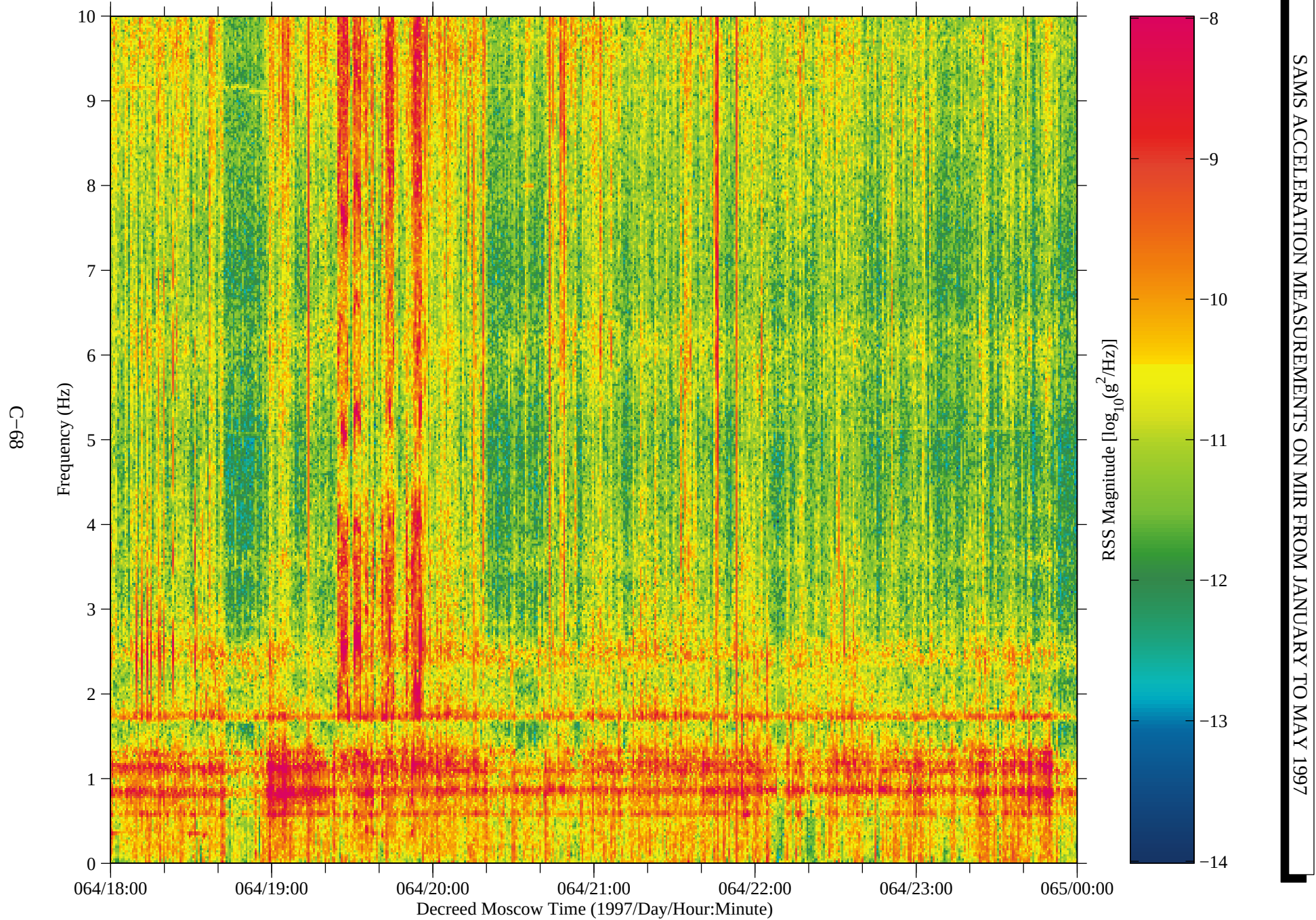
Figure 59: SAMS data from Mir, TSH B (fc=10 Hz)
