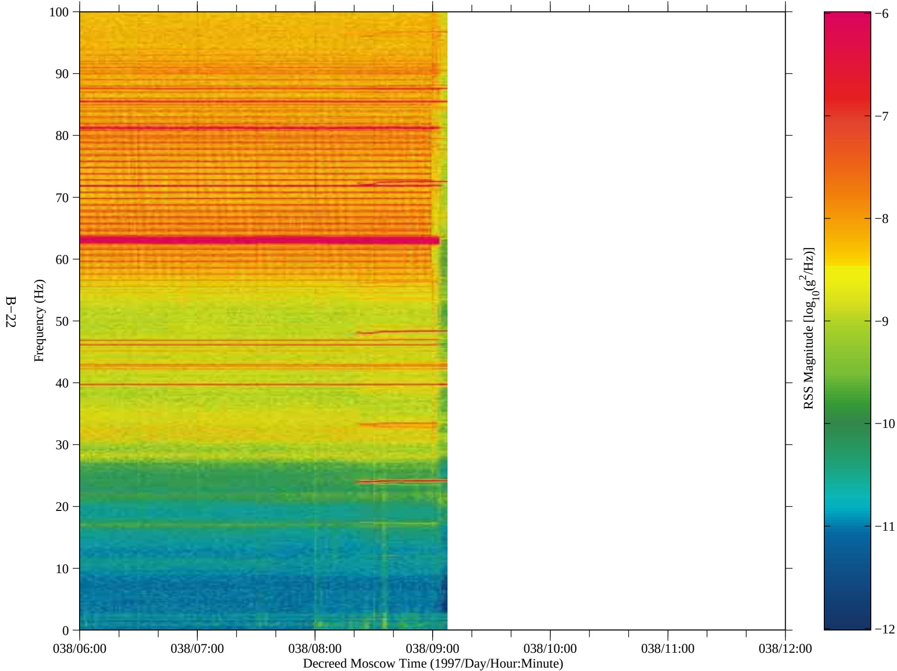
Figure 18: SAMS data from Mir, TSH A (fc=100 Hz)
