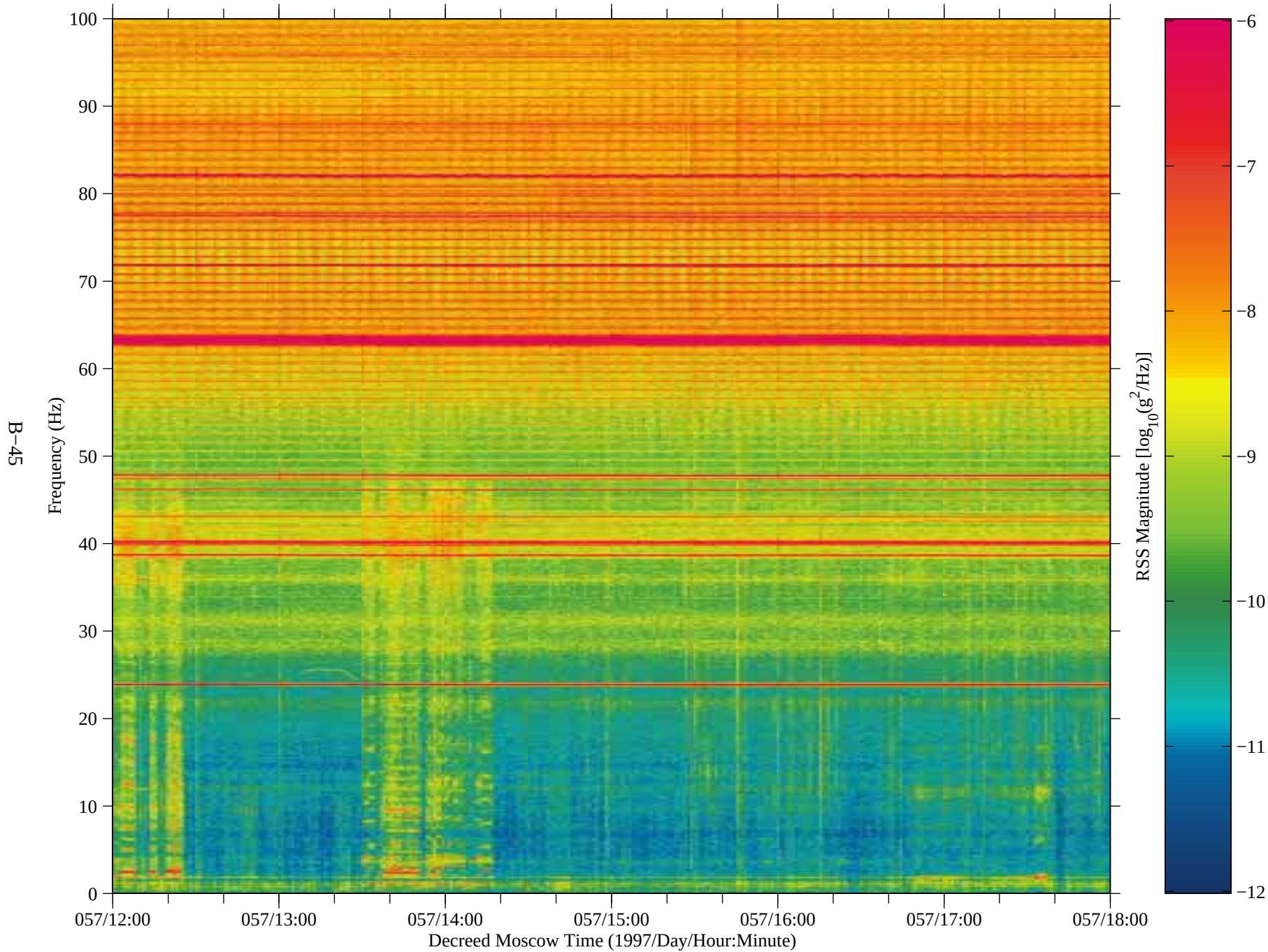
Figure 37: SAMS data from Mir, TSH A (fc=100 Hz)
