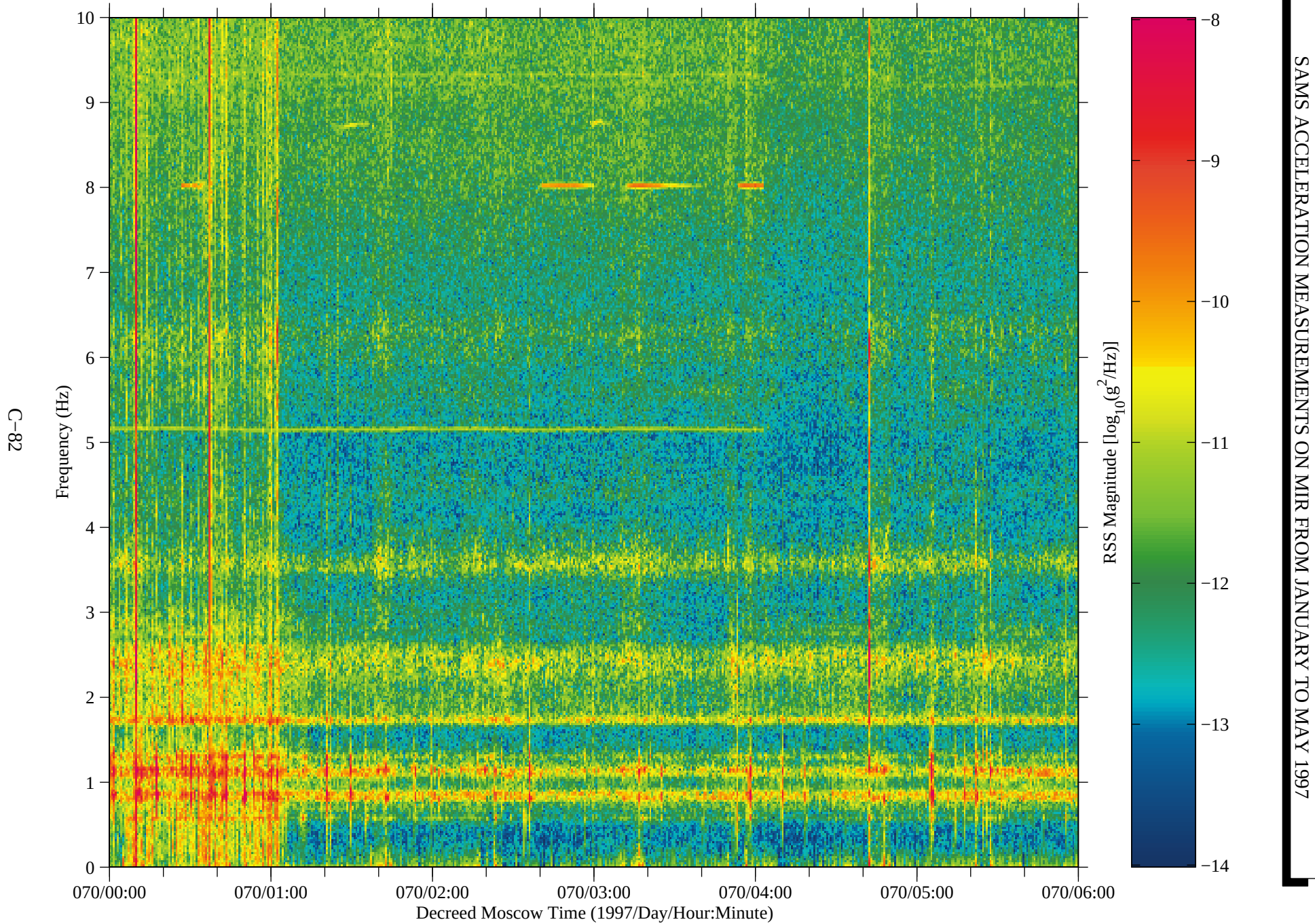
Figure 72: SAMS data from Mir, TSH B (fc=10 Hz)
