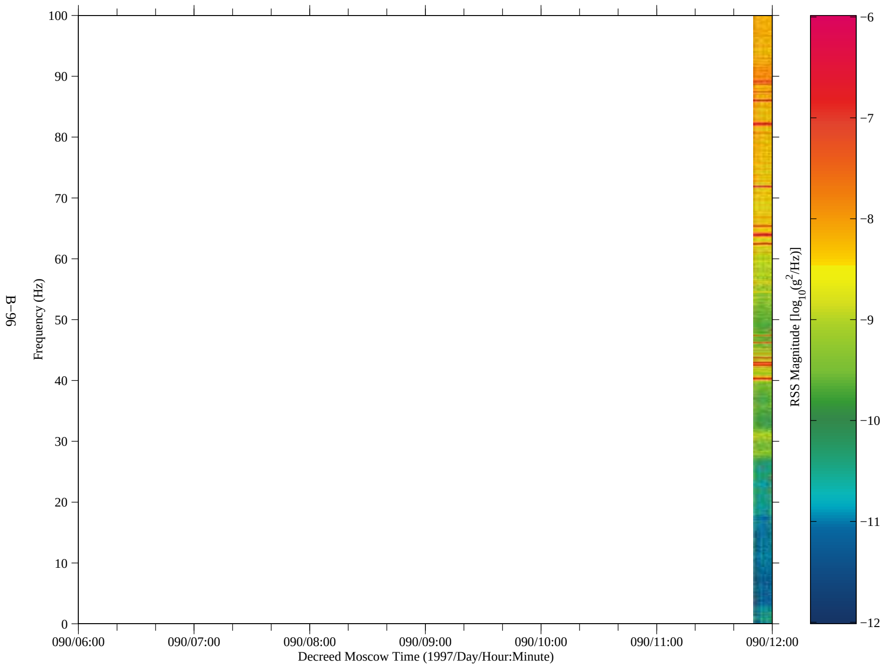
Figure 84: SAMS data from Mir, TSH A (fc=100 Hz)
