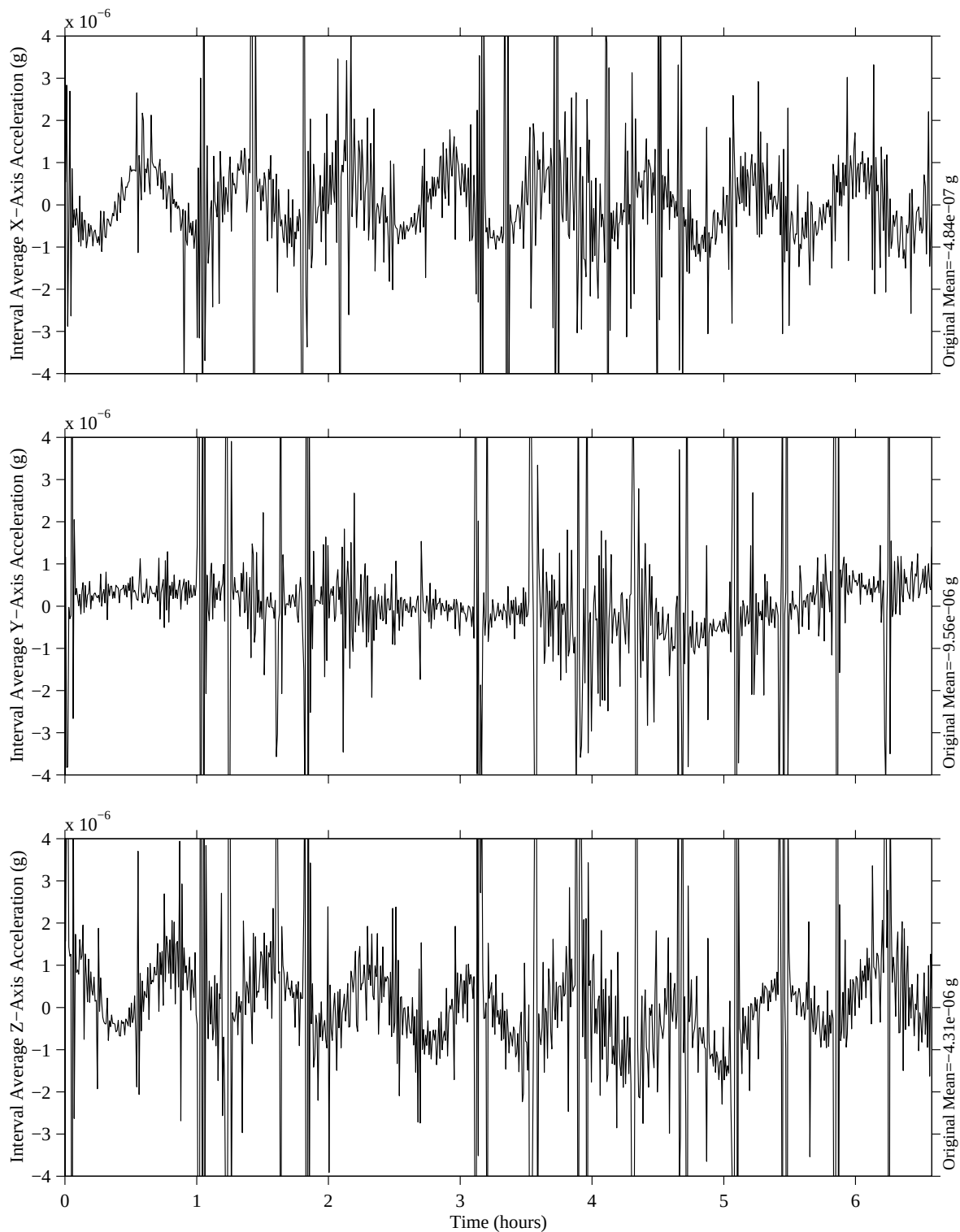
Figure 10. Earth-oriented attitude quasi-steady accelerations
