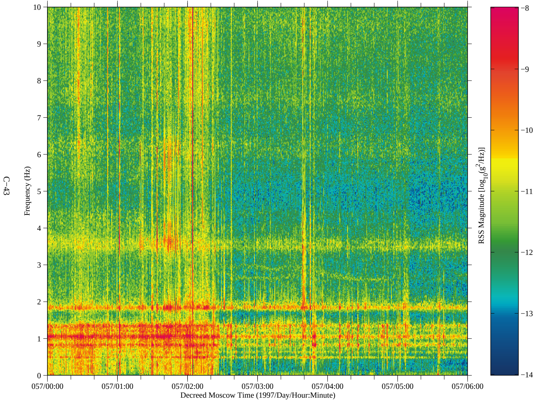
Figure 35: SAMS data from Mir, TSH B (fc=10 Hz)
