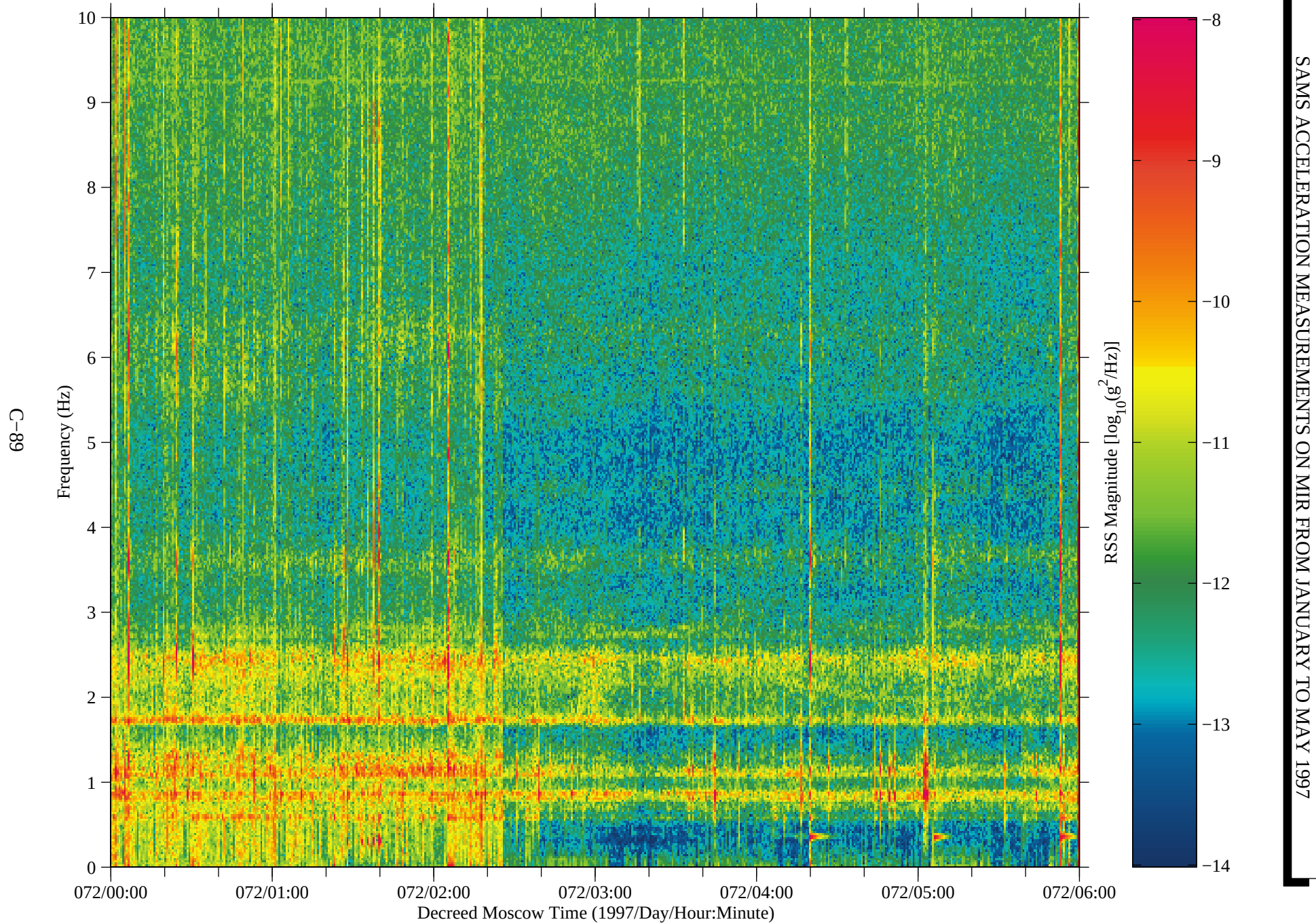
Figure 78: SAMS data from Mir, TSH B (fc=10 Hz)
