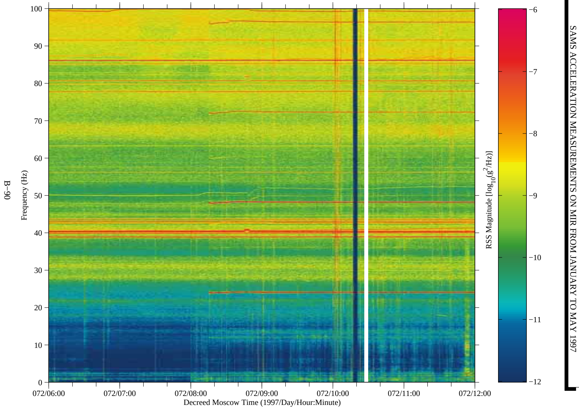
Figure 79: SAMS data from Mir, TSH A (fc=100 Hz)
