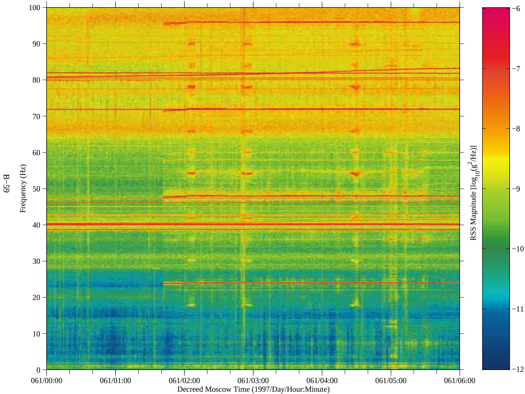
Figure 51: SAMS data from Mir, TSH A (fc=100 Hz)
