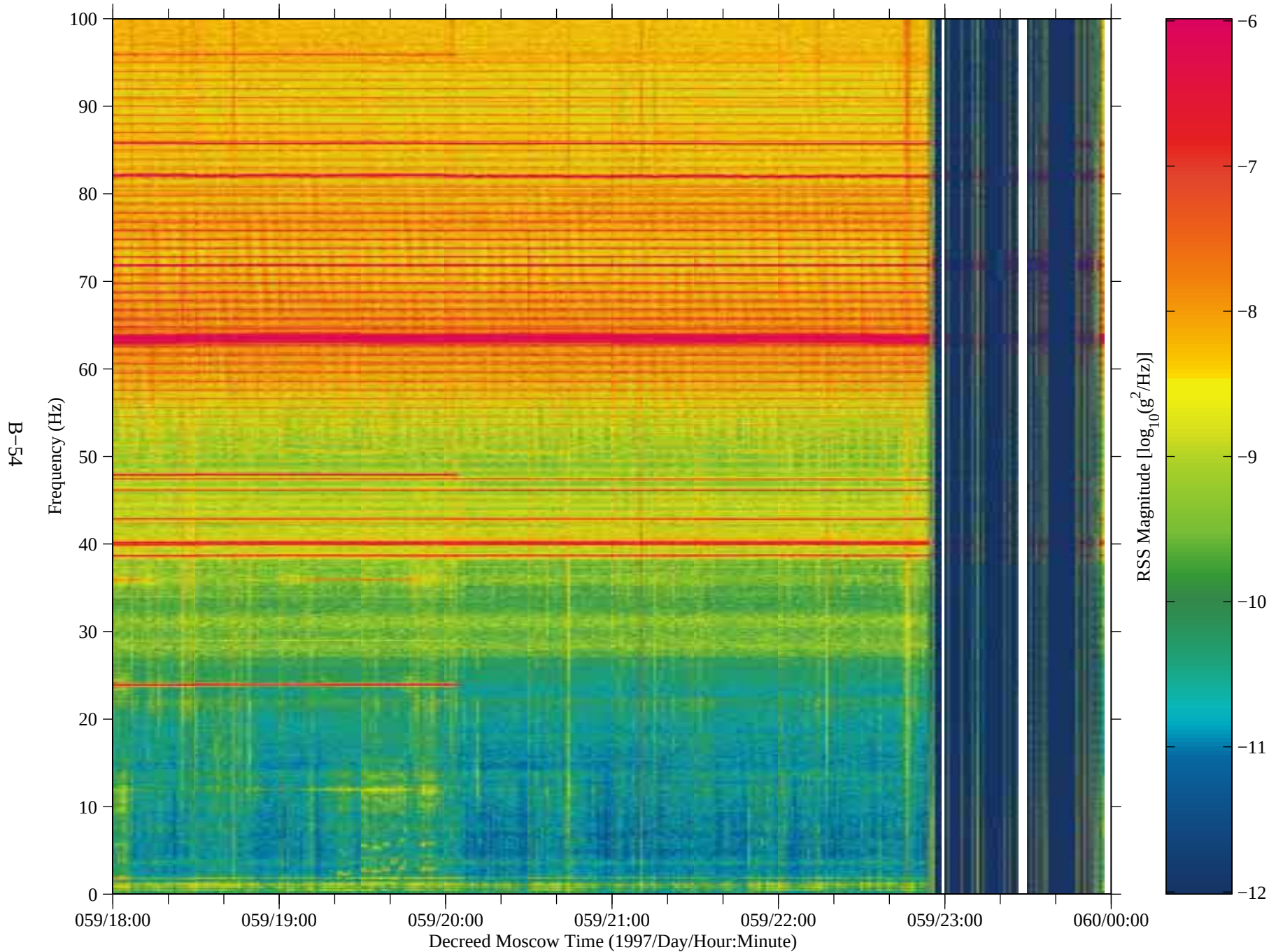
Figure 46: SAMS data from Mir, TSH A (fc=100 Hz)
