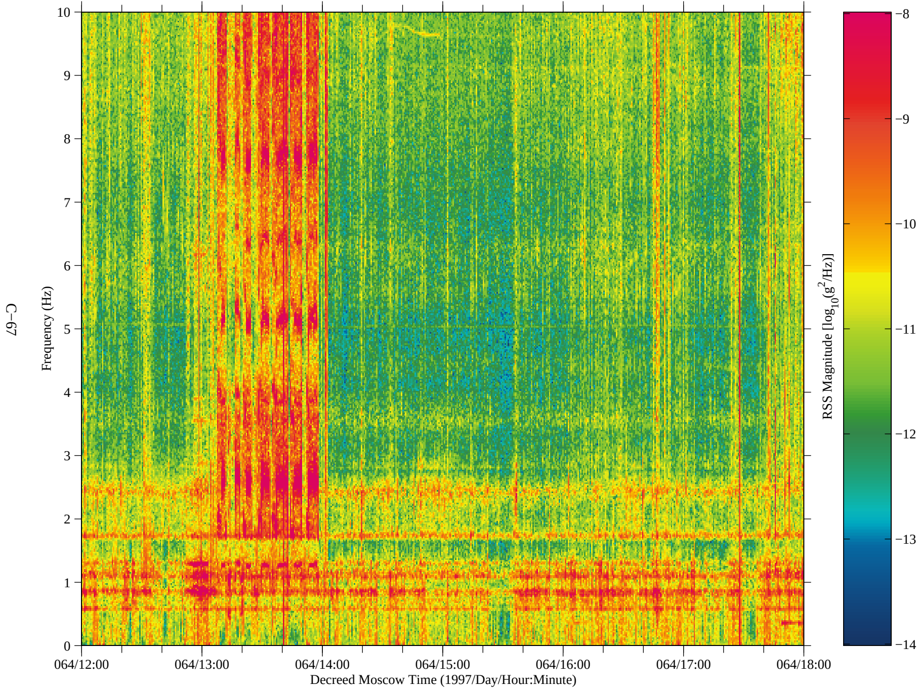
Figure 58: SAMS data from Mir, TSH B (fc=10 Hz)
