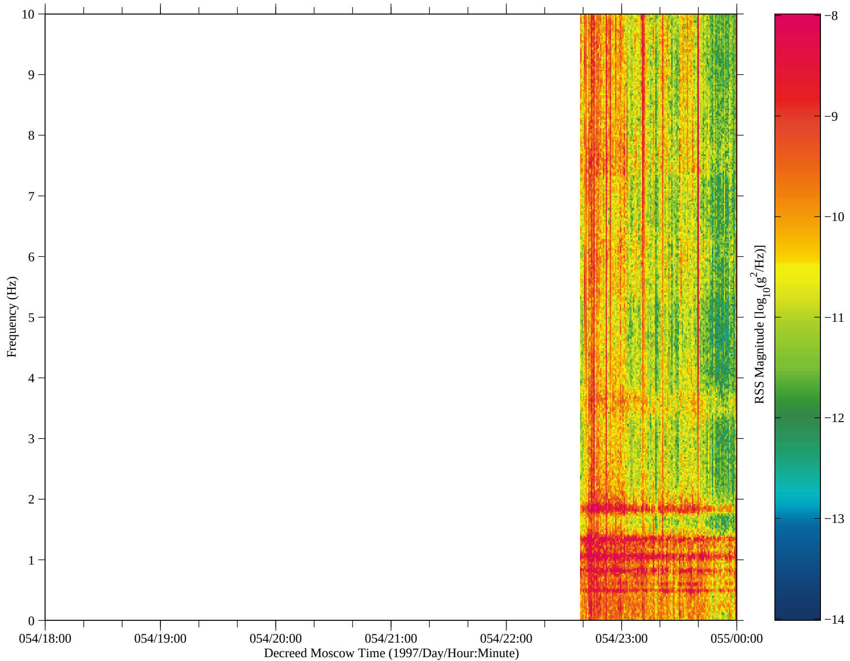
Figure 27: SAMS data from Mir, TSH B (fc=10 Hz)
