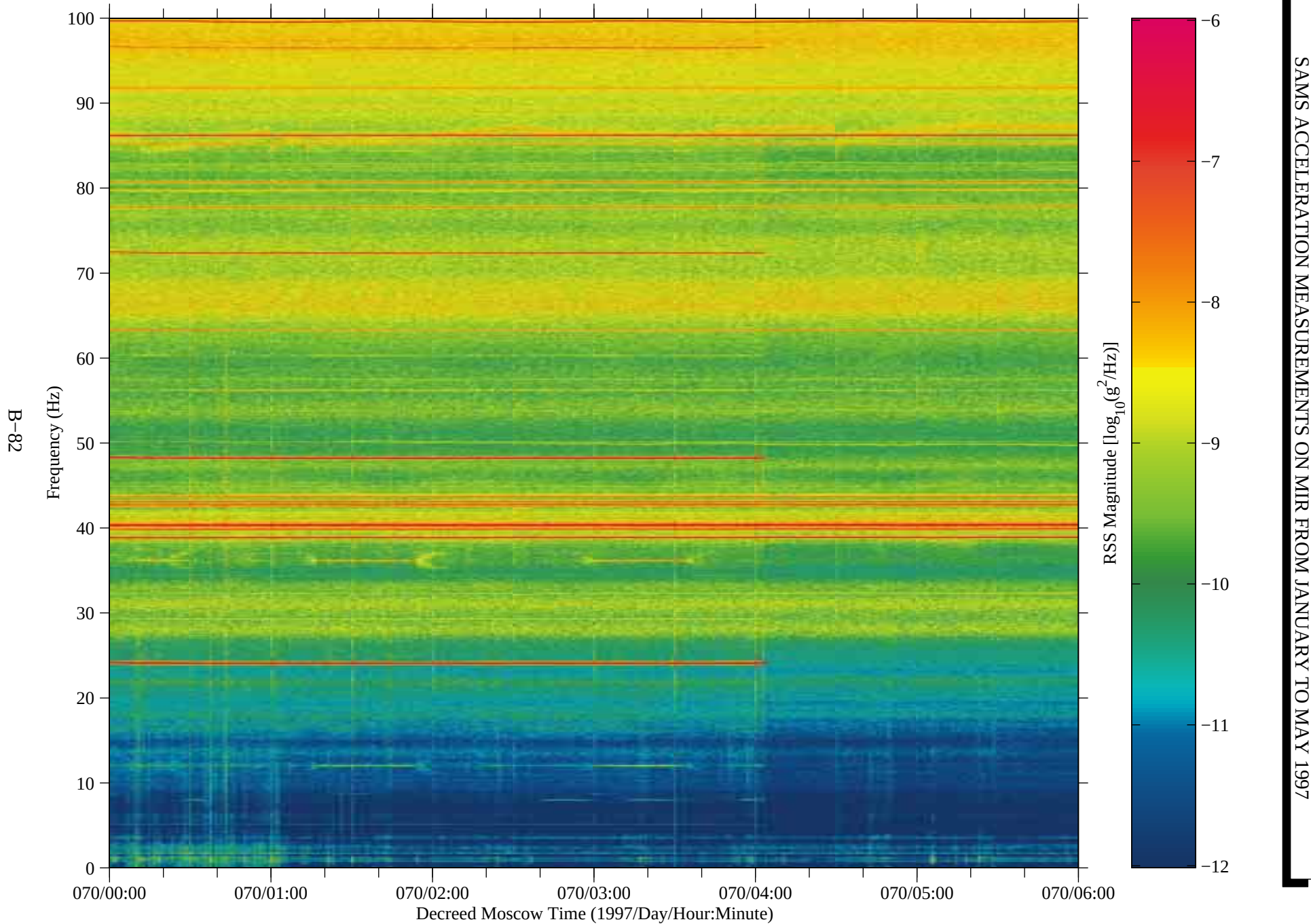
Figure 72: SAMS data from Mir, TSH A (fc=100 Hz)
