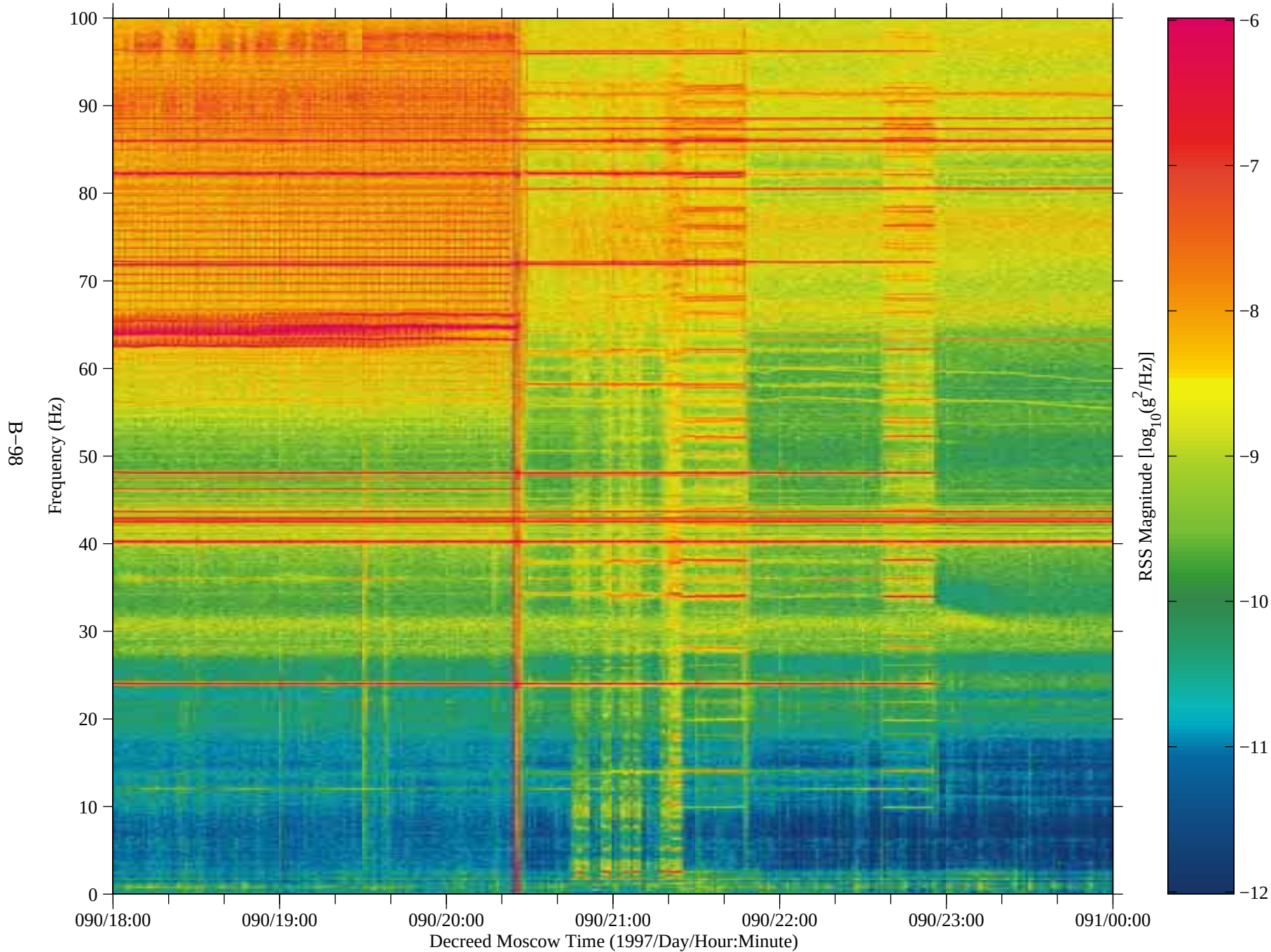
Figure 86: SAMS data from Mir, TSH A (fc=100 Hz)
