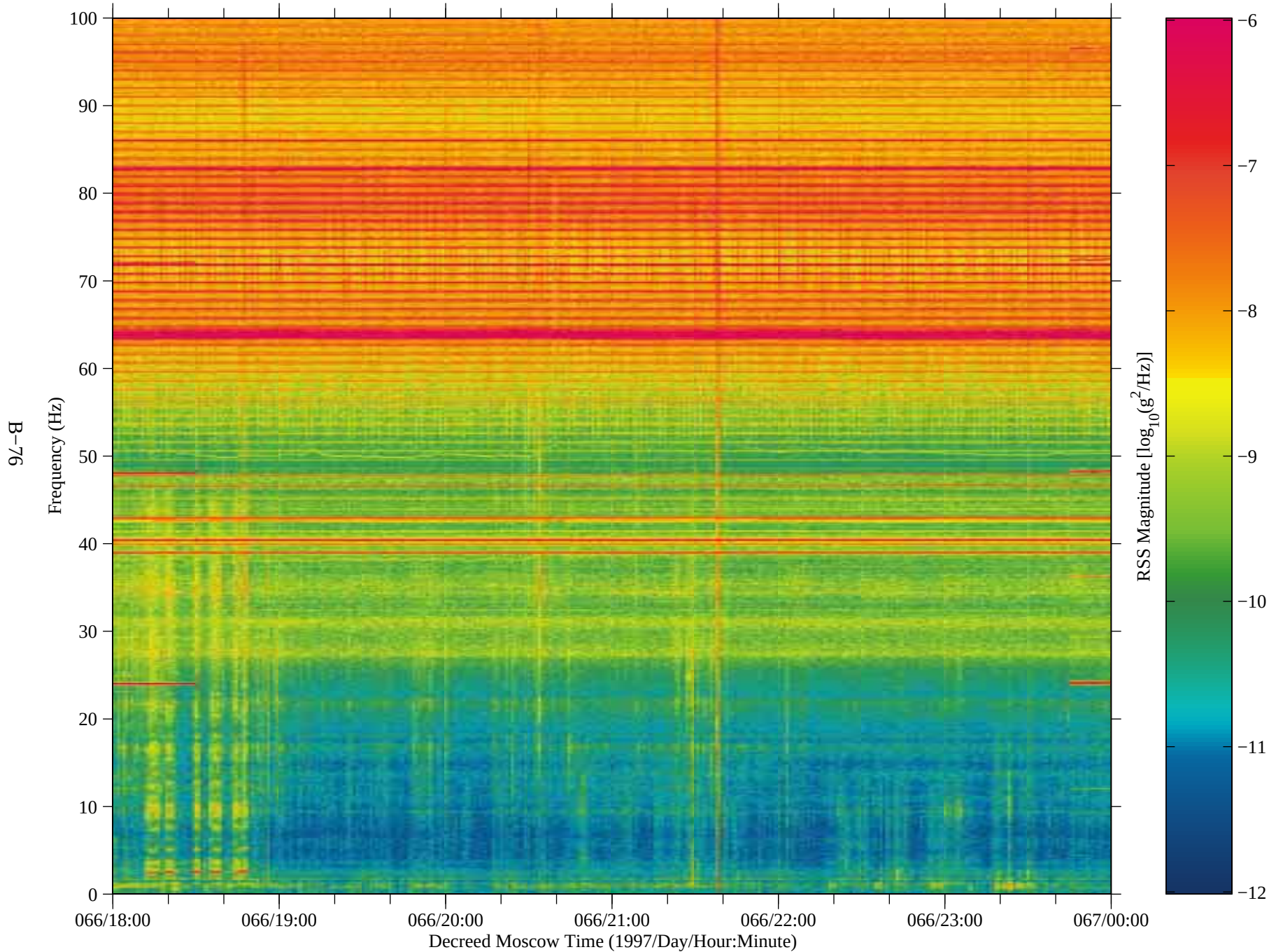
Figure 67: SAMS data from Mir, TSH A (fc=100 Hz)
