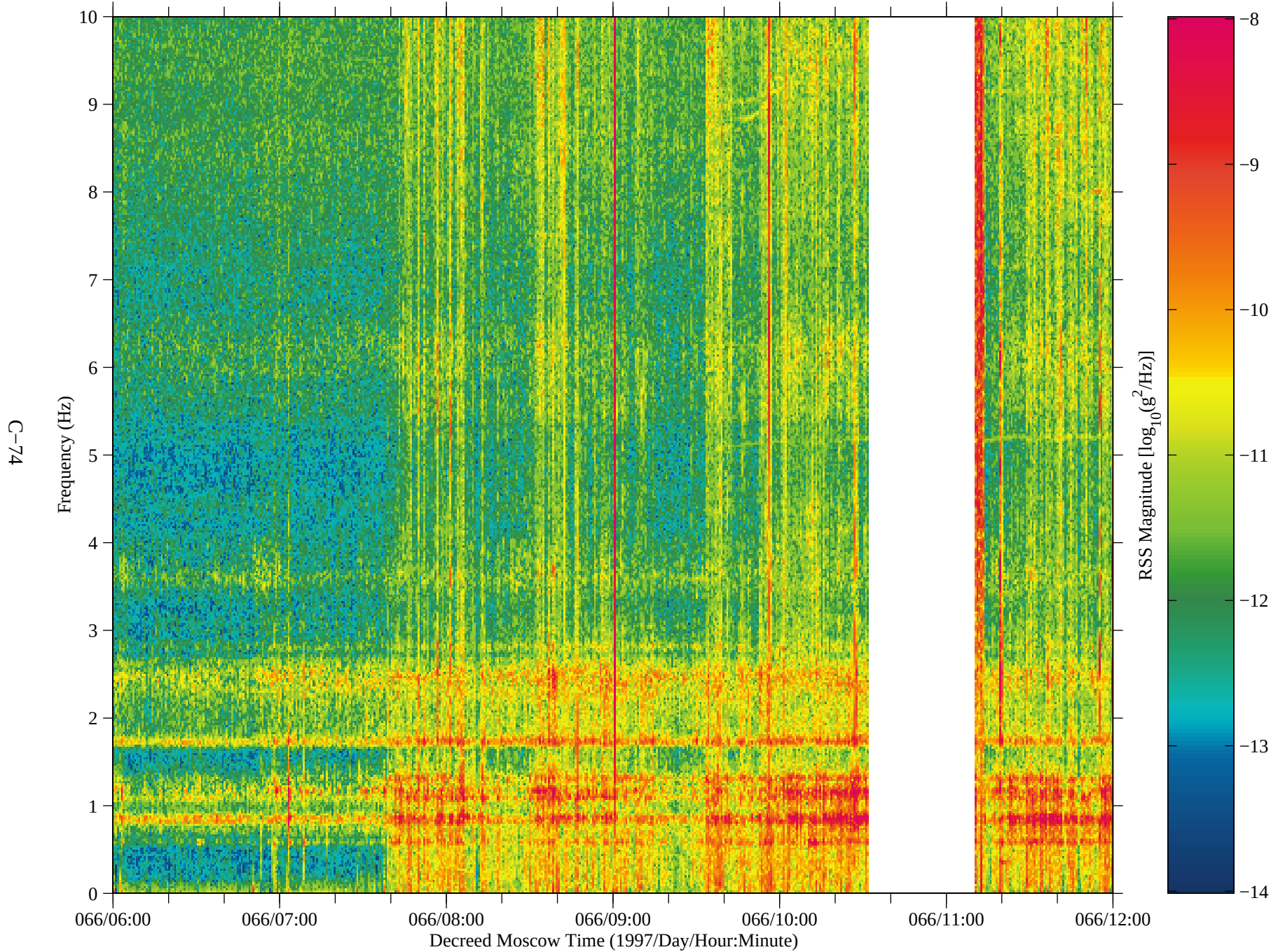
Figure 65: SAMS data from Mir, TSH B (fc=10 Hz)
