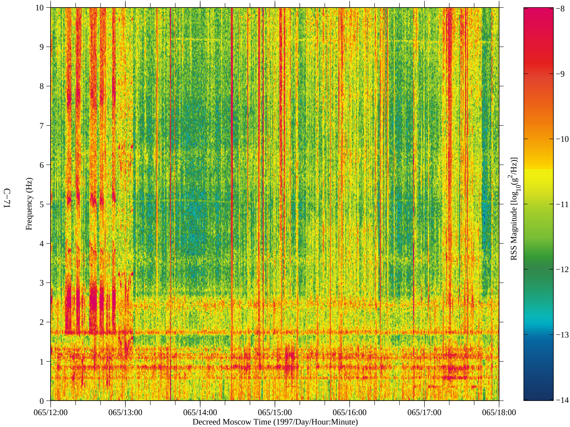
Figure 62: SAMS data from Mir, TSH B (fc=10 Hz)
