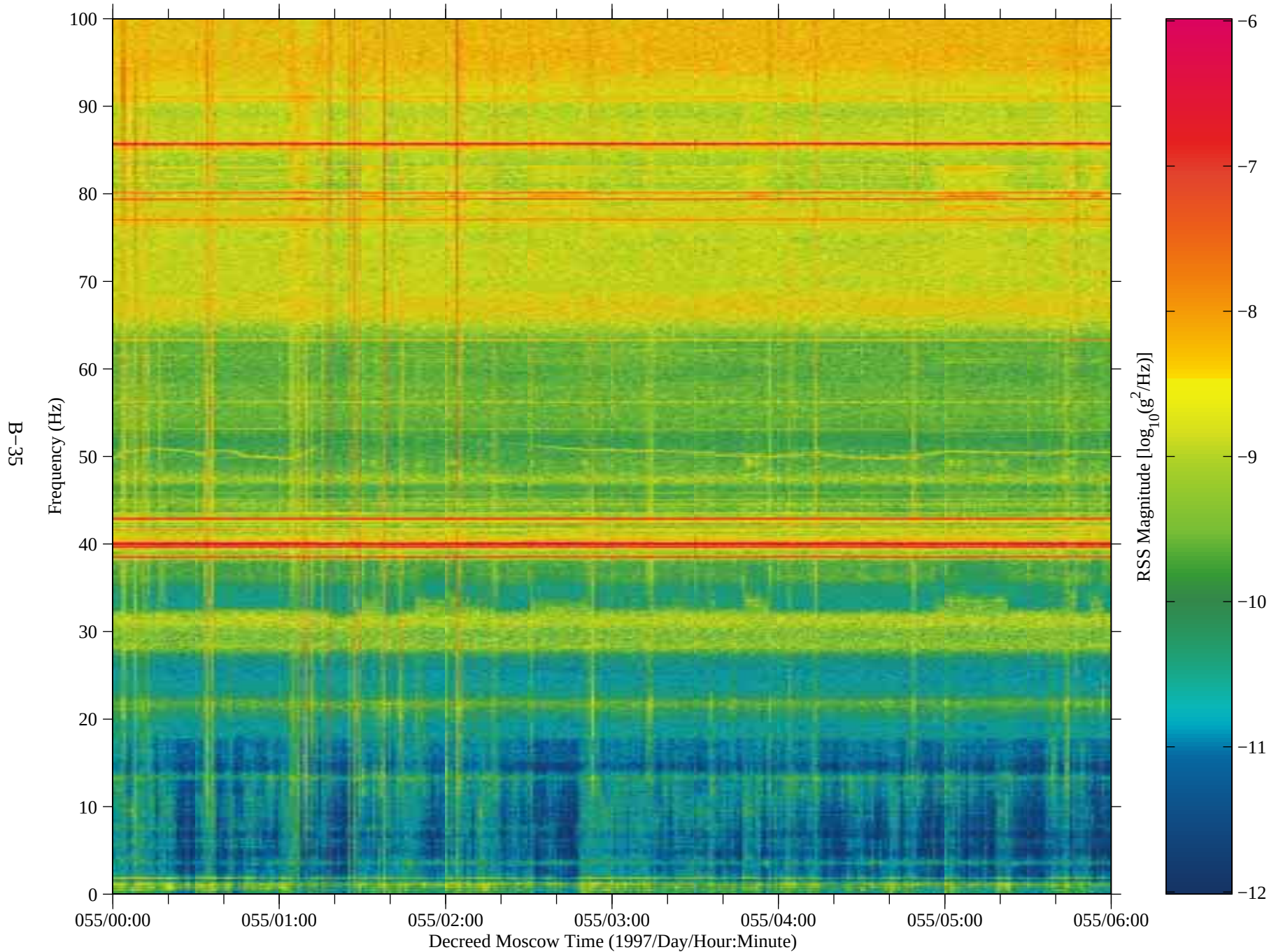
Figure 28: SAMS data from Mir, TSH A (fc=100 Hz)
