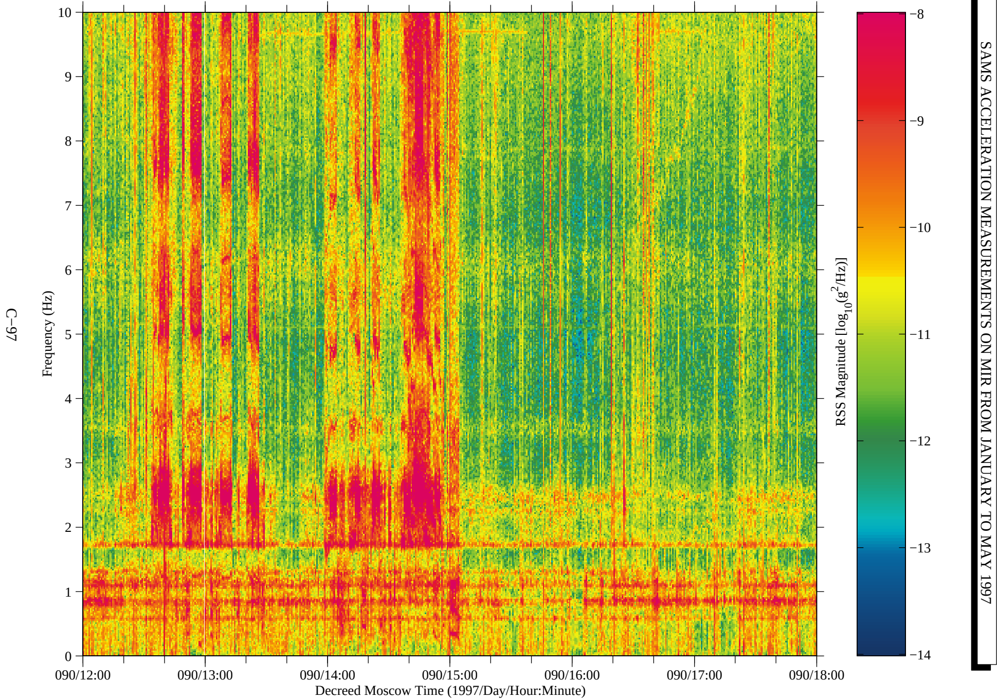
Figure 85: SAMS data from Mir, TSH B (fc=10 Hz)
