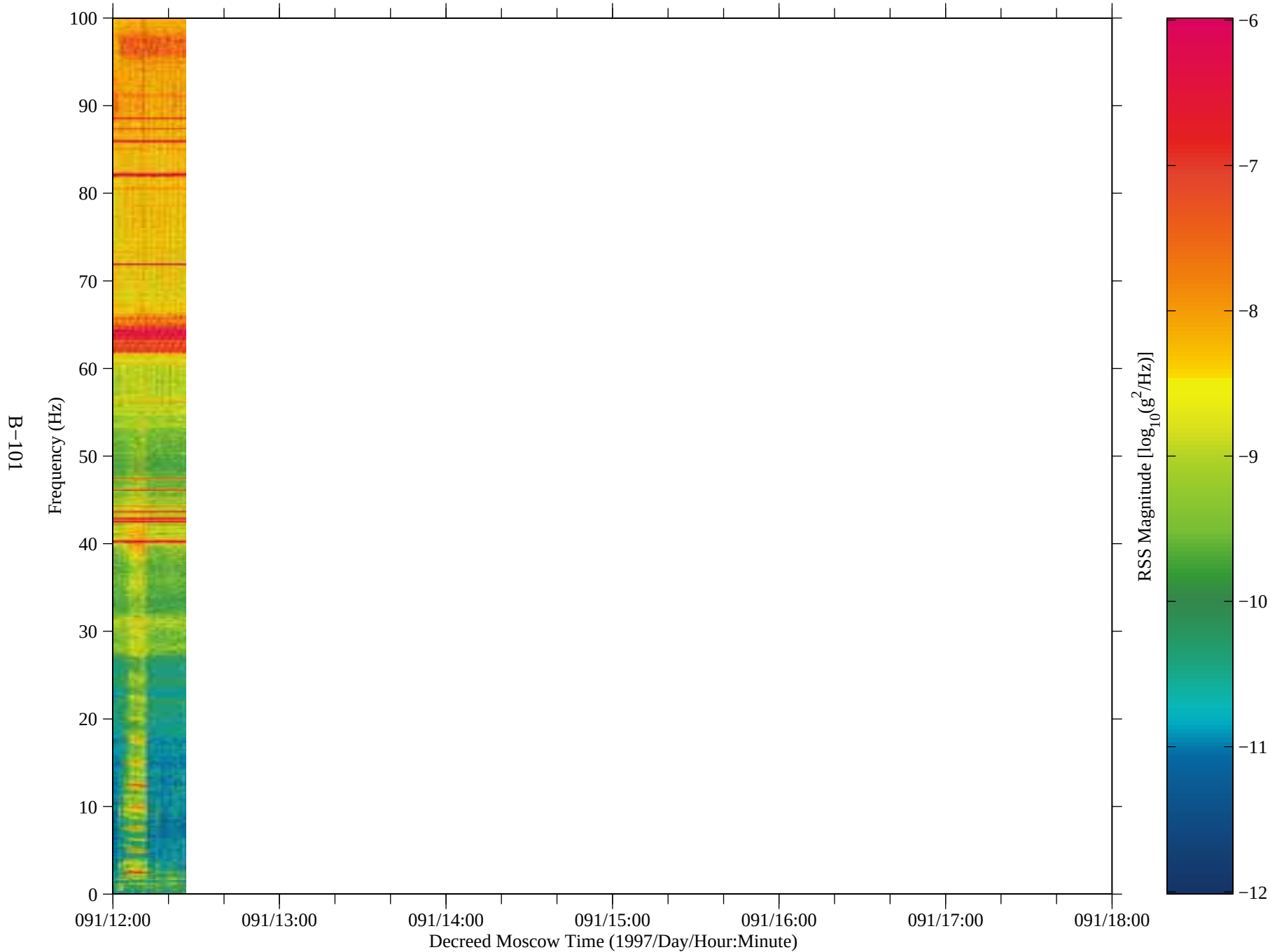
Figure 89: SAMS data from Mir, TSH A (fc=100 Hz)
