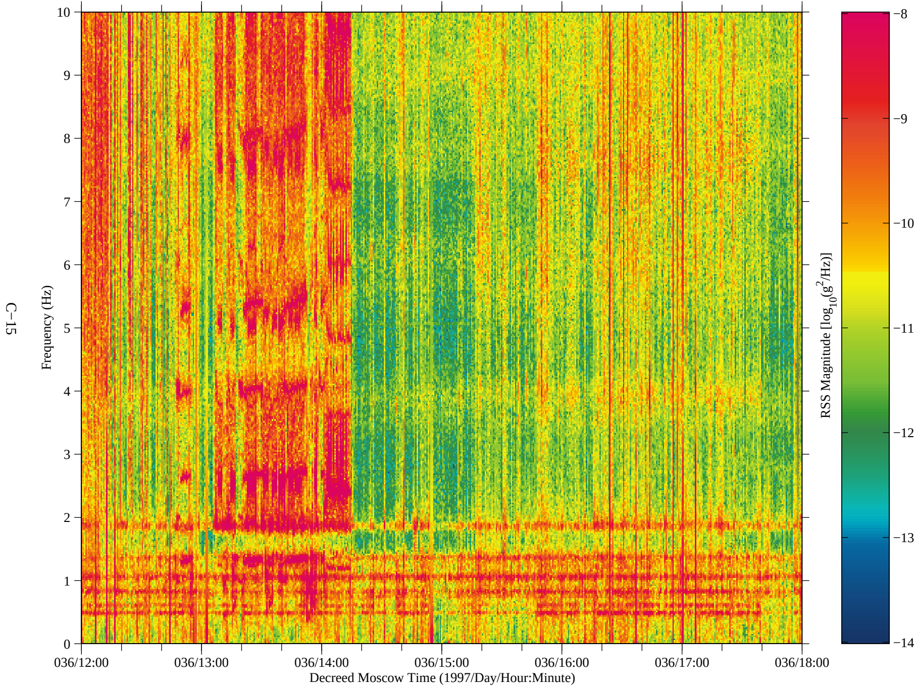
Figure 11: SAMS data from Mir, TSH B (fc=10 Hz)
