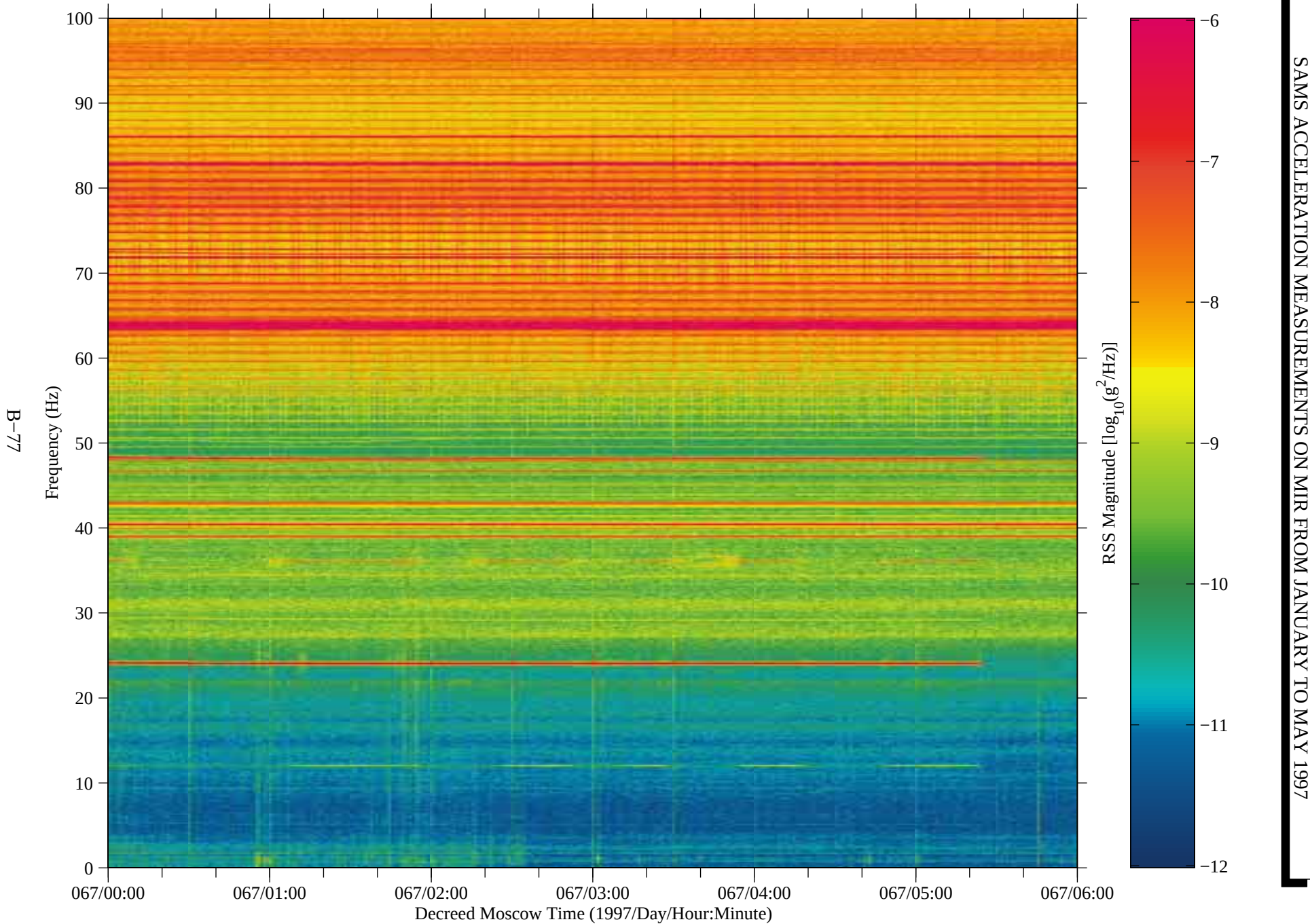
Figure 68: SAMS data from Mir, TSH A (fc=100 Hz)
