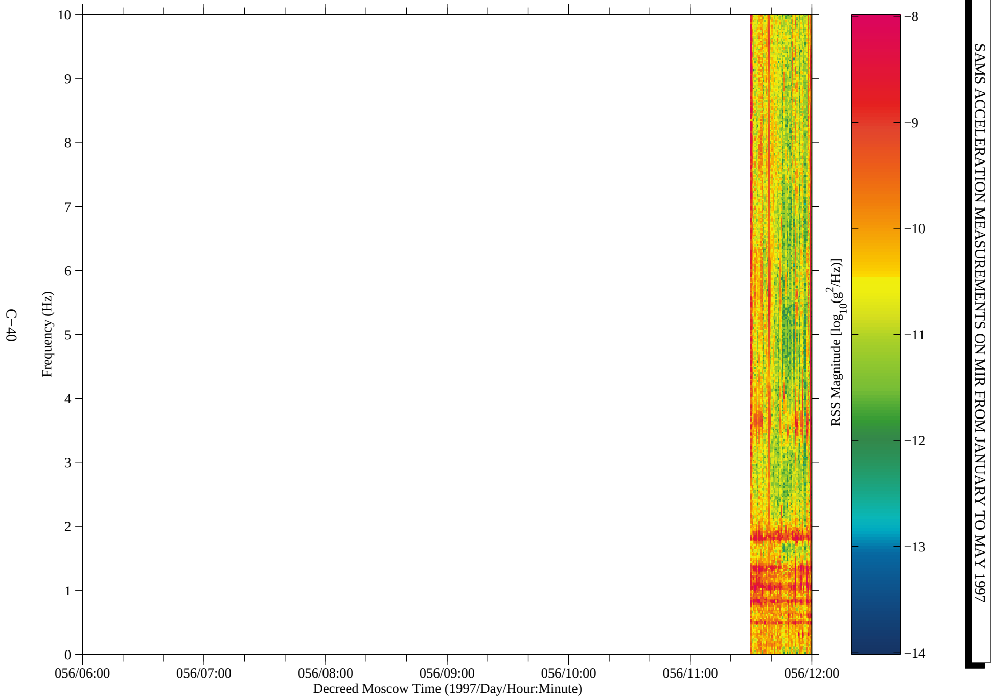
Figure 32: SAMS data from Mir, TSH B (fc=10 Hz)
