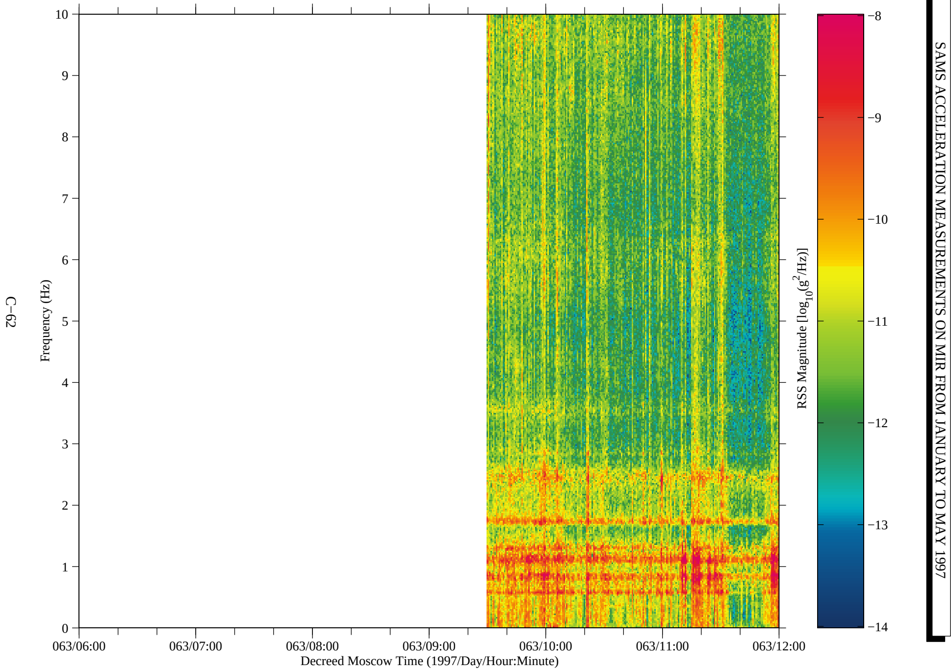
Figure 53: SAMS data from Mir, TSH B (fc=10 Hz)
