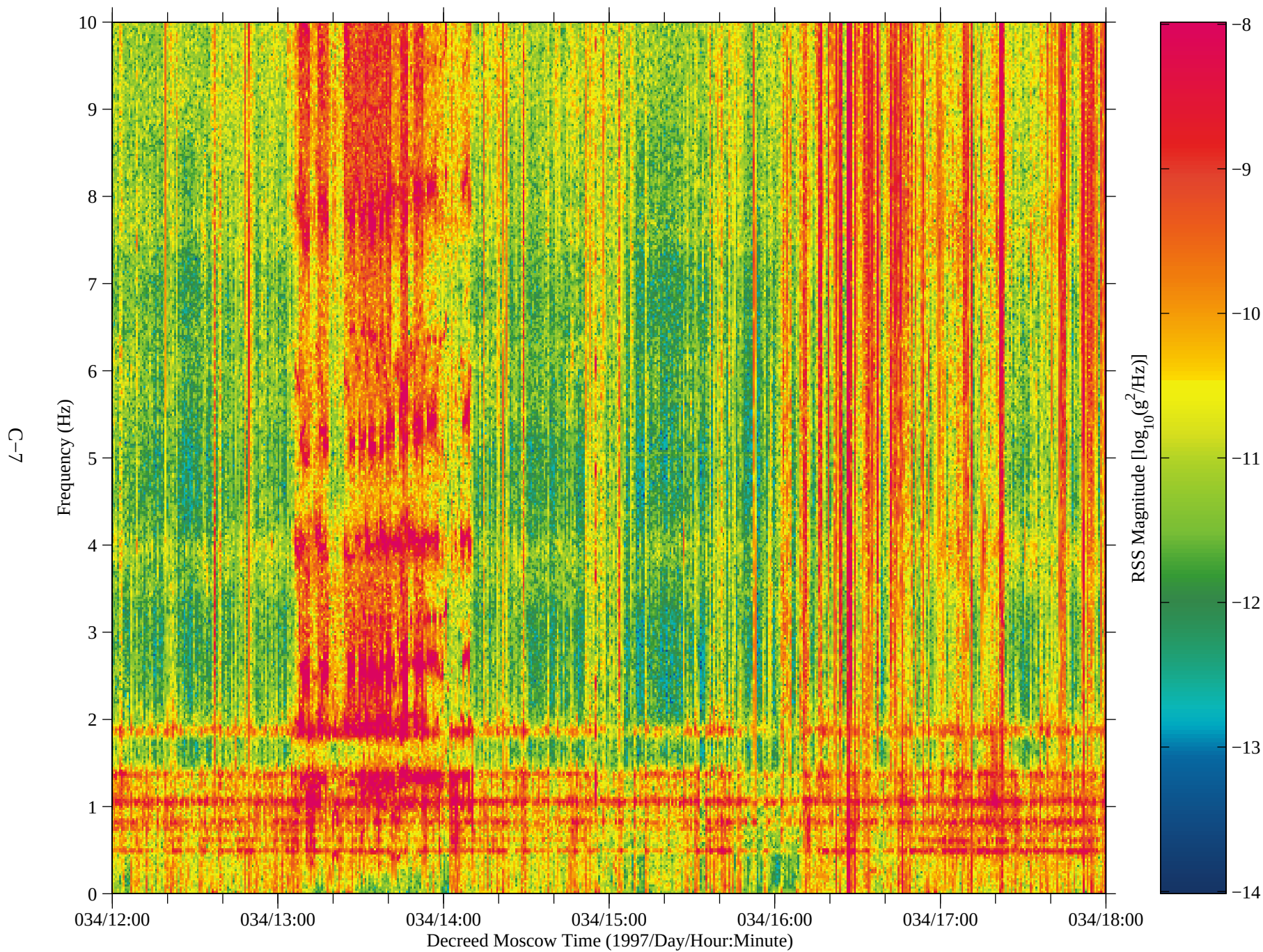
Figure 3: SAMS data from Mir, TSH B (fc=10 Hz)
