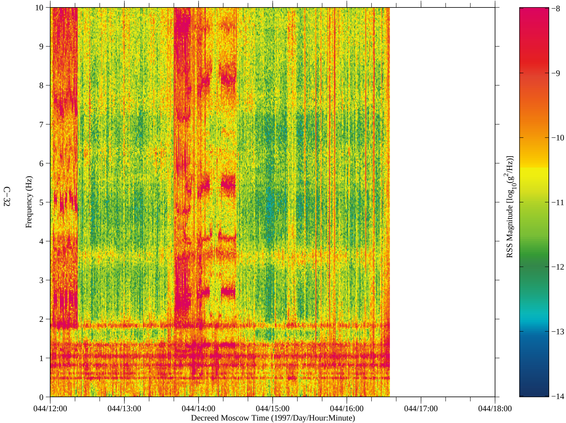
Figure 26: SAMS data from Mir, TSH B (fc=10 Hz)
