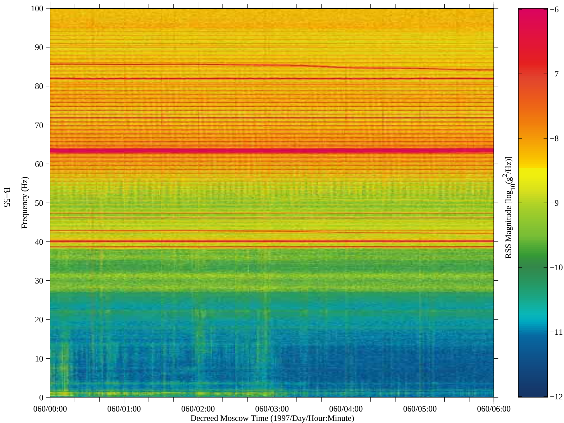
Figure 47: SAMS data from Mir, TSH A (fc=100 Hz)
