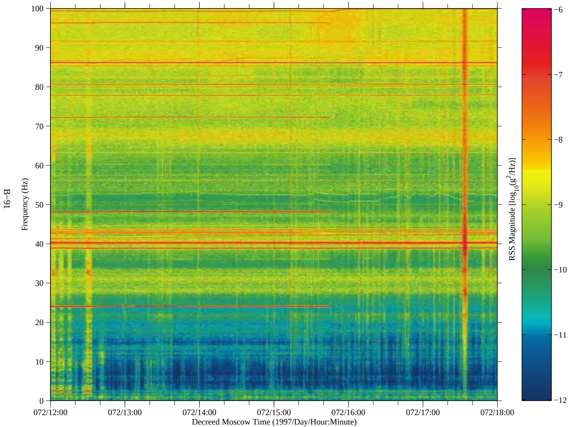
Figure 80: SAMS data from Mir, TSH A (fc=100 Hz)
