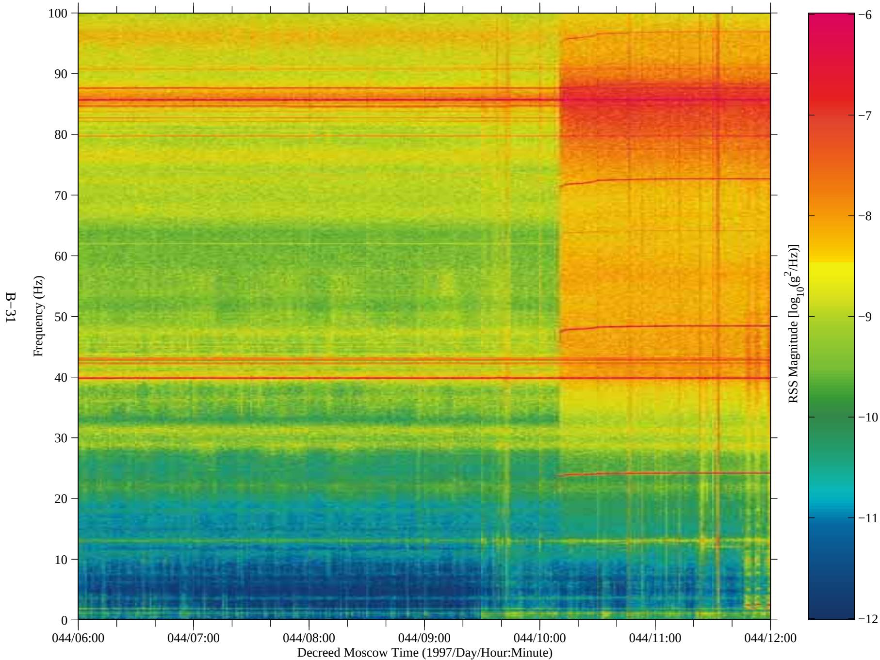
Figure 25: SAMS data from Mir, TSH A (fc=100 Hz)
