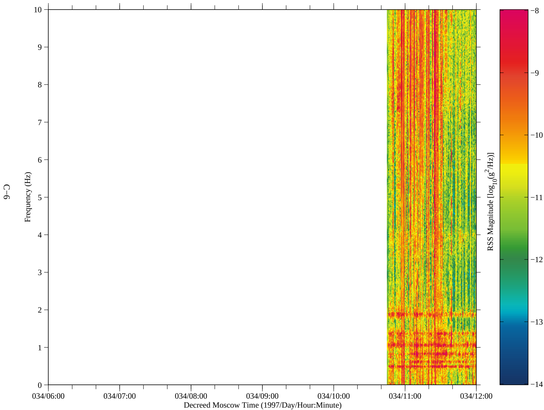
Figure 2: SAMS data from Mir, TSH B (fc=10 Hz)
