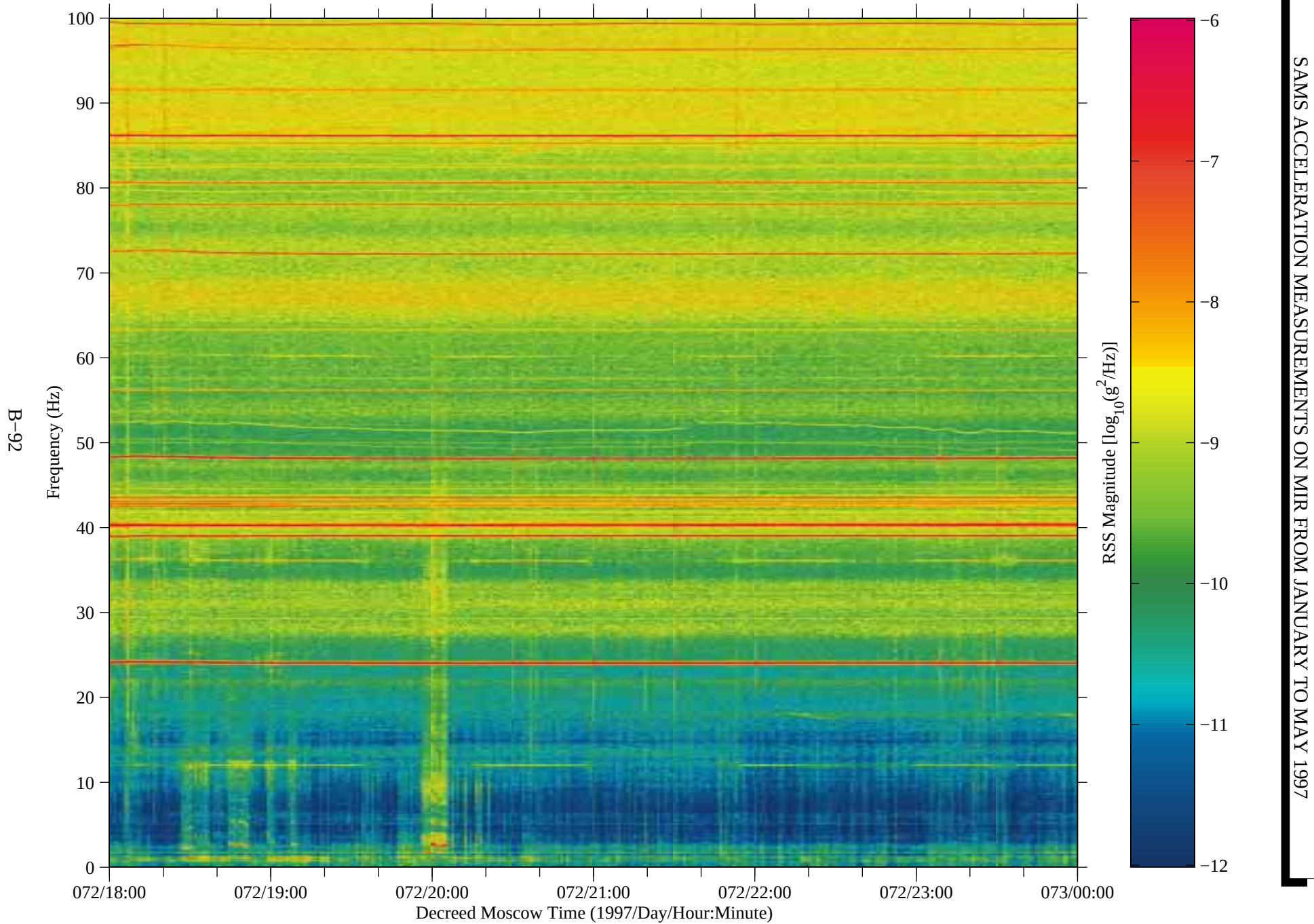
Figure 81: SAMS data from Mir, TSH A (fc=100 Hz)
