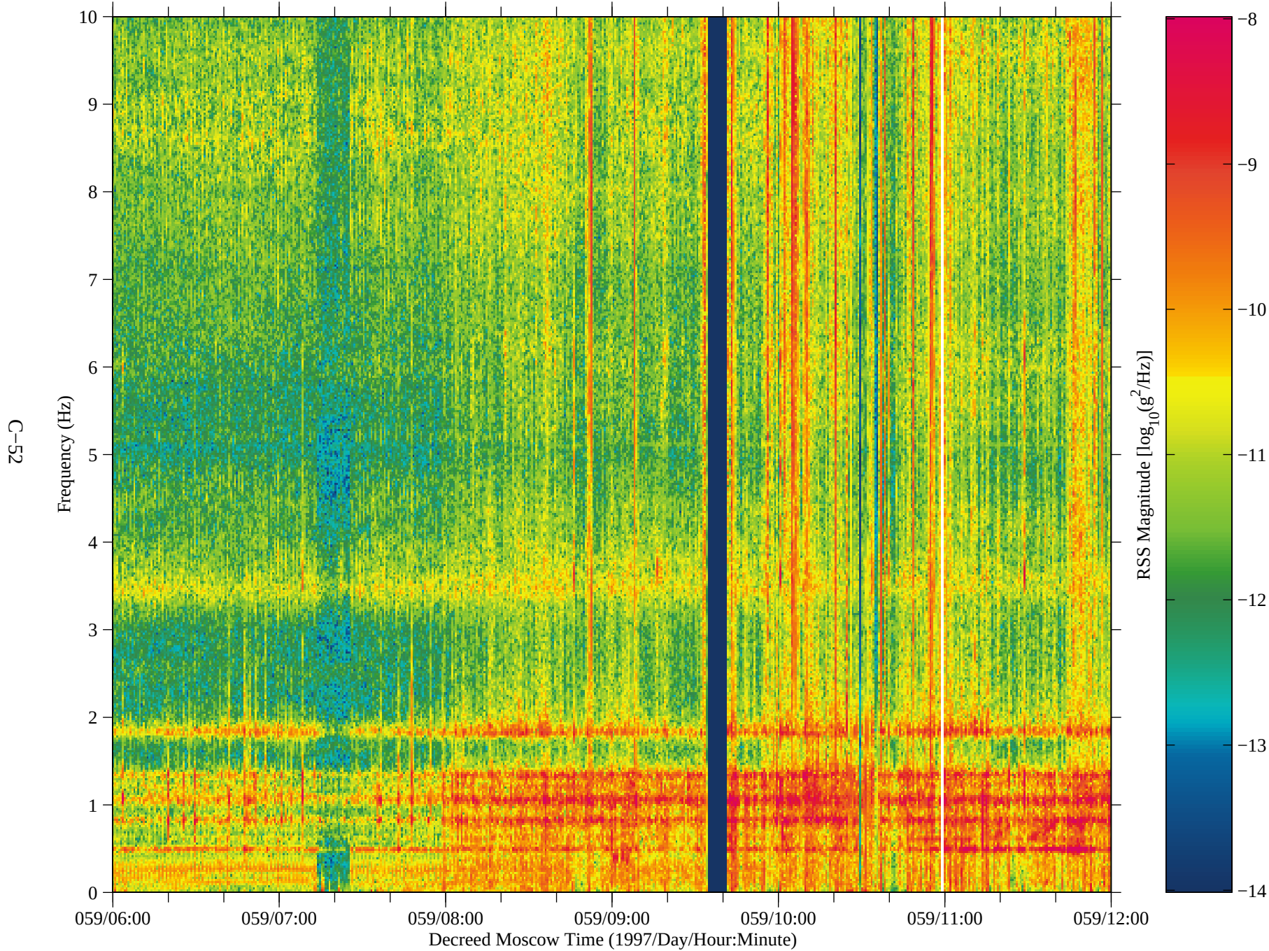
Figure 44: SAMS data from Mir, TSH B (fc=10 Hz)
