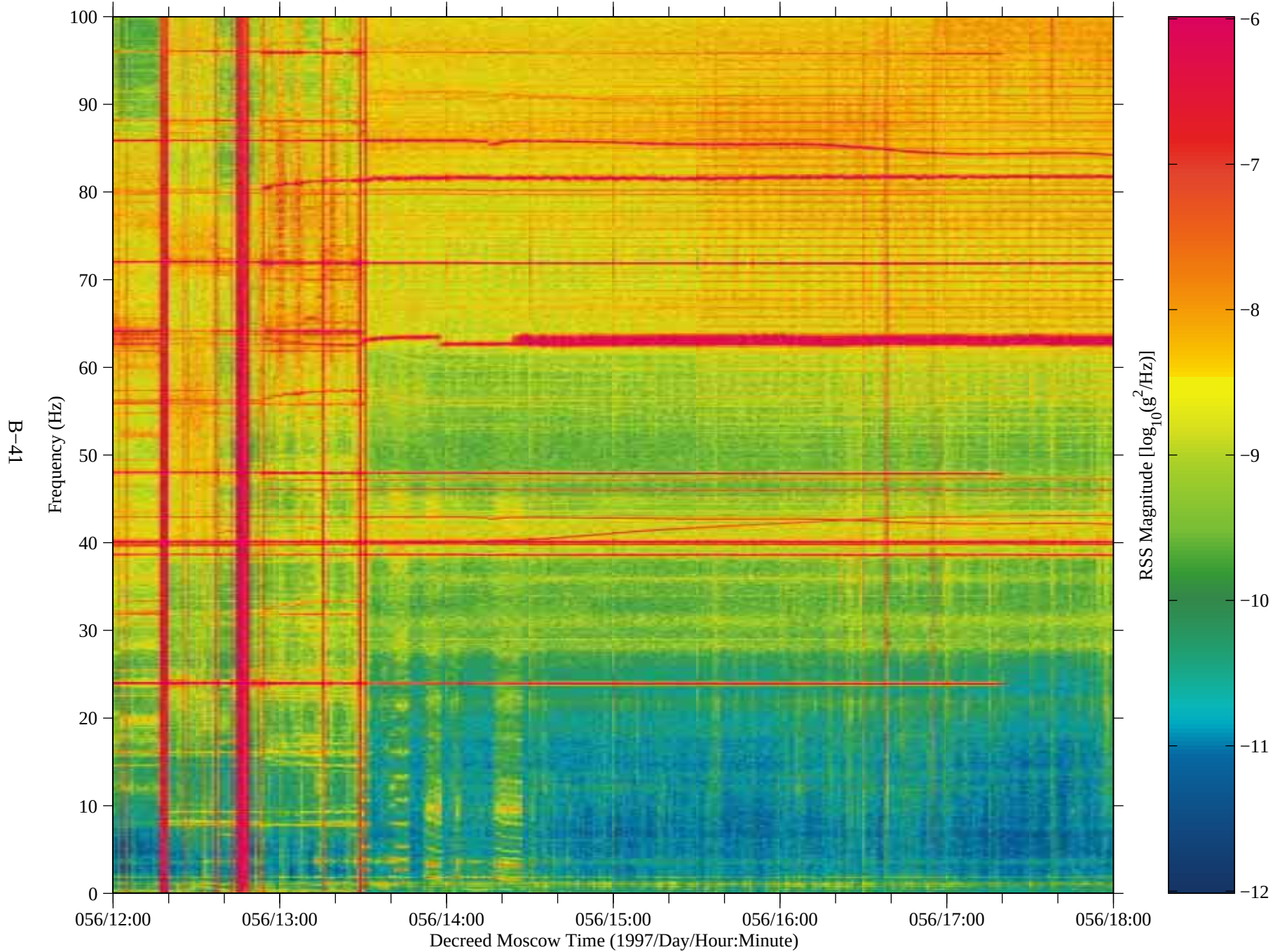
Figure 33: SAMS data from Mir, TSH A (fc=100 Hz)
