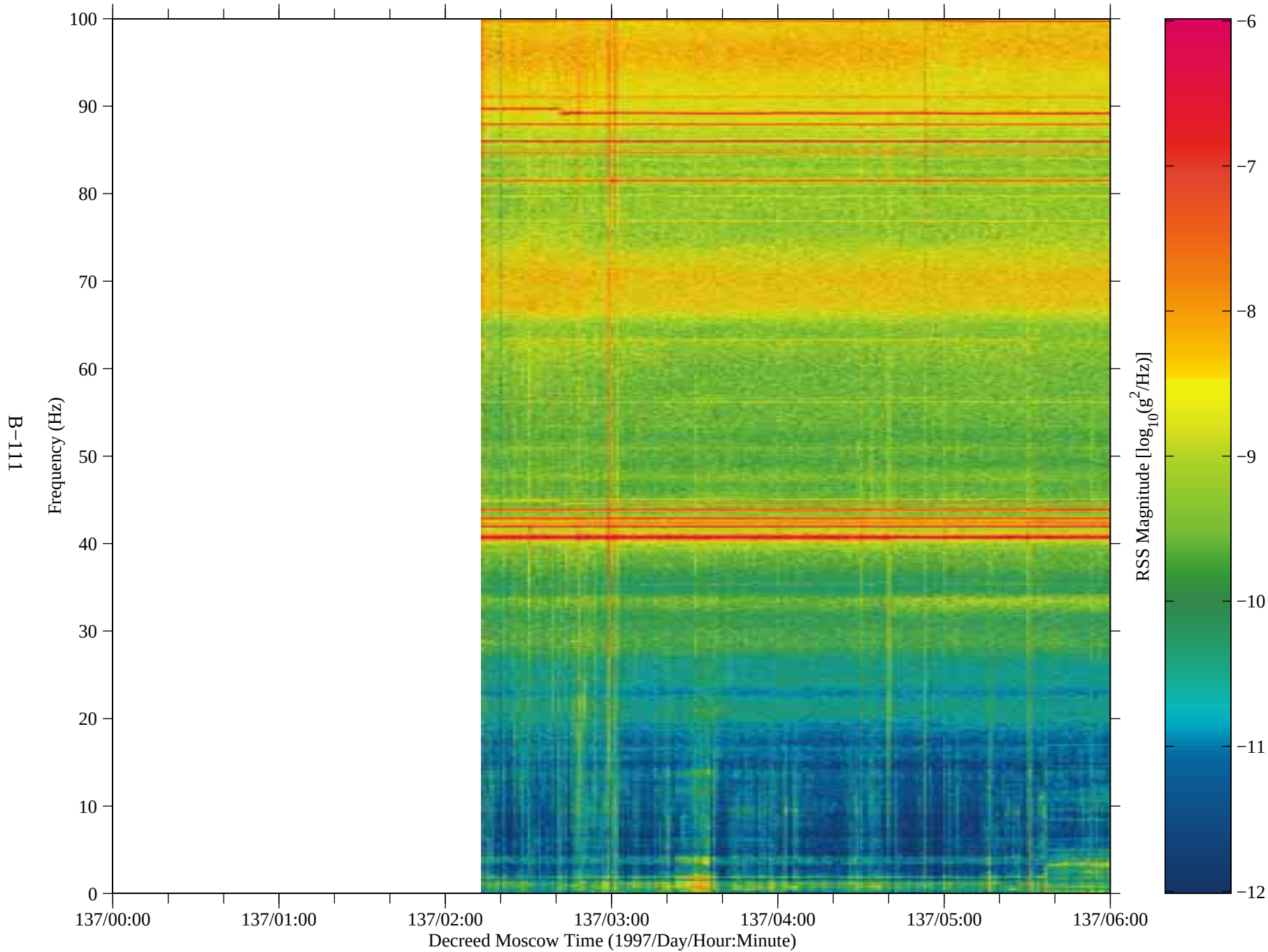
Figure 96: SAMS data from Mir, TSH A (fc=100 Hz)
