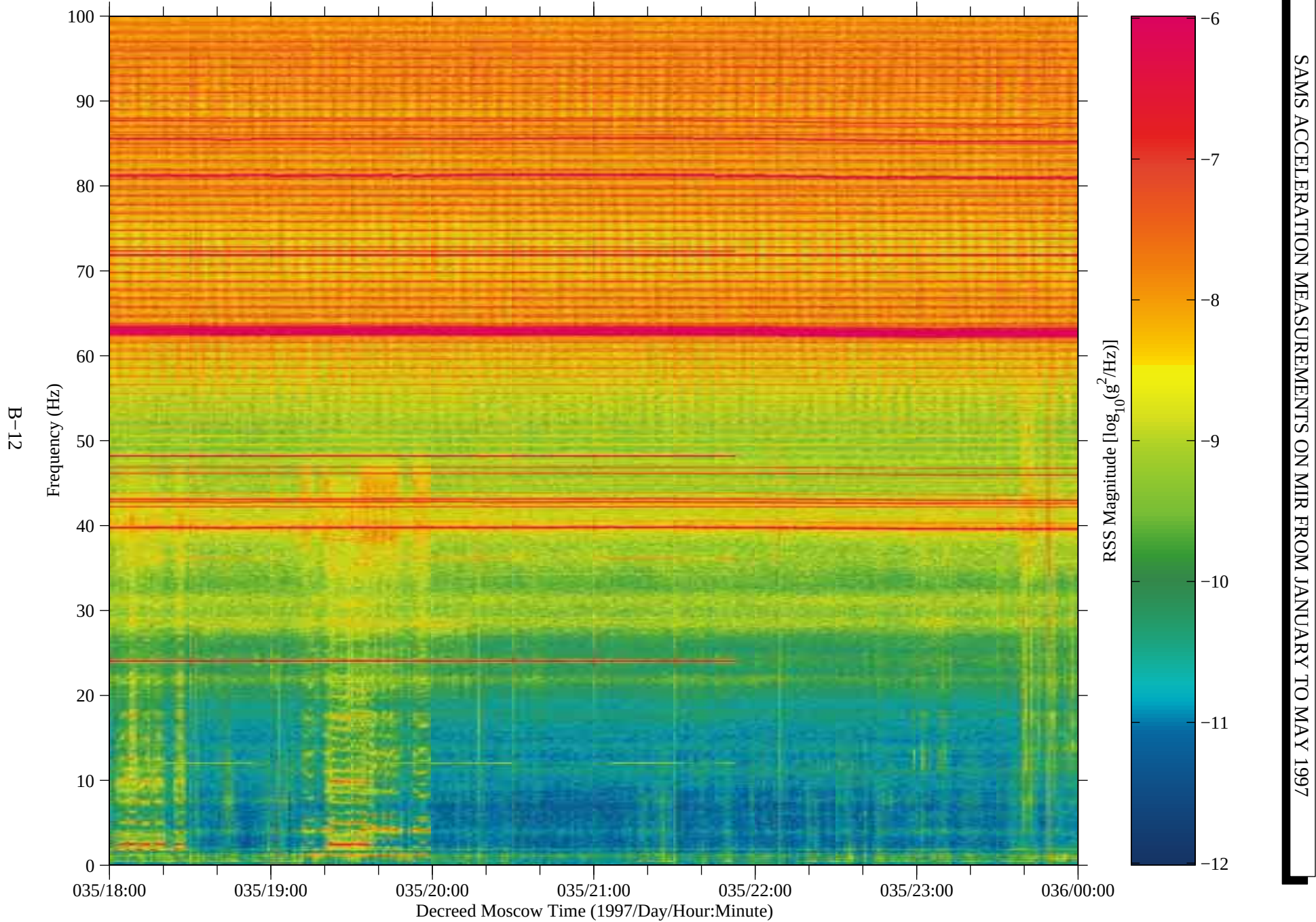
Figure 8: SAMS data from Mir, TSH A (fc=100 Hz)
