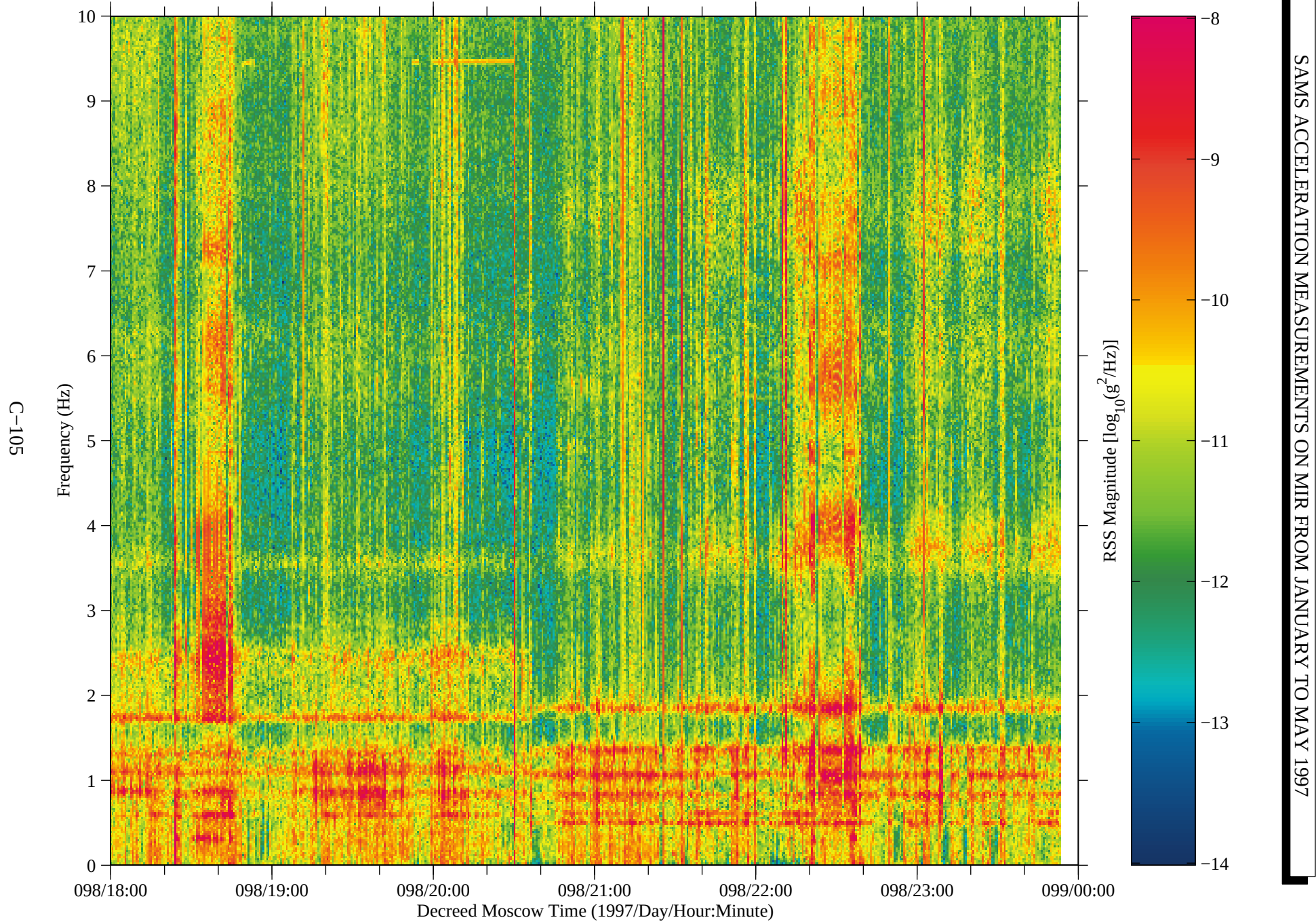
Figure 92: SAMS data from Mir, TSH B (fc=10 Hz)
