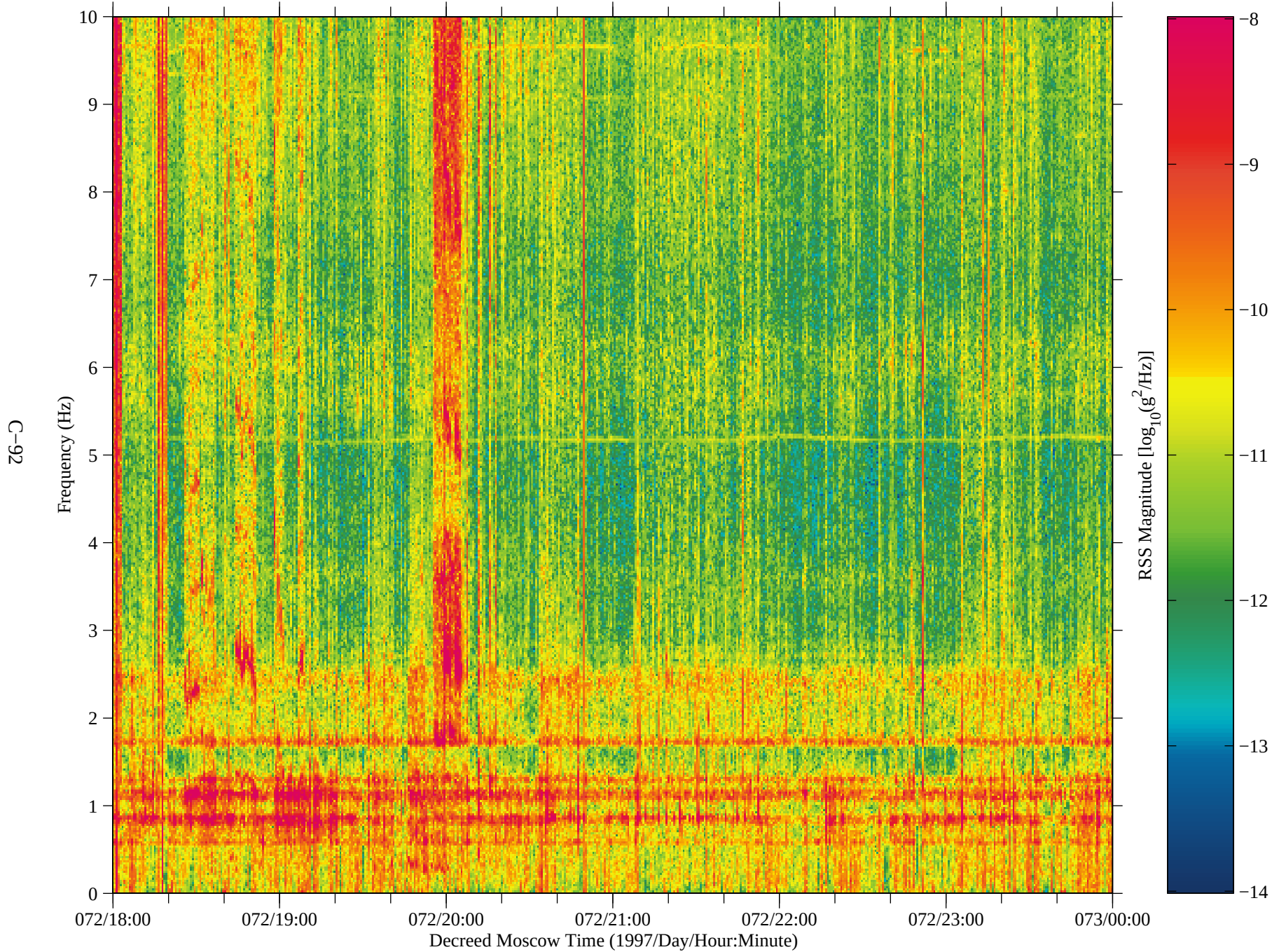
Figure 81: SAMS data from Mir, TSH B (fc=10 Hz)
