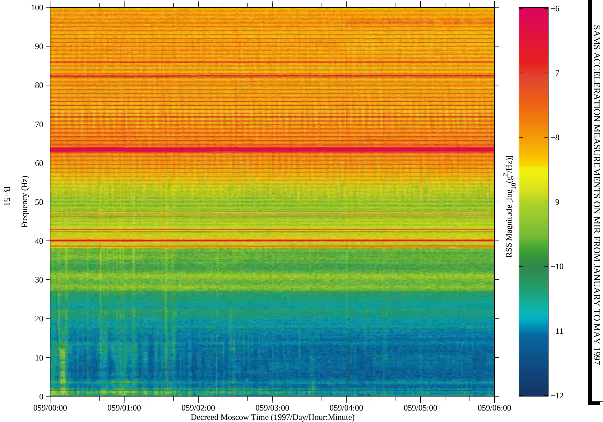
Figure 43: SAMS data from Mir, TSH A (fc=100 Hz)
