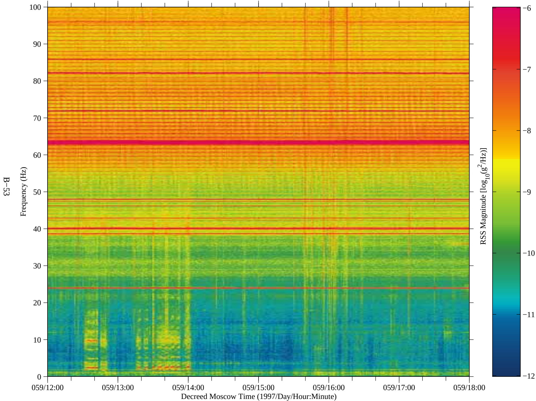
Figure 45: SAMS data from Mir, TSH A (fc=100 Hz)
