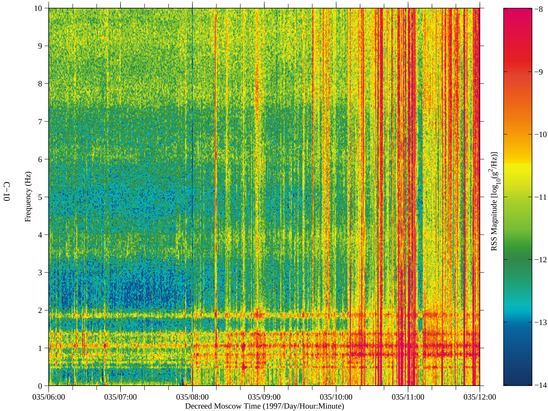
Figure 6: SAMS data from Mir, TSH B (fc=10 Hz)
