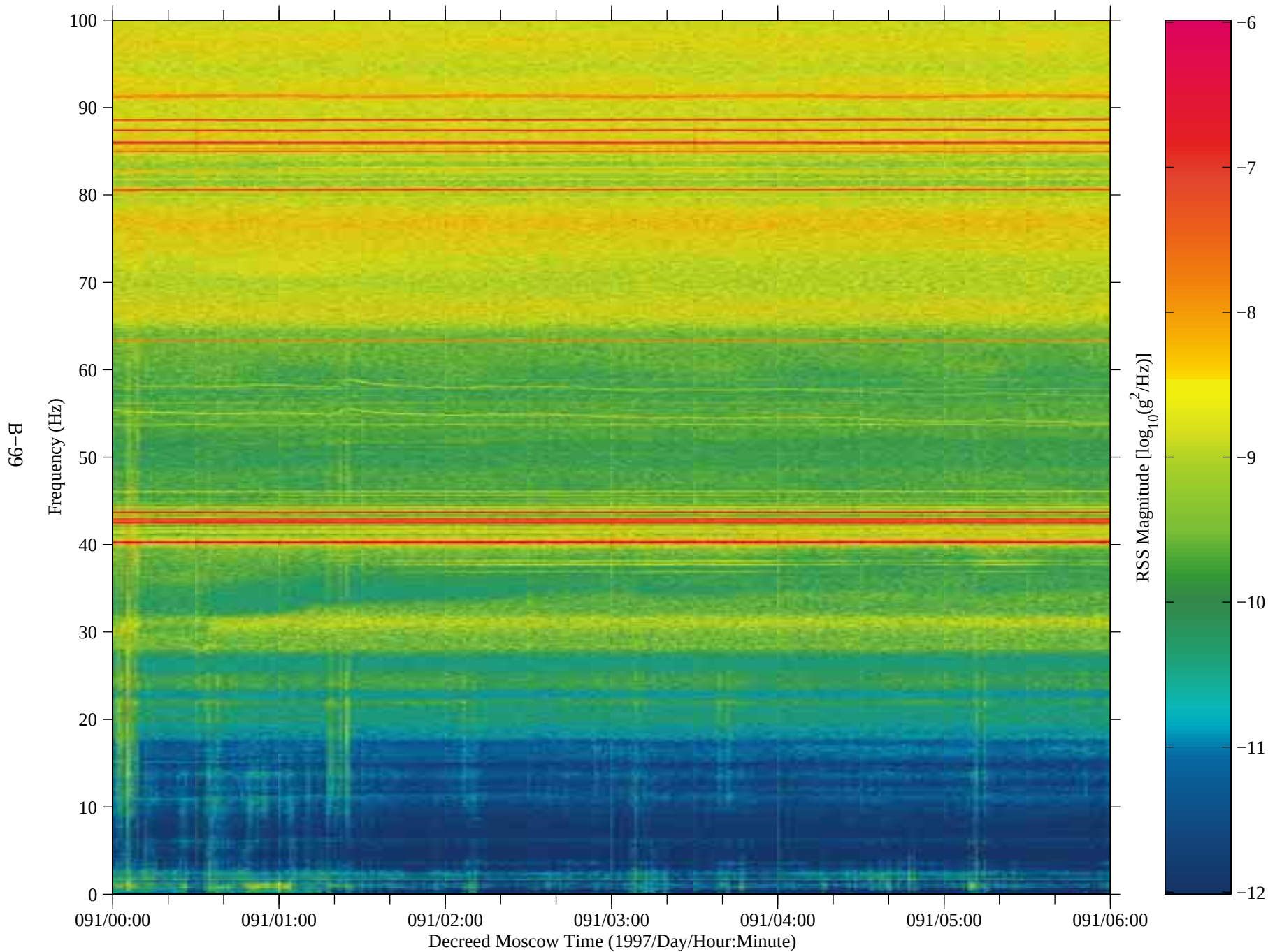
Figure 87: SAMS data from Mir, TSH A (fc=100 Hz)
