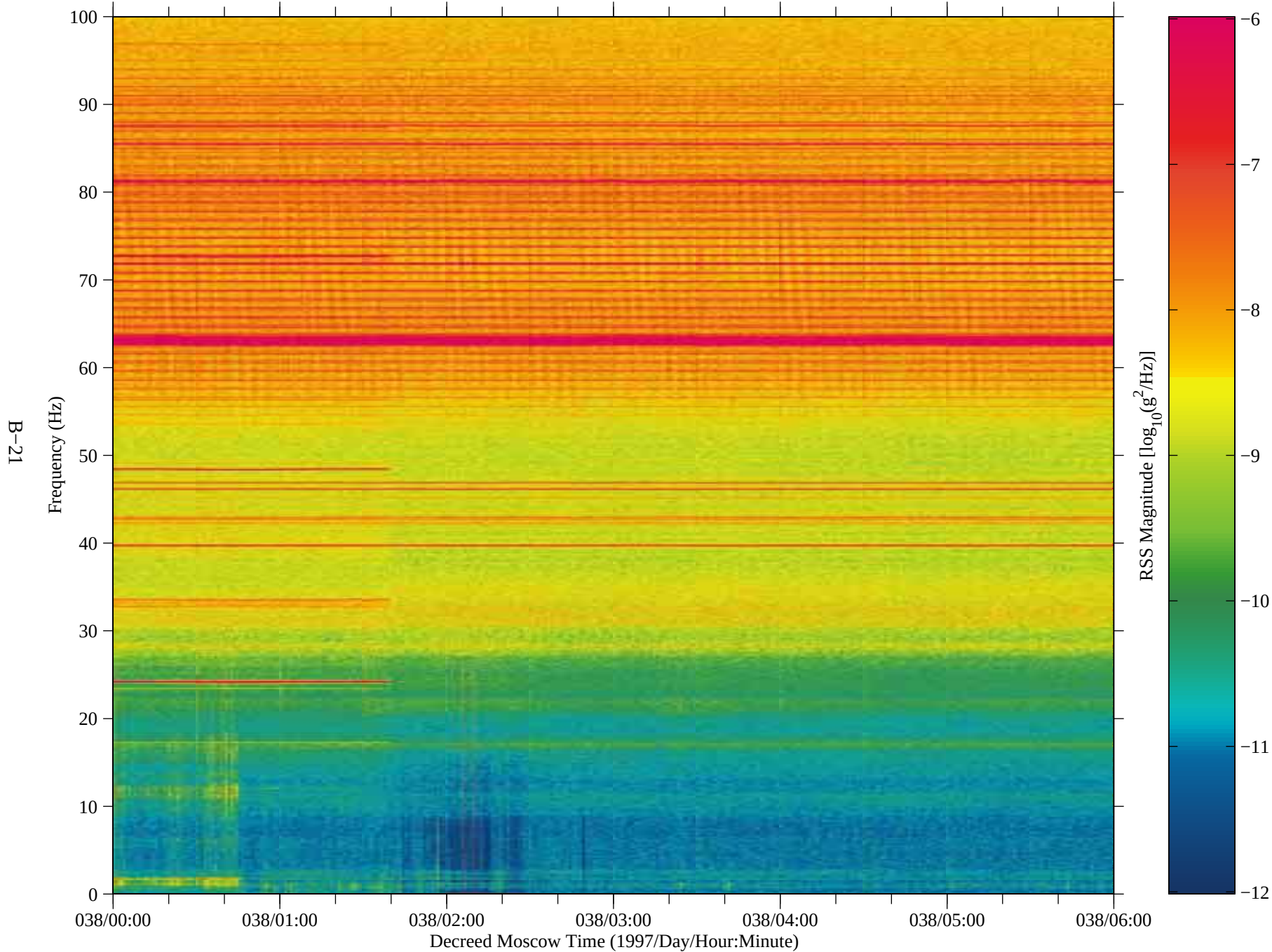
Figure 17: SAMS data from Mir, TSH A (fc=100 Hz)
