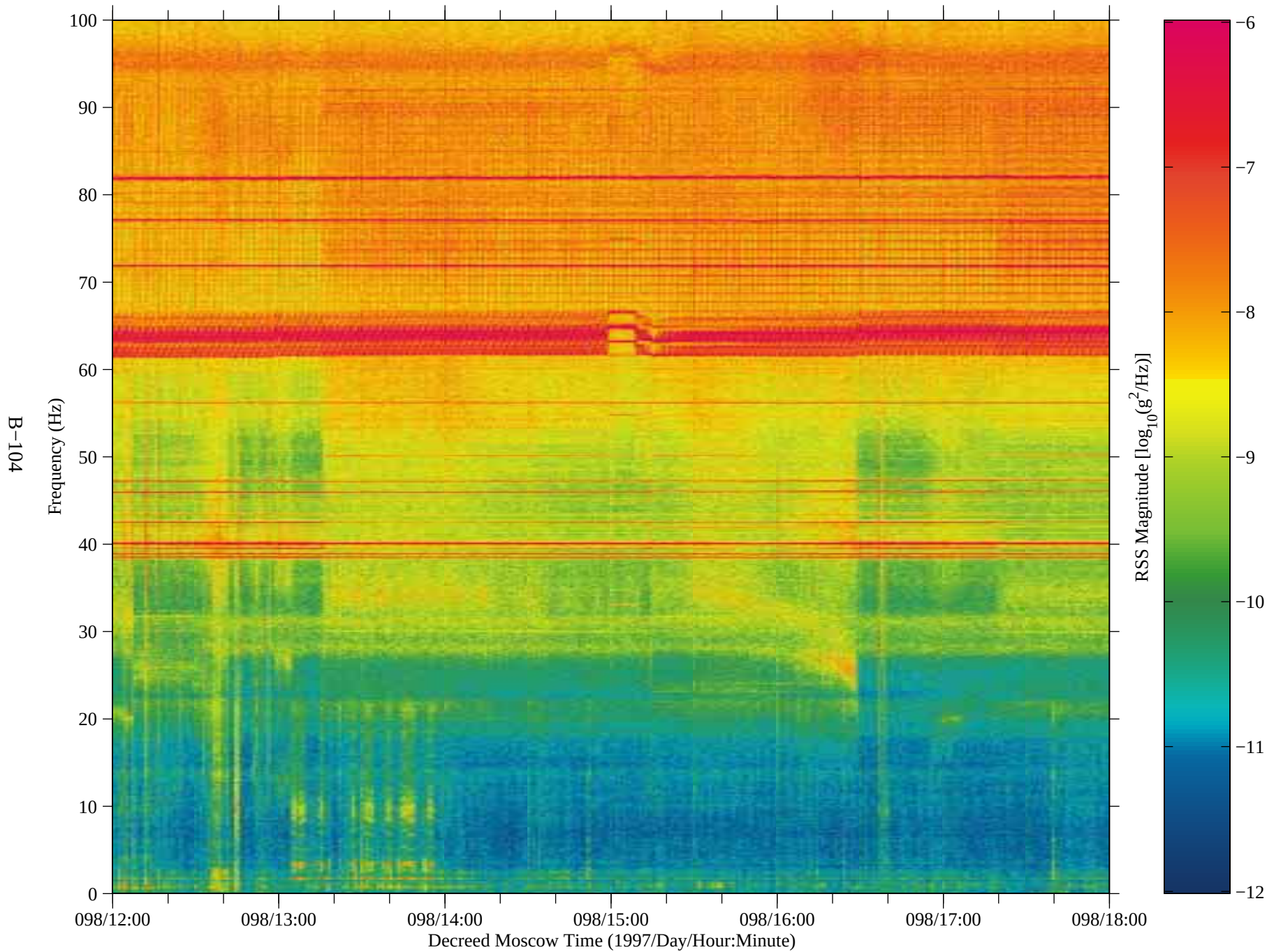
Figure 91: SAMS data from Mir, TSH A (fc=100 Hz)
