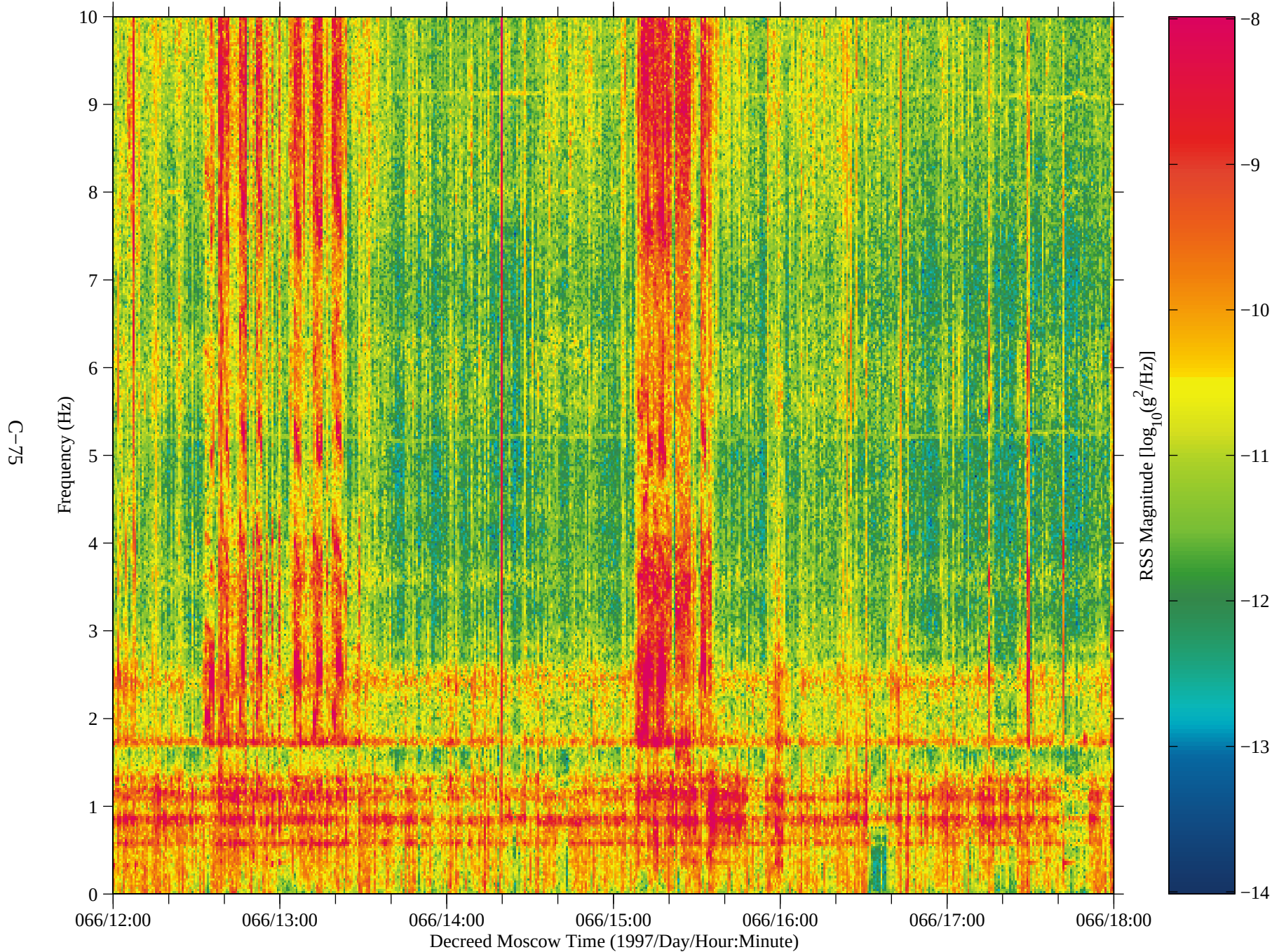
Figure 66: SAMS data from Mir, TSH B (fc=10 Hz)
