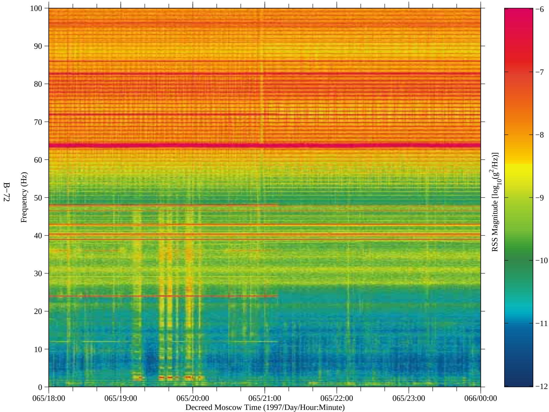
Figure 63: SAMS data from Mir, TSH A (fc=100 Hz)
