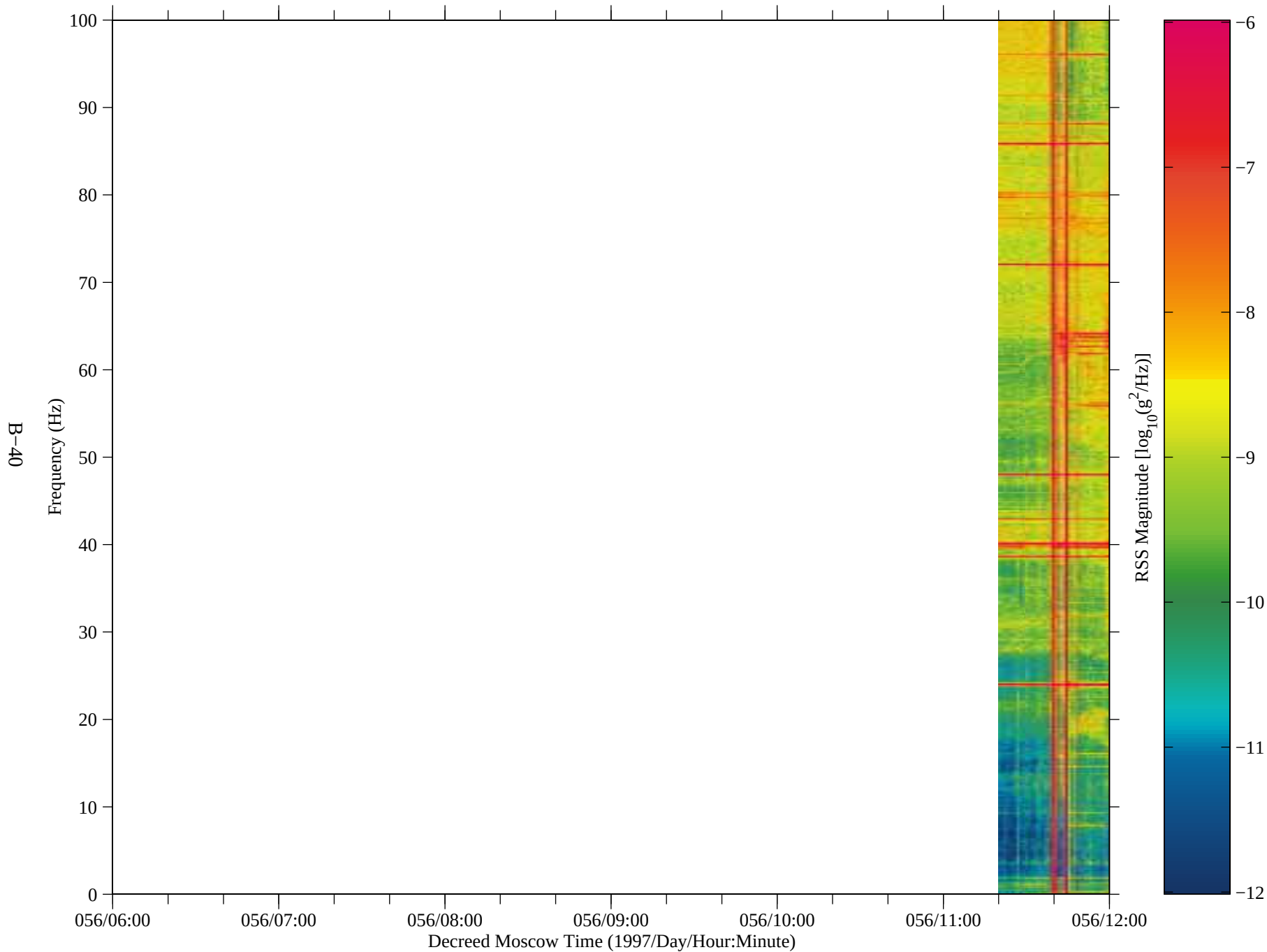
Figure 32: SAMS data from Mir, TSH A (fc=100 Hz)
