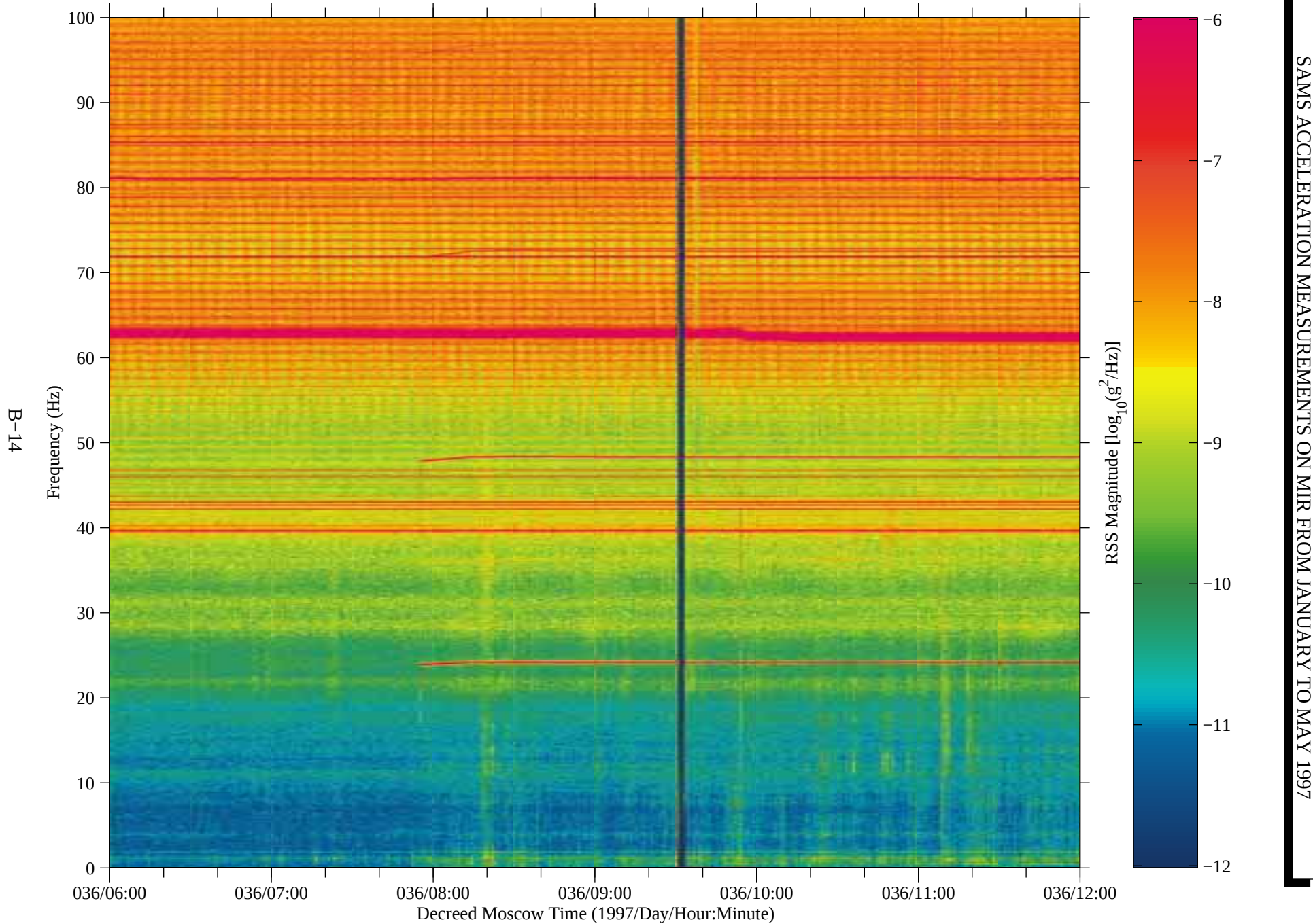
Figure 10: SAMS data from Mir, TSH A (fc=100 Hz)
