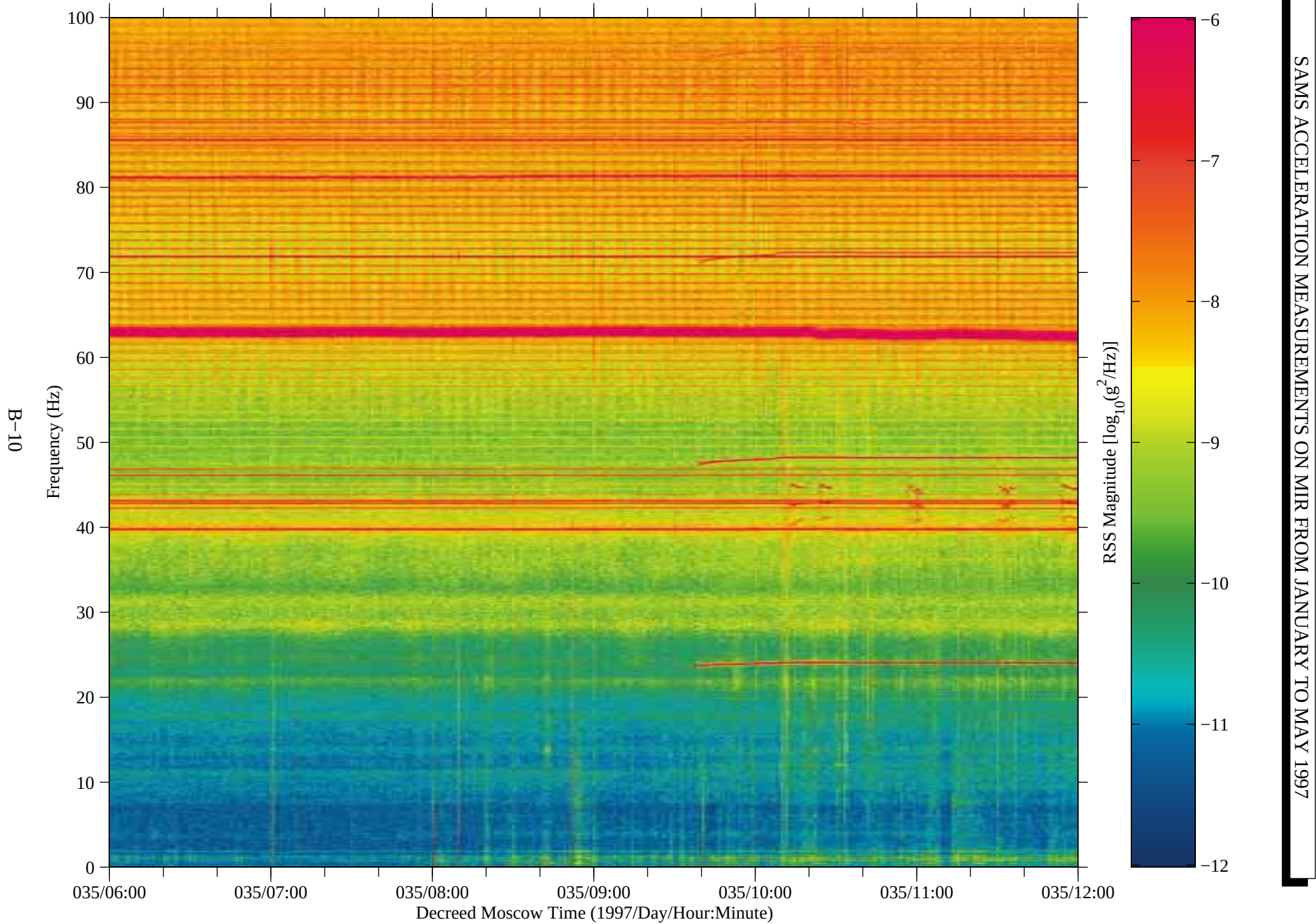
Figure 6: SAMS data from Mir, TSH A (fc=100 Hz)
