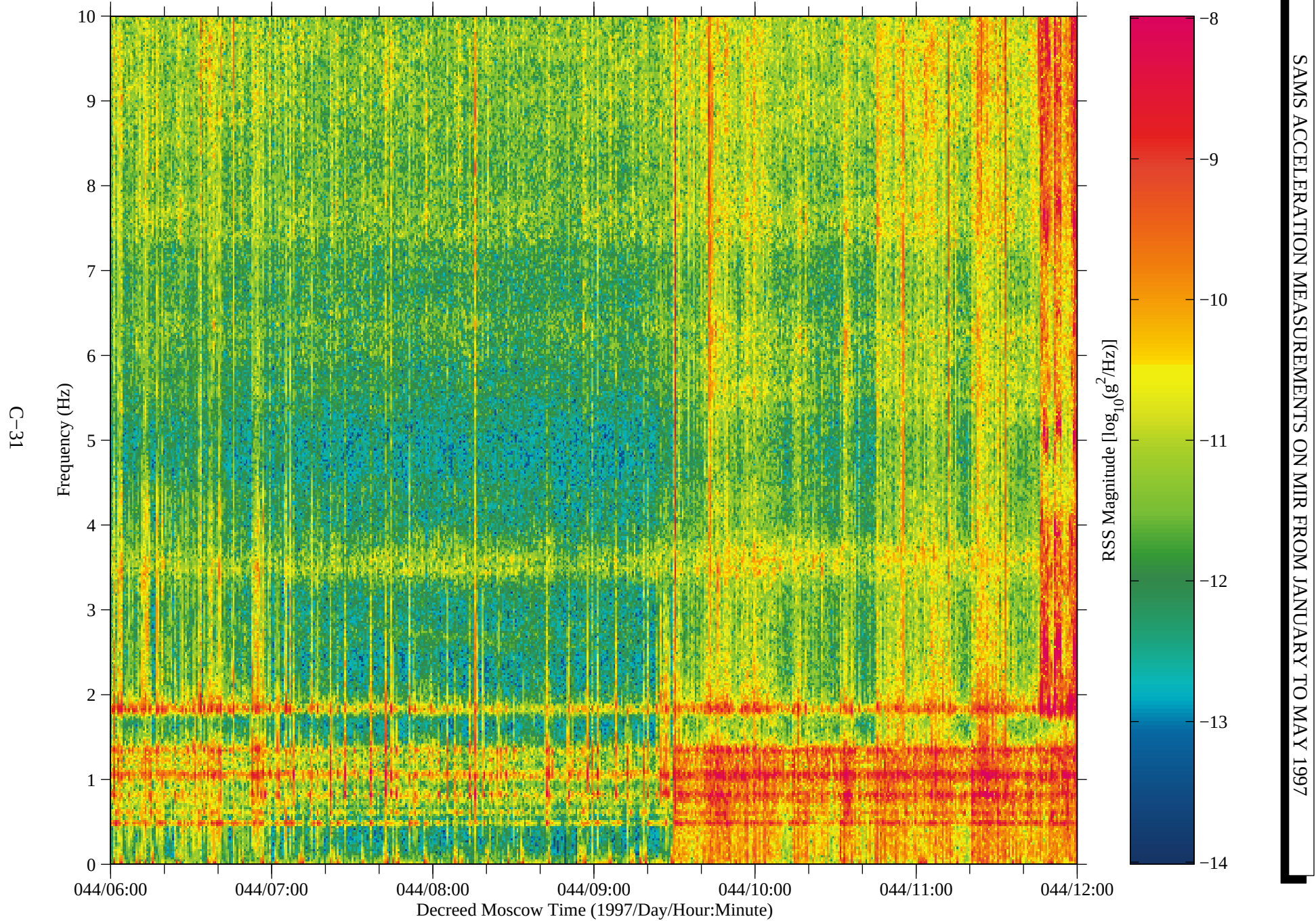
Figure 25: SAMS data from Mir, TSH B (fc=10 Hz)
