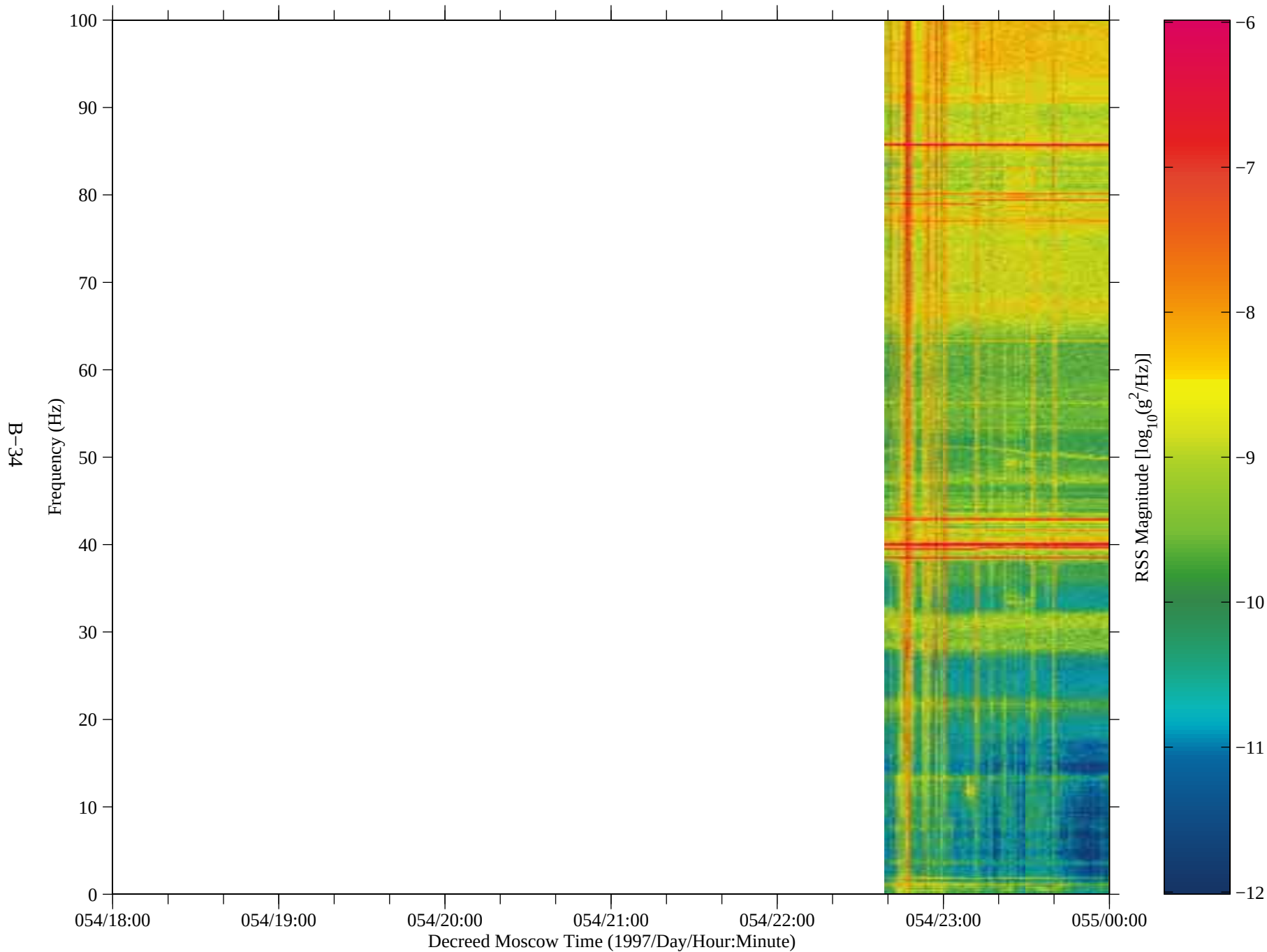
Figure 27: SAMS data from Mir, TSH A (fc=100 Hz)
