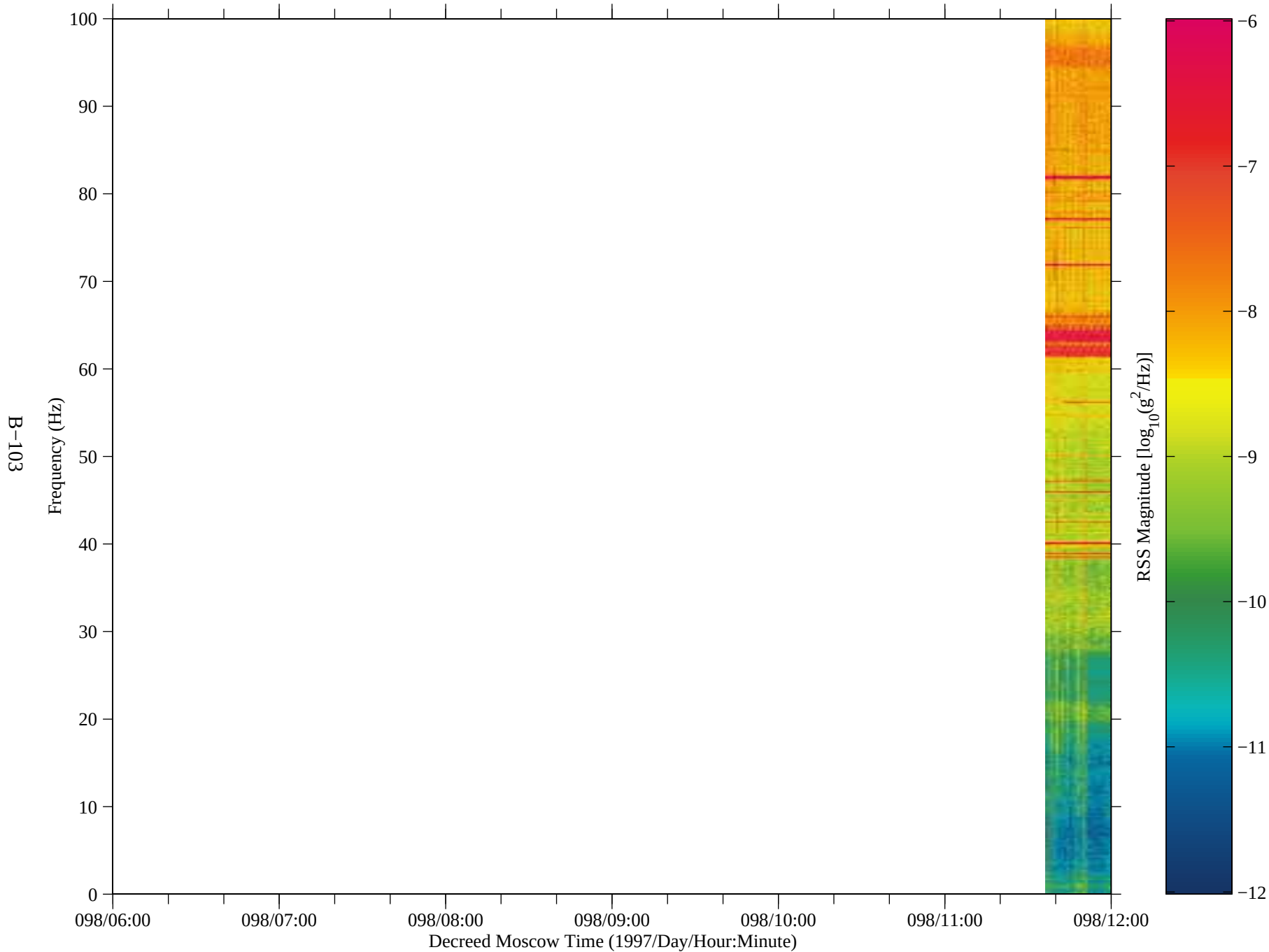
Figure 90: SAMS data from Mir, TSH A (fc=100 Hz)
