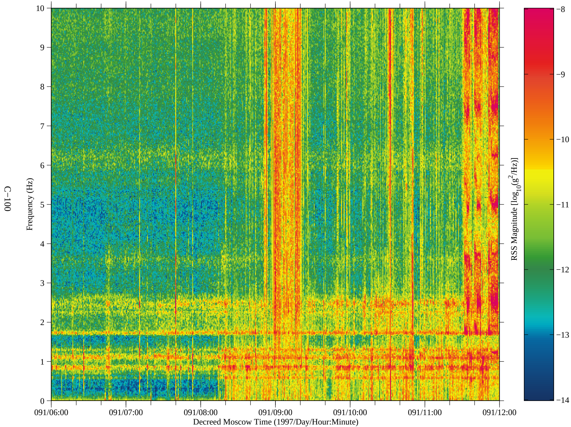
Figure 88: SAMS data from Mir, TSH B (fc=10 Hz)
