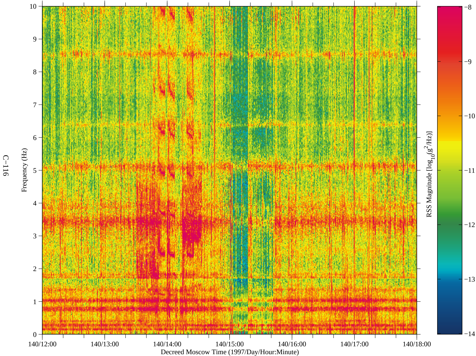
Figure 100: SAMS data from Mir, TSH B (fc=10 Hz)
