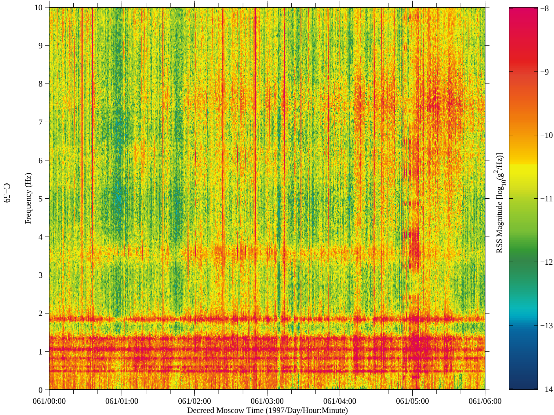
Figure 51: SAMS data from Mir, TSH B (fc=10 Hz)
