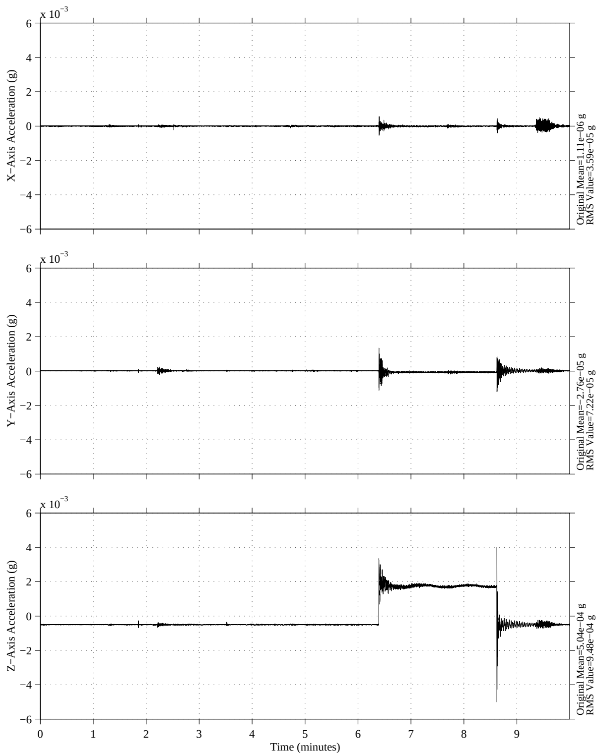
Figure 5. Reboost Operation
