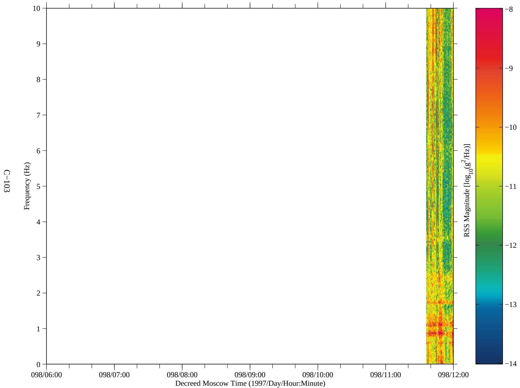
Figure 90: SAMS data from Mir, TSH B (fc=10 Hz)
