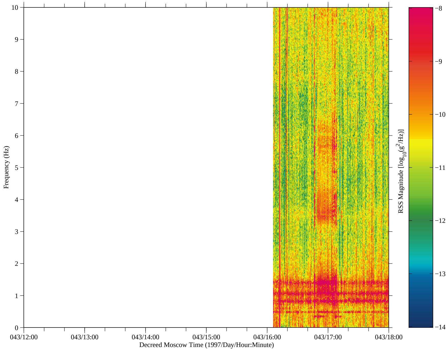
Figure 22: SAMS data from Mir, TSH B (fc=10 Hz)
