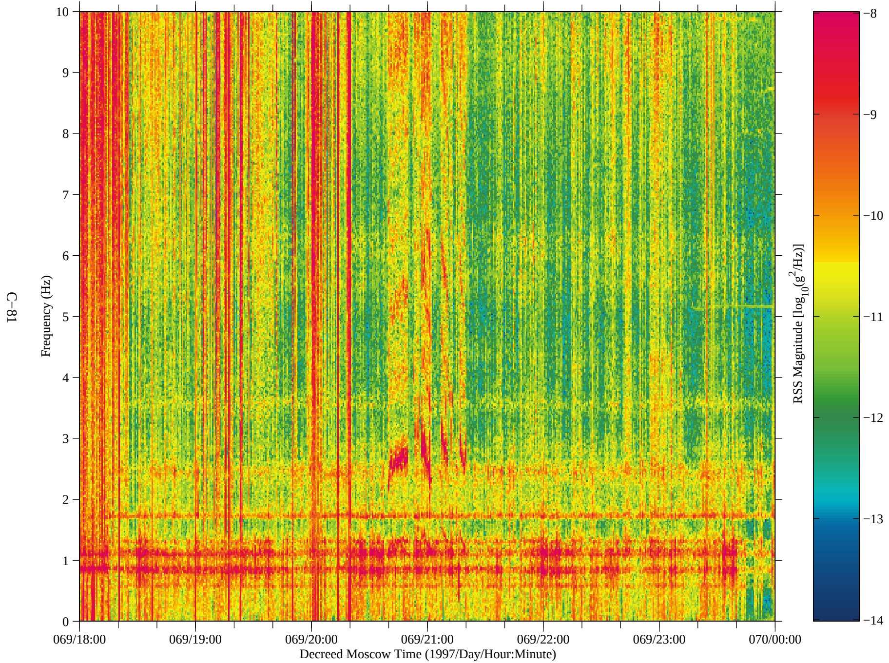
Figure 71: SAMS data from Mir, TSH B (fc=10 Hz)
