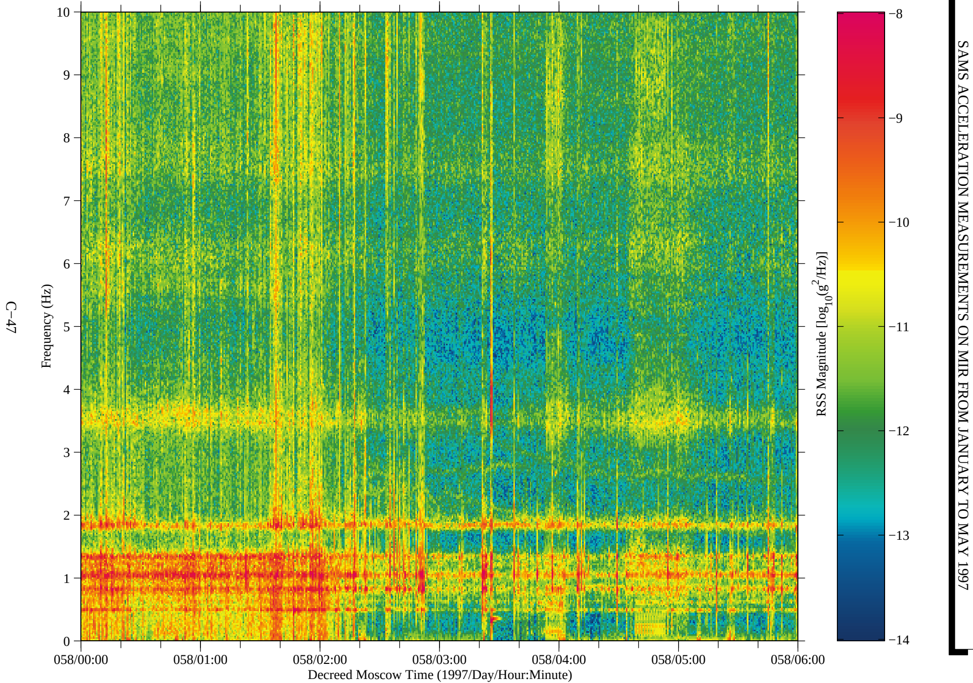
Figure 39: SAMS data from Mir, TSH B (fc=10 Hz)
