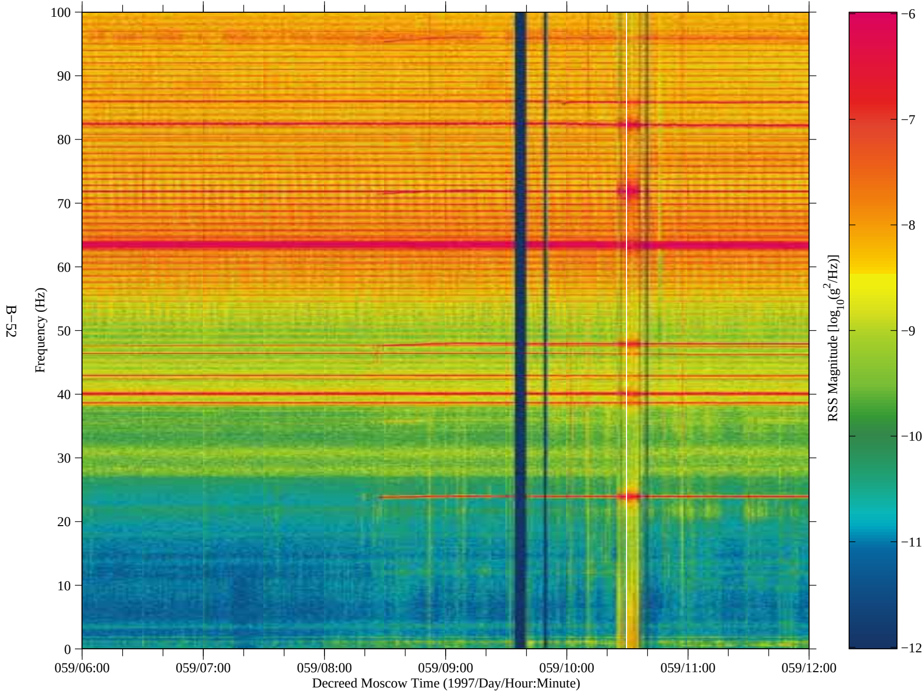
Figure 44: SAMS data from Mir, TSH A (fc=100 Hz)
