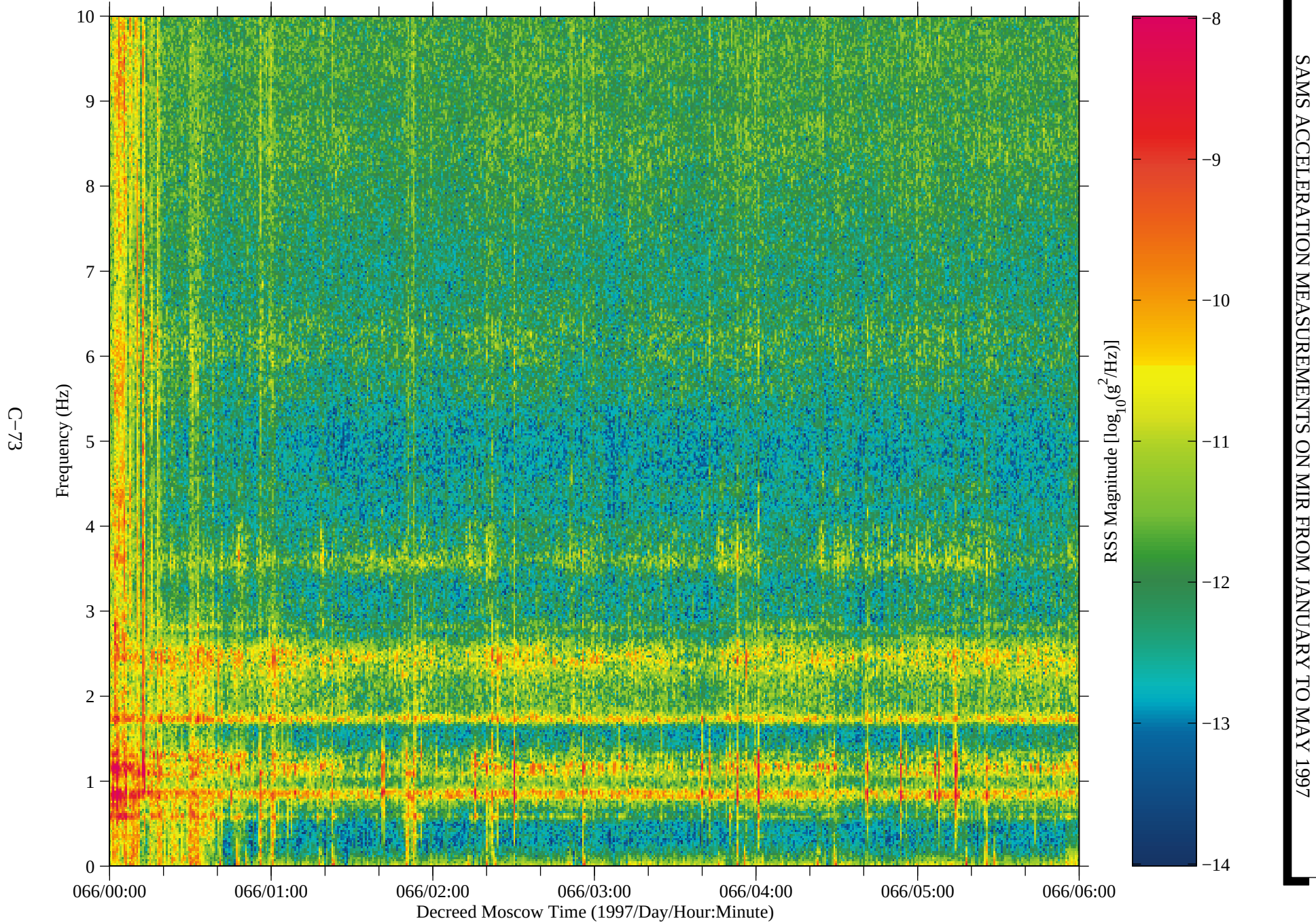
Figure 64: SAMS data from Mir, TSH B (fc=10 Hz)
