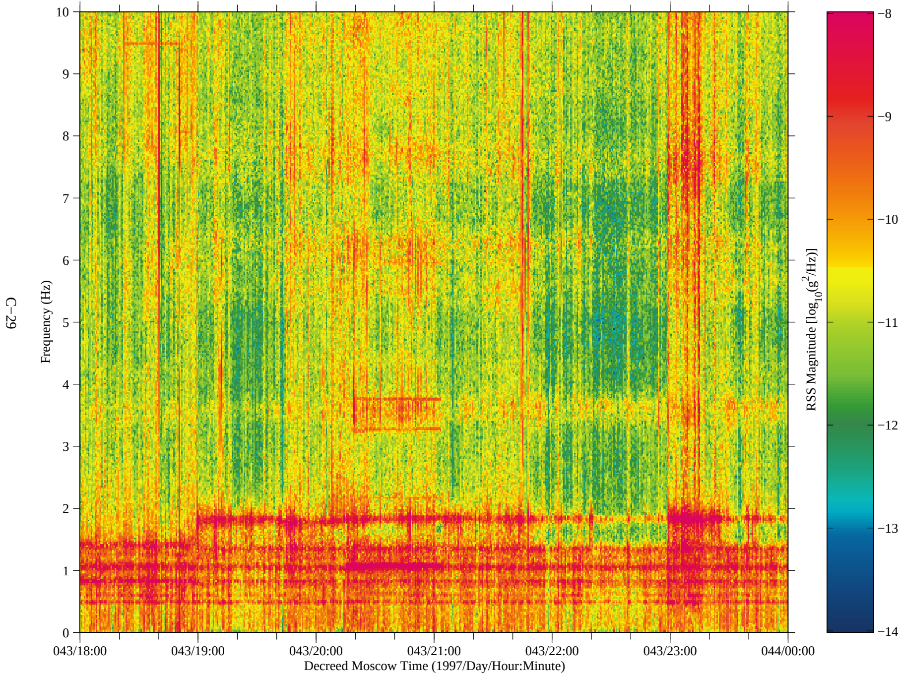
Figure 23: SAMS data from Mir, TSH B (fc=10 Hz)
