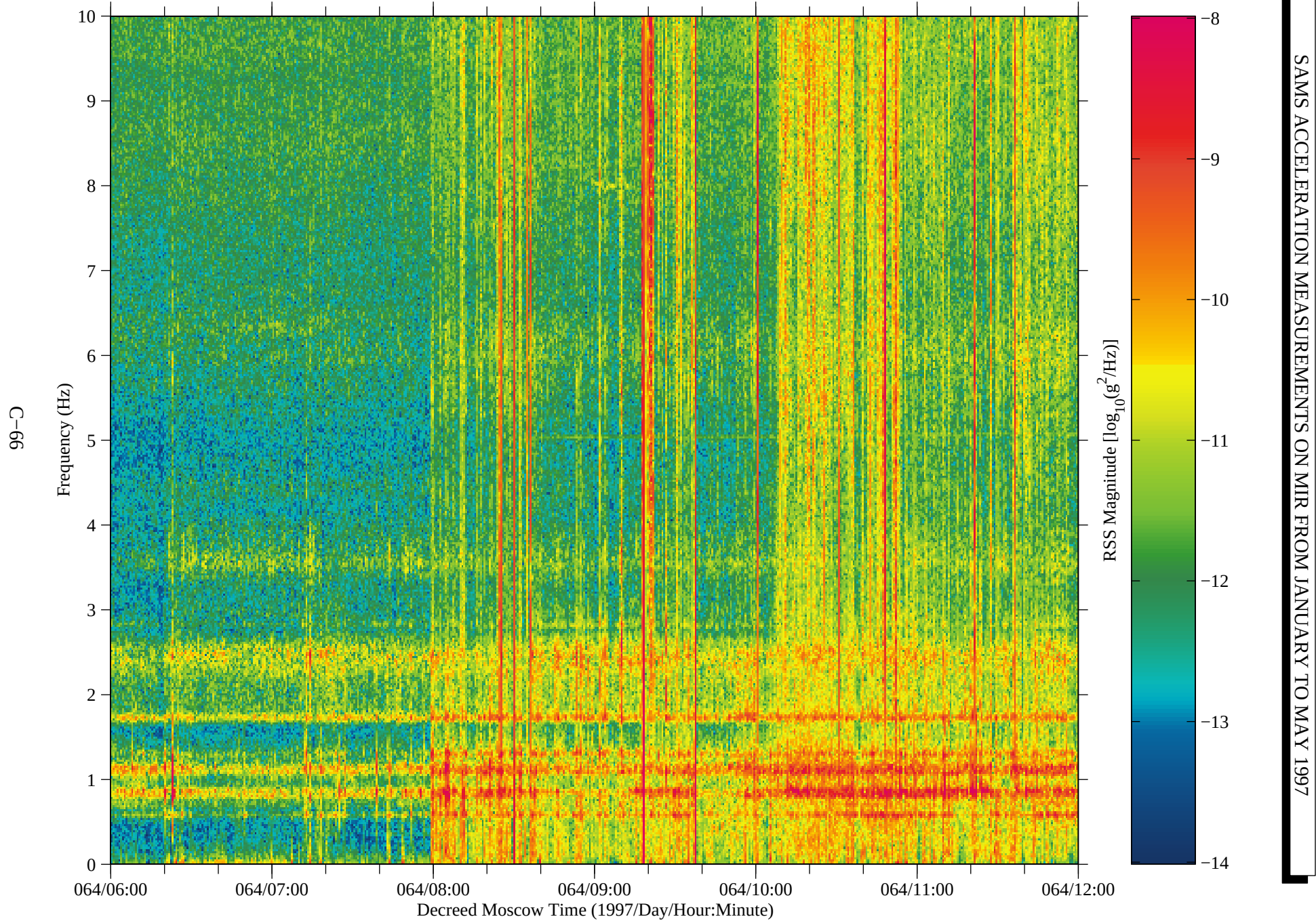
Figure 57: SAMS data from Mir, TSH B (fc=10 Hz)
