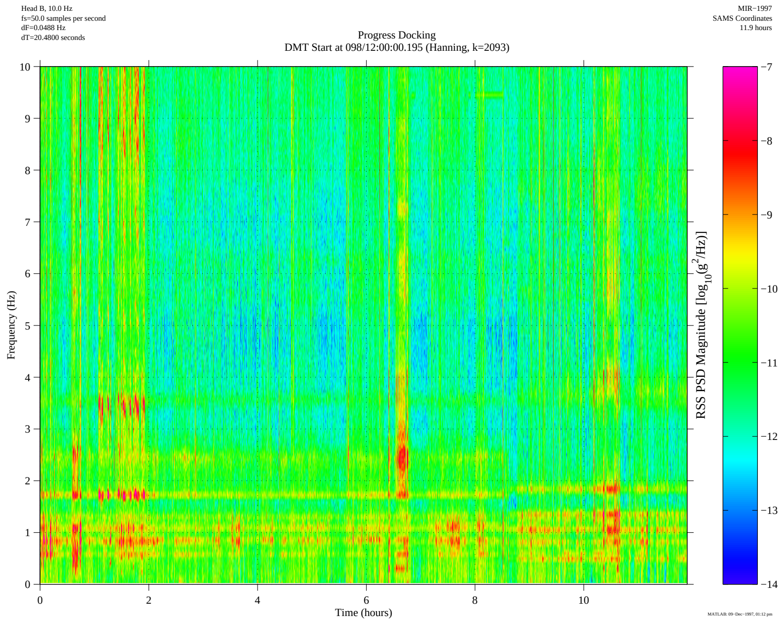
Figure 9. Progress docking
