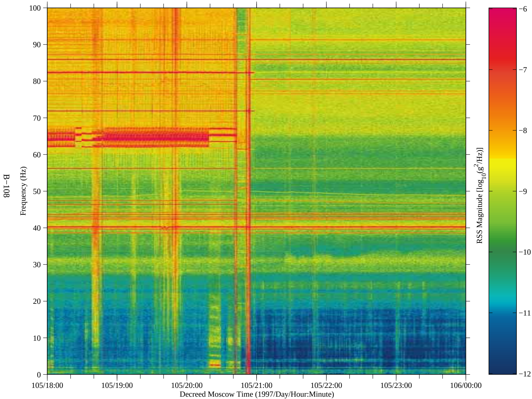
Figure 94: SAMS data from Mir, TSH A (fc=100 Hz)
