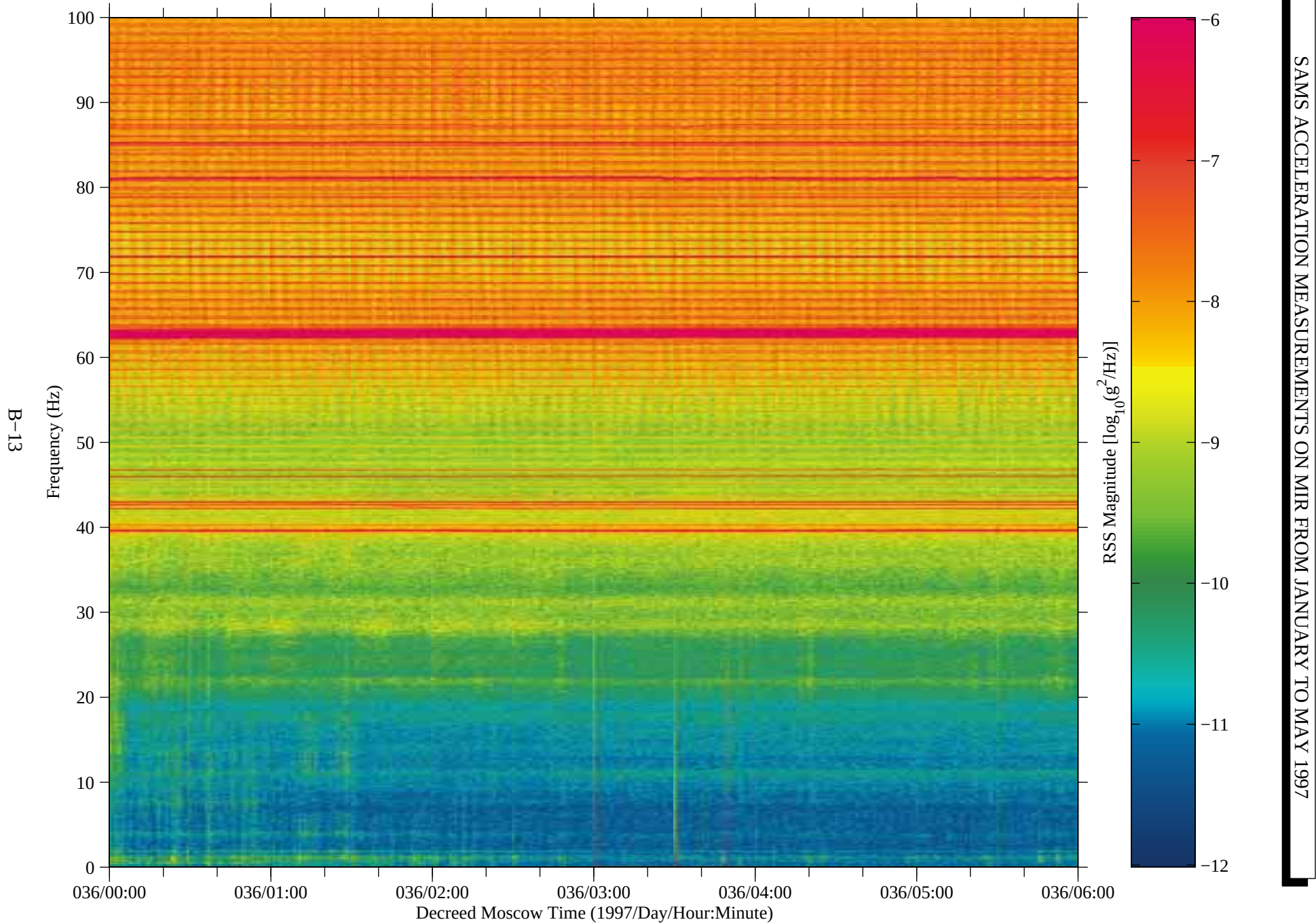
Figure 9: SAMS data from Mir, TSH A (fc=100 Hz)
