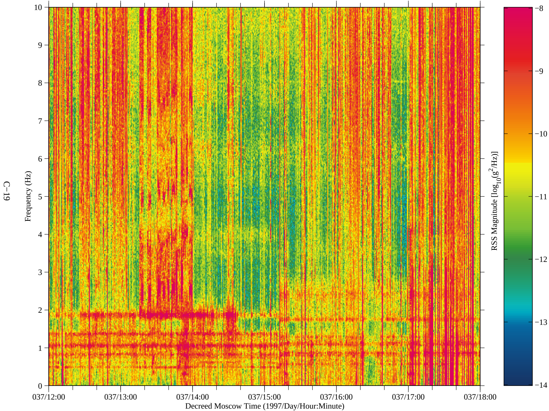
Figure 15: SAMS data from Mir, TSH B (fc=10 Hz)
