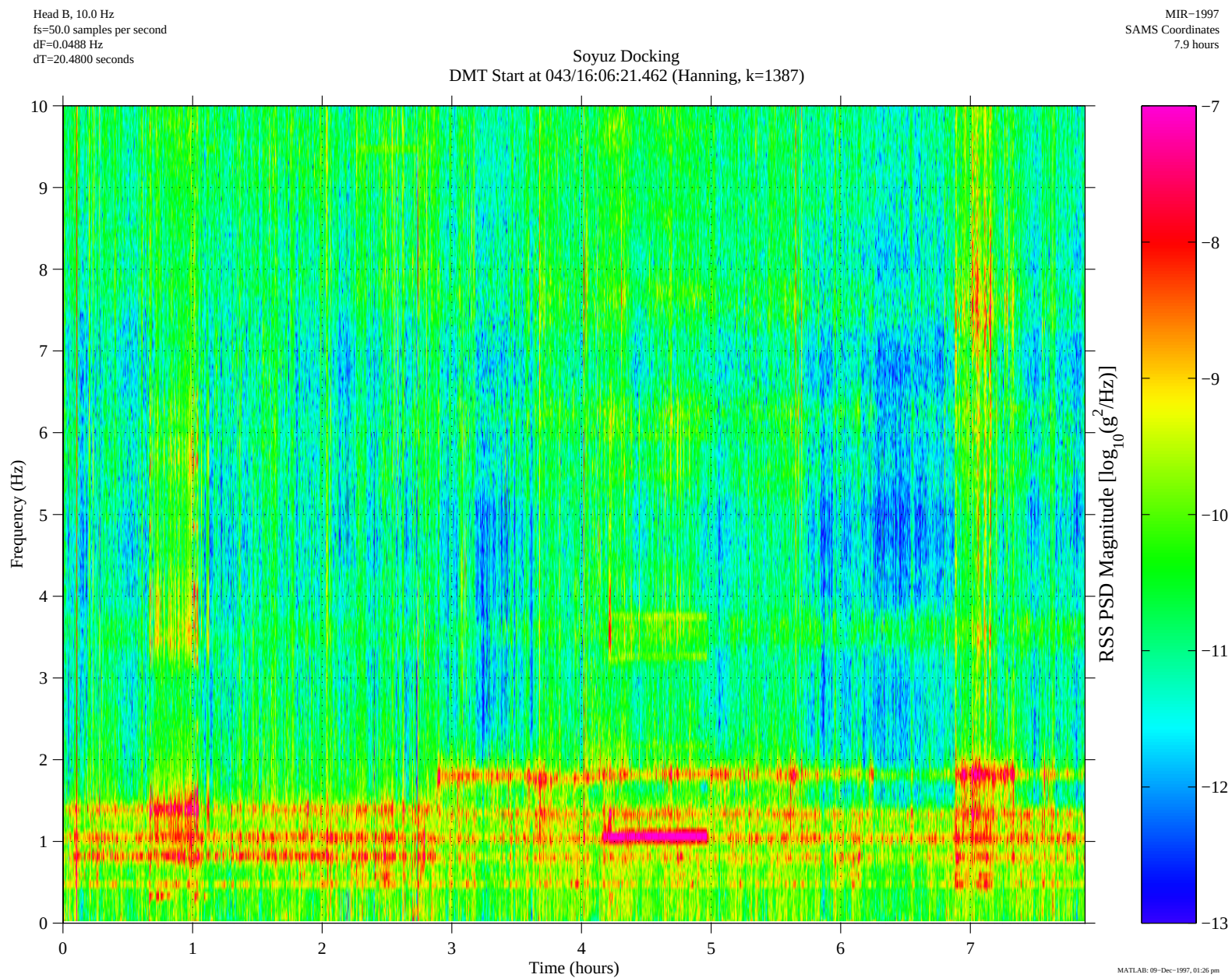
Figure 7. Soyuz docking
