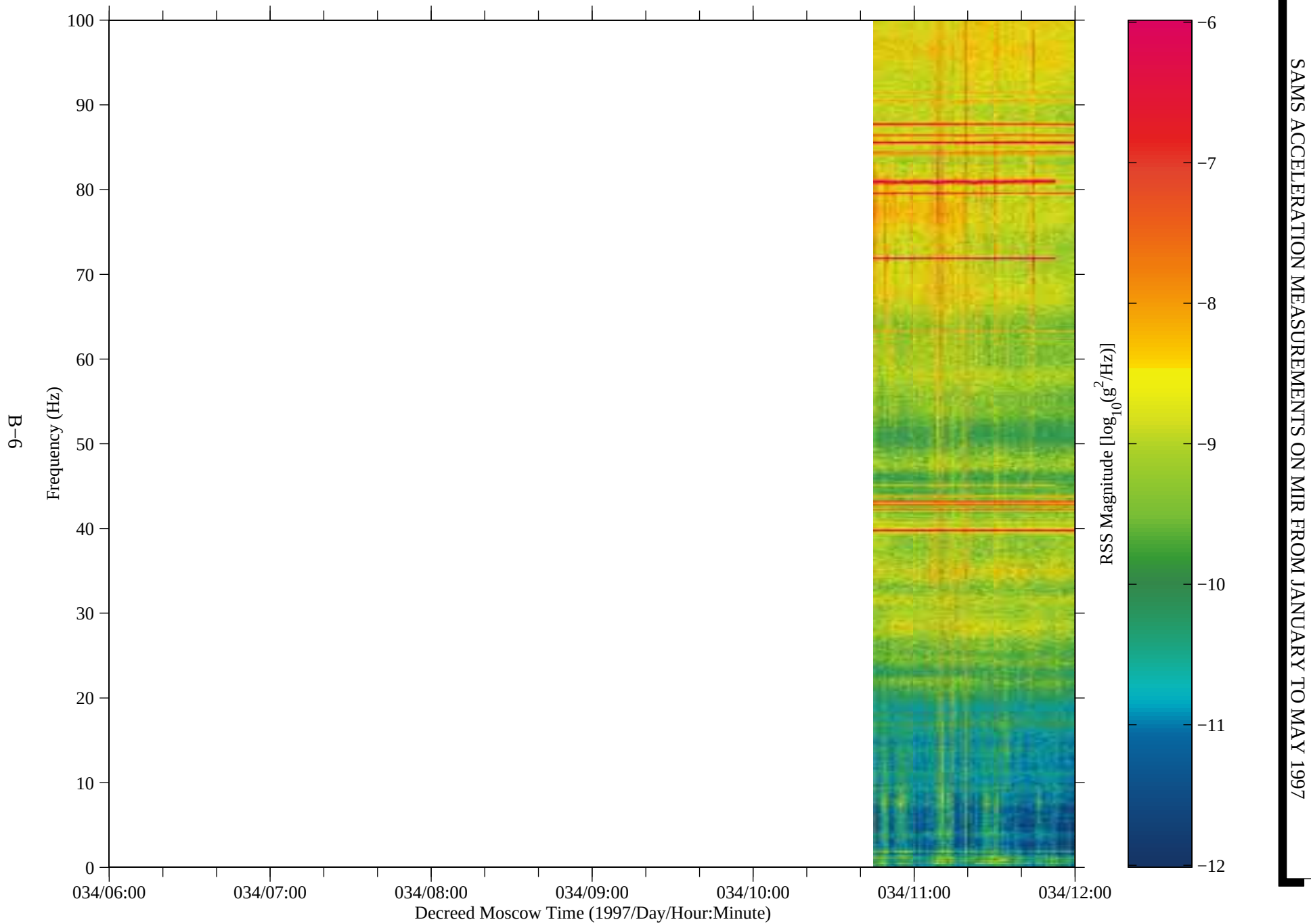
Figure 2: SAMS data from Mir, TSH A (fc=100 Hz)
