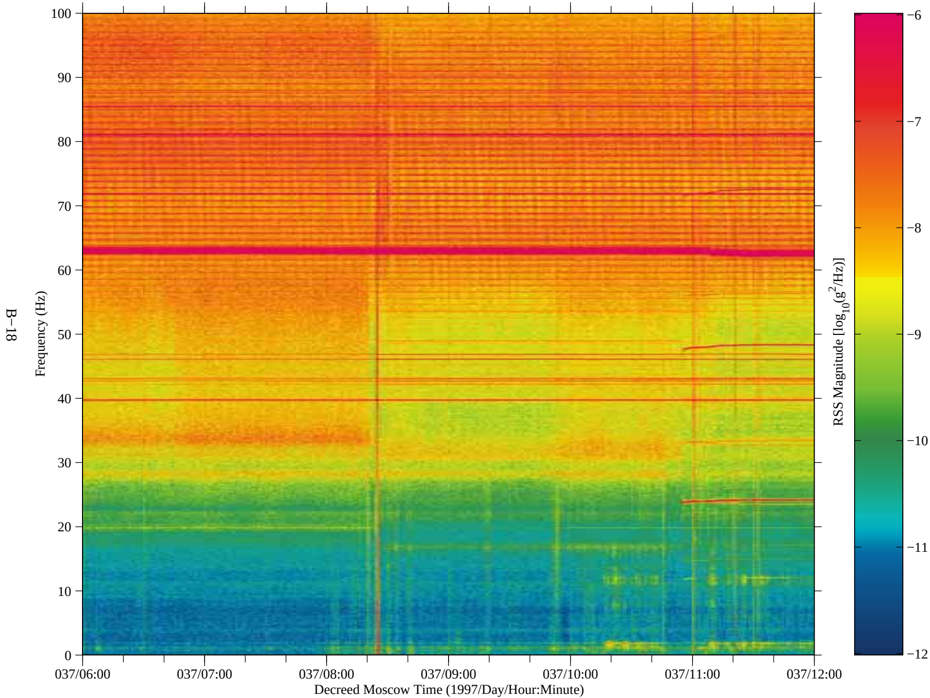
Figure 14: SAMS data from Mir, TSH A (fc=100 Hz)
