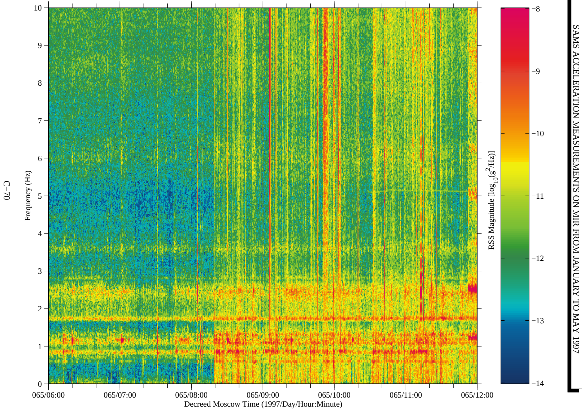
Figure 61: SAMS data from Mir, TSH B (fc=10 Hz)
