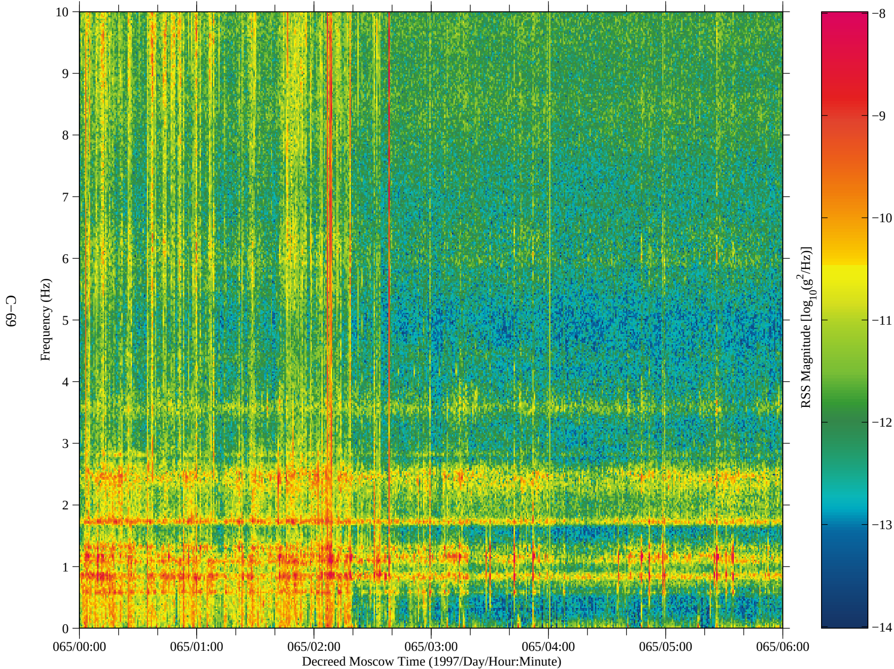
Figure 60: SAMS data from Mir, TSH B (fc=10 Hz)
