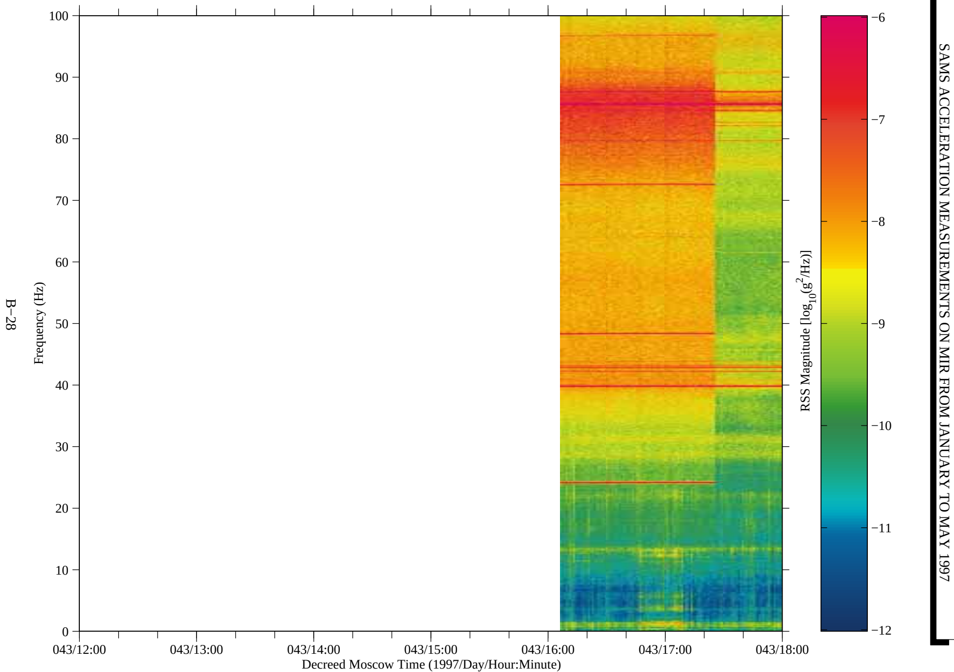
Figure 22: SAMS data from Mir, TSH A (fc=100 Hz)
