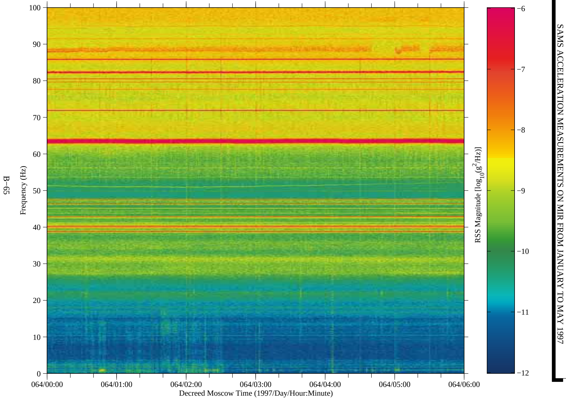
Figure 56: SAMS data from Mir, TSH A (fc=100 Hz)
