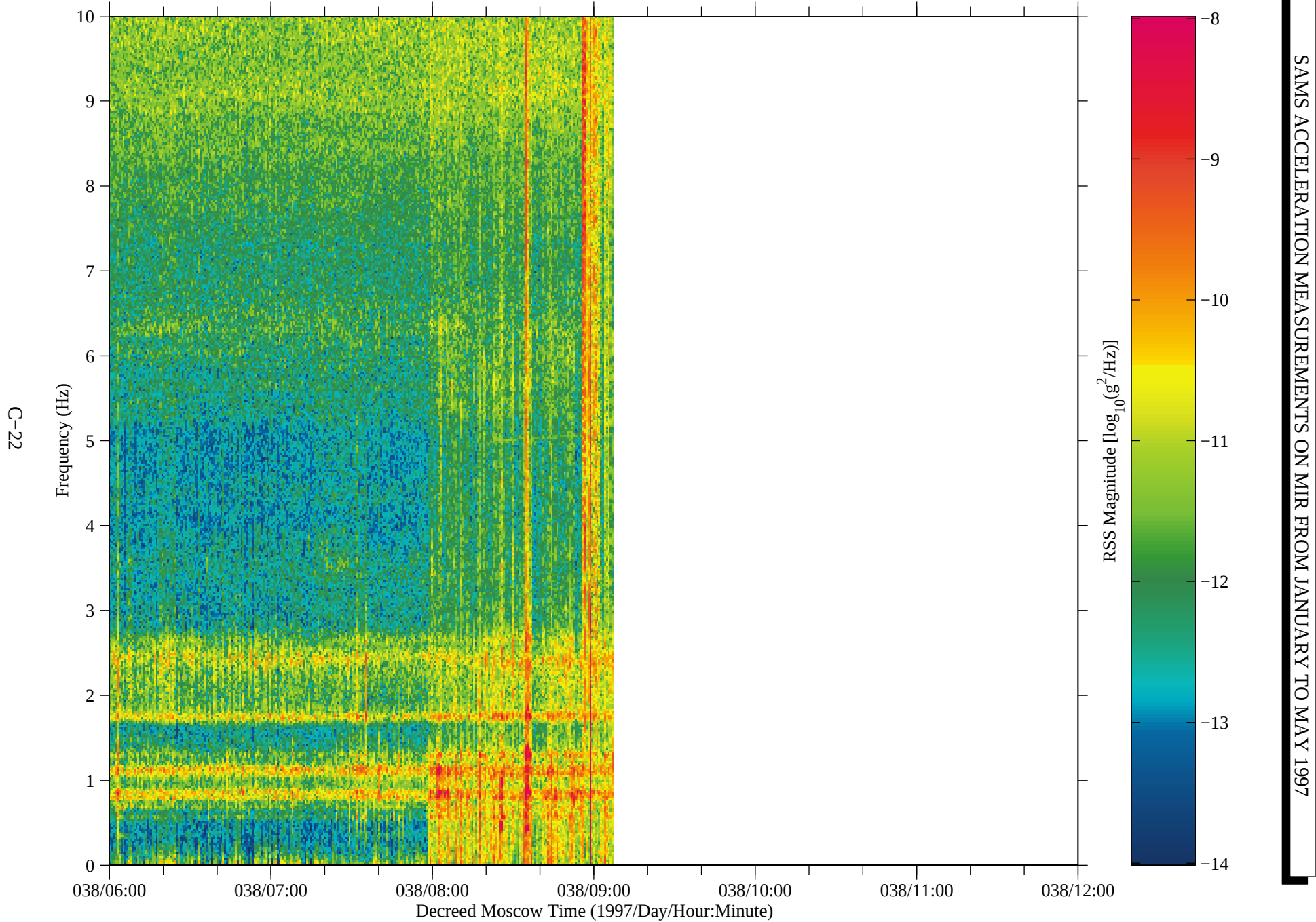
Figure 18: SAMS data from Mir, TSH B (fc=10 Hz)
