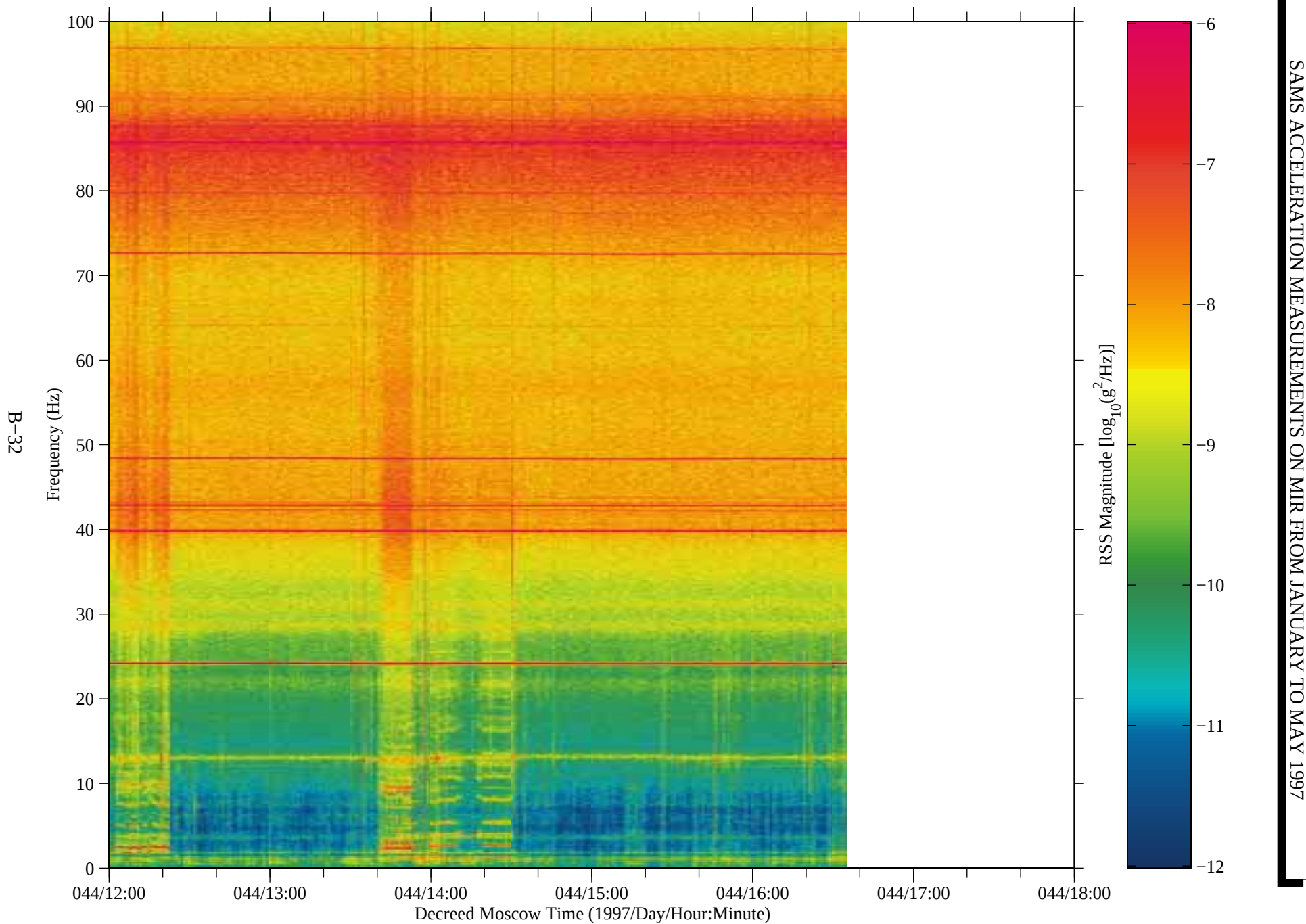
Figure 26: SAMS data from Mir, TSH A (fc=100 Hz)
