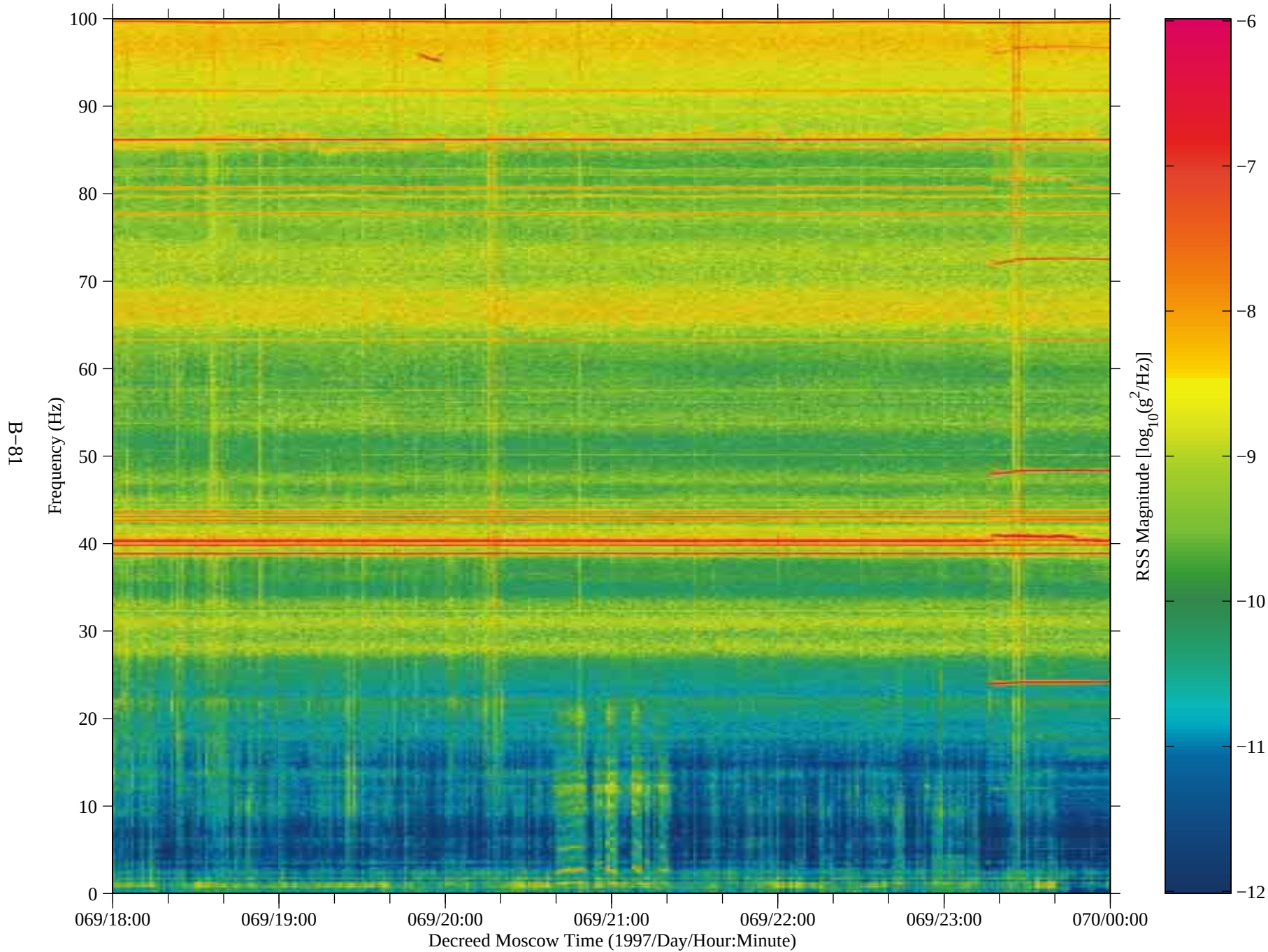
Figure 71: SAMS data from Mir, TSH A (fc=100 Hz)
