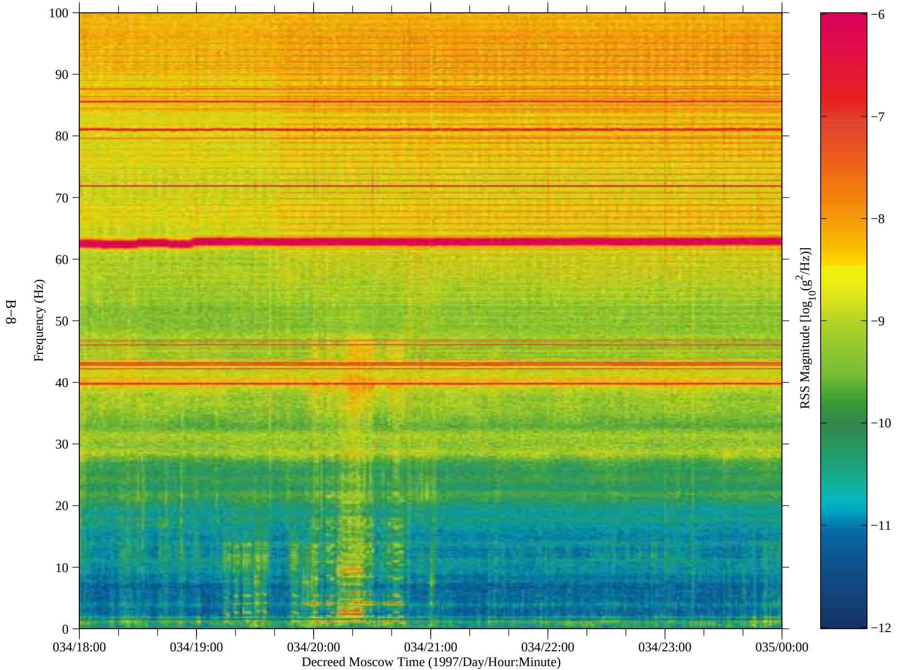
Figure 4: SAMS data from Mir, TSH A (fc=100 Hz)
