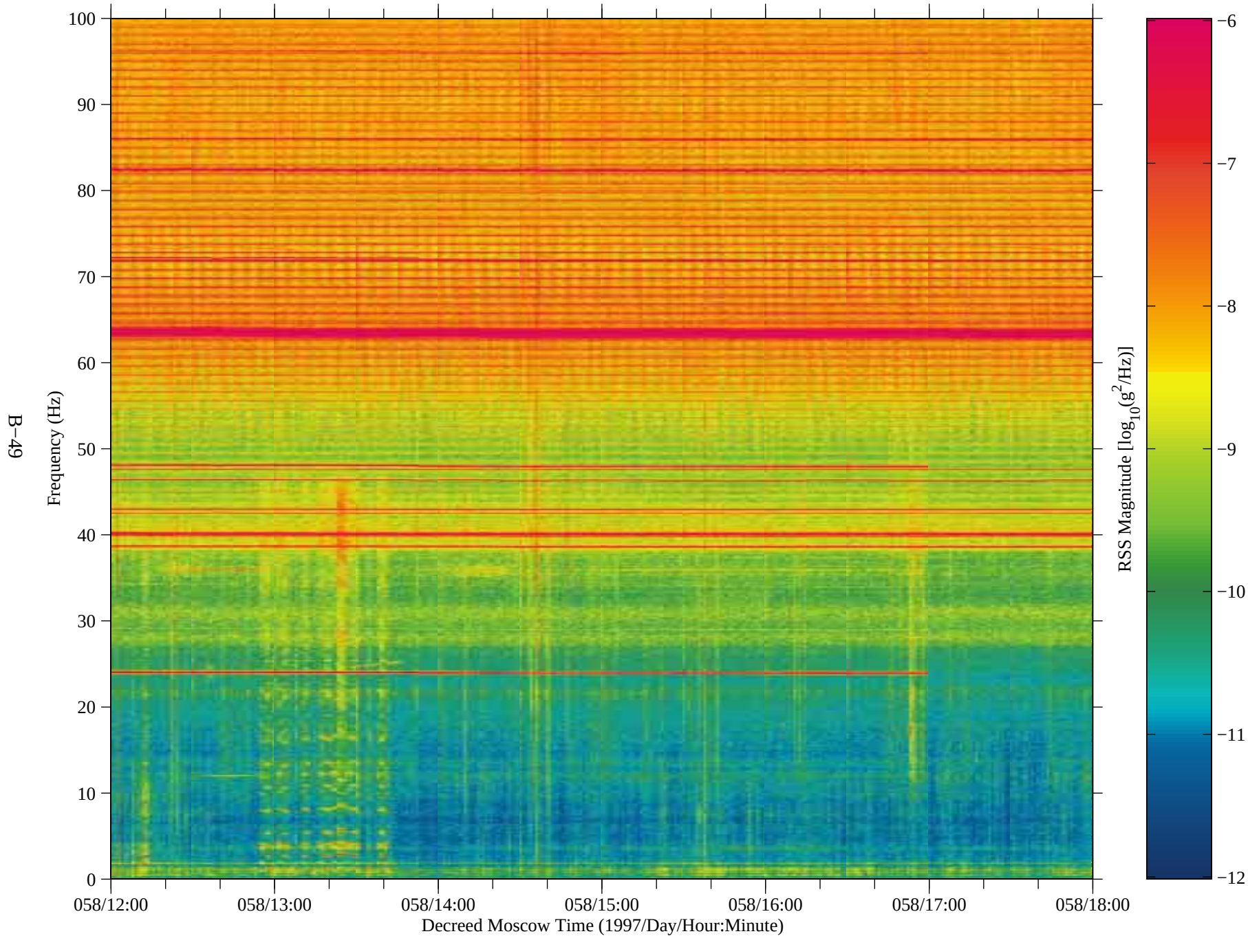
Figure 41: SAMS data from Mir, TSH A (fc=100 Hz)
