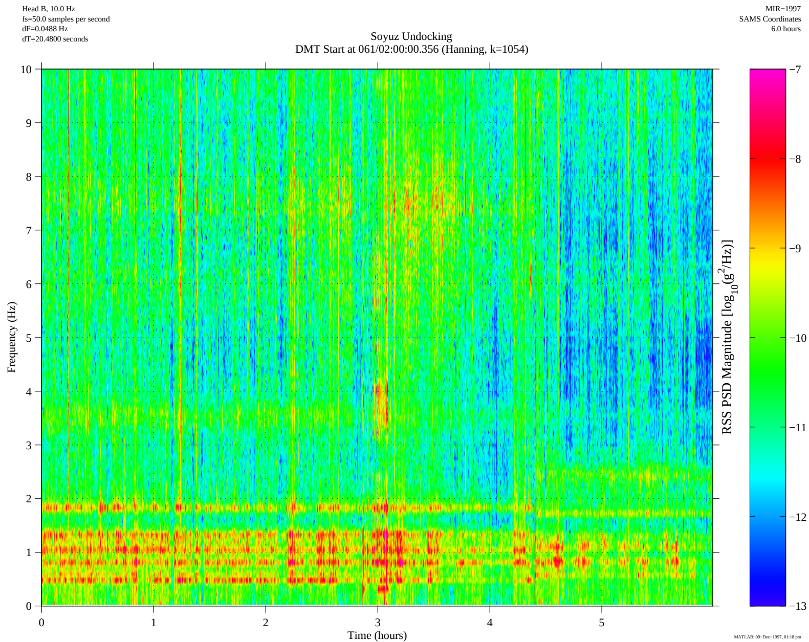
Figure 8. Soyuz undocking
