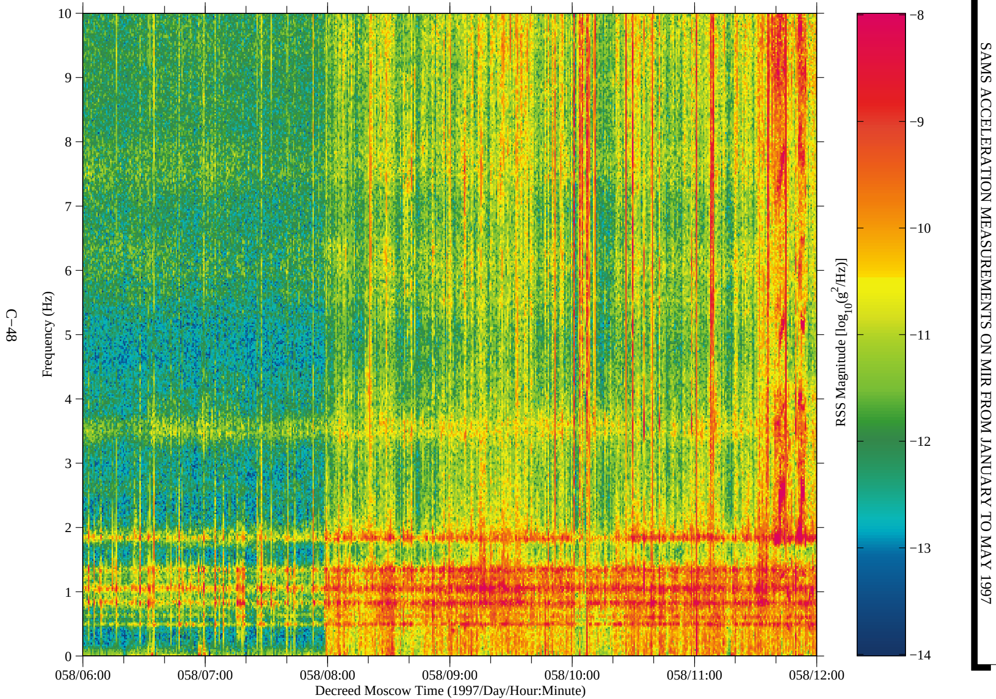
Figure 40: SAMS data from Mir, TSH B (fc=10 Hz)
