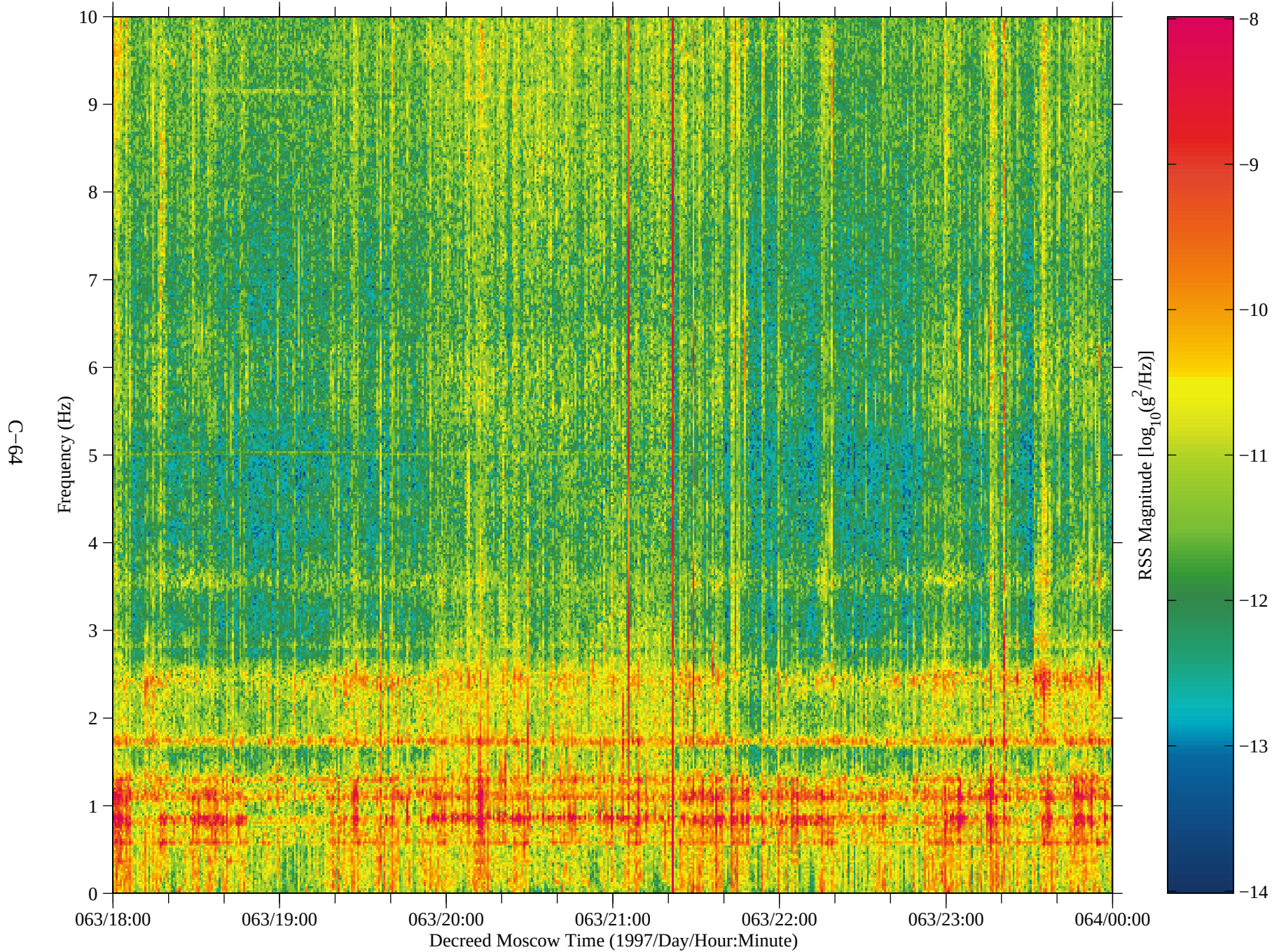
Figure 55: SAMS data from Mir, TSH B (fc=10 Hz)
