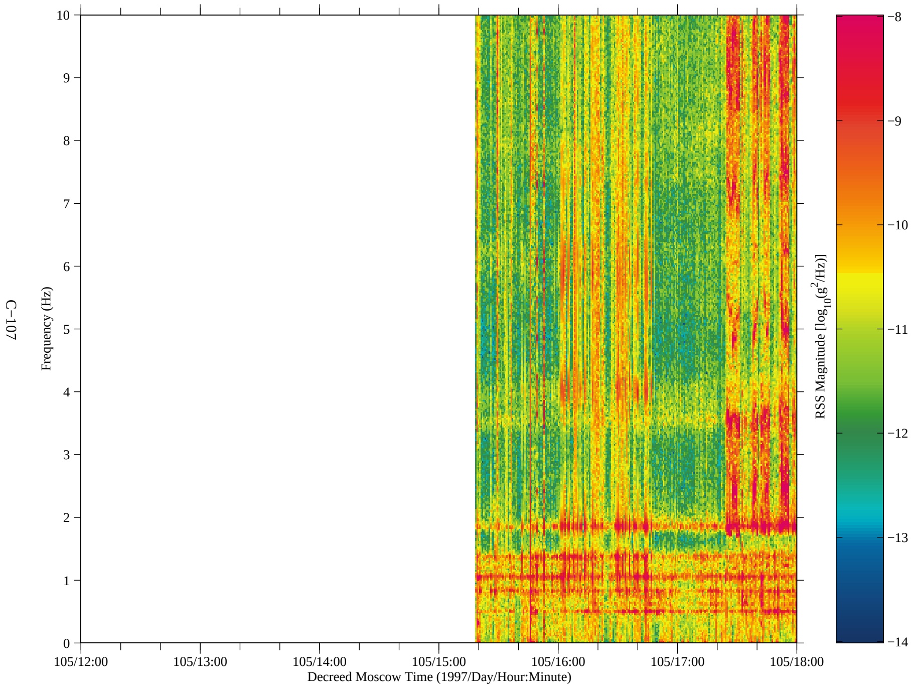
Figure 93: SAMS data from Mir, TSH B (fc=10 Hz)
