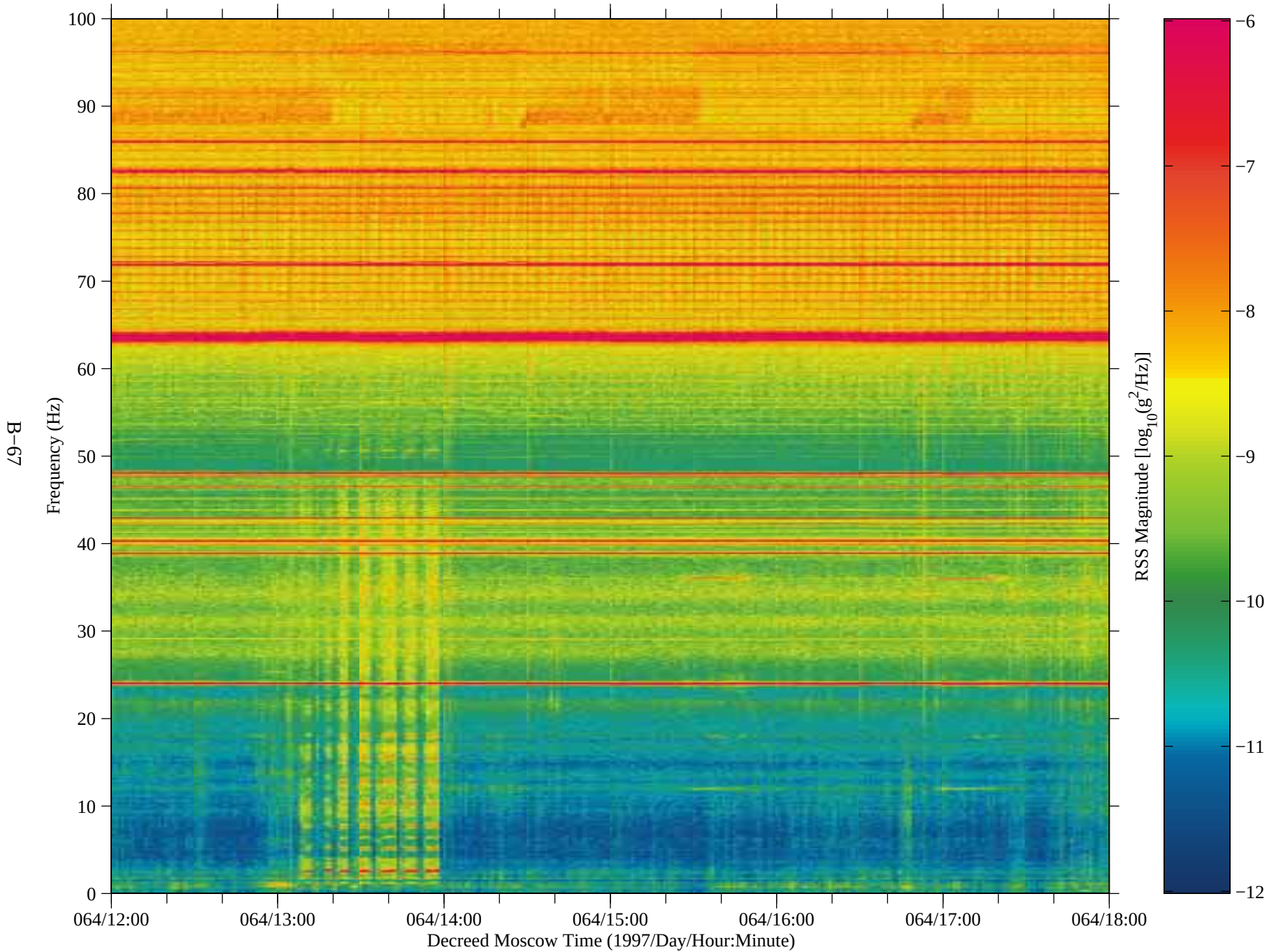
Figure 58: SAMS data from Mir, TSH A (fc=100 Hz)
