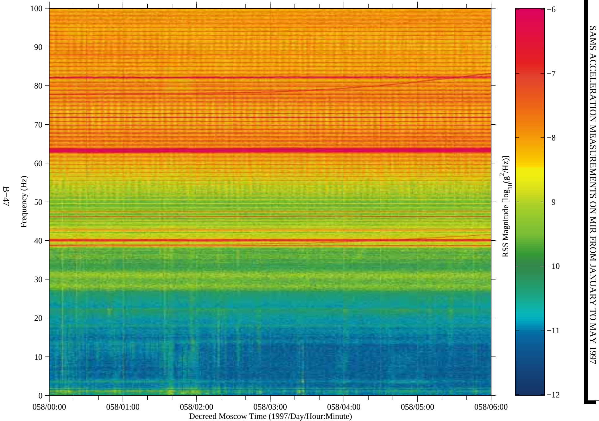
Figure 39: SAMS data from Mir, TSH A (fc=100 Hz)
