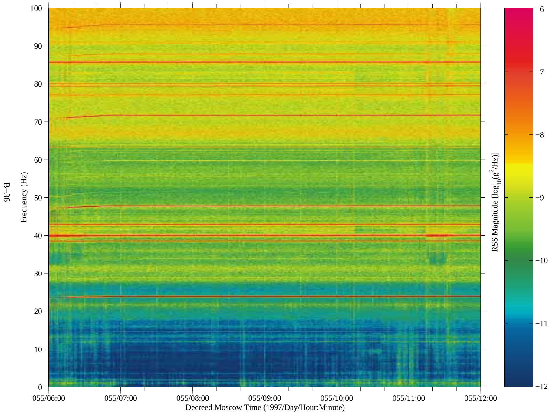
Figure 29: SAMS data from Mir, TSH A (fc=100 Hz)
