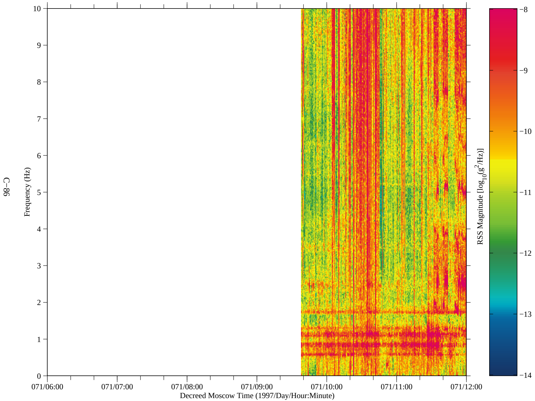
Figure 75: SAMS data from Mir, TSH B (fc=10 Hz)
