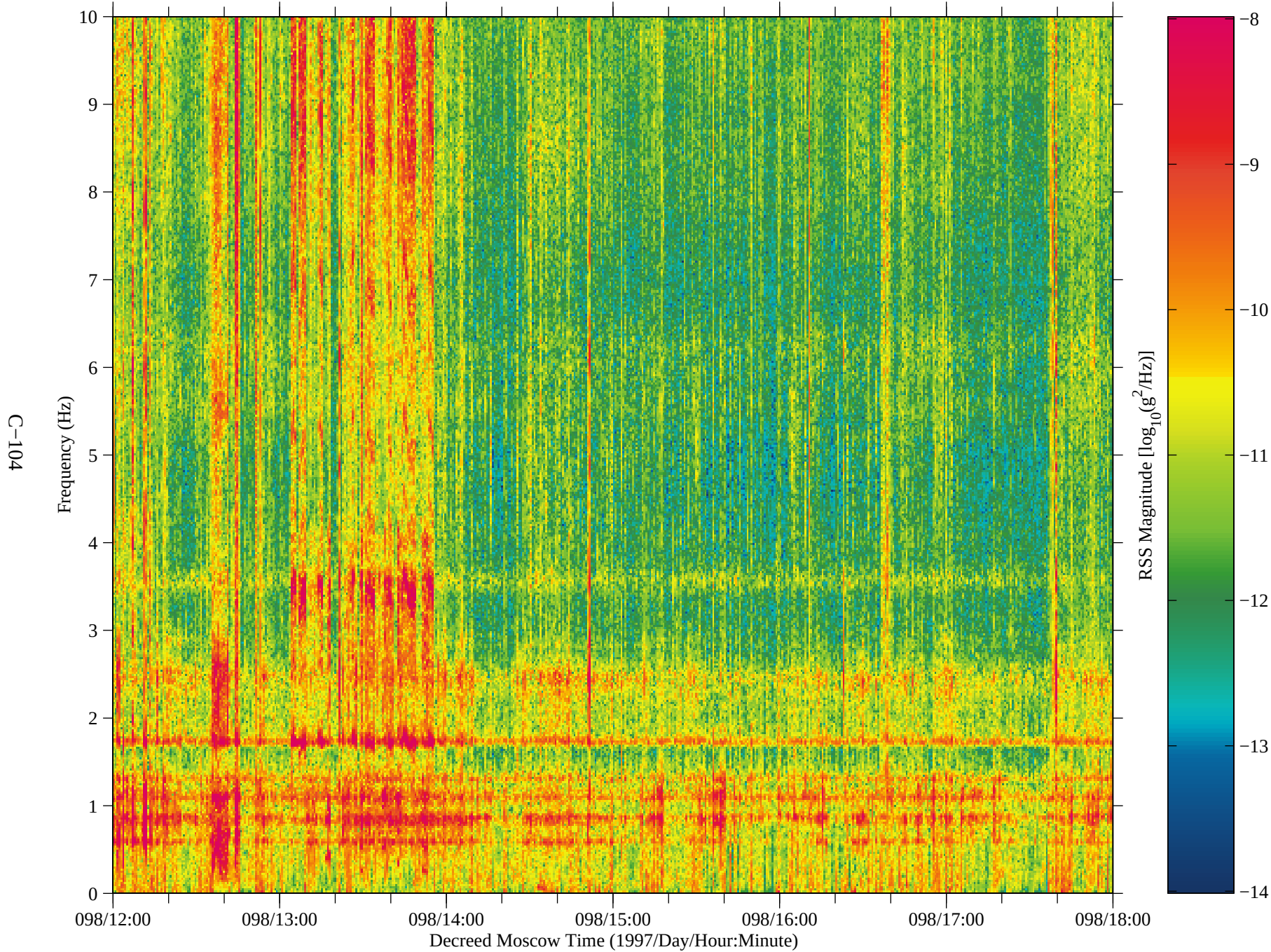
Figure 91: SAMS data from Mir, TSH B (fc=10 Hz)
