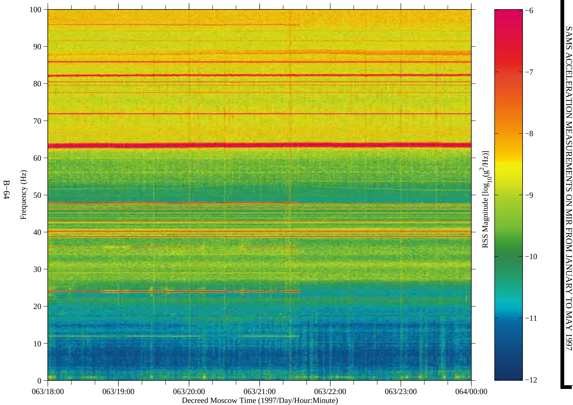
Figure 55: SAMS data from Mir, TSH A (fc=100 Hz)
