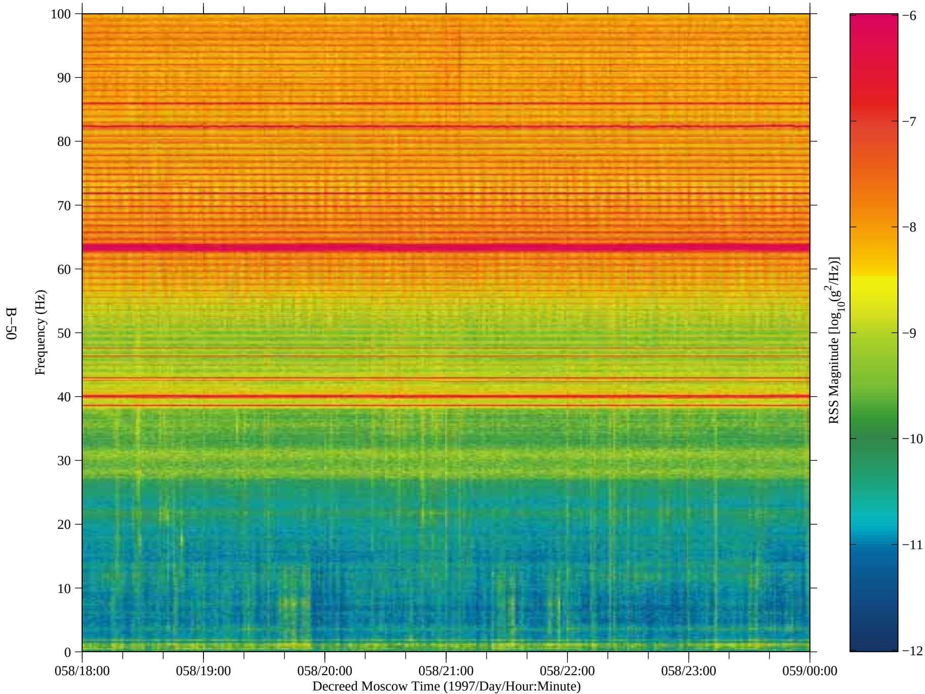
Figure 42: SAMS data from Mir, TSH A (fc=100 Hz)
