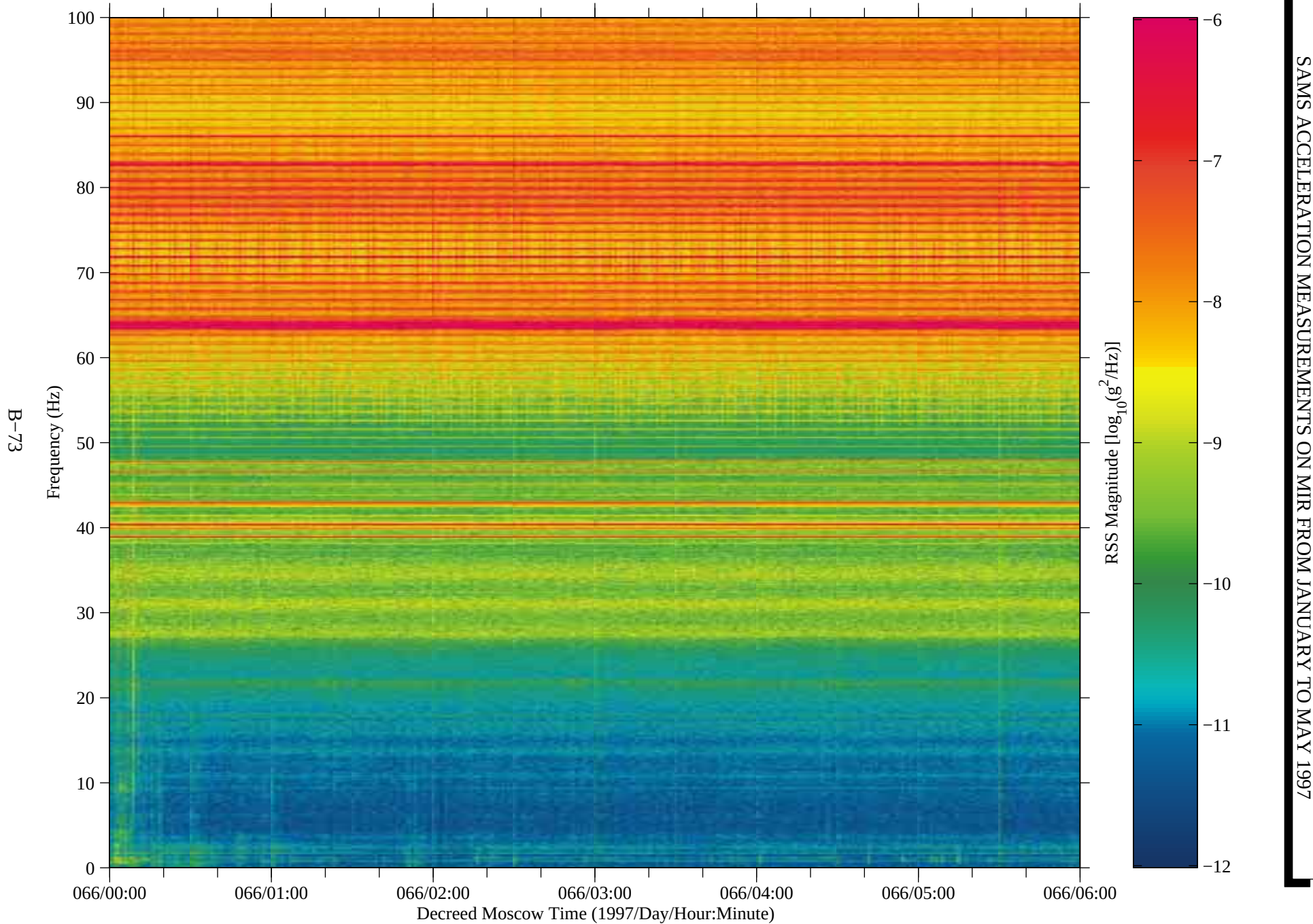
Figure 64: SAMS data from Mir, TSH A (fc=100 Hz)
