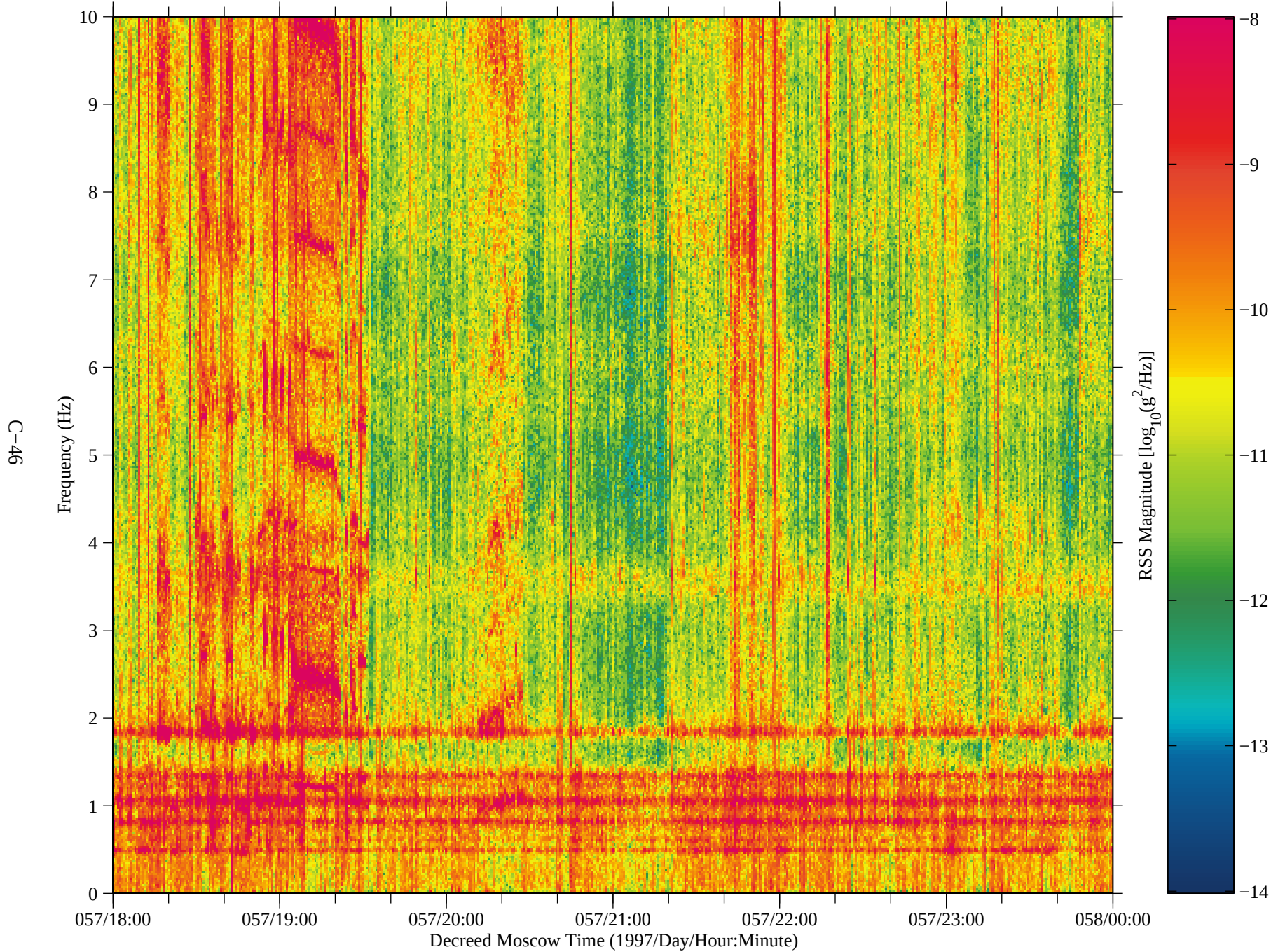
Figure 38: SAMS data from Mir, TSH B (fc=10 Hz)
