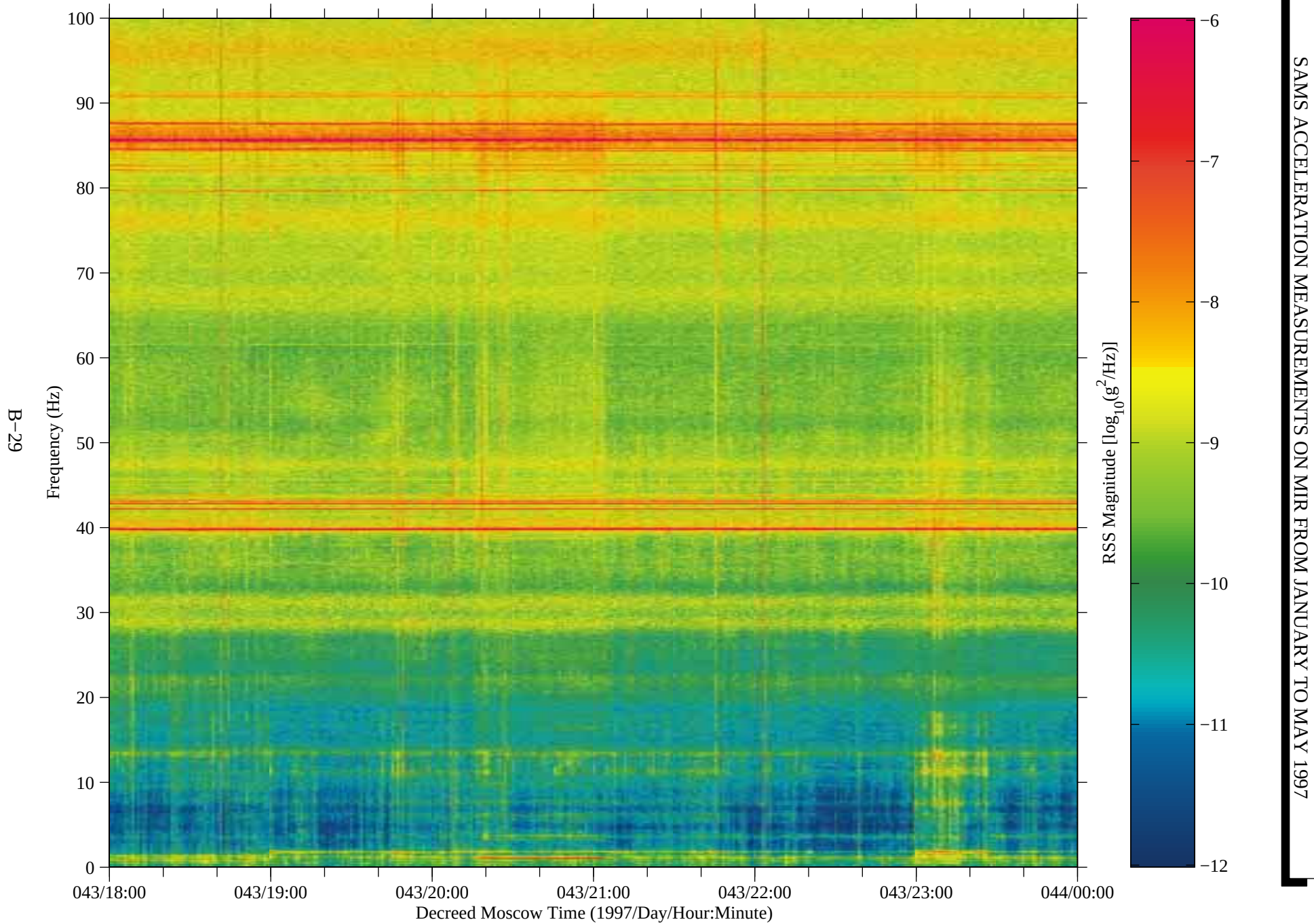
Figure 23: SAMS data from Mir, TSH A (fc=100 Hz)
