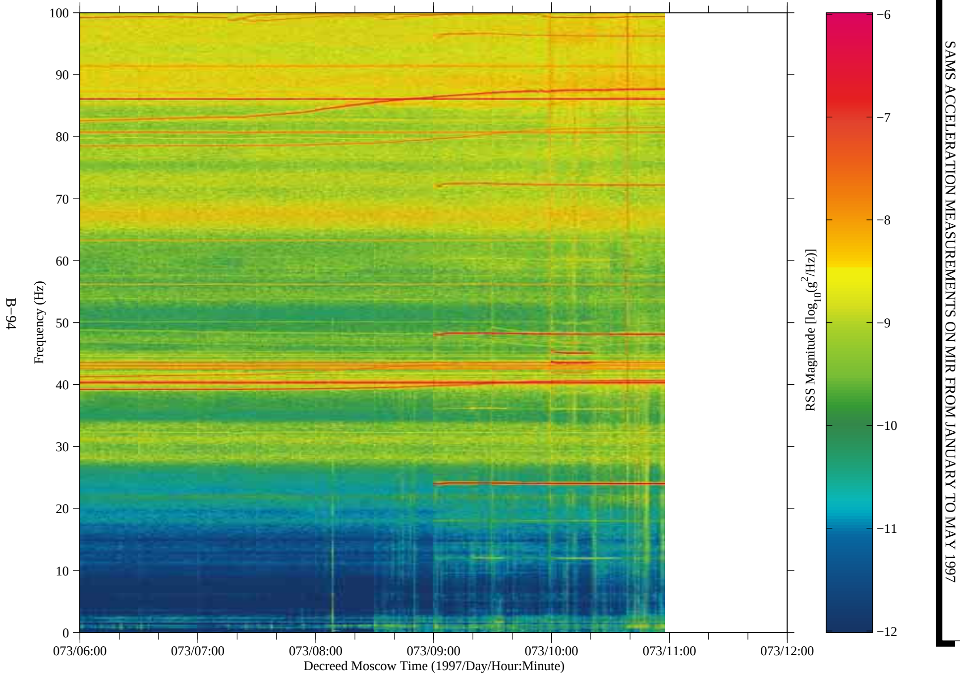
Figure 83: SAMS data from Mir, TSH A (fc=100 Hz)
