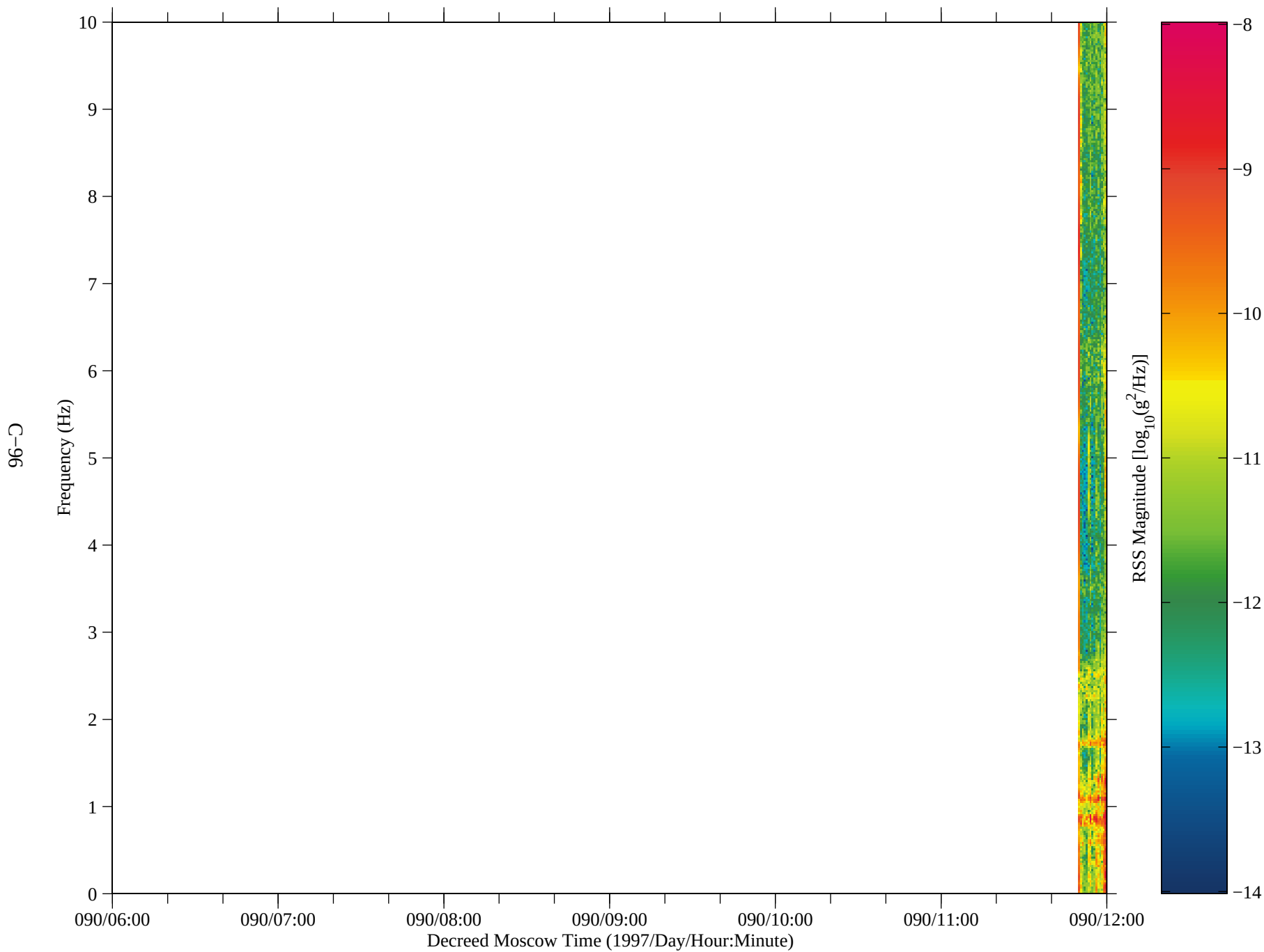
Figure 84: SAMS data from Mir, TSH B (fc=10 Hz)
