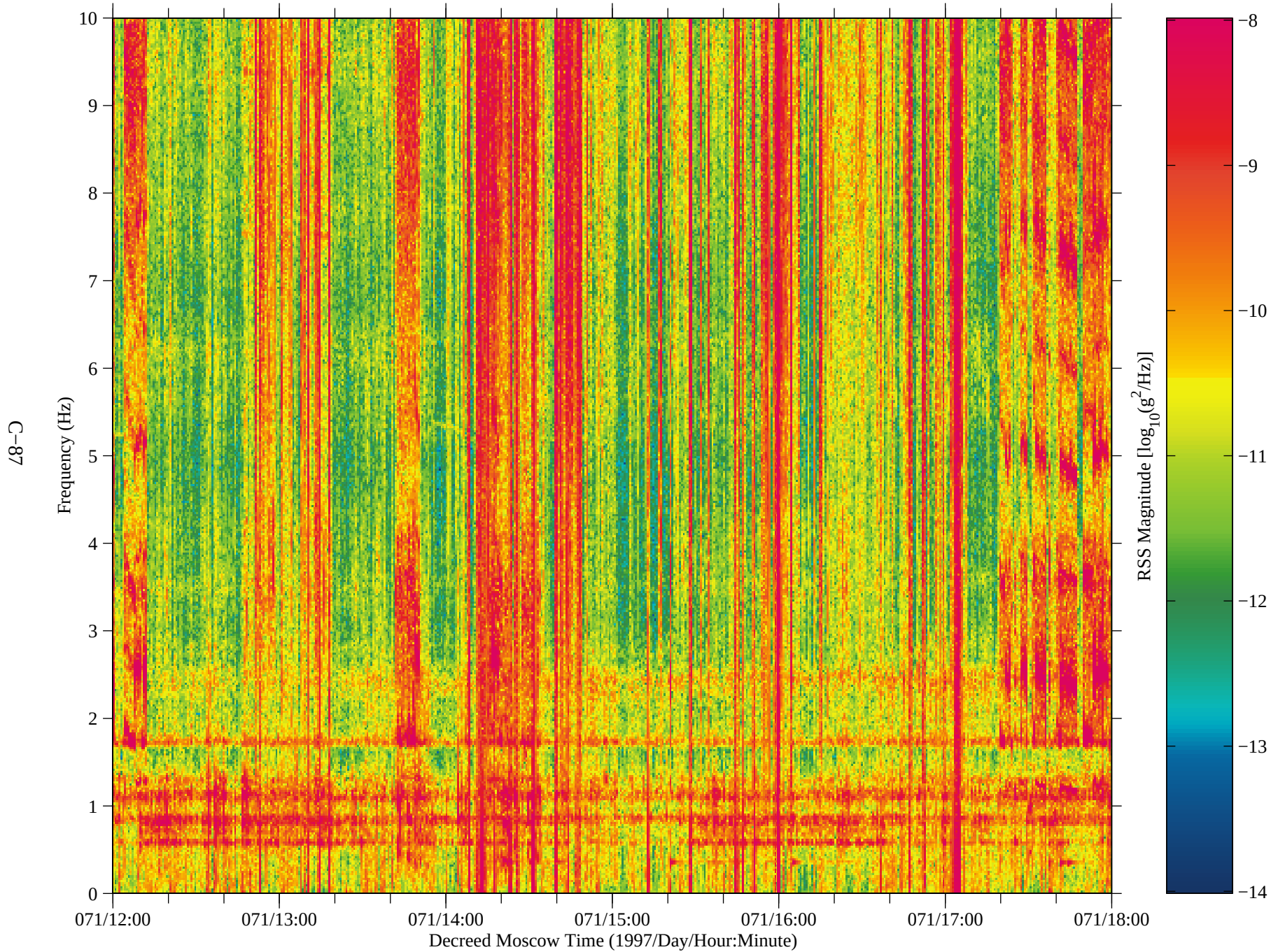
Figure 76: SAMS data from Mir, TSH B (fc=10 Hz)
