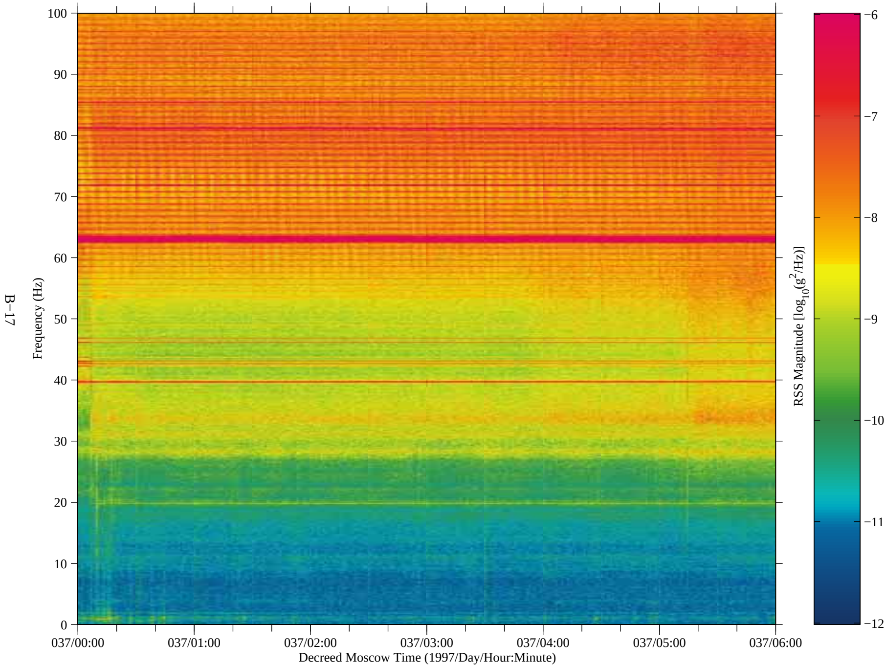
Figure 13: SAMS data from Mir, TSH A (fc=100 Hz)
