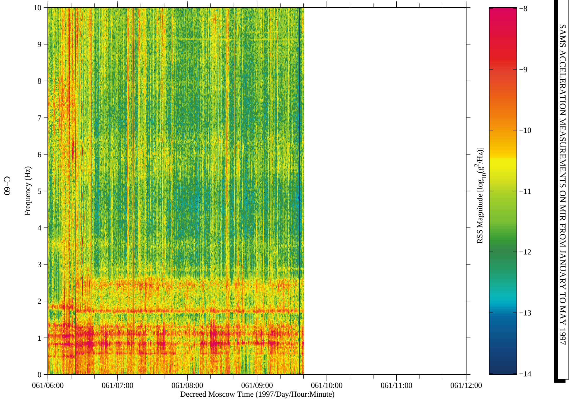
Figure 52: SAMS data from Mir, TSH B (fc=10 Hz)
