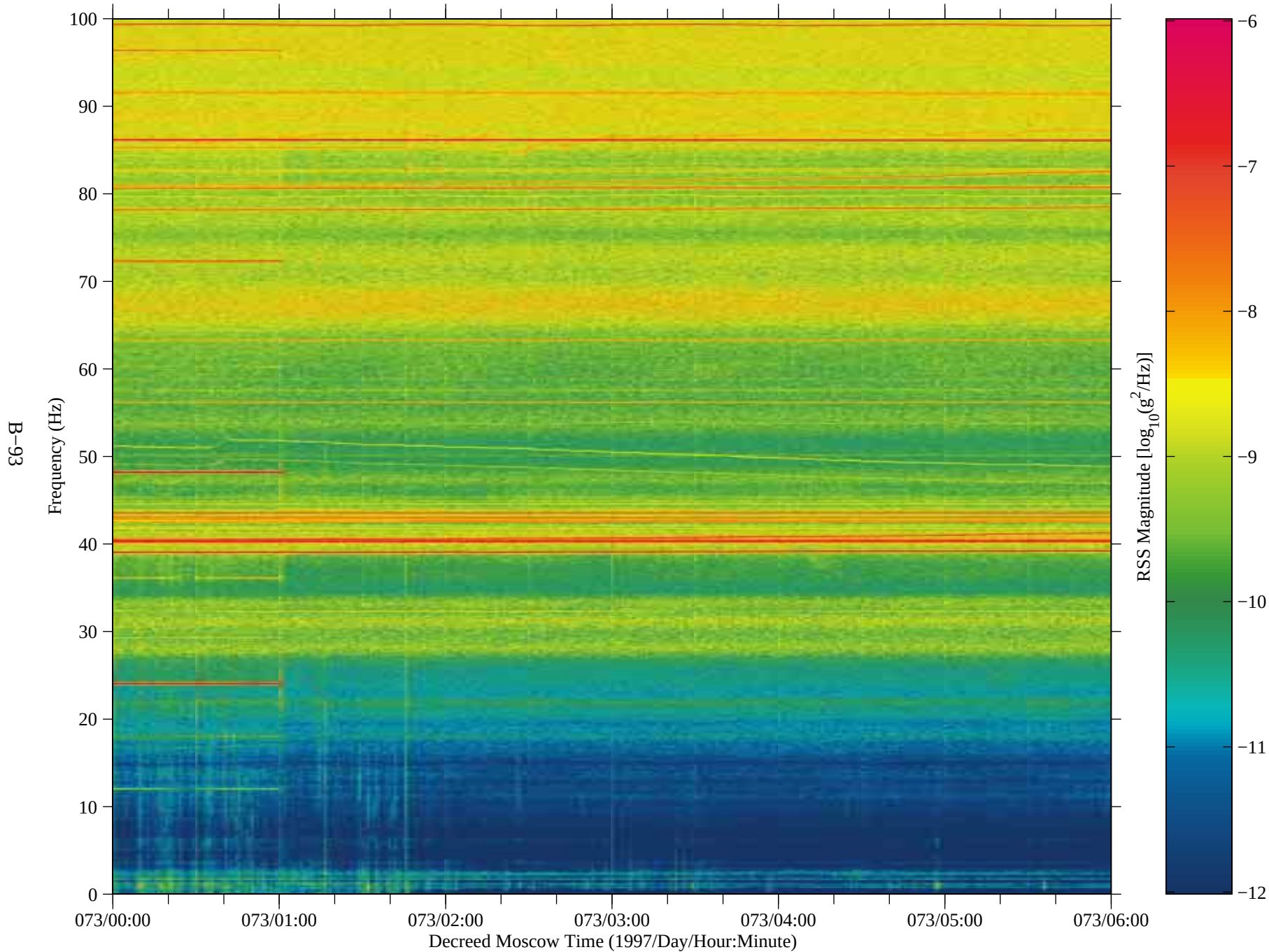
Figure 82: SAMS data from Mir, TSH A (fc=100 Hz)
