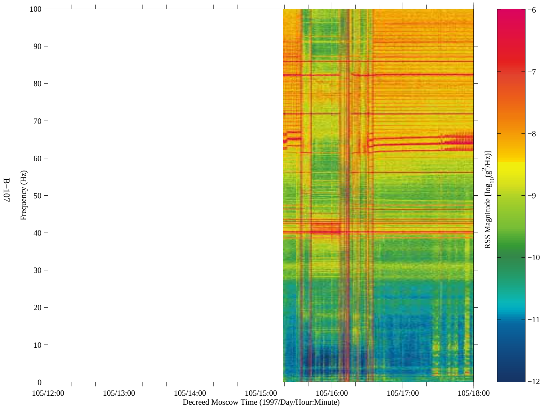
Figure 93: SAMS data from Mir, TSH A (fc=100 Hz)
