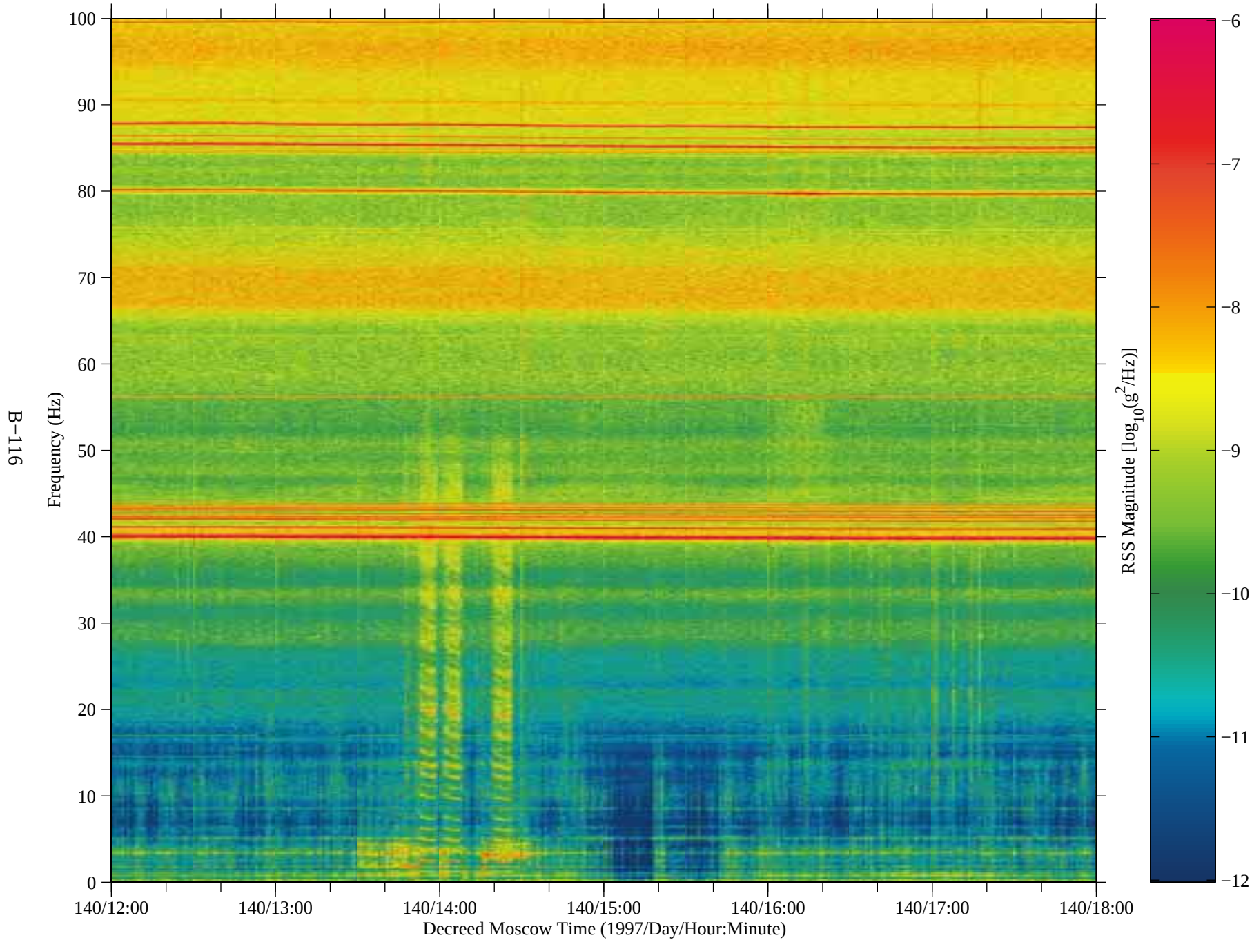
Figure 100: SAMS data from Mir, TSH A (fc=100 Hz)
