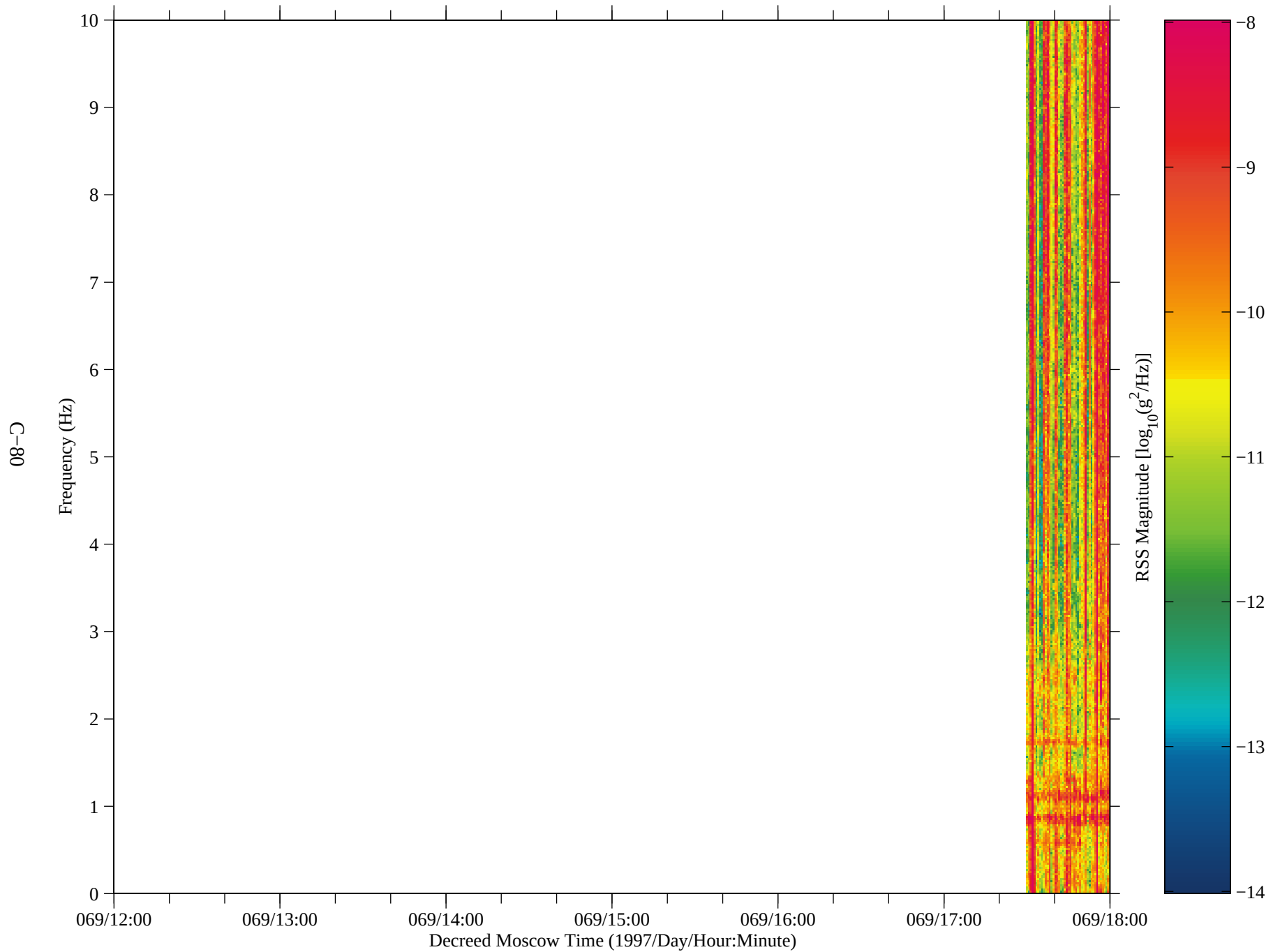
Figure 70: SAMS data from Mir, TSH B (fc=10 Hz)
