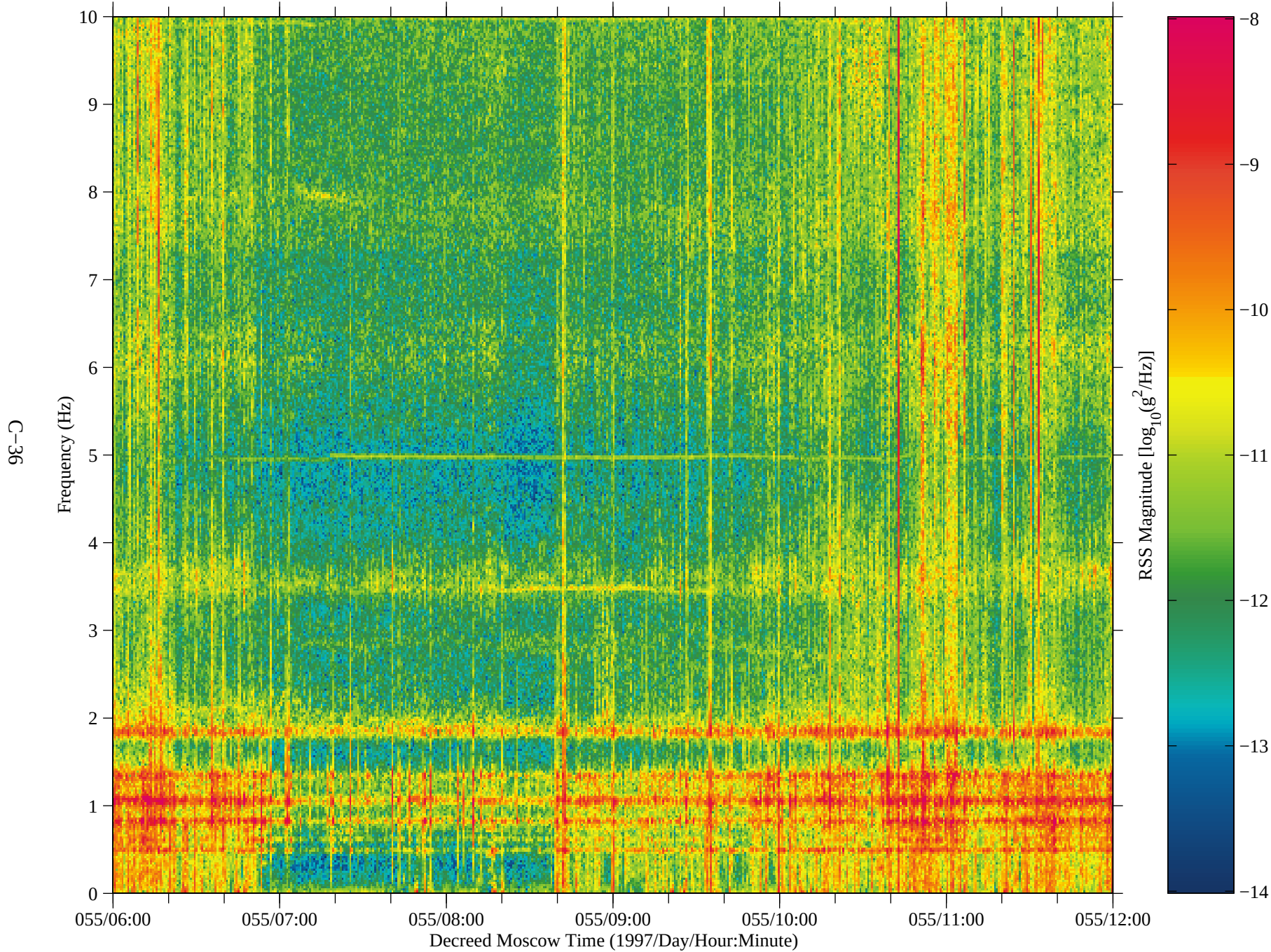
Figure 29: SAMS data from Mir, TSH B (fc=10 Hz)
