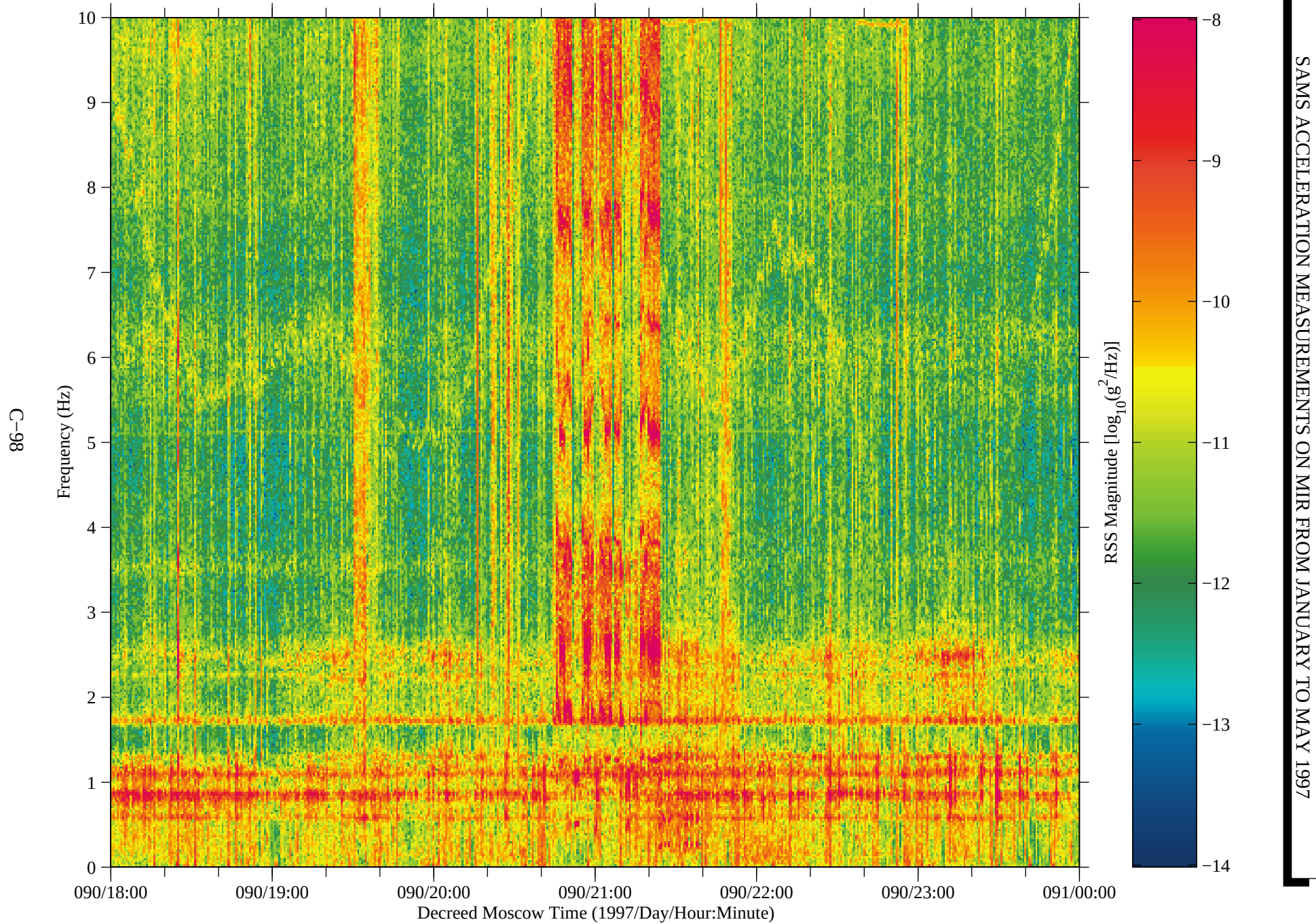
Figure 86: SAMS data from Mir, TSH B (fc=10 Hz)
