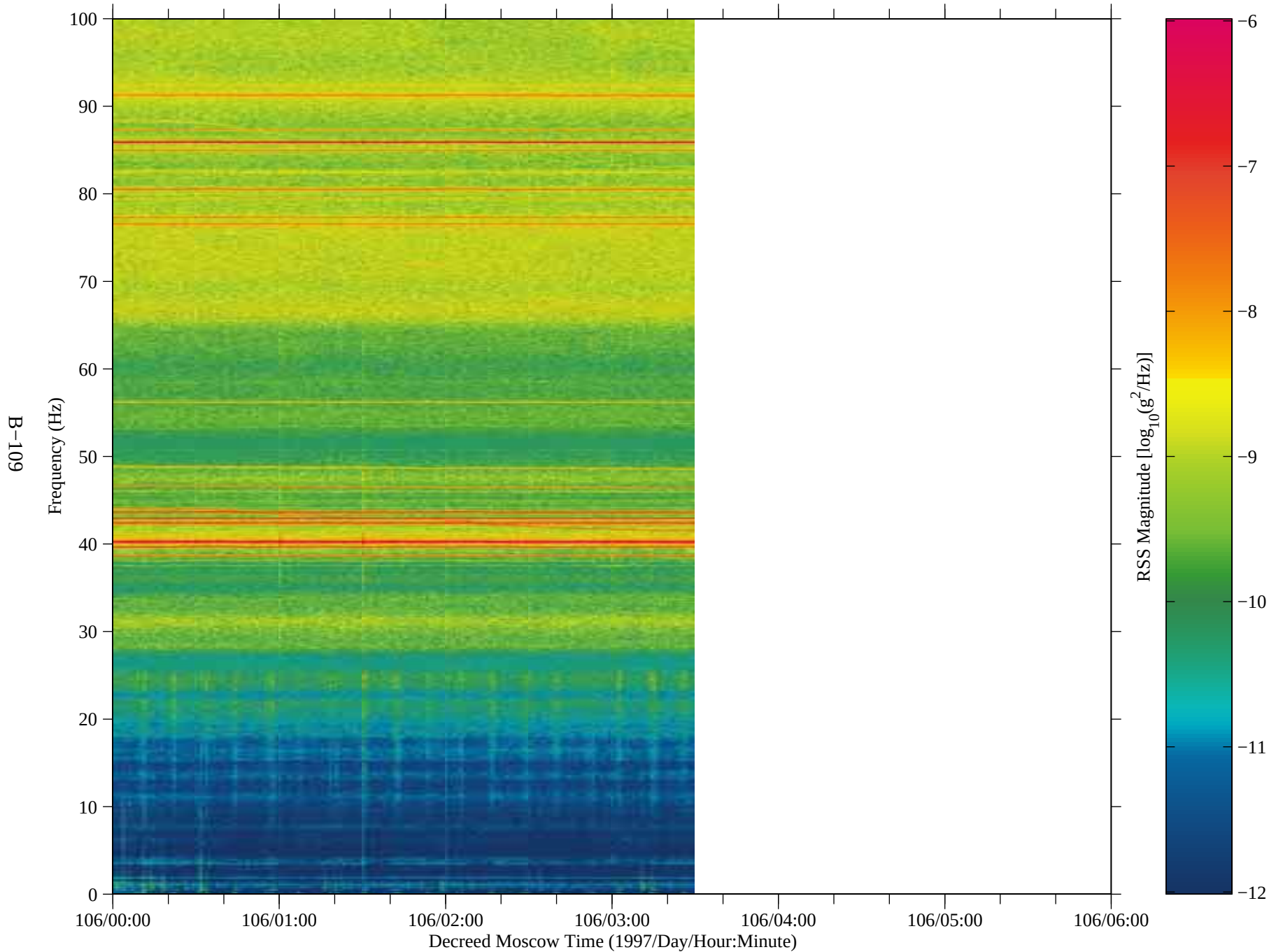
Figure 95: SAMS data from Mir, TSH A (fc=100 Hz)
