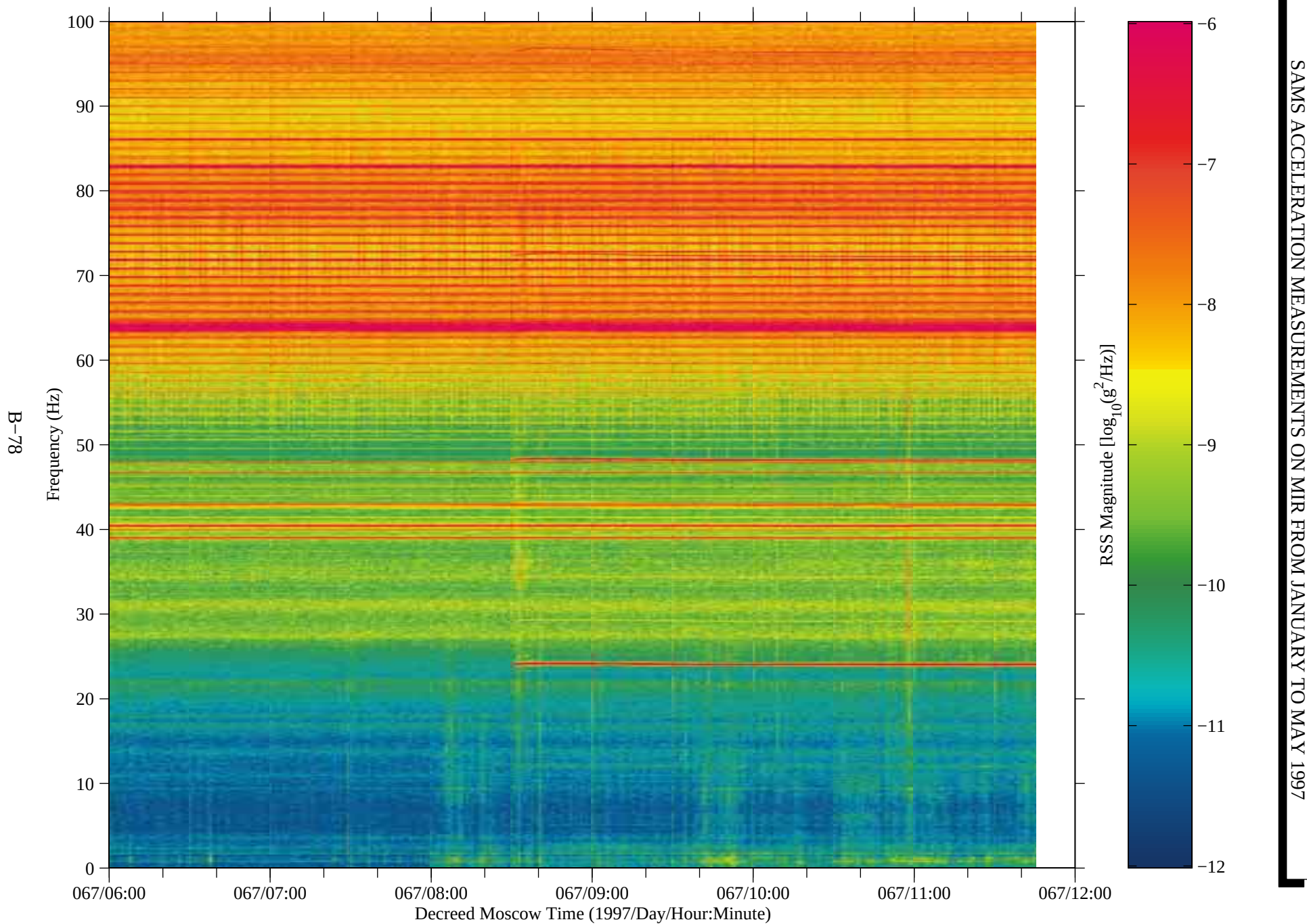
Figure 69: SAMS data from Mir, TSH A (fc=100 Hz)
