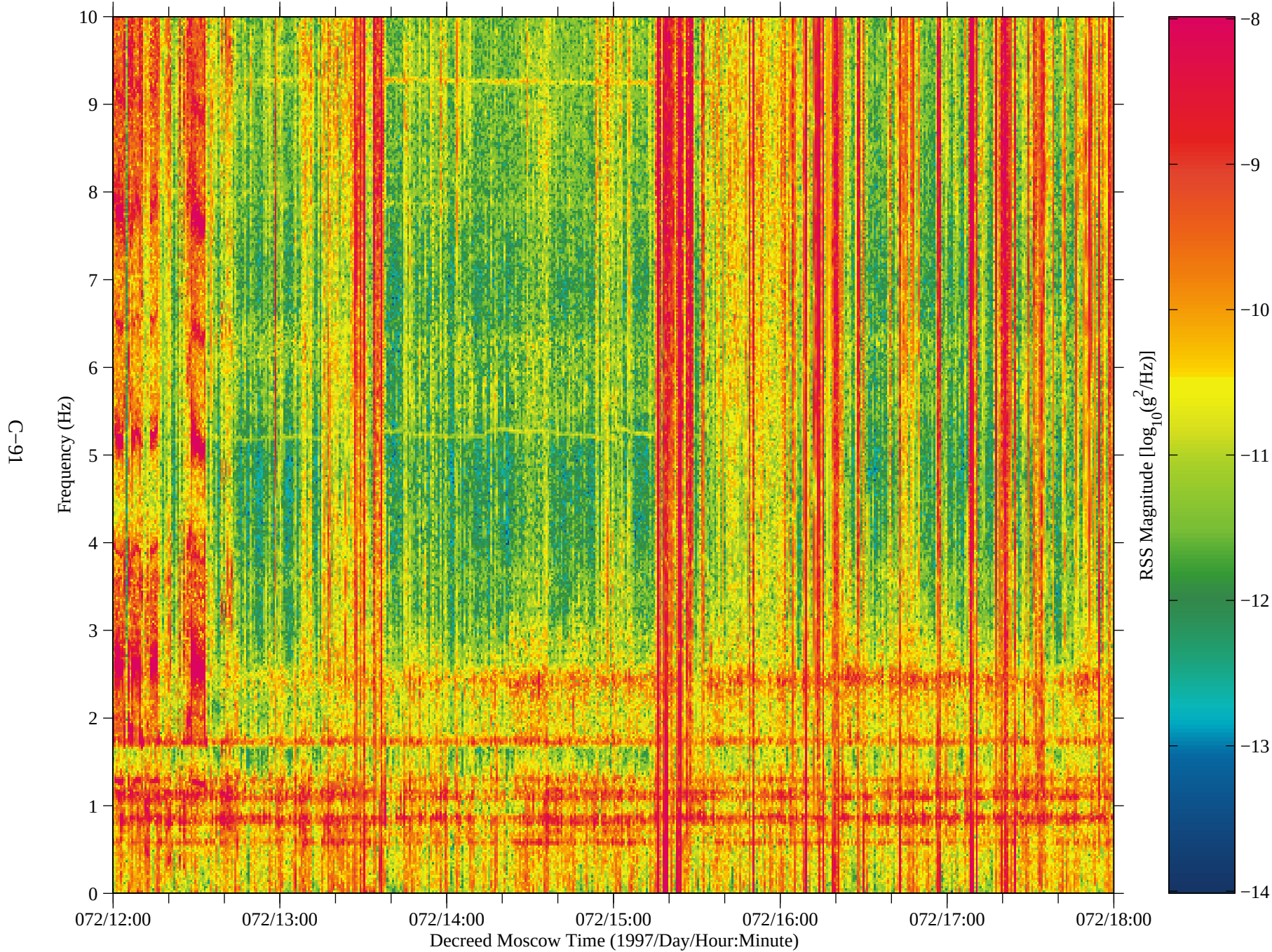
Figure 80: SAMS data from Mir, TSH B (fc=10 Hz)
