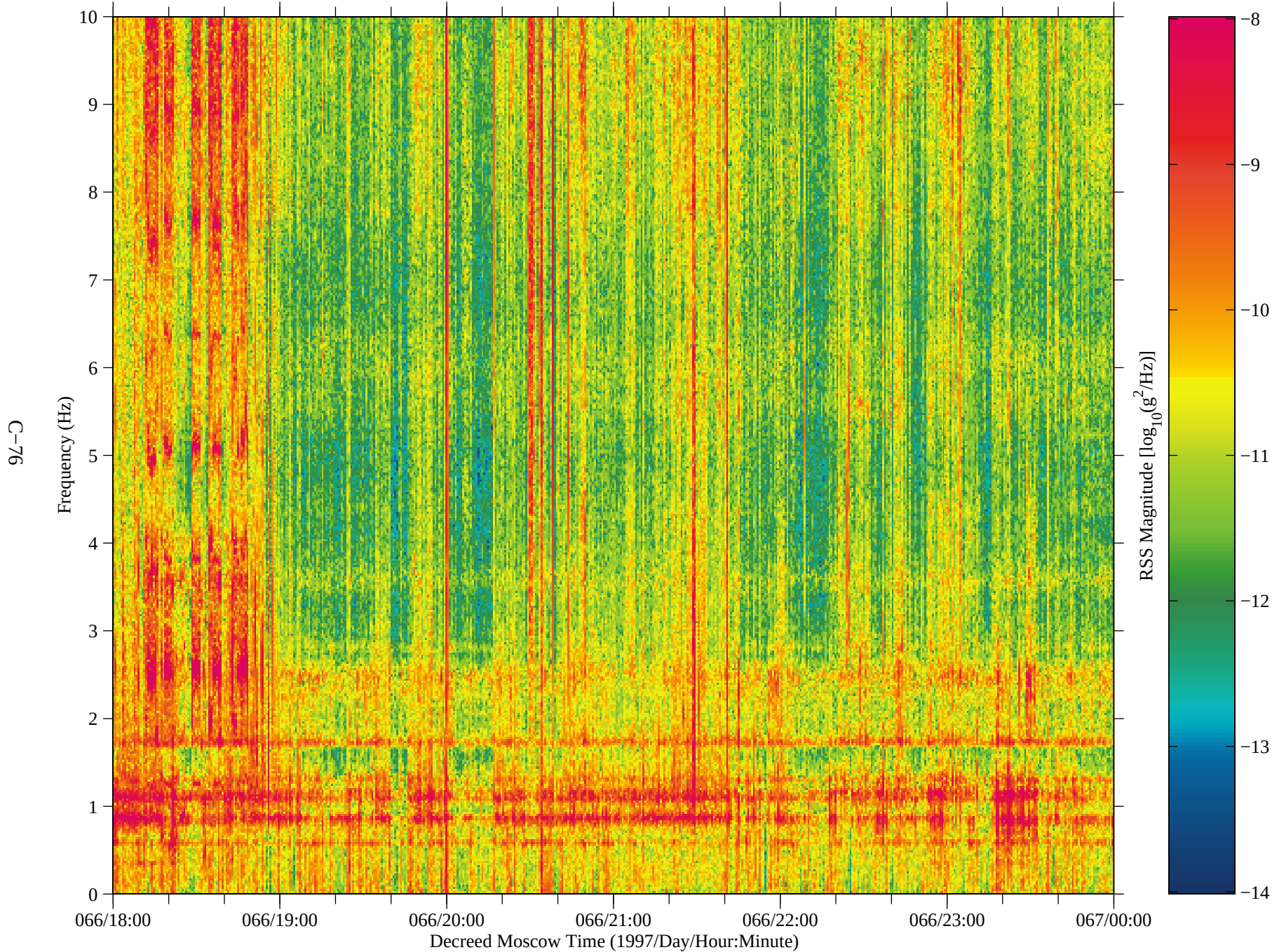
Figure 67: SAMS data from Mir, TSH B (fc=10 Hz)
