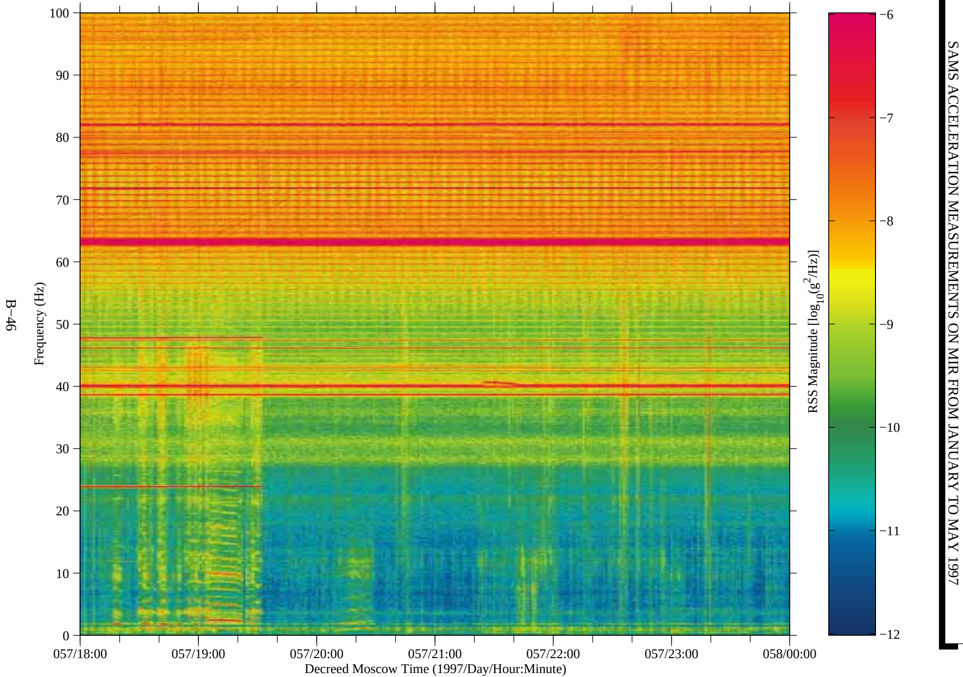
Figure 38: SAMS data from Mir, TSH A (fc=100 Hz)
