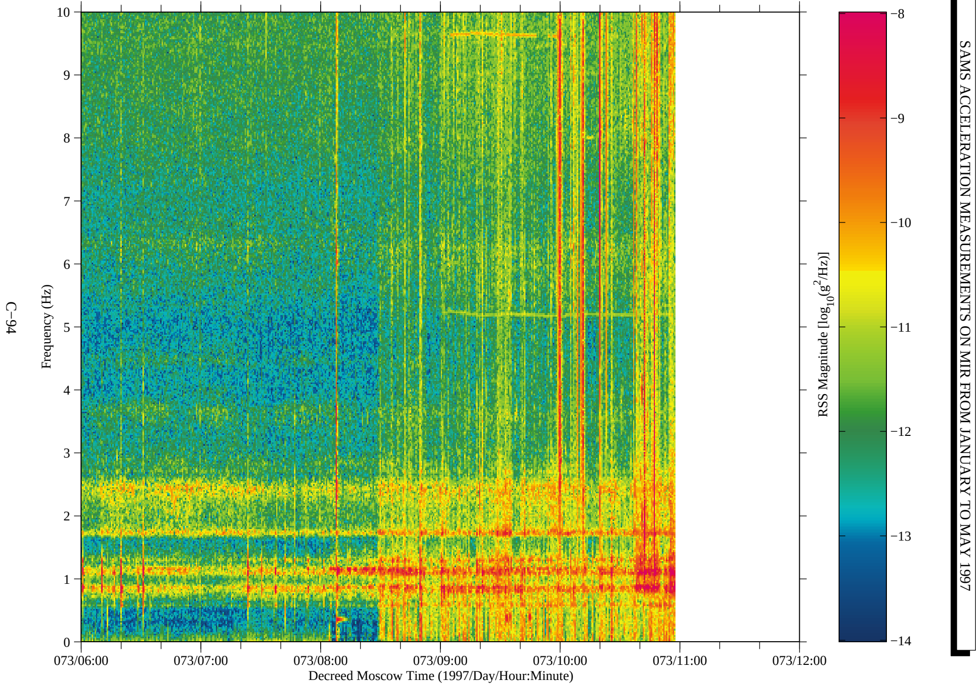
Figure 83: SAMS data from Mir, TSH B (fc=10 Hz)
