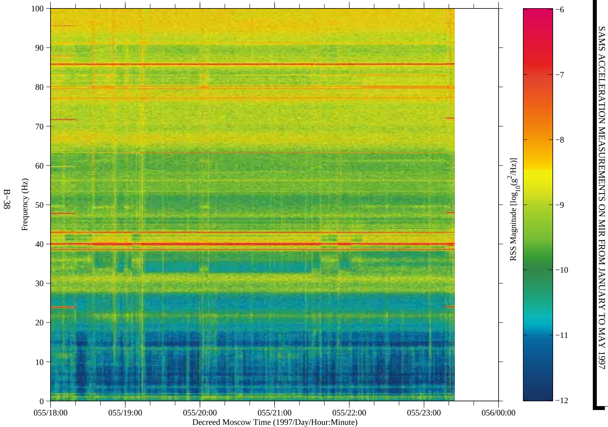
Figure 31: SAMS data from Mir, TSH A (fc=100 Hz)
