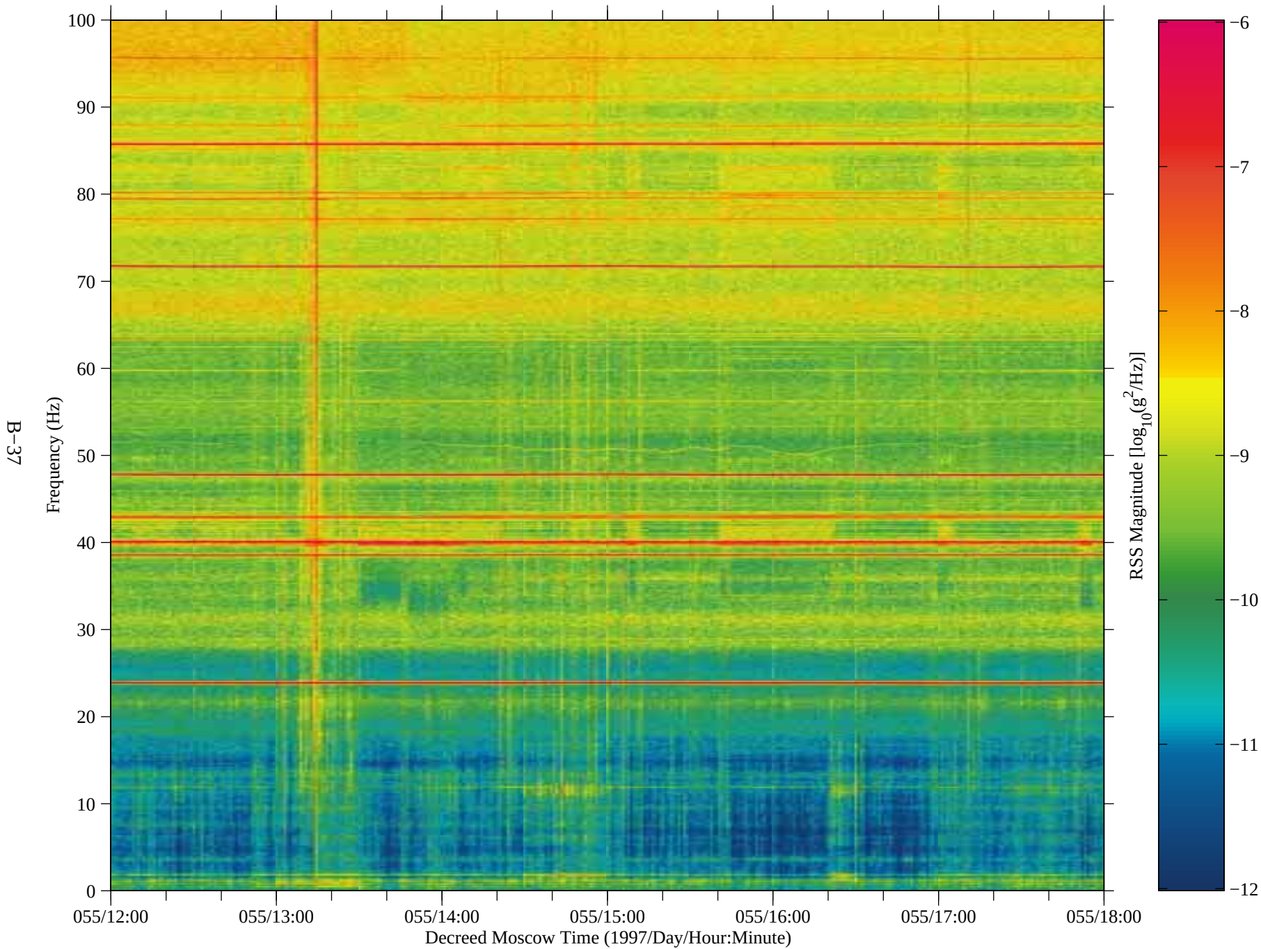
Figure 30: SAMS data from Mir, TSH A (fc=100 Hz)
