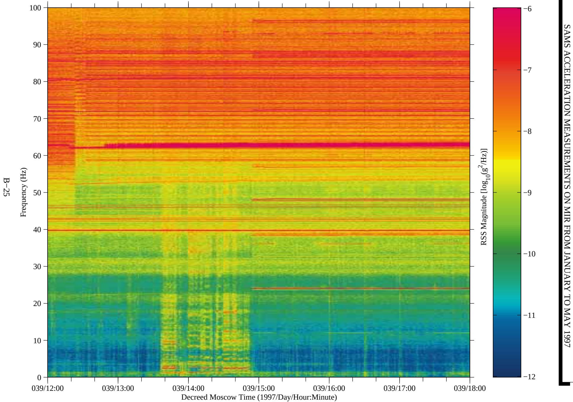
Figure 20: SAMS data from Mir, TSH A (fc=100 Hz)
