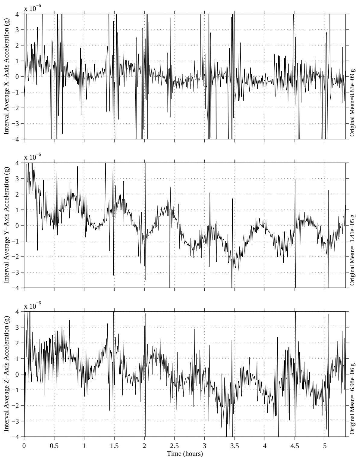
Figure 11. Solar inertial attitude quasi-steady accelerations
