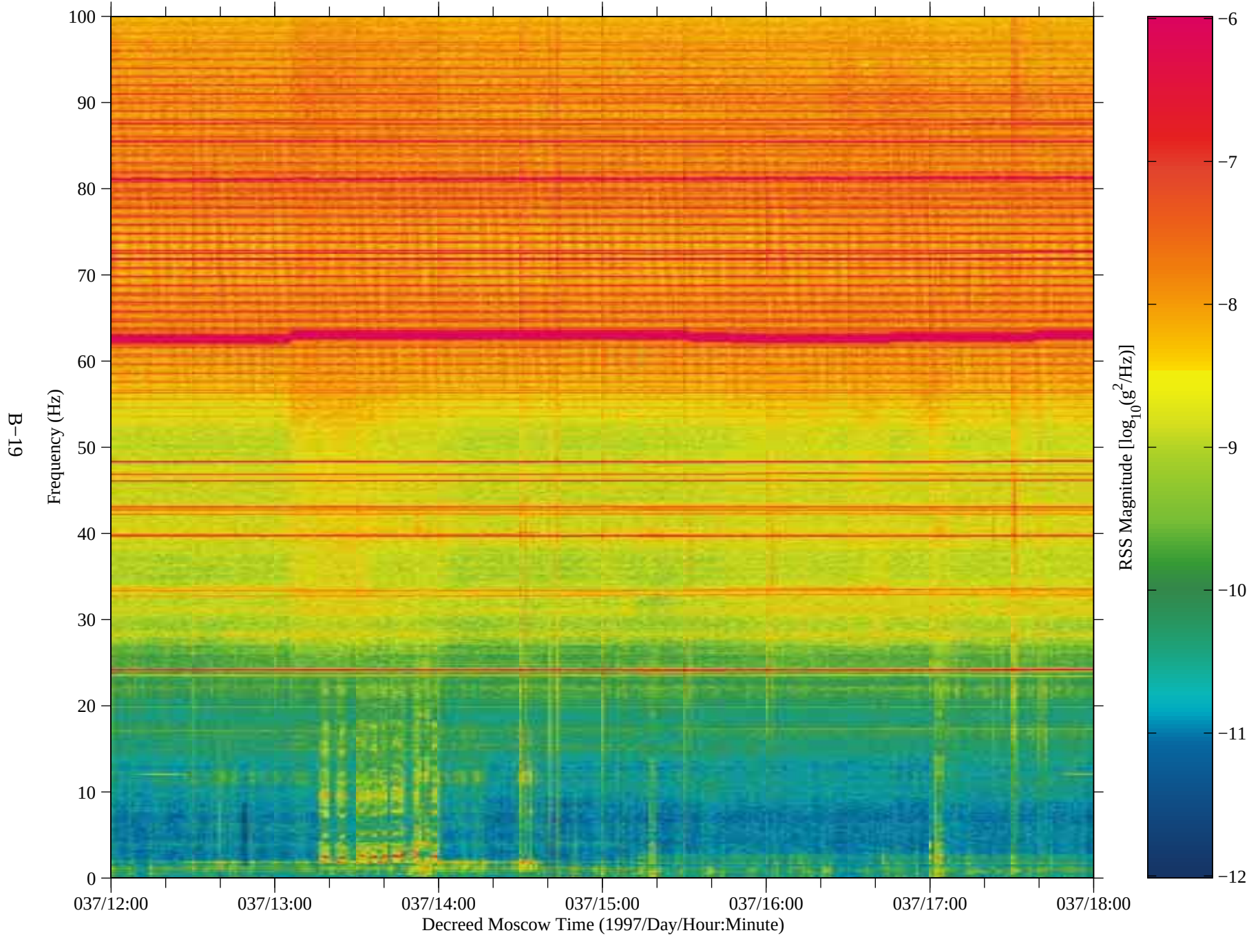
Figure 15: SAMS data from Mir, TSH A (fc=100 Hz)
