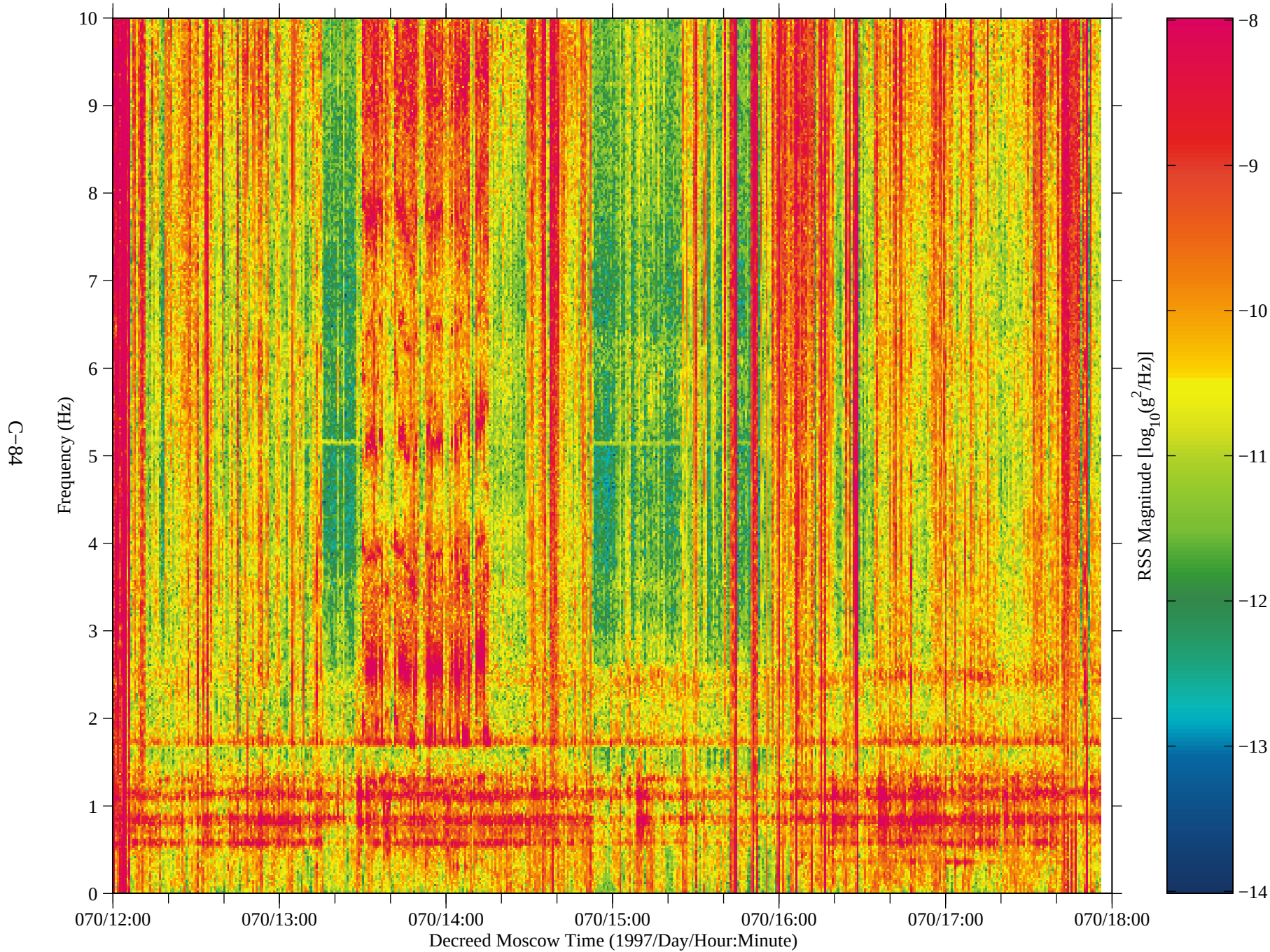
Figure 74: SAMS data from Mir, TSH B (fc=10 Hz)
