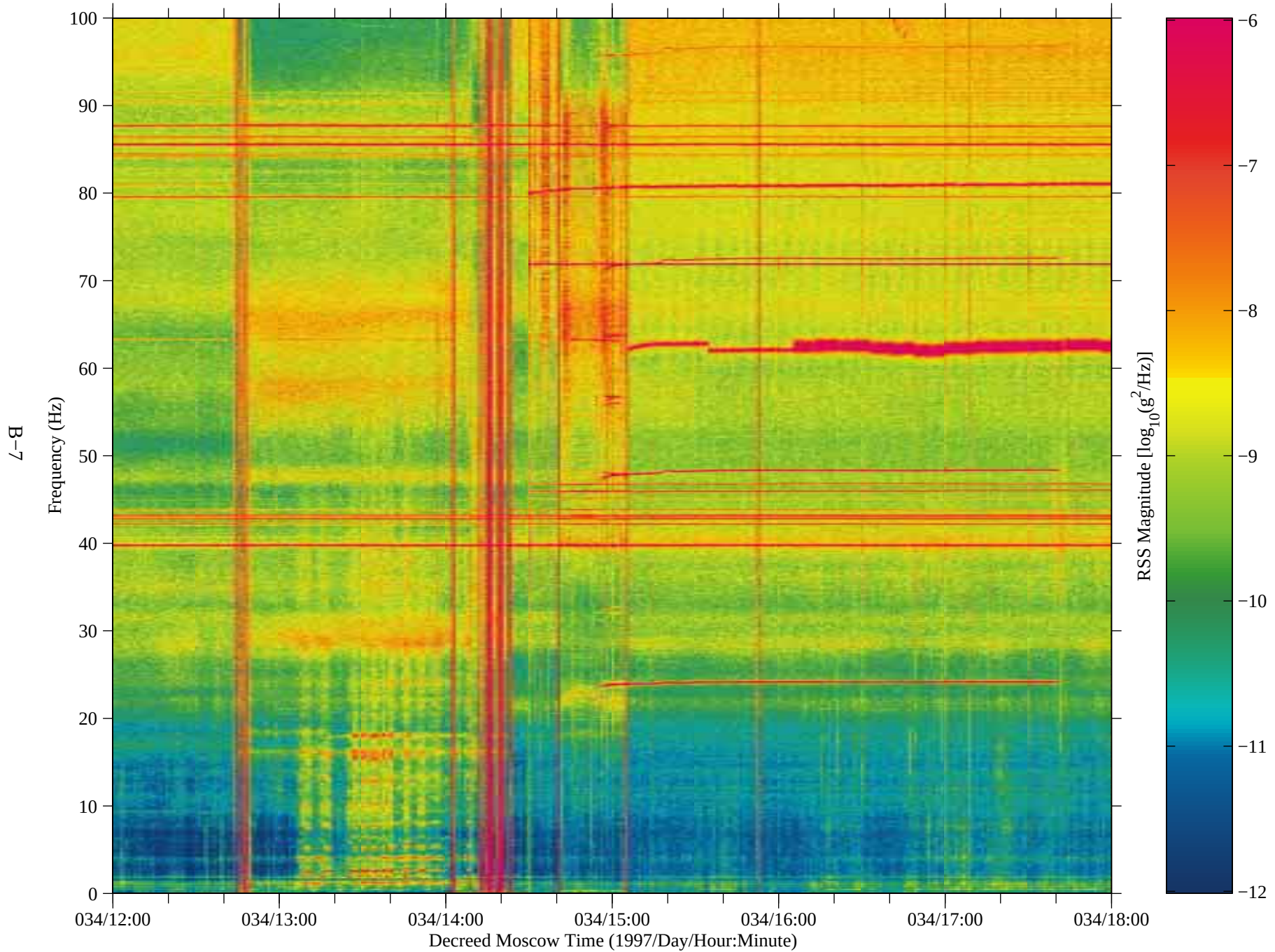
Figure 3: SAMS data from Mir, TSH A (fc=100 Hz)
