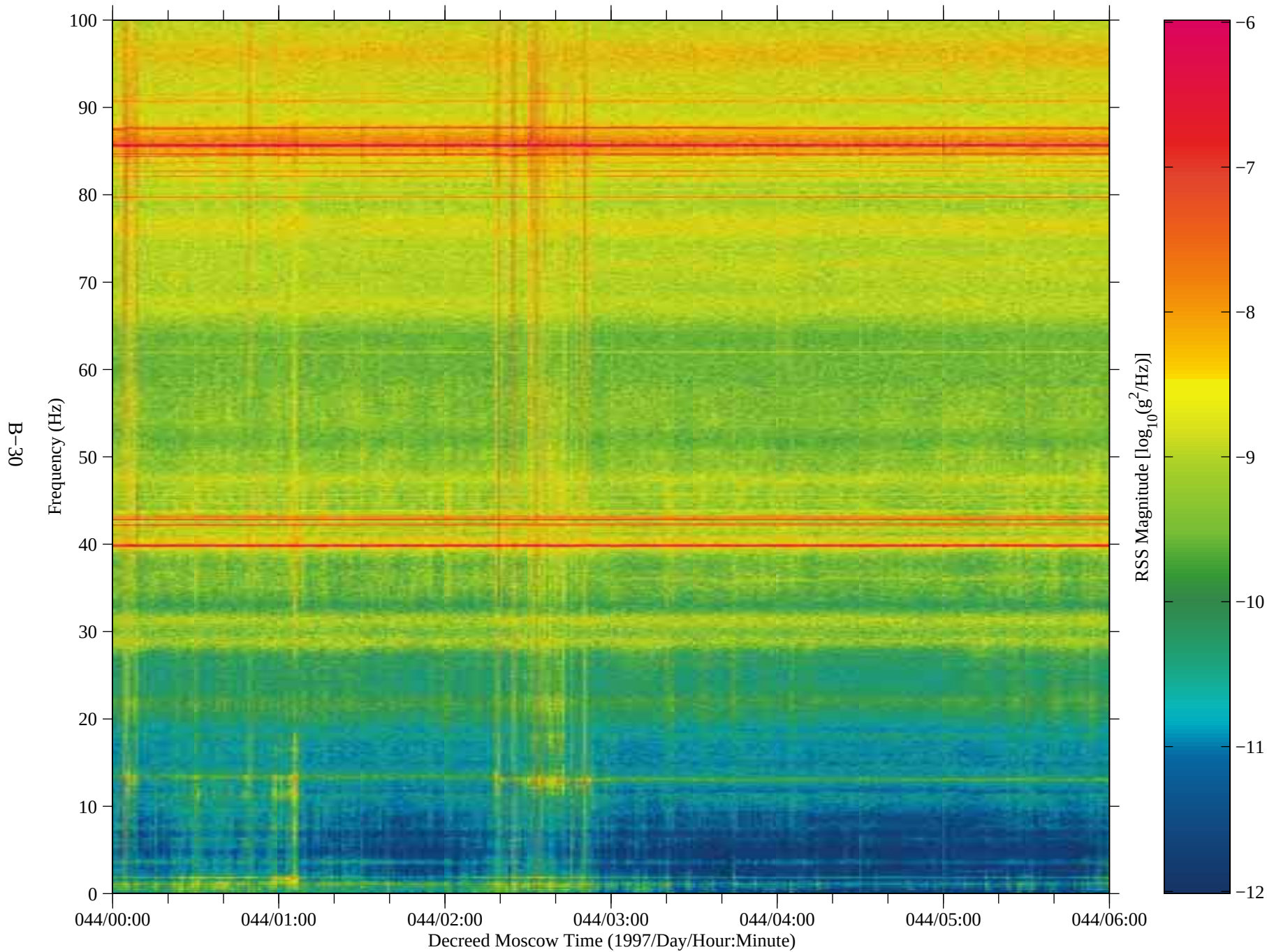
Figure 24: SAMS data from Mir, TSH A (fc=100 Hz)
