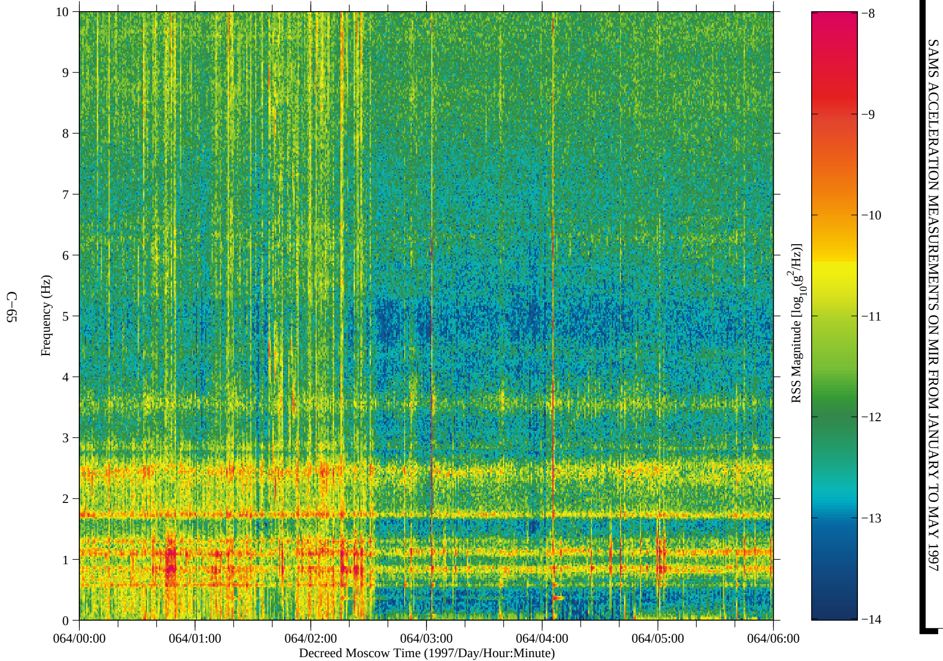
Figure 56: SAMS data from Mir, TSH B (fc=10 Hz)
