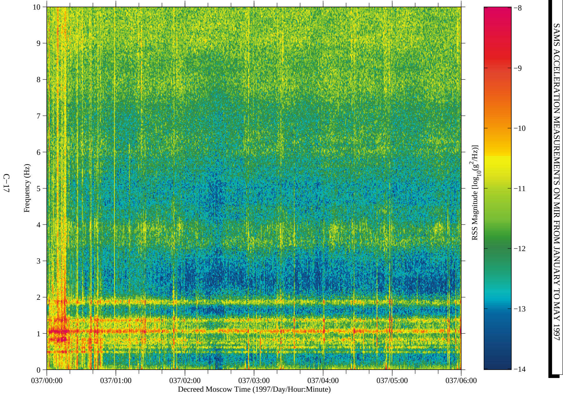
Figure 13: SAMS data from Mir, TSH B (fc=10 Hz)
