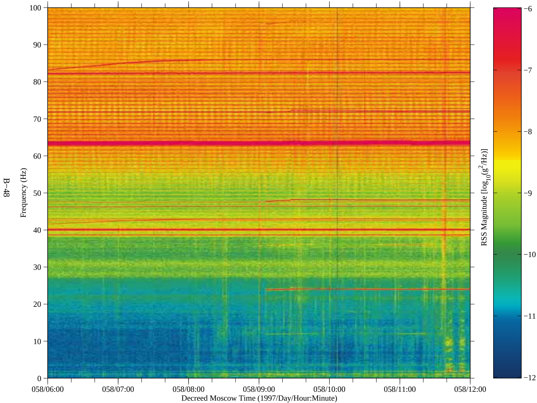
Figure 40: SAMS data from Mir, TSH A (fc=100 Hz)
