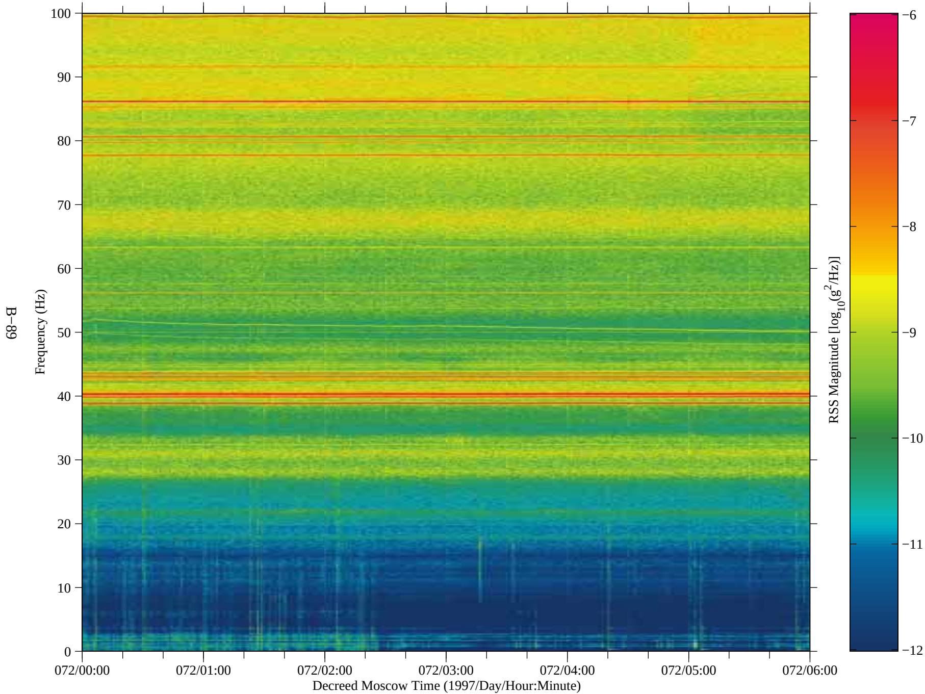
Figure 78: SAMS data from Mir, TSH A (fc=100 Hz)
