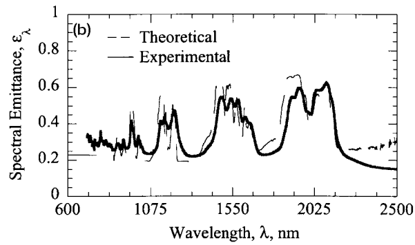
Fig. 10. Comparison of experimental and calculated spectral emittance of \text{Er}_{1.5}\text{Ho}_{1.5}\text{Al}_5\text{O}_{12} with platinum substrate. Thickness, d = 0.65 mm, substrate temperature, T_s = 1218 K, front face temperature, T_f = 1128 K, \Delta T = 0.074 . (a) 600 < \lambda < 10,000 nm. (b) 600 < \lambda < 2500 nm.
