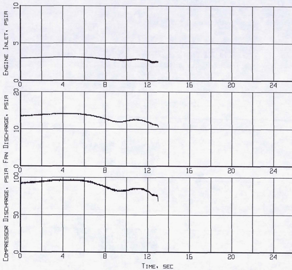
Figure B10-6. Measured inlet/engine entry and engine internal pressures time histories (Flight 240, Test Point 43b).
