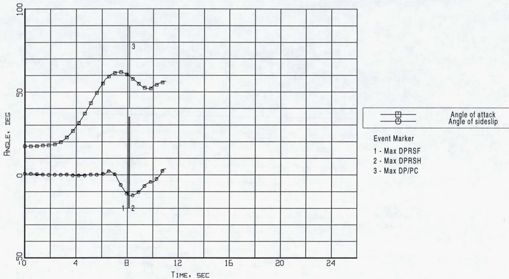
Figure B7-11. Event markers superposed on the aerodynamic flowstream descriptor time histories (Flight 238, Test Point 40b).
