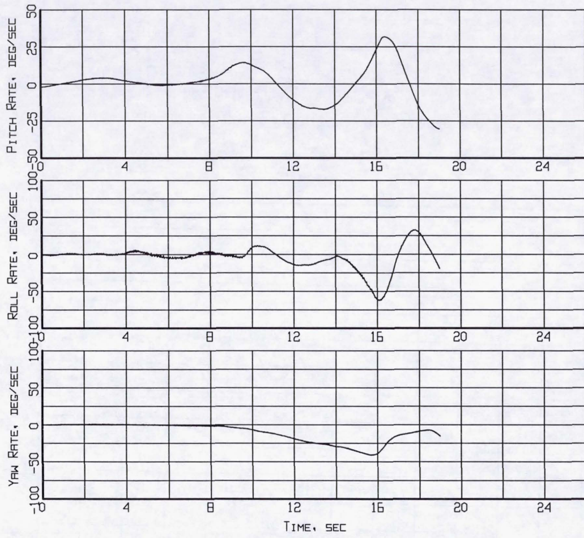
Figure B1-2. Aircraft Motion - Rate-of-Change of Pitch, Roll and Heading (Flight 239, Test Point 34b).
