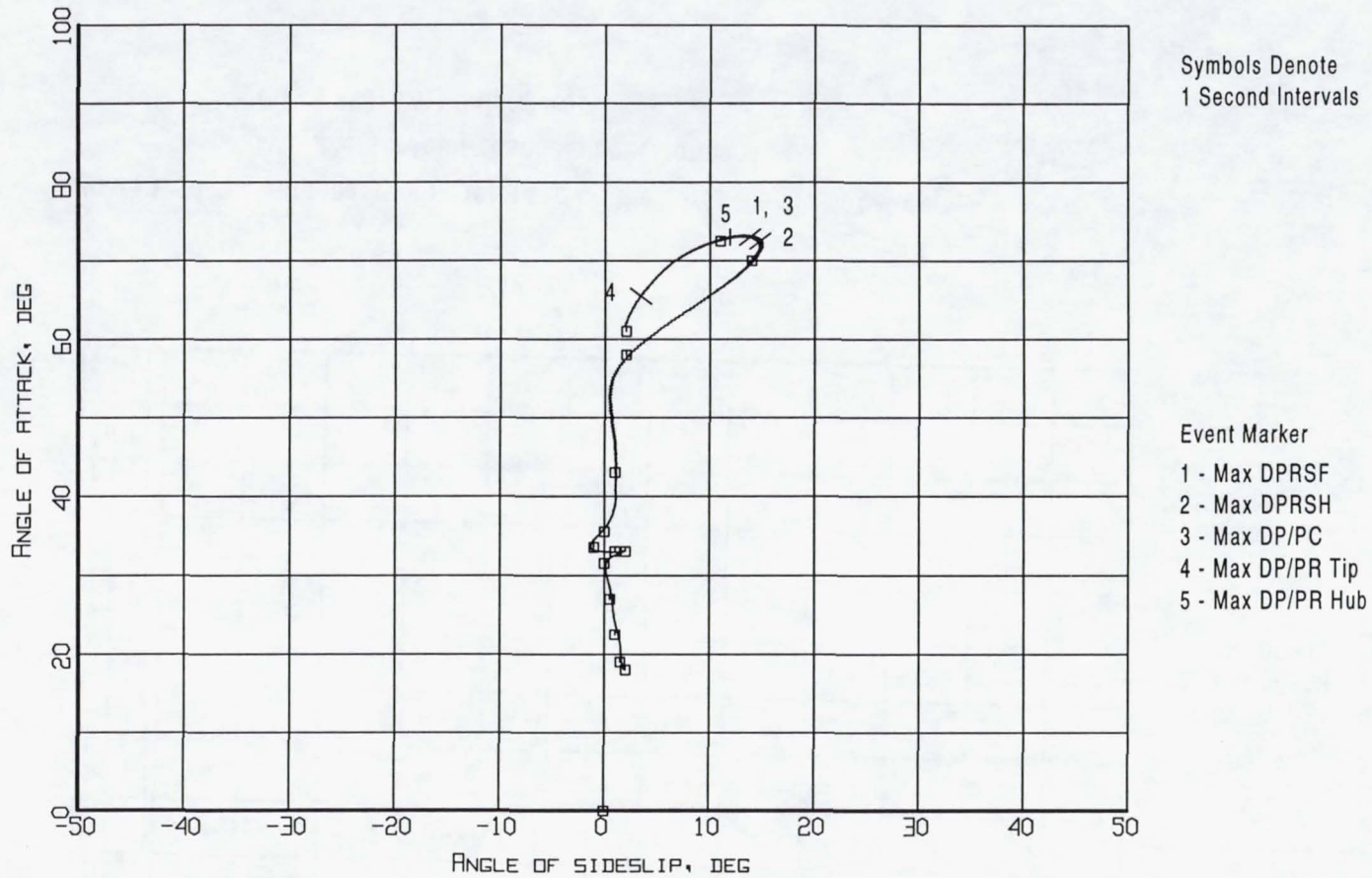
Figure B1-13. Event markers superposed on the aerodynamic flowstream descriptors trajectory (Flight 239, Test Point 34b).
