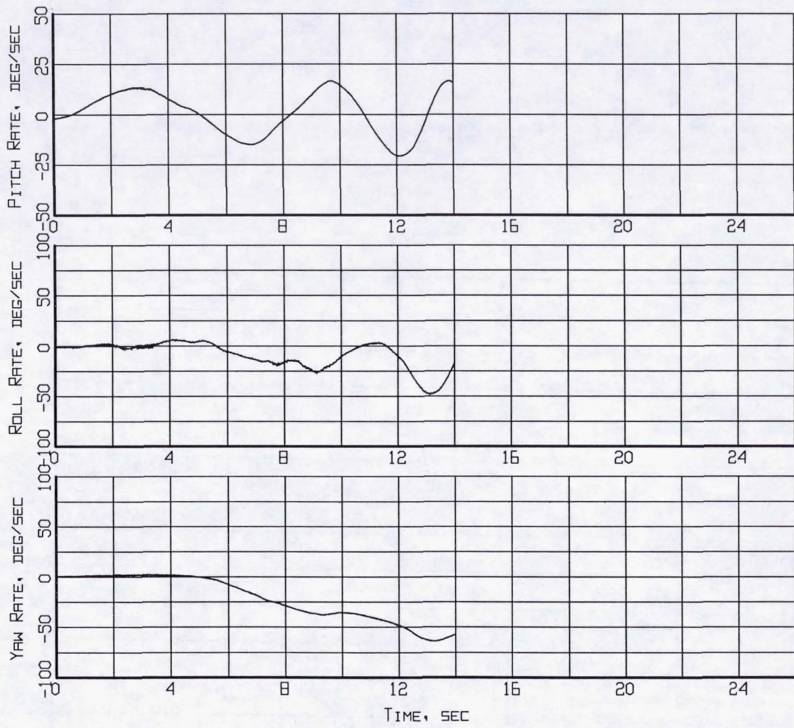
Figure B3-2. Aircraft Motion - Rate-of-Change of Pitch, Roll and Heading (Flight 238, Test Point 36b).
