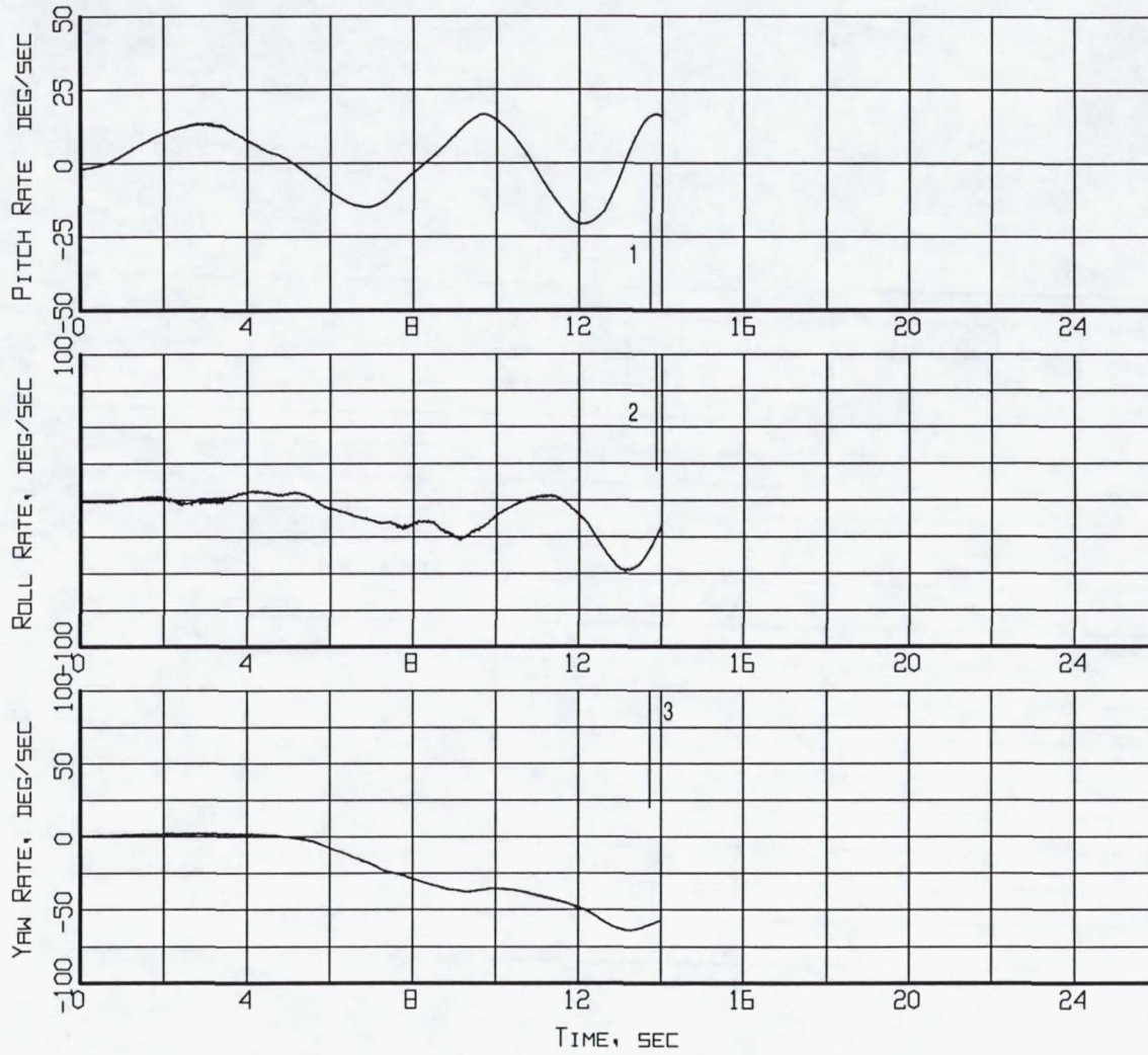
Figure B3-9. Event markers superposed on the aircraft motion time histories (Flight 238, Test Point 36b).
