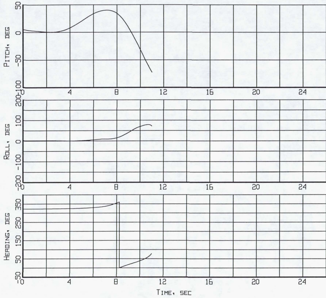
Figure B7-1. Aircraft attitude - Pitch, Roll, and Heading (Flight 238, Test Point 40b).
