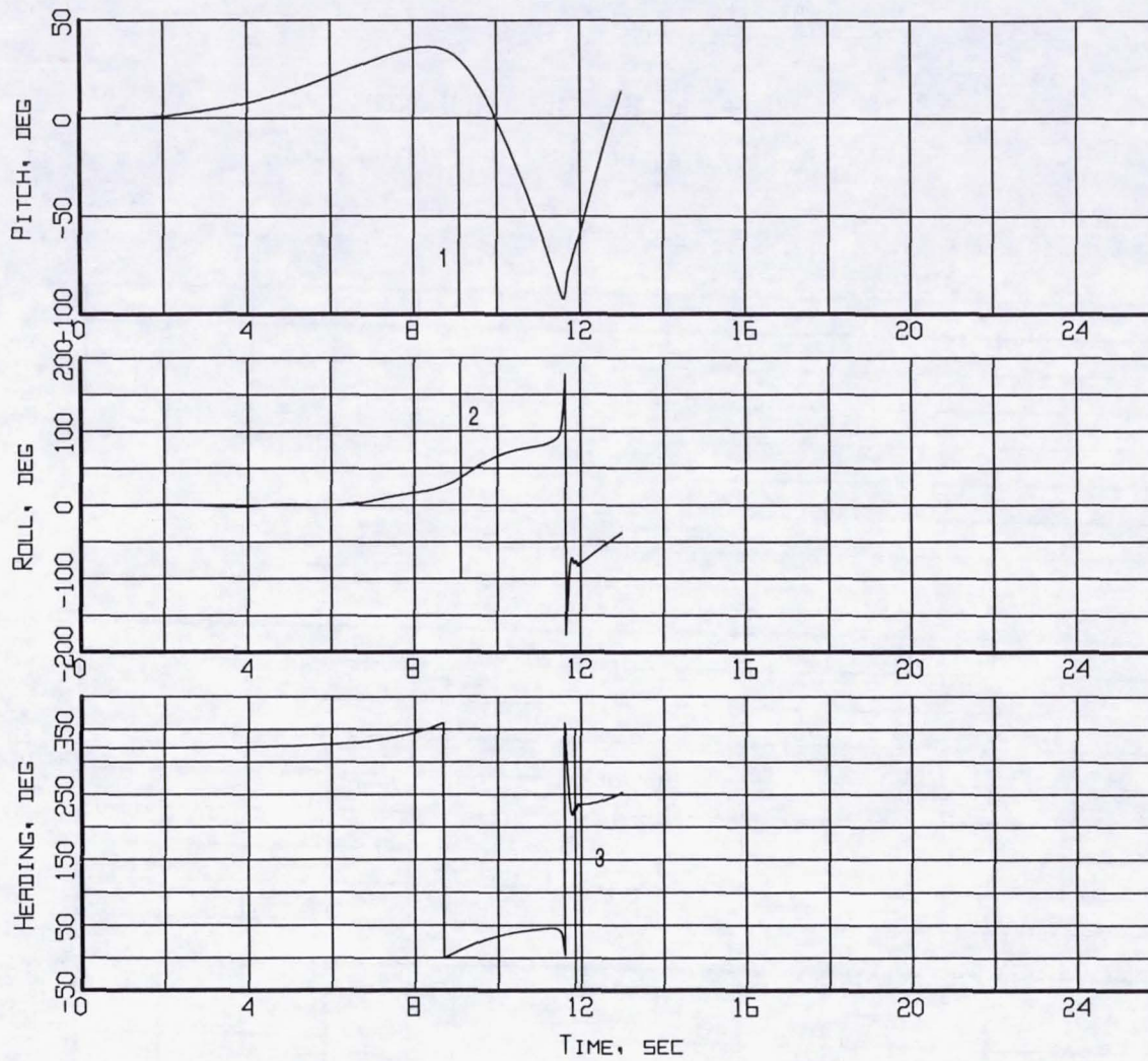
Figure B10-8. Event markers superposed on the aircraft attitude time histories (Flight 240, Test Point 43b).
