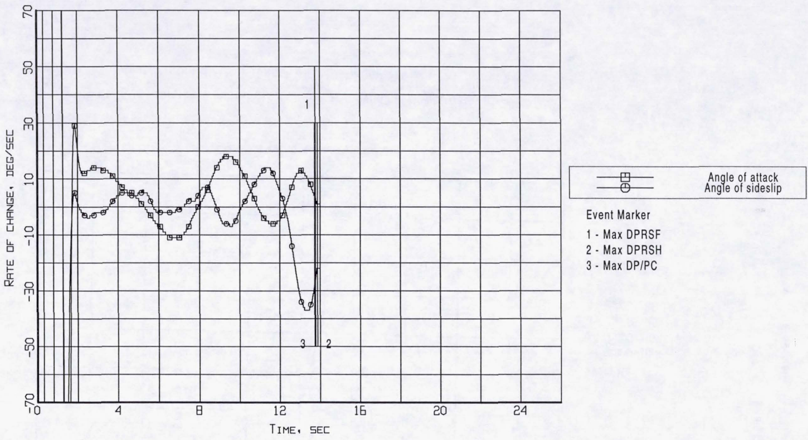
Figure B3-12. Event markers superposed on the aerodynamic flowstream descriptors rate-of-change time histories (Flight 238, Test Point 36b).
