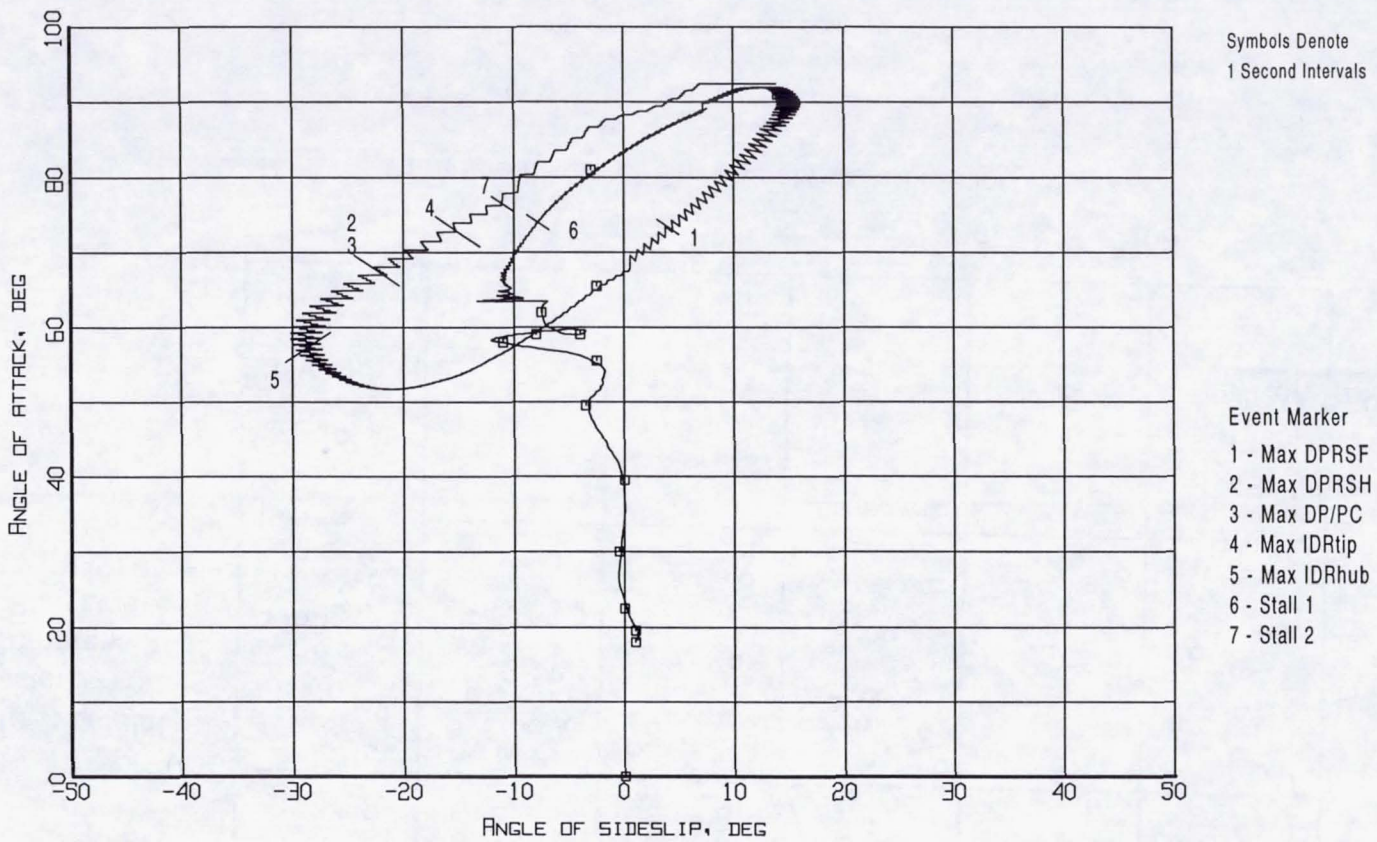
Figure 16. Event markers superposed on the aerodynamic flowstream descriptors trajectory (Flight 240, Test Point 45b).
