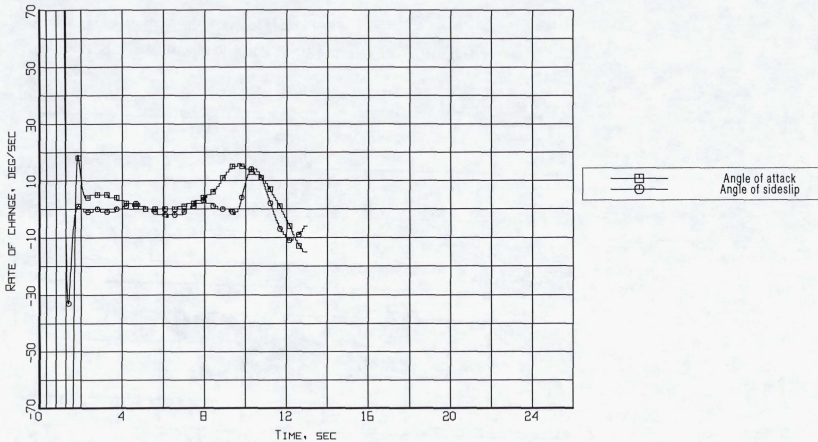
Figure B1-4. Aerodynamic flowstream descriptors - rate of change of angle of attack and angle of sideslip (Flight 239, Test Point 34b).
