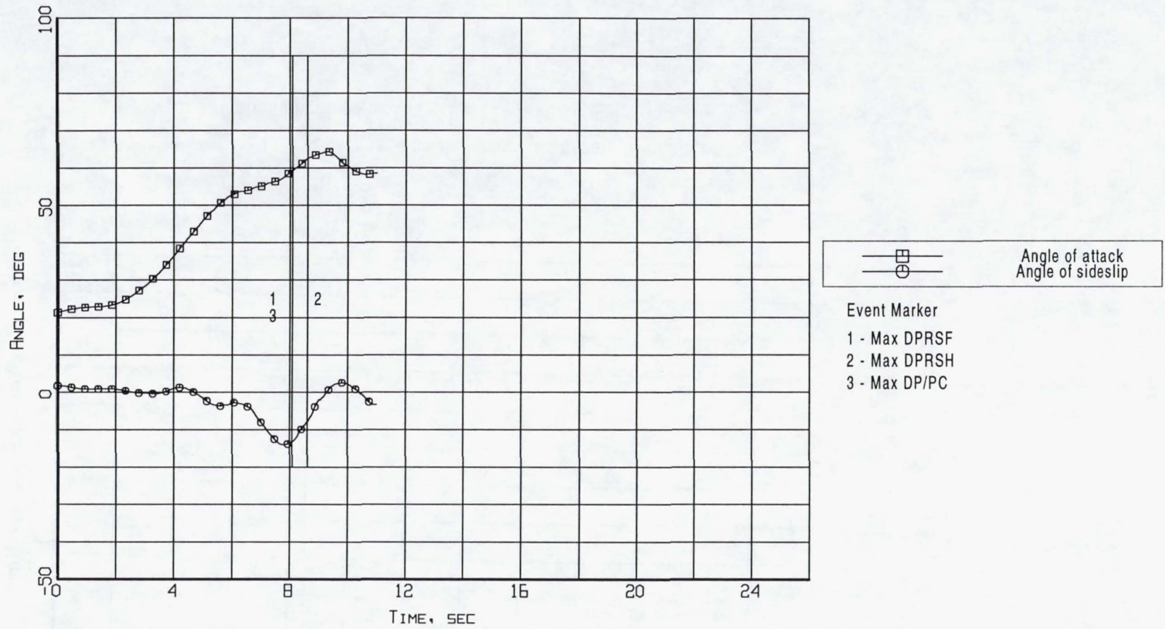
Figure B8-11. Event markers superposed on the aerodynamic flowstream descriptor time histories (Flight 240, Test Point 41b).
