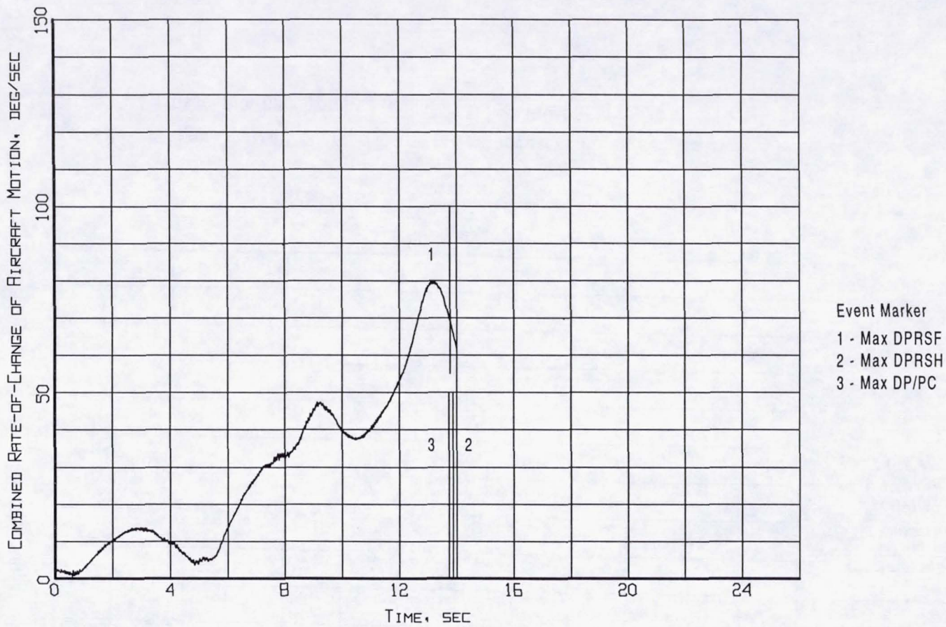
Figure B3-10. Event markers superposed on the combined of rate-of-change of aircraft motion time history (Flight 238, Test Point 36b).
