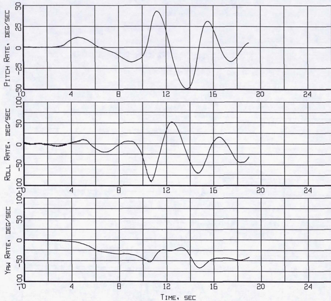
Figure B4-2. Aircraft Motion - Rate-of-Change of Pitch, Roll and Heading (Flight 239, Test Point 37b).
