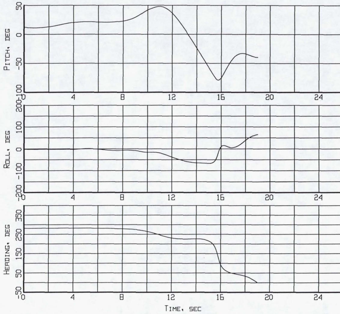
Figure B1-1. Aircraft attitude - Pitch, Roll, and Heading (Flight 239, Test Point 34b).
