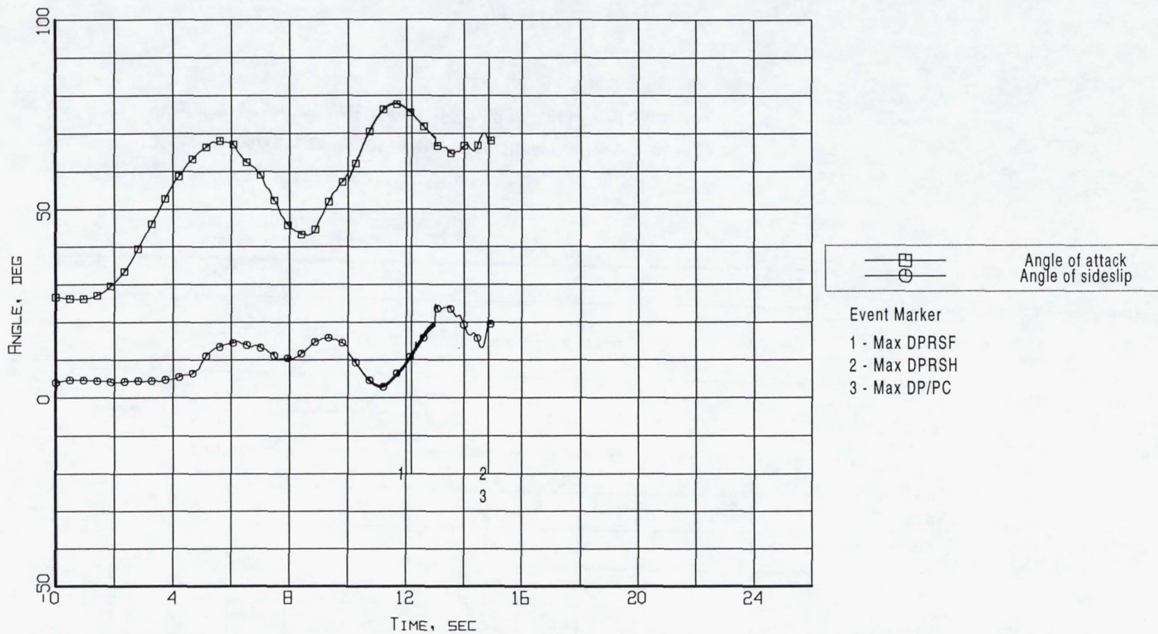
Figure B2-11. Event markers superposed on the aerodynamic flowstream descriptor time histories (Flight 238, Test Point 35b).
