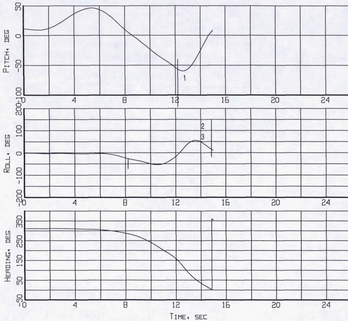
Figure B2-8. Event markers superposed on the aircraft attitude time histories (Flight 238, Test Point 35b).
