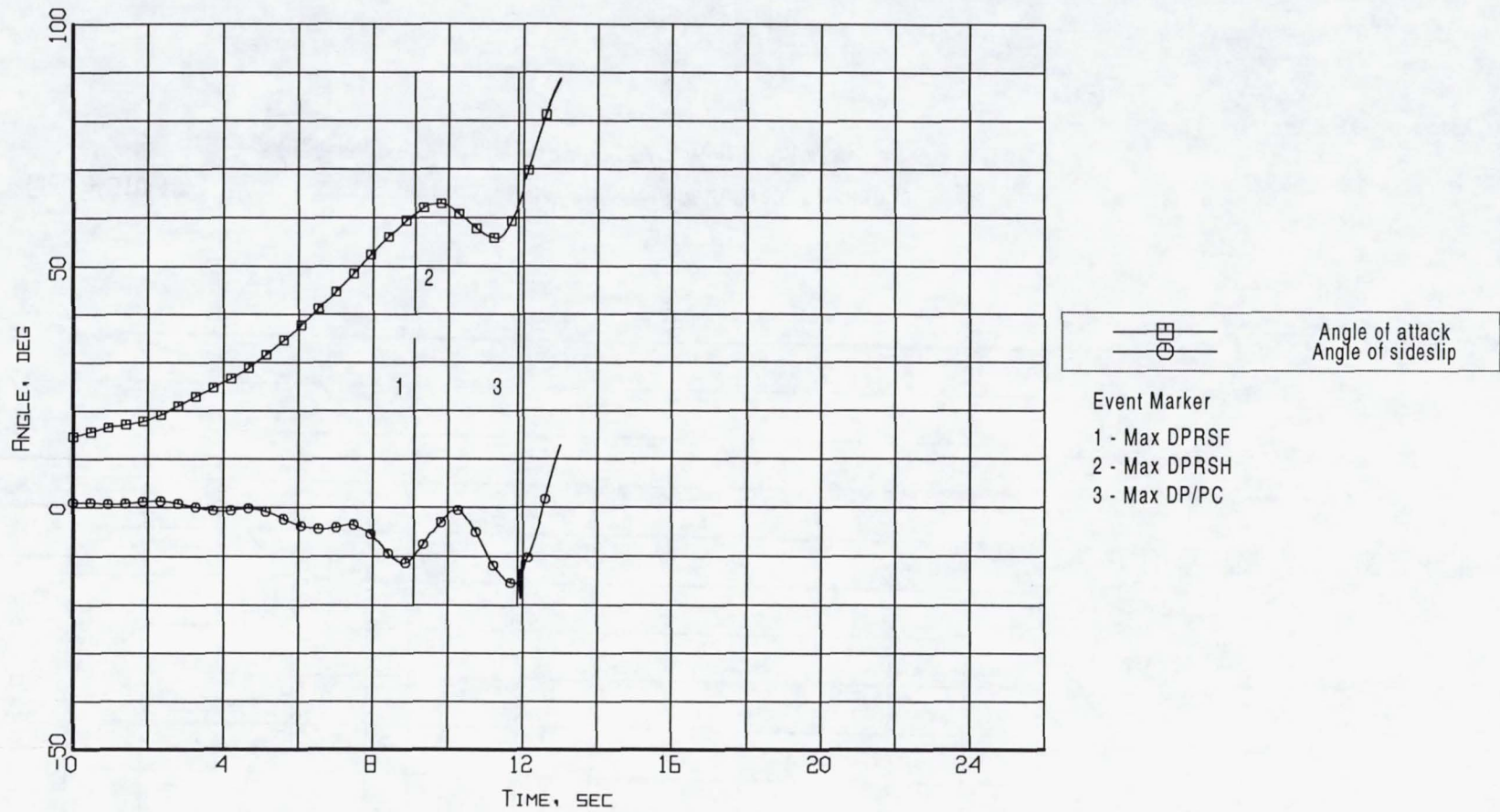
Figure B10-11. Event markers superposed on the aerodynamic flowstream descriptor time histories (Flight 240, Test Point 43b).
