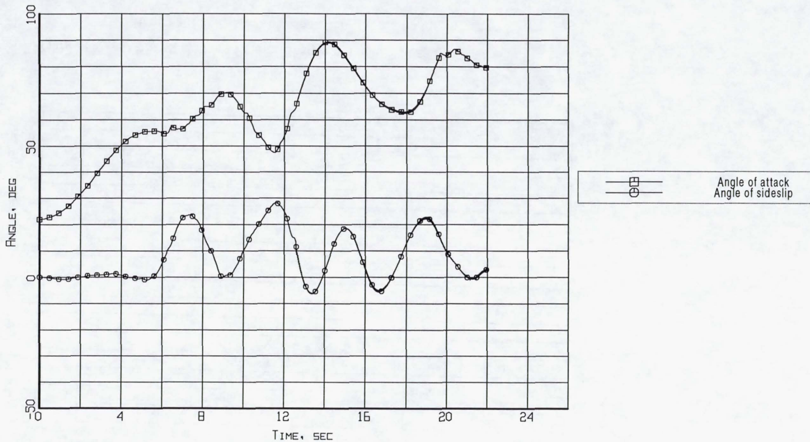
Figure B5-3. Aerodynamic flowstream descriptors - angle of attack and angle of sideslip (Flight 238, Test Point 38b).
