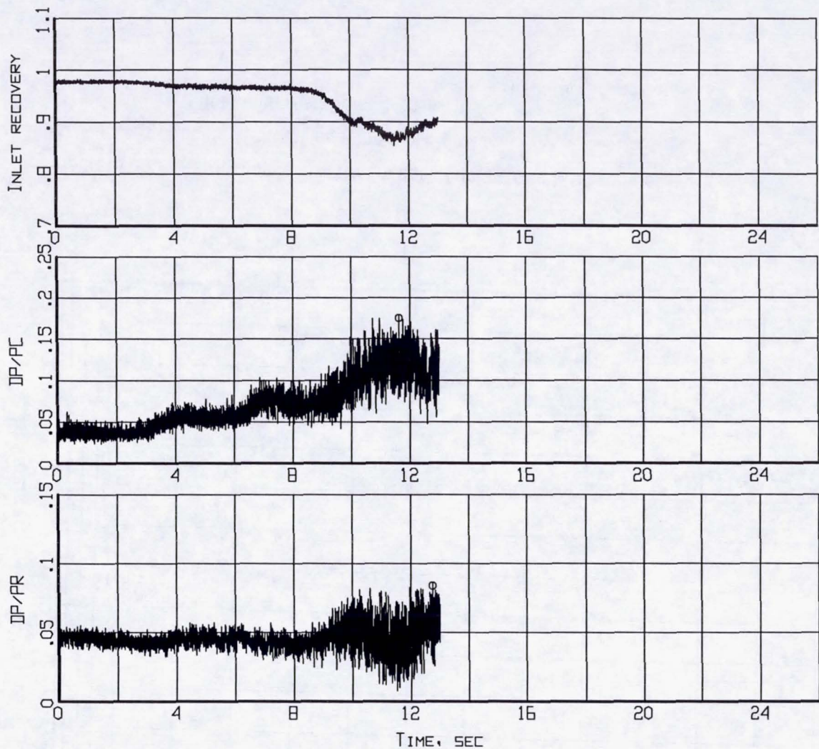
Figure B1-5. Time histories of inlet recovery and distortion descriptors (Flight 239, Test Point 34b).
