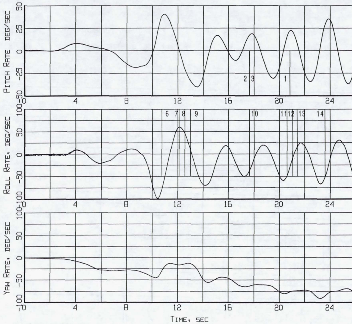
Figure B6-9. Event markers superposed on the aircraft motion time histories (Flight 239, Test Point 39b).
