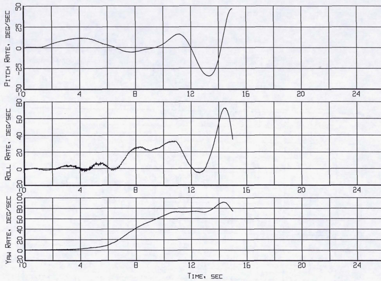
Figure 4. Aircraft Motion - Rate-of-Change of Pitch, Roll and Heading (Flight 240, Test Point 45b).
