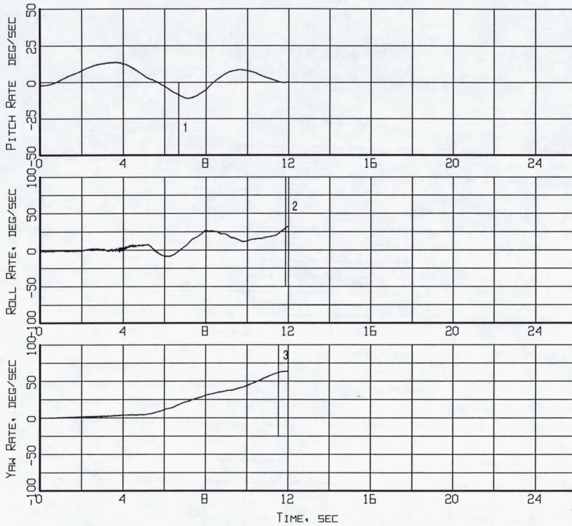
Figure B9-9. Event markers superposed on the aircraft motion time histories (Flight 238, Test Point 42b).
