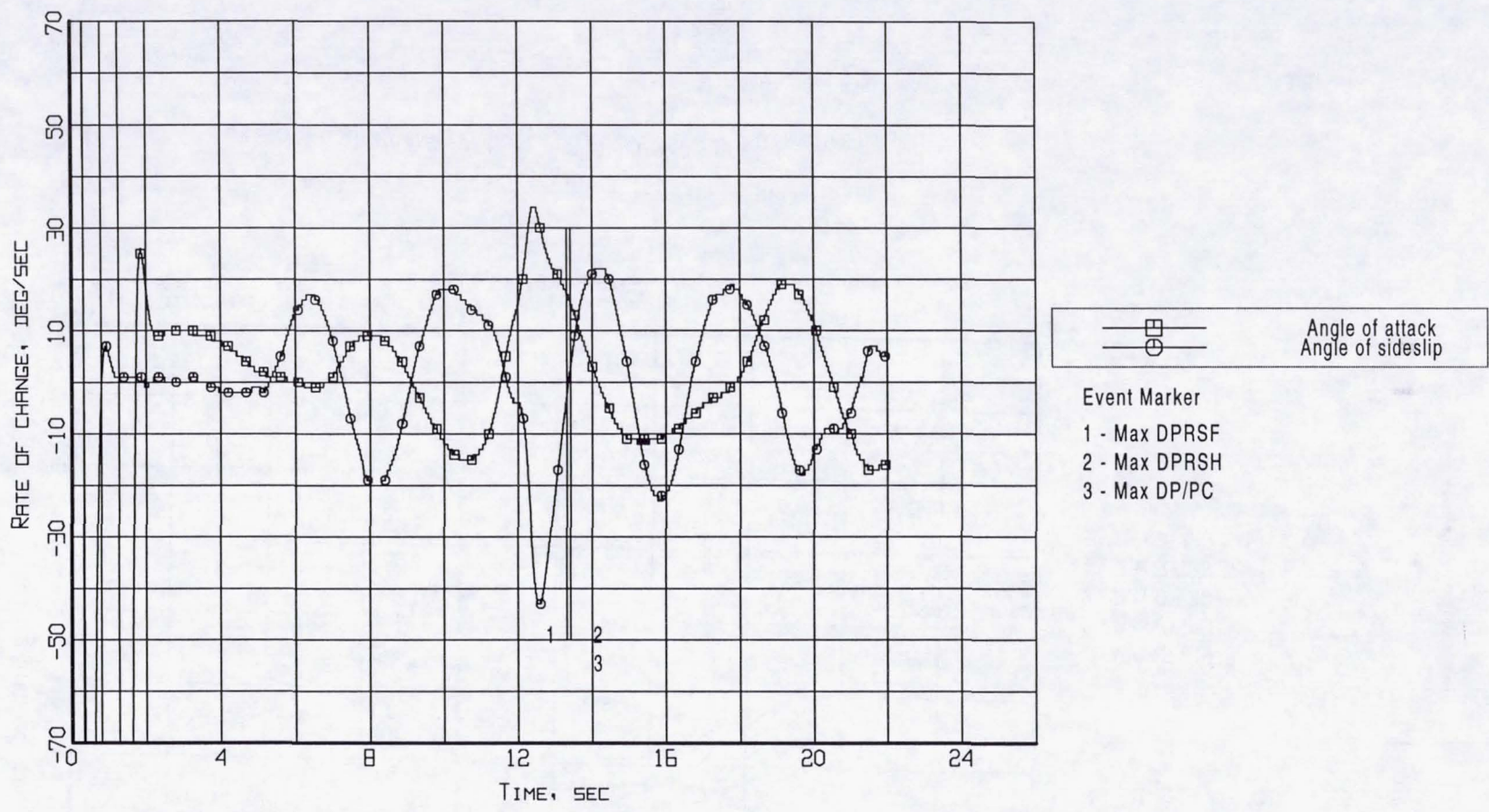
Figure B5-12. Event markers superposed on the aerodynamic flowstream descriptors rate-of-change time histories (Flight 238, Test Point 38b).
