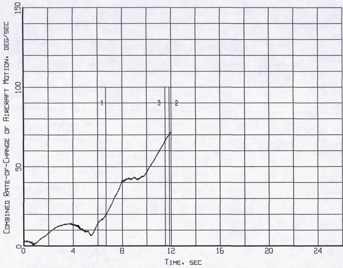
Figure B9-10. Event markers superposed on the combined of rate-of-change of aircraft motion time history (Flight 238, Test Point 42b).
