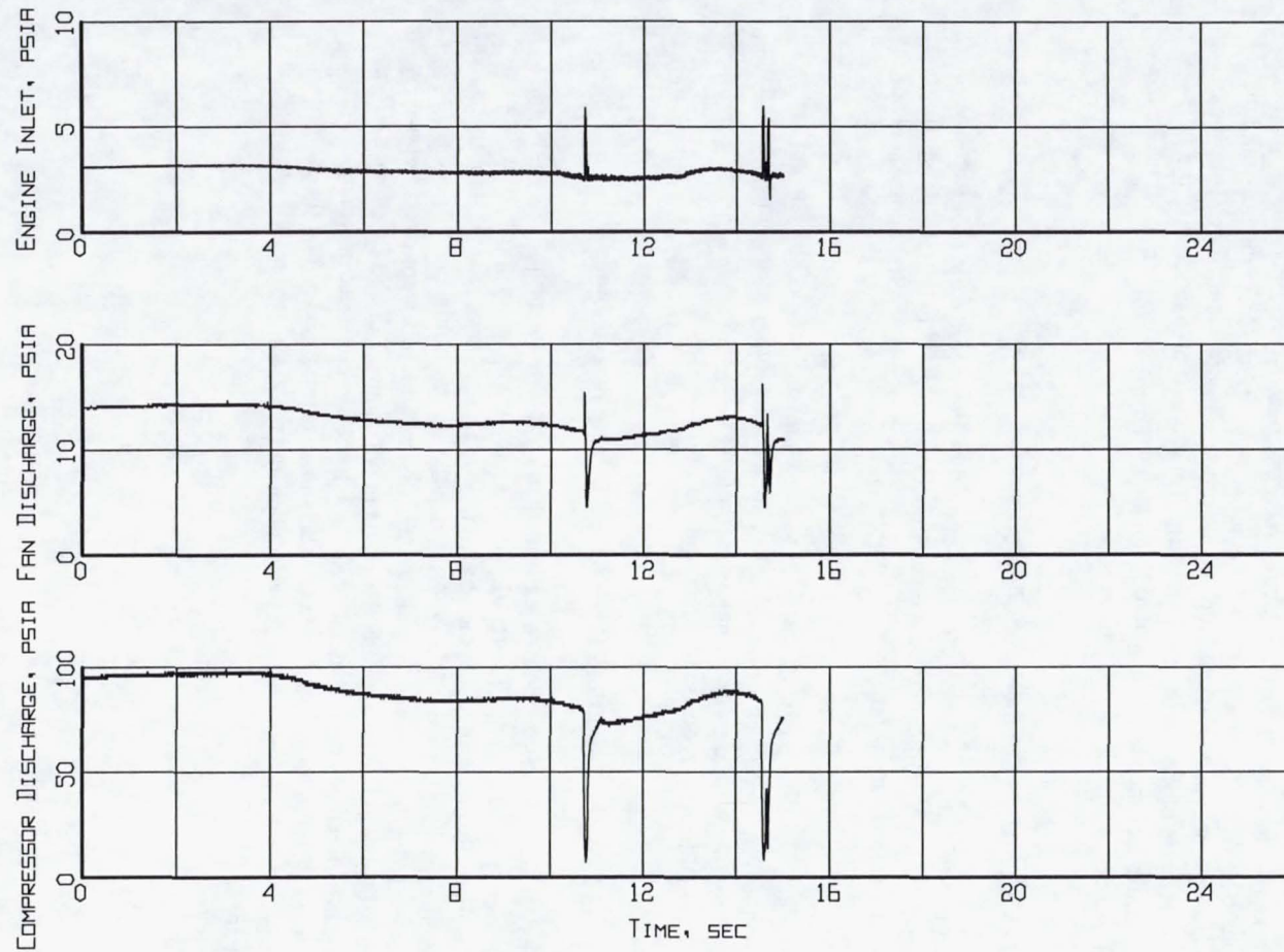
Figure 9. Measured inlet/engine entry and engine internal pressures time histories (Flight 240, Test Point 45b).
