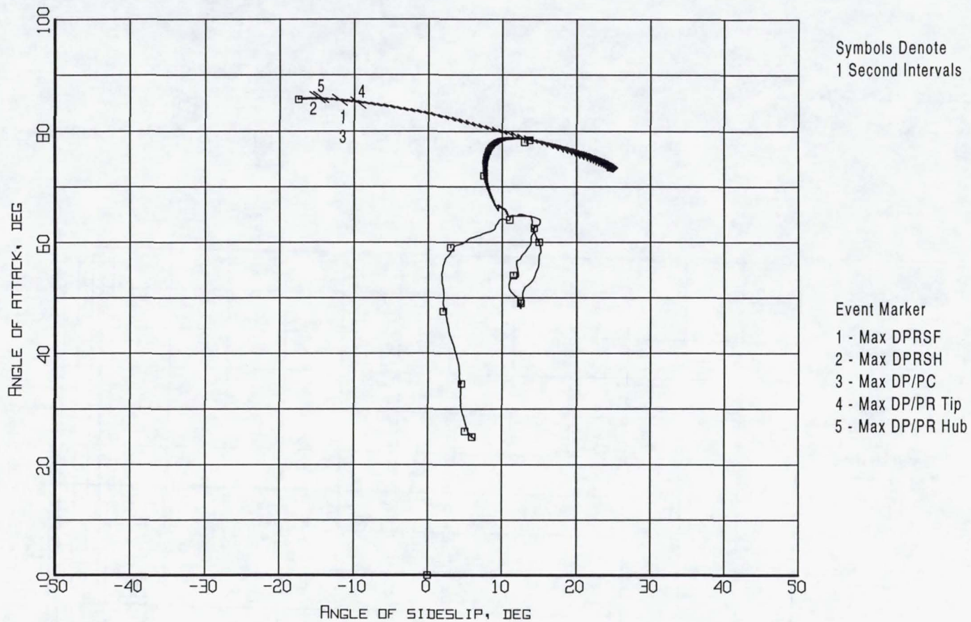
Figure B3-13. Event markers superposed on the aerodynamic flowstream descriptors trajectory (Flight 238, Test Point 36b).
