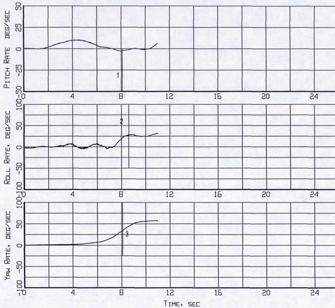
Figure B8-9. Event markers superposed on the aircraft motion time histories (Flight 240, Test Point 41b).
