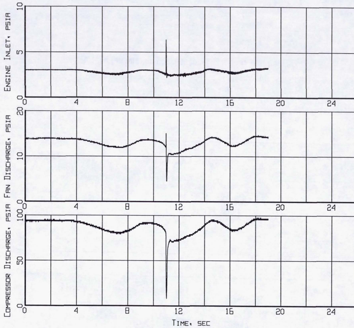
Figure B4-6. Measured inlet/engine entry and engine internal pressures time histories (Flight 239, Test Point 37b).
