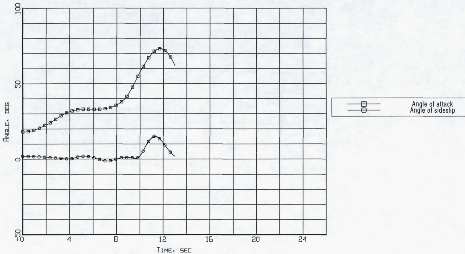
Figure B1-3. Aerodynamic flowstream descriptors - angle of attack and angle of sideslip (Flight 239, Test Point 34b).
