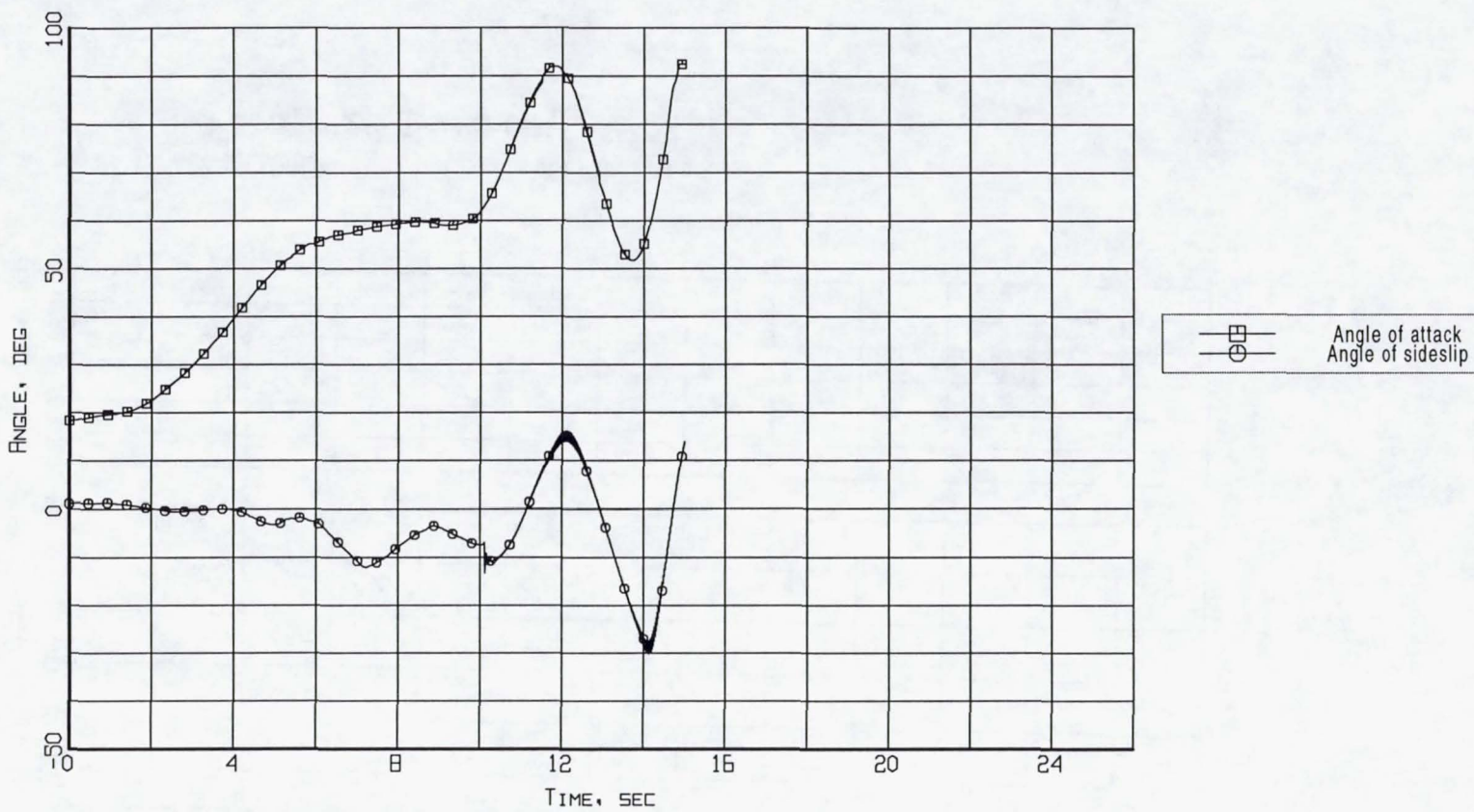
Figure 5. Aerodynamic flowstream descriptors - angle of attack and angle of sideslip (Flight 240, Test Point 45b).
