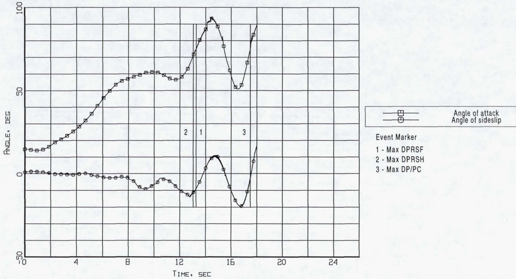
Figure B11-11. Event markers superposed on the aerodynamic flowstream descriptor time histories (Flight 238, Test Point 44b).
