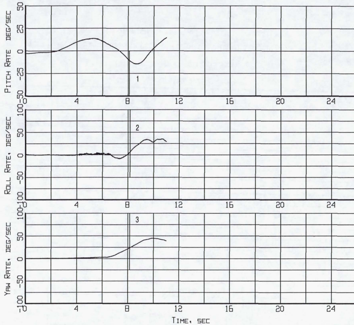
Figure B7-9. Event markers superposed on the aircraft motion time histories (Flight 238, Test Point 40b).
