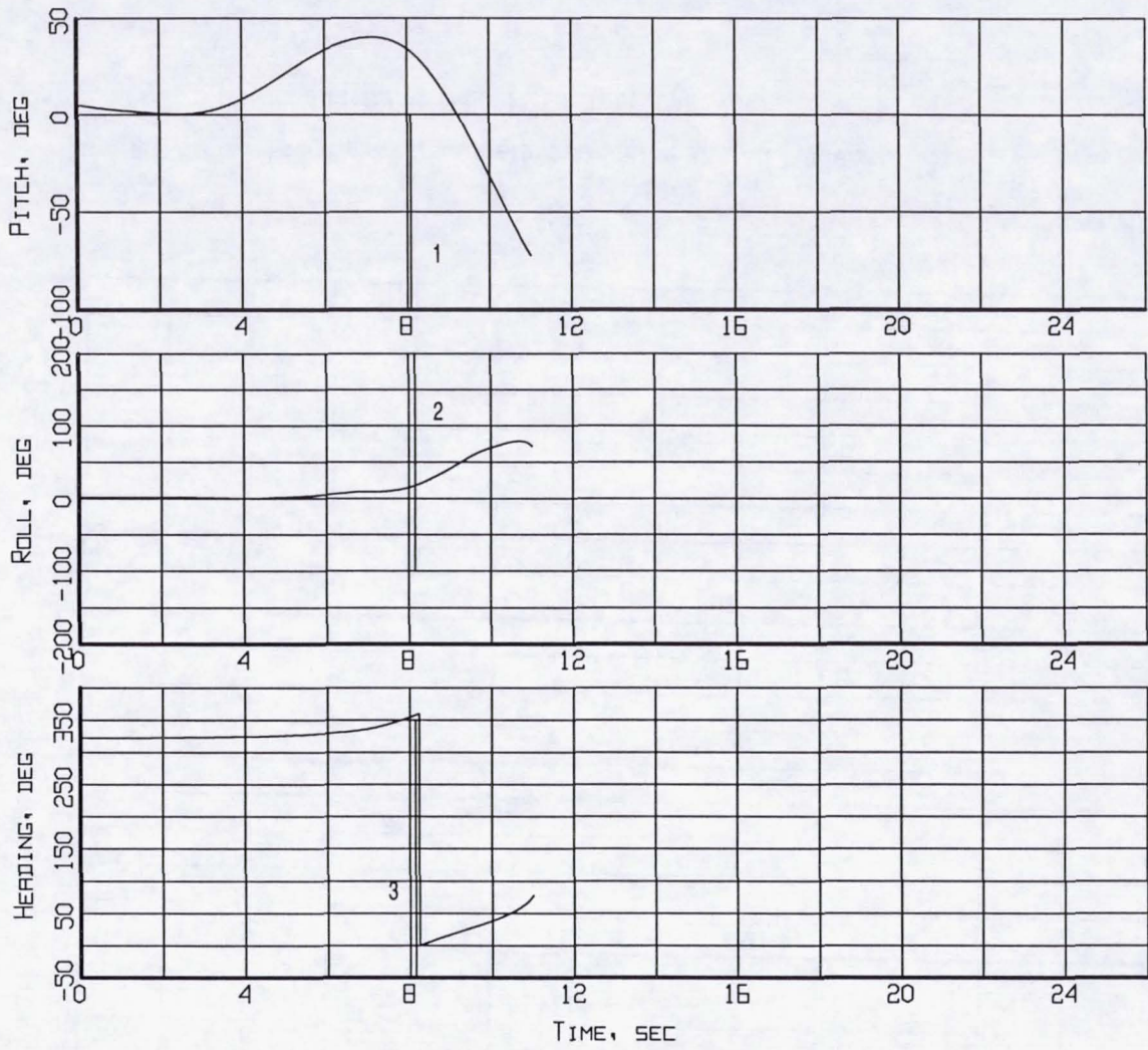
Figure B7-8. Event markers superposed on the aircraft attitude time histories (Flight 238, Test Point 40b).
