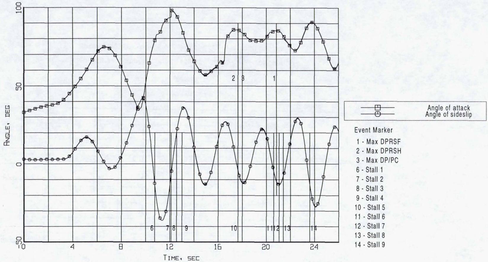
Figure B6-11. Event markers superposed on the aerodynamic flowstream descriptor time histories (Flight 239, Test Point 39b).
