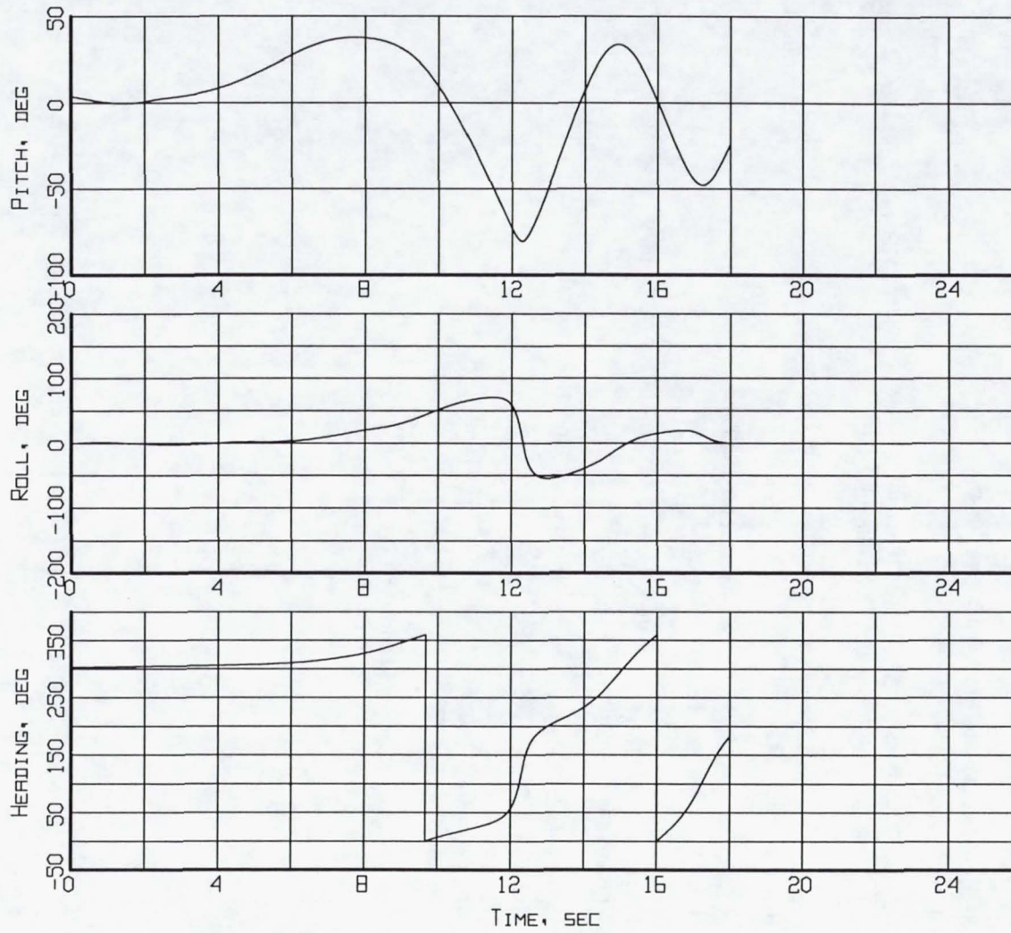
Figure B11-1. Aircraft attitude - Pitch, Roll, and Heading (Flight 238, Test Point 44b).
