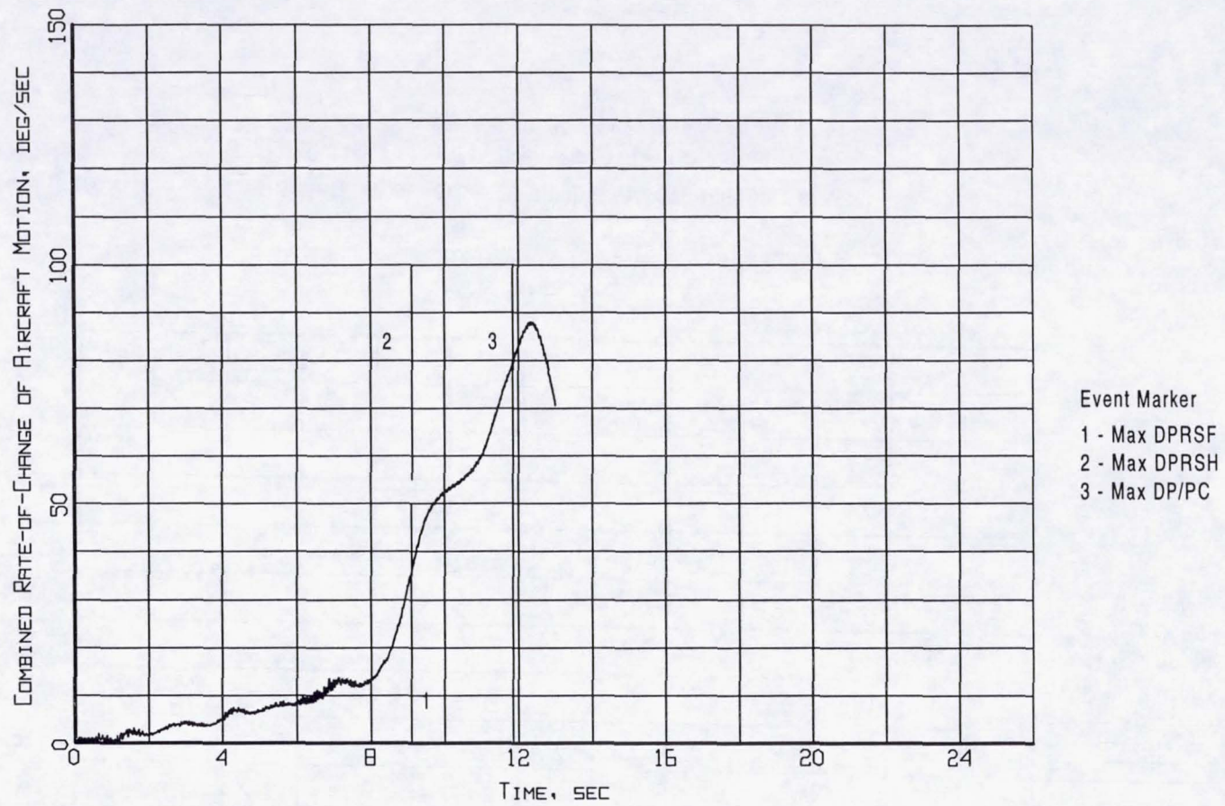
Figure B10-10. Event markers superposed on the combined of rate-of-change of aircraft motion time history (Flight 240, Test Point 43b).
