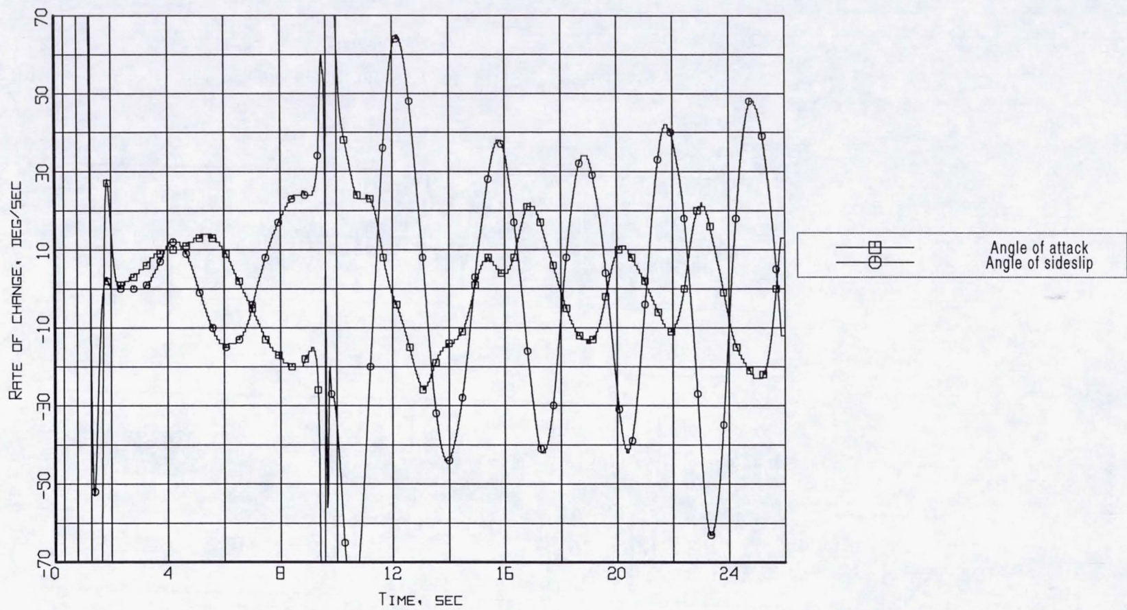
Figure B6-4. Aerodynamic flowstream descriptors - rate of change of angle of attack and angle of sideslip (Flight 239, Test Point 39b).
