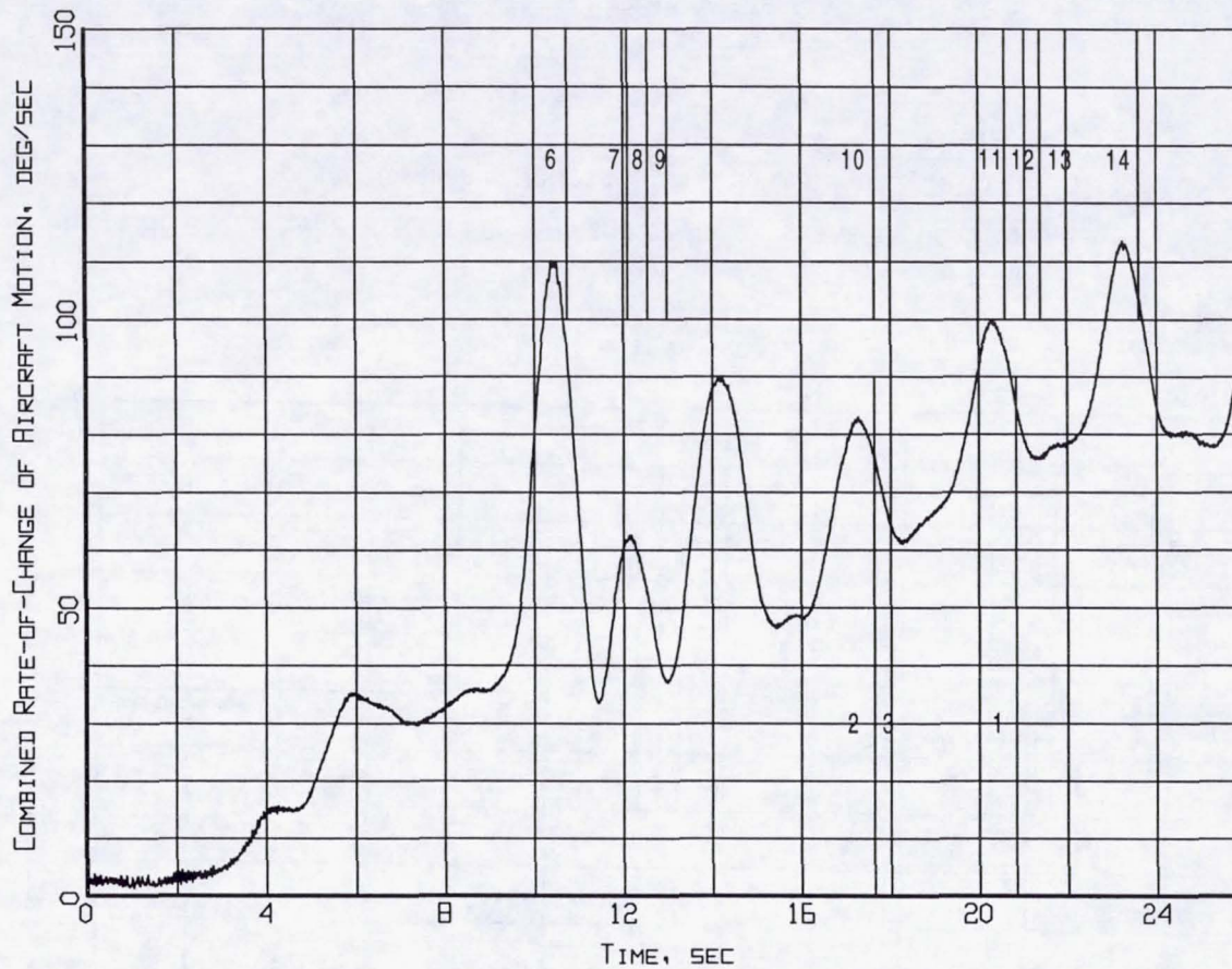
Figure B6-10. Event markers superposed on the combined of rate-of-change of aircraft motion time history (Flight 239, Test Point 39b).
