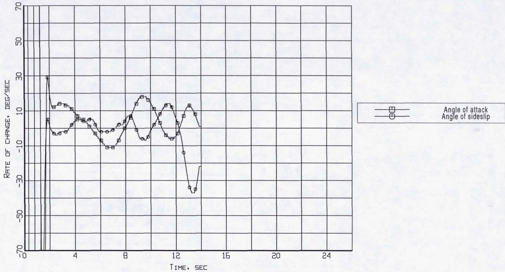
Figure B3-4. Aerodynamic flowstream descriptors - rate of change of angle of attack and angle of sideslip (Flight 238, Test Point 36b).
