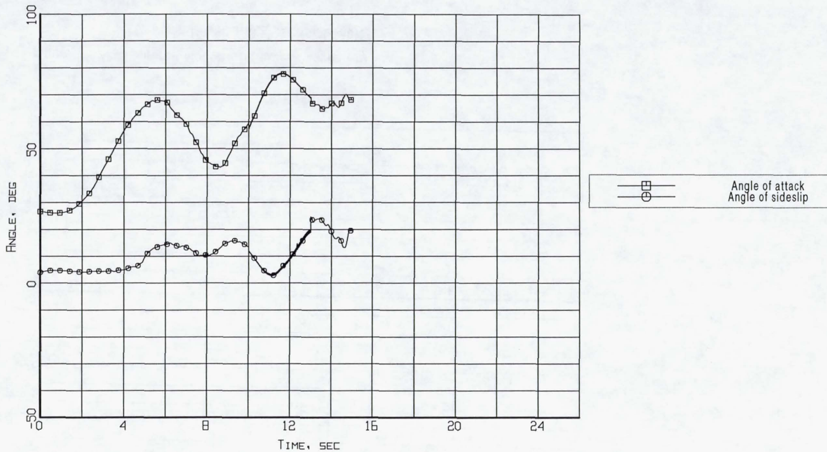
Figure B2-3. Aerodynamic flowstream descriptors - angle of attack and angle of sideslip (Flight 238, Test Point 35b).
