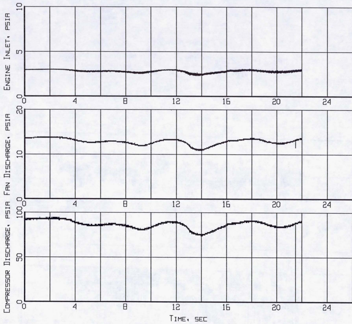
Figure B5-6. Measured inlet/engine entry and engine internal pressures time histories (Flight 238, Test Point 38b).
