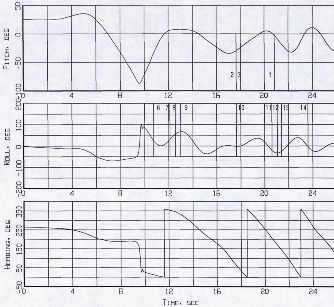
Figure B6-8. Event markers superposed on the aircraft attitude time histories (Flight 239, Test Point 39b).
