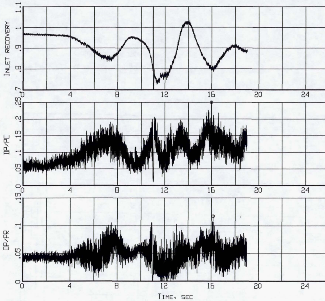
Figure B4-5. Time histories of inlet recovery and distortion descriptors (Flight 239, Test Point 37b).
