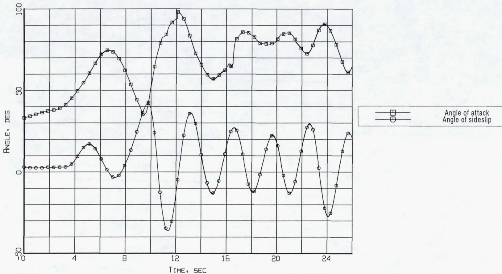
Figure B6-3. Aerodynamic flowstream descriptors - angle of attack and angle of sideslip (Flight 239, Test Point 39b).
