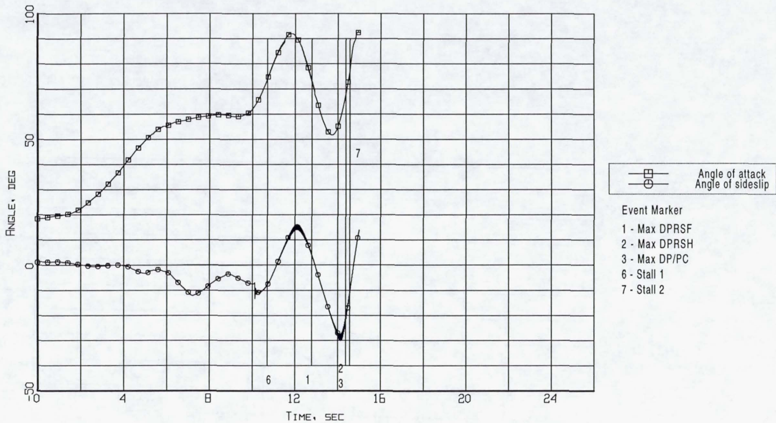
Figure 14. Event markers superposed on the angle-of-attack and angle-of-sideslip time histories (Flight 240, Test Point 45b).
