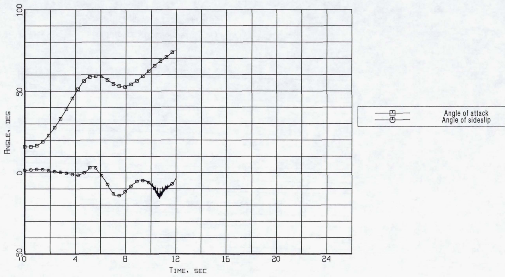
Figure B9-3. Aerodynamic flowstream descriptors - angle of attack and angle of sideslip (Flight 238, Test Point 42b).
