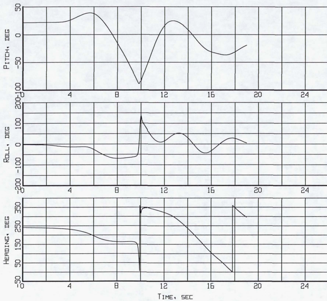
Figure B4-1. Aircraft attitude - Pitch, Roll, and Heading (Flight 239, Test Point 37b).
