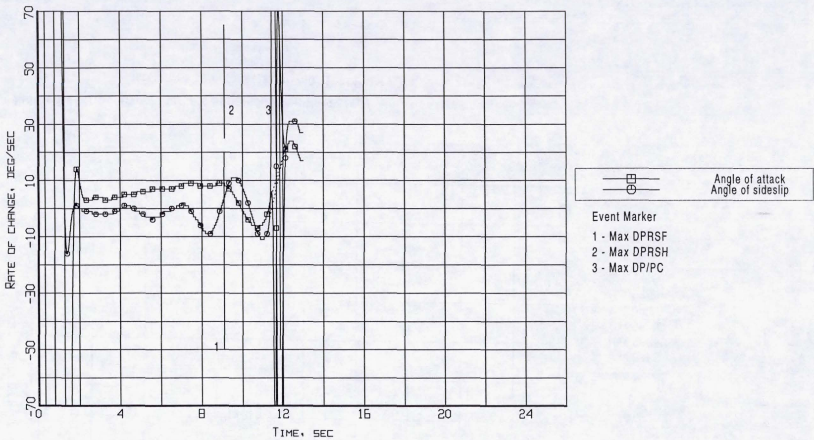
Figure B10-12. Event markers superposed on the aerodynamic flowstream descriptors rate-of-change time histories (Flight 240, Test Point 43b).
