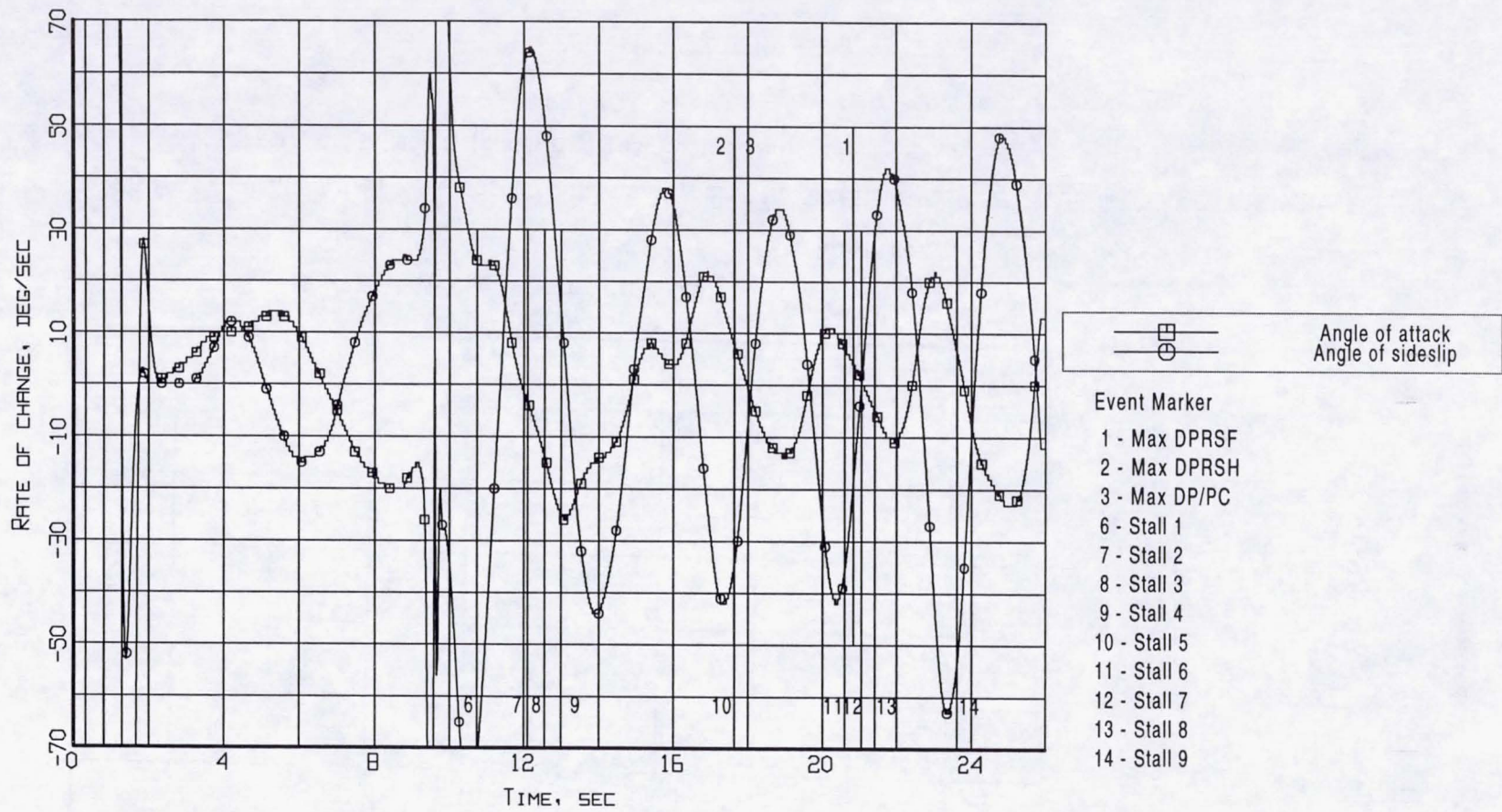
Figure B6-12. Event markers superposed on the aerodynamic flowstream descriptors rate-of-change time histories (Flight 239, Test Point 39b).
