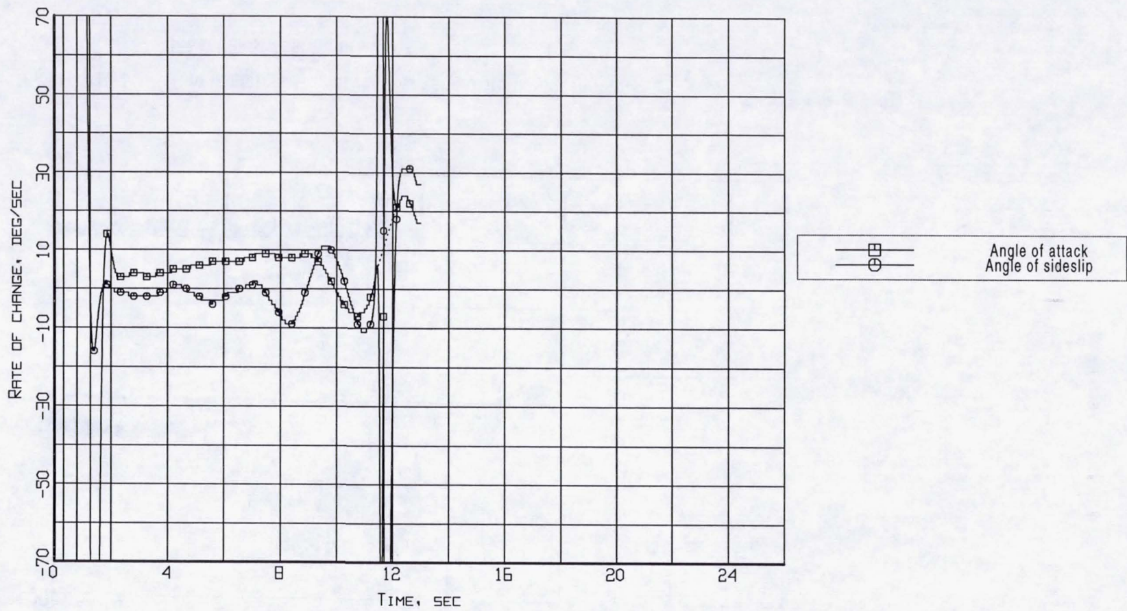
Figure B10-4. Aerodynamic flowstream descriptors - rate of change of angle of attack and angle of sideslip (Flight 240, Test Point 43b).
