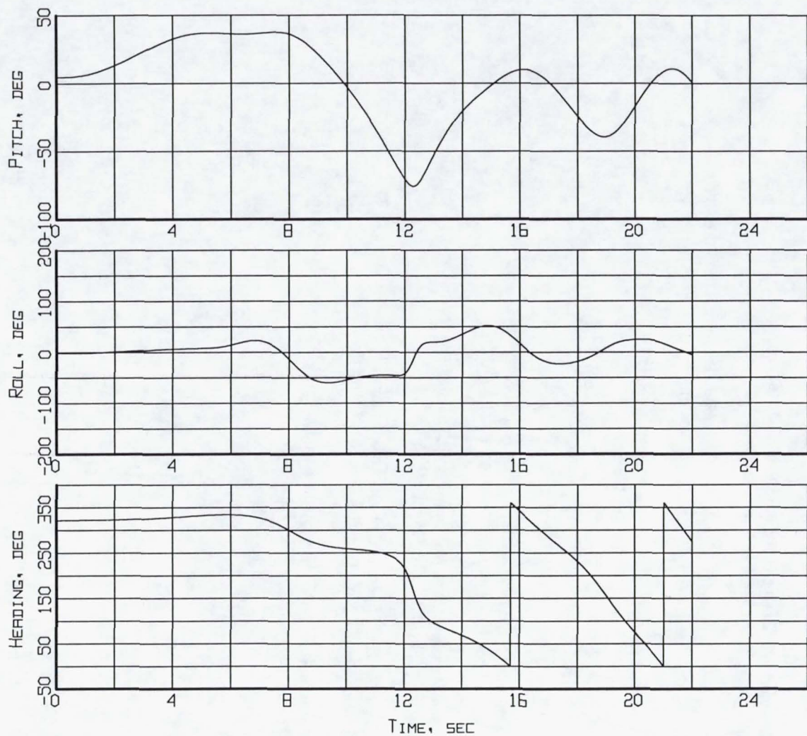
Figure B5-1. Aircraft attitude - Pitch, Roll, and Heading (Flight 238, Test Point 38b).
