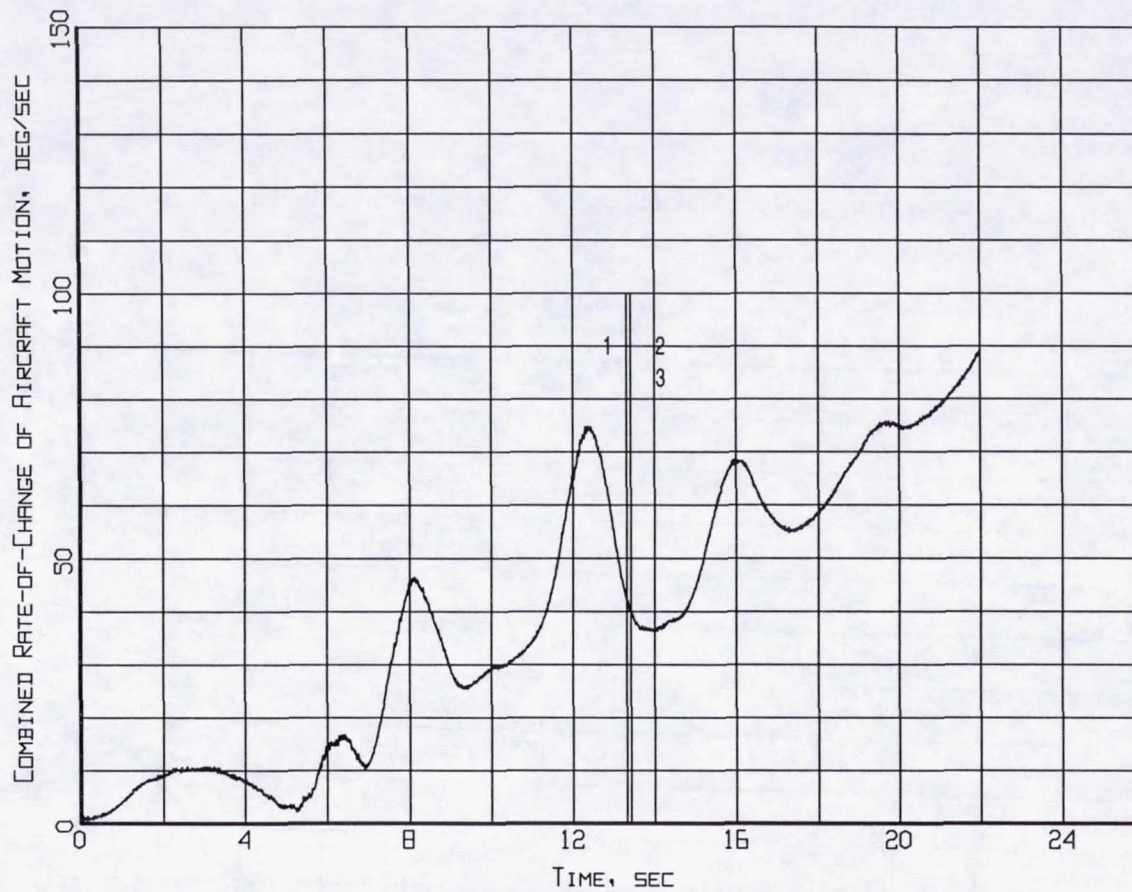
Figure B5-10. Event markers superposed on the combined of rate-of-change of aircraft motion time history (Flight 238, Test Point 38b).
