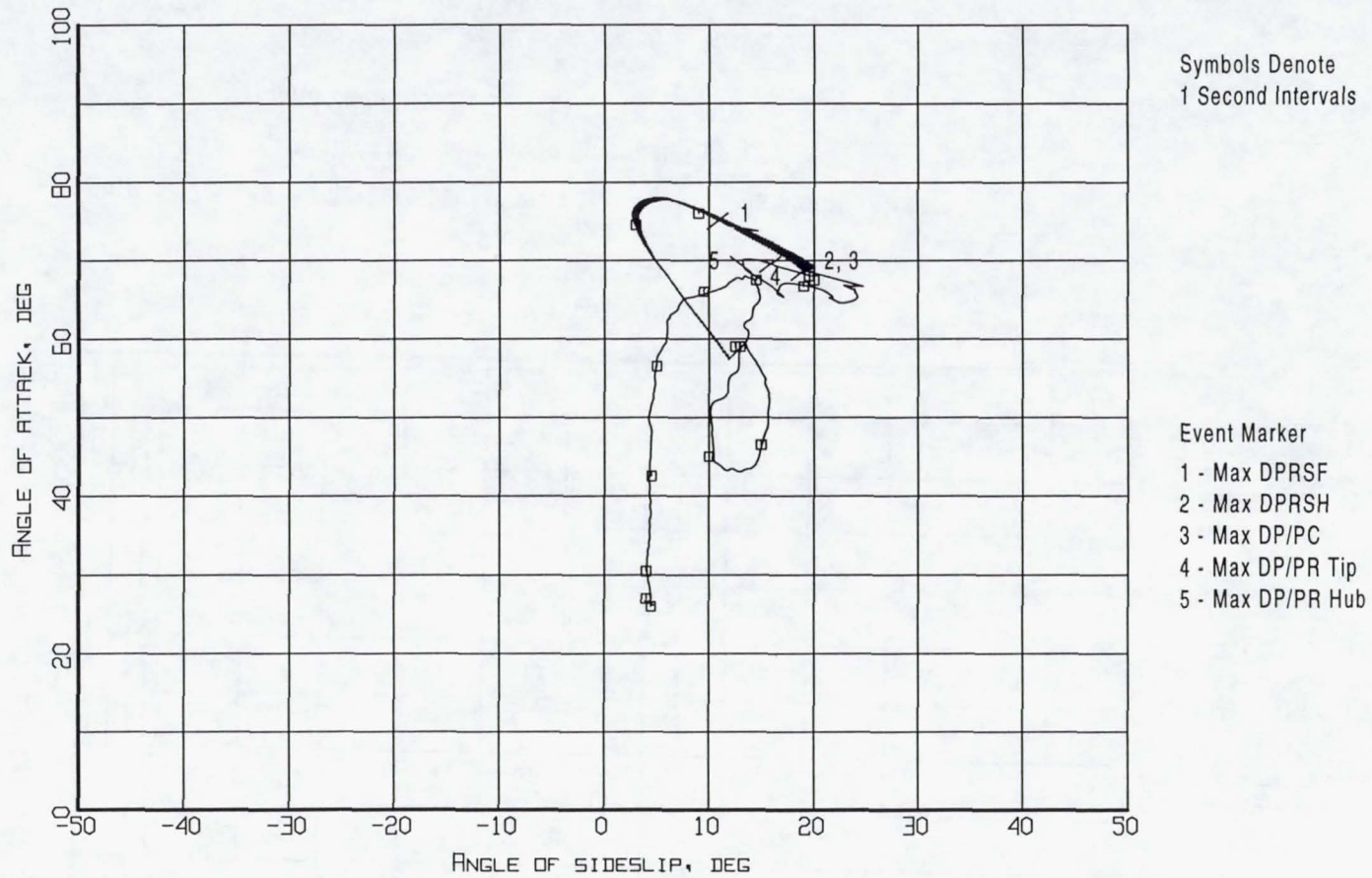
Figure B2-13. Event markers superposed on the aerodynamic flowstream descriptors trajectory (Flight 238, Test Point 35b).
