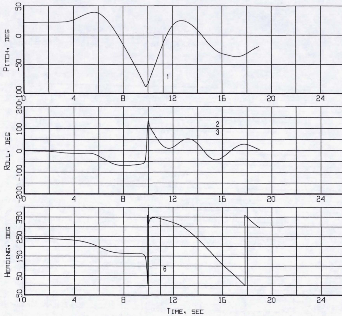
Figure B4-8. Event markers superposed on the aircraft attitude time histories (Flight 239, Test Point 37b).
