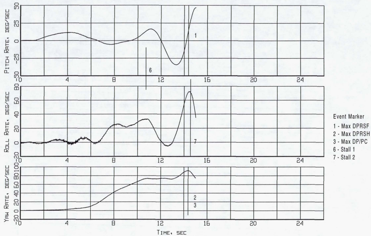
Figure 12. Event markers superposed on the aircraft motion time histories (Flight 240, Test Point 45b).
