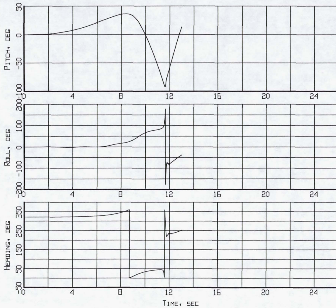
Figure B10-1. Aircraft attitude - Pitch, Roll, and Heading (Flight 240, Test Point 43b).
