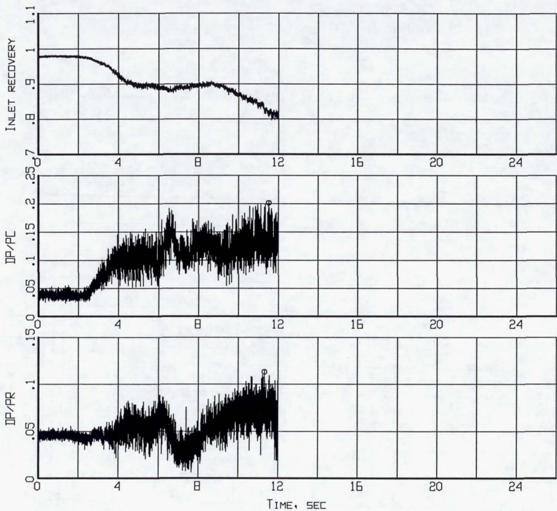
Figure B9-5. Time histories of inlet recovery and distortion descriptors (Flight 238, Test Point 42b).
