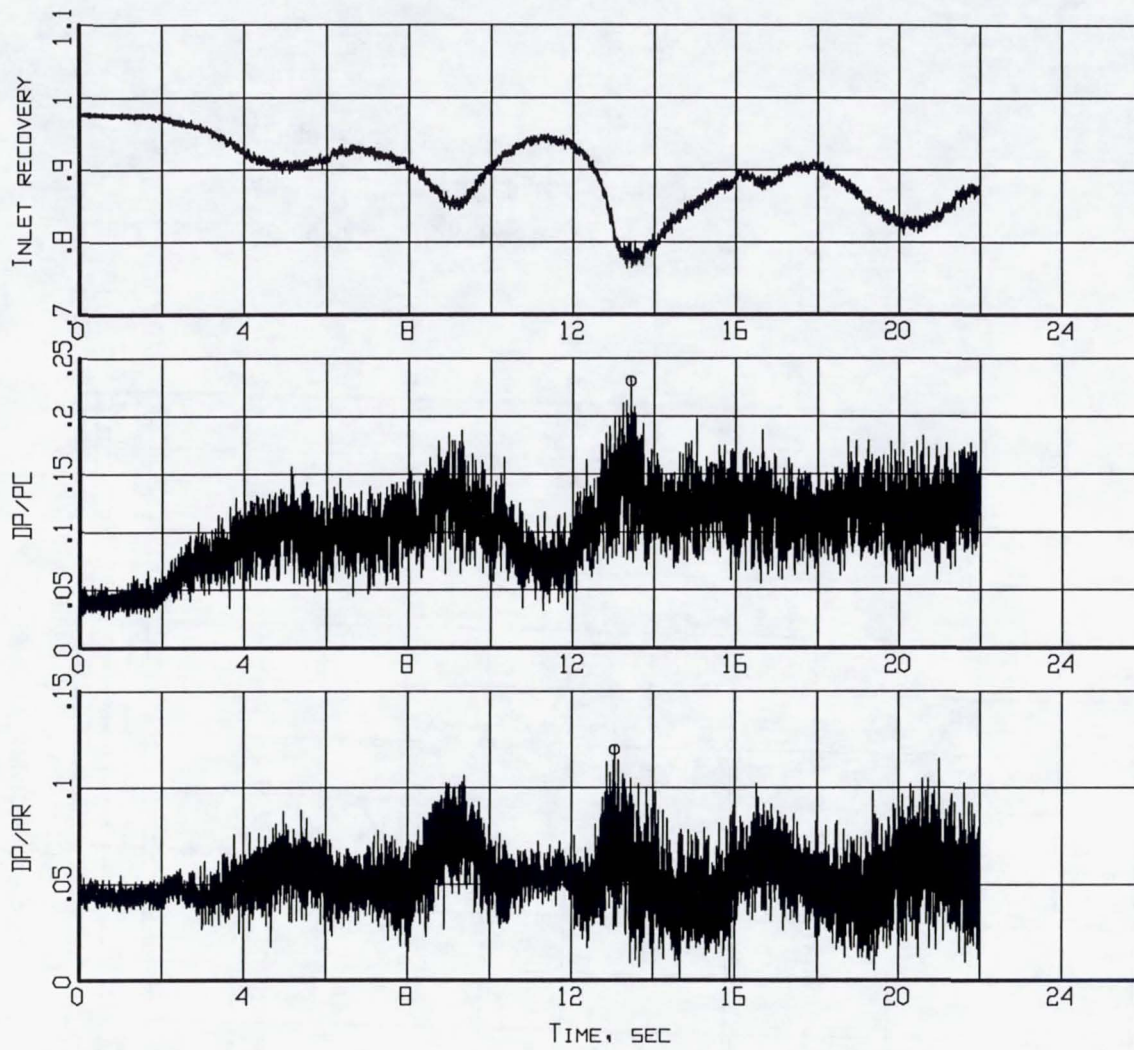
Figure B5-5. Time histories of inlet recovery and distortion descriptors (Flight 238, Test Point 38b).
