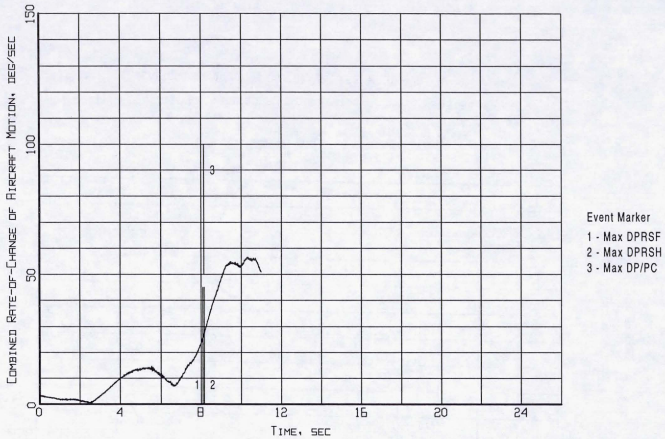
Figure B7-10. Event markers superposed on the combined of rate-of-change of aircraft motion time history (Flight 238, Test Point 40b).
