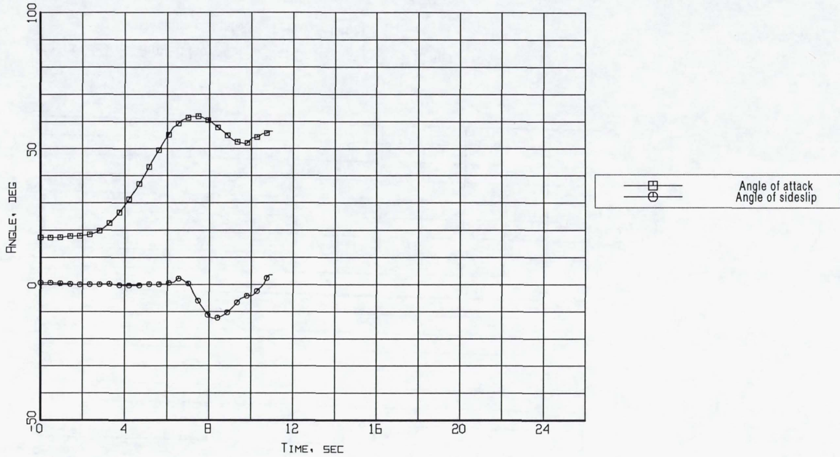
Figure B7-3. Aerodynamic flowstream descriptors - angle of attack and angle of sideslip (Flight 238, Test Point 40b).
