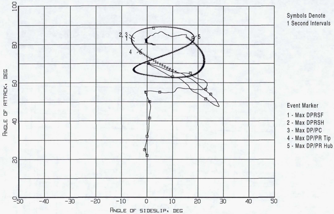
Figure B5-13. Event markers superposed on the aerodynamic flowstream descriptors trajectory (Flight 238, Test Point 38b).
