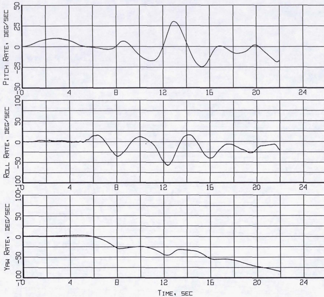
Figure B5-2. Aircraft Motion - Rate-of-Change of Pitch, Roll and Heading (Flight 238, Test Point 38b).
