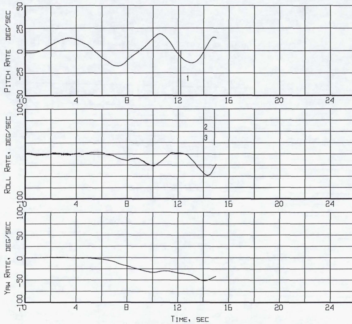
Figure B2-9. Event markers superposed on the aircraft motion time histories (Flight 238, Test Point 35b).
