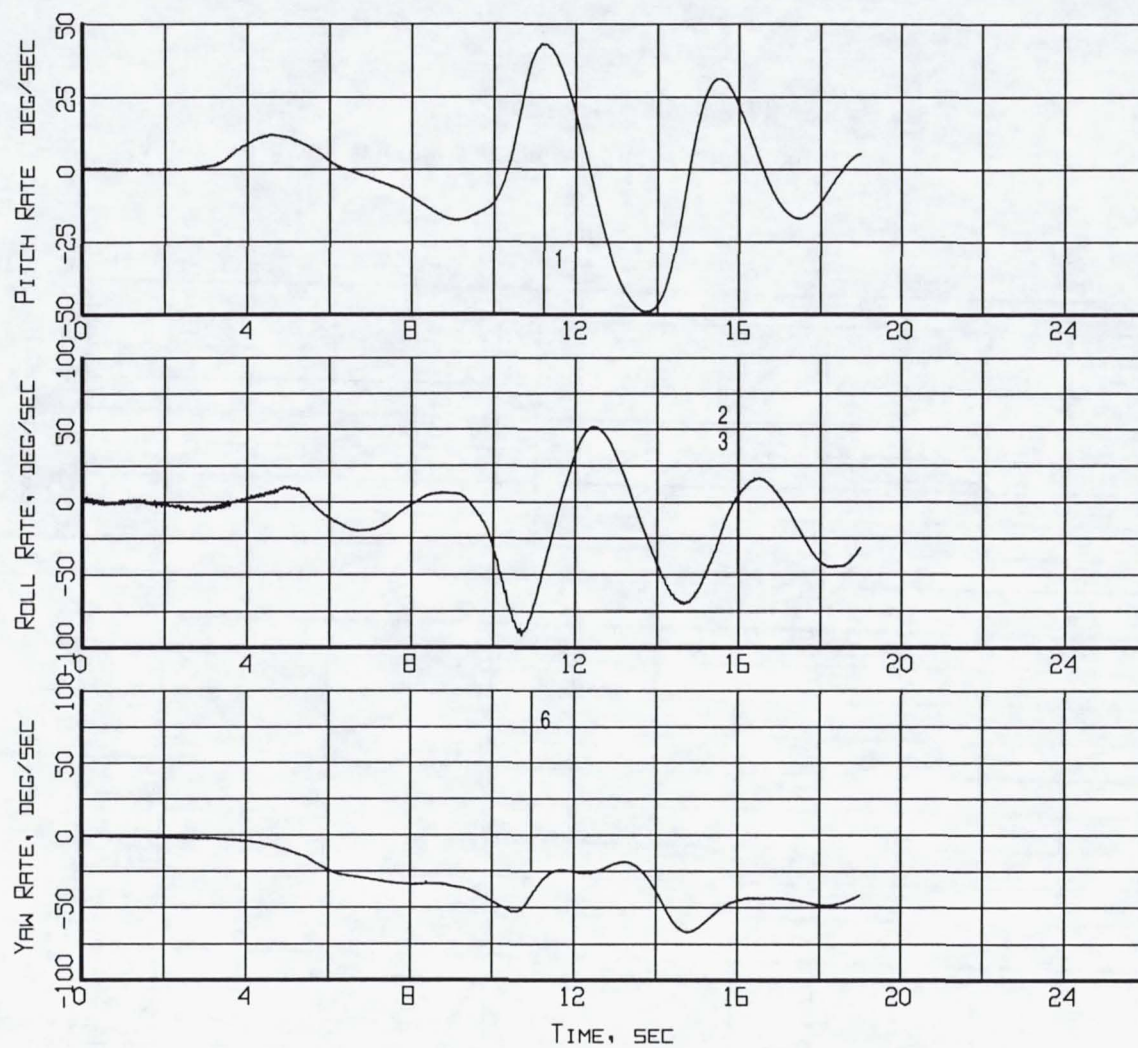
Figure B4-9. Event markers superposed on the aircraft motion time histories (Flight 239, Test Point 37b).
