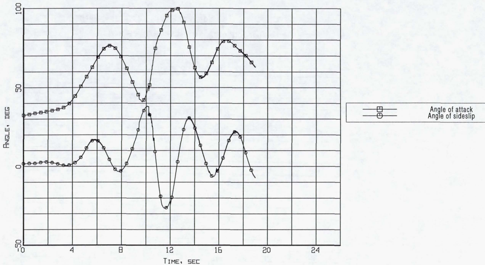
Figure B4-3. Aerodynamic flowstream descriptors - angle of attack and angle of sideslip (Flight 239, Test Point 37b).
