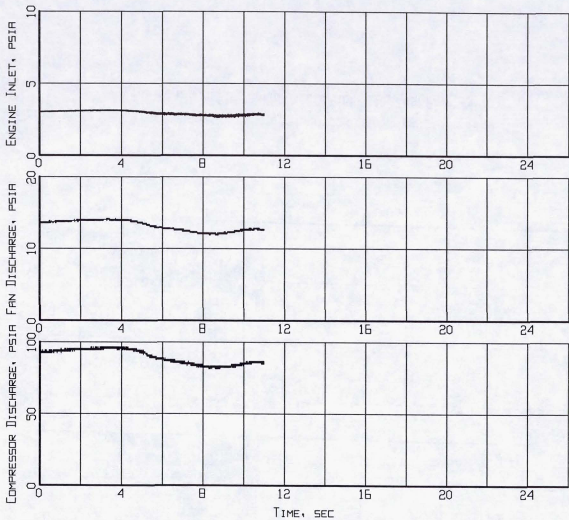
Figure B8-6. Measured inlet/engine entry and engine internal pressures time histories (Flight 240, Test Point 41b).
