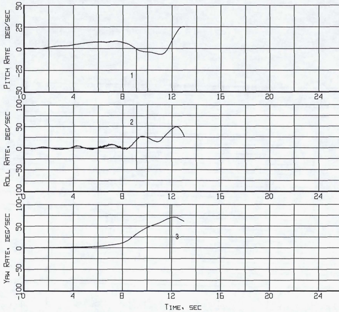
Figure B10-9. Event markers superposed on the aircraft motion time histories (Flight 240, Test Point 43b).
