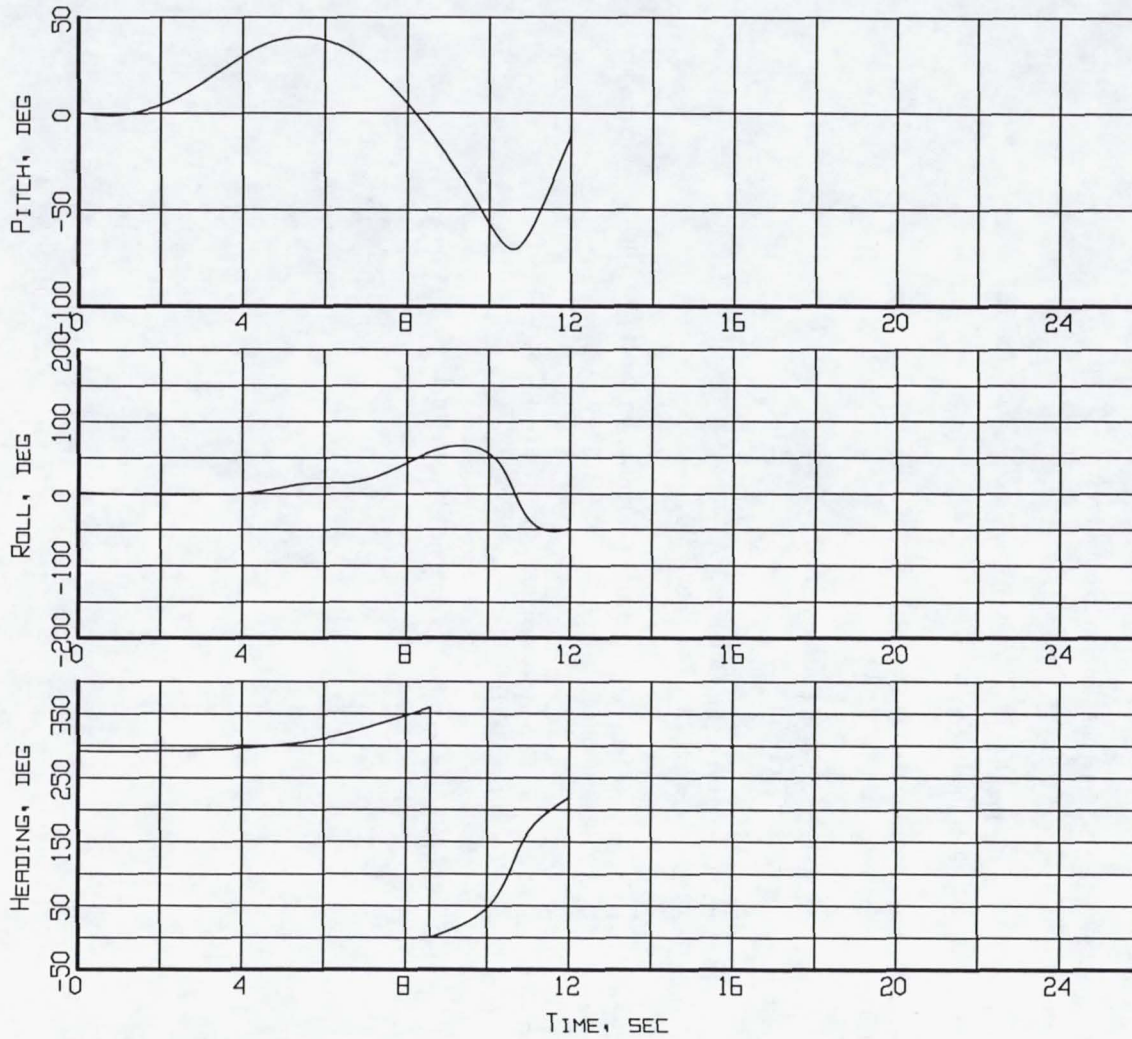
Figure B9-1. Aircraft attitude - Pitch, Roll, and Heading (Flight 238, Test Point 42b).
