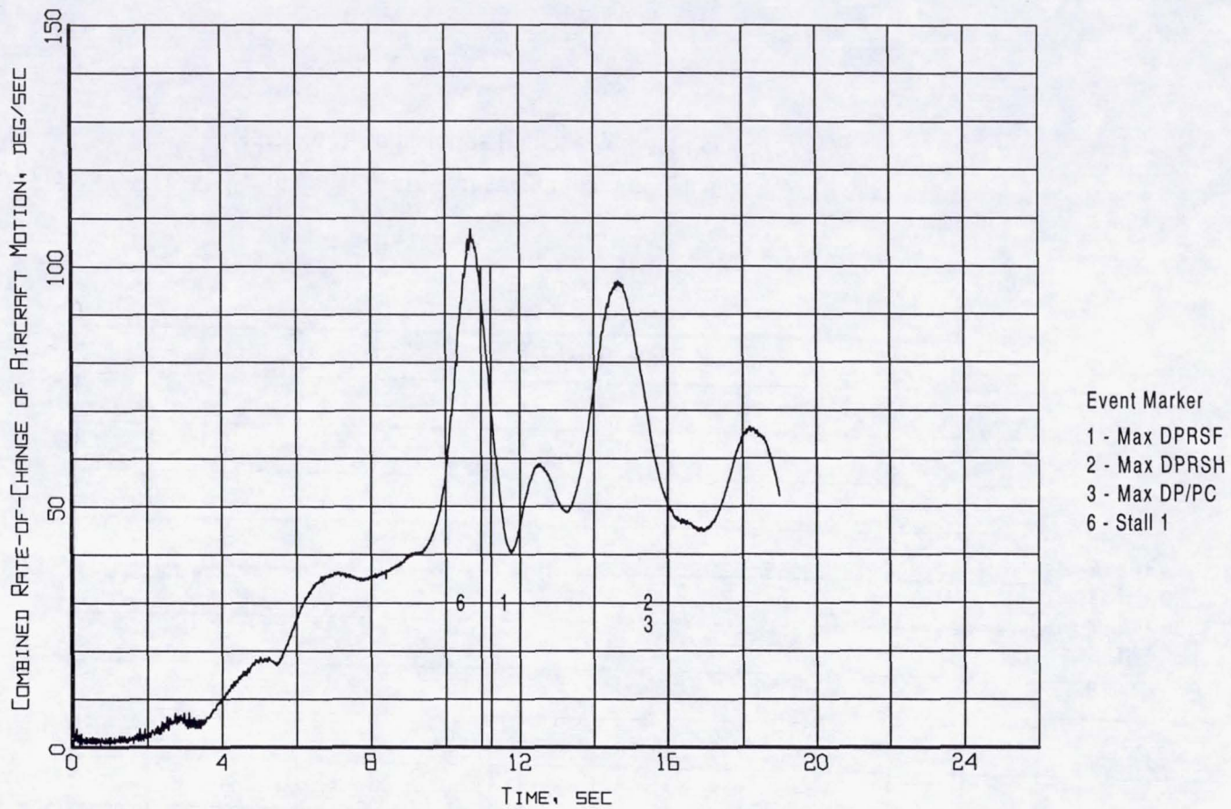
Figure B4-10. Event markers superposed on the combined of rate-of-change of aircraft motion time history (Flight 239, Test Point 37b).
