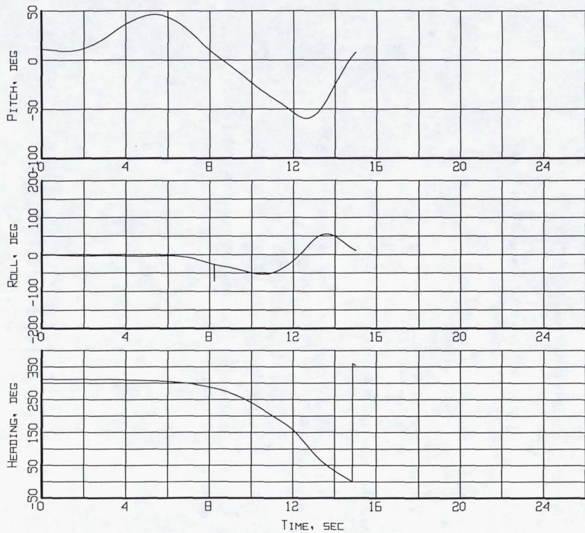
Figure B2-1. Aircraft attitude - Pitch, Roll, and Heading (Flight 238, Test Point 35b).
