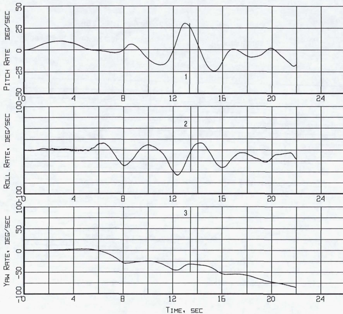
Figure B5-9. Event markers superposed on the aircraft motion time histories (Flight 238, Test Point 38b).
