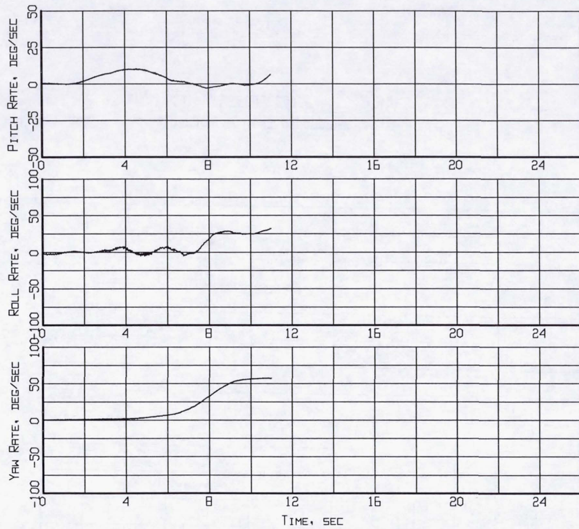
Figure B8-2. Aircraft Motion - Rate-of-Change of Pitch, Roll and Heading (Flight 240, Test Point 41b).
