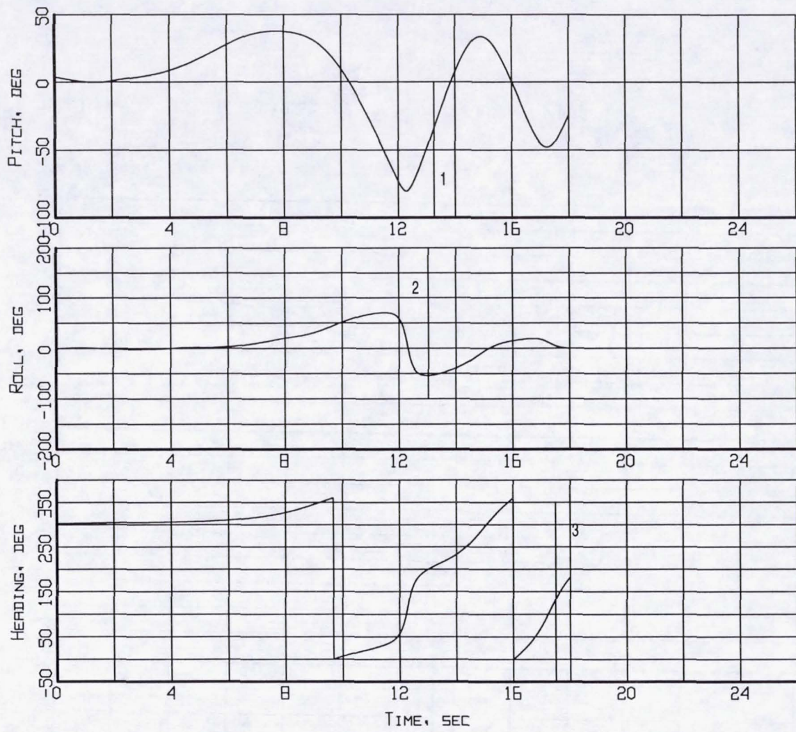
Figure B11-8. Event markers superposed on the aircraft attitude time histories (Flight 238, Test Point 44b).
