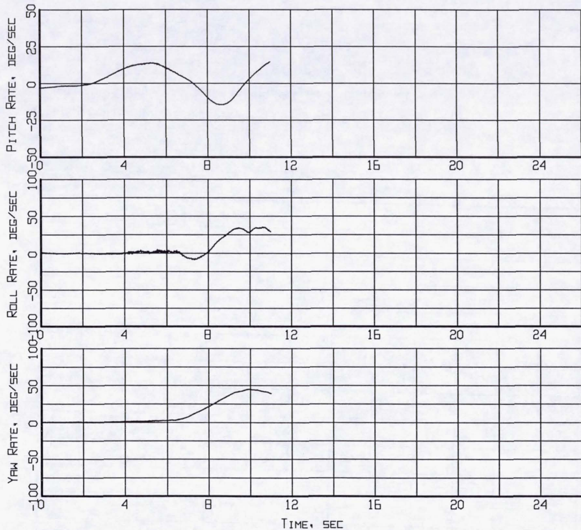
Figure B7-2. Aircraft Motion - Rate-of-Change of Pitch, Roll and Heading (Flight 238, Test Point 40b).
