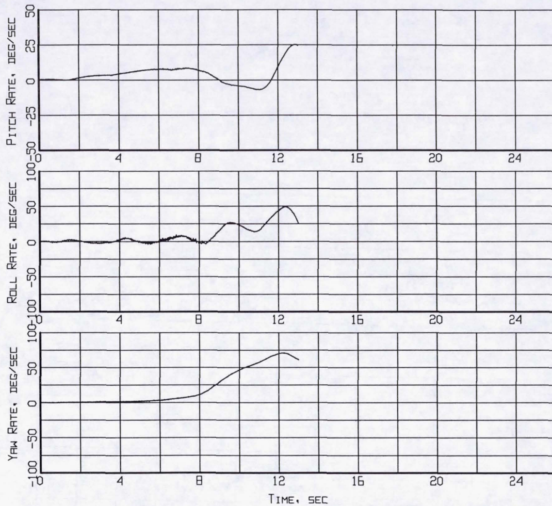
Figure B10-2. Aircraft Motion - Rate-of-Change of Pitch, Roll and Heading (Flight 240, Test Point 43b).
