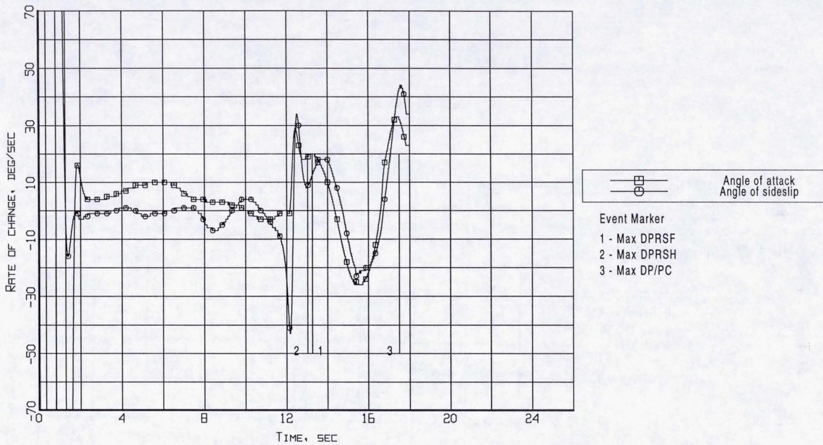
Figure B11-12. Event markers superposed on the aerodynamic flowstream descriptors rate-of-change time histories (Flight 238, Test Point 44b).
