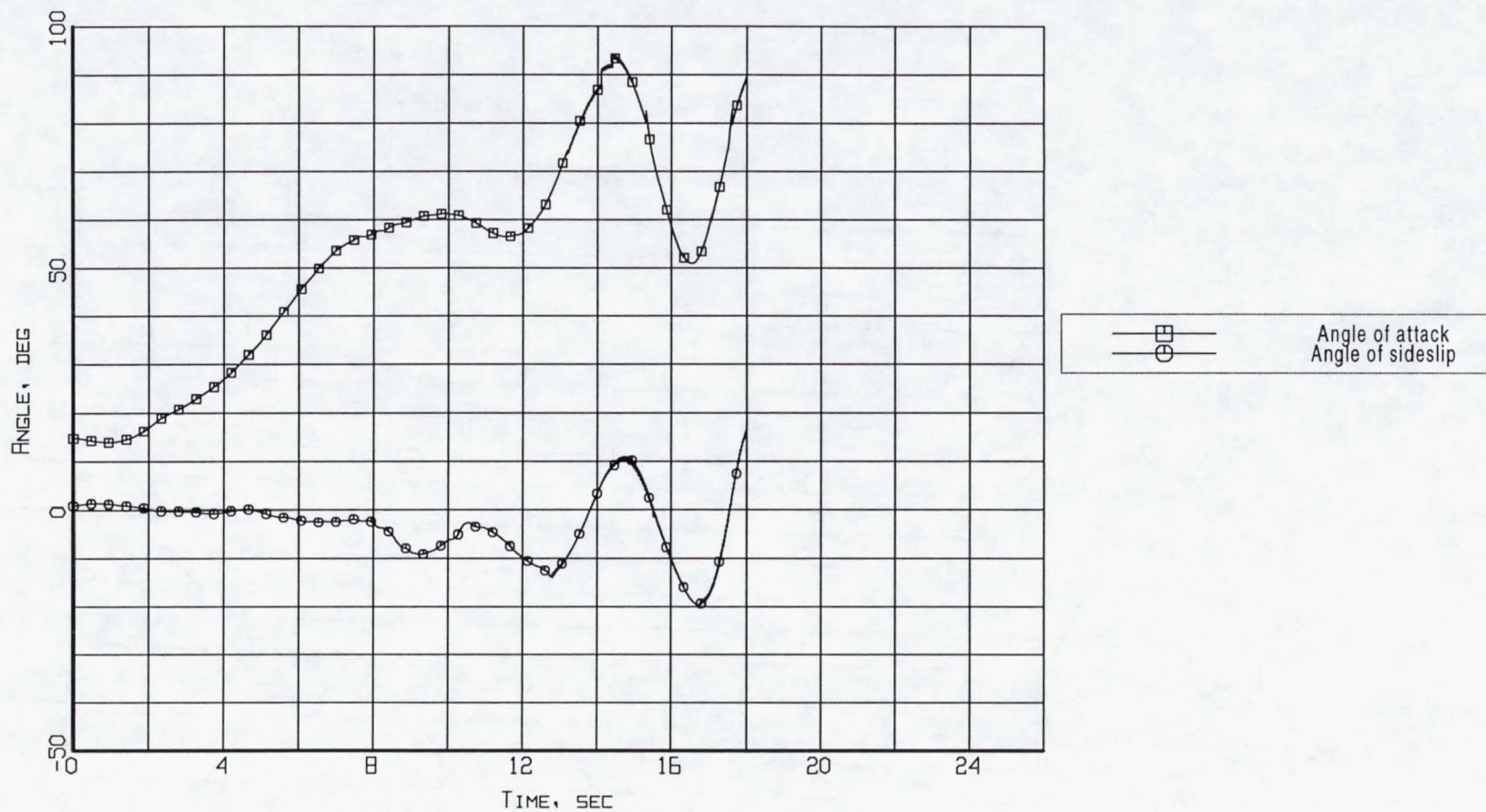
Figure B11-3. Aerodynamic flowstream descriptors - angle of attack and angle of sideslip (Flight 238, Test Point 44b).
