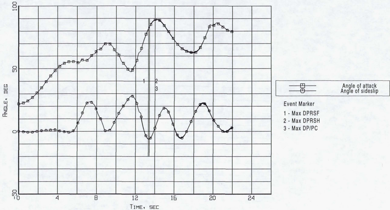
Figure B5-11. Event markers superposed on the aerodynamic flowstream descriptor time histories (Flight 238, Test Point 38b).
