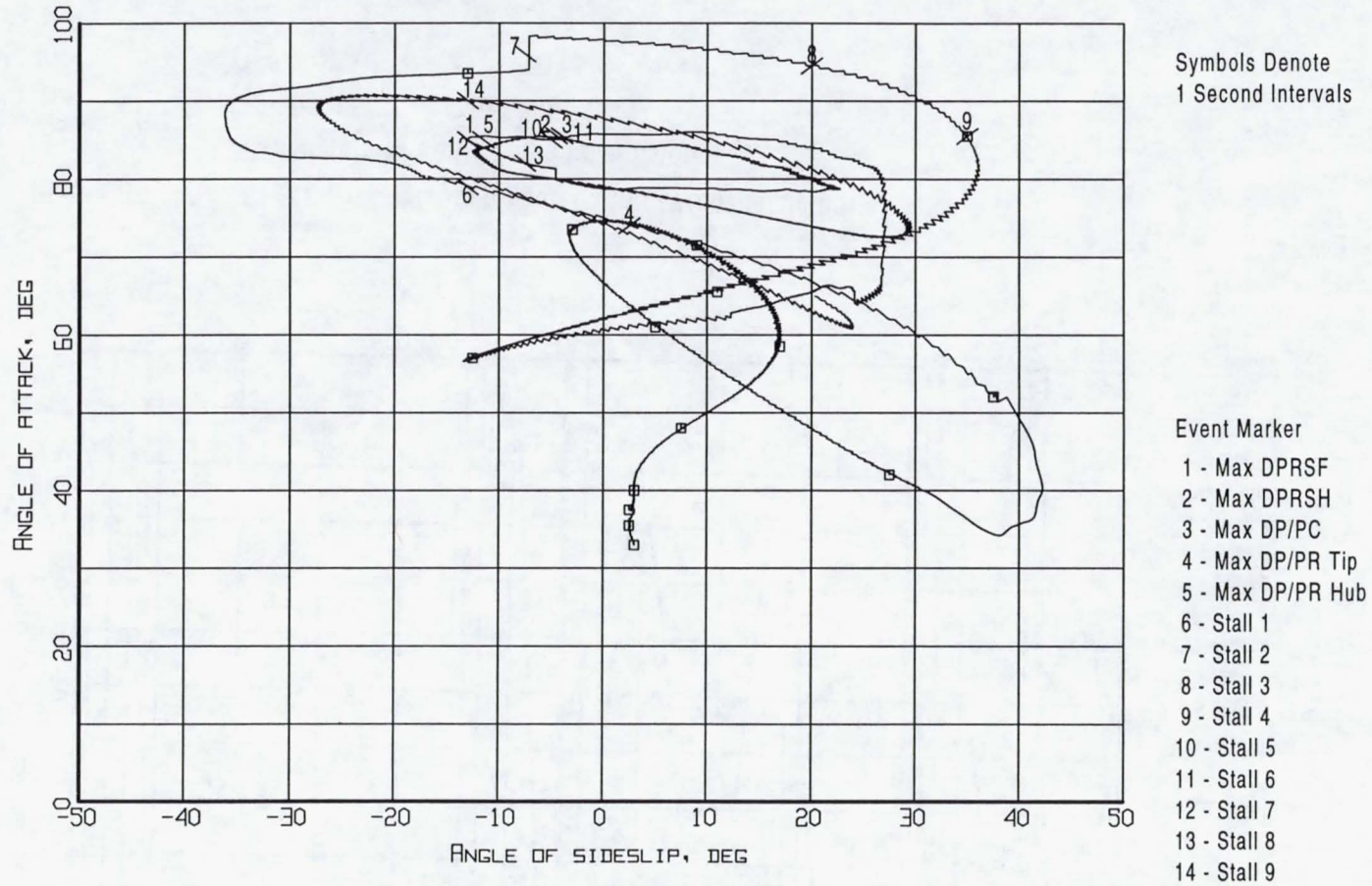
Figure B6-13. Event markers superposed on the aerodynamic flowstream descriptors trajectory (Flight 239, Test Point 39b).
