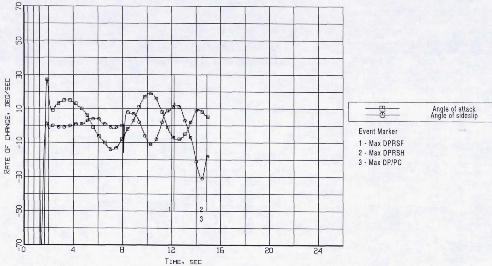
Figure B2-12. Event markers superposed on the aerodynamic flowstream descriptors rate-of-change time histories (Flight 238, Test Point 35b).
