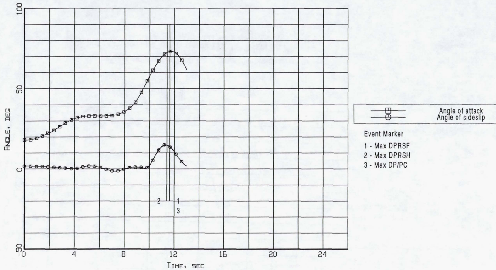
Figure B1-11. Event markers superposed on the aerodynamic flowstream descriptor time histories (Flight 239, Test Point 34b).
