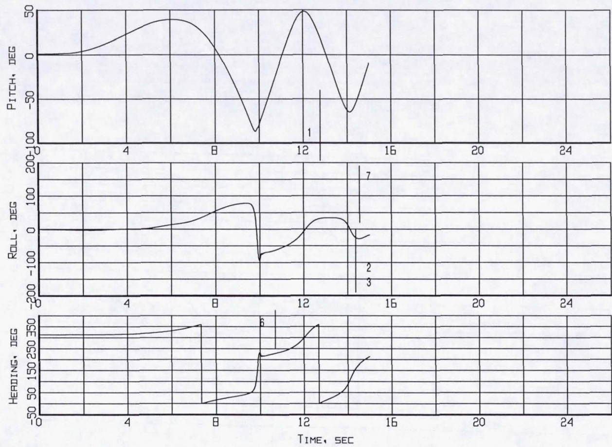
Figure 11. Event markers superposed on the aircraft attitude time histories (Flight 240, Test Point 45b).
