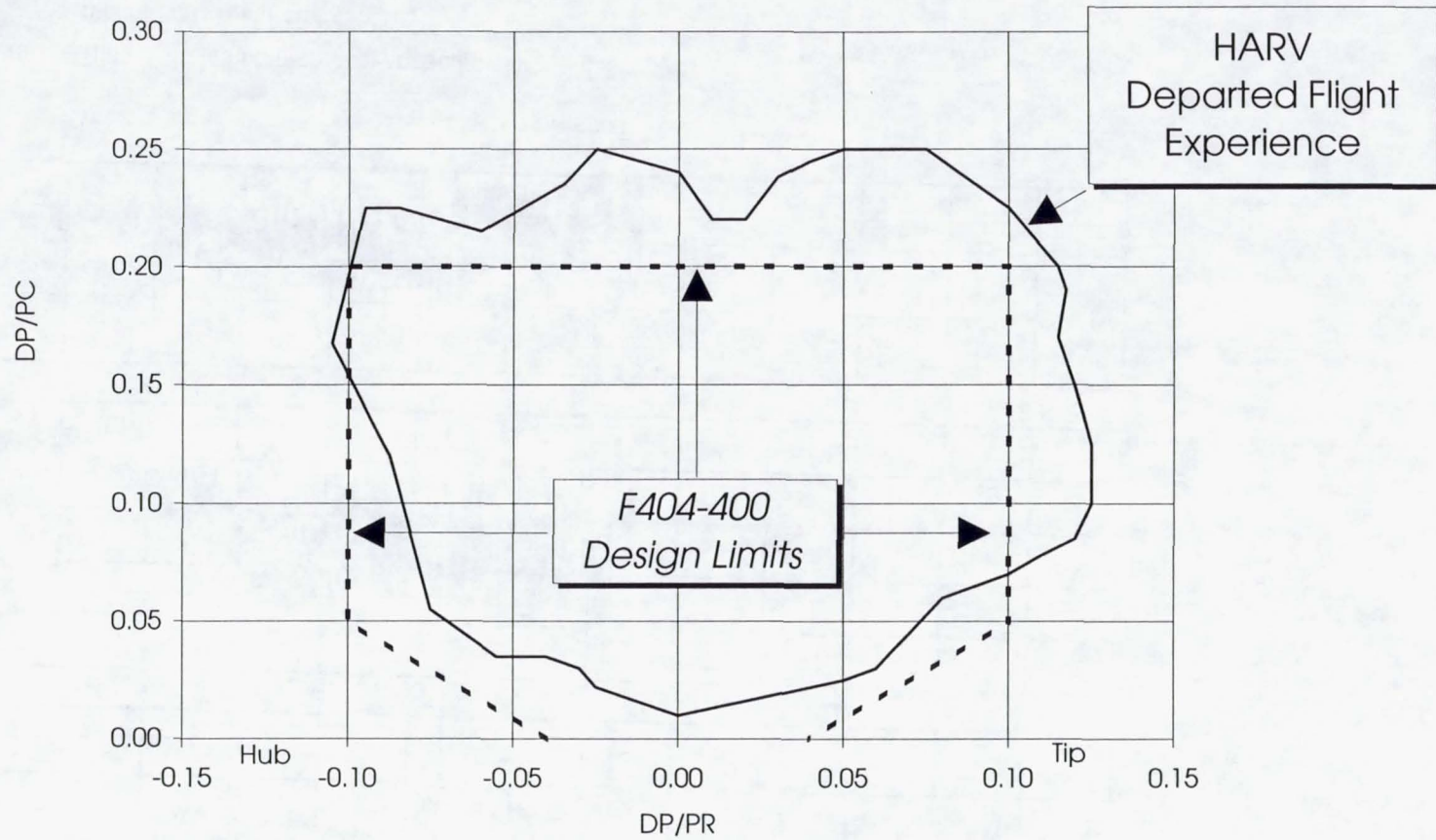
Figure 8. Bounds of time-variant circumferential and radial total-pressure distortion levels experienced during departed flight relative to the F404-GE-400 engine design guidance limits.
