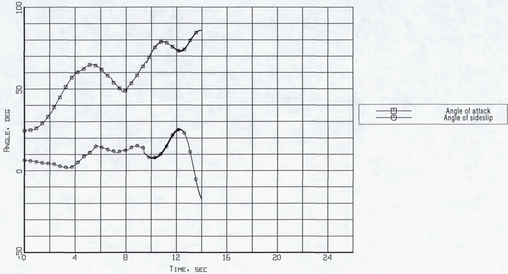
Figure B3-3. Aerodynamic flowstream descriptors - angle of attack and angle of sideslip (Flight 238, Test Point 36b).
