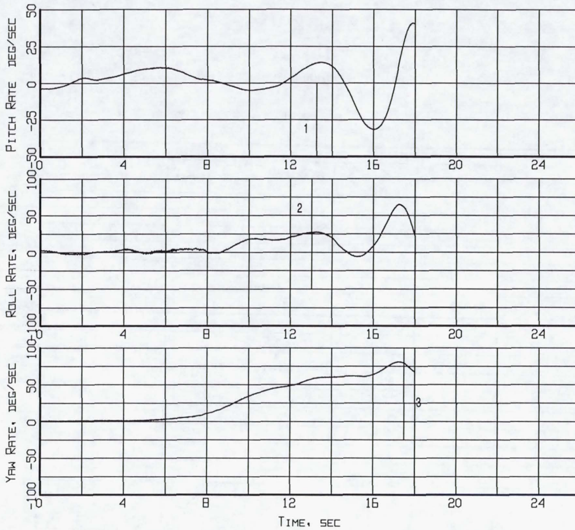
Figure B11-9. Event markers superposed on the aircraft motion time histories (Flight 238, Test Point 44b).
