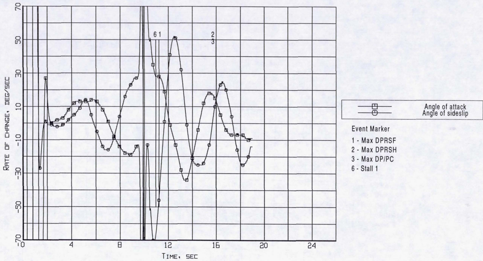
Figure B4-12. Event markers superposed on the aerodynamic flowstream descriptors rate-of-change time histories (Flight 239, Test Point 37b).
