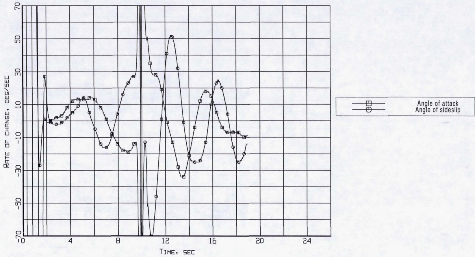
Figure B4-4. Aerodynamic flowstream descriptors - rate of change of angle of attack and angle of sideslip (Flight 239, Test Point 37b).
