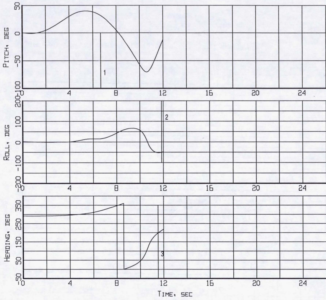
Figure B9-8. Event markers superposed on the aircraft attitude time histories (Flight 238, Test Point 42b).
