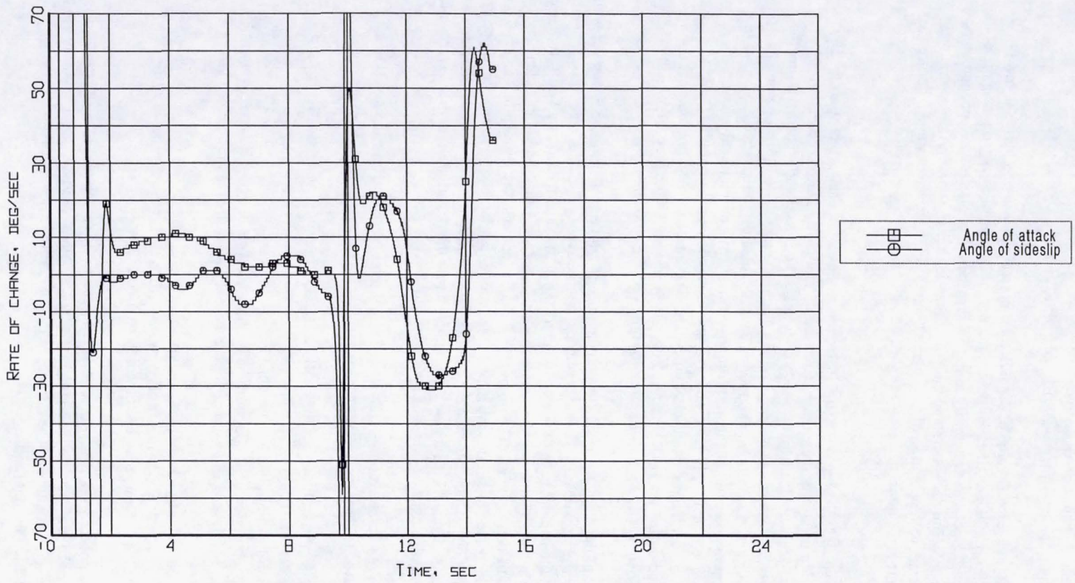
Figure 6. Aerodynamic flowstream descriptors - rate of change of angle of attack and angle of sideslip (Flight 240, Test Point 45b).
