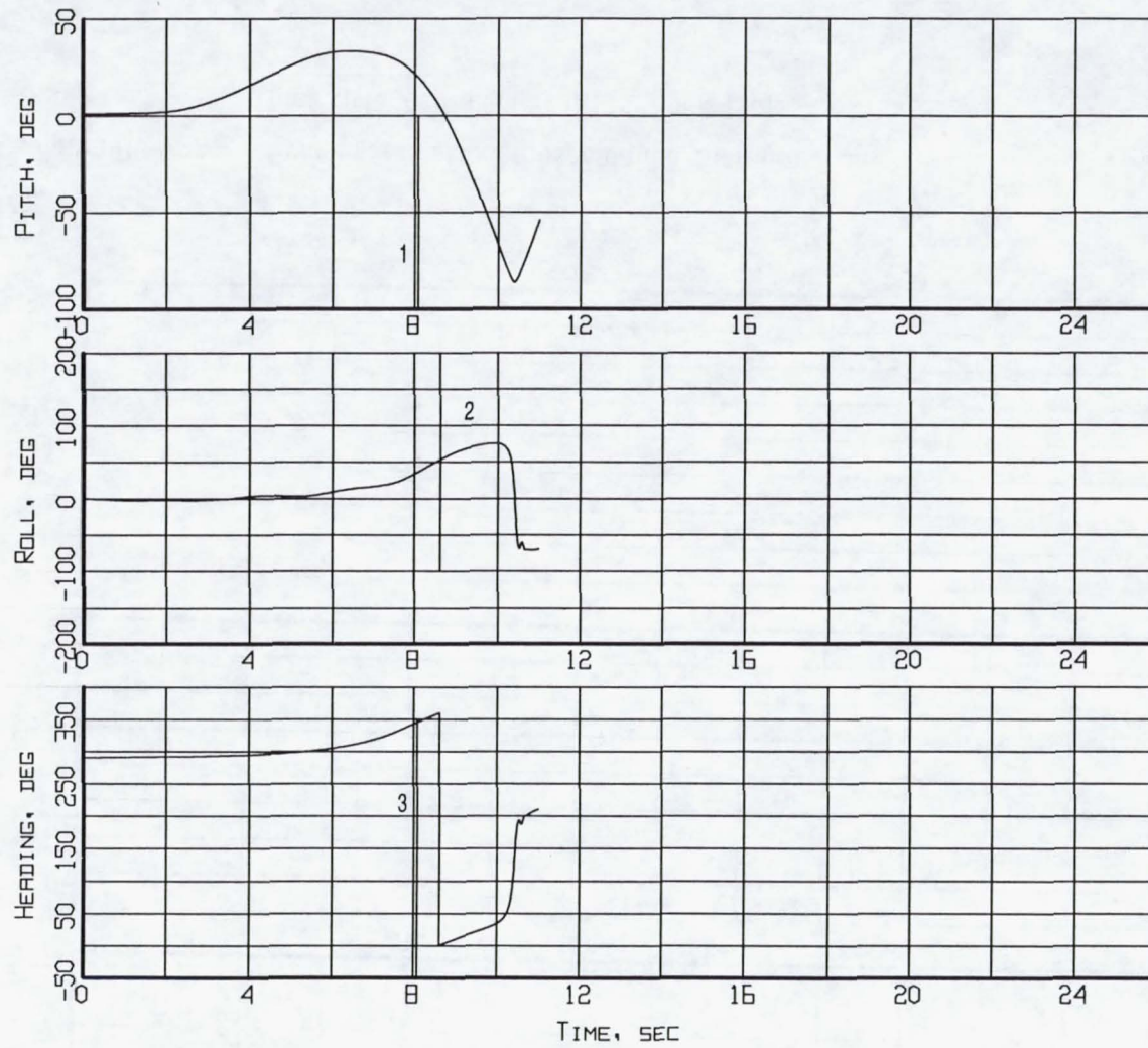
Figure B8-8. Event markers superposed on the aircraft attitude time histories (Flight 240, Test Point 41b).
