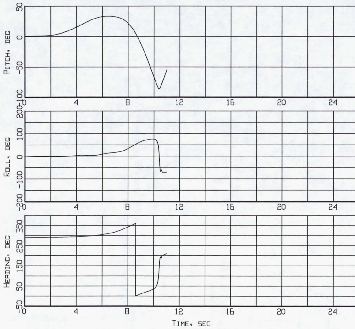
Figure B8-1. Aircraft attitude - Pitch, Roll, and Heading (Flight 240, Test Point 41b).
