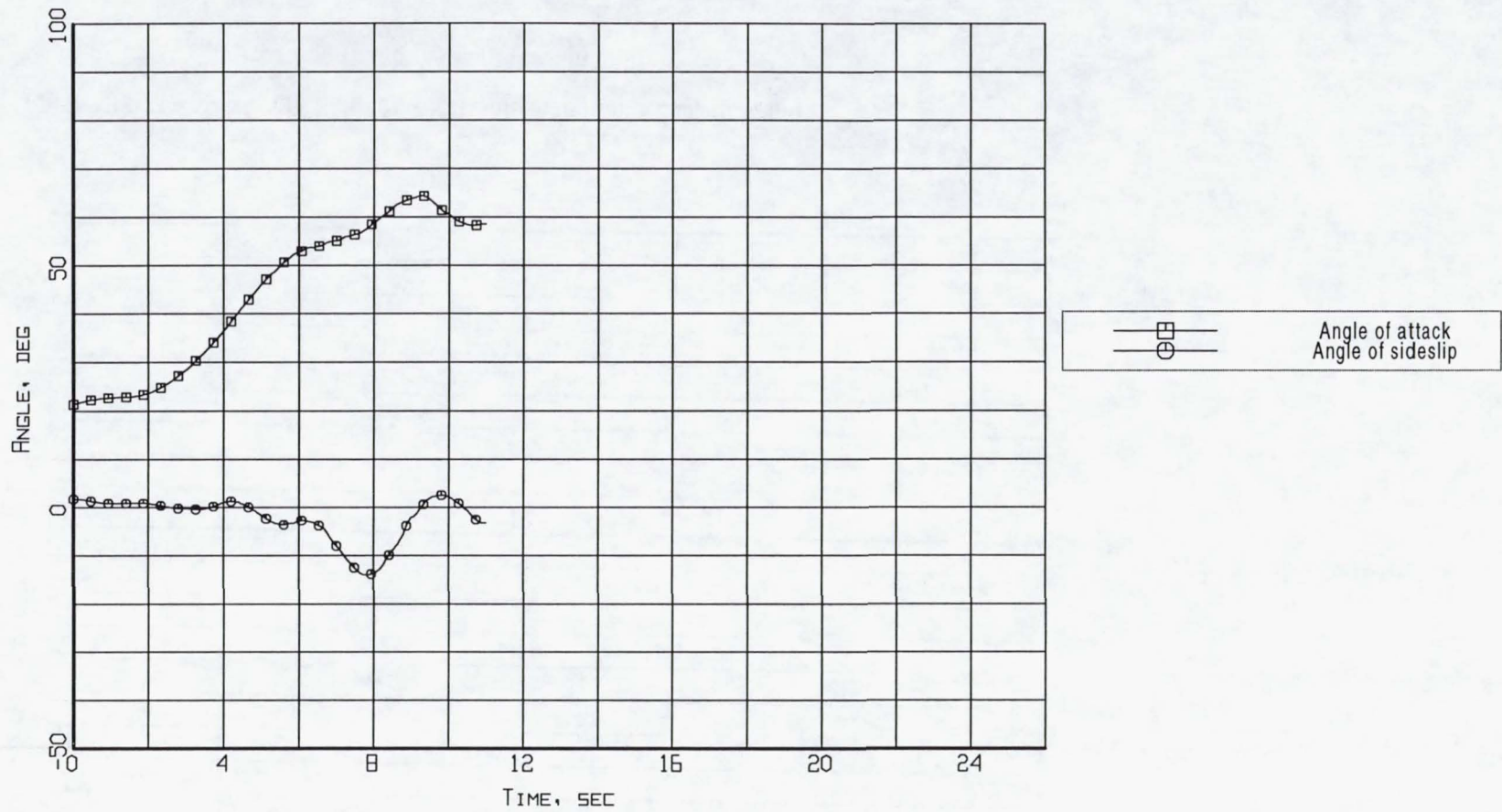
Figure B8-3. Aerodynamic flowstream descriptors - angle of attack and angle of sideslip (Flight 240, Test Point 41b).
