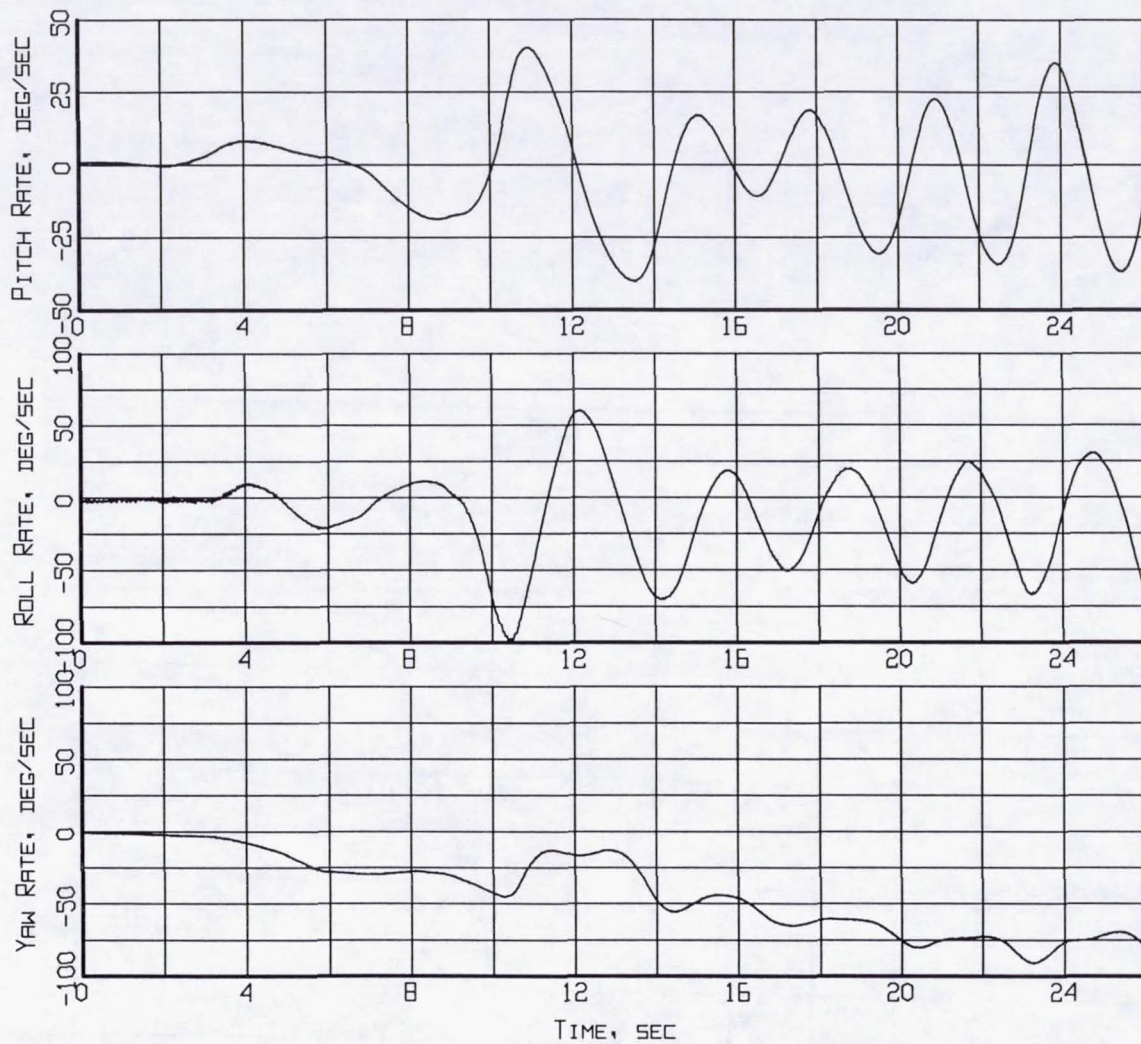
Figure B6-2. Aircraft Motion - Rate-of-Change of Pitch, Roll and Heading (Flight 239, Test Point 39b).
