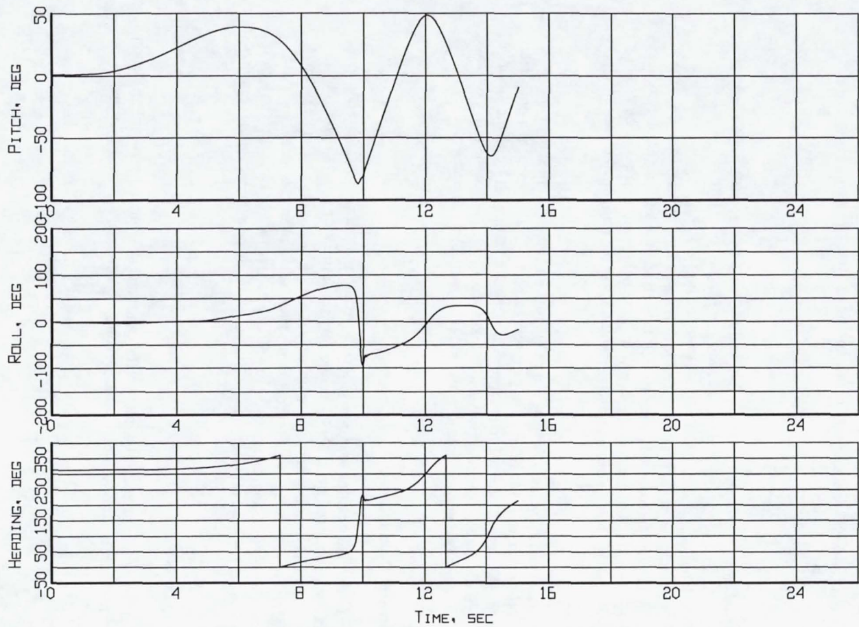
Figure 3. Aircraft attitude - Pitch, Roll, and Heading (Flight 240, Test Point 45b).
