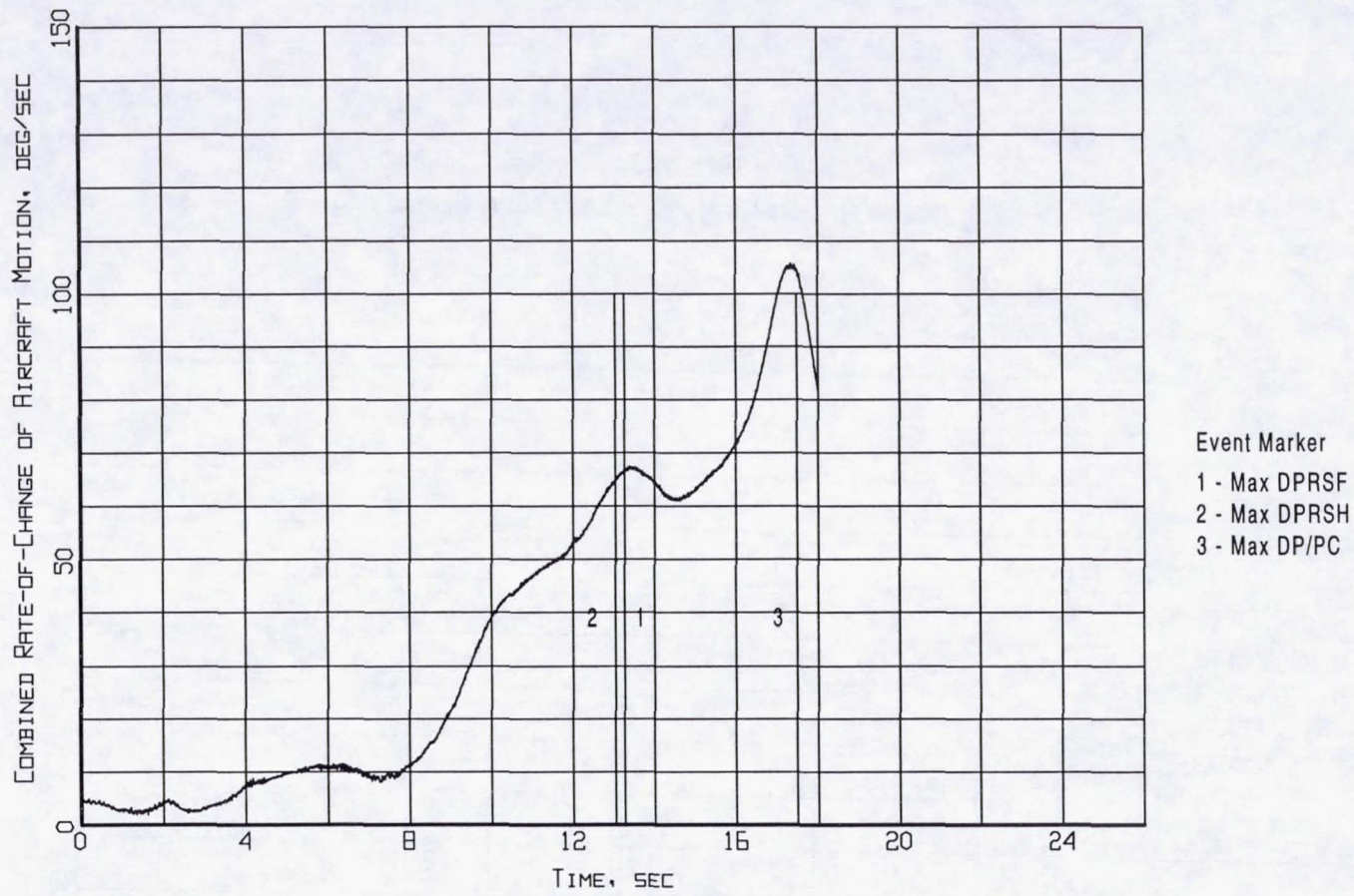
Figure B11-10. Event markers superposed on the combined of rate-of-change of aircraft motion time history (Flight 238, Test Point 44b).
