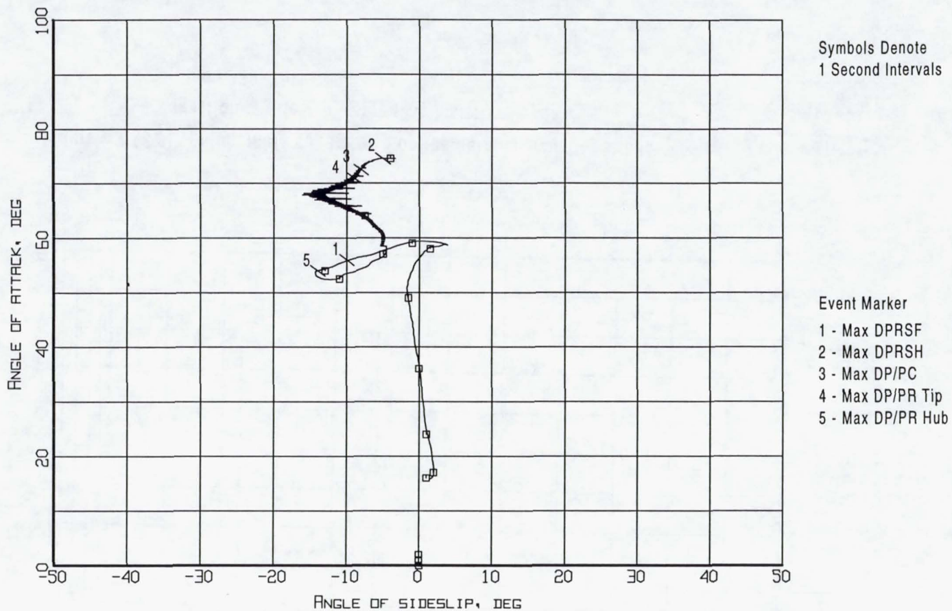
Figure B9-13. Event markers superposed on the aerodynamic flowstream descriptors trajectory (Flight 238, Test Point 42b).
