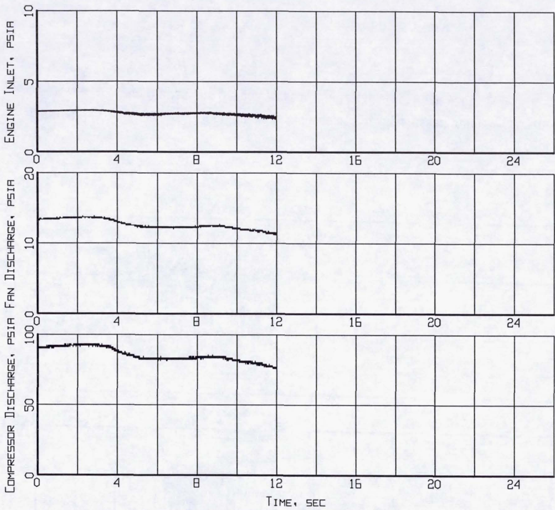
Figure B9-6. Measured inlet/engine entry and engine internal pressures time histories (Flight 238, Test Point 42b).
