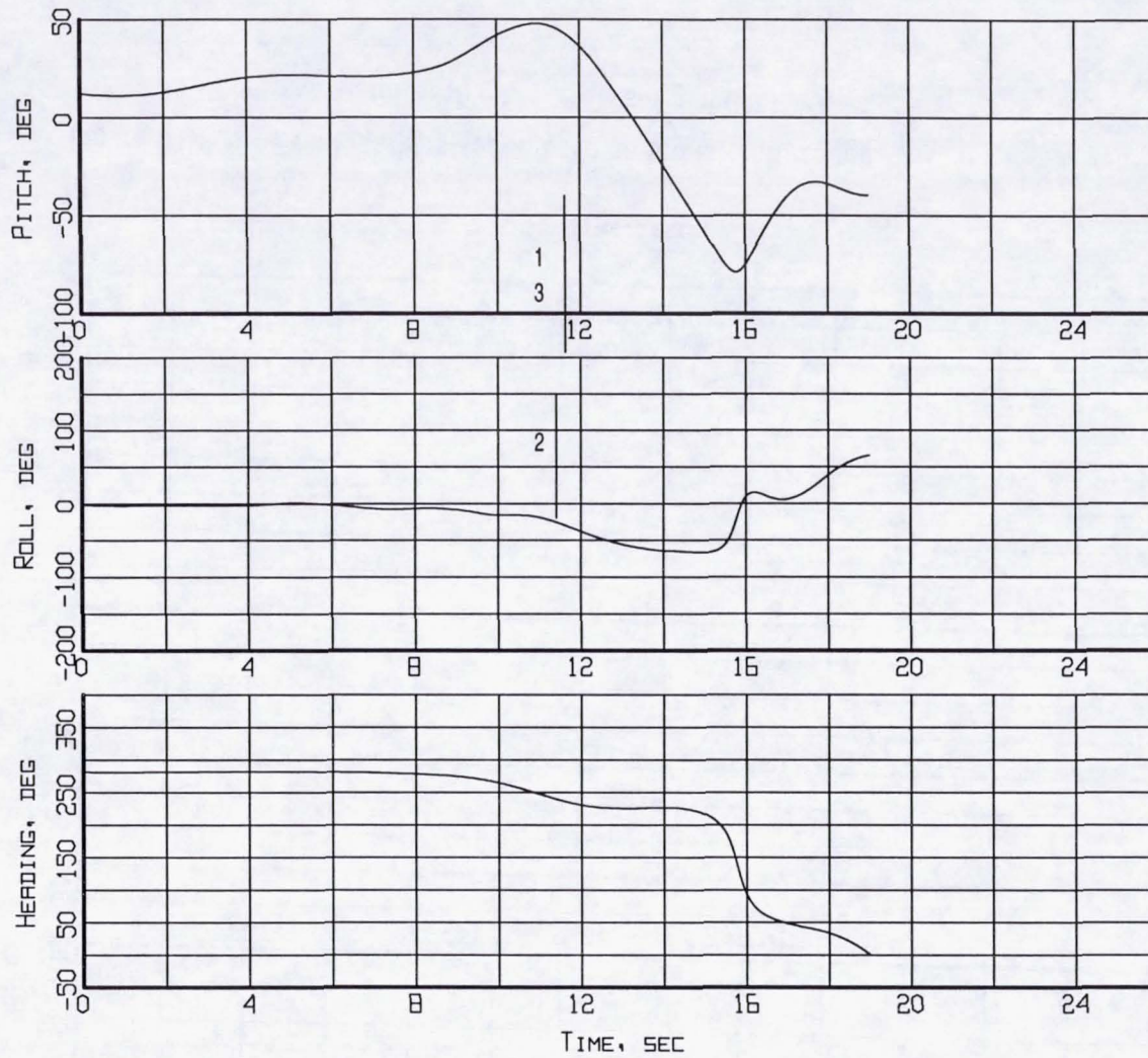
Figure B1-8. Event markers superposed on the aircraft attitude time histories (Flight 239, Test Point 34b).
