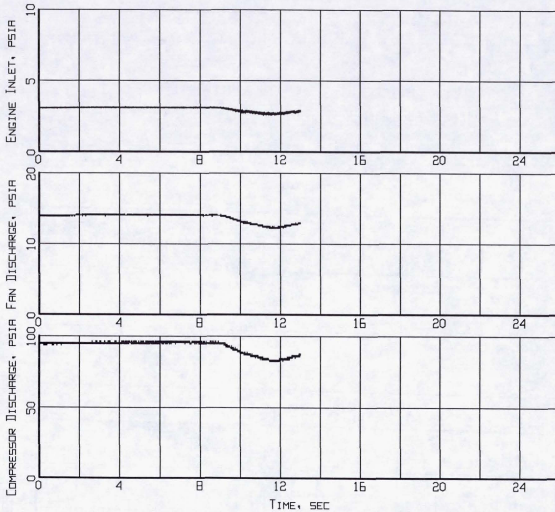
Figure B1-6. Measured inlet/engine entry and engine internal pressures time histories (Flight 239, Test Point 34b).
