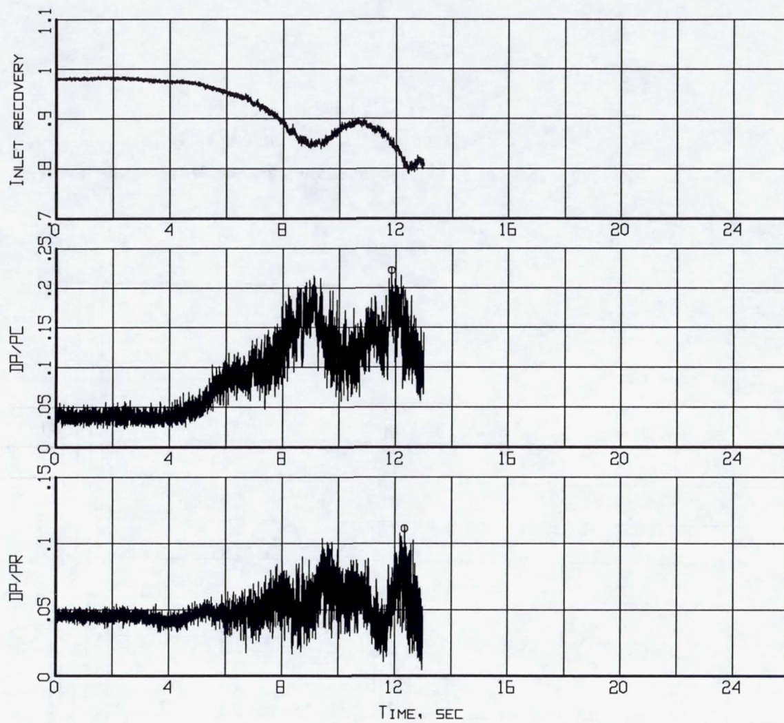
Figure B10-5. Time histories of inlet recovery and distortion descriptors (Flight 240, Test Point 43b).
