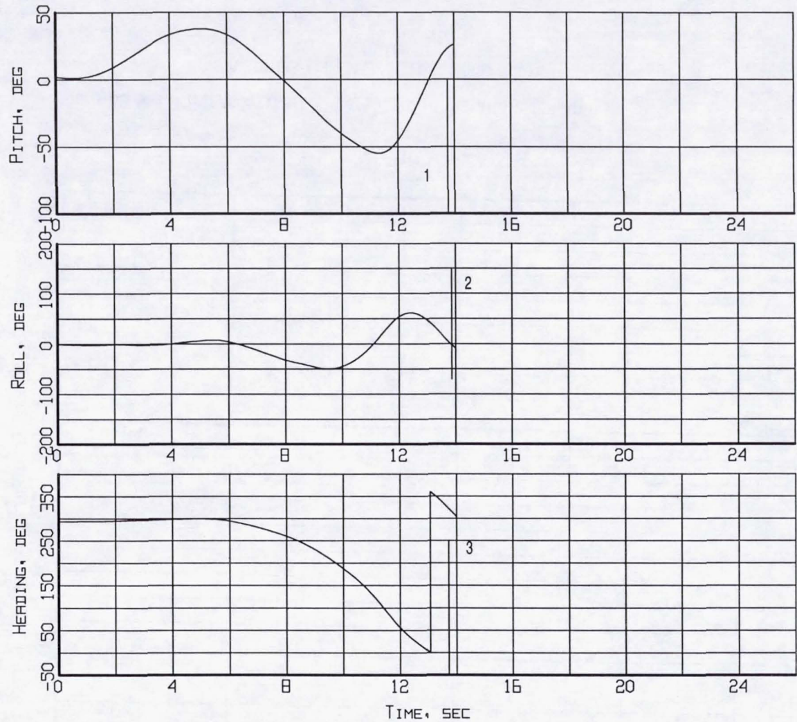
Figure B3-8. Event markers superposed on the aircraft attitude time histories (Flight 238, Test Point 36b).
