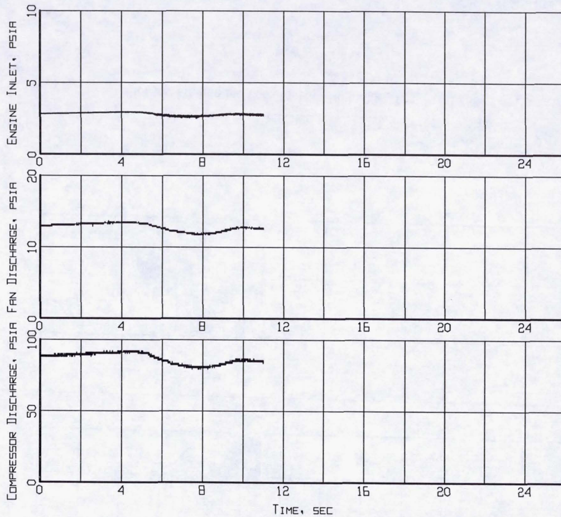
Figure B7-6. Measured inlet/engine entry and engine internal pressures time histories (Flight 238, Test Point 40b).
