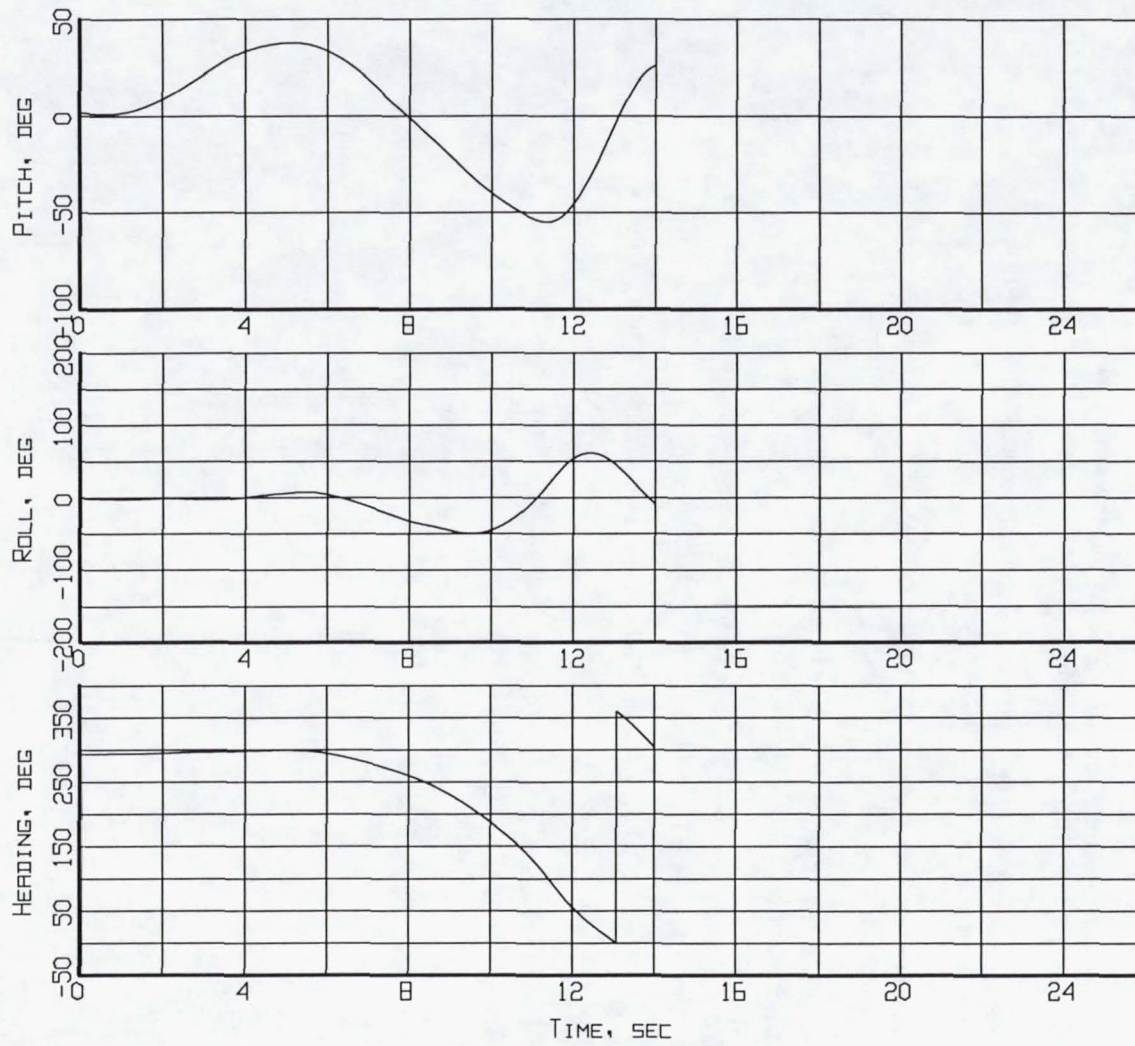
Figure B3-1. Aircraft attitude - Pitch, Roll, and Heading (Flight 238, Test Point 36b).
