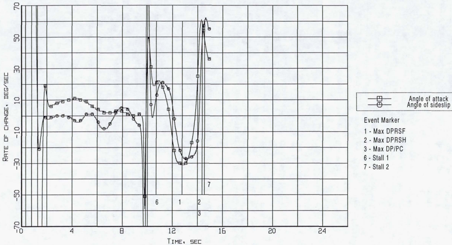
Figure 15. Event markers superposed on the rate-of-change of angle-of-attack and angle-of-sideslip time histories (Flight 240, Test Point 45b).
