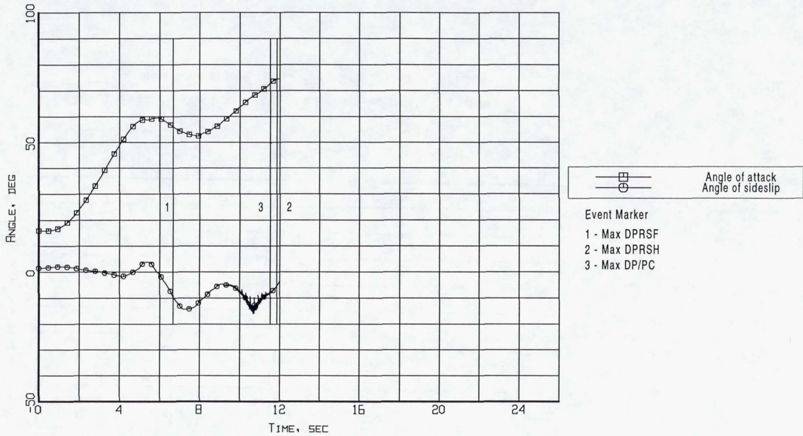
Figure B9-11. Event markers superposed on the aerodynamic flowstream descriptor time histories (Flight 238, Test Point 42b).
