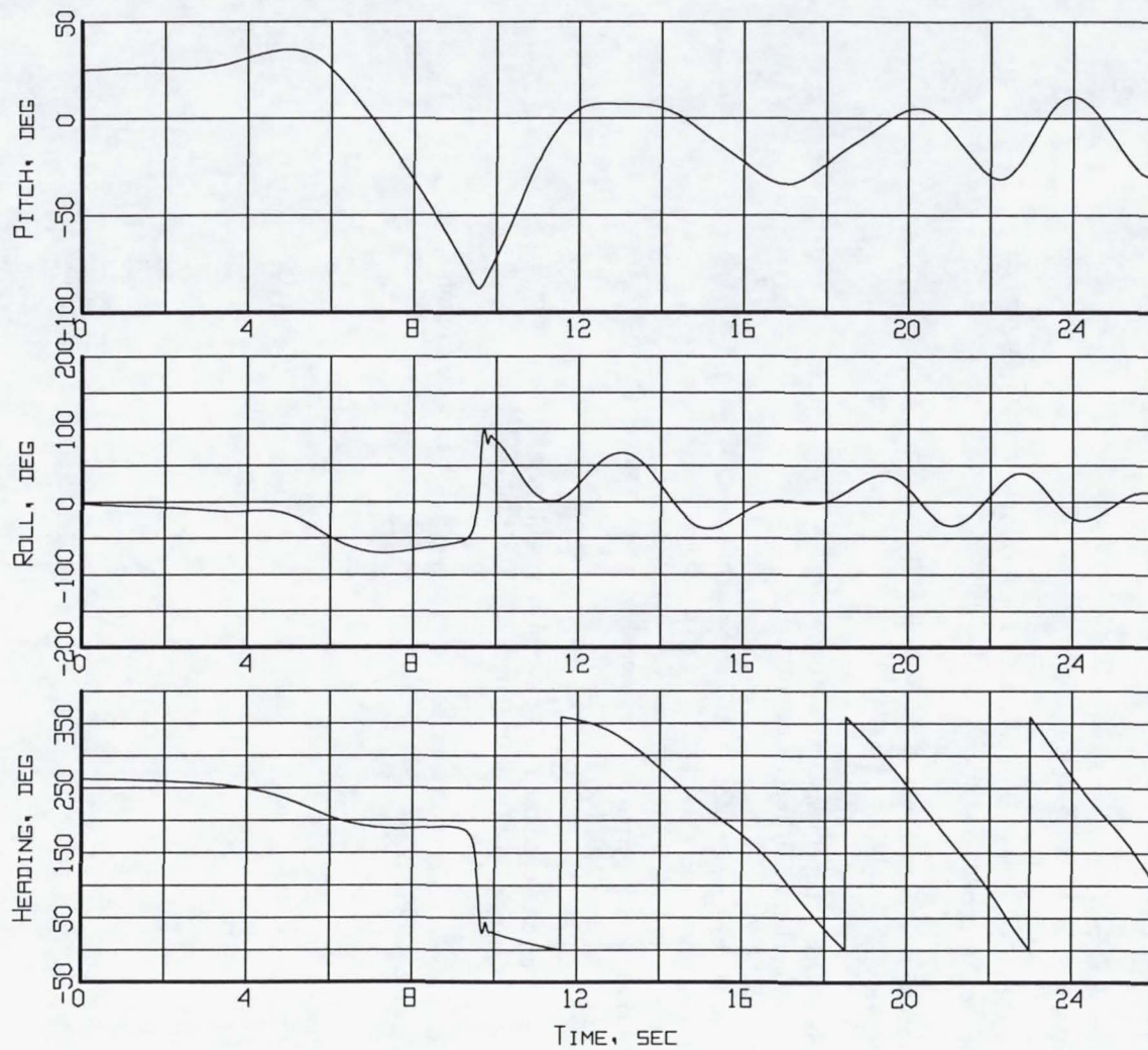
Figure B6-1. Aircraft attitude - Pitch, Roll, and Heading (Flight 239, Test Point 39b).
