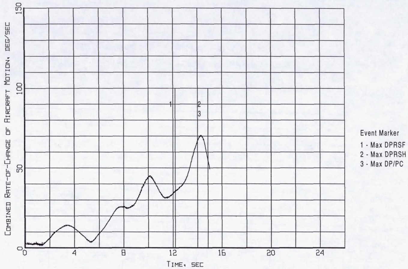
Figure B2-10. Event markers superposed on the combined of rate-of-change of aircraft motion time history (Flight 238, Test Point 35b).
