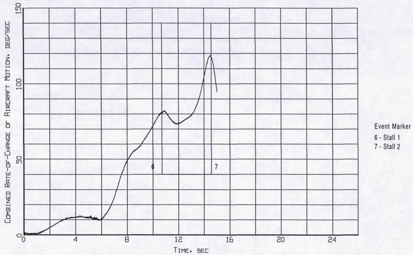
Figure 13. Event markers superposed on the combined of rate-of-change of aircraft motion time history (Flight 240, Test Point 45b).
