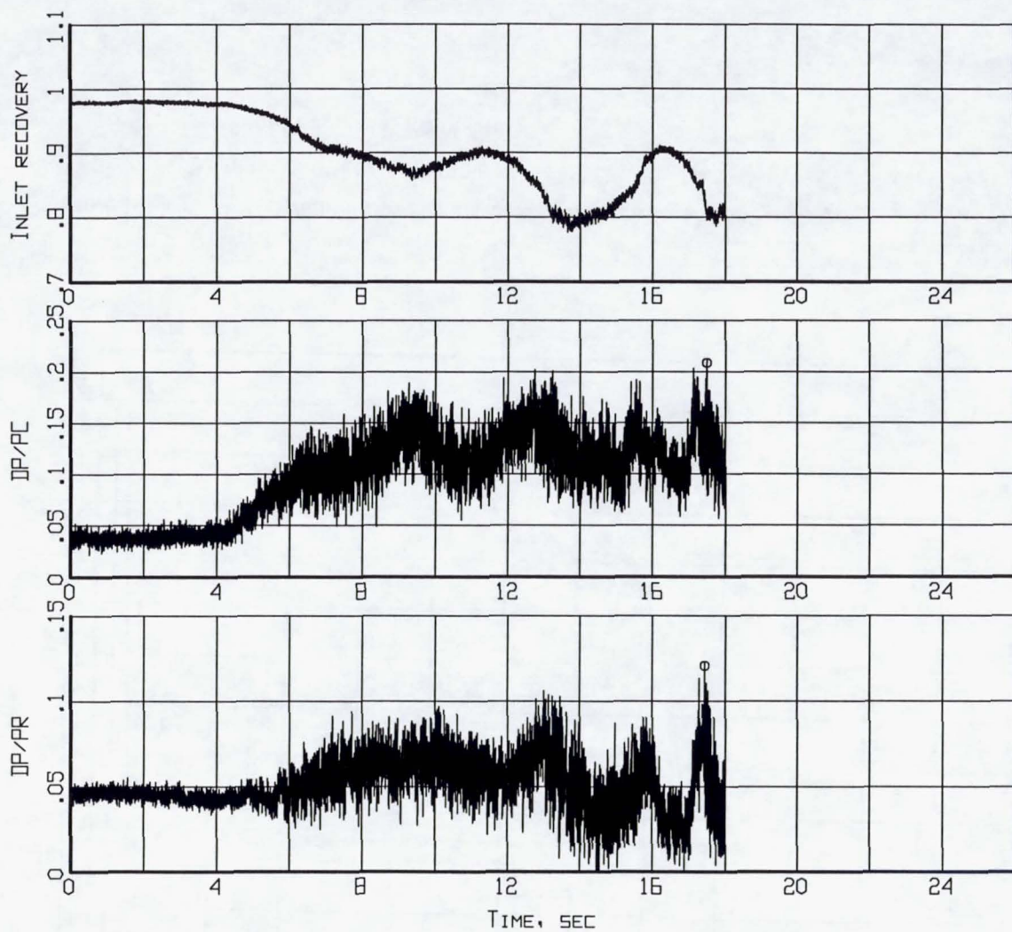
Figure B11-5. Time histories of inlet recovery and distortion descriptors (Flight 238, Test Point 44b).
