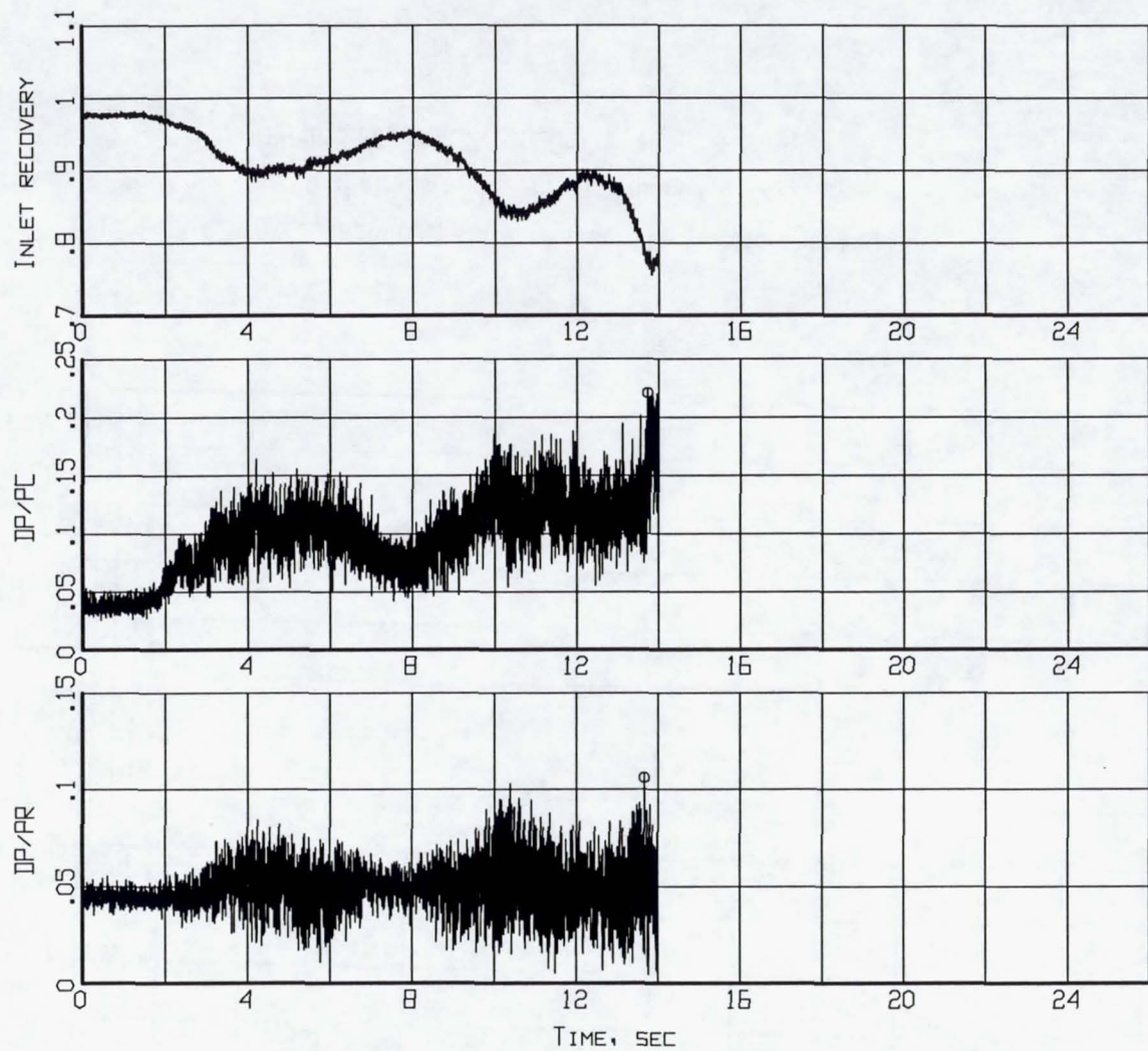
Figure B3-5. Time histories of inlet recovery and distortion descriptors (Flight 238, Test Point 36b).
