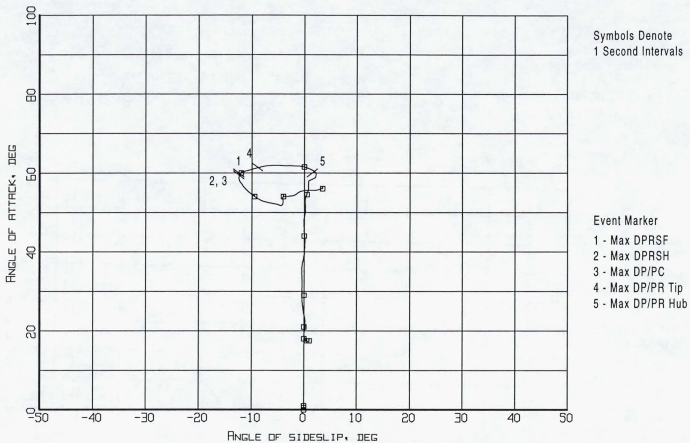
Figure B7-13. Event markers superposed on the aerodynamic flowstream descriptors trajectory (Flight 238, Test Point 40b).
