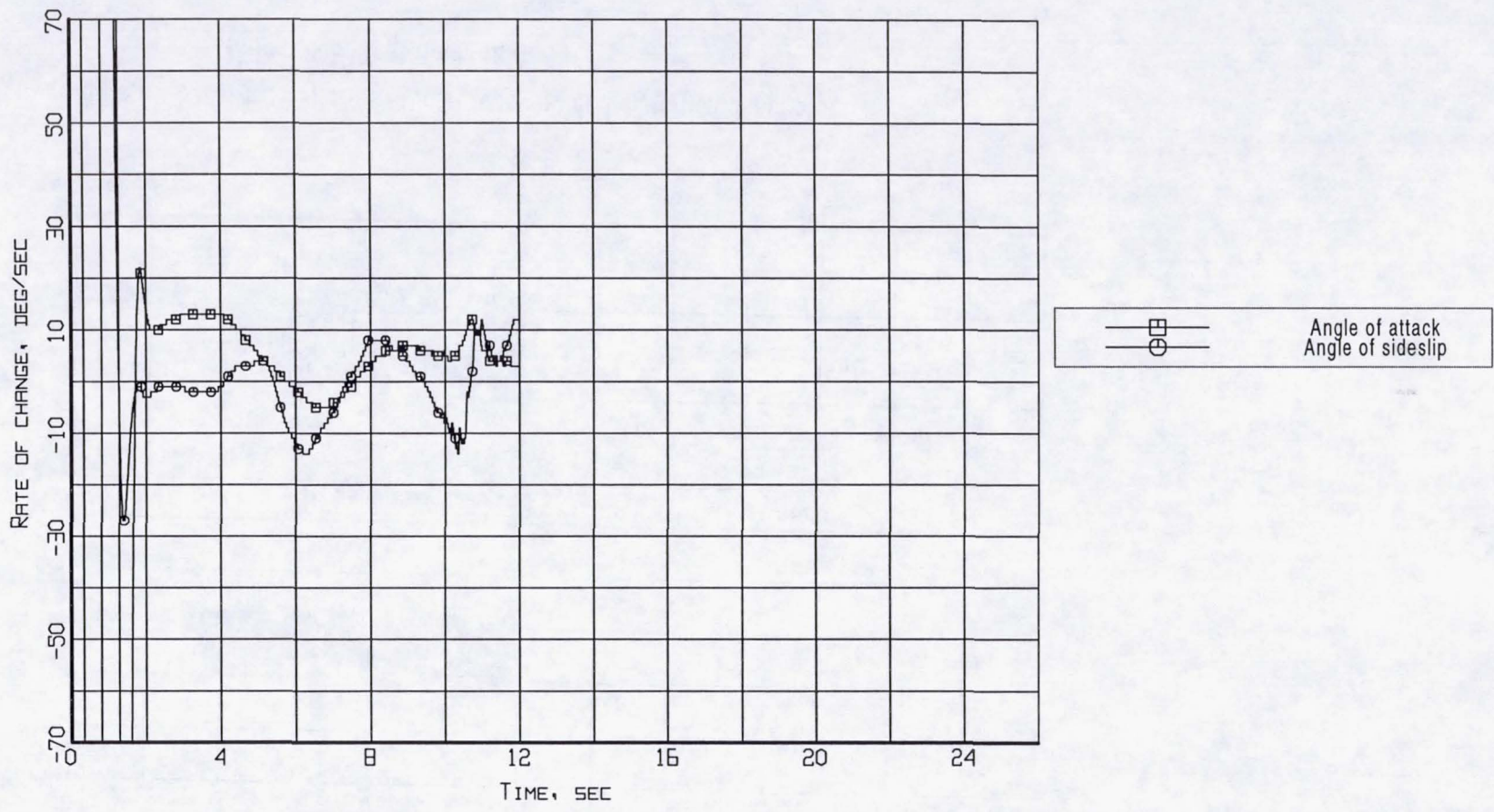
Figure B9-4. Aerodynamic flowstream descriptors - rate of change of angle of attack and angle of sideslip (Flight 238, Test Point 42b).
