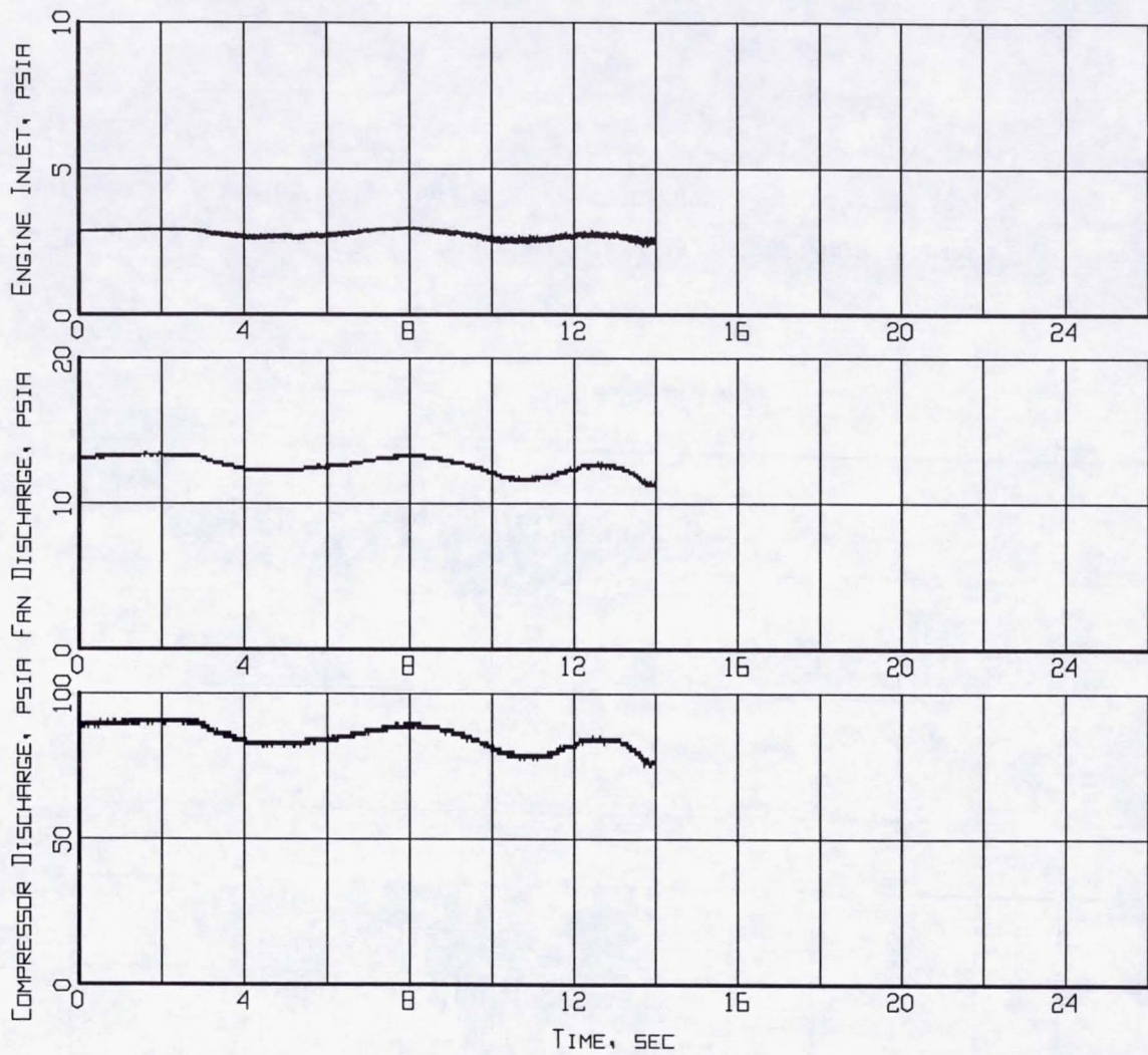
Figure B3-6. Measured inlet/engine entry and engine internal pressures time histories (Flight 238, Test Point 36b).
