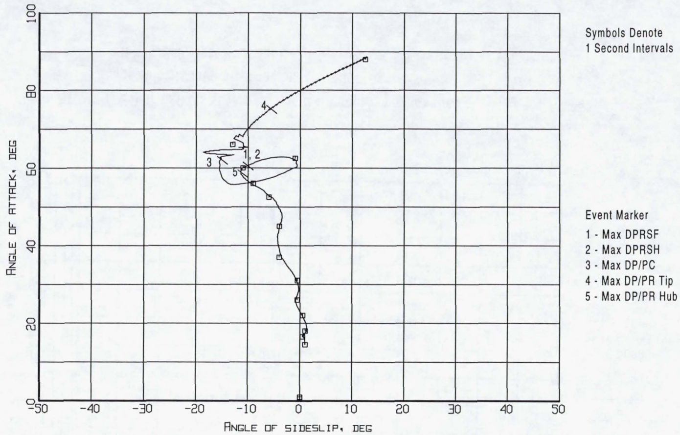
Figure B10-13. Event markers superposed on the aerodynamic flowstream descriptors trajectory (Flight 240, Test Point 43b).
