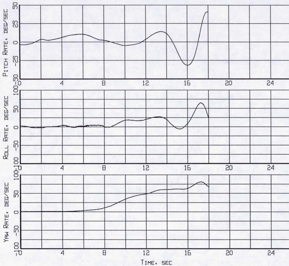
Figure B11-2. Aircraft Motion - Rate-of-Change of Pitch, Roll and Heading (Flight 238, Test Point 44b).
