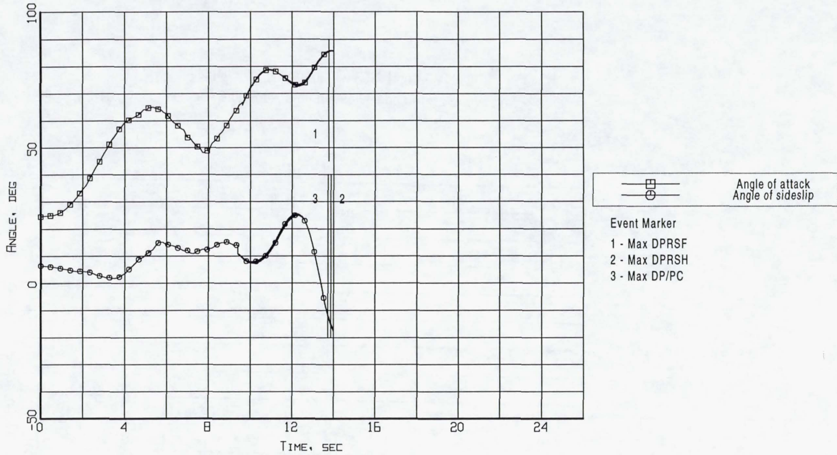
Figure B3-11. Event markers superposed on the aerodynamic flowstream descriptor time histories (Flight 238, Test Point 36b).
