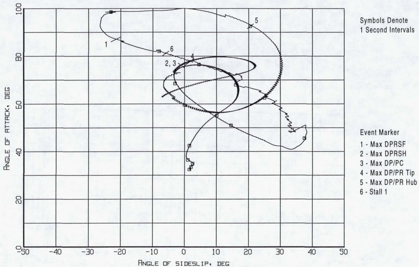
Figure B4-13. Event markers superposed on the aerodynamic flowstream descriptors trajectory (Flight 239, Test Point 37b).
