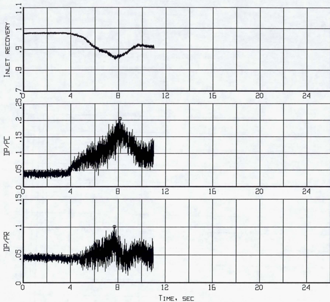
Figure B7-5. Time histories of inlet recovery and distortion descriptors (Flight 238, Test Point 40b).
