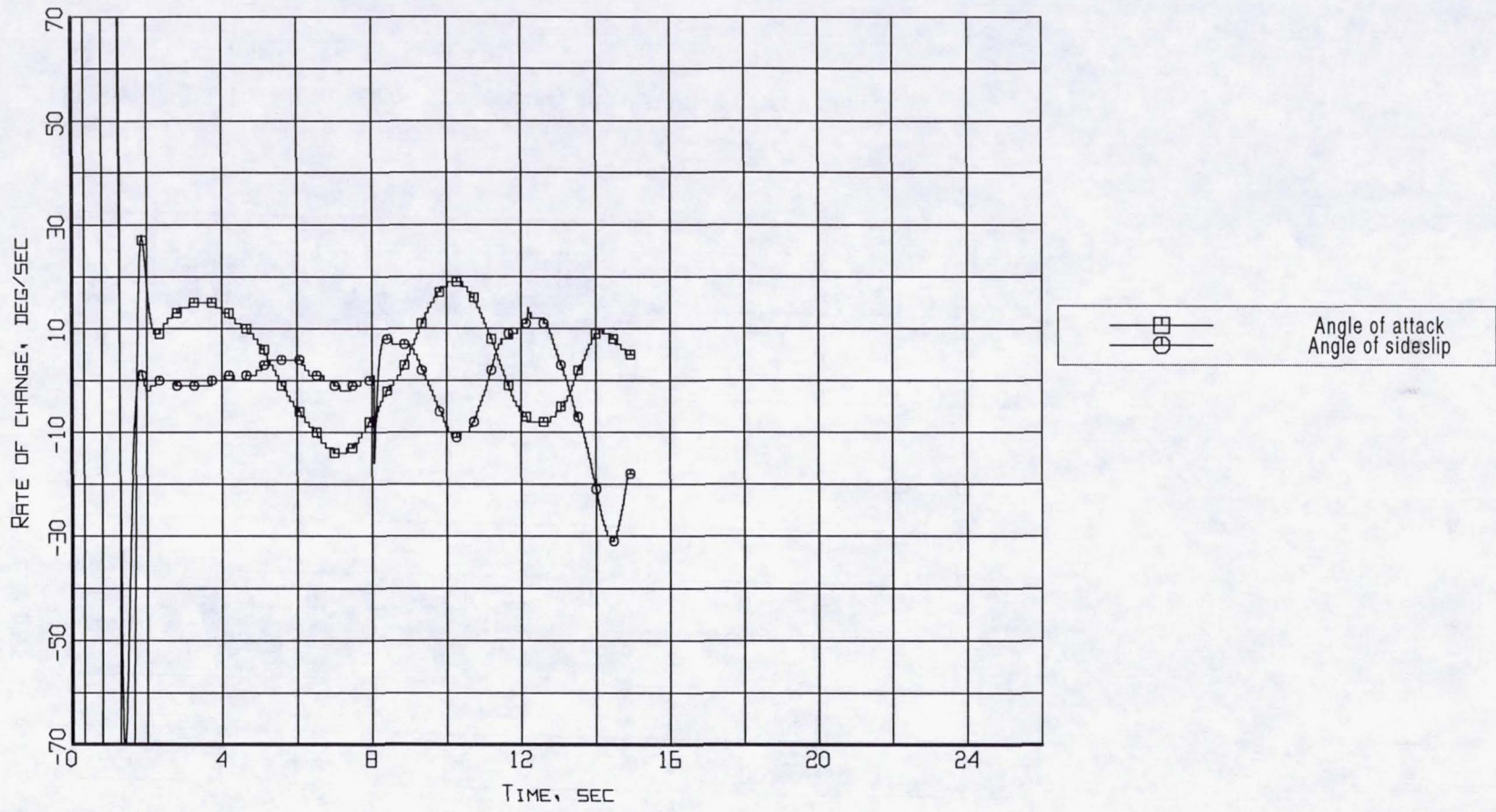
Figure B2-4. Aerodynamic flowstream descriptors - rate of change of angle of attack and angle of sideslip (Flight 238, Test Point 35b).
