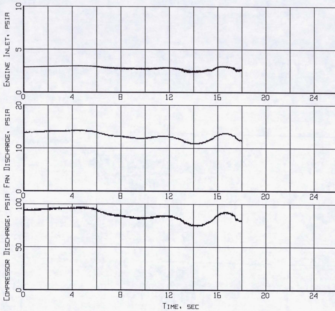
Figure B11-6. Measured inlet/engine entry and engine internal pressures time histories (Flight 238, Test Point 44b).
