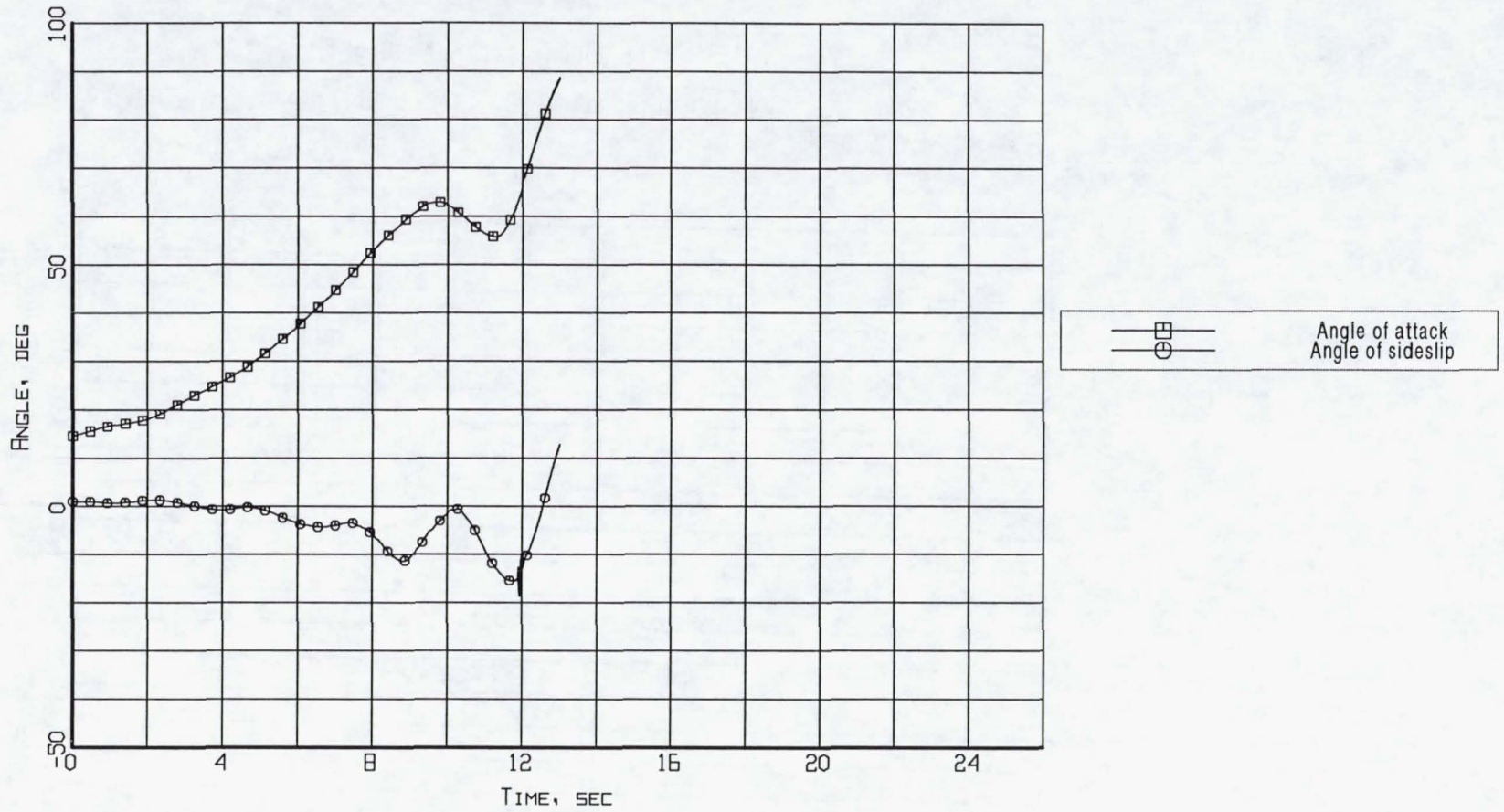
Figure B10-3. Aerodynamic flowstream descriptors - angle of attack and angle of sideslip (Flight 240, Test Point 43b).
