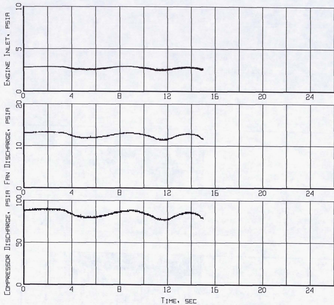
Figure B2-6. Measured inlet/engine entry and engine internal pressures time histories (Flight 238, Test Point 35b).
