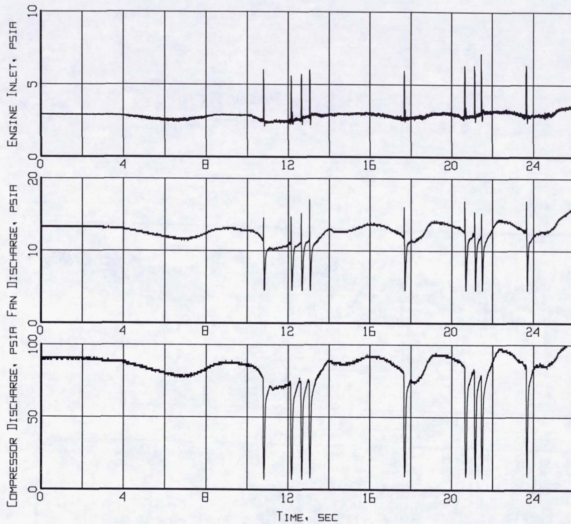
Figure B6-6. Measured inlet/engine entry and engine internal pressures time histories (Flight 239, Test Point 39b).
