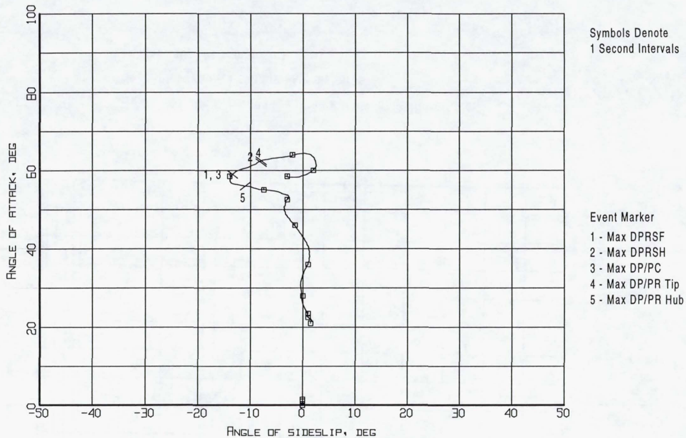
Figure B8-13. Event markers superposed on the aerodynamic flowstream descriptors trajectory (Flight 240, Test Point 41b).
