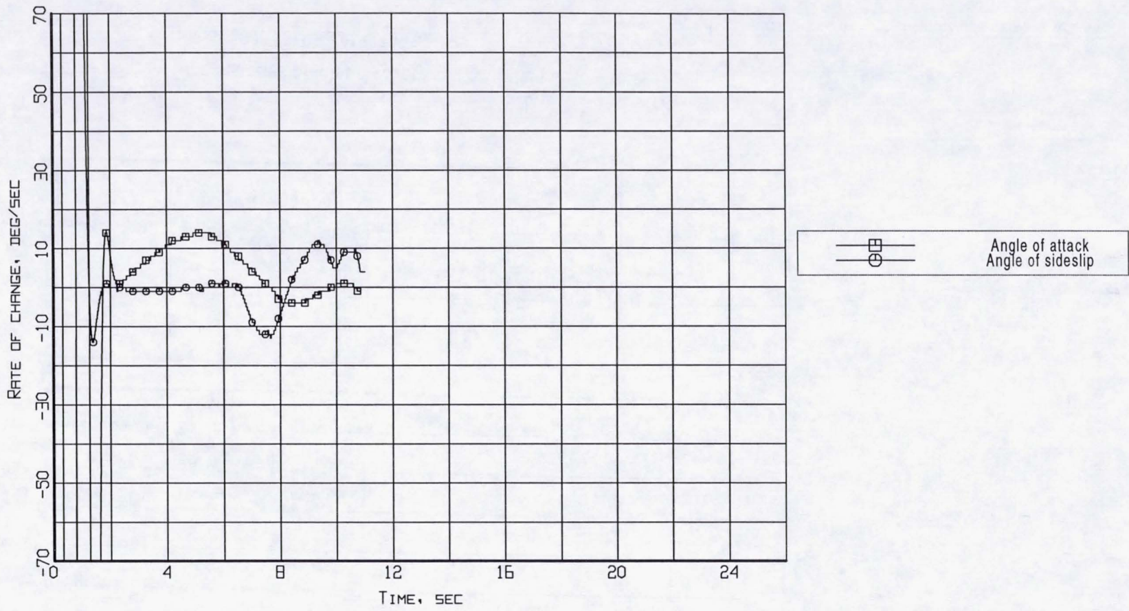
Figure B7-4. Aerodynamic flowstream descriptors - rate of change of angle of attack and angle of sideslip (Flight 238, Test Point 40b).
