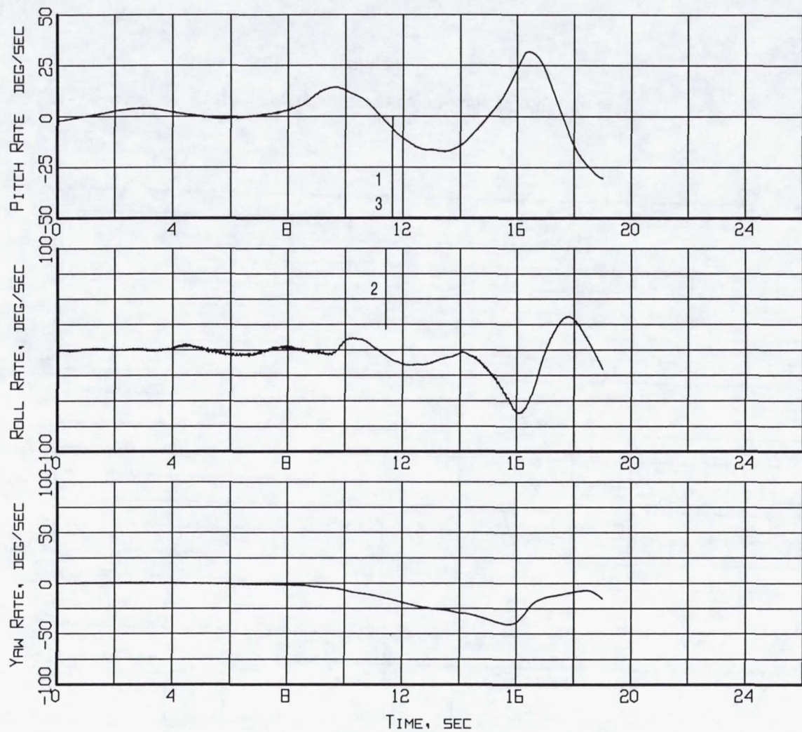
Figure B1-9. Event markers superposed on the aircraft motion time histories (Flight 239, Test Point 34b).
