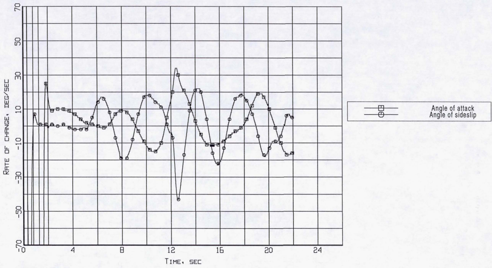
Figure B5-4. Aerodynamic flowstream descriptors - rate of change of angle of attack and angle of sideslip (Flight 238, Test Point 38b).
