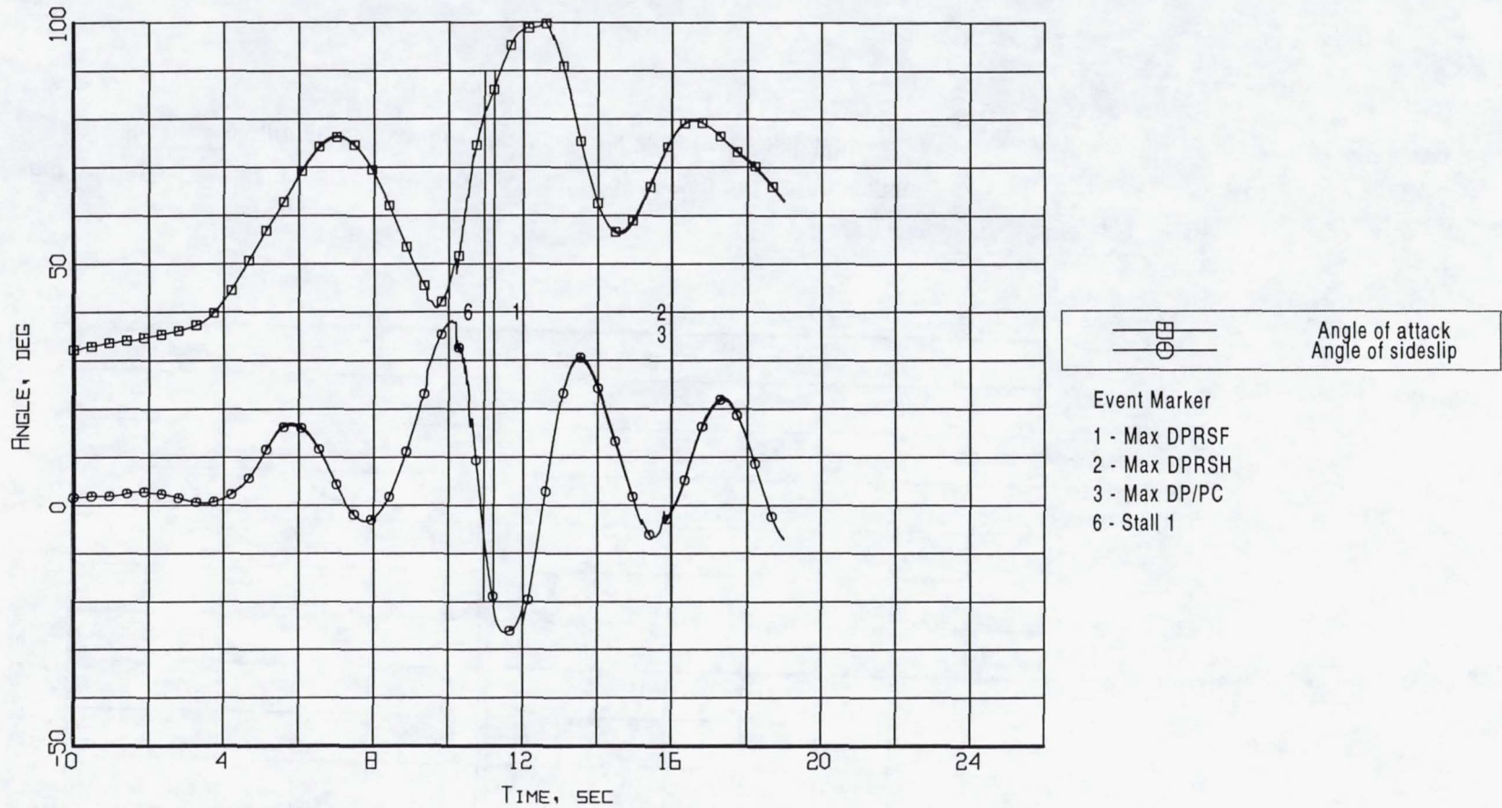
Figure B4-11. Event markers superposed on the aerodynamic flowstream descriptor time histories (Flight 239, Test Point 37b).
