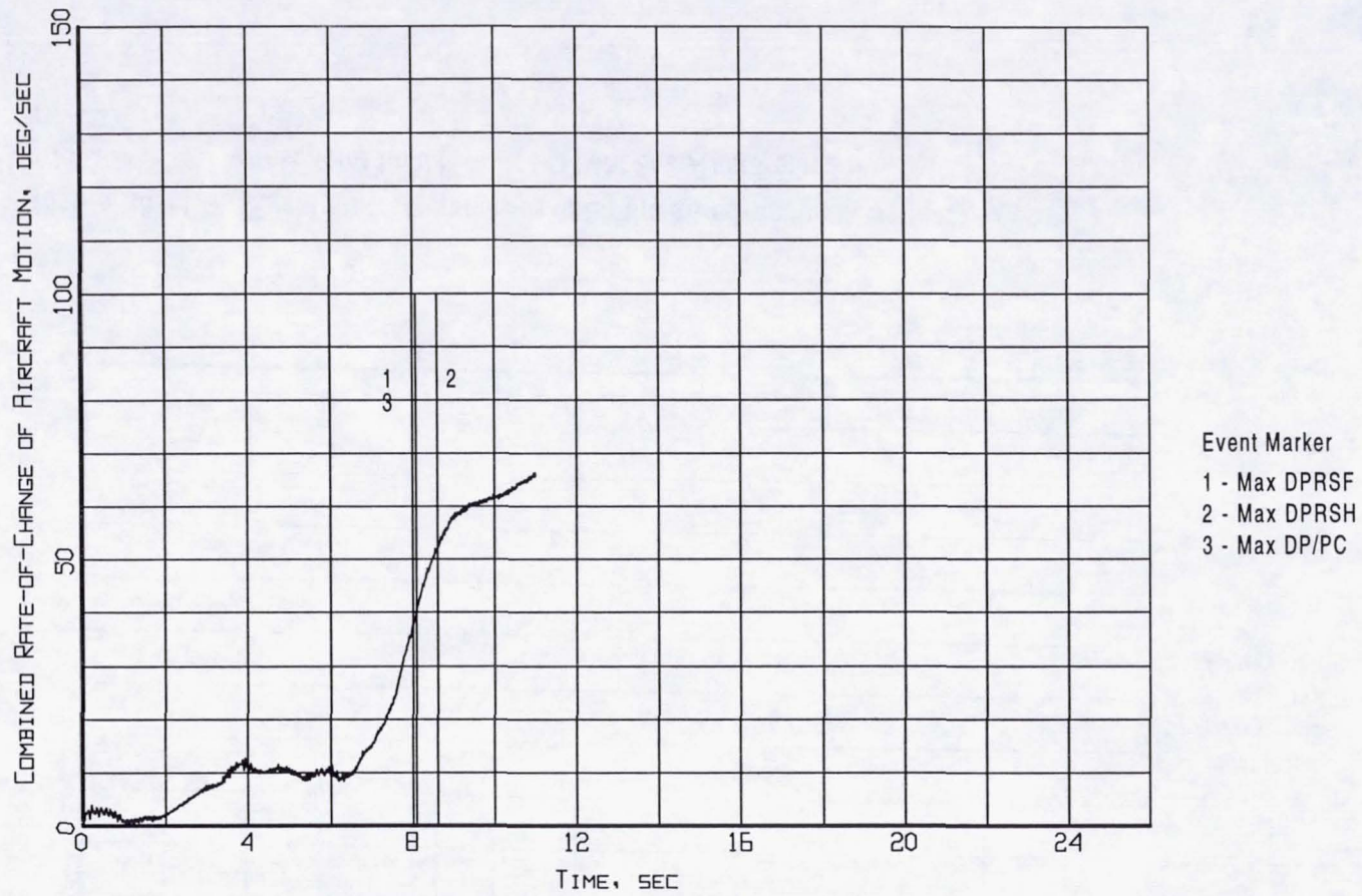
Figure B8-10. Event markers superposed on the combined of rate-of-change of aircraft motion time history (Flight 240, Test Point 41b).
