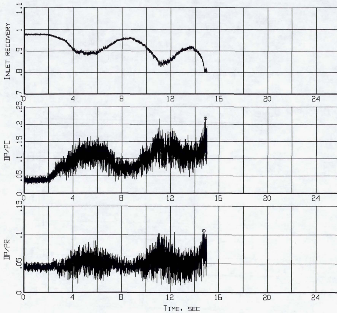
Figure B2-5. Time histories of inlet recovery and distortion descriptors (Flight 238, Test Point 35b).
