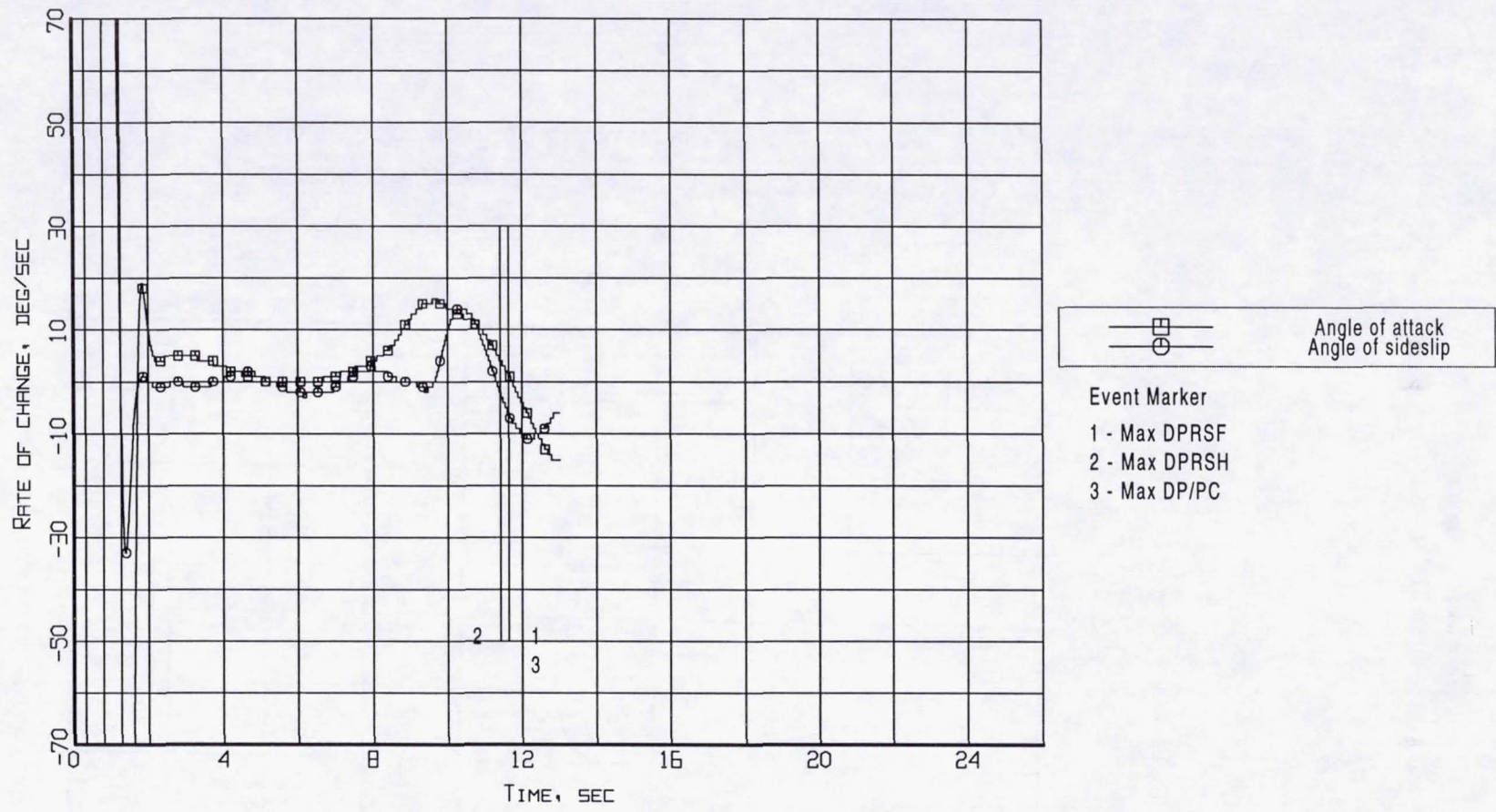
Figure B1-12. Event markers superposed on the aerodynamic flowstream descriptors rate-of-change time histories (Flight 239, Test Point 34b).
