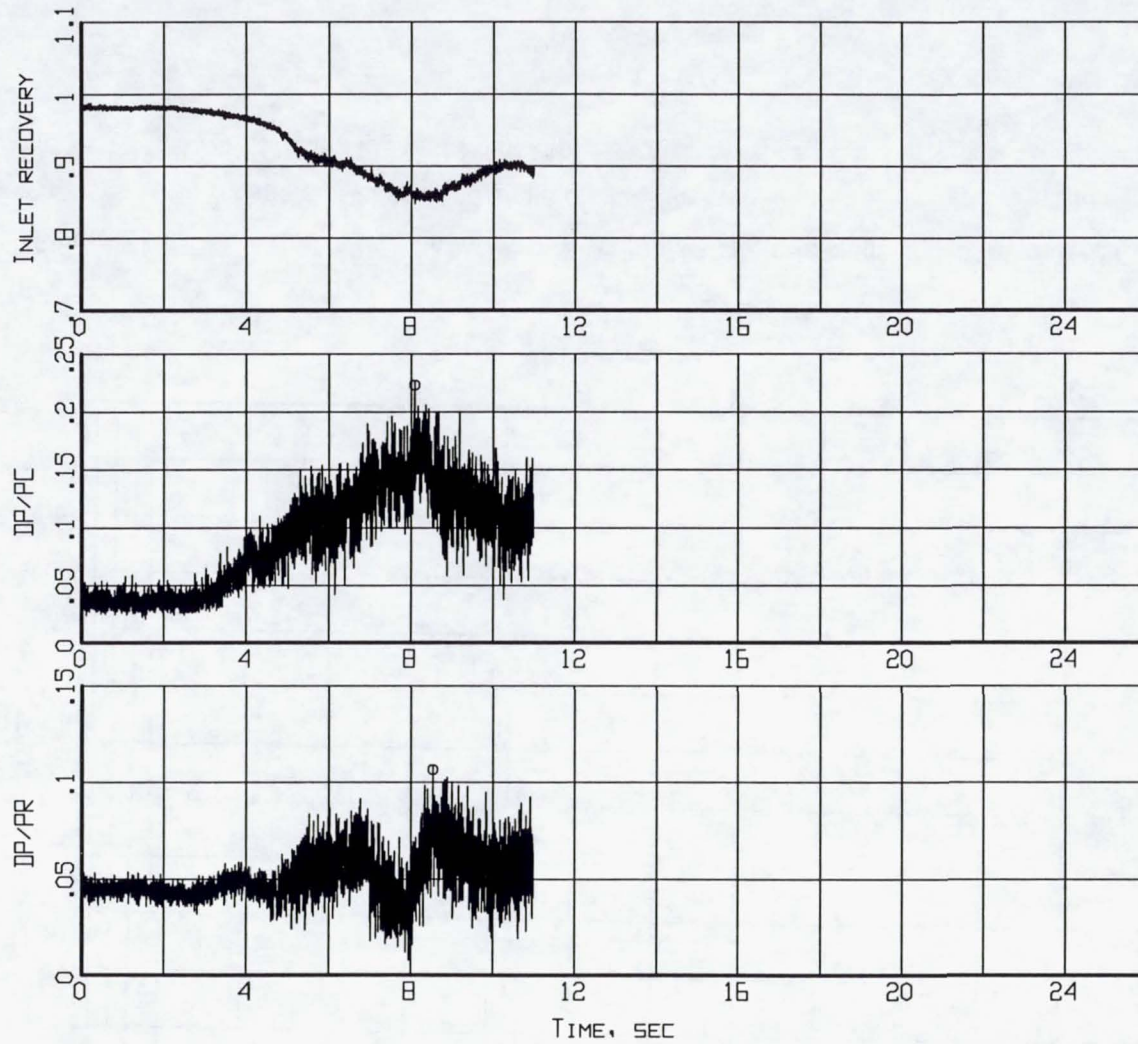
Figure B8-5. Time histories of inlet recovery and distortion descriptors (Flight 240, Test Point 41b).
