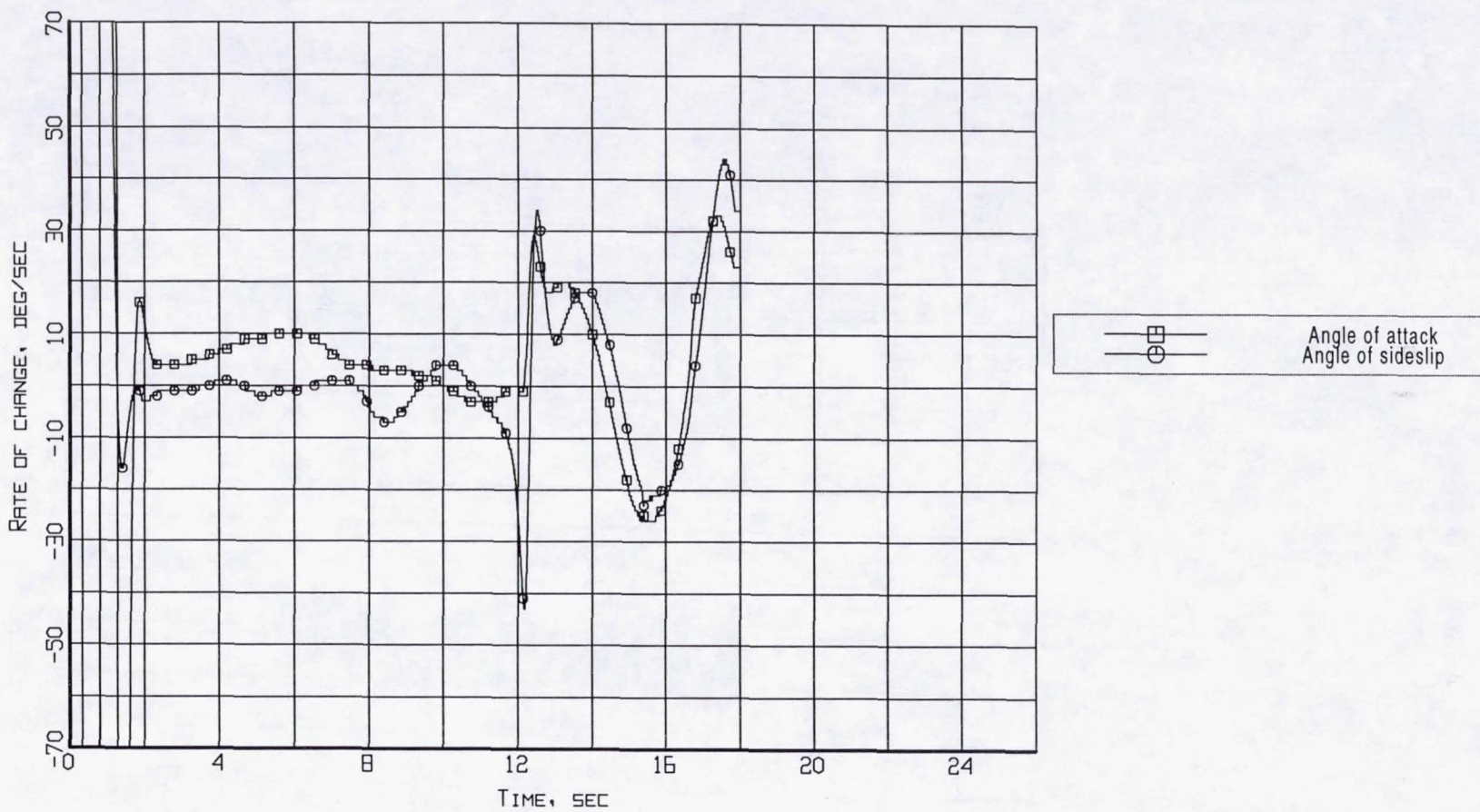
Figure B11-4. Aerodynamic flowstream descriptors - rate of change of angle of attack and angle of sideslip (Flight 238, Test Point 44b).
