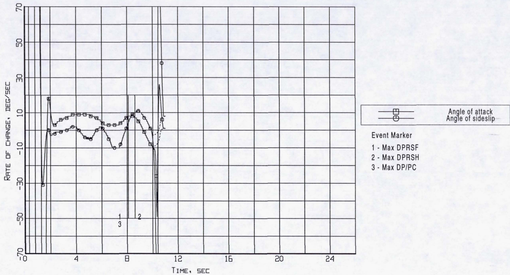
Figure B8-12. Event markers superposed on the aerodynamic flowstream descriptors rate-of-change time histories (Flight 240, Test Point 41b).
