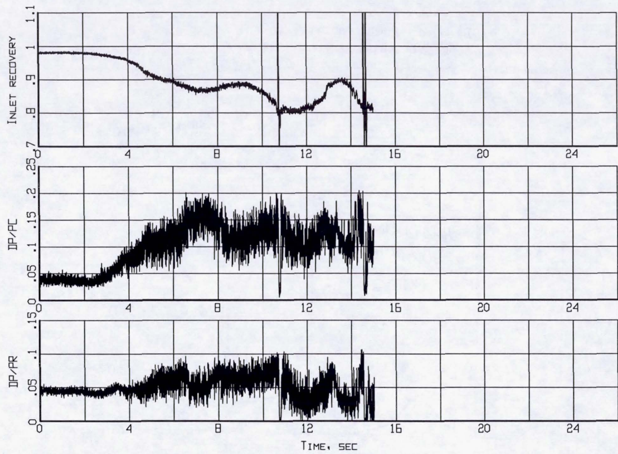
Figure 7. Time histories of inlet recovery and distortion descriptors (Flight 240, Test Point 45b).
