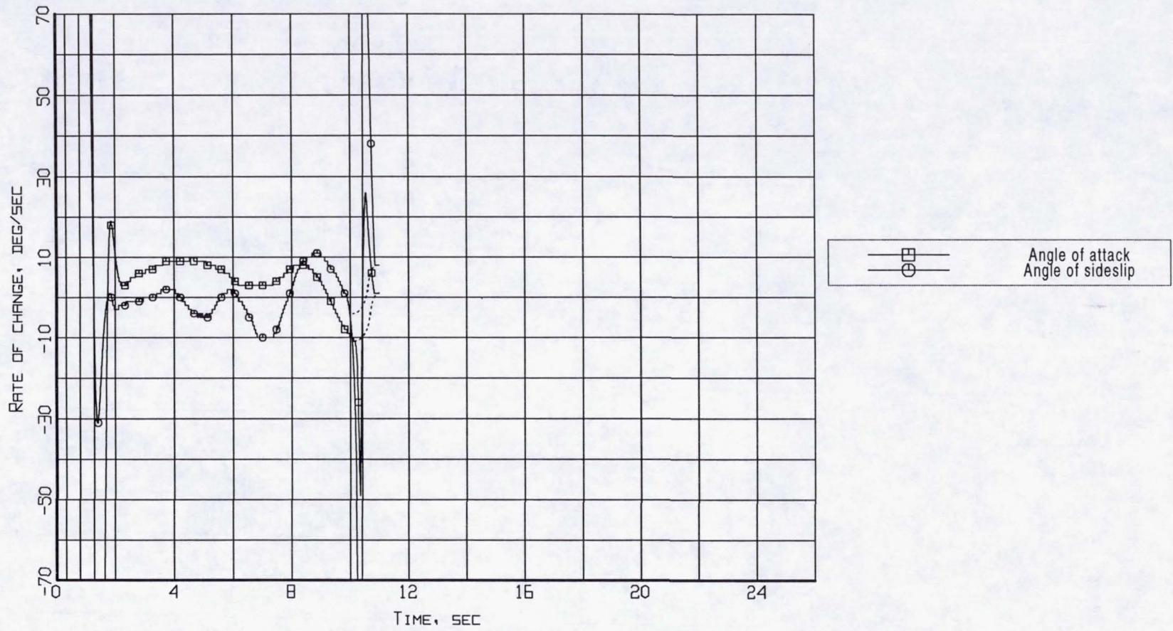
Figure B8-4. Aerodynamic flowstream descriptors - rate of change of angle of attack and angle of sideslip (Flight 240, Test Point 41b).
