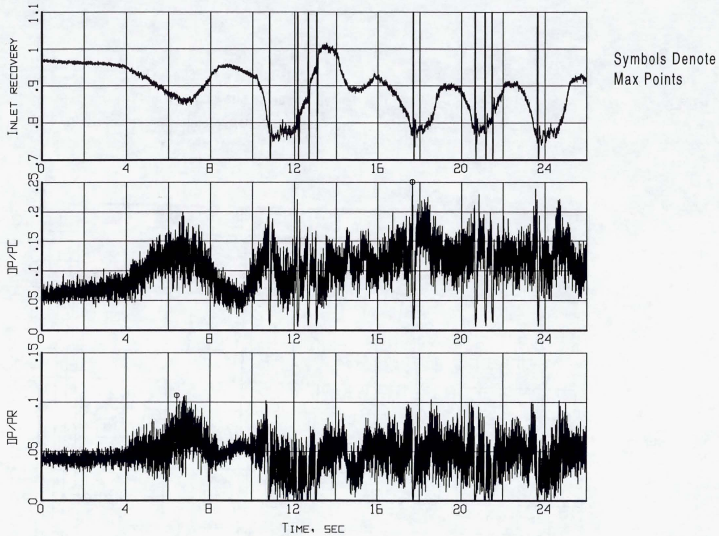
Figure B6-5. Time histories of inlet recovery and distortion descriptors (Flight 239, Test Point 39b).
