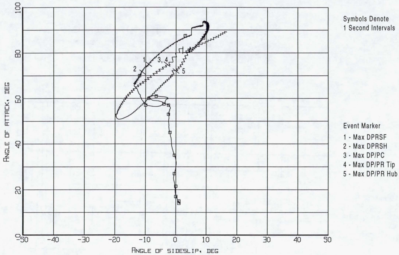
Figure B11-13. Event markers superposed on the aerodynamic flowstream descriptors trajectory (Flight 238, Test Point 44b).
