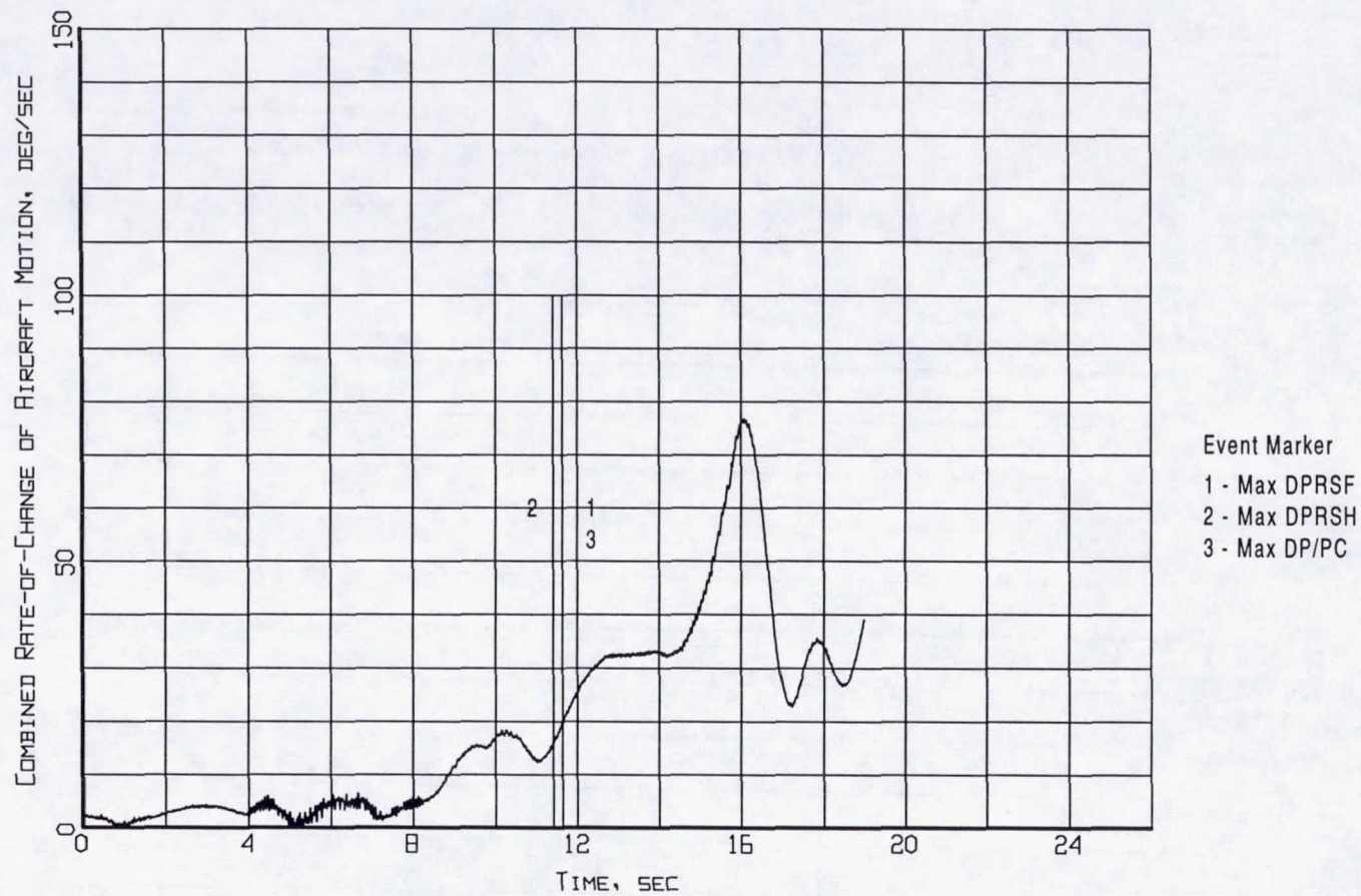
Figure B1-10. Event markers superposed on the combined of rate-of-change of aircraft motion time history (Flight 239, Test Point 34b).
