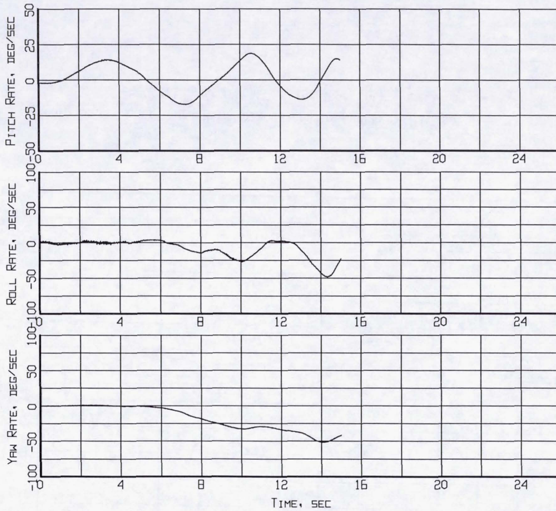
Figure B2-2. Aircraft Motion - Rate-of-Change of Pitch, Roll and Heading (Flight 238, Test Point 35b).
