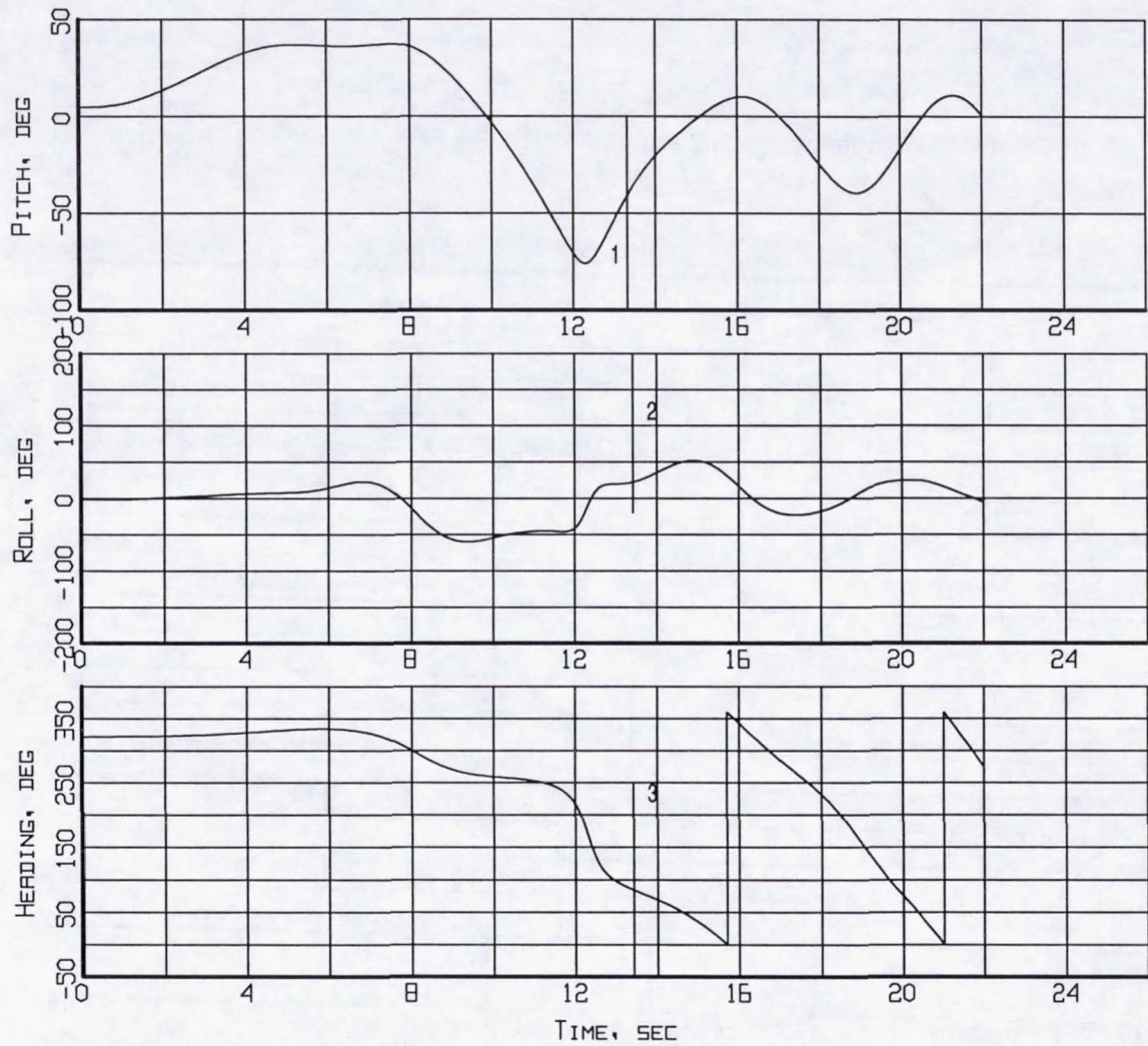
Figure B5-8. Event markers superposed on the aircraft attitude time histories (Flight 238, Test Point 38b).
