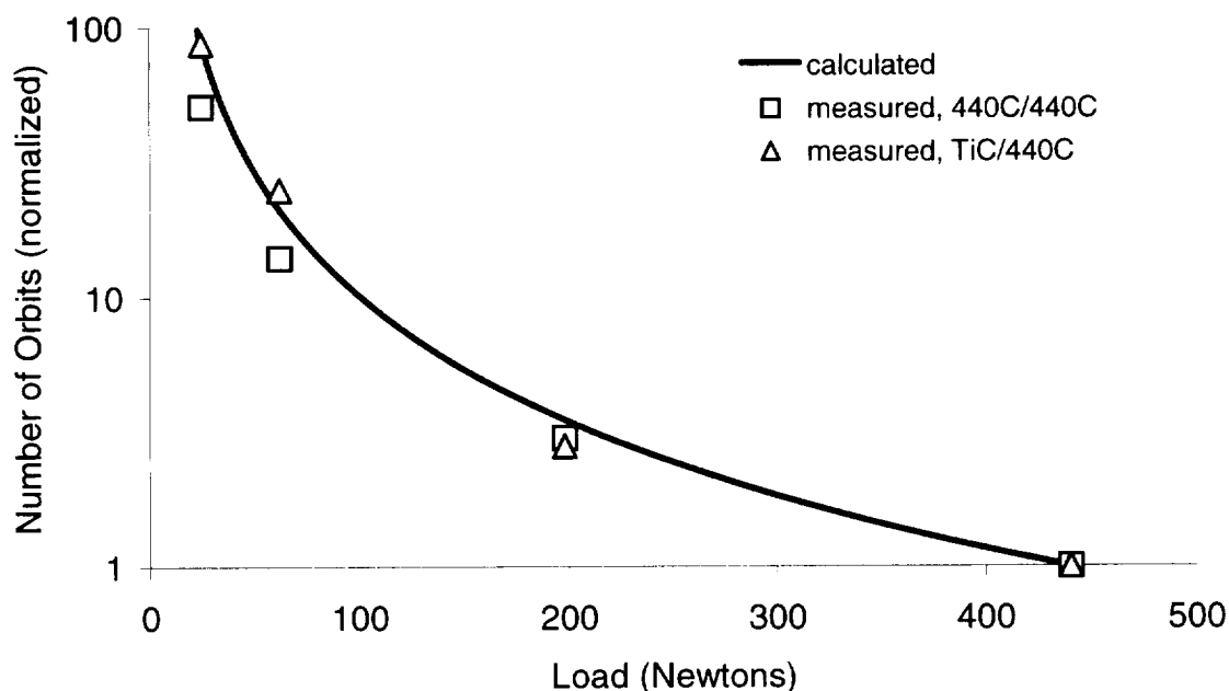
Figure 5. Relative lifetime of Krytox 143AC as a function of load in the BoP Tribometer
