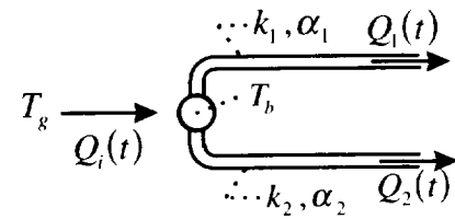
Figure 7-7-1.—Dynamic thermocouple.
