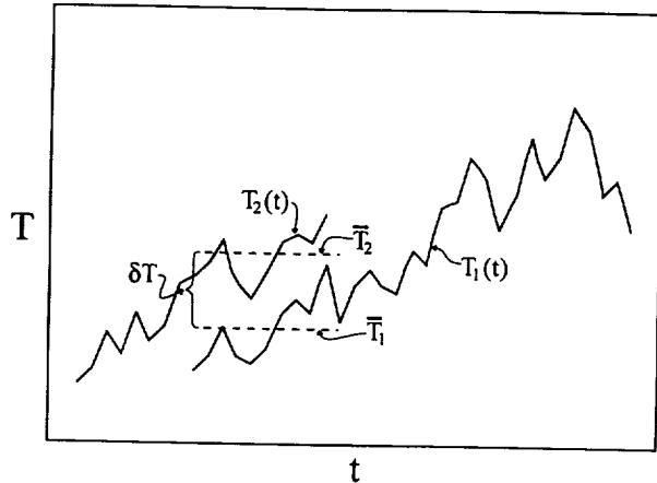
Figure 2. Illustration of how two temperature records are combined. The bias \delta T between the two records is the difference between their averages over the common period of data. The second record is shifted vertically by \delta T and T_1 and T_2 are then averaged.
