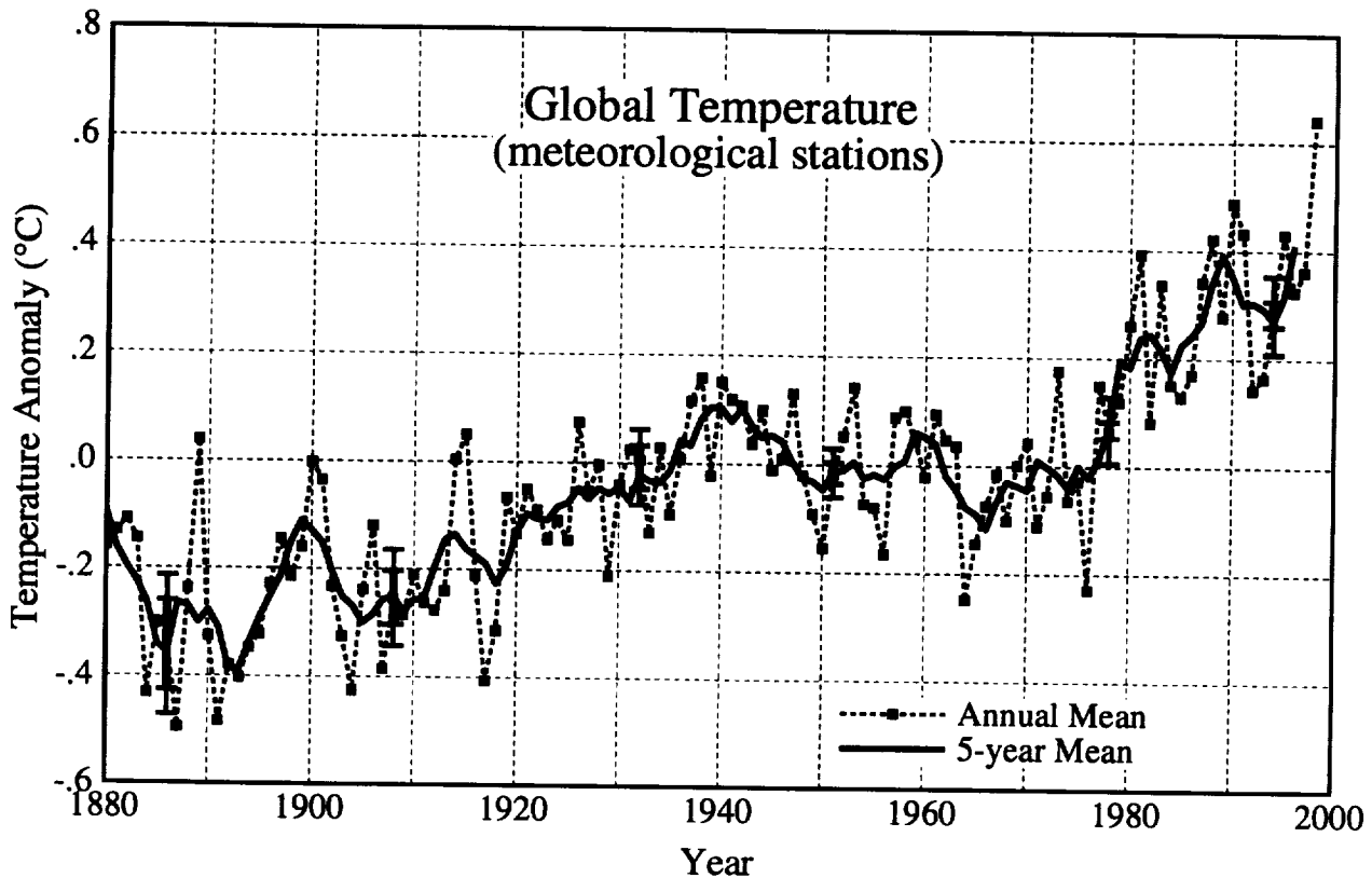
Figure 5. Global annual-mean surface air temperature change based on the meteorological station network. Uncertainty bars (95% confidence limits), shown for both the annual and 5-year means, are based on spatial sampling analysis of HL87.
