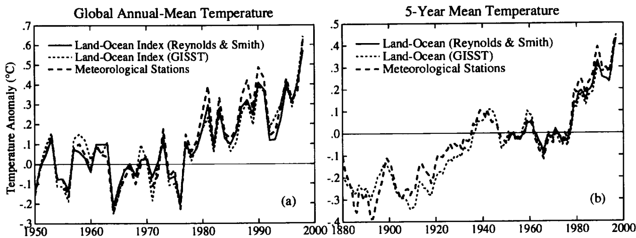
Figure 9. (a) Global annual-mean change of land-ocean temperature index with SSTs based on Reynolds and Smith (1994) compared with the (near) global surface air temperature anomaly based on the meteorological station network (Figure 5), (b) 5-year mean of this land-ocean temperature index, the same index with GISST (Parker et al., 1995; Rayner et al., 1996) used for the SST, and the near-global temperature change based on only land meteorological stations.
