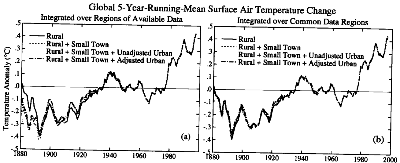
Figure 6. (a) Global 5-year-running-mean surface air temperature change based on rural, rural plus small town, all stations without any homogeneity adjustment, and all stations with the urban records adjusted as described in section 5. (b) same as (a), but with the region used to calculate global temperature restricted to the common area where the temperature is defined for all data sets.
