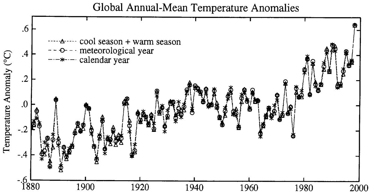
Figure 17. Annual mean temperature anomalies for cool season + warm season (Nov-Oct), meteorological year (Dec-Nov), and calendar year (Jan-Dec).
