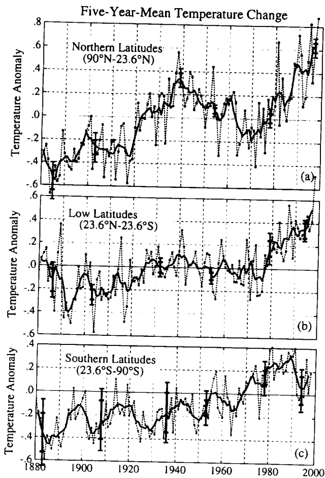
Figure 7. Five-year-running-mean temperature change for three latitude bands that cover 30%, 40% and 30% of the global area. Uncertainty bars (95% confidence limits) are based on spatial sampling analysis of HL87.
