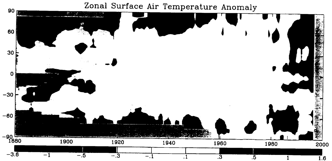
Figure 13. Five-year-running-mean of zonal surface temperature anomaly since 1880, based on surface air temperature measurements at meteorological stations. At each latitude the zero point of temperature is the 1951-1980 mean.
