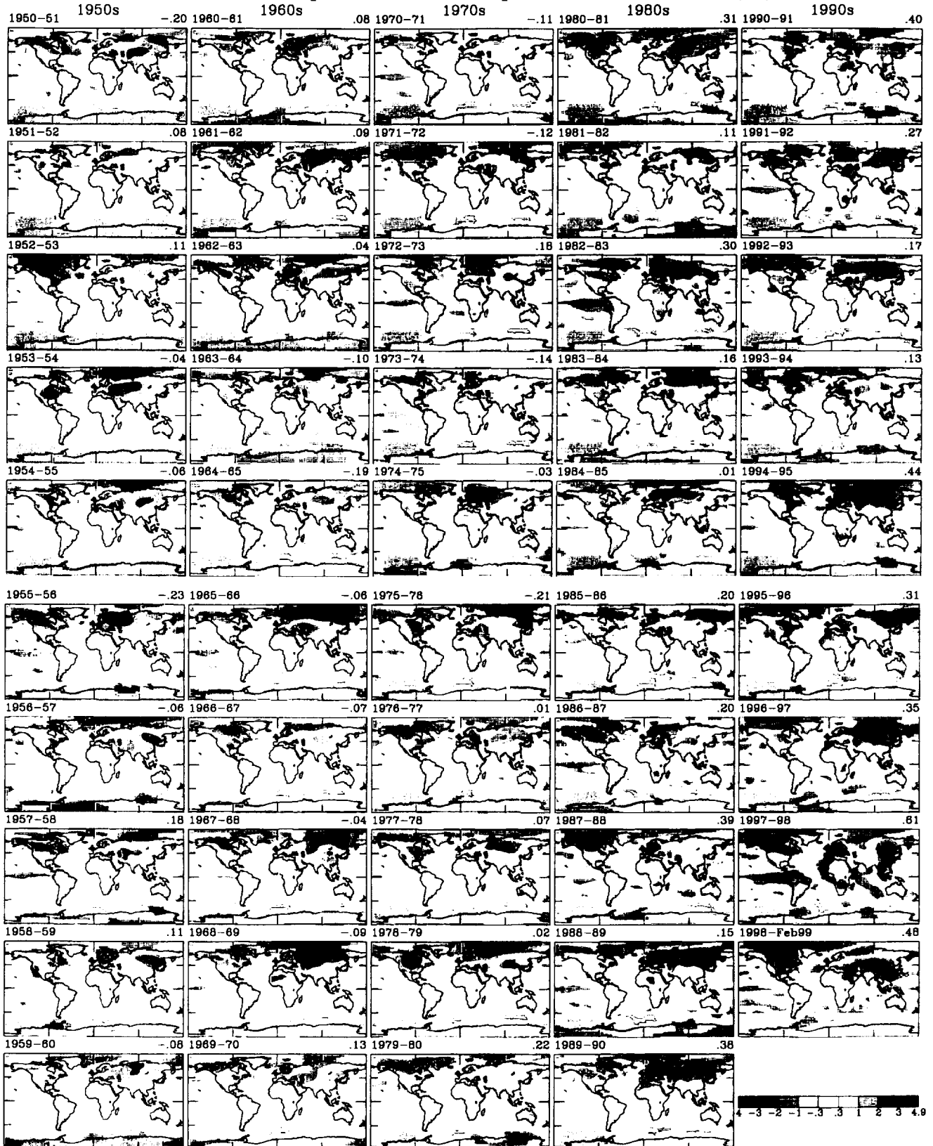
Figure 16a. Surface temperature anomalies for the (Northern Hemisphere) cool season for the past five decades.
