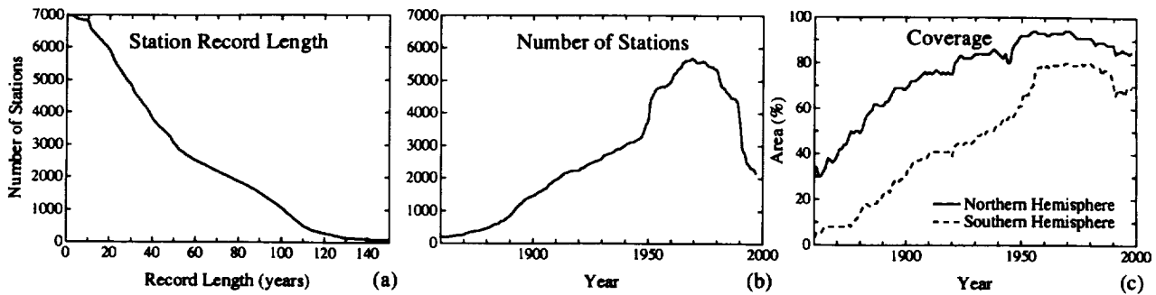
Figure 1. (a) Number of stations with record length n years or longer, (b) number of stations with defined annual temperature anomaly as a function of time, and (c) percent of hemispheric area located within 1200 km of a station.
