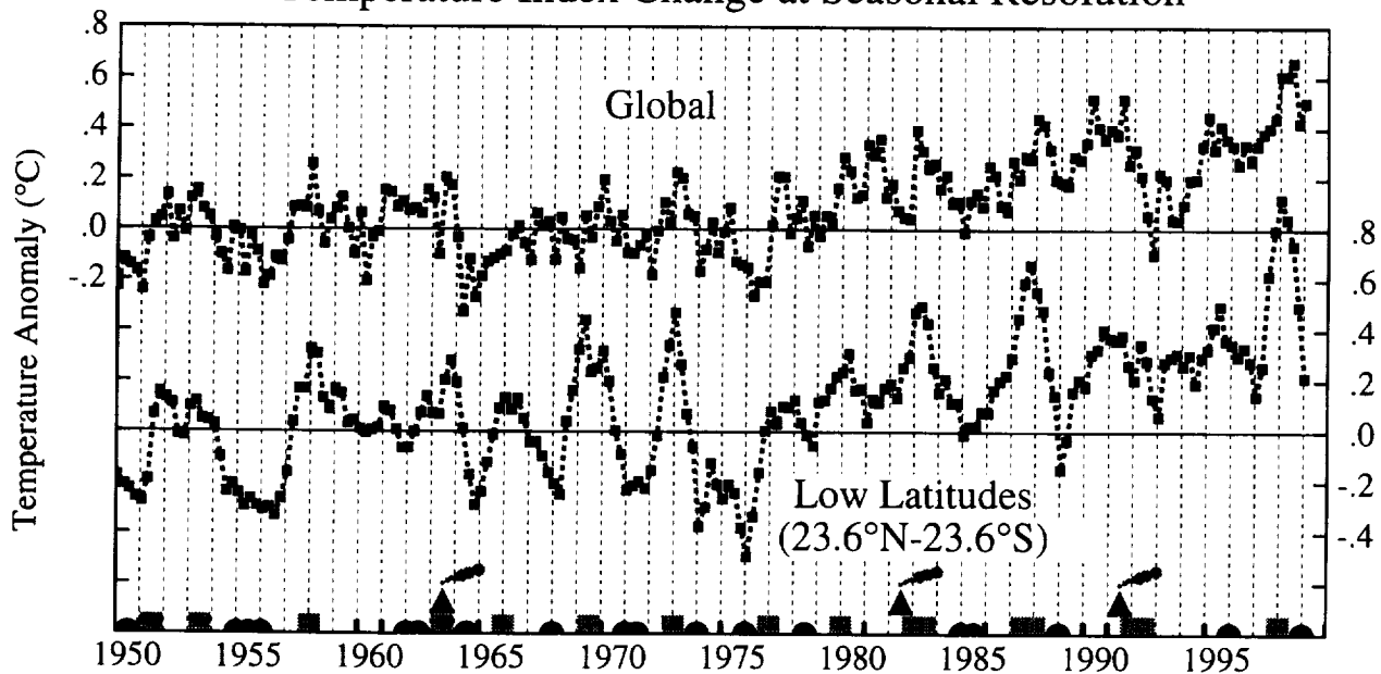
Figure 10. Temperature index change since 1950 at seasonal resolution, for the globe and for low latitudes. Semi-circles mark La Ninas, rectangles mark El Ninos, and triangles mark large volcanos.
