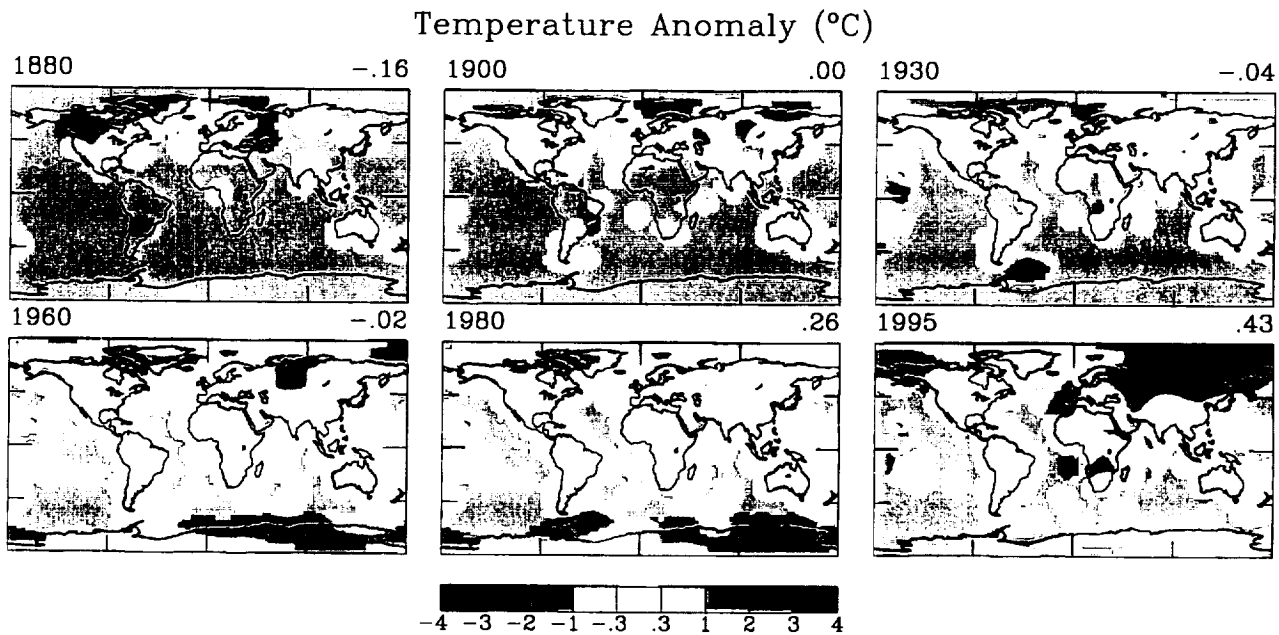
Figure 3. Temperature anomalies, relative to the base period 1951-1980, for six years that illustrate the change of station coverage with time (cf. Fig. 1c).
