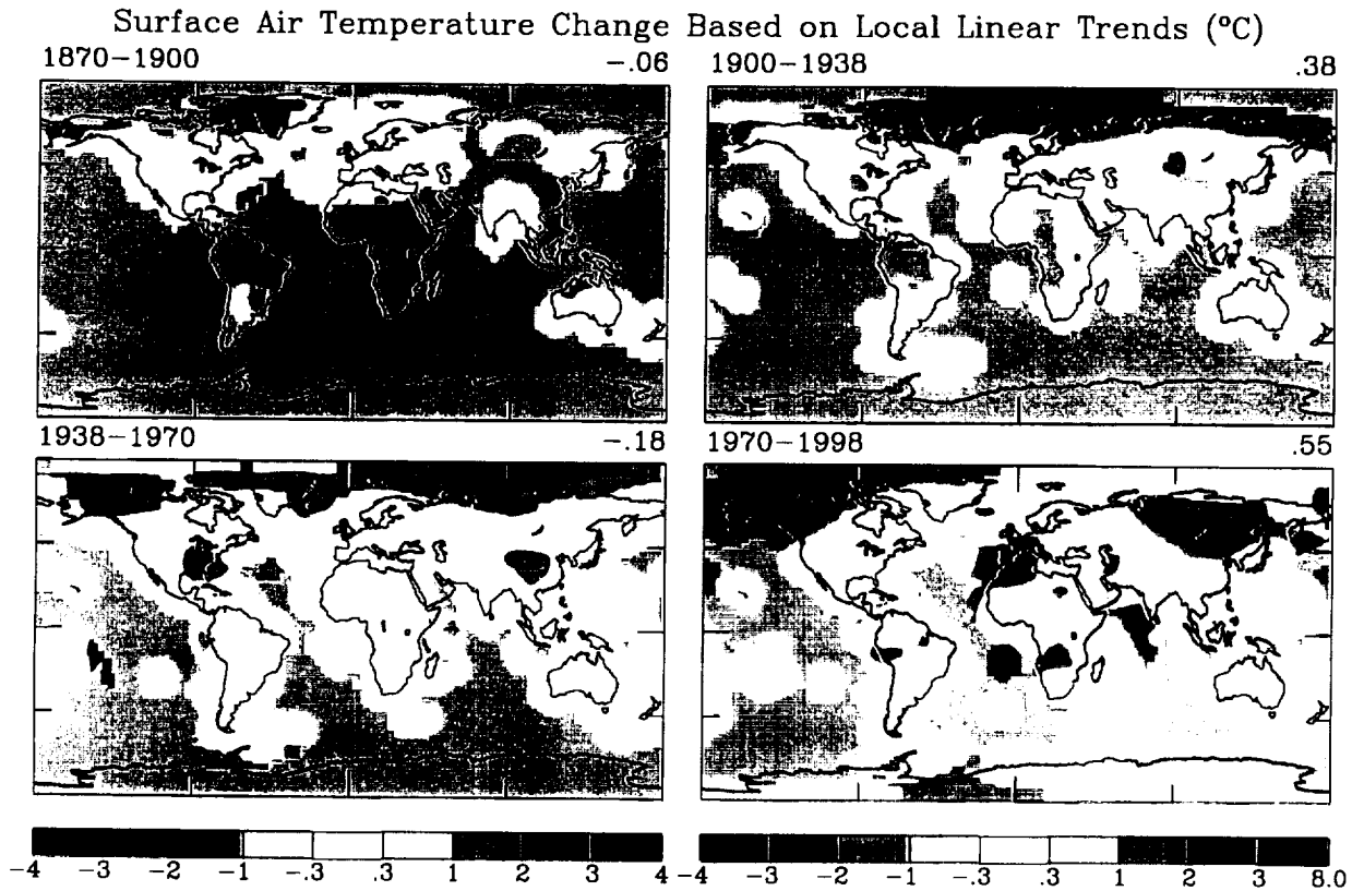
Figure 12. Surface air temperature change for the periods 1870-1900, 1900-1938, 1938-1970 and 1970-1998 based on local linear trends derived from only meteorological station data.
