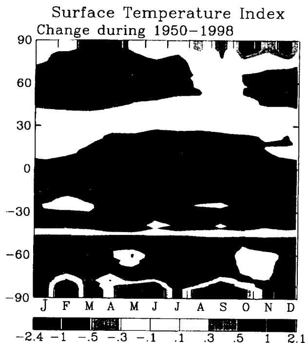
Figure 15. Zonal mean change of surface temperature index during 1950-1998 as a function of month.
