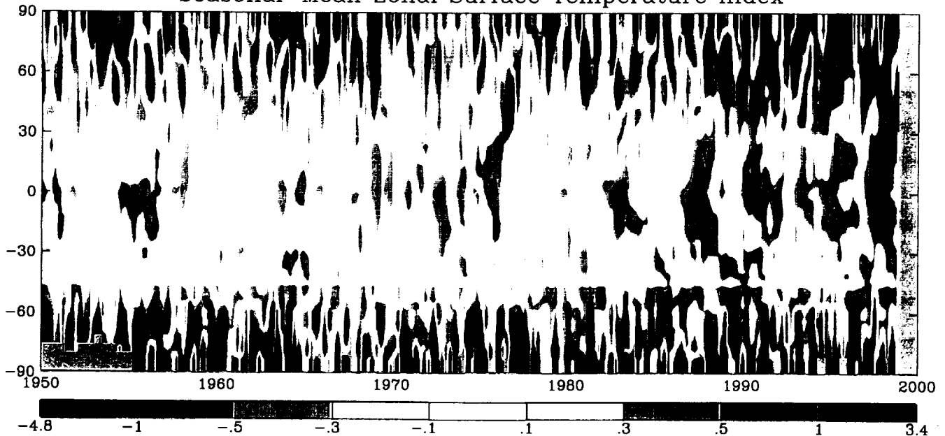
Figure 14. Seasonal-mean zonal surface temperature index since 1950, based on the land-ocean temperature index. At each latitude and season the zero point of temperature in the 1951-1980 mean.
