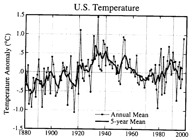
Figure 8. Annual-mean surface air temperature (meteorological year, December-November) for the contiguous 48 United States relative to the 1951-1980 mean.
