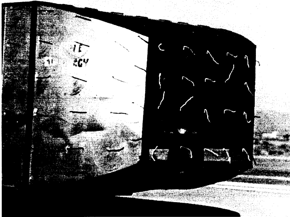
(a) Configuration H (truncated boattail). Conventional C_D = 0.242 .
