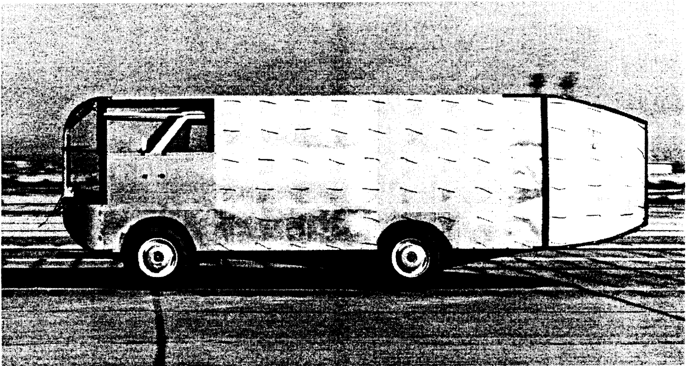
(b) Configuration H. Conventional C_D = 0.242 .
