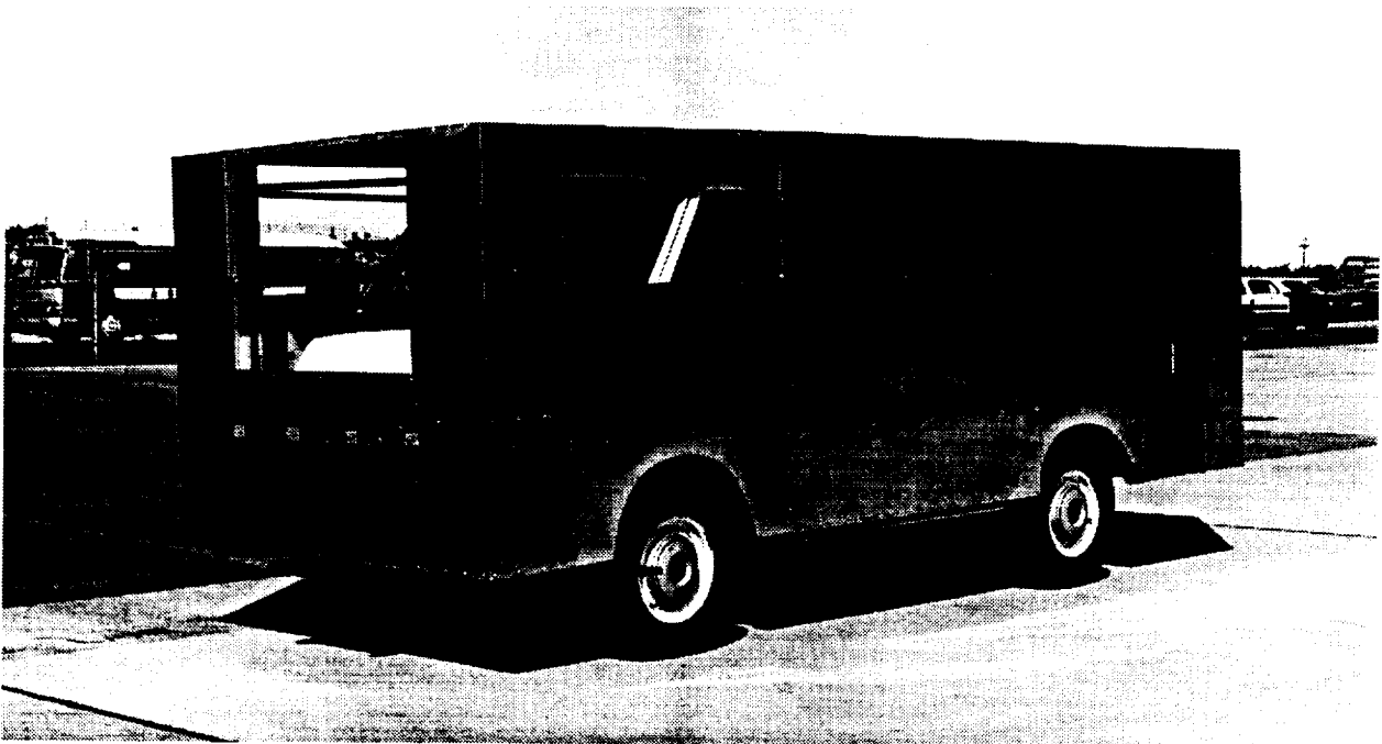
(b) Test van configuration A (all square corners).
