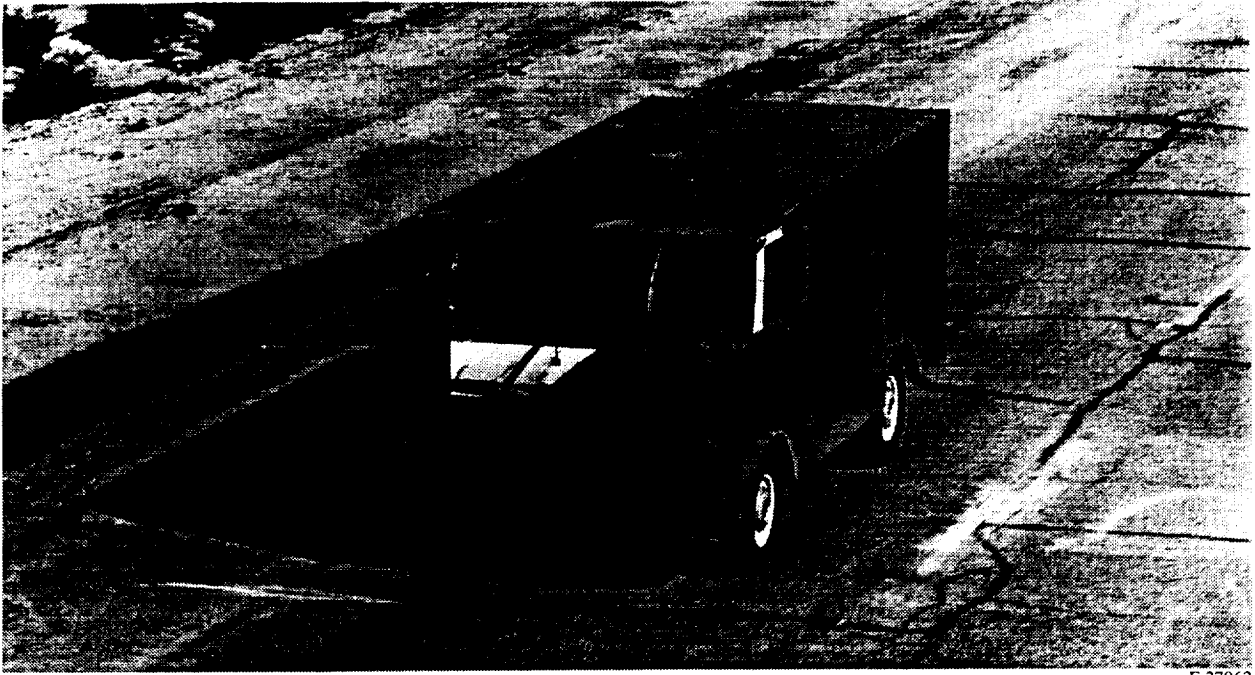
(c) View showing attached-flow tuft pattern on upper surface when front corners are rounded.
