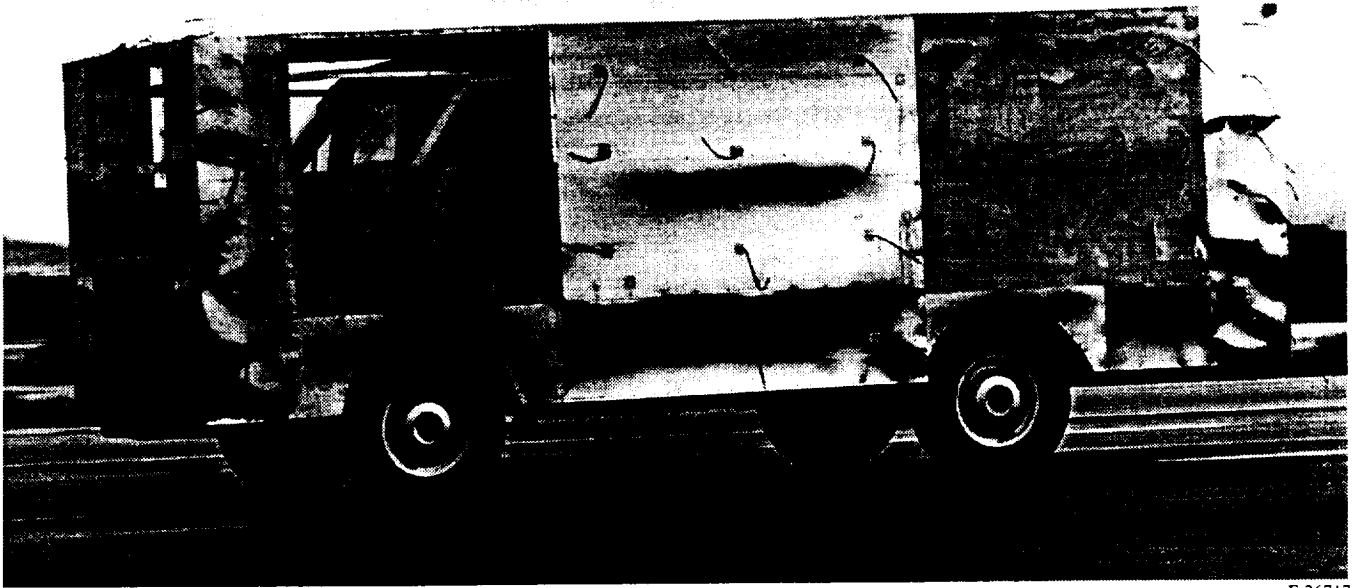
(a) Configuration A (baseline). Conventional C_D = 0.89 .
