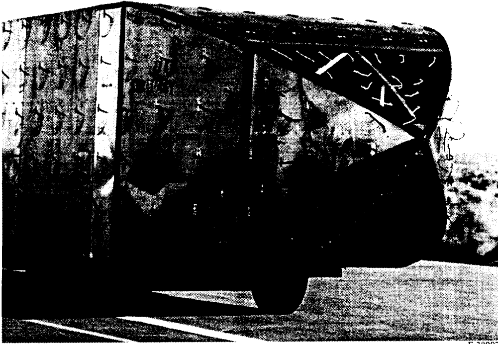
(b) Configuration G (full boattail). Conventional C_D = 0.238 .
