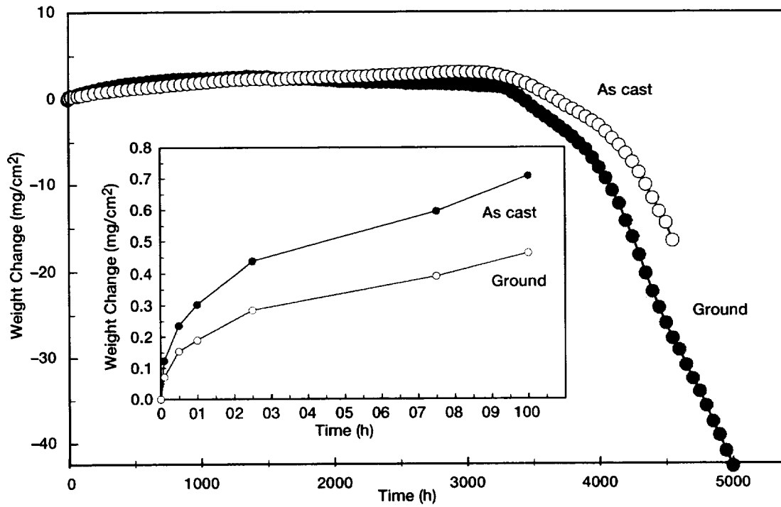
Figure 3.—Oxidation kinetics of In939 at 870 °C with 1 hr cycle.
