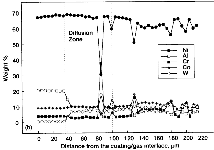
Figure 9.—Concentration profile of elements in VPA-coated Re108. (a) As-processed. (b) 9000 hr in Ar-5% H 2 .
