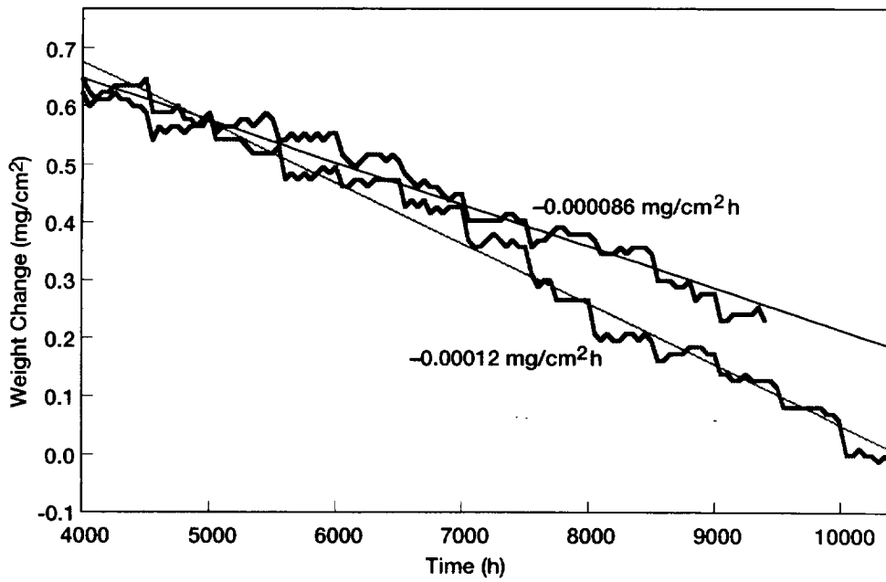
Figure 6.—Linear weight loss rate of VPA-coated Re108 at 980 °C with 1 hr cycle.
