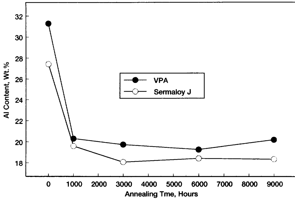
Figure 10.—Plot of Al concentration in the coating vs. the annealing time. (VPA: 980 °C, Sermaloy J: 870 °C)
