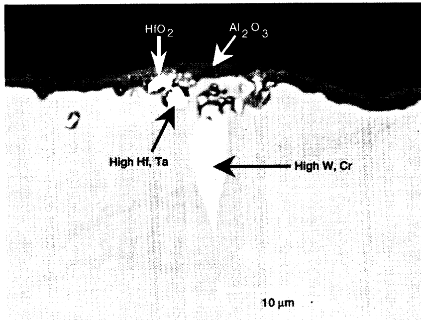
Figure 7.—Cross-section of VPA-coated Re108 after 1000 hr at 980 °C with 1 hr cycle. (a) Low magnification, showing the coating and the diffusion zone. (b) High magnification showing the oxide scale.
