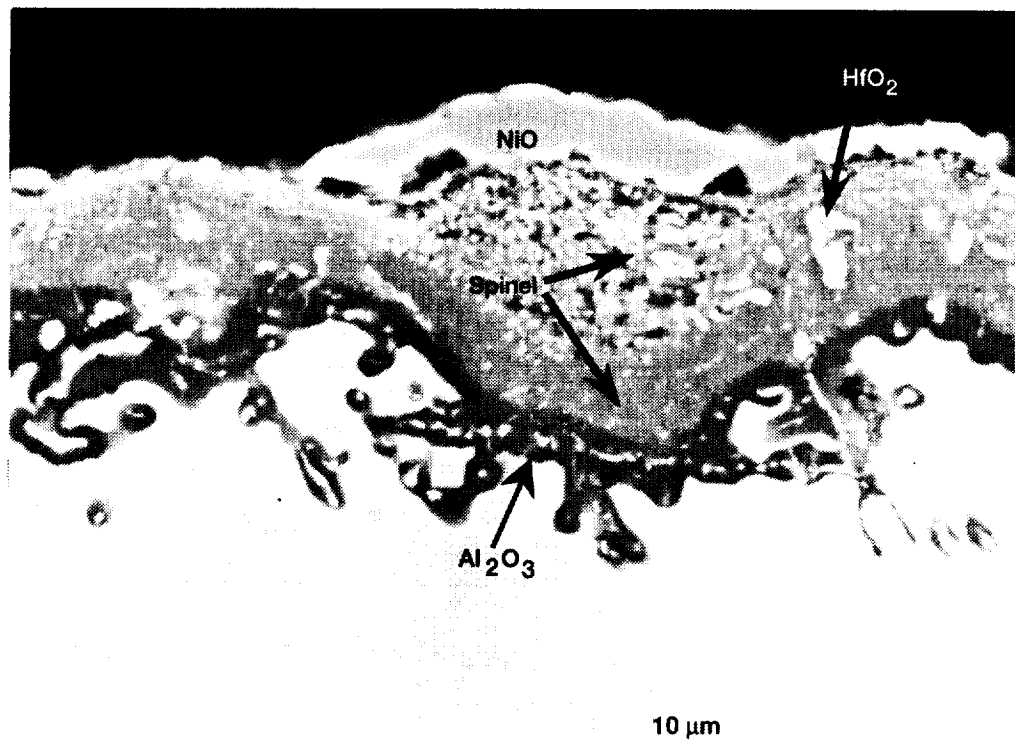
Figure 2.—Cross-section of Re 108 after 4500 hr at 980 °C with 1 hr cycle.
