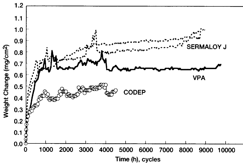
Figure 8.—Oxidation kinetics of coated In939 at 870 °C with 1 hr cycle.
