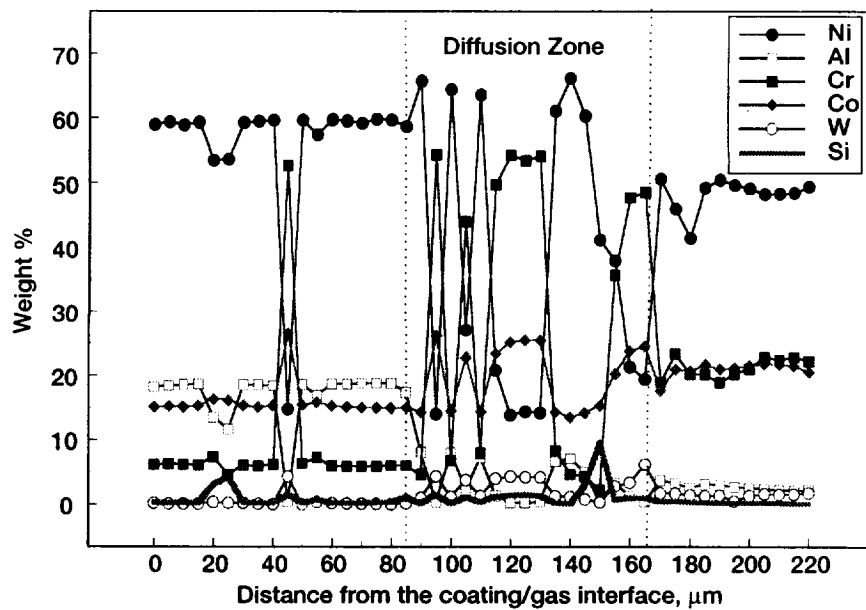
Figure 13.—Concentration profile of elements in SERMALOY J-coated In939. (a) As-processed. (b) 9000 hr in Ar-5% H 2 .
