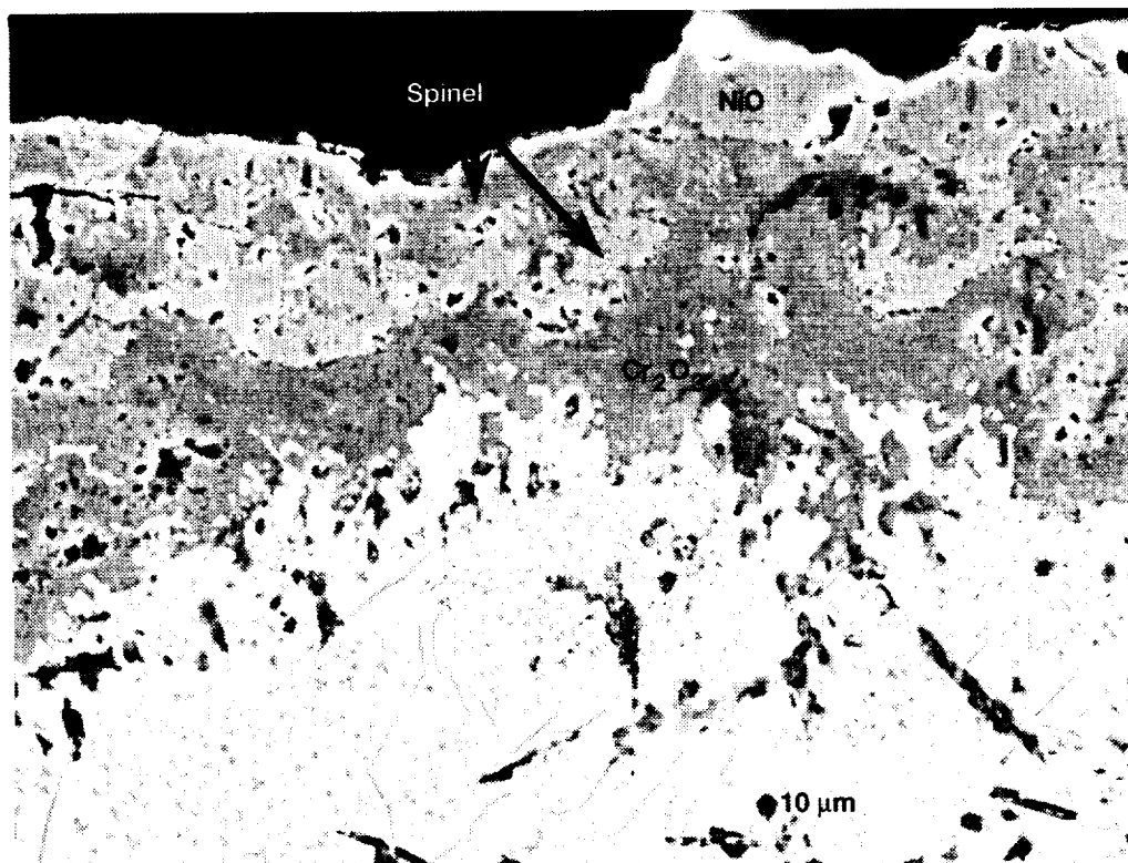
Figure 4.—Cross-section of In939 after 4500 hr at 870 °C with 1 hr cycle.
