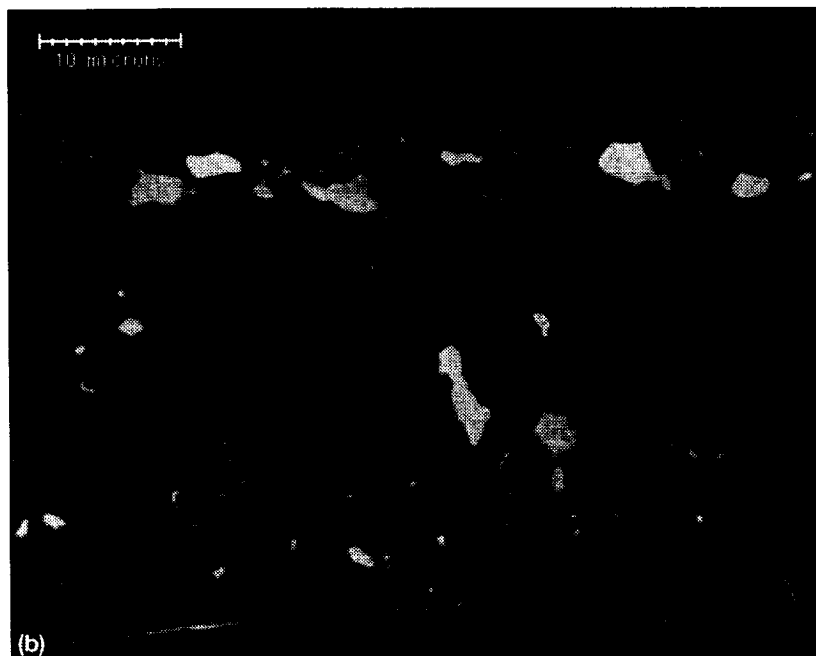
Figure 12.—Cross-section of VPA-coated Re108 after 9000 hr in Ar-5% H 2 at 980 °C. (a) Low magnification, showing the coating and the diffusion zone. (b) High magnification, showing the diffusion zone.
