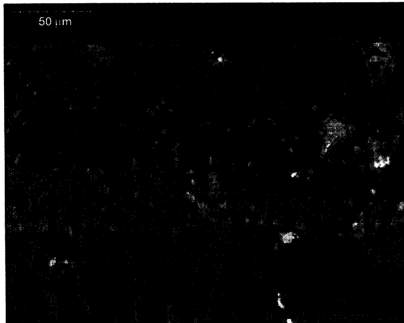
Figure 15.—Cross-section of SERMALOY J-coated In939 after 9000 hr in Ar-5% H 2 at 870 °C.
