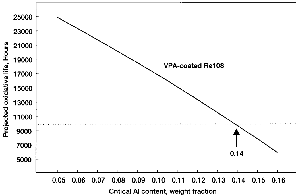
Figure 16.—Plot of oxidative life vs. critical Al content for VPA-coated Re108 at 980 °C with 1 hr cycle.
