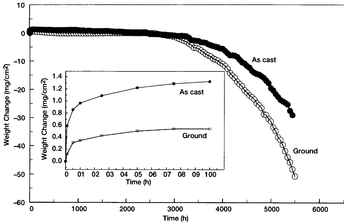
Figure 1.—Oxidation kinetics of Re108 at 980 °C with 1 hr cycle.
