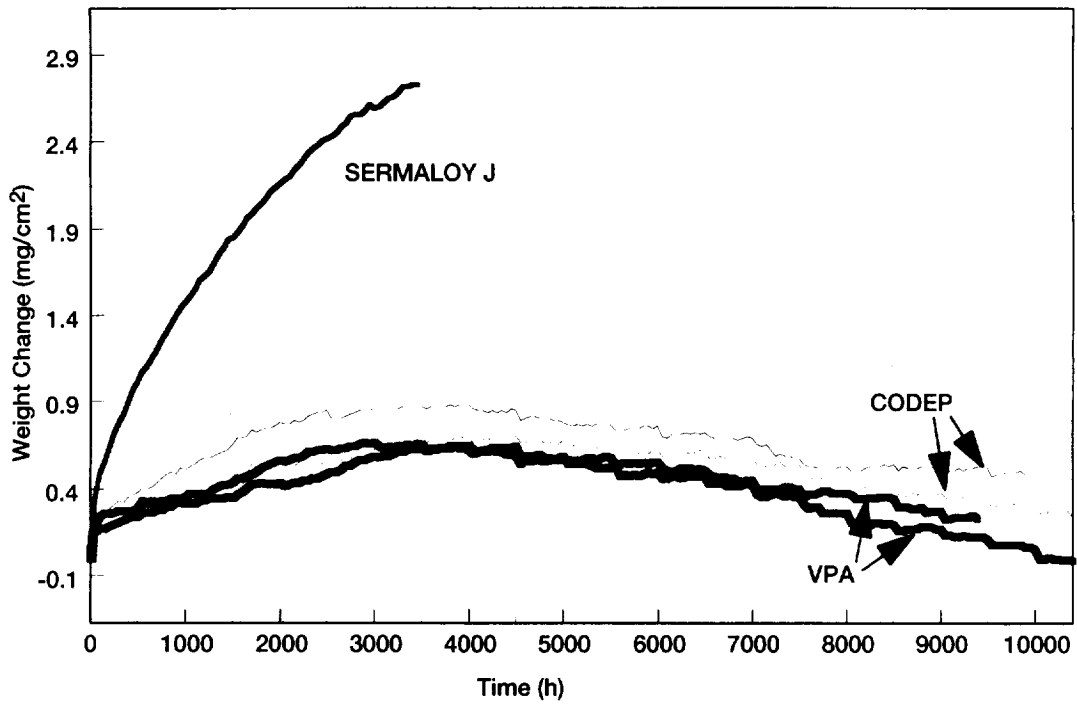
Figure 5.—Oxidation kinetics of coated Re108 at 980 °C with 1 hr cycle.
