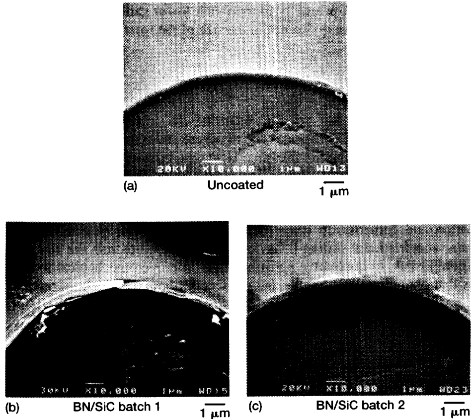
Figure 5: SEM micrographs showing interface failure during fiber push-in for celsian matrix composites reinforced with Hi-Nicalon fibers (a) uncoated, (b) BN/SiC batch 1, and (c) BN/SiC batch 2 coatings
