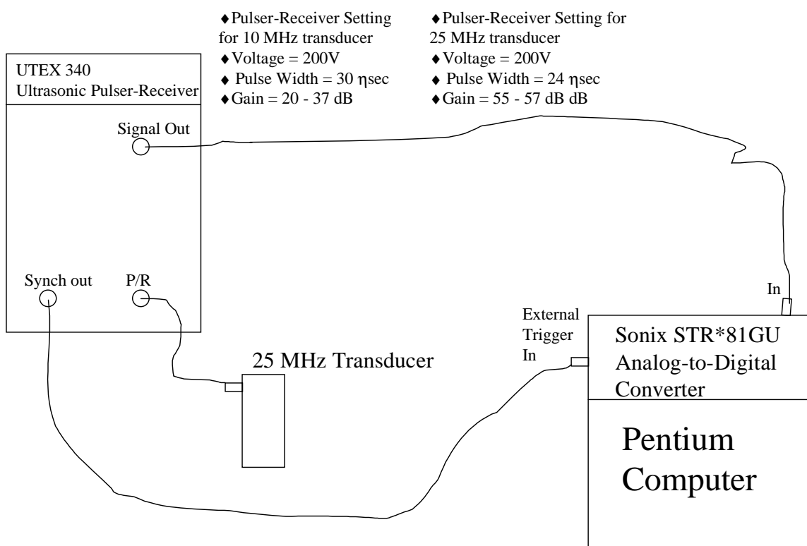
Figure 8. Instrumentation set-up.
