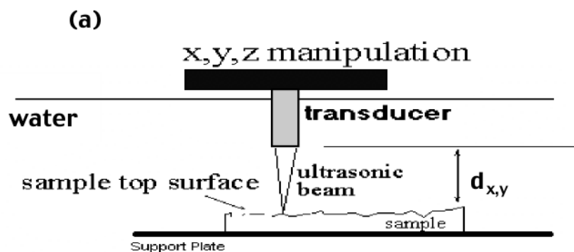
Figure 1.—Experimental set-up for ultrasonic surface profilometry (a) schematic of basic principle and set-up for samples.
