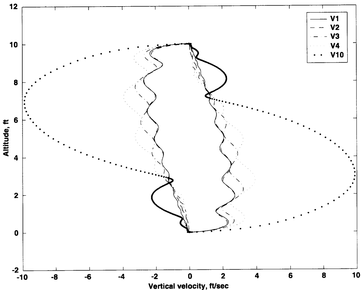
Figure B5. Predicted phase-plane responses.
