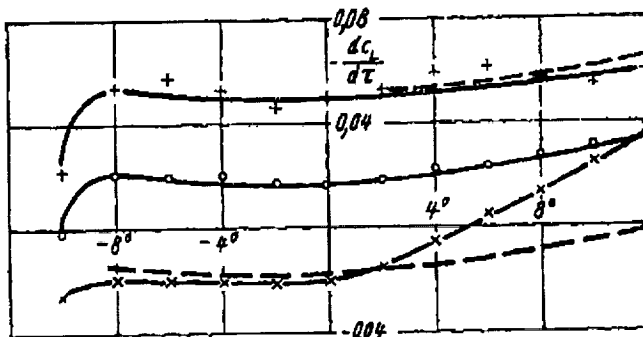
Figure 17.- Rolling moment in yaw under fuselage effect. (Tests from NACA-T.N. 730) + High wing arrangement o Mid wing arrangement x Low wing arrangement --- Theoretical values for high- and low-wing arrangement.
