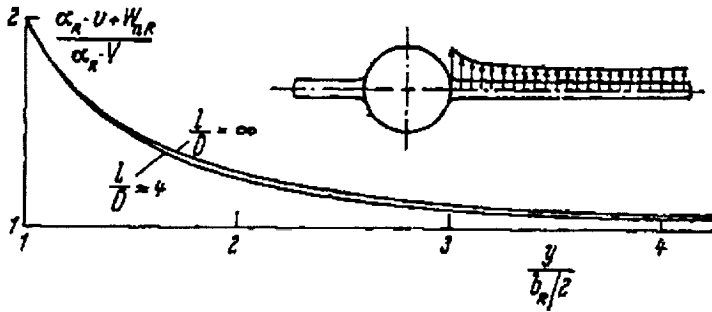
Figure 9.- Transverse flow about axially symmetrical fuselage ( l/D = 4 ) and about circular cylinder ( l/D = \infty ).
