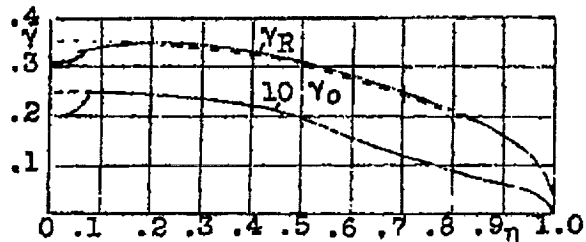
Figure 15.- Lift distribution of low-wing arrangement.
