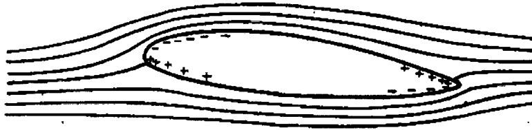
Figure 1.- Fuselage in ideal flow. + Positive pressure - Negative pressure
