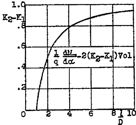
Figure 2.- Munk's correction factors for the unstable moments of surfaces of revolution.
