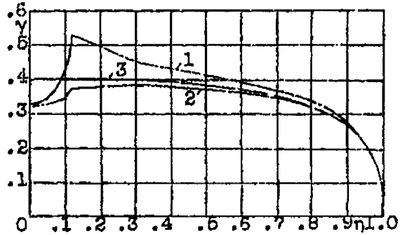
Figure 14.- Lift distribution of a mid-wing arrangement with circular fuselage and rectangular wing, \Lambda = 6 . Dimensions correspond to the conditions in NACA Report 540.
