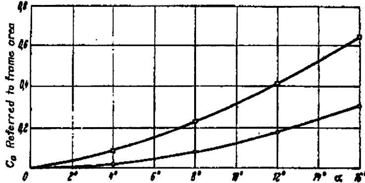
Figure 3.- Lift of the fuselage alone. o Normal } NACA-Report 540 □ Rectangular }
