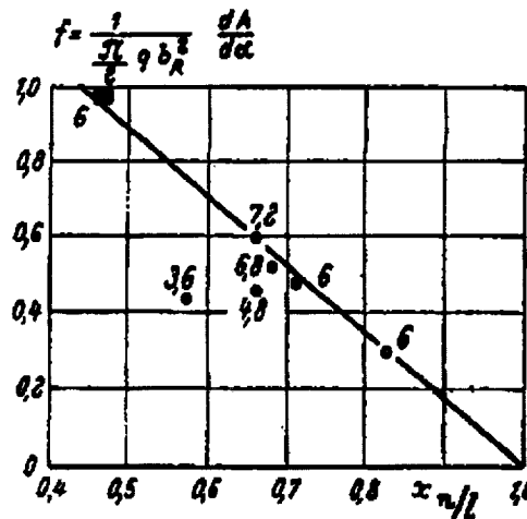
Figure 5 - Neutral stability point of frictional lift. Inscripted numbers indicate slenderness ratio.
