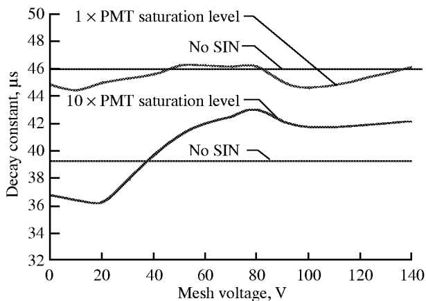
Figure 25. Effect of mesh potential on decay constant of combined simulated lidar return and SIN signal for two different PMT saturation levels.
