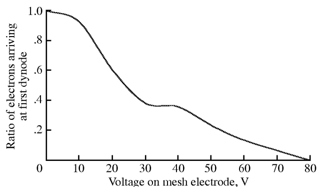
Figure 10. Effect of electrode mesh on SIN in SIMION simulation.
