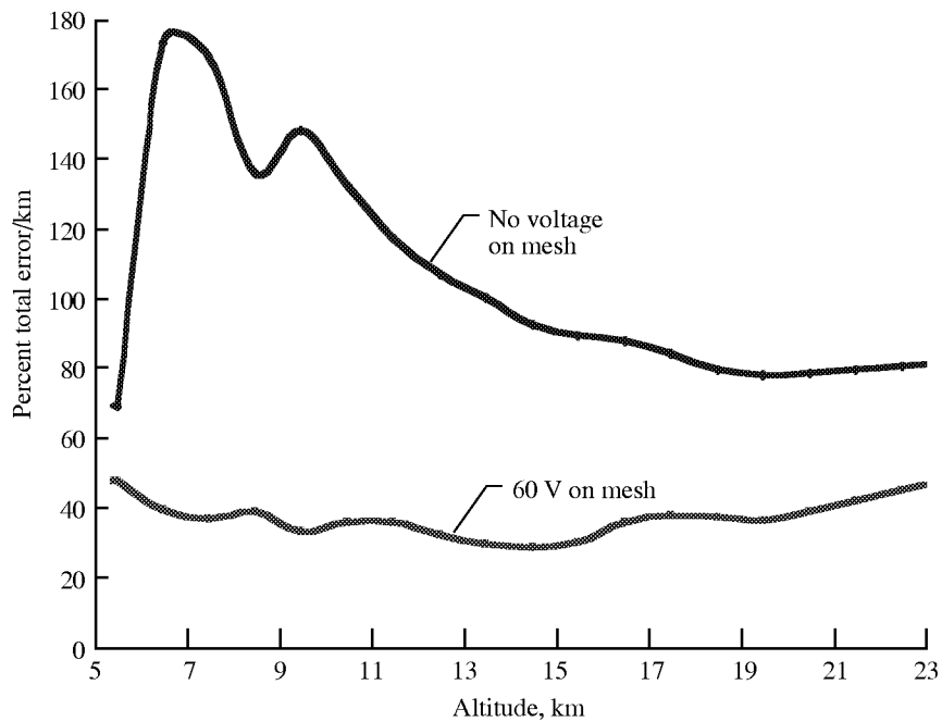
Figure 27. Effect of mesh voltage on actual lidar return signal for tropospheric measurements.
