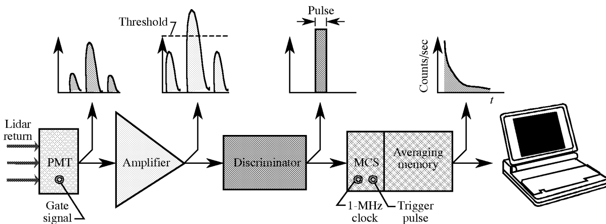
Figure 7. Photon-counting schematic.
