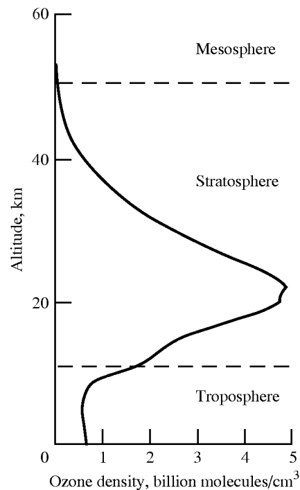
Figure 1. Distribution of ozone in atmosphere as function of altitude. (From ref. 3.)
