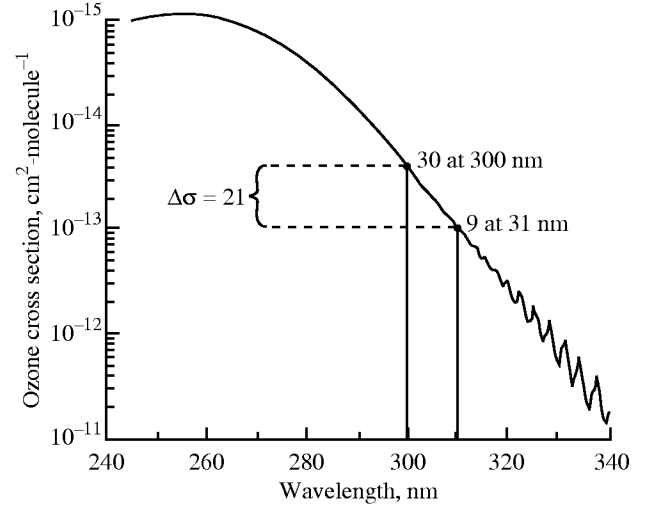
Figure 5. Ozone absorption cross section versus wavelength. (Data from ref. 20.)
