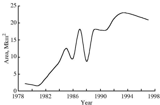
Figure 3. Changes in size of ozone hole over Antarctic between 1979 and 1997 (September 9–October 10).
