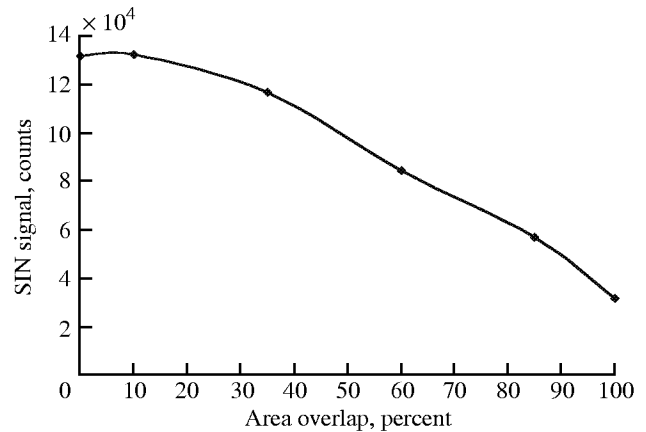
Figure 23. Effect of area overlap between mesh electrode pulse and saturating LED 1 pulse on signal-induced noise.
