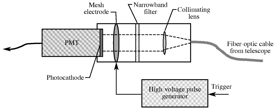
Figure 17. Path of lidar return from receiver system to photon-counting setup.
