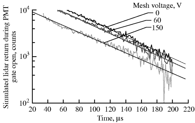
Figure 24. LED 2 simulated lidar return signals during PMT gate open time with variable mesh electrode voltage.
