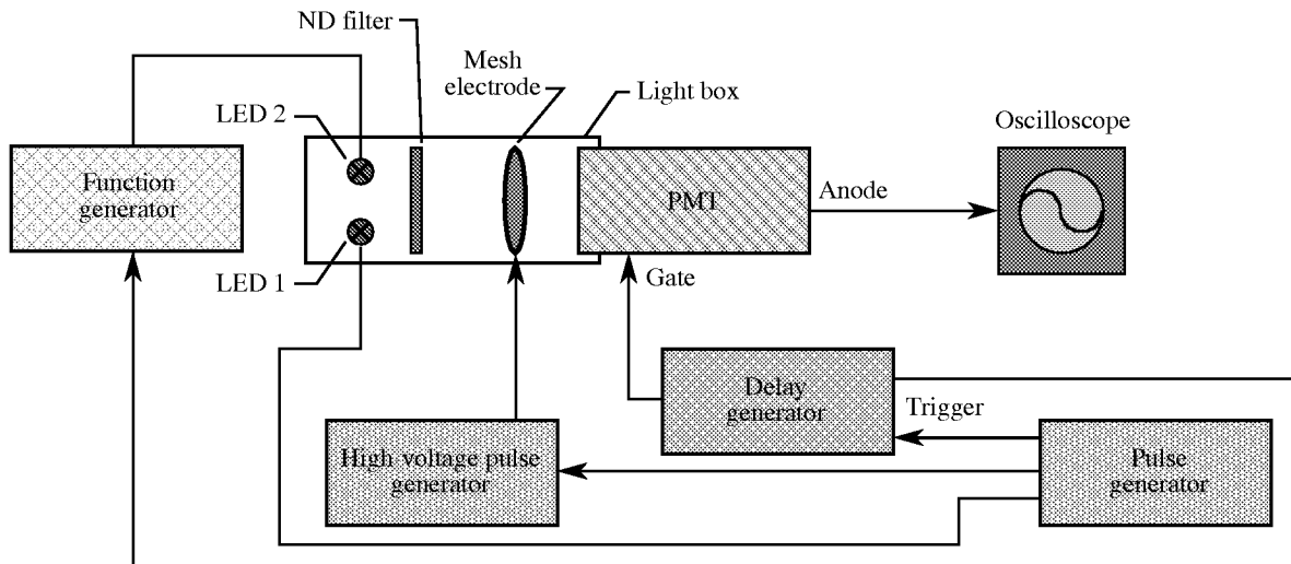
Figure 14. Experimental setup for simulation of lidar return signal and characterization of signal-induced noise.
