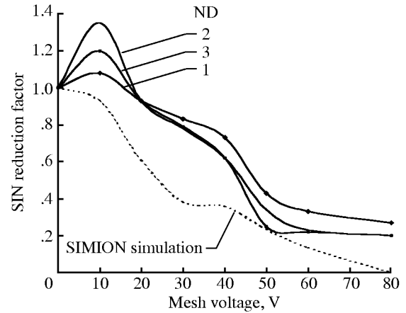
Figure 19. Effect of mesh voltage on signal-induced noise at different PMT saturation levels.
