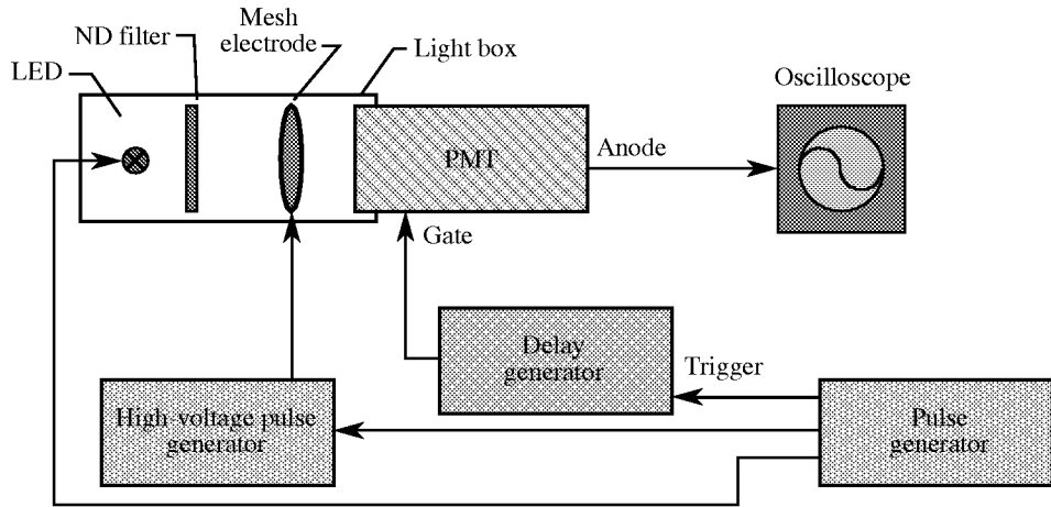
Figure 11. Experimental setup for examining mesh electrode effect on SIN.
