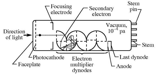
Figure 6. Schematic of typical PMT. (From ref. 23.)
