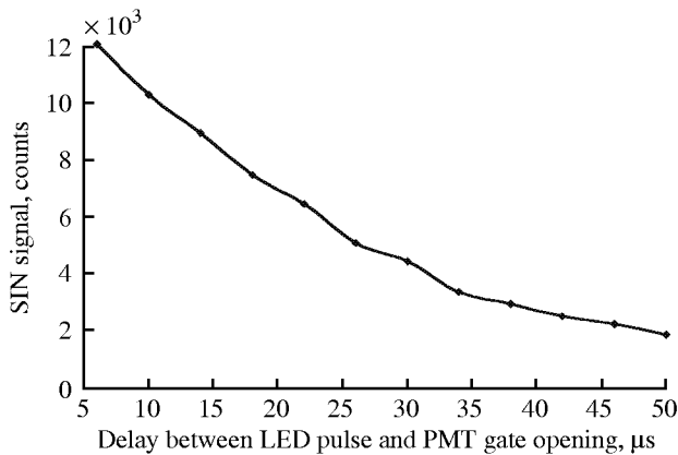
Figure 22. Correlation between SIN and time interval between LED and gate opening.
