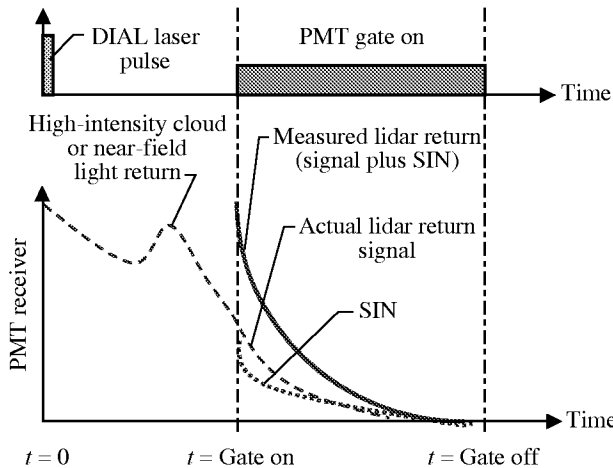
Figure 4. Formation of measured lidar signal by addition of SIN to actual lidar return.
