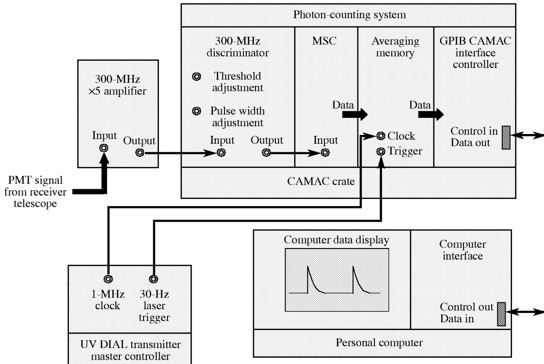
Figure 18. Photon-counting system setup. (From ref. 33.)
