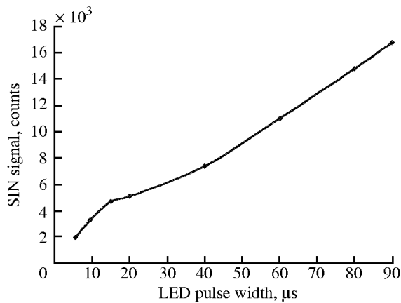
Figure 21. Correlation between signal-induced noise and LED pulse width.
