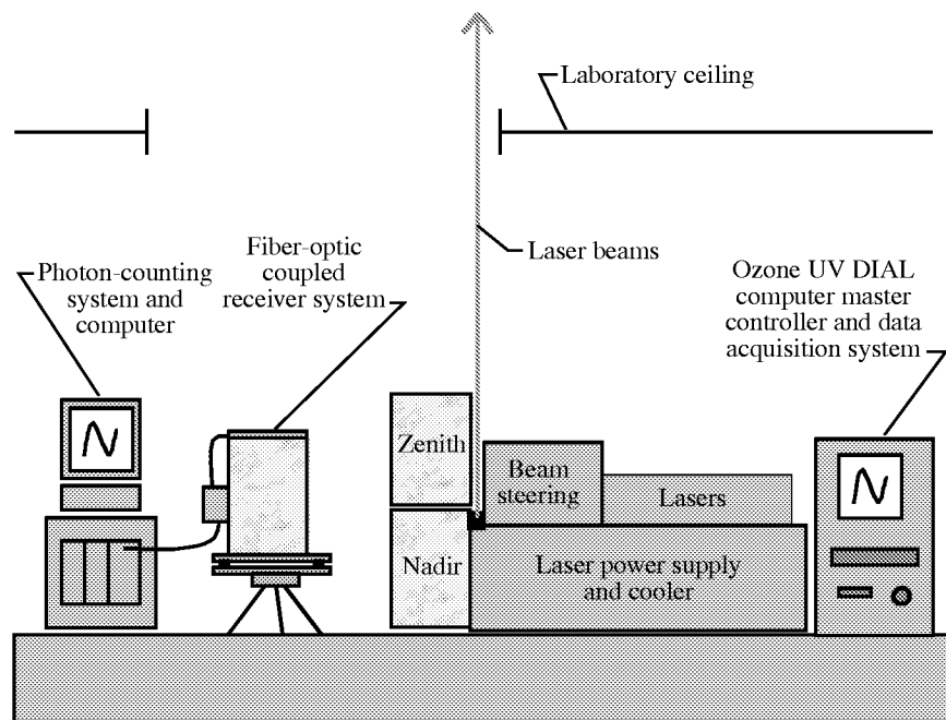
Figure 16. Ozone UV DIAL system for ground-based measurements at Langley Research Center. (From ref. 33.)
