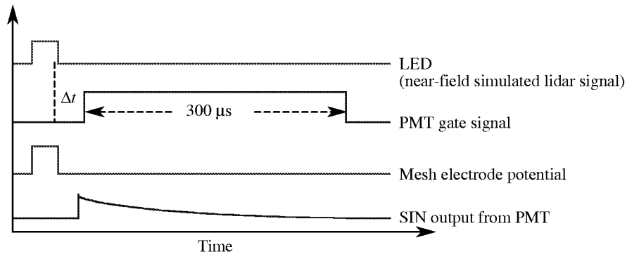
Figure 12. Timing diagram for analysis of SIN.
