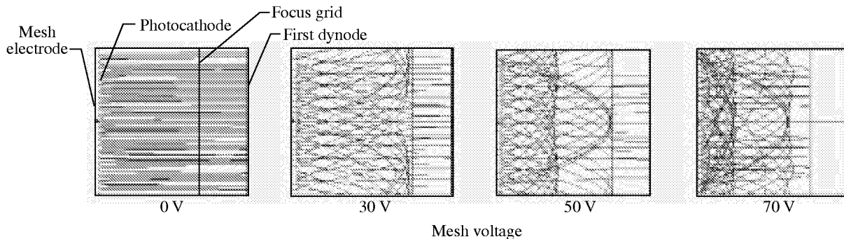
Figure 9. SIMION simulation of effect of mesh electrode on PMT electron trajectories.
