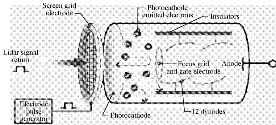
Figure 8. Signal-induced noise suppression system.
