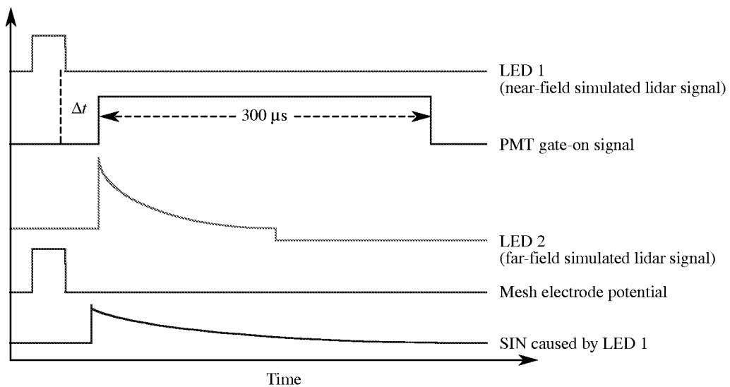
Figure 15. Timing diagram for simulation of lidar returns.
