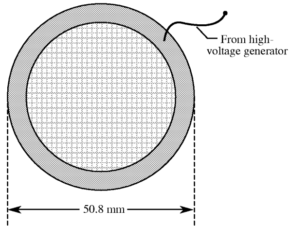
Figure 13. Mesh electrode used in front of PMT photocathode.
