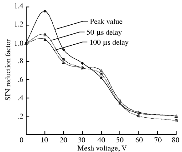
Figure 20. Effect of mesh voltage on signal-induced noise at different delay times after PMT gate opening.
