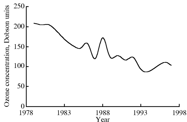
Figure 2. Lowest ozone concentrations over Antarctic between 1979 and 1997 (September 9–October 10).
