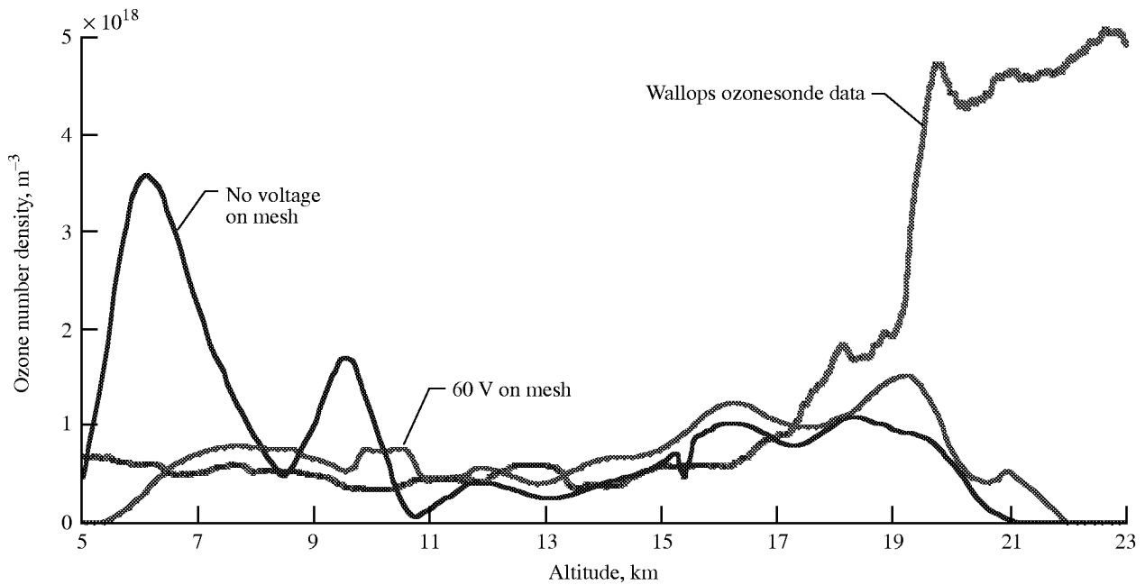
Figure 26. Comparison between ozone data from Wallops ozonesonde and ground-based tropospheric measurements conducted at Langley Research Center.
