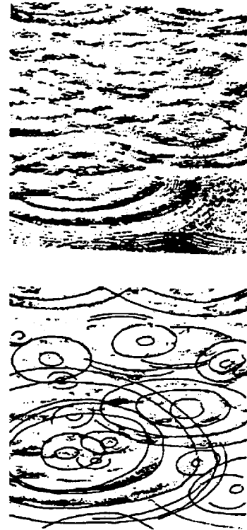
Fig. 1. Multiring impact overprint in water, showing cancellation and reinforcement wave patterns.
