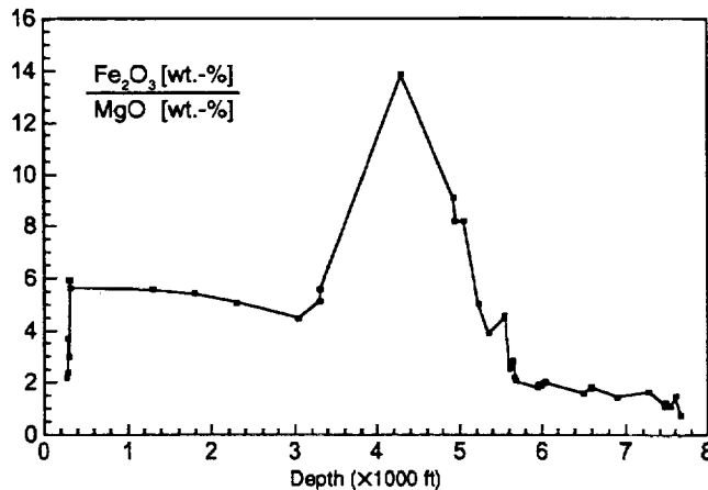
Fig. 1. Variation of the Fe 2 O 3 /MgO-ratio (wt.-%) in samples of the drill core 70011. The maximum value is not correlated to a lithological boundary (granophyre = 400–5000 ft; quartz-gabbro = 5000–6000 ft; norite = 6000–7500 ft; Sublayer = 7500–8000 ft).
