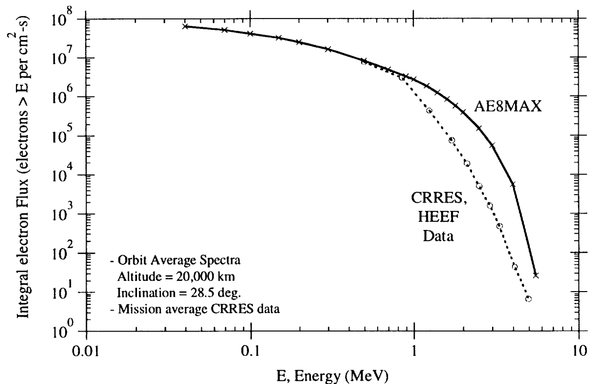
Fig. 5-10. Comparison of outer belt trapped electron spectrum based on CRRES satellite measurements with spectrum predicted using AE8MAX model.
