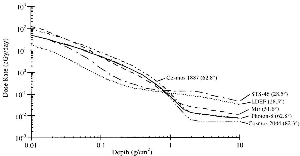
Fig. 2-10. Comparison of predicted dose rates.
