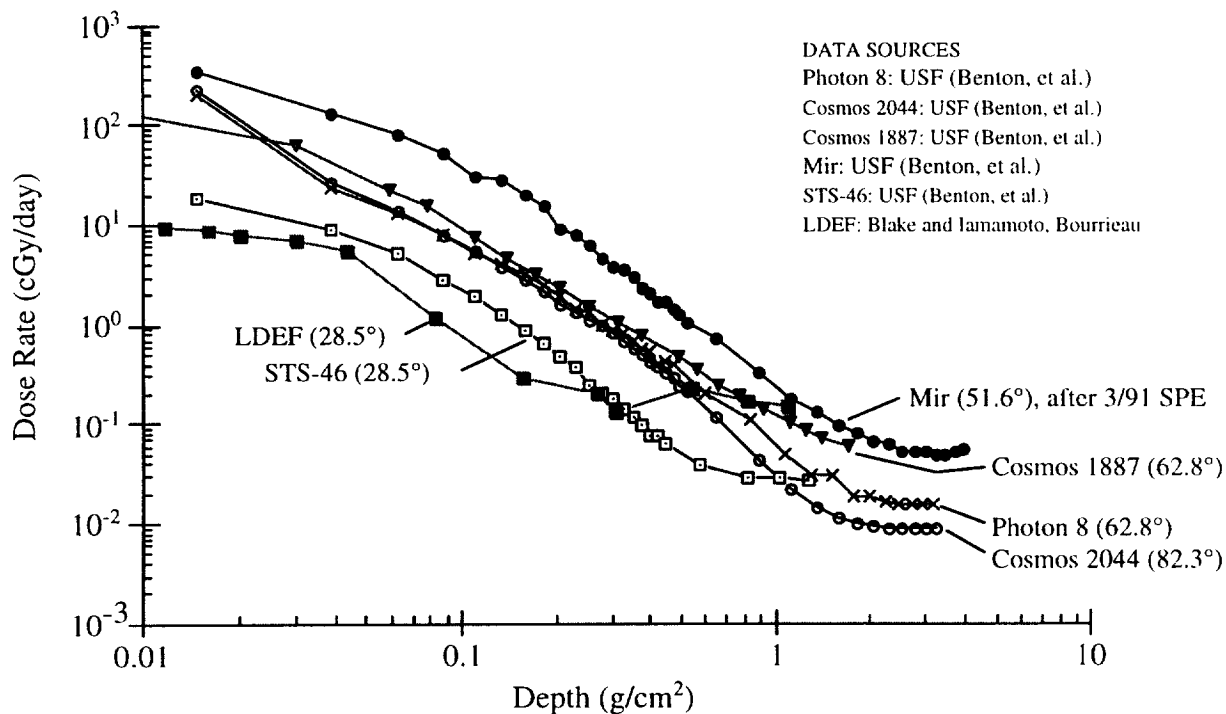
Fig. 2- 9. Comparison of measured dose rates.
