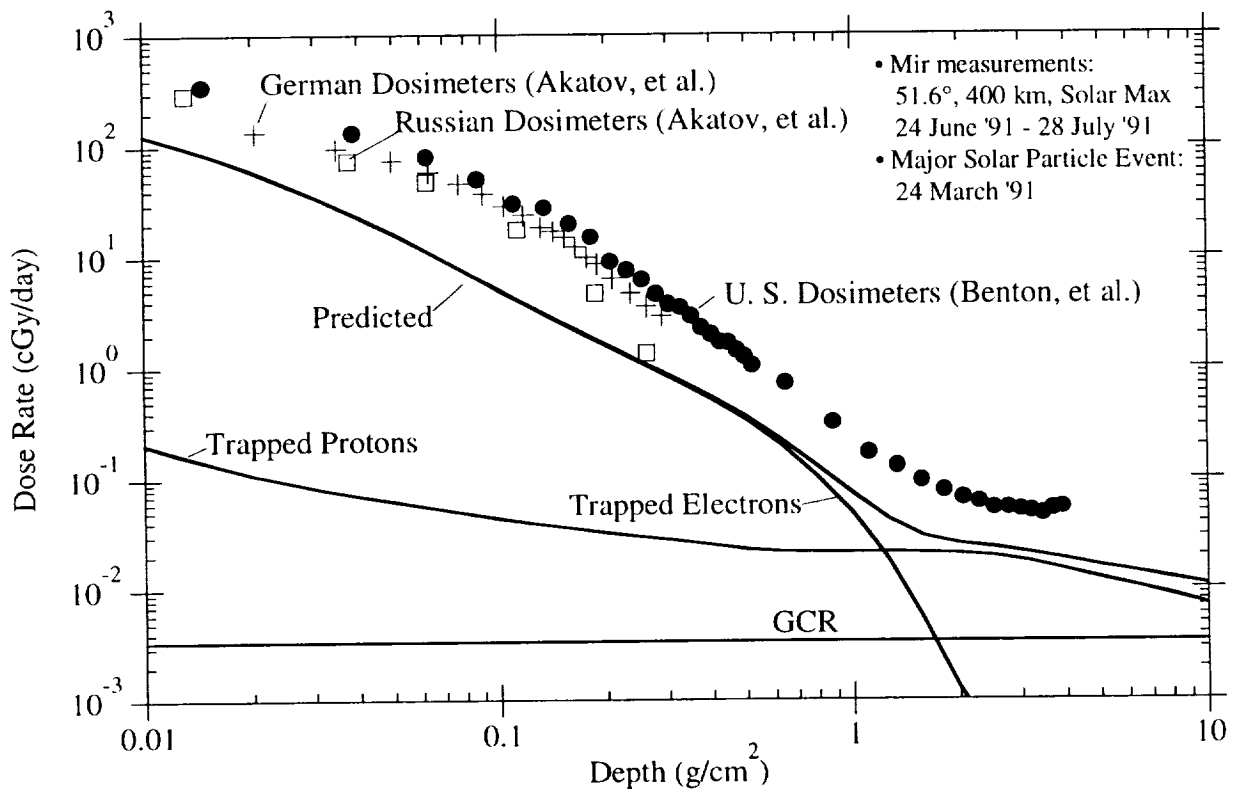
Fig. 2- 4. Predicted vs. measured dose rate on Mir space station.
