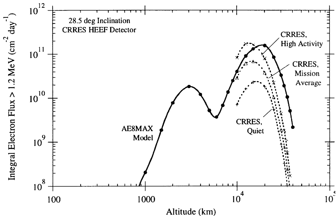
Fig. 5-9. Comparison of electron flux > 1.2 MeV based on CRRES satellite measurements for various geomagnetic activity conditions with AE8MAX trapped electron model predictions.
