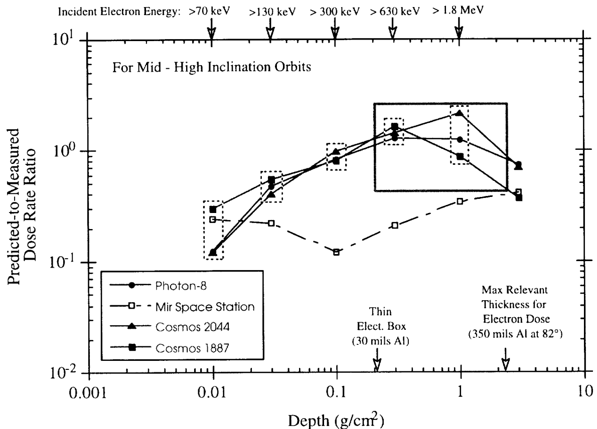
Fig. 2- 13. Ratio of predicted-to-measured dose rates for mid and high inclination orbits.
