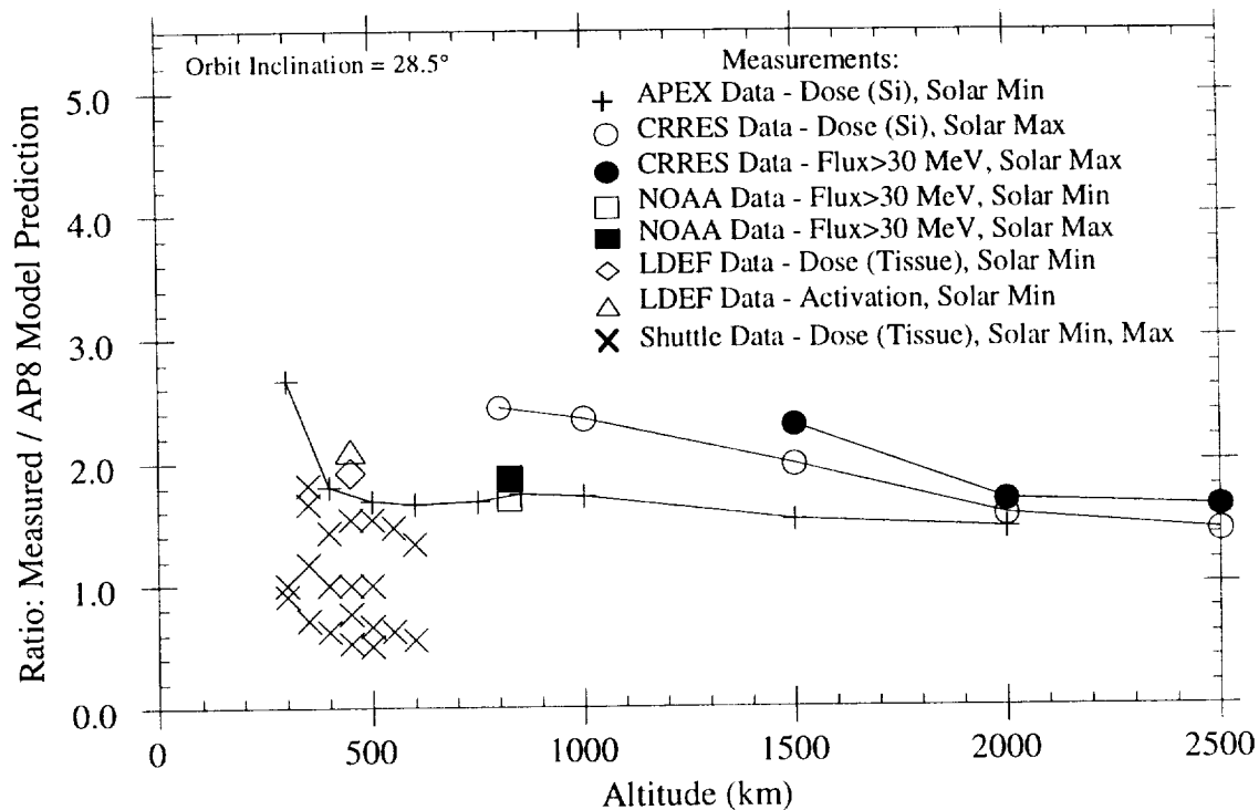
Fig. 3-10 Measured-to-predicted dose ratio calculated here based on Shuttle data compared with data-model ratios from ref. [3-2] using other flight data (all for circular, 28.5 deg. inclination orbits).
