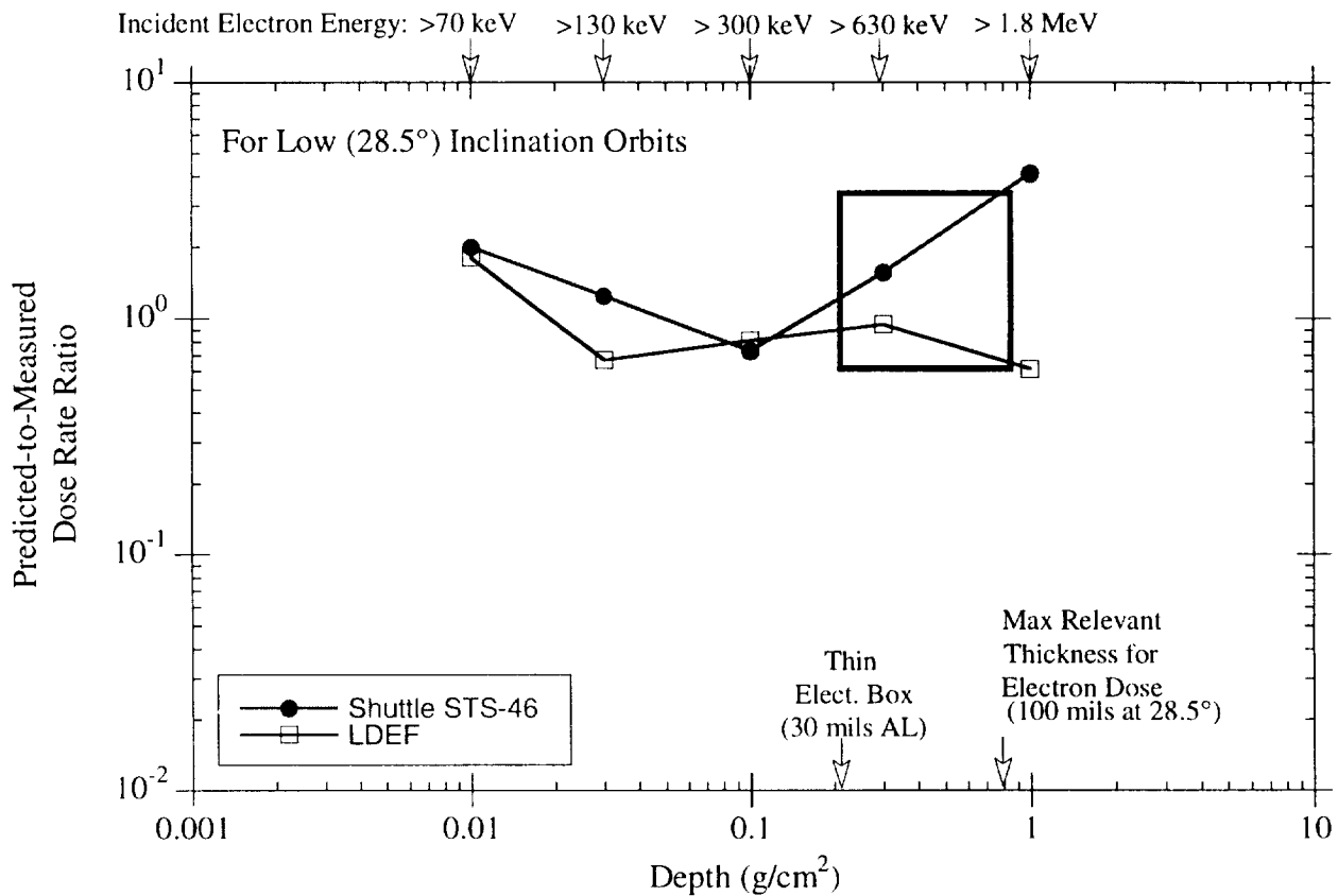
Fig. 2- 12. Ratio of predicted-to-measured dose rates for low inclination ( 28.5^\circ ) orbits.
