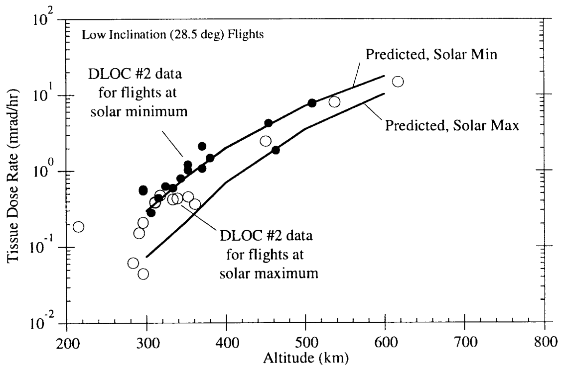
Fig. 3-6. Comparison of predicted and measured dose rates for low-inclination Shuttle flights.
