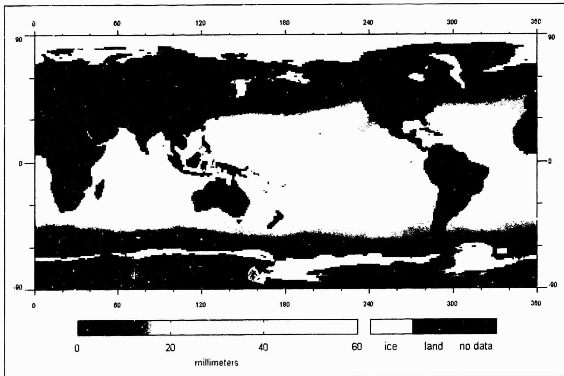
Total integrated water vapor over the global oceans as retrieved from DMSP Special Sensor Microwave/Imager (SSM/I) data during January 1998.
