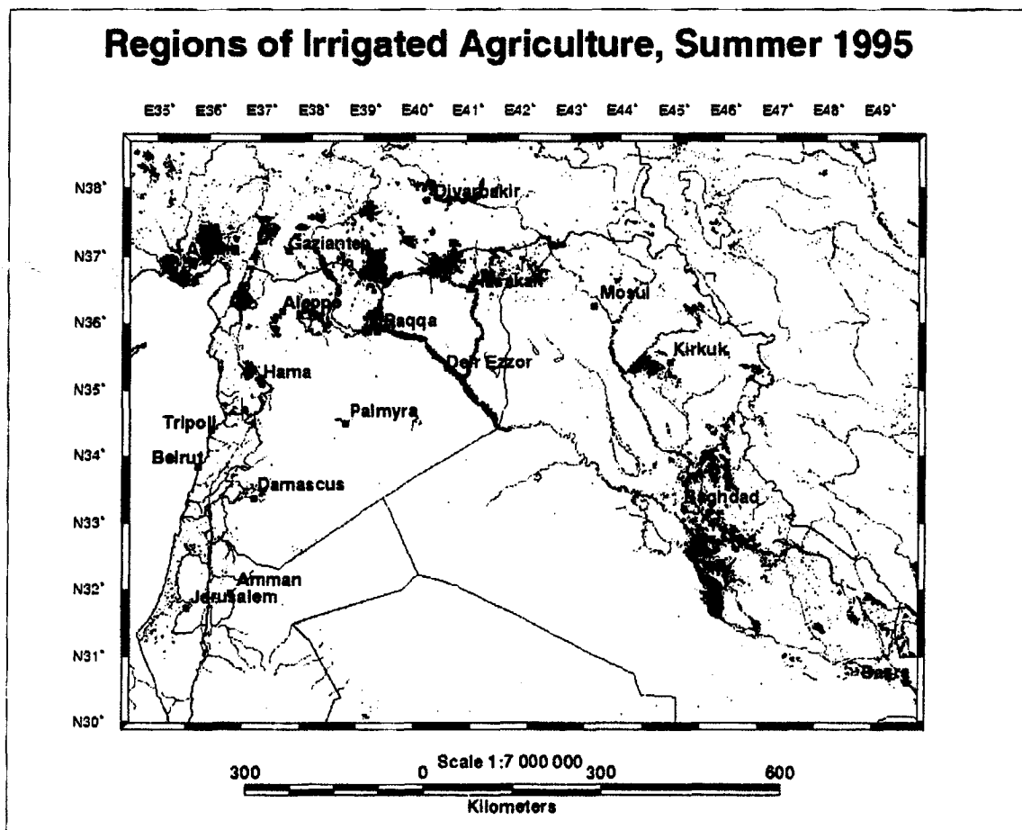
Using composite AVHRR imagery and simple models, several aspects of Middle East hydrology can be monitored including upland snow cover, river discharge, irrigated agriculture, and rain-fed farming. This image shows, with a spatial resolution of one kilometer, the active irrigated agriculture during the summer of 1995. The largest of these regions are on the lower Ceyhan near Adana in Turkey, the GAP project in Turkey near the Syrian border, new projects near Raqqa and Aleppo in Syria, historic farms along the Syrian Euphrates and in Mesopotamia near Baghdad, Iraq. These patterns of irrigation have changed dramatically over the last 15 years.
