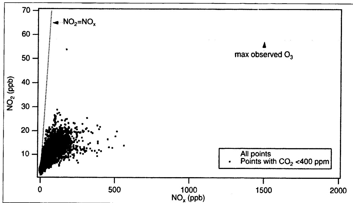
Relationship of \text{NO}_2 to \text{NO}_x in an urban area. Data collected with a mobile TDL spectrometer on city and highway roads of Manchester, NH, 2:30-9 pm EDT on 26 August 1998. The darker points are those with corresponding \text{CO}_2 < 400 ppm and thus are not a result of directly sampling a combustion source such as vehicle exhaust.
