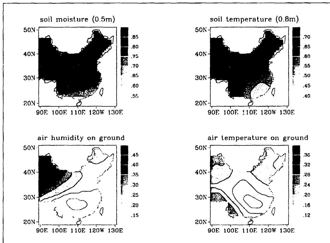
One month-lag autocorrelation coefficients in China, indicating the strongest persistence in soil moisture, and in increasing tendency in persistence from moist to dry climate regimes.
