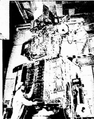
The ETM+ scanner (above) being prepared prior to shipment for installation on the Landsat 7 platform (right). Landat 7 was successfully launched from Vandenberg Air Force Base on April 15, 1999.
