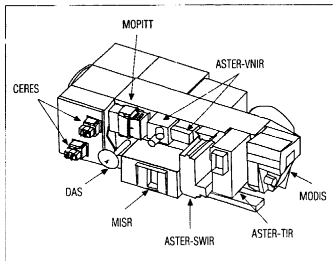
Figure 7. Terra Platform and Payload.
