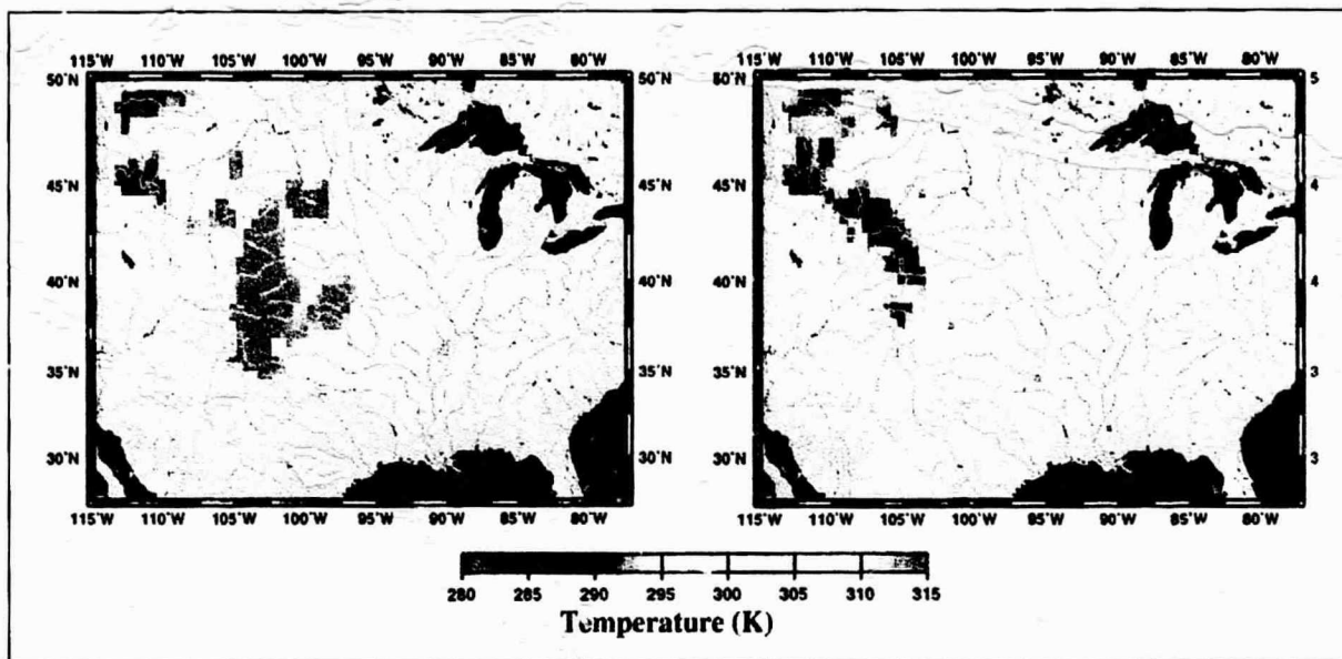
The advantage of satellite-based temperature estimation is the ability to continuously map over large regions. The images above show surface temperature (left) and air temperature (right) retrievals for the entire Mississippi basin at the AVHRR overpass time for 19 June, 1987. Note the relative difference between the two fields and the area of considerably warmer surface temperatures to the west, and the cooler air temperatures in the mountains forming the western border of the basin. (After Dubayah and Lettenmaier, 1997.)
