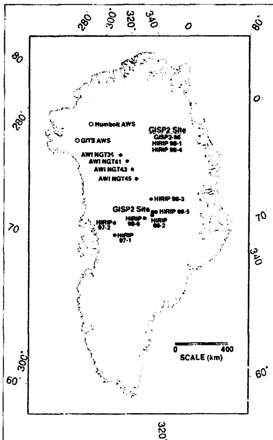
Location of high-resolution isotope profiles used in this study.
