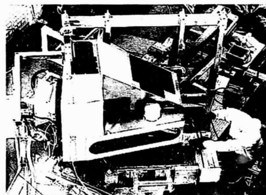
The Moderate-resolution Imaging Spectroradiometer (MODIS) instruments—built to NASA specifications by Santa Barbara Remote Sensing—represent the finest in engineering of spaceflight hardware for remote sensing of the atmosphere, land, and ocean. MODIS is scheduled for flight on Terra and EOS PM.
