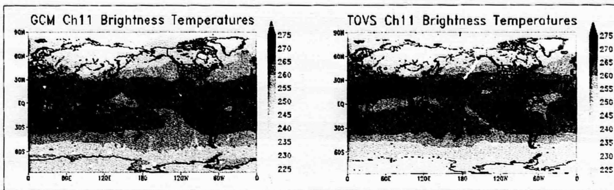
Comparisons of observed January TOVS/HIRS channel 11 brightness temperatures with brightness temperatures calculated using data derived from the CSU GCM.
