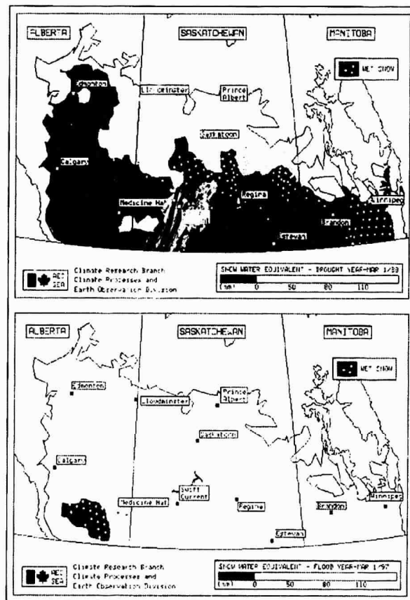
Passive microwave (SSM/I)-derived snow water equivalent for March 1, 1988 (drought year) and March 1, 1997 (flood year) on the Canadian prairies (shaded area).
