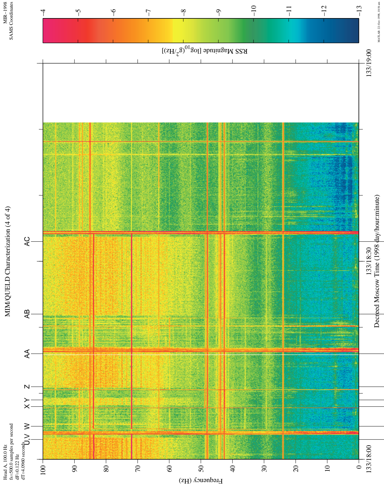
Figure 9. MIM characterization test (fourth hour).
