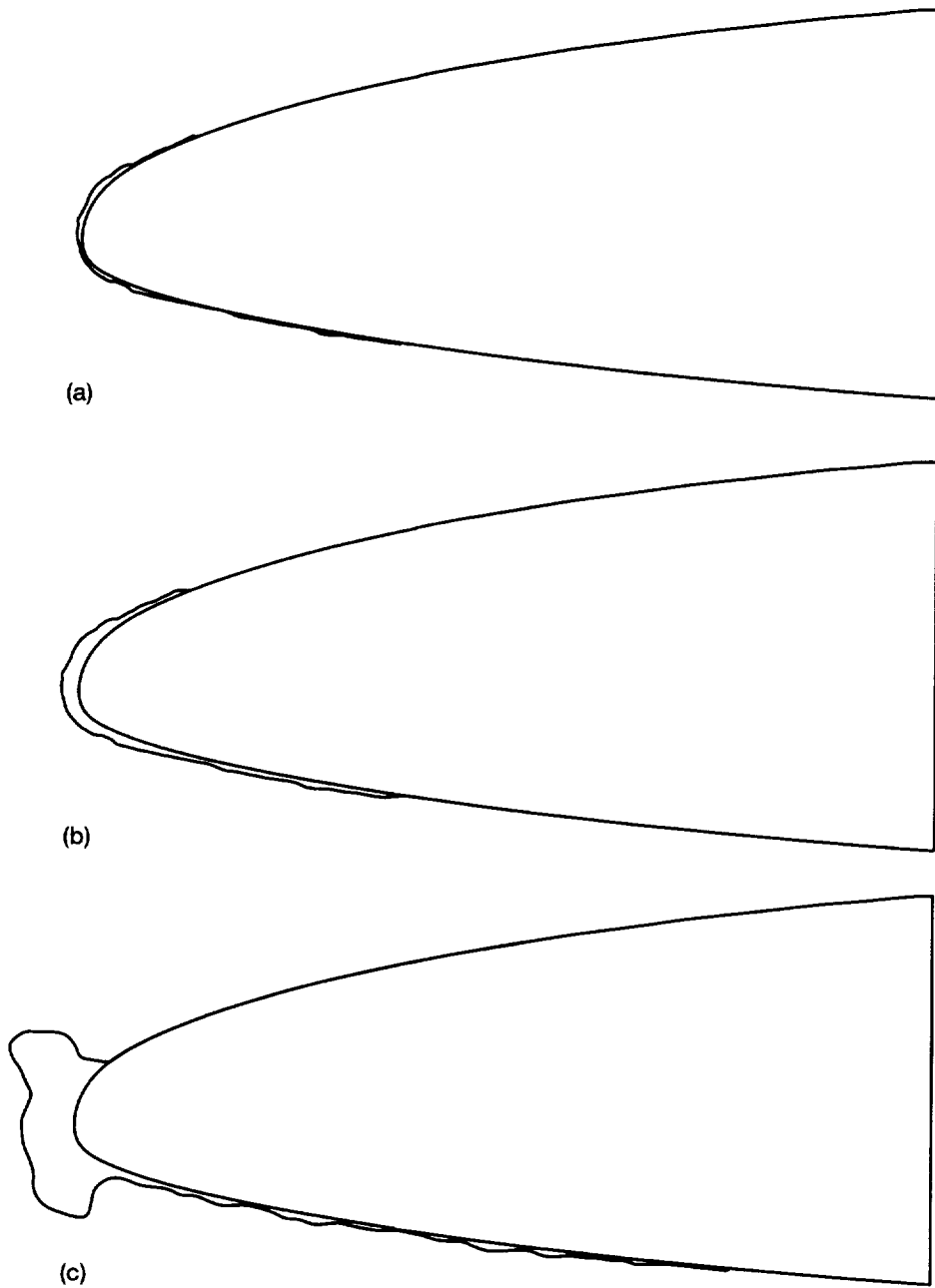
Figure 9.—Smoothed two-dimensional ice shapes for LTPT general aviation model tests. (a) 2-min (run 621). (b) 6-min (run 622). (c) 22.5-min (run 623). Speed, 130 kn; attitude, 2°; total temperature, T_t , 26.4 °F; median volumetric diameter, MVD , 20 \mu\text{m} ; liquid water content, LWC , 0.54 \text{g}/\text{m}^3 .
