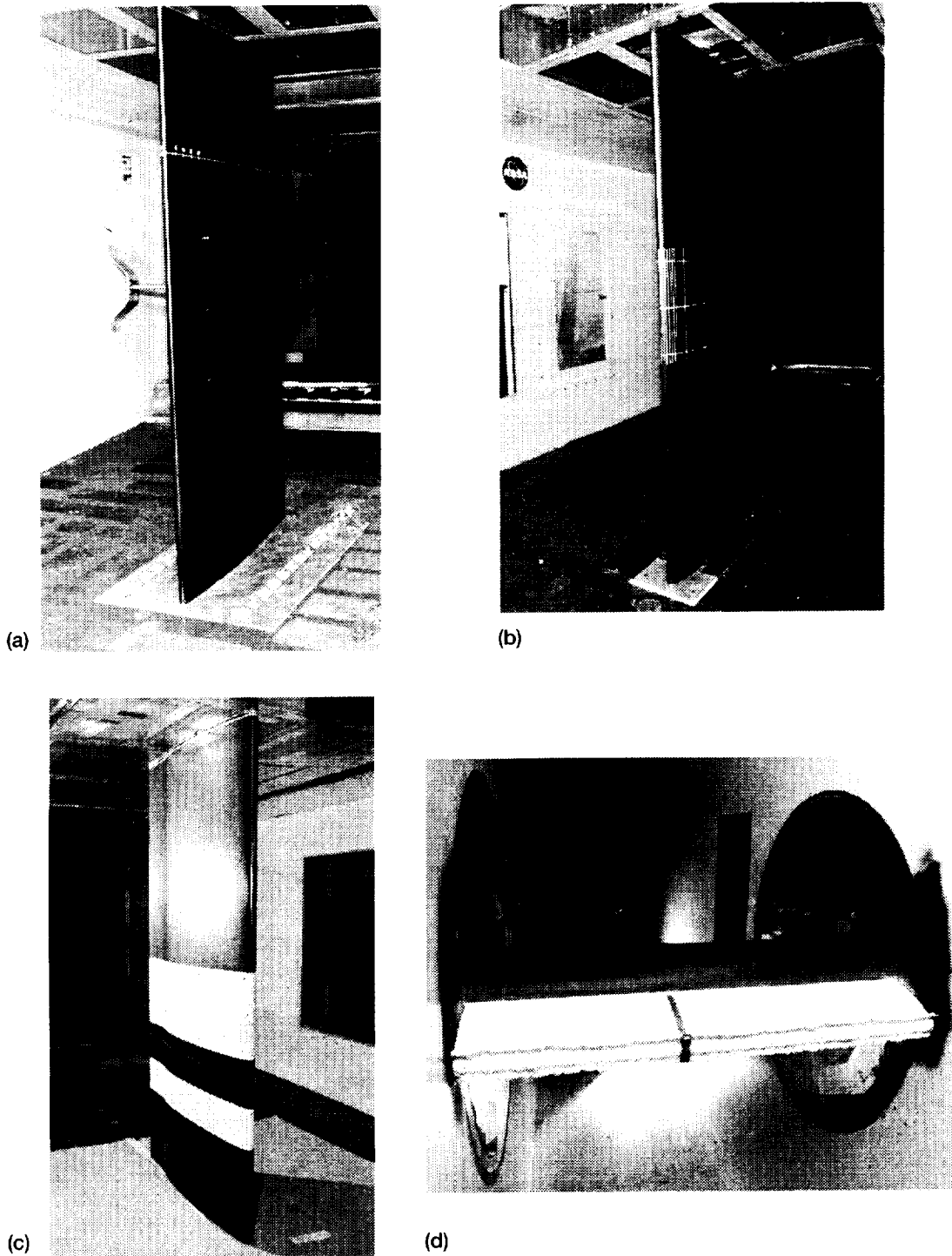
Figure 3.—Models used in the Modern Airfoil Program. (a) Business jet model. (b) Commercial transport model. (c) General aviation model. (d) General aviation model used in Low-Turbulence Pressure Tunnel (LTPT).
