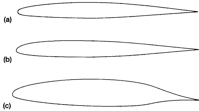
Figure 1.—Airfoils used in the Modern Airfoil Program. (a) Business jet airfoil. (b) Commercial transport airfoil. (c) General aviation airfoil.
