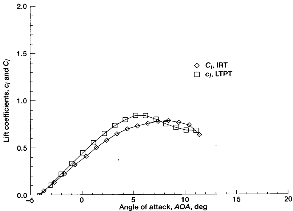
Figure 14.—Comparison of IRT and LTPT lift coefficients ( C_l and c_l , respectively) for 22.5-min ice shape (run 623). Lift coefficient C_l was calculated from force balance measurements; lift coefficient c_l was calculated from surface pressure taps.
