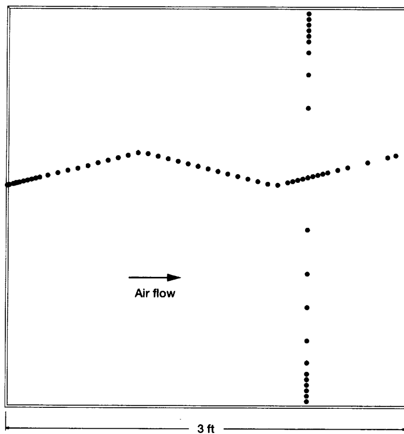
Figure 5.—Upper surface pressure taps on LTPT general aviation model.
