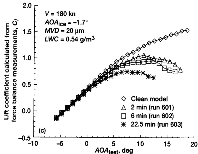
Figure 15.—Effect of various icing exposure times on lift for different models at a total temperature of 30 °F (IRT). (a) Business jet. (b) Commercial transport. (c) General aviation. Velocity, V ; median volumetric diameter, MVD ; liquid water content, LWC ; angle of attack at which ice accretions were formed, AOA_{ice} ; angle of attack during testing, AOA_{test} .
