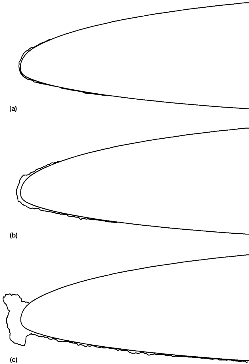
Figure 8.—Tracings of ice shapes for LTPT general aviation model tests. (a) 2-min (run 621). (b) 6-min (run 622). (c) 22.5-min (run 623). Speed, 130 kn; altitude, 2°; total temperature, T_t , 26.4 °F; median volumetric diameter, MVD , 20 \mu\text{m} ; liquid water content, LWC , 0.54 \text{g}/\text{m}^3 .
