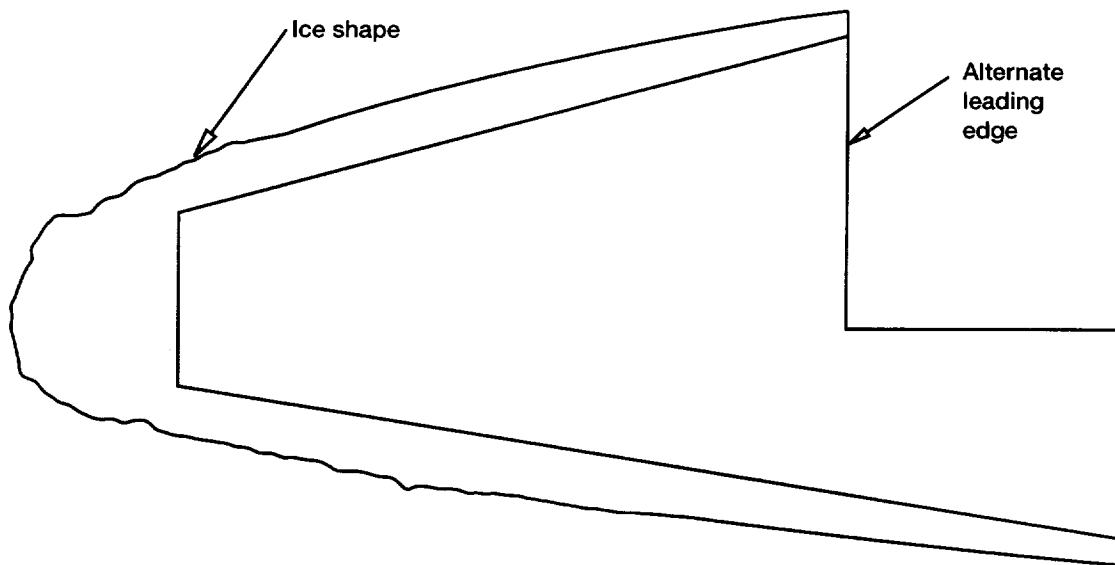
Figure 4.—Cross section of alternate leading edge with ice shape for LTPT general aviation model.
