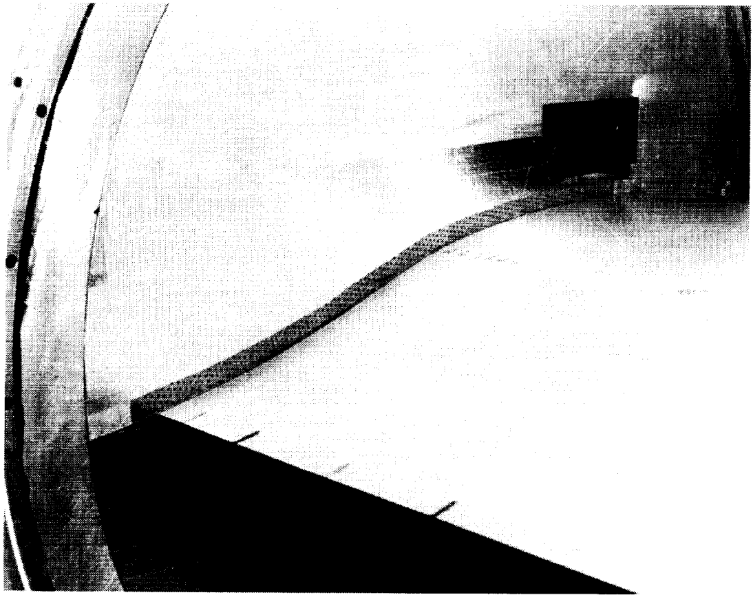
Figure 7.—Sidewall venting over trailing edge of general aviation model in LTPT.
