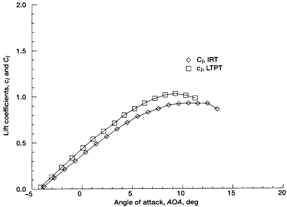
Figure 13.—Comparison of IRT and LTPT lift coefficients ( C_l and c_l , respectively) for 6-min ice shape (run 622). Lift coefficient C_l was calculated from force balance measurements; lift coefficient c_l was calculated from surface pressure taps.
