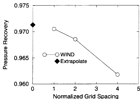
Figure 1. The pressure recoveries for the supersonic diffuser.
