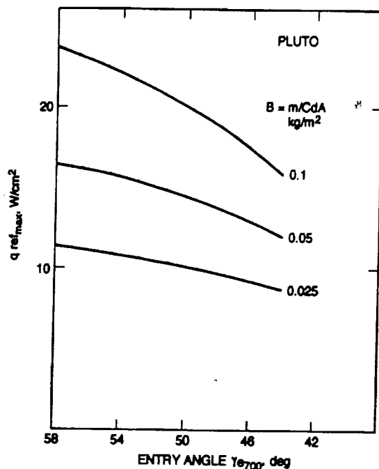
Figure 11. Peak stagnation point pressure for Pluto entry versus entry angle, for ballutes with m/CdA = 0.025, 0.05 , and 0.1 \text{ kg/m}^2 .
