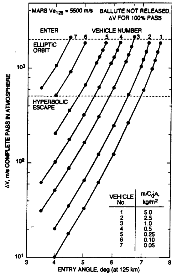
Figure 2. Delta-V loss for 7 ballute sizes versus entry angle.
