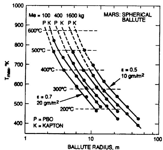
Figure 6. Peak temperature for the ballutes versus ballute radius, for PBO and Kapton, for entry mass values of 100, 400 and 1600 kg.
