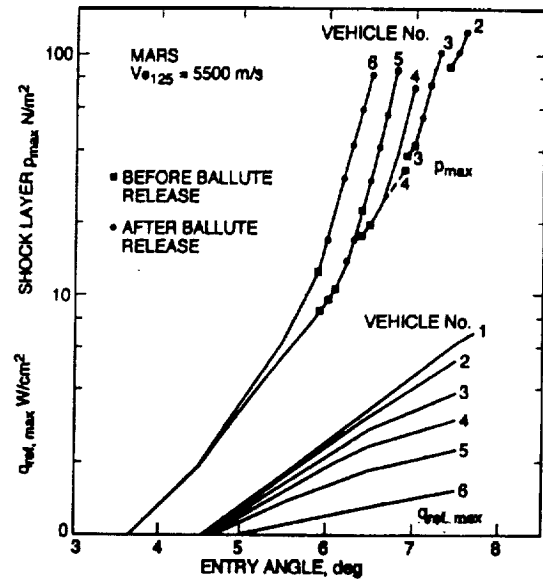
Figure 5. Peak stagnation pressure and peak reference convective heating rate for the ballutes versus entry angle.
