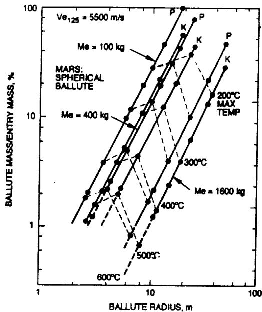
Figure 7. Mass fraction of the ballute system (net, ballute, gas, bottle) versus ballute radius, for PBO and Kapton, for entry mass 100, 400 and 1600 kg.
