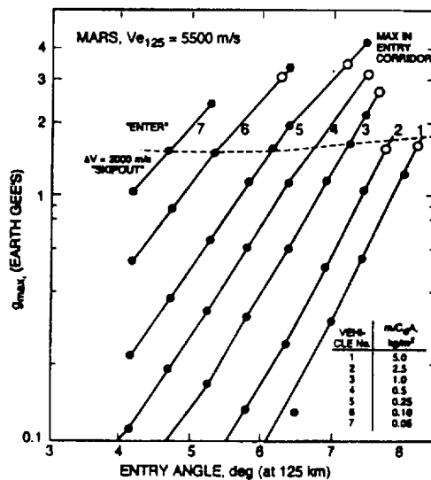
Figure 4. Peak g-load versus entry angle for the 7 ballutes.
