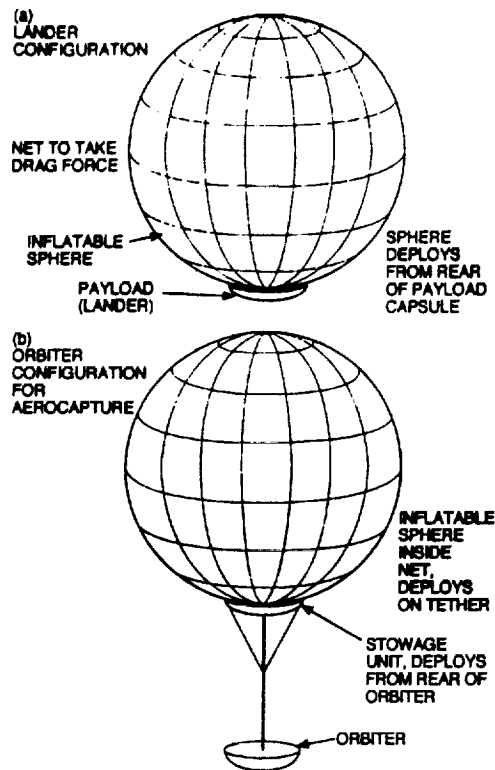
Figure 1: Ballute Shapes: (a) sphere: lander configuration; (b) sphere: orbiter configuration
