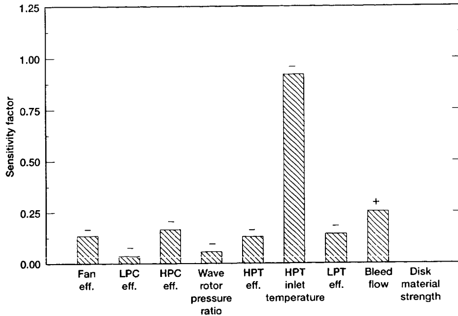
Figure 7.—Sensitivity of engine net thrust.
