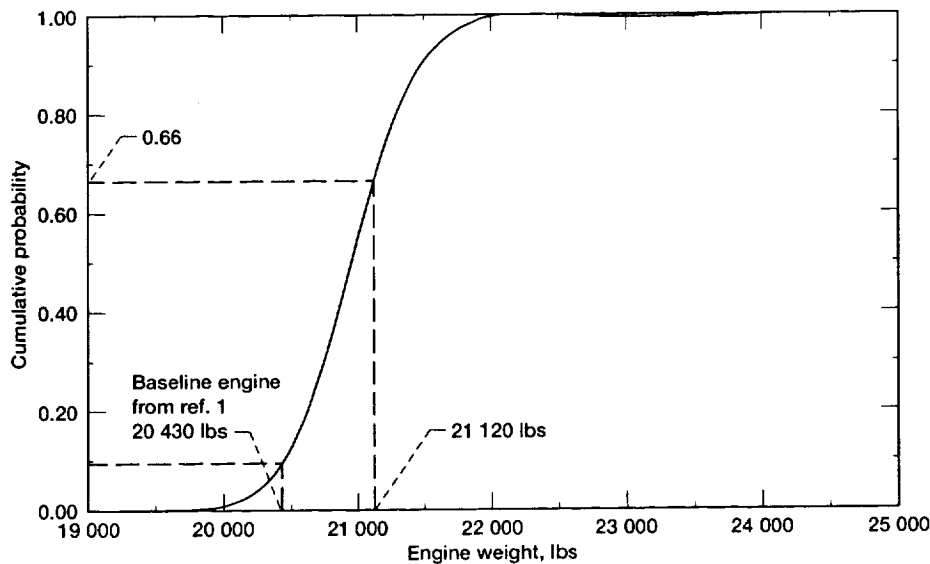
Figure 8.—CDF of wave rotor-enhanced turbofan engine weight.
