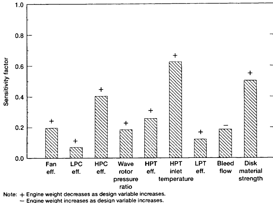
Figure 9.—Sensitivity of engine weight.
