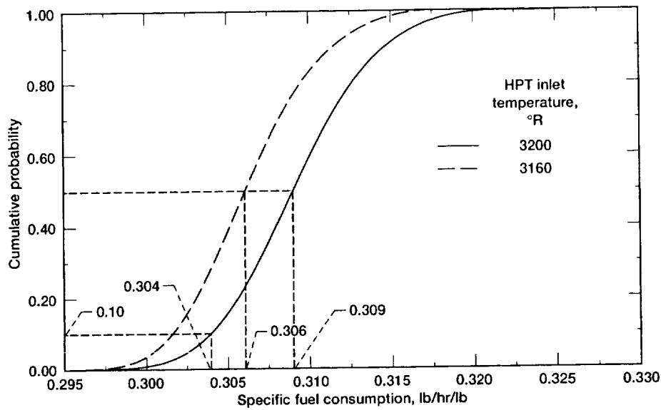
Figure 3.—CDF of wave rotor-enhanced turbofan engine SFC.
