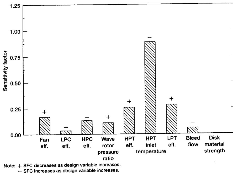
Figure 4.—Sensitivity of specific fuel consumption.
