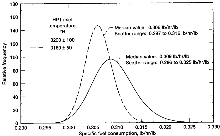
Figure 5.—PDF of wave rotor-enhanced turbofan engine SFC.
