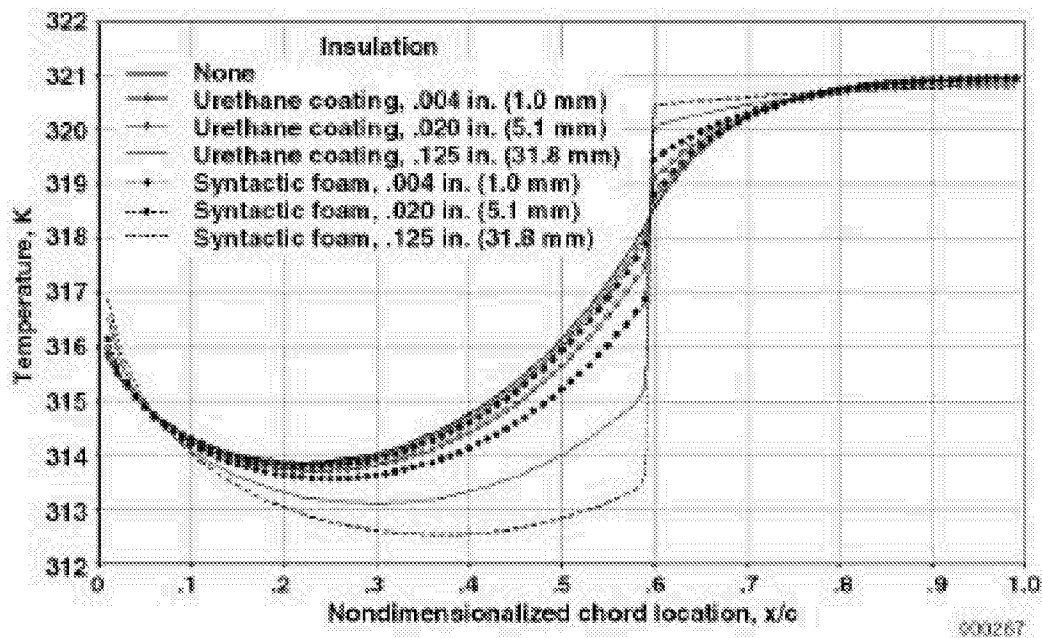
Fig. 6. Steady state surface temperature distributions with insulation. Three percent biconvex airfoil, 3 ft chord, M_\infty = 1.4 , 24,500 ft (standard atmosphere). Transition fixed at 60 percent of chord.
