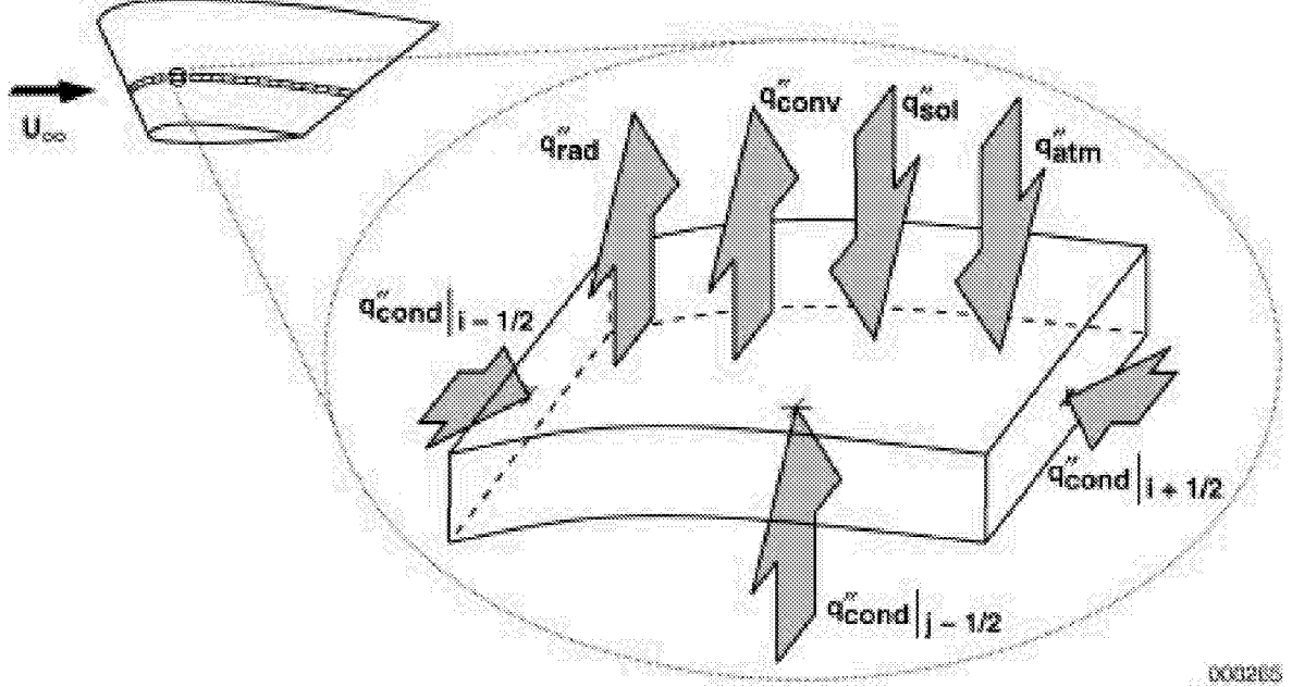
Fig. 4. Heat transfer mechanisms on a wing in flight.
