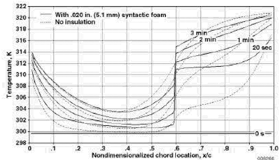
Fig. 5. Temperature distribution history with .020 in. (5.1 mm) syntactic foam. Three percent biconvex airfoil, 3 ft chord, M_\infty = 1.4 , 24,500 ft (standard atmosphere), uniform initial temperature of 80 °F (300 K). Transition fixed at 60 percent of chord.
