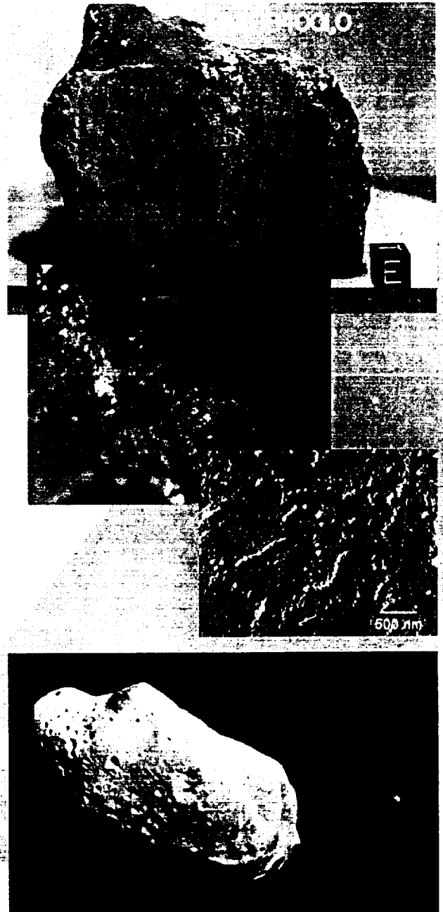
Top: Martian meteorite ALH84001.
