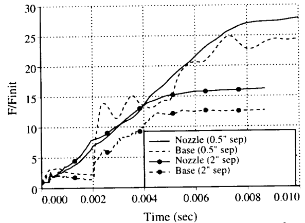
Fig. 5. Flyer nozzle and base force history from inviscid 2D simulations at 0.5” and 2” separation (from Ref. 16).
