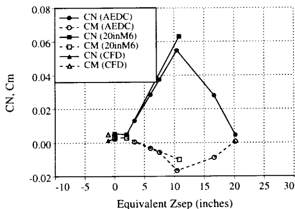
Fig. 10. Wind tunnel and computed aerodynamic coefficients at X_{sep}=-9 ".
