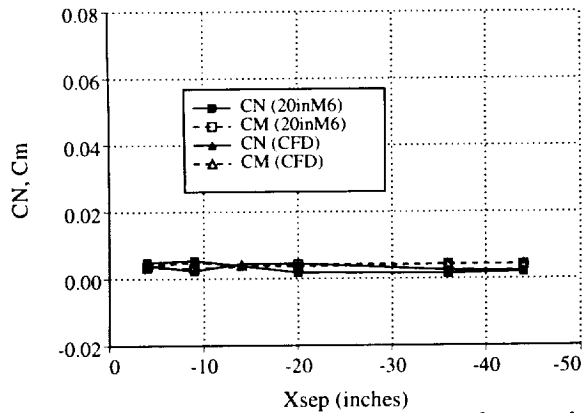
Fig. 7. Comparison of steady-state force and moment coefficients for several separation distances.
