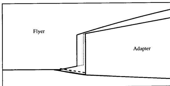
Fig. 14. Schematic of earlier thin seal (solid), wind tunnel seal (dashed), and current flight design (dotted).
