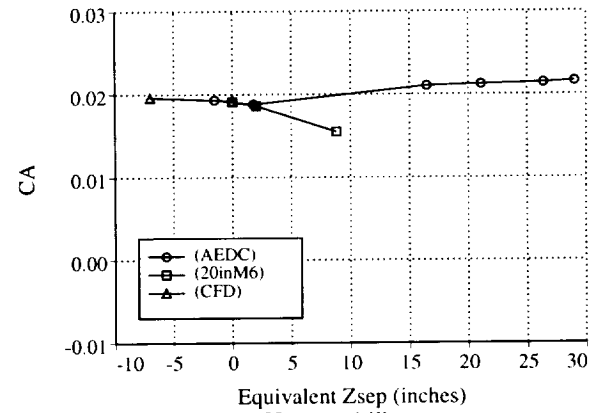
Fig. 12. Wind tunnel and computed aerodynamic coefficients at X_{sep}=-44'' .
