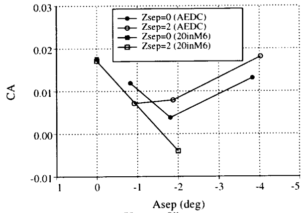
Fig. 8. Wind tunnel aerodynamic coefficients vs. A_{sep} , at X_{sep}=-9'' .
