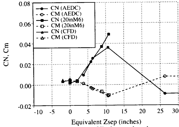
Fig. 11. Wind tunnel and computed aerodynamic coefficients at X_{sep}=-20'' .
