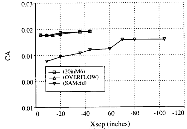
Fig. 13. CFD prediction of aerodynamic interference variation with X_{sep} .
