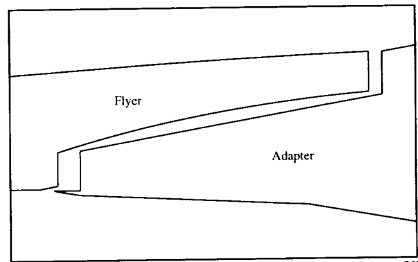
Fig. 4. Centerline flyer/adapter gap geometry at 2” separation.
