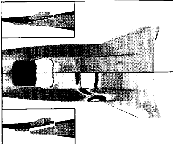
Fig. 9. Pressure on the underside of the research vehicle at A_{sep}=0 (top) and -1^\circ (bottom), at X_{sep}=-4 " and Z_{sep}=0 .
