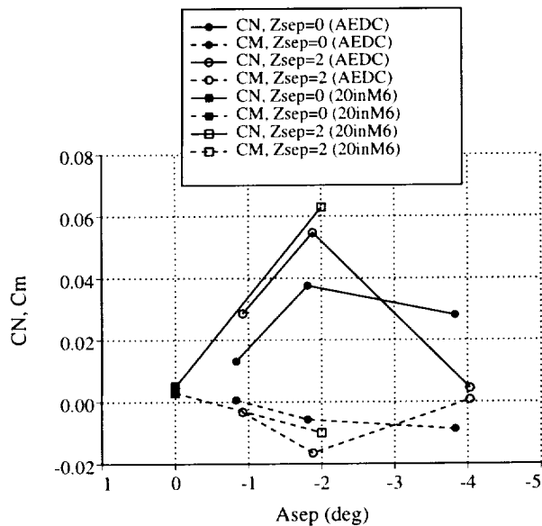
Fig. 8. Wind tunnel aerodynamic coefficients vs. A_{sep} , at X_{sep}=-9'' .
