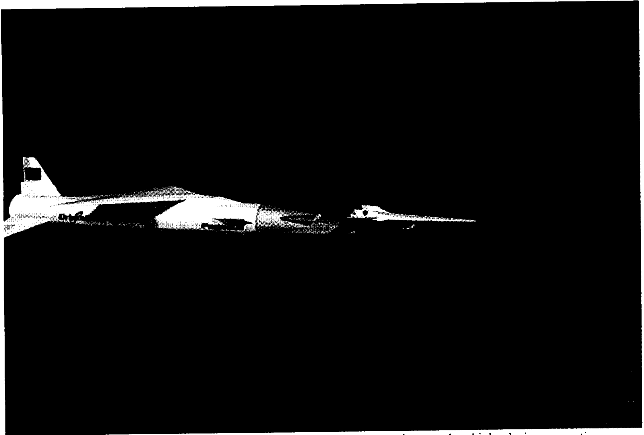
Fig. 1. Hyper-X launch vehicle consisting of booster, adapter and research vehicle, during separation.
