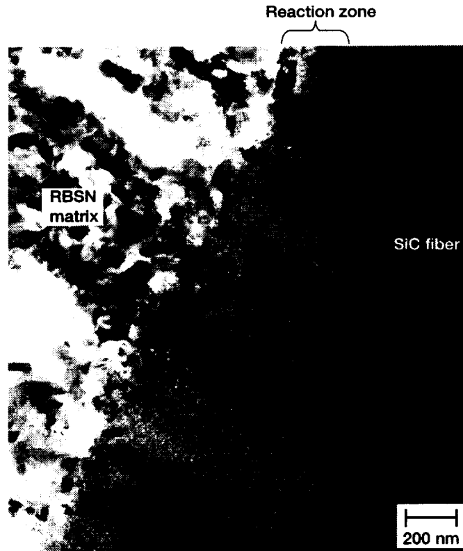
Figure 6.—TEM micrograph of the fiber/matrix interface region of an uncoated Hi-Nicalon SiC/RBSN composite ( V_f \sim 0.24 ) with NiO showing reaction between the SiC fiber and NiO additive.
