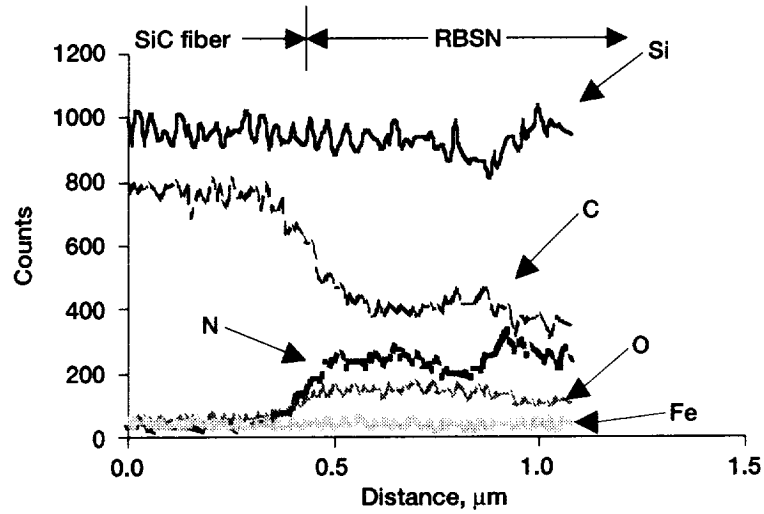
Figure 5.—EDX line profile across the fiber/matrix interface region of an uncoated Hi-Nicalon SiC/RBSN composite without NiO additive showing no apparent reaction between the SiC filament and RBSN matrix.
