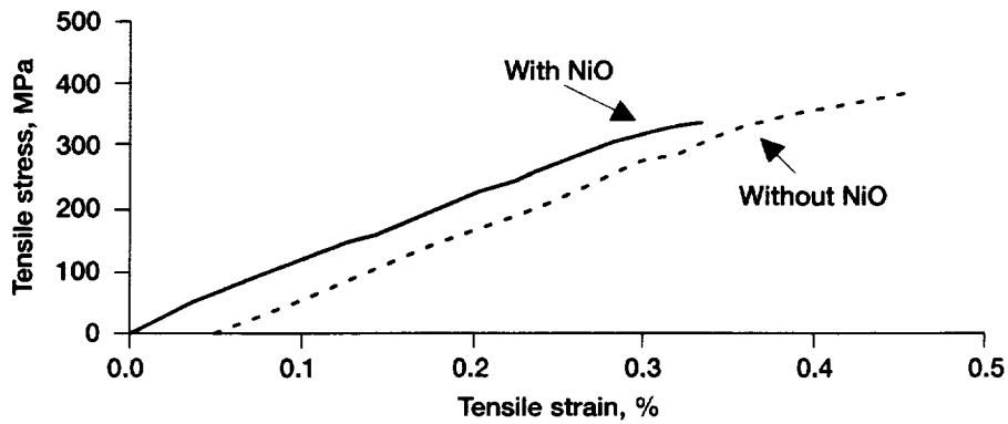
Figure 11.—Room temperature tensile stress-strain behavior for 1-D BN/SiC coated Hi-Nicalon SiC/RBSN composites ( V_f \sim 0.24 ) with and without NiO additive.
