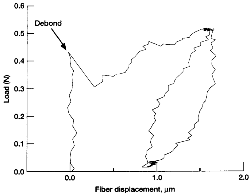
Figure 16.—Typical fiber push-in test behavior for the BN/SiC coated Hi-Nicalon SiC/RBSN composites.
