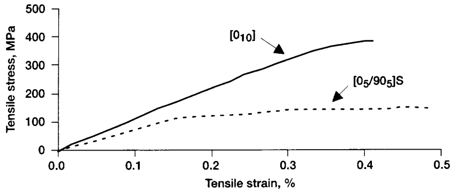
Figure 13.—Comparison of room-temperature tensile stress curves of 1-D and 2-D BN/SiC coated Hi-Nicalon SiC/RBSN composites ( V_f=0.24 ) with NiO additive.
