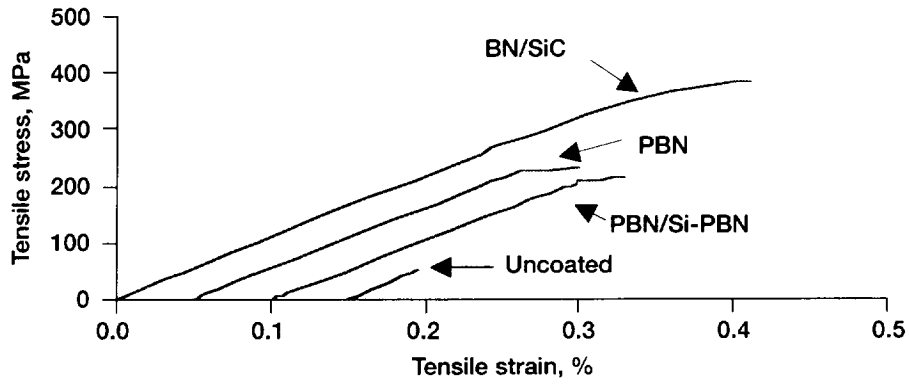
Figure 12.—Typical room temperature tensile stress-strain behavior for 1-D uncoated, PBN, PBN/Si-rich PBN, and BN/SiC coated Hi-Nicalon SiC/RBSN composite ( V_f=0.24 ) with NiO additive.
