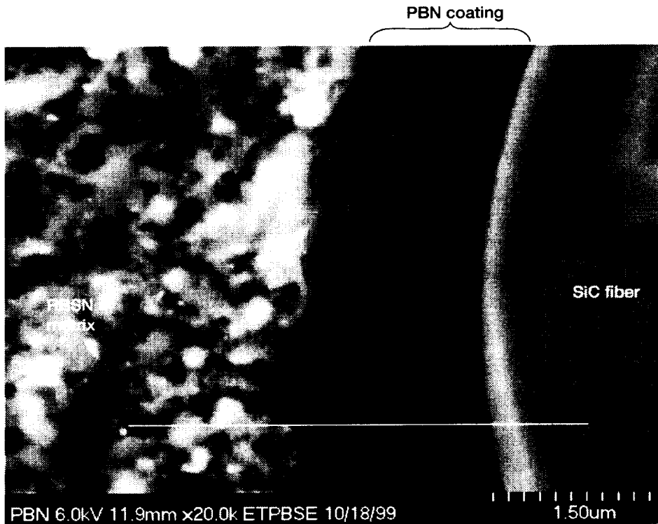
Figure 8.—FESEM micrograph of the interface region of a PBN coated Hi-Nicalon SiC/RBSN composites with NiO additive.
