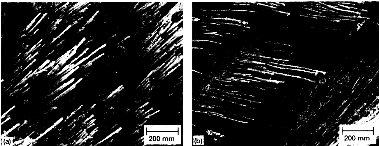
Figure 14.—SEM photographs of the tensile fracture surfaces of BN/SiC coated Hi-Nicalon SiC/RBSN composites ( V_f=0.24 ): (a) 1-D, (b) 2-D.
