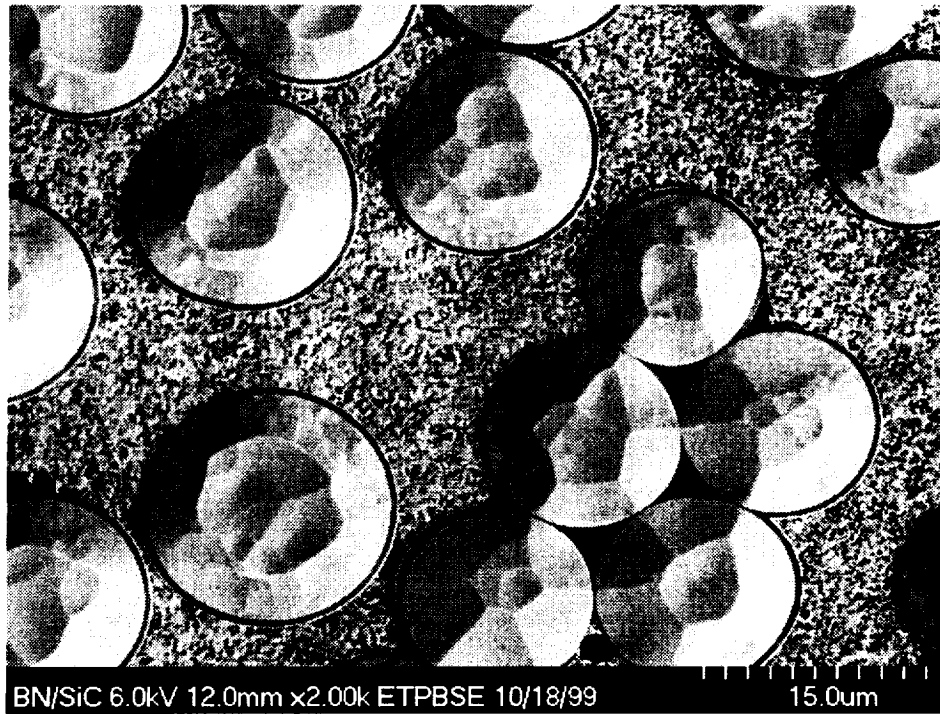
Figure 3.—FESEM micrograph of the cross-section of the BN/SiC coated Hi-Nicalon SiC/RBSN composite ( V_f \sim 0.24 ) showing uncoated regions in a cluster of fibers.
