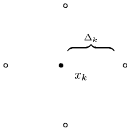
FIG. 2.1. A simple instance of pattern search
