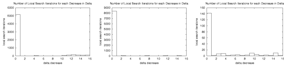
FIG. 6.1. NLess, Compass, & HJ in 4 variables
