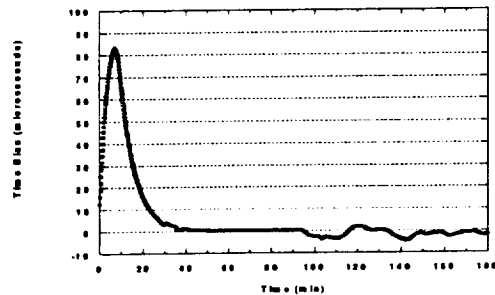
Figure 15. Case 3 BlackJack Time Bias vs. Time
