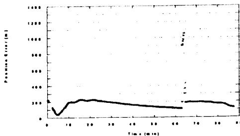
Figure 7. Difference between Real-Time and Post-Processed Position Solutions vs. Time
