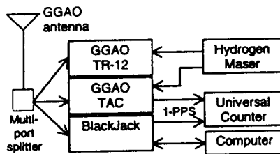
Figure 3. Case 3 Test Configuration
