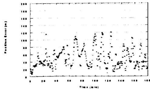
Figure 16. Case 3 TR-12 Position Error vs. Time
