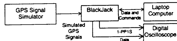
Figure 2. Case 2 Test Configuration
