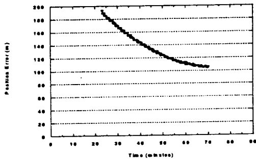
Figure 8. Case 2.1 Position Error vs. Time
