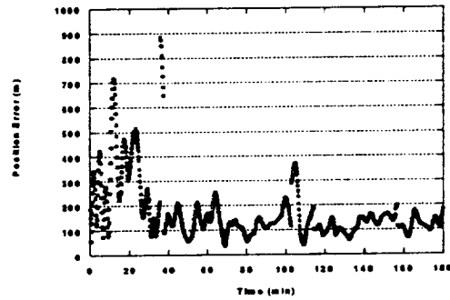
Figure 14. Case 3 BlackJack Position Error vs. Time
