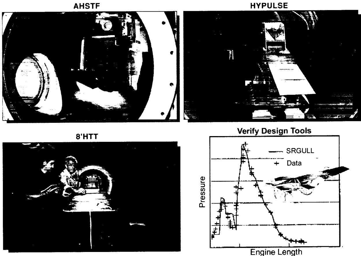
Figure 4. Design/Risk Reduction: Mach 7 Module Testing.
