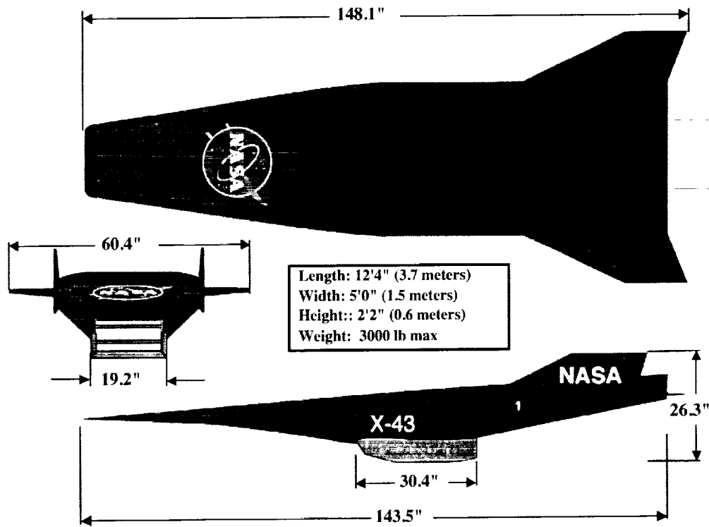
Figure 1. X-43 Vehicle Geometry.
