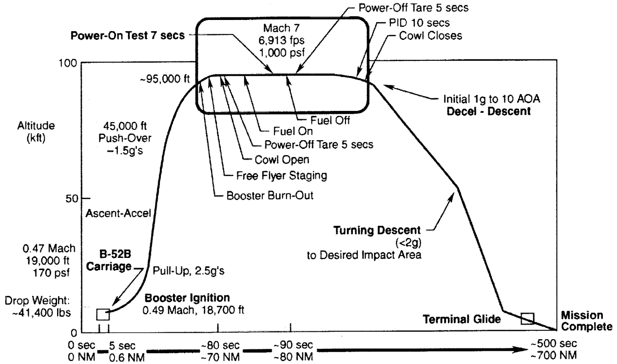
Figure 9. X-43 Mach 7 Flight Trajectory.
