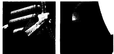
Design Reference Points: The Moons of the Outer Planets and Beyond.
