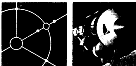
Design Reference Points: Libration Points and Lunar System.
