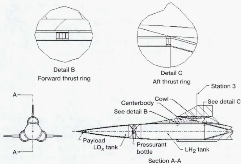
Figure 1.—GTX vehicle.
