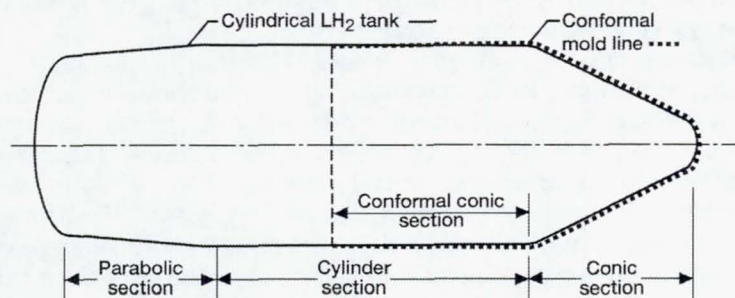
Figure 4.—Liquid hydrogen tank.
